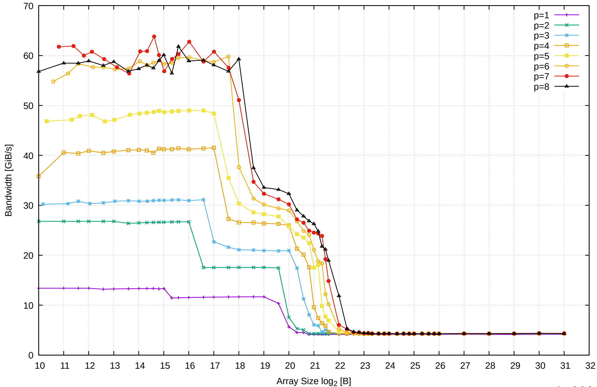
Pine64 RockPro64 Rockchip RK3399 - 4GB - Parallel Memory Bandwidth - ScanRead64PtrUnrollLoop
