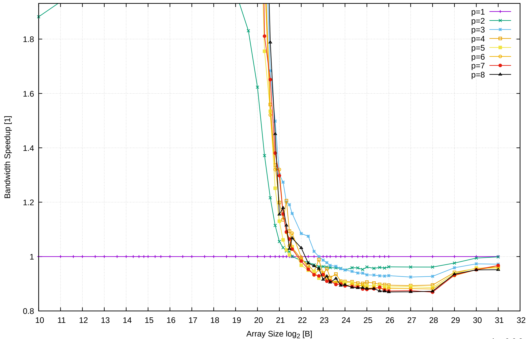
Pine64 RockPro64 Rockchip RK3399 - 4GB - Speedup of Parallel Memory Bandwidth (enlarged) - ScanWrite64PtrSimpleLoop
