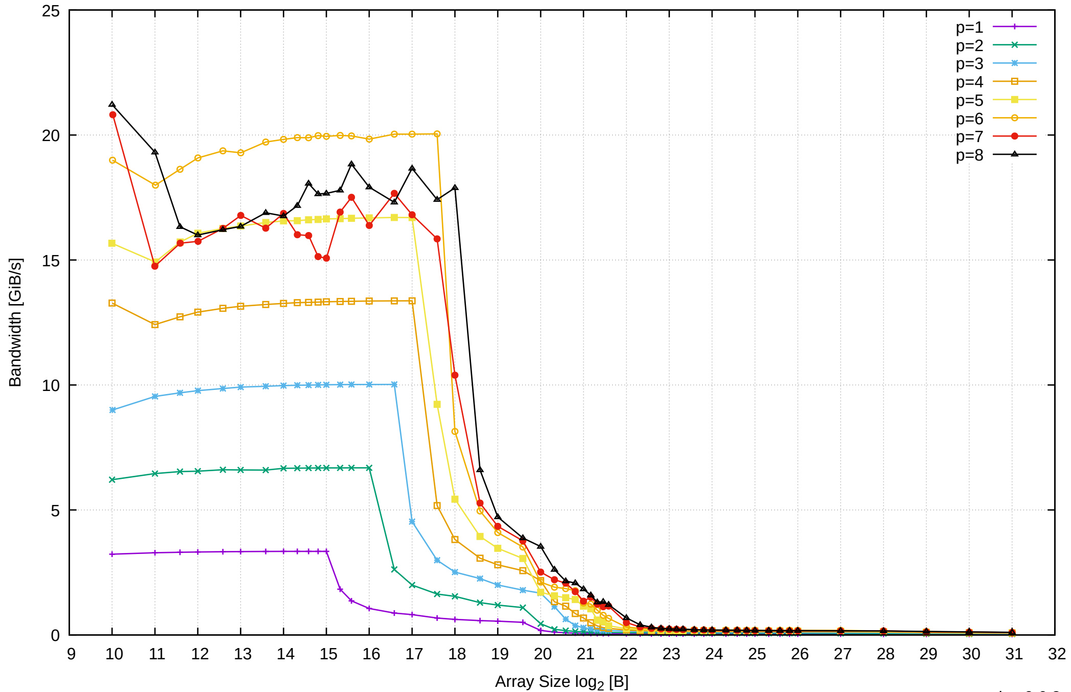
Pine64 RockPro64 Rockchip RK3399 - 4GB - Parallel Memory Bandwidth - PermRead64SimpleLoop
