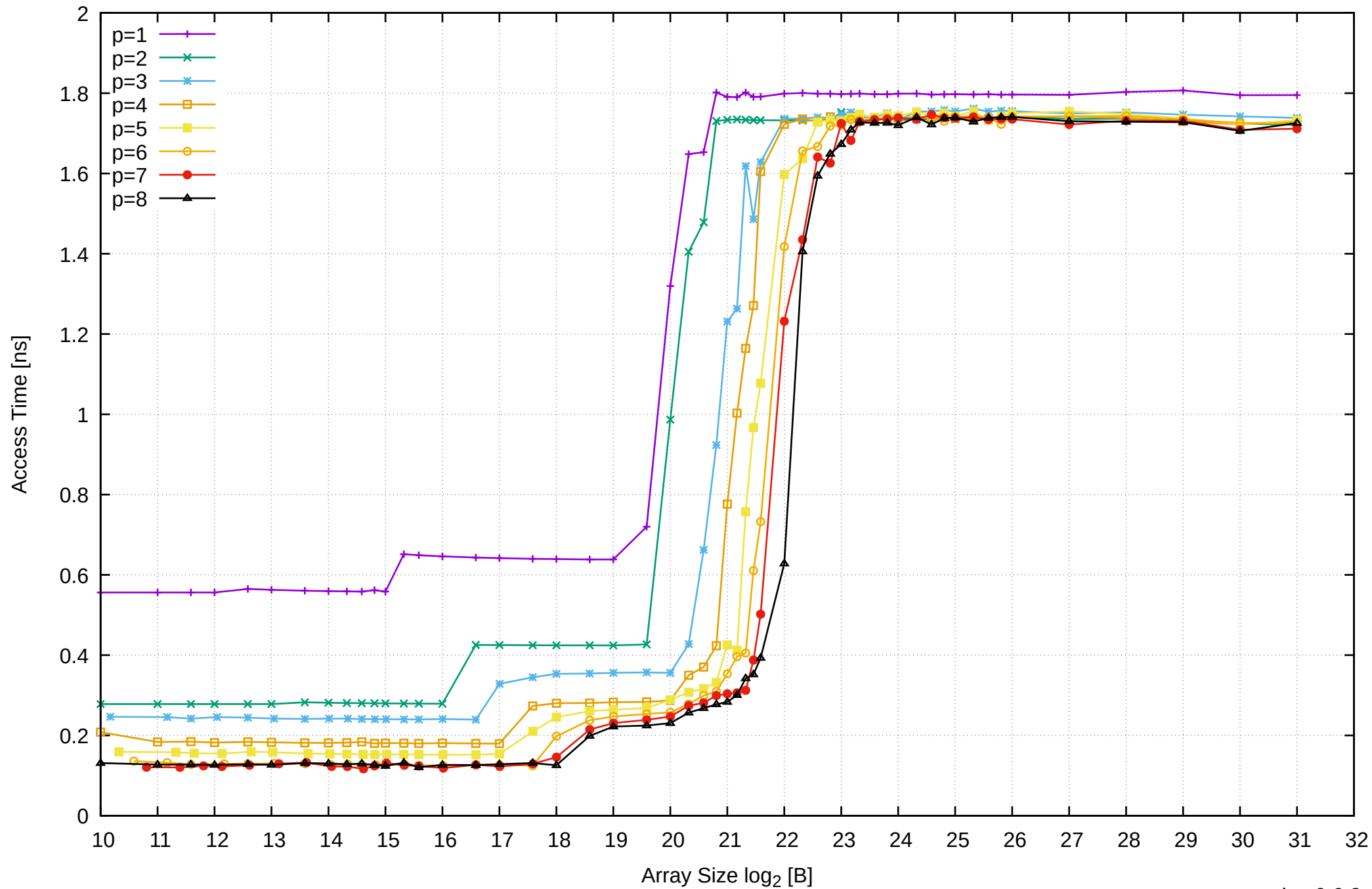
Pine64 RockPro64 Rockchip RK3399 - 4GB - Parallel Memory Access Time - ScanRead64PtrUnrollLoop
