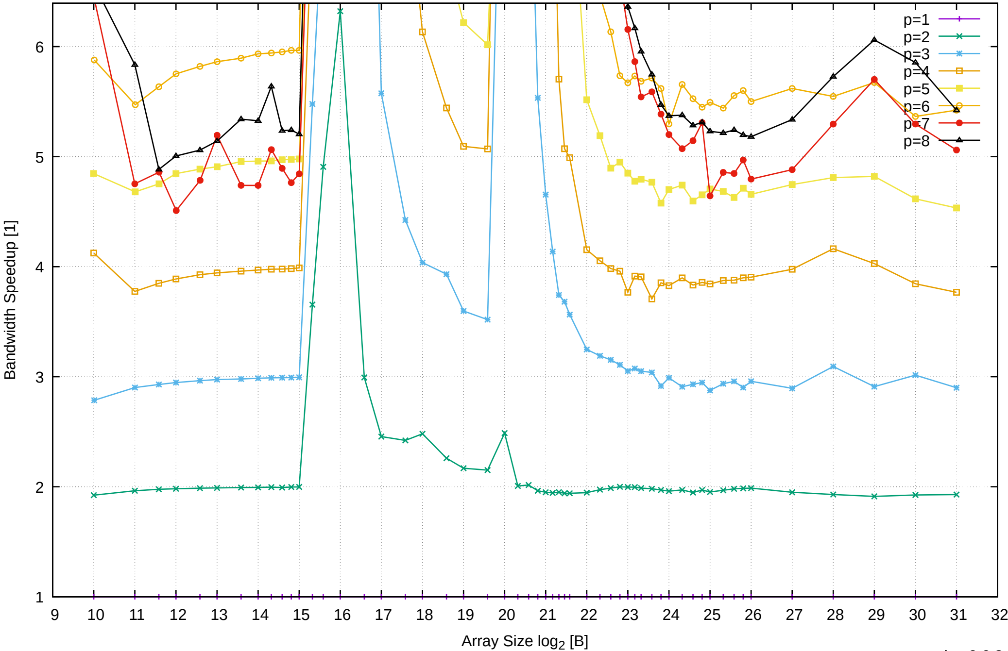
Pine64 RockPro64 Rockchip RK3399 - 4GB - Speedup of Parallel Memory Bandwidth (enlarged) - cPermRead64SimpleLoop
