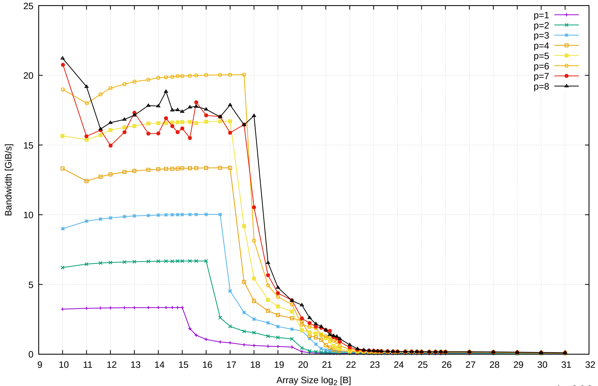
Pine64 RockPro64 Rockchip RK3399 - 4GB - Parallel Memory Bandwidth - cPermRead64SimpleLoop
