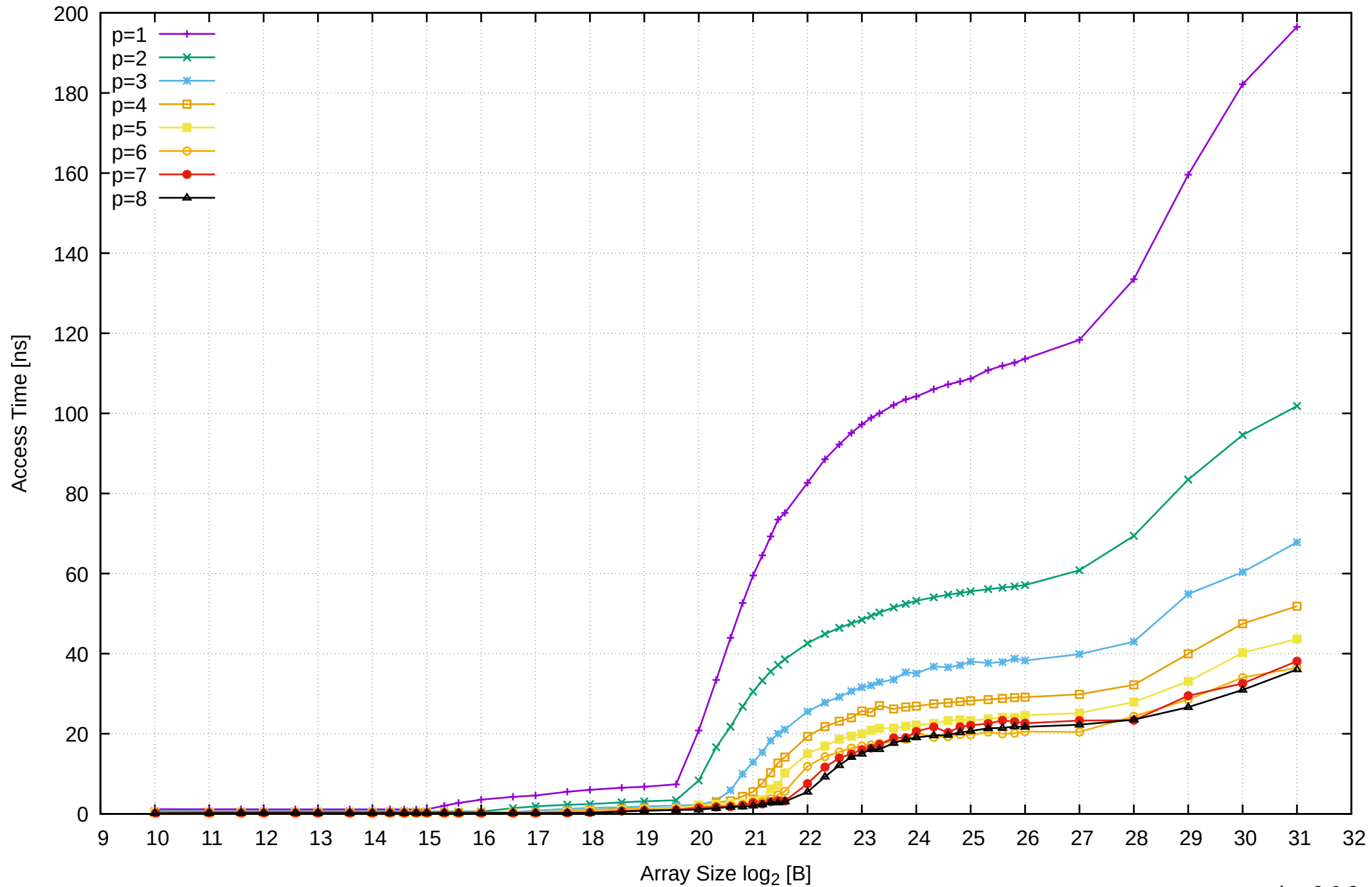
Pine64 RockPro64 Rockchip RK3399 - 4GB - Parallel Memory Access Time - PermRead64SimpleLoop
