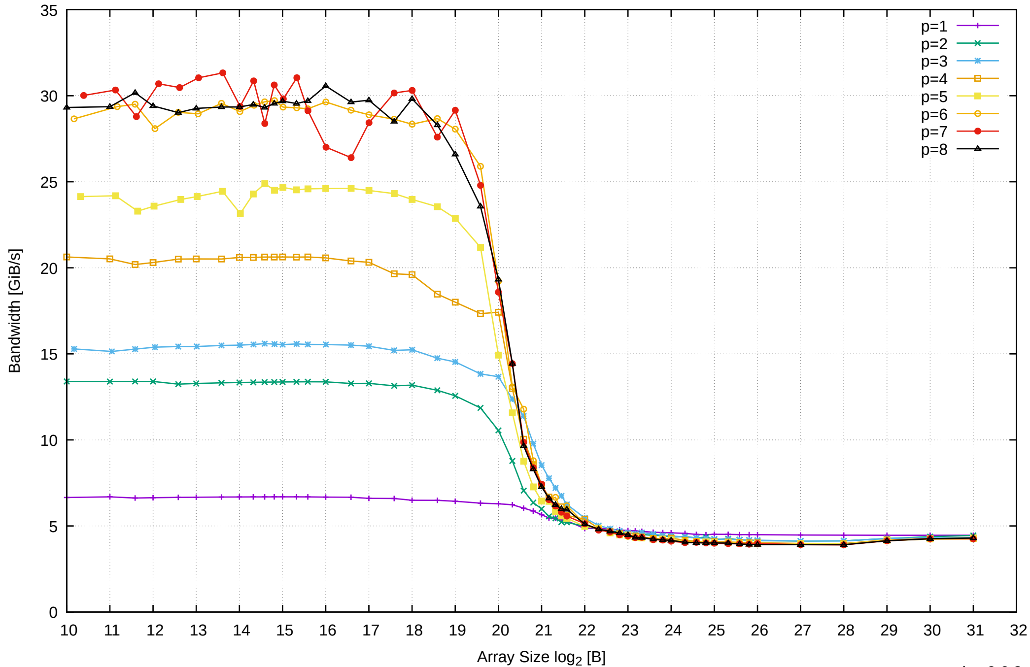
Pine64 RockPro64 Rockchip RK3399 - 4GB - Parallel Memory Bandwidth - ScanWrite32PtrUnrollLoop
