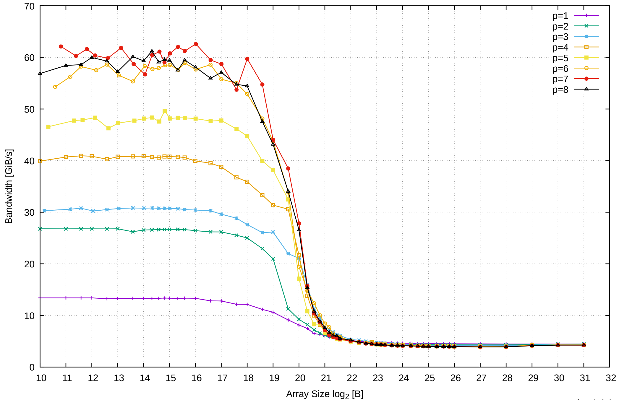
Pine64 RockPro64 Rockchip RK3399 - 4GB - Parallel Memory Bandwidth - ScanWrite64PtrUnrollLoop
