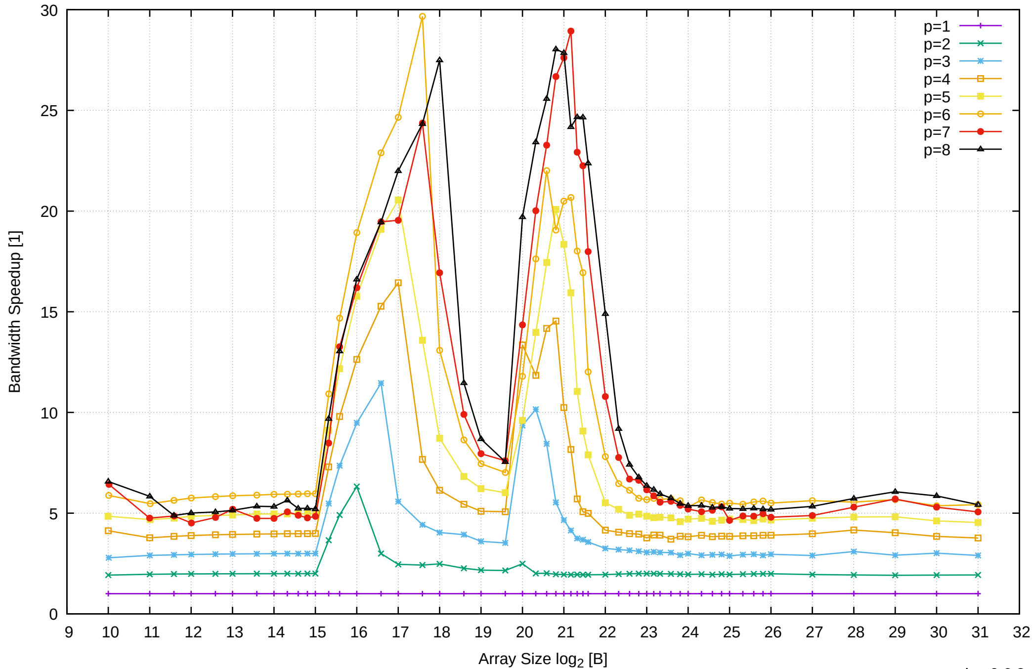
Pine64 RockPro64 Rockchip RK3399 - 4GB - Speedup of Parallel Memory Bandwidth - cPermRead64SimpleLoop
