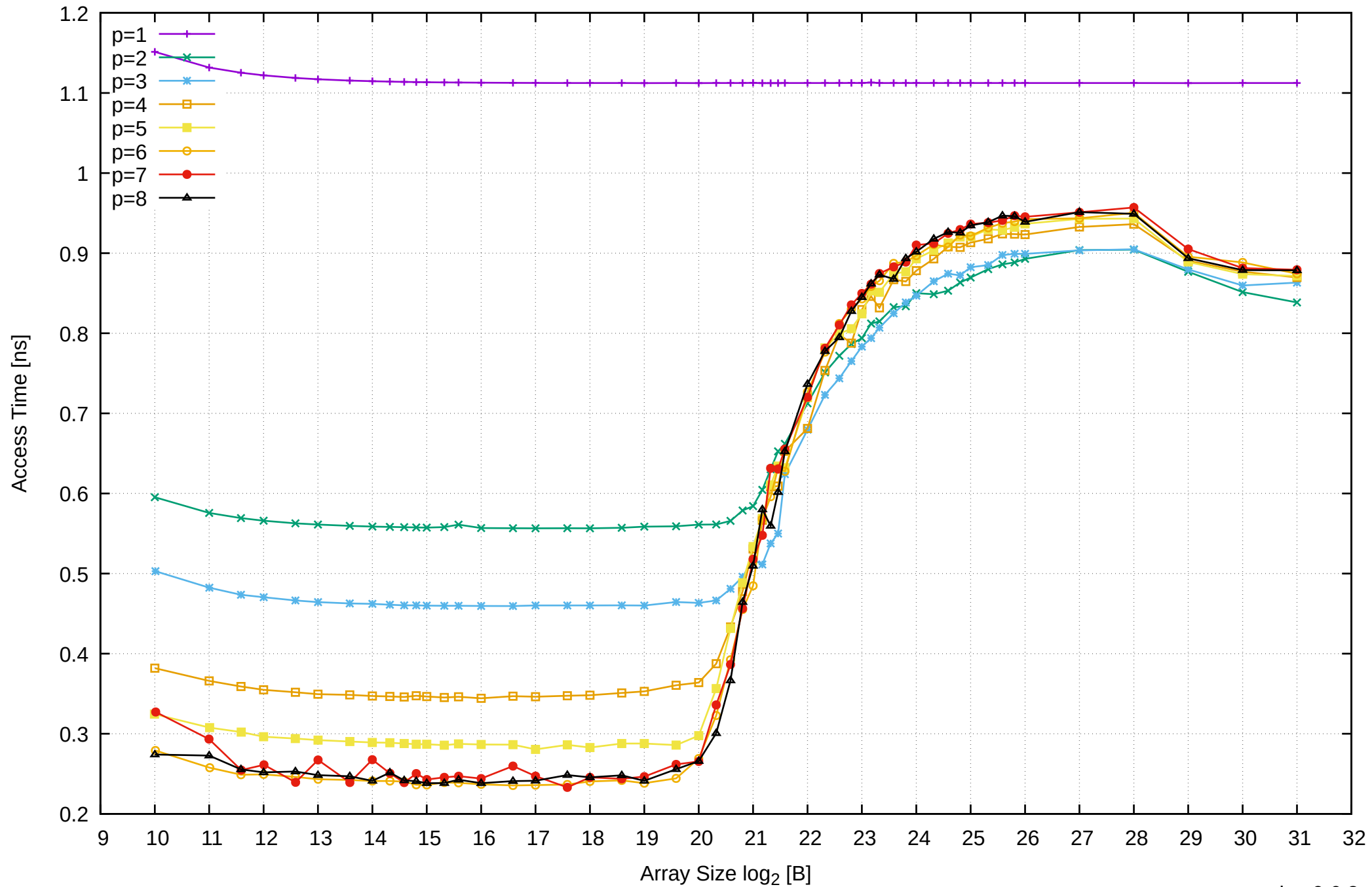
Pine64 RockPro64 Rockchip RK3399 - 4GB - Parallel Memory Access Time - ScanWrite32PtrSimpleLoop
