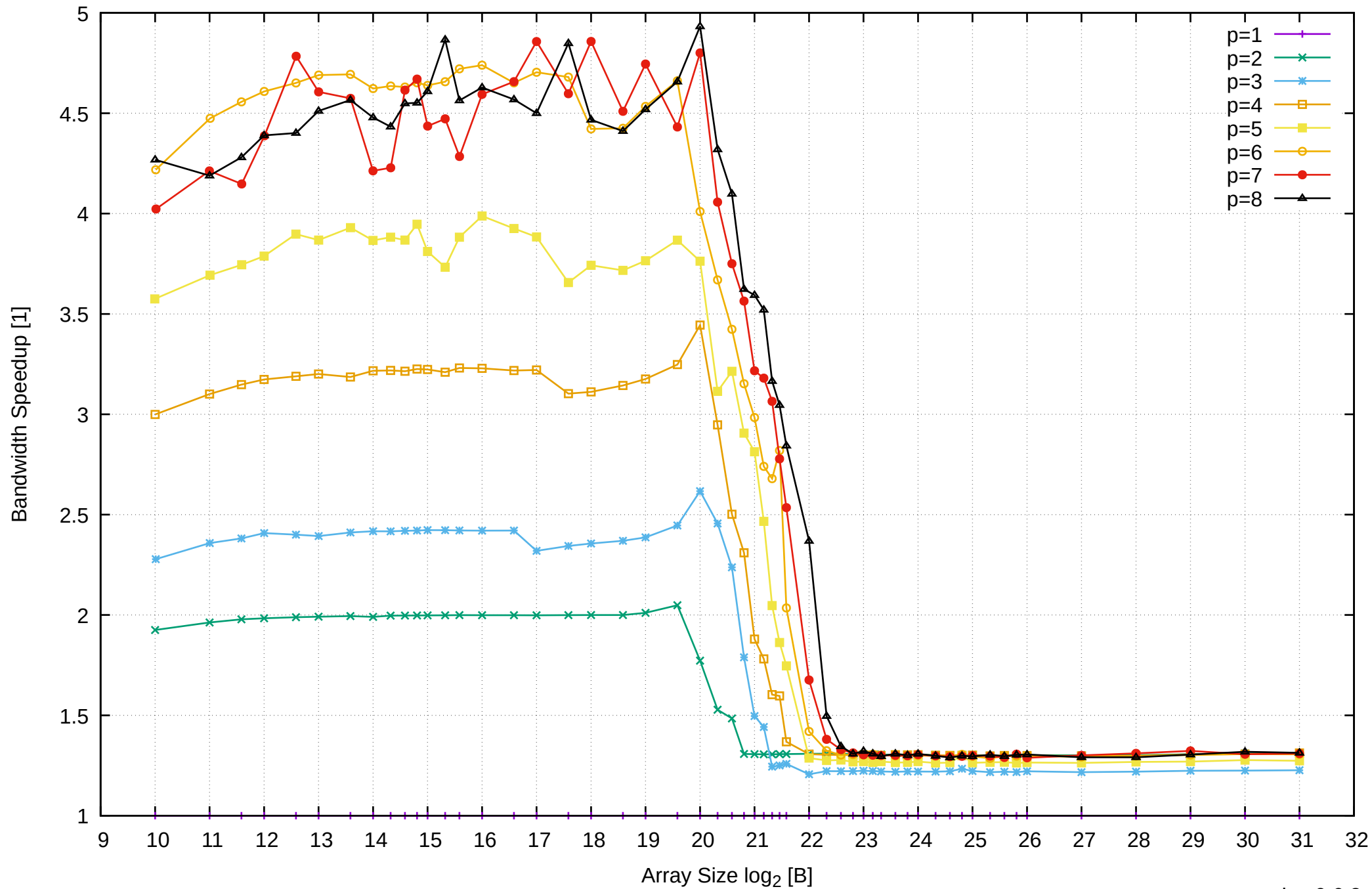
Pine64 RockPro64 Rockchip RK3399 - 4GB - Speedup of Parallel Memory Bandwidth - ScanRead32PtrSimpleLoop
