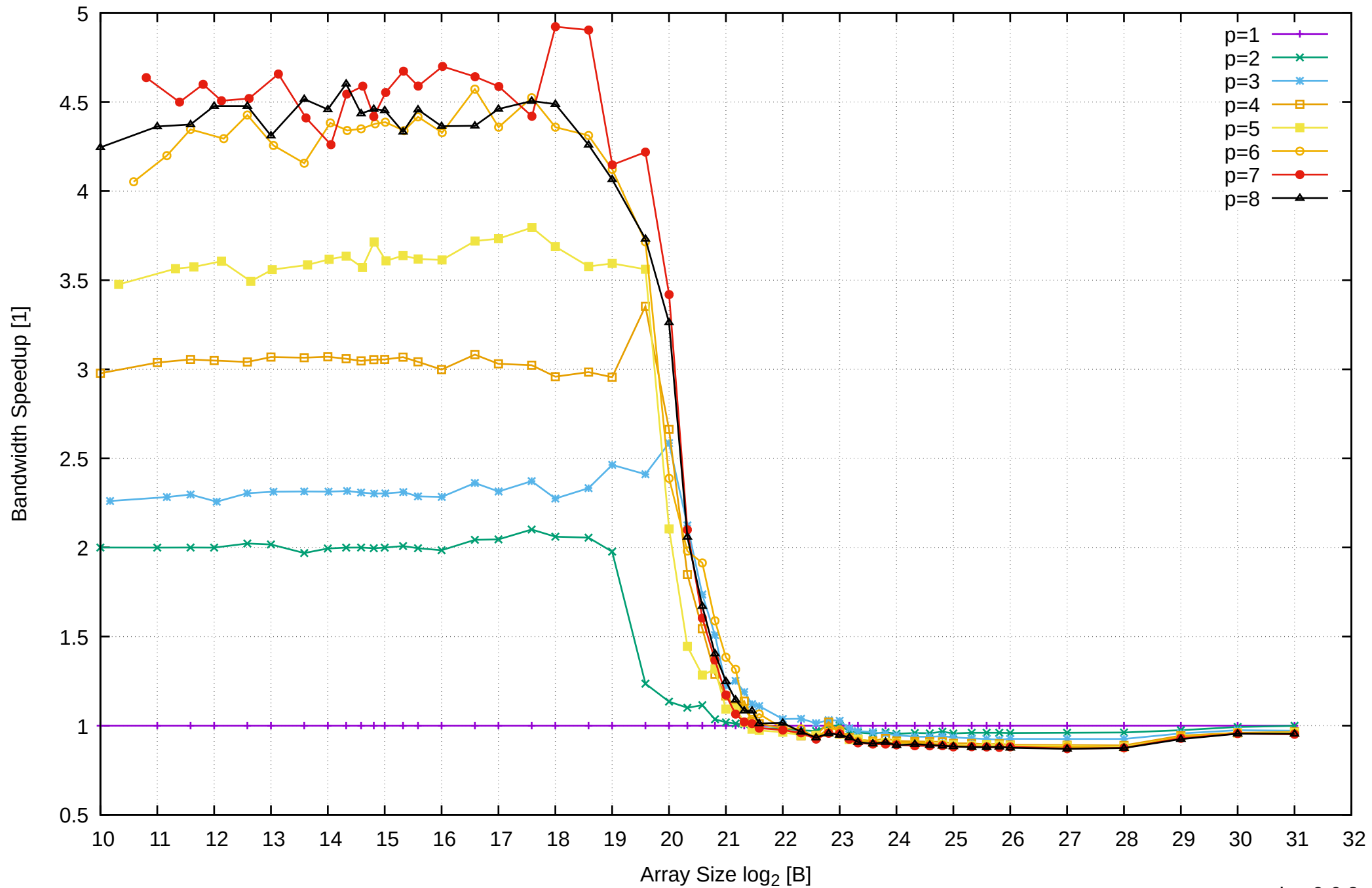
Pine64 RockPro64 Rockchip RK3399 - 4GB - Speedup of Parallel Memory Bandwidth - ScanWrite64PtrUnrollLoop
