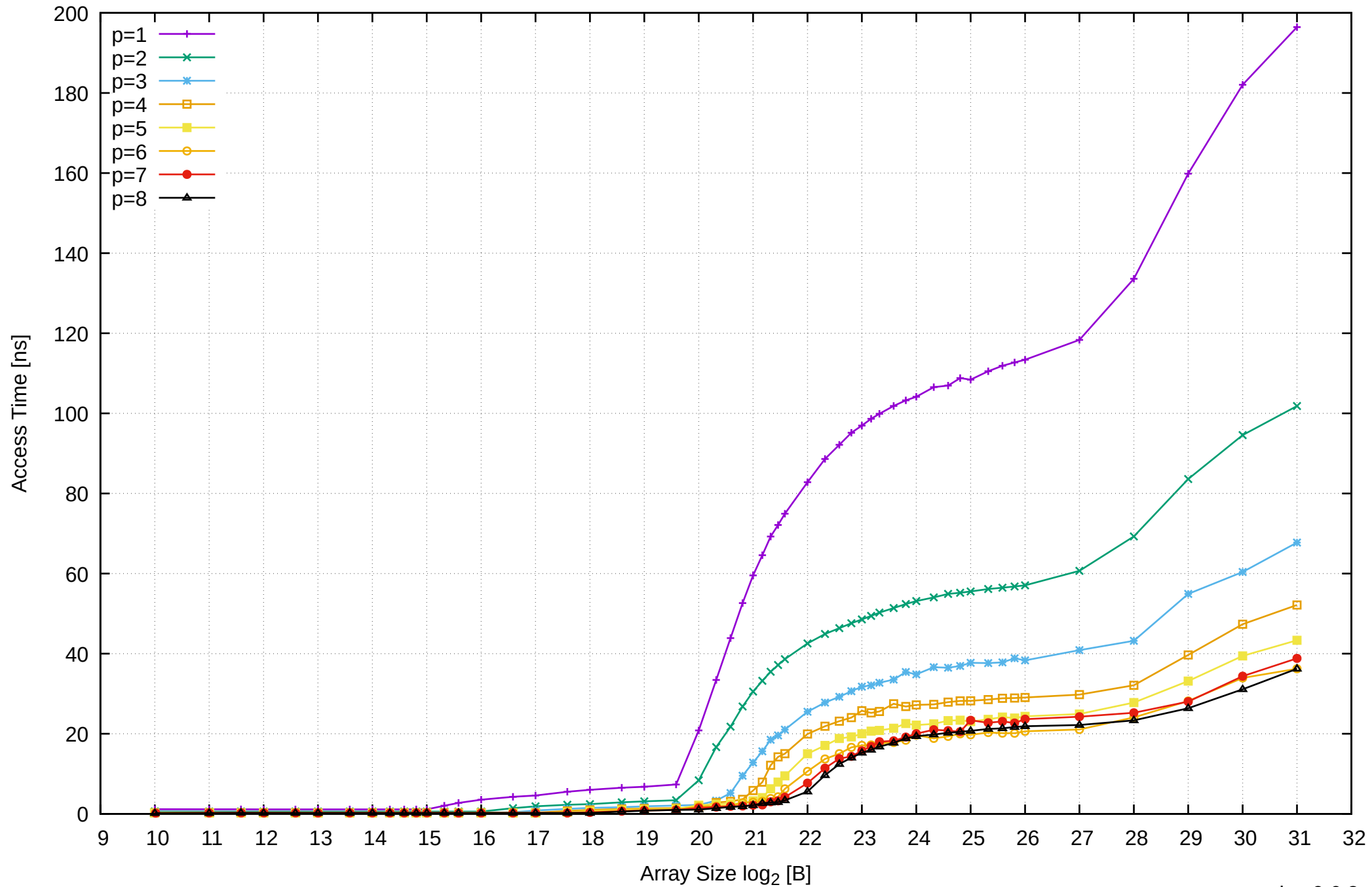
Pine64 RockPro64 Rockchip RK3399 - 4GB - Parallel Memory Access Time - cPermRead64SimpleLoop
