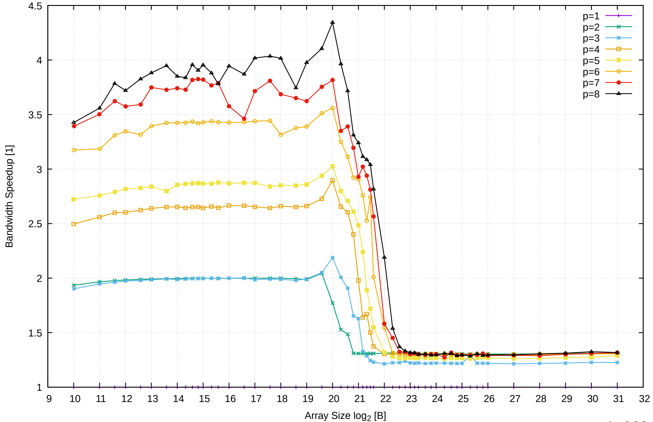
Pine64 RockPro64 Rockchip RK3399 - 4GB - Speedup of Parallel Memory Bandwidth - ScanRead32IndexSimpleLoop
