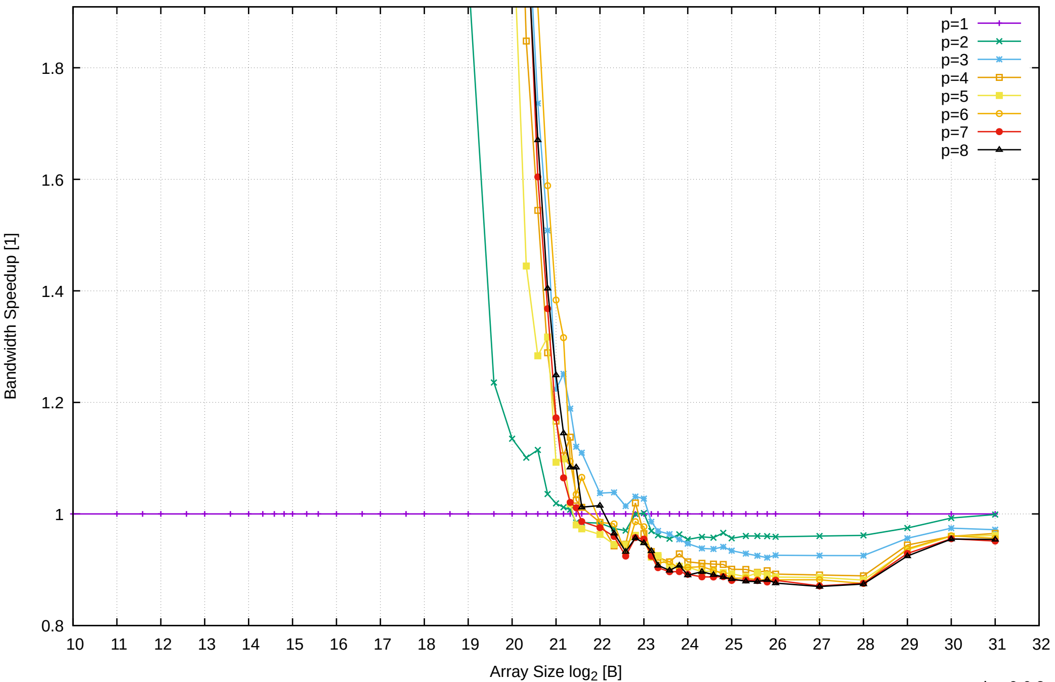
Pine64 RockPro64 Rockchip RK3399 - 4GB - Speedup of Parallel Memory Bandwidth (enlarged) - ScanWrite64PtrUnrollLoop
