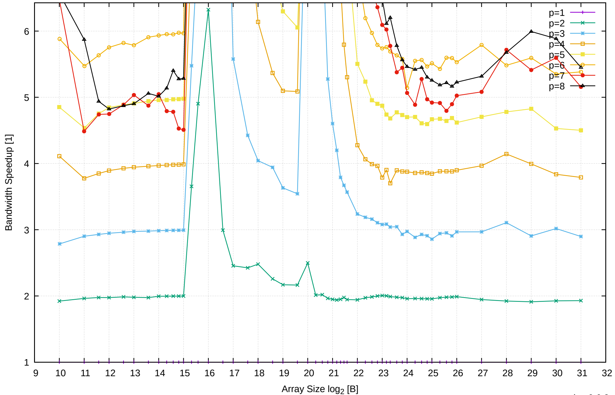
Pine64 RockPro64 Rockchip RK3399 - 4GB - Speedup of Parallel Memory Bandwidth (enlarged) - PermRead64SimpleLoop
