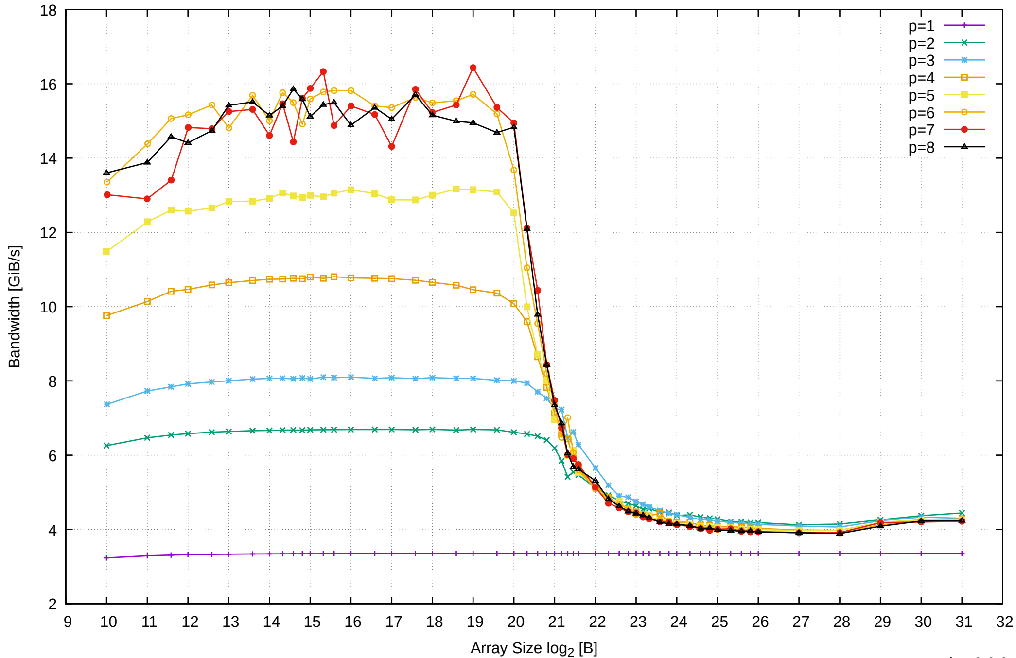
Pine64 RockPro64 Rockchip RK3399 - 4GB - Parallel Memory Bandwidth - cScanWrite32IndexSimpleLoop
