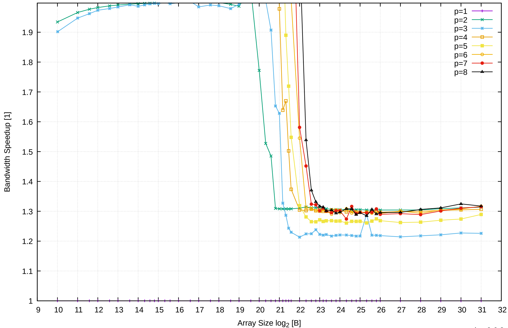
Pine64 RockPro64 Rockchip RK3399 - 4GB - Speedup of Parallel Memory Bandwidth (enlarged) - ScanRead32IndexSimpleLoop
