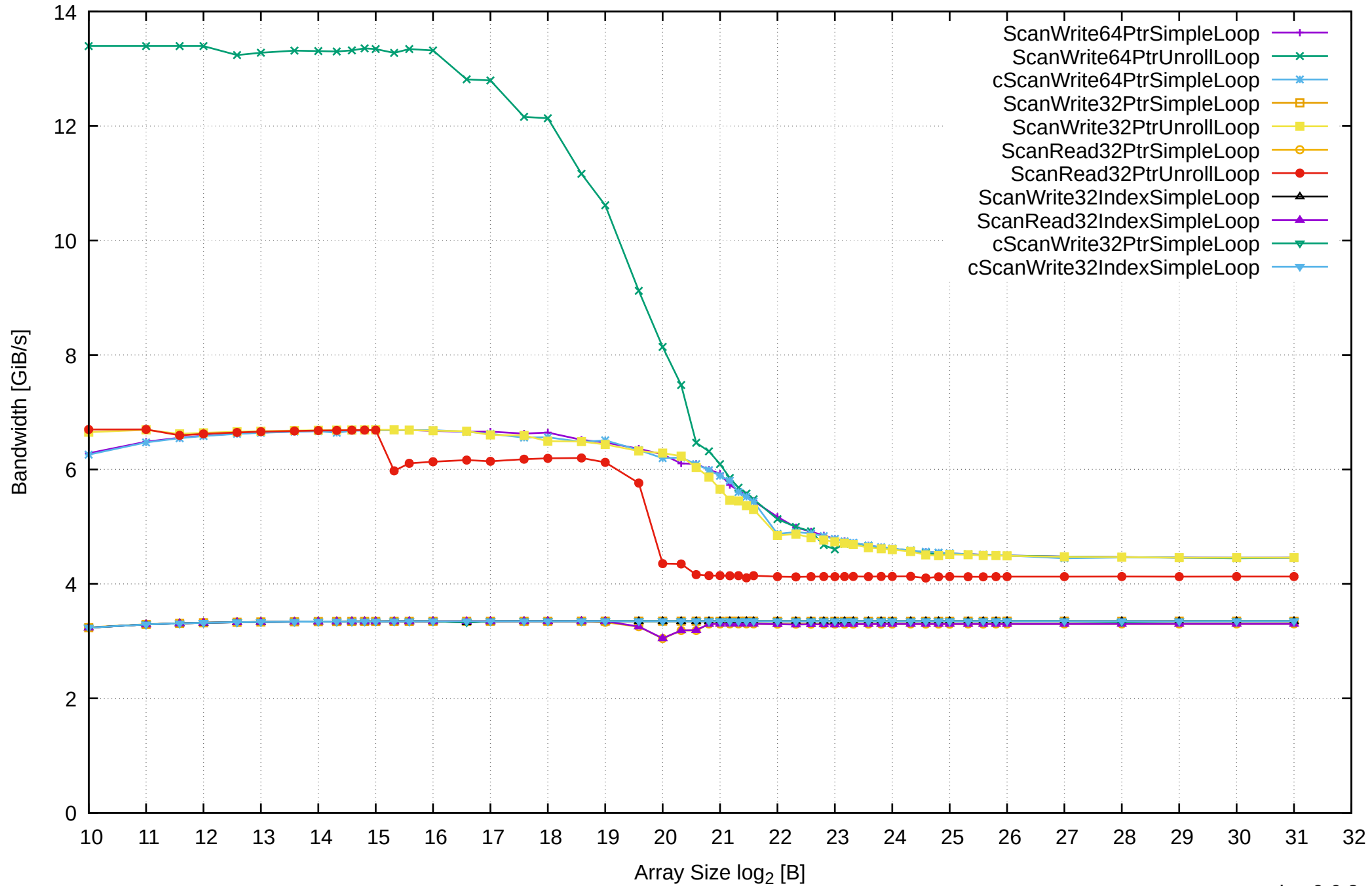
Pine64 RockPro64 Rockchip RK3399 - 4GB - One Thread Memory Bandwidth (only 64-bit Reads)
