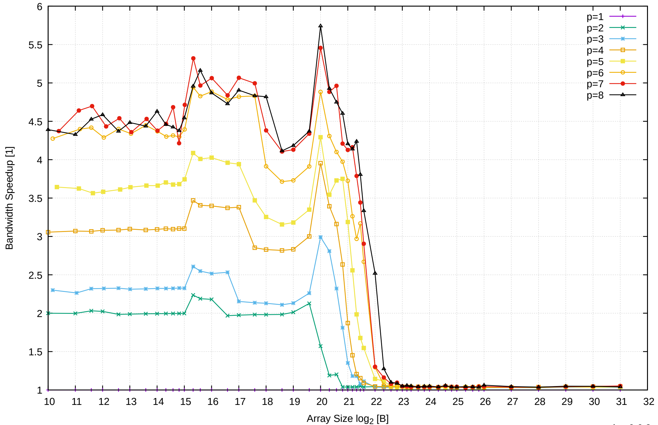
Pine64 RockPro64 Rockchip RK3399 - 4GB - Speedup of Parallel Memory Bandwidth - ScanRead32PtrUnrollLoop
