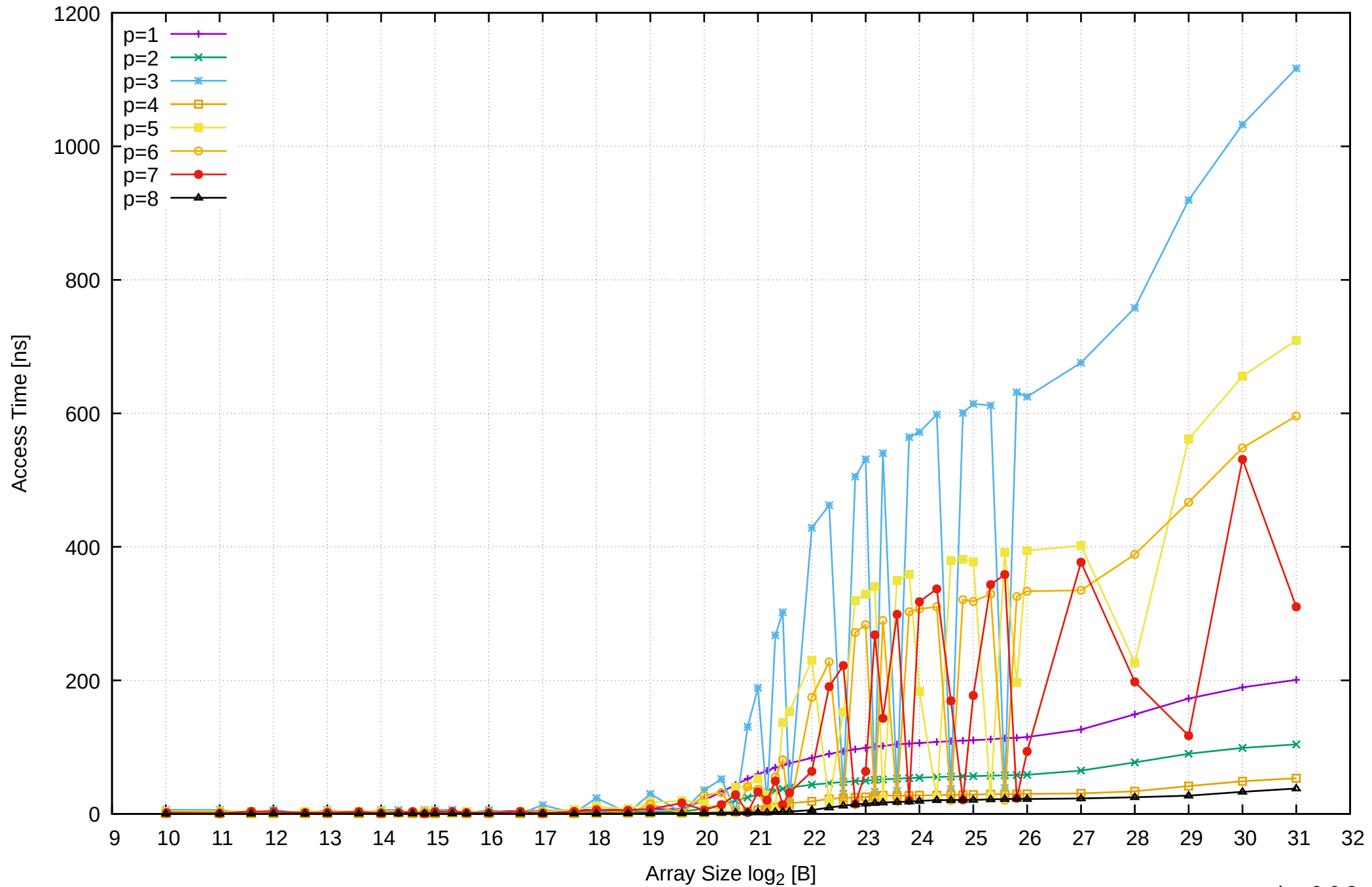
Pine64 RockPro64 Rockchip RK3399 - 4GB - Parallel Memory Access Time - PermRead64UnrollLoop
