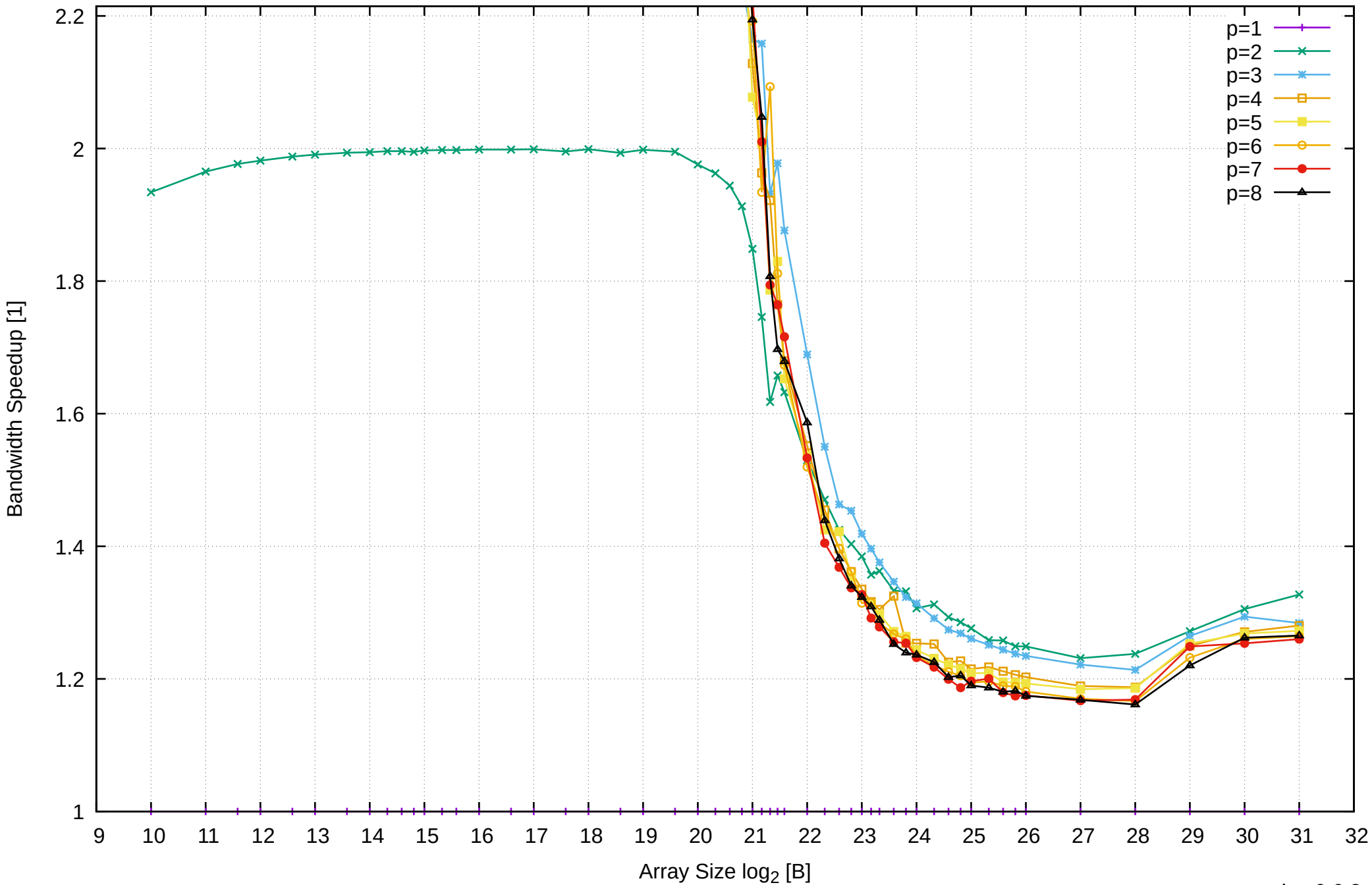
Pine64 RockPro64 Rockchip RK3399 - 4GB - Speedup of Parallel Memory Bandwidth (enlarged) - cScanWrite32IndexSimpleLoop
