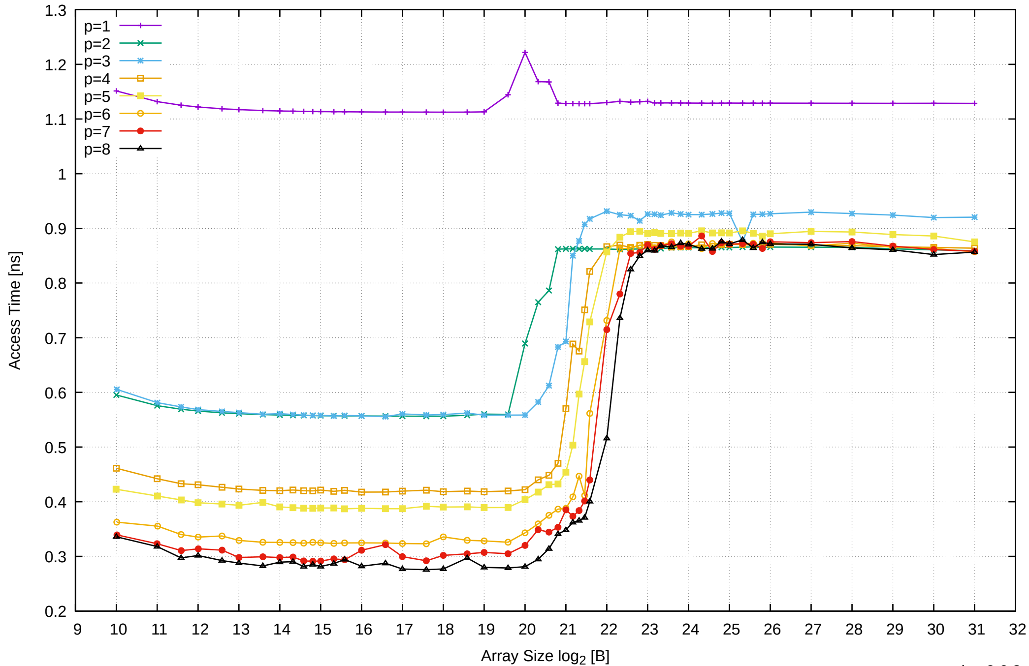
Pine64 RockPro64 Rockchip RK3399 - 4GB - Parallel Memory Access Time - ScanRead32IndexSimpleLoop
