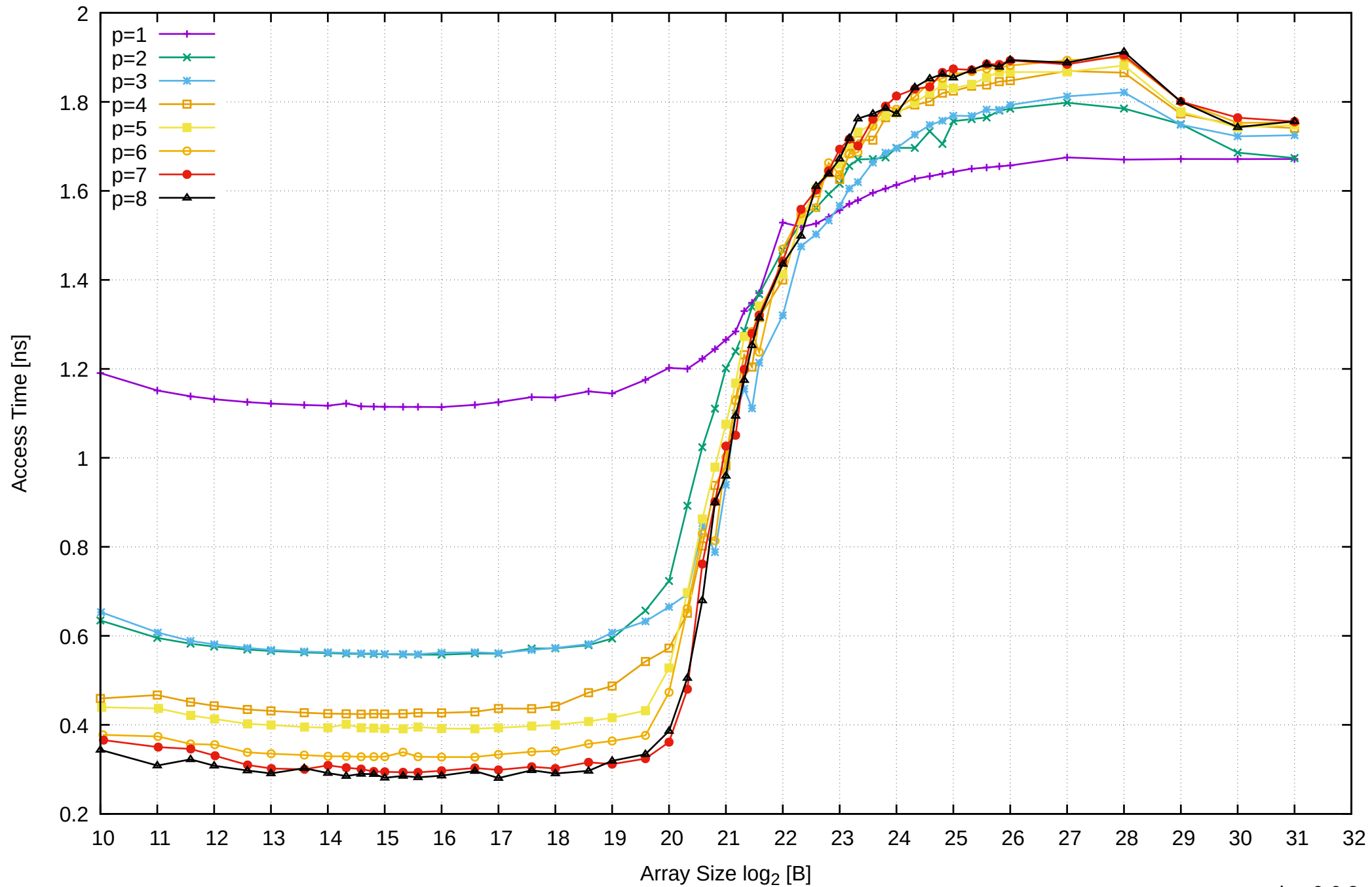
Pine64 RockPro64 Rockchip RK3399 - 4GB - Parallel Memory Access Time - cScanWrite64PtrSimpleLoop
