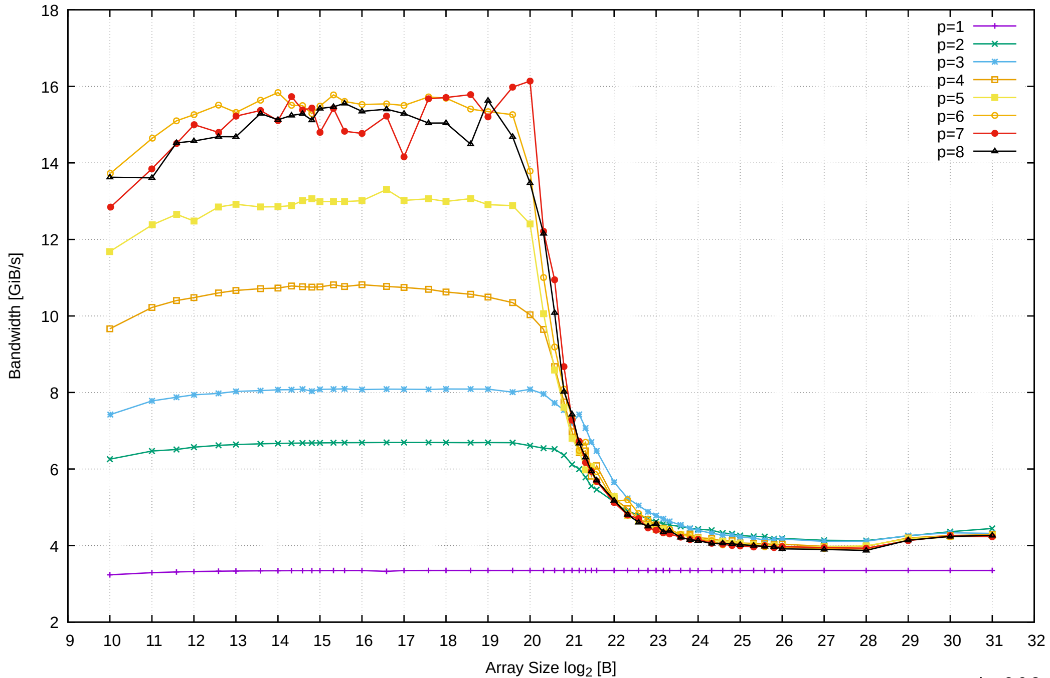
Pine64 RockPro64 Rockchip RK3399 - 4GB - Parallel Memory Bandwidth - ScanWrite32IndexSimpleLoop
