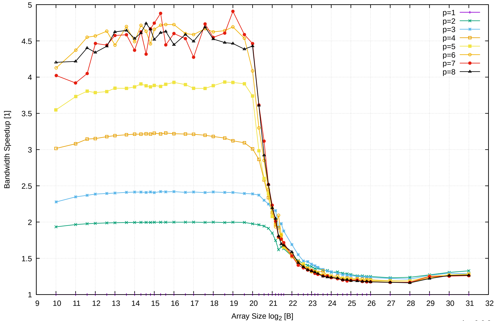
Pine64 RockPro64 Rockchip RK3399 - 4GB - Speedup of Parallel Memory Bandwidth - cScanWrite32IndexSimpleLoop
