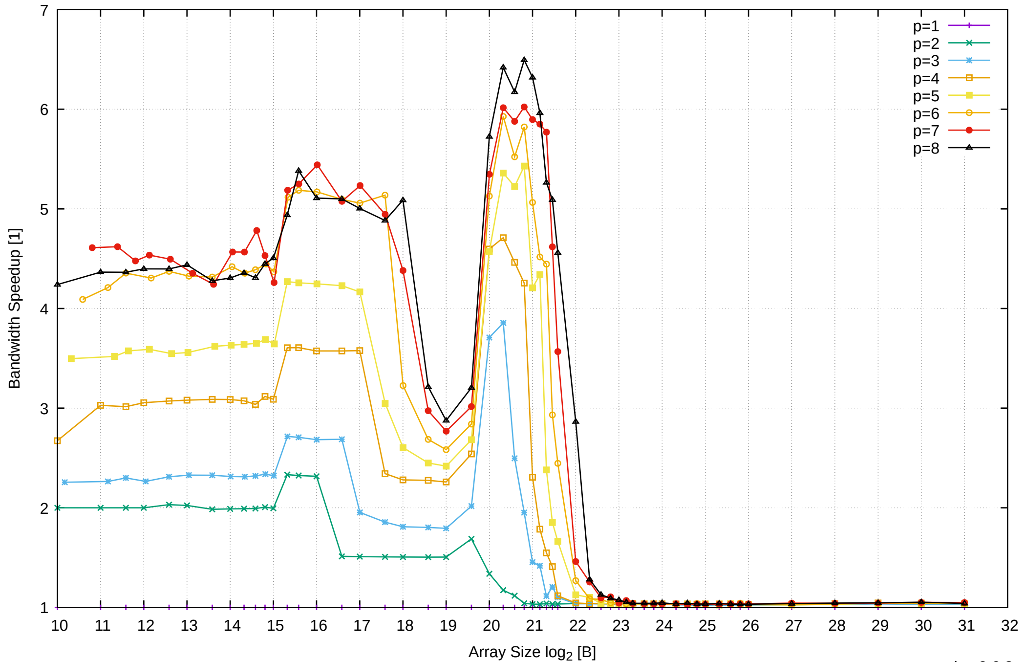
Pine64 RockPro64 Rockchip RK3399 - 4GB - Speedup of Parallel Memory Bandwidth - ScanRead64PtrUnrollLoop
