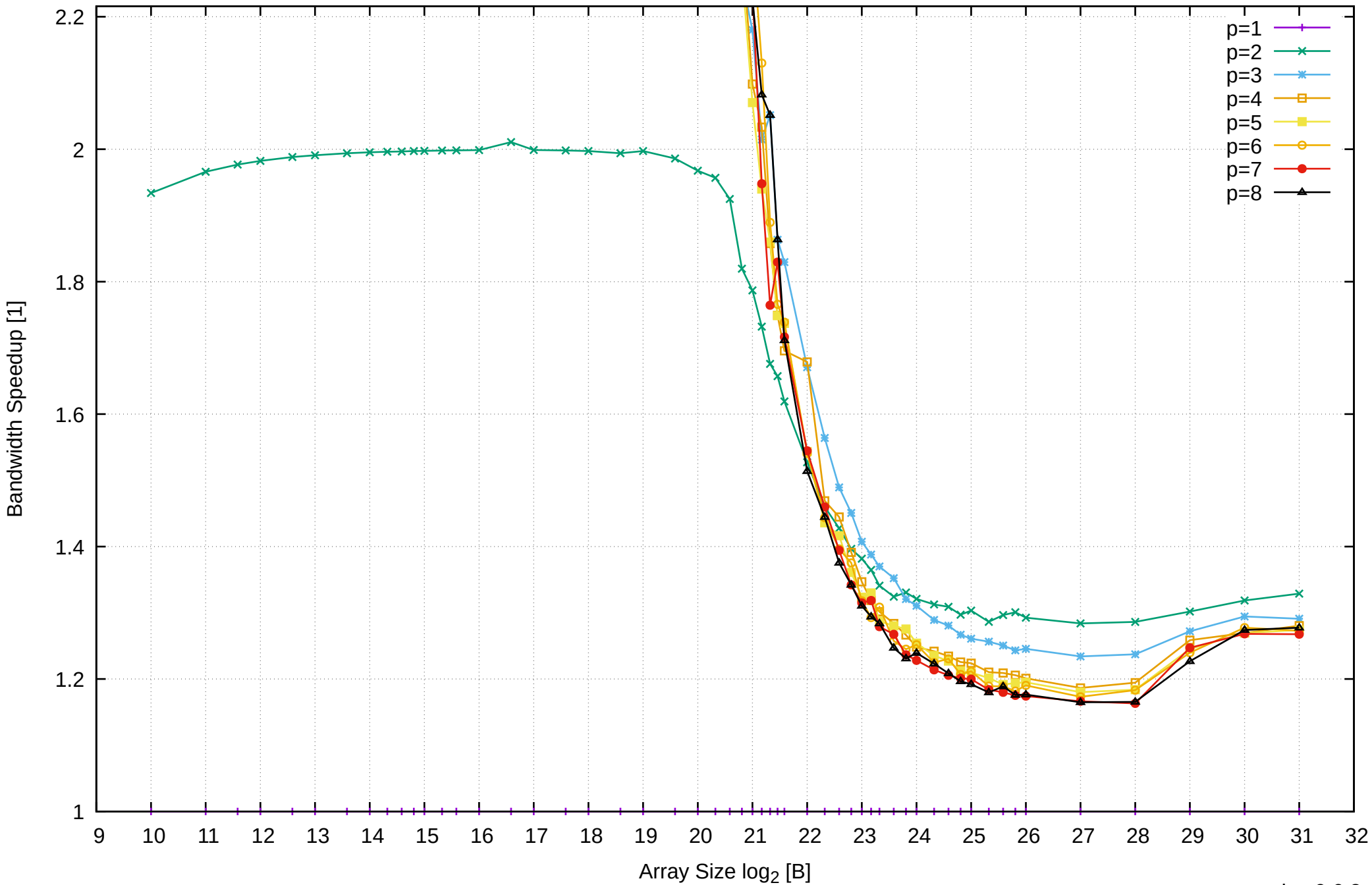
Pine64 RockPro64 Rockchip RK3399 - 4GB - Speedup of Parallel Memory Bandwidth (enlarged) - cScanWrite32PtrSimpleLoop
