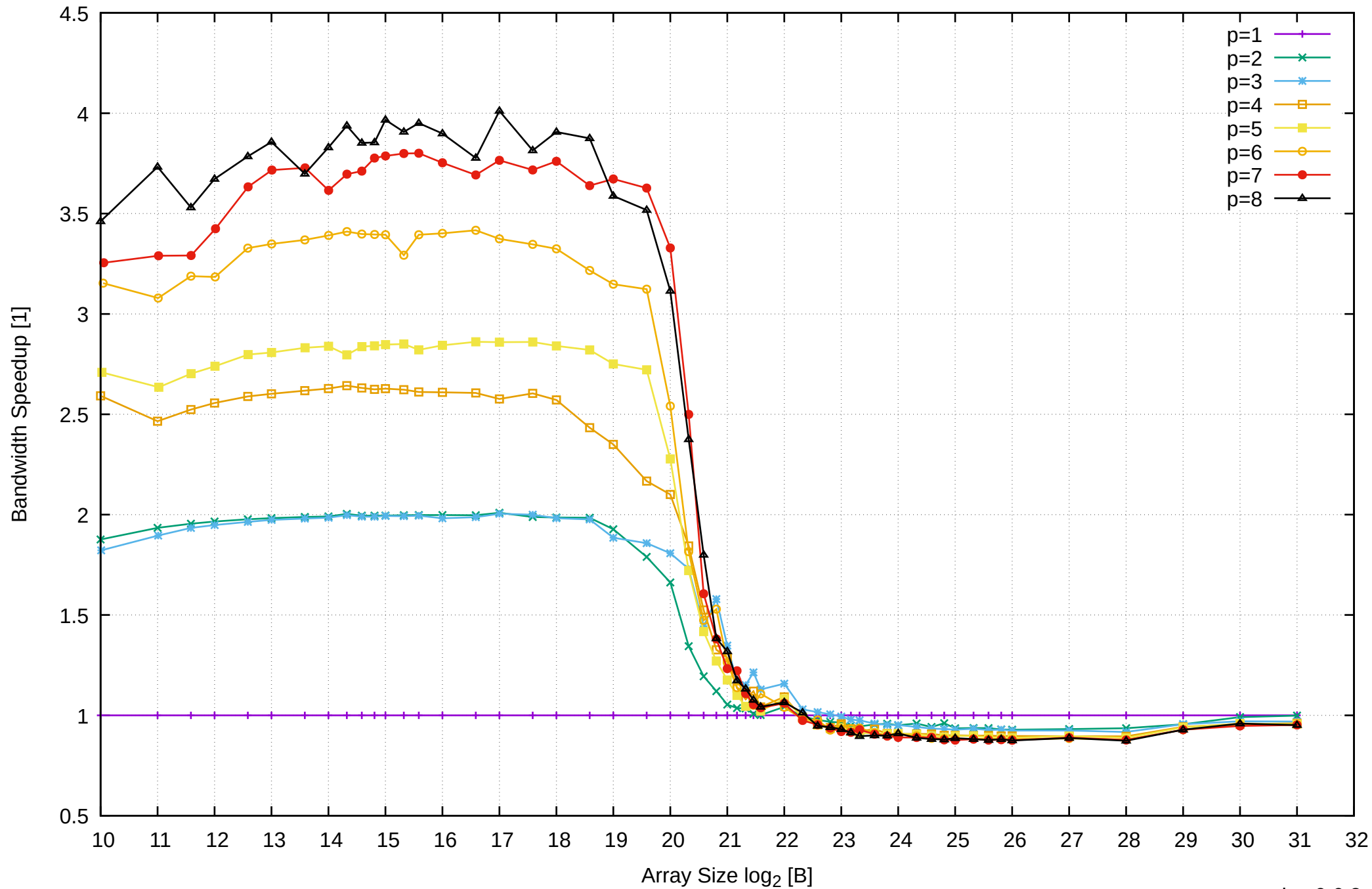
Pine64 RockPro64 Rockchip RK3399 - 4GB - Speedup of Parallel Memory Bandwidth - cScanWrite64PtrSimpleLoop
