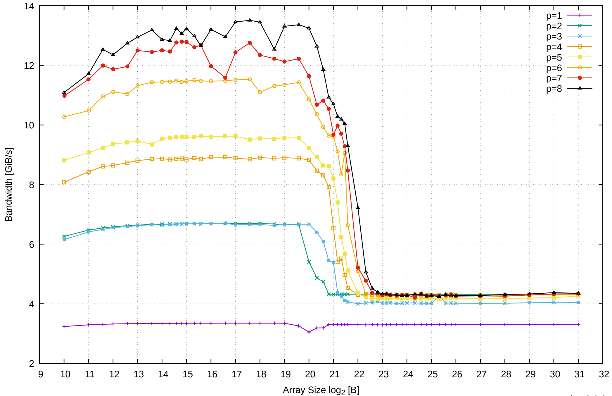
Pine64 RockPro64 Rockchip RK3399 - 4GB - Parallel Memory Bandwidth - ScanRead32IndexSimpleLoop
