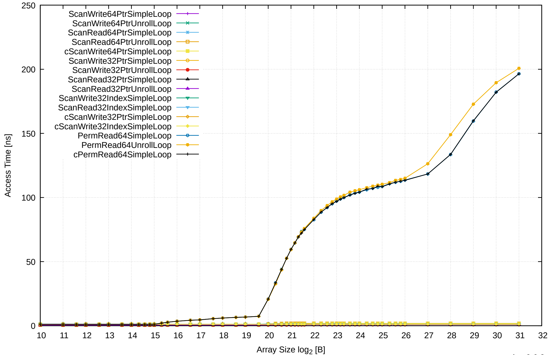
Pine64 RockPro64 Rockchip RK3399 - 4GB - One Thread Memory Latency (Access Time)
