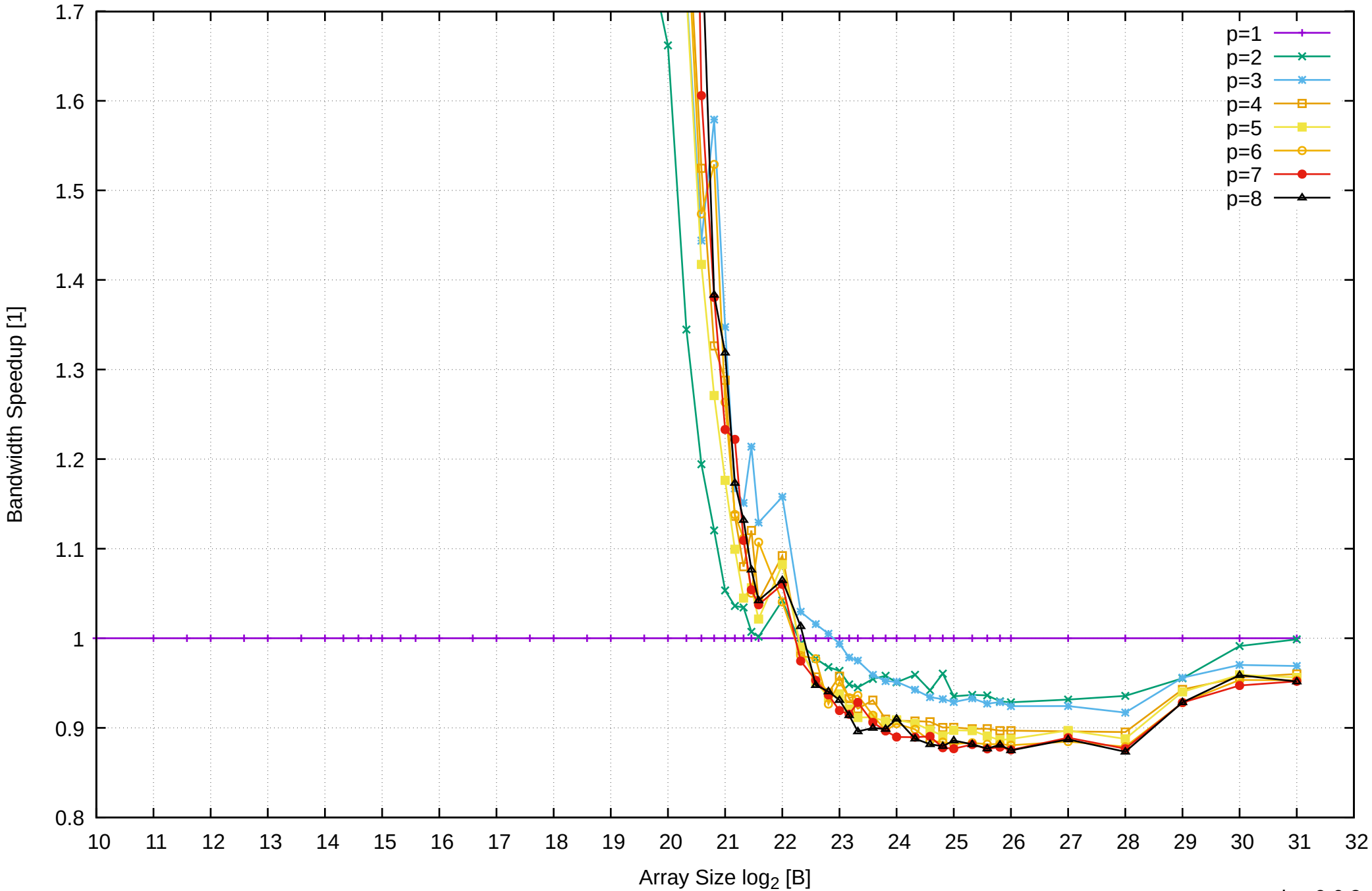
Pine64 RockPro64 Rockchip RK3399 - 4GB - Speedup of Parallel Memory Bandwidth (enlarged) - cScanWrite64PtrSimpleLoop
