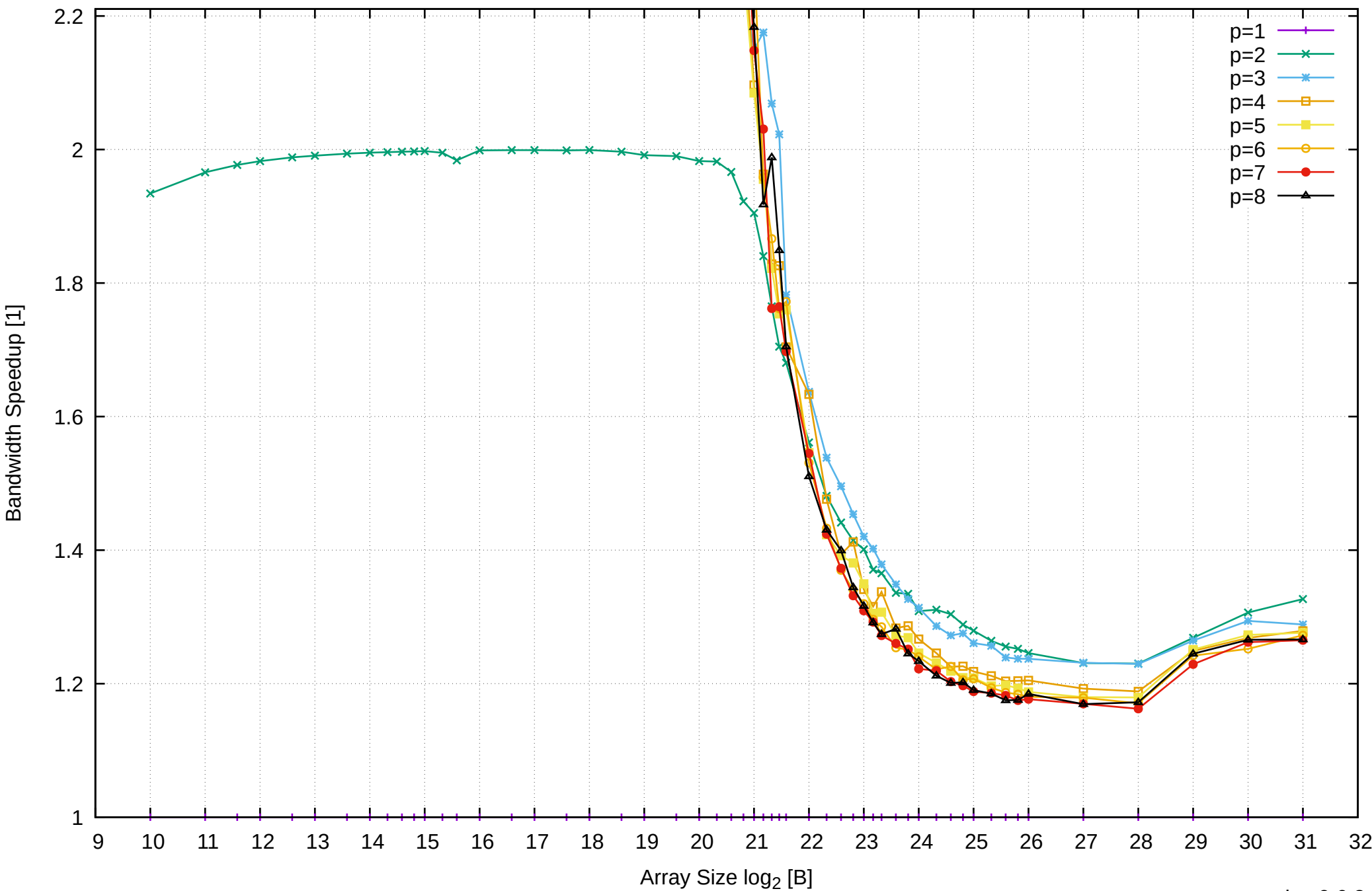
Pine64 RockPro64 Rockchip RK3399 - 4GB - Speedup of Parallel Memory Bandwidth (enlarged) - ScanWrite32PtrSimpleLoop
