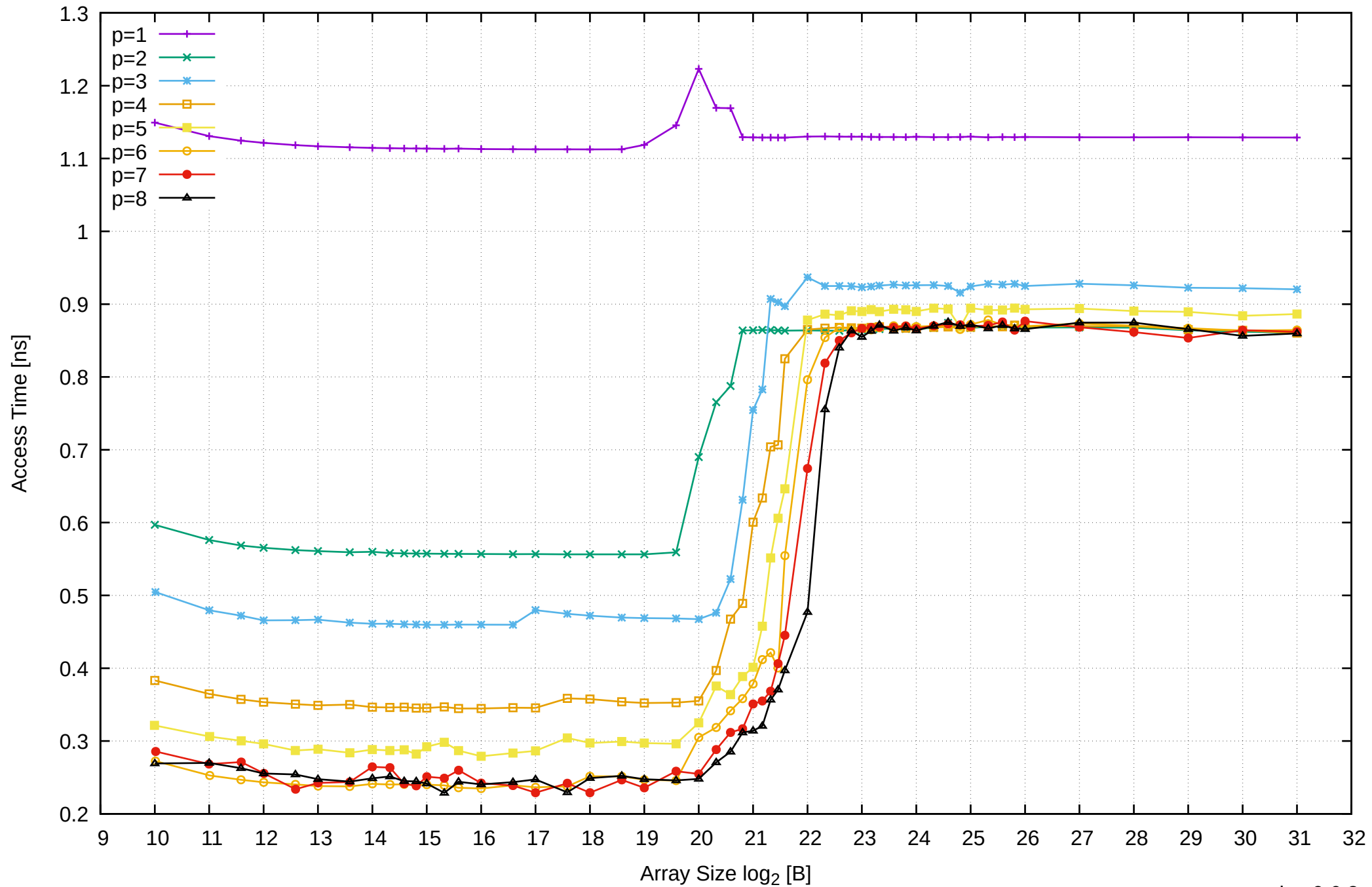
Pine64 RockPro64 Rockchip RK3399 - 4GB - Parallel Memory Access Time - ScanRead32PtrSimpleLoop
