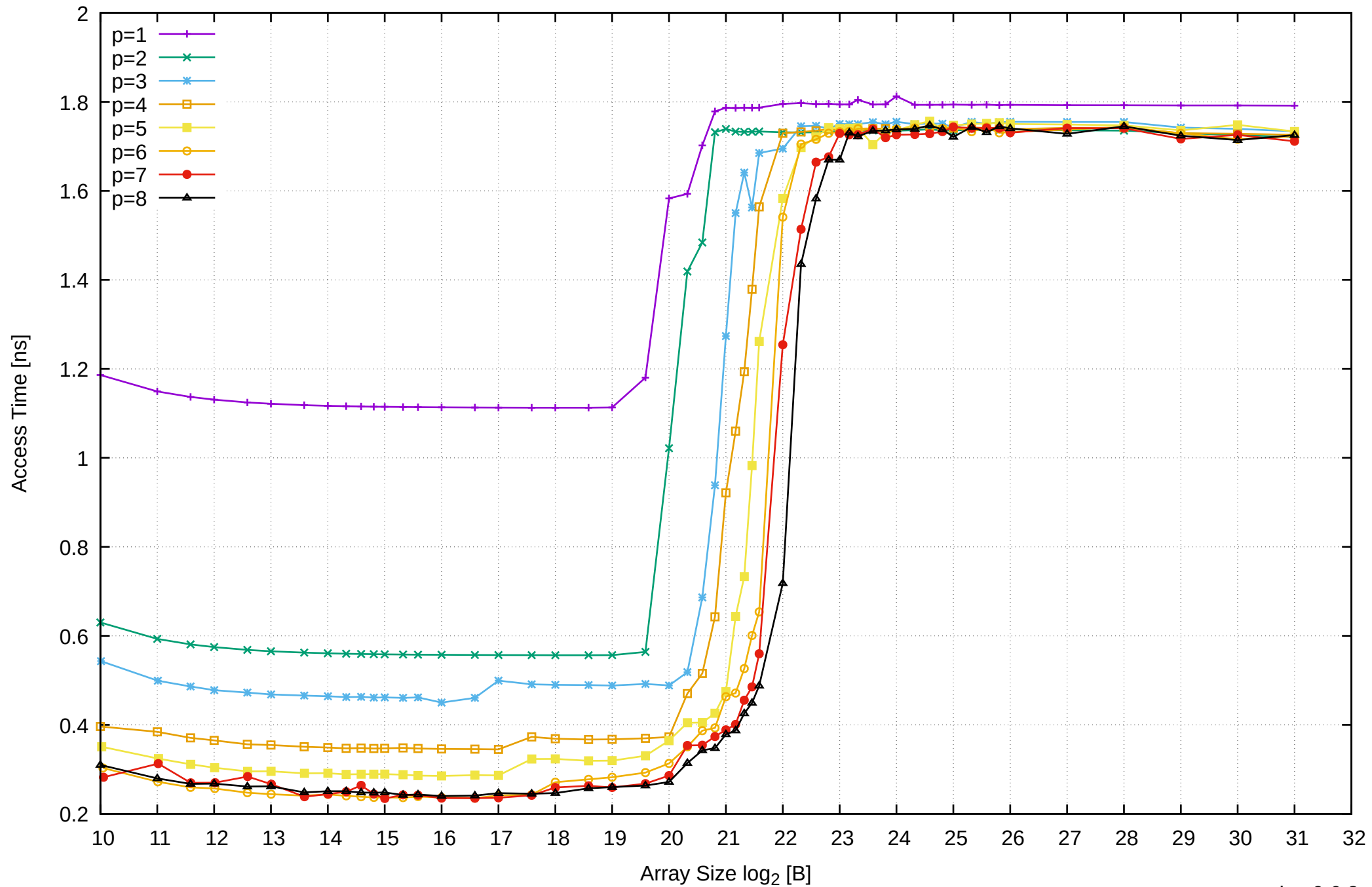
Pine64 RockPro64 Rockchip RK3399 - 4GB - Parallel Memory Access Time - ScanRead64PtrSimpleLoop
