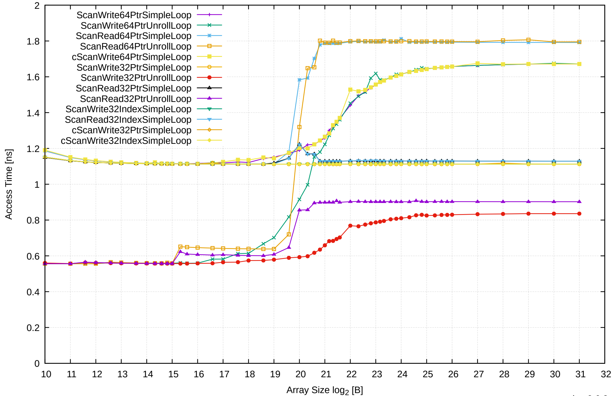
Pine64 RockPro64 Rockchip RK3399 - 4GB - One Thread Memory Latency (excluding Permutation)
