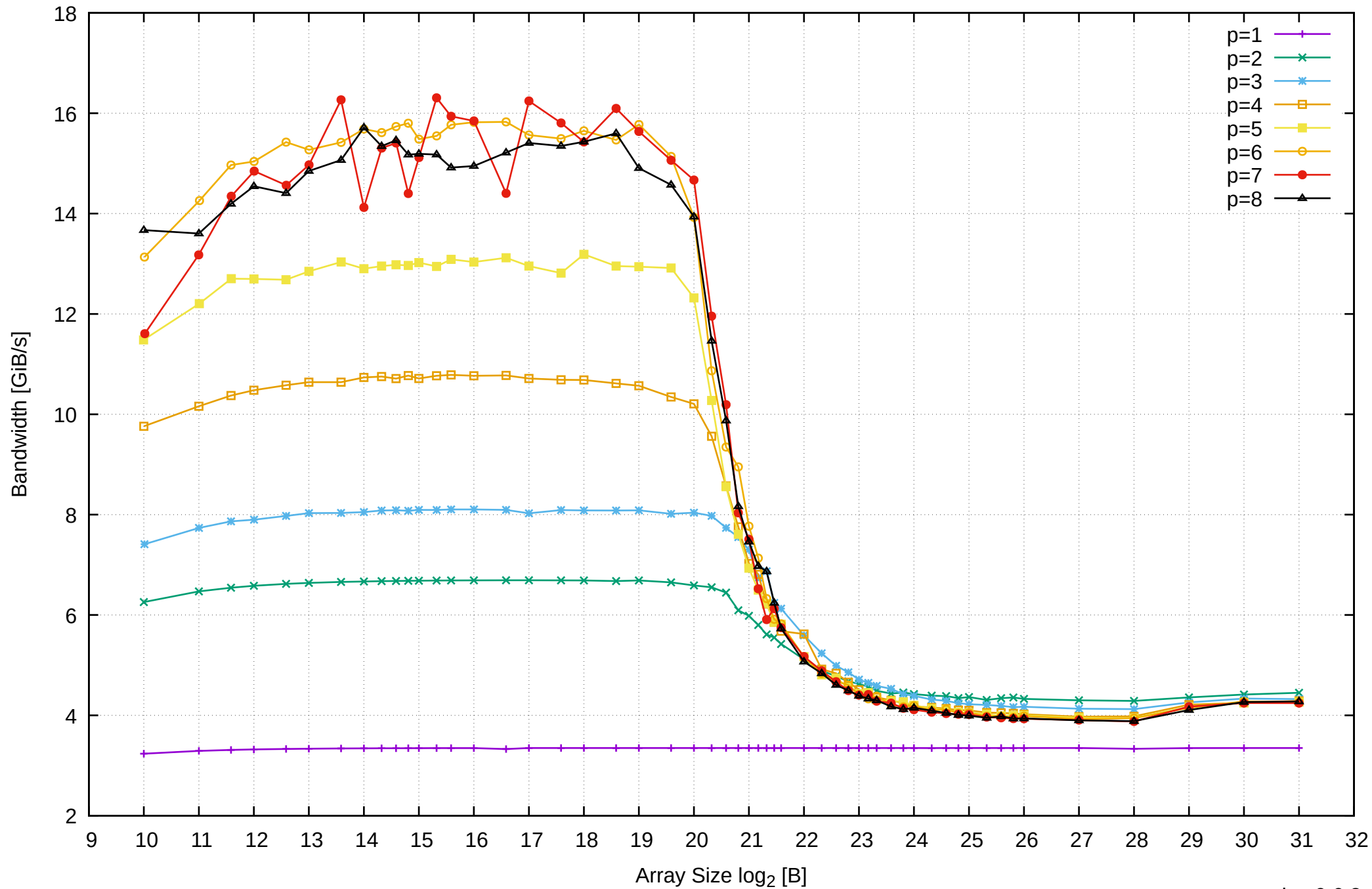
Pine64 RockPro64 Rockchip RK3399 - 4GB - Parallel Memory Bandwidth - cScanWrite32PtrSimpleLoop
