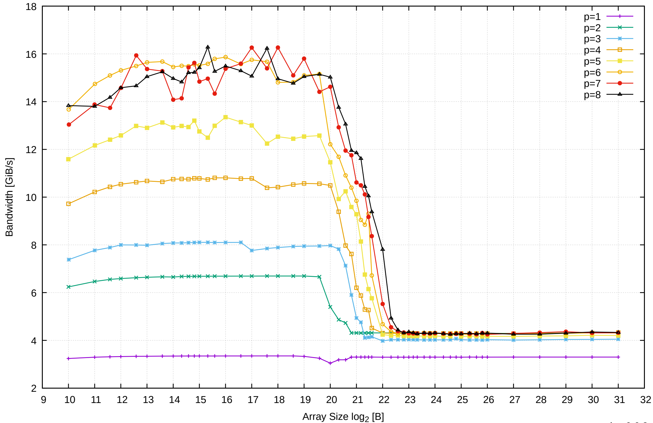
Pine64 RockPro64 Rockchip RK3399 - 4GB - Parallel Memory Bandwidth - ScanRead32PtrSimpleLoop
