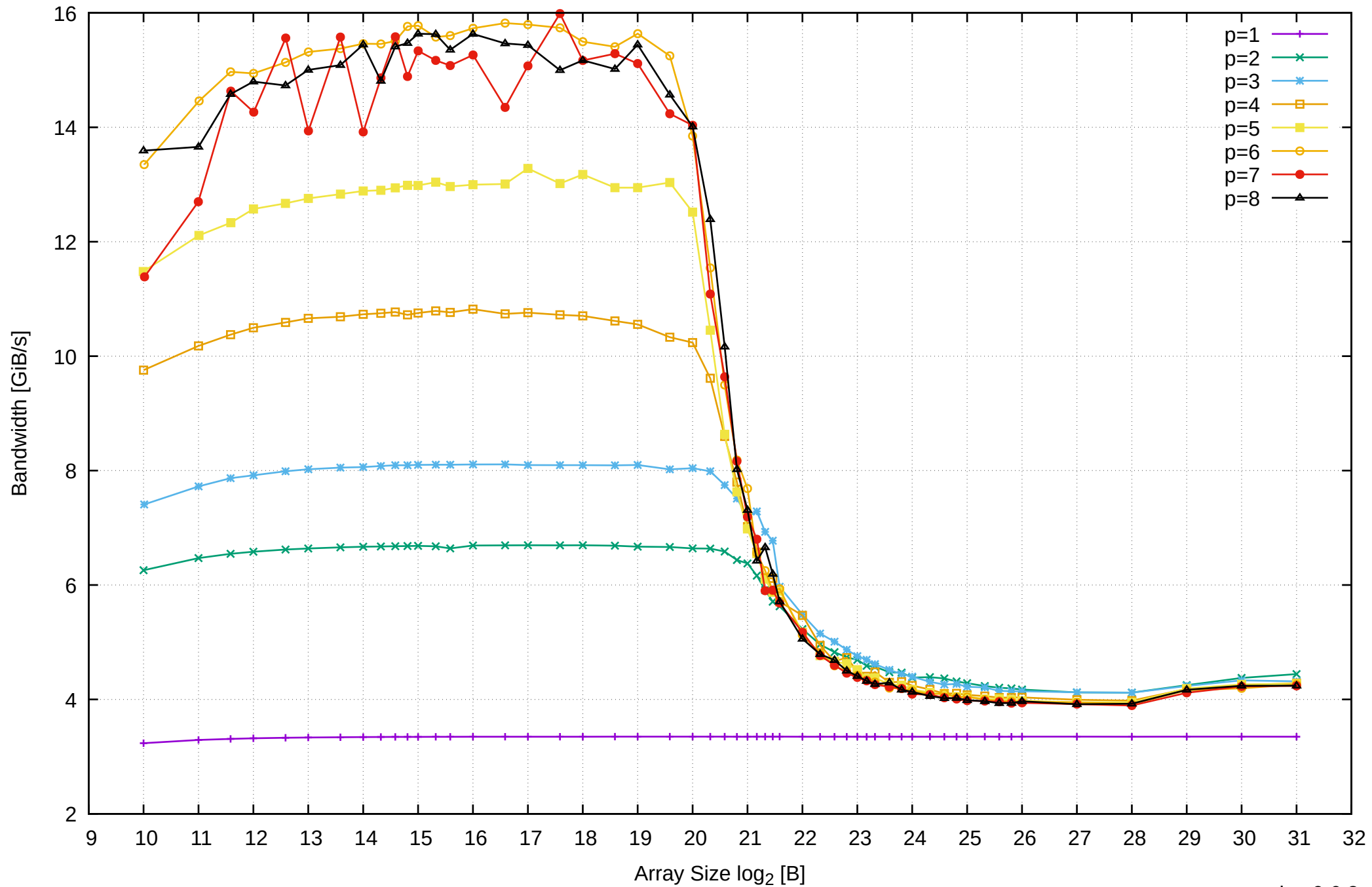
Pine64 RockPro64 Rockchip RK3399 - 4GB - Parallel Memory Bandwidth - ScanWrite32PtrSimpleLoop
