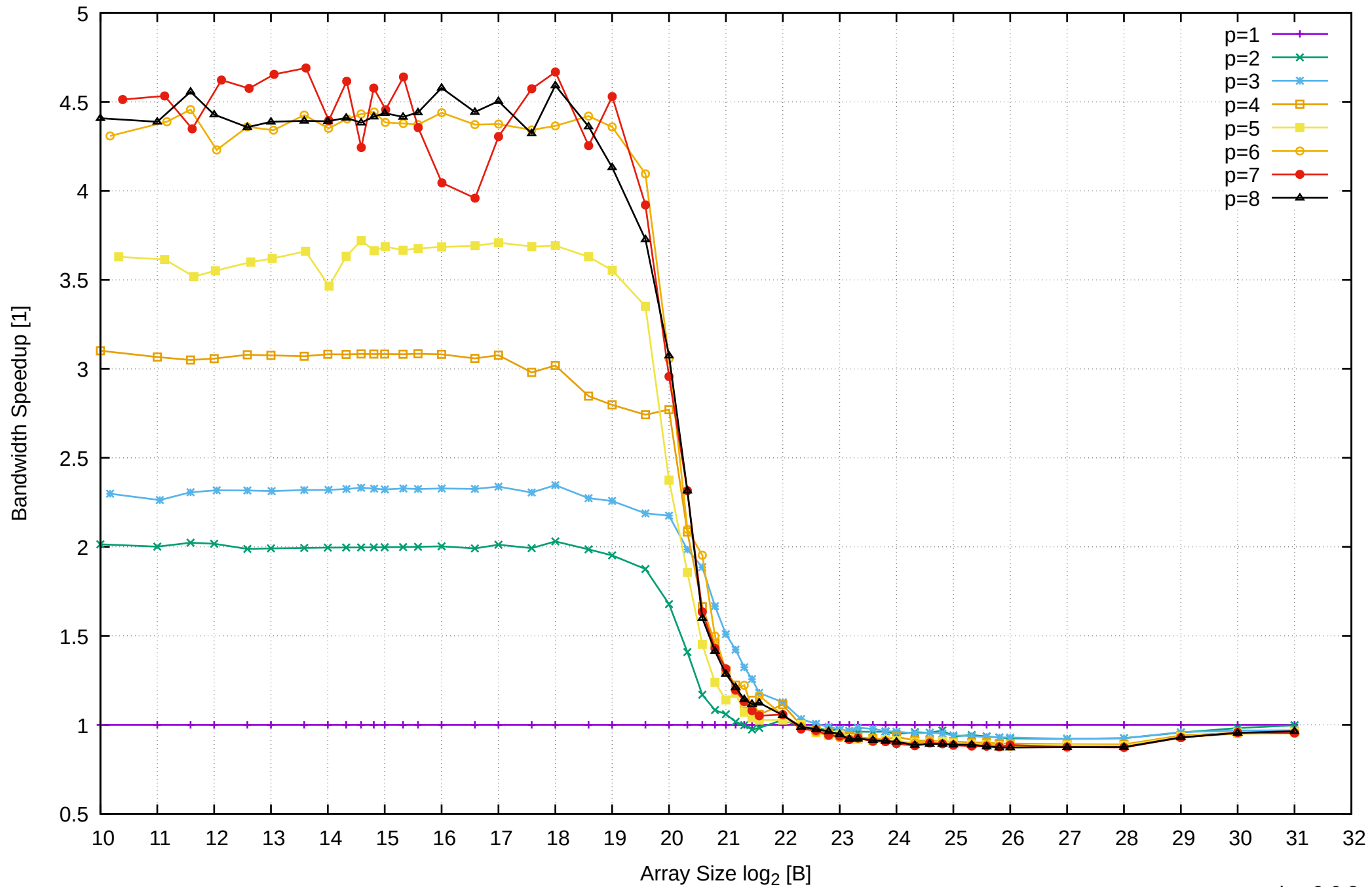
Pine64 RockPro64 Rockchip RK3399 - 4GB - Speedup of Parallel Memory Bandwidth - ScanWrite32PtrUnrollLoop
