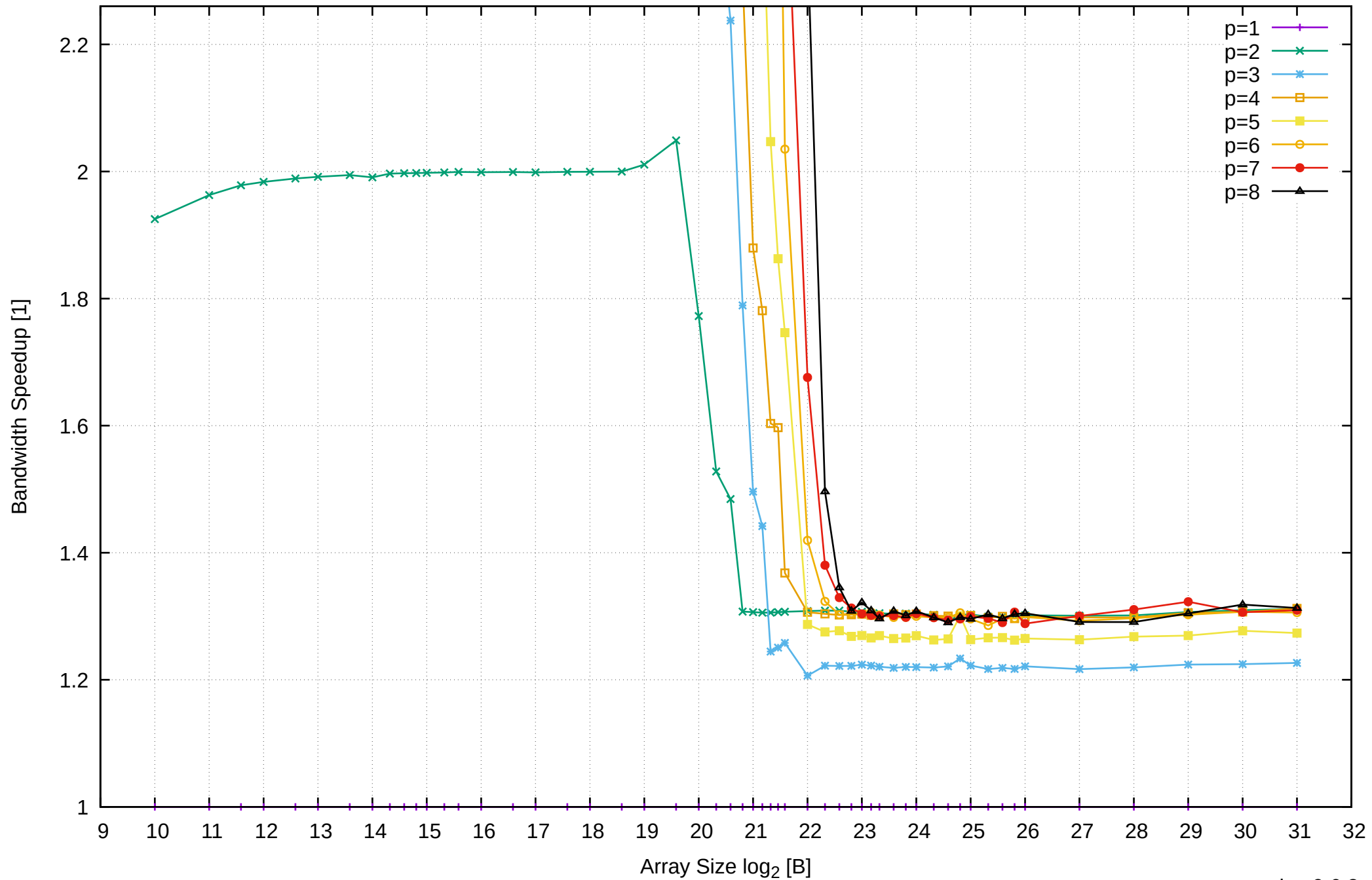
Pine64 RockPro64 Rockchip RK3399 - 4GB - Speedup of Parallel Memory Bandwidth (enlarged) - ScanRead32PtrSimpleLoop
