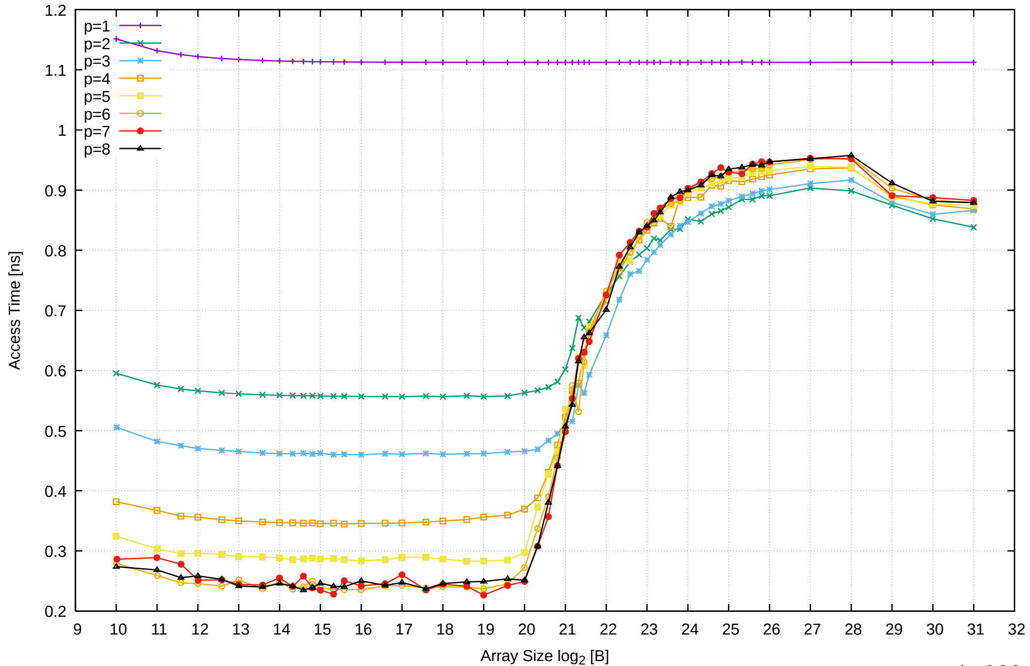
Pine64 RockPro64 Rockchip RK3399 - 4GB - Parallel Memory Access Time - cScanWrite32IndexSimpleLoop
