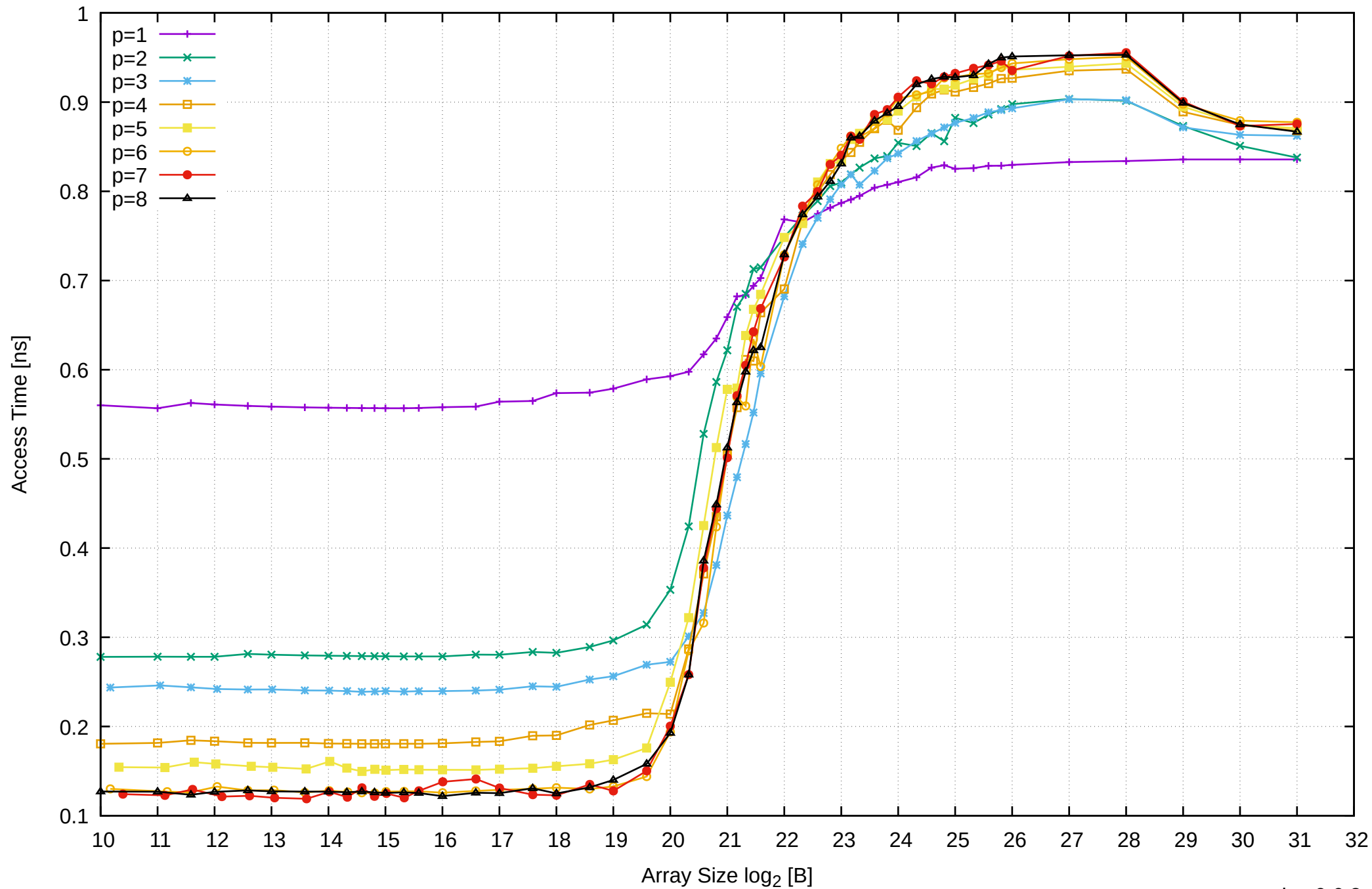
Pine64 RockPro64 Rockchip RK3399 - 4GB - Parallel Memory Access Time - ScanWrite32PtrUnrollLoop
