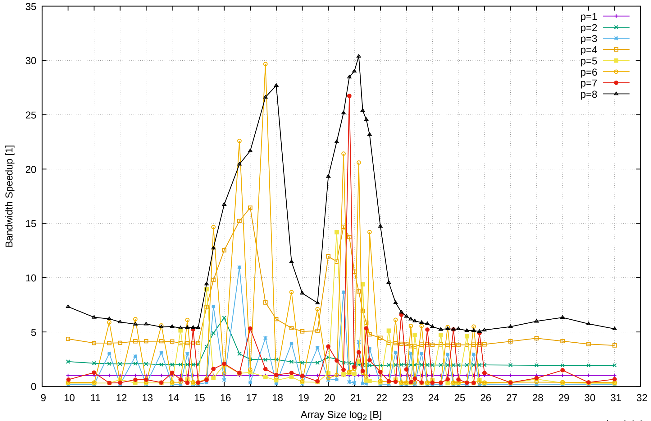
Pine64 RockPro64 Rockchip RK3399 - 4GB - Speedup of Parallel Memory Bandwidth - PermRead64UnrollLoop
