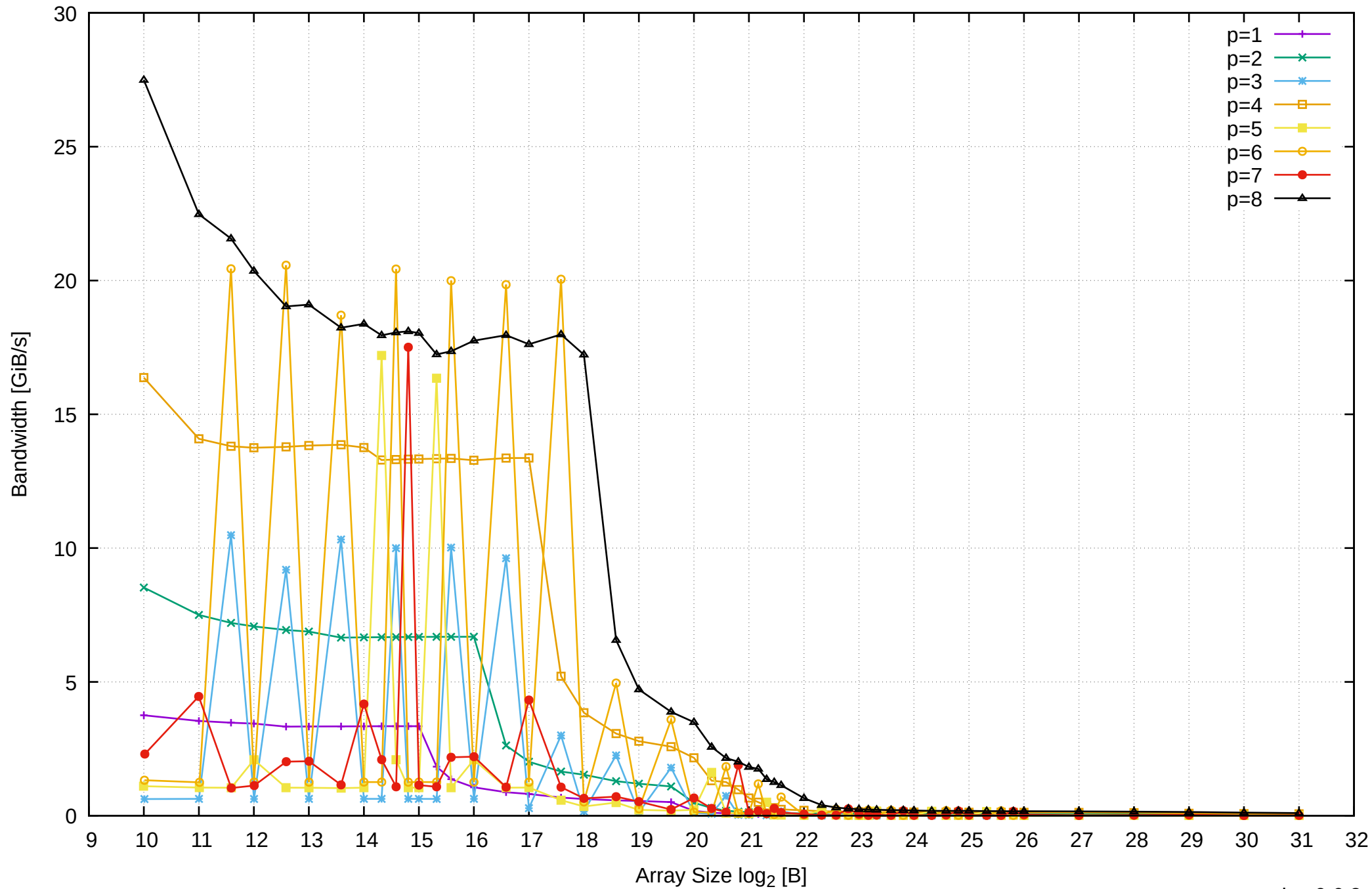
Pine64 RockPro64 Rockchip RK3399 - 4GB - Parallel Memory Bandwidth - PermRead64UnrollLoop
