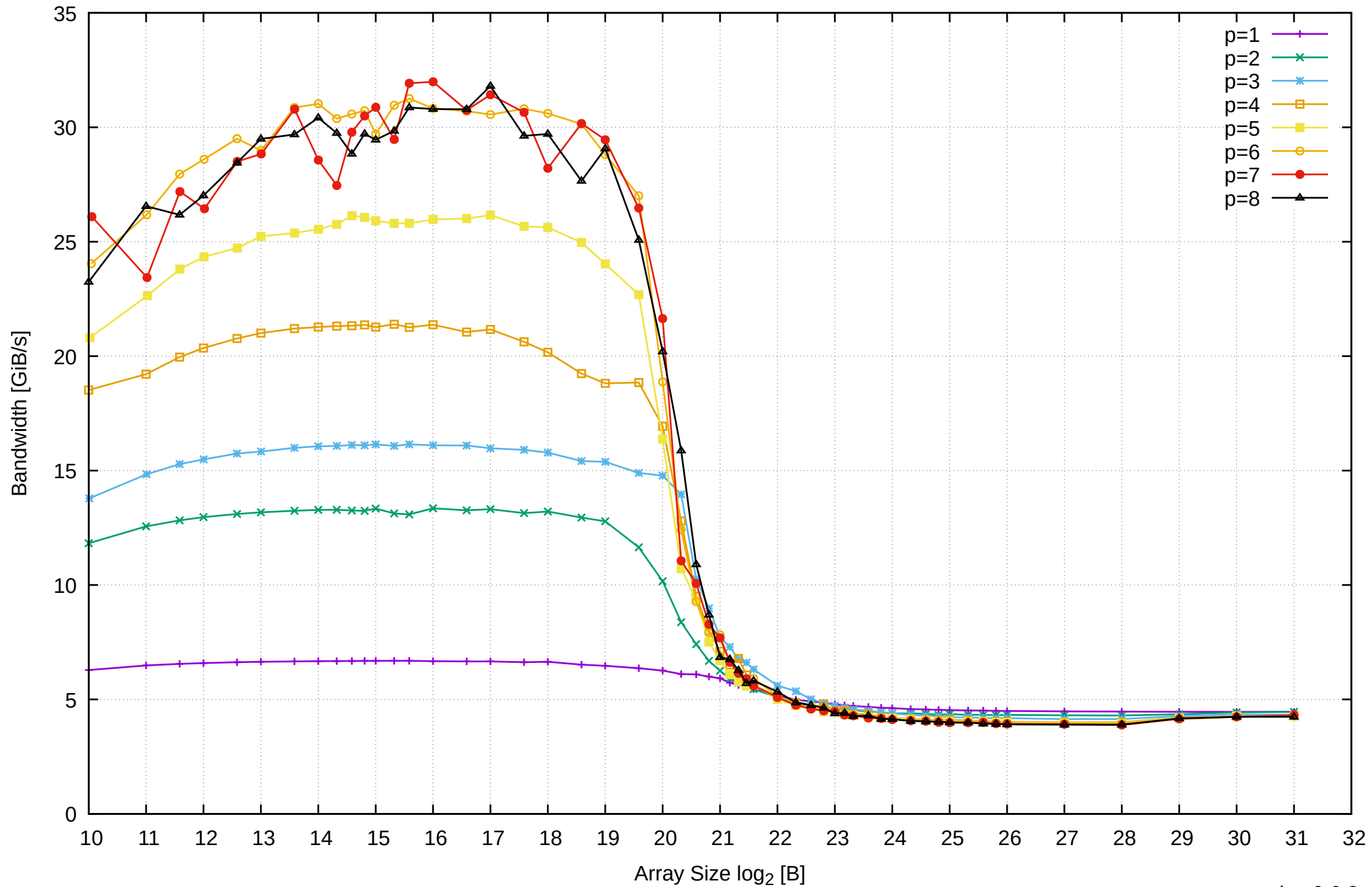
Pine64 RockPro64 Rockchip RK3399 - 4GB - Parallel Memory Bandwidth - ScanWrite64PtrSimpleLoop
