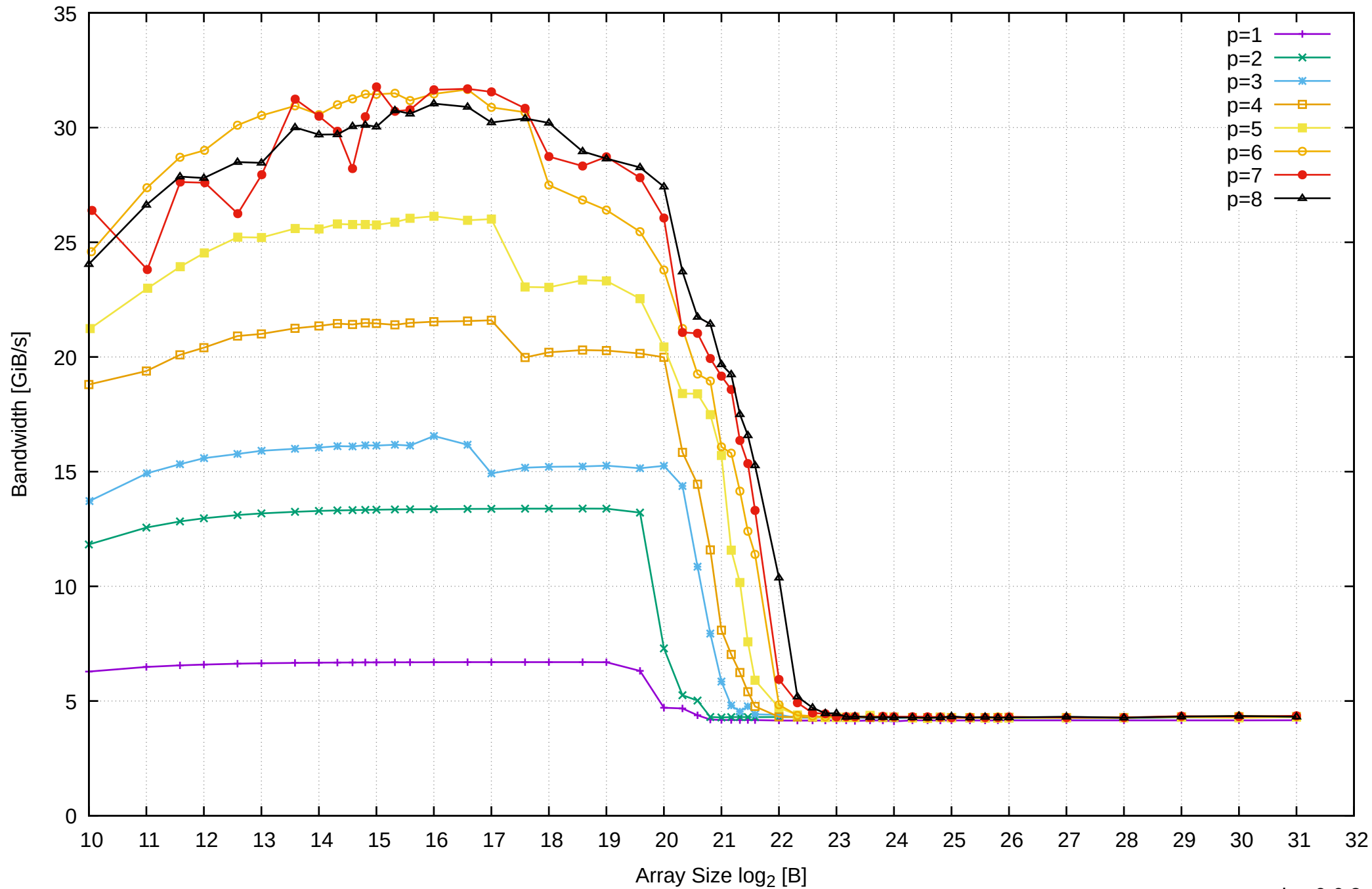
Pine64 RockPro64 Rockchip RK3399 - 4GB - Parallel Memory Bandwidth - ScanRead64PtrSimpleLoop
