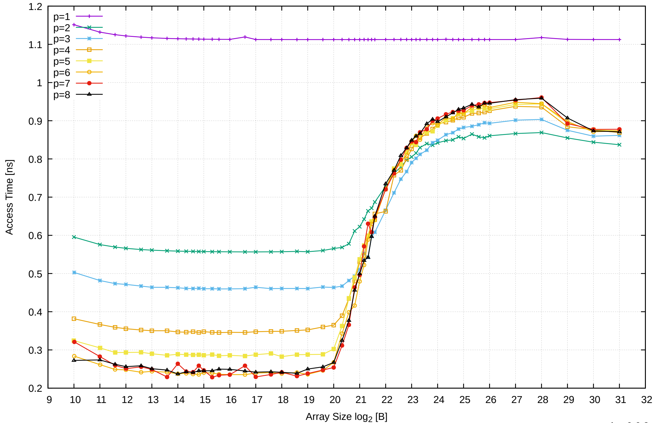
Pine64 RockPro64 Rockchip RK3399 - 4GB - Parallel Memory Access Time - cScanWrite32PtrSimpleLoop
