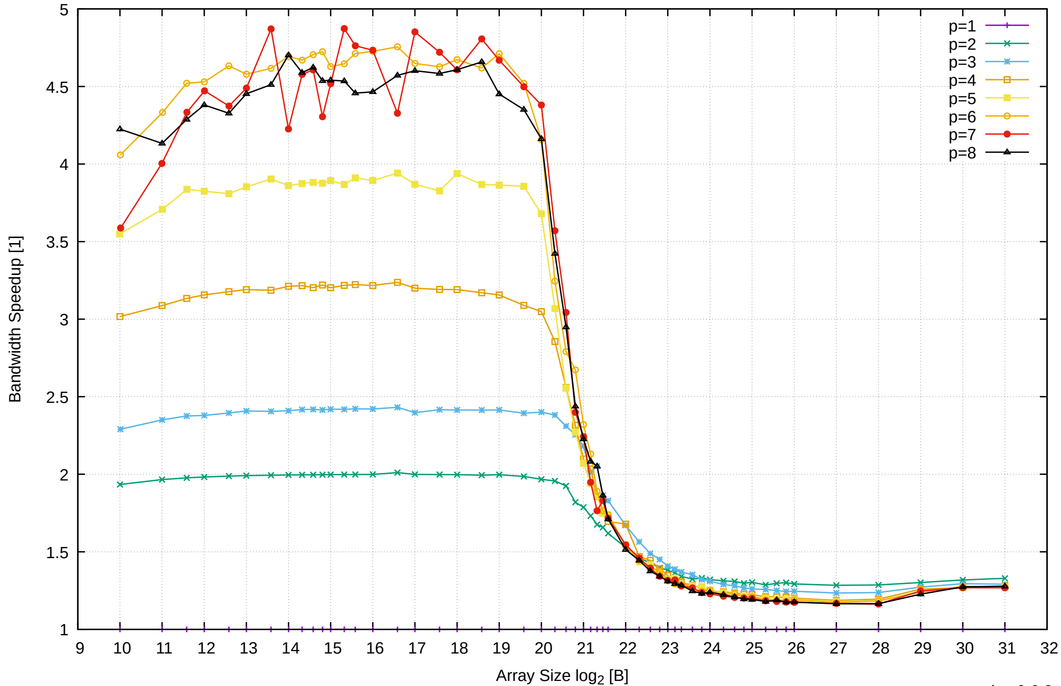
Pine64 RockPro64 Rockchip RK3399 - 4GB - Speedup of Parallel Memory Bandwidth - cScanWrite32PtrSimpleLoop
