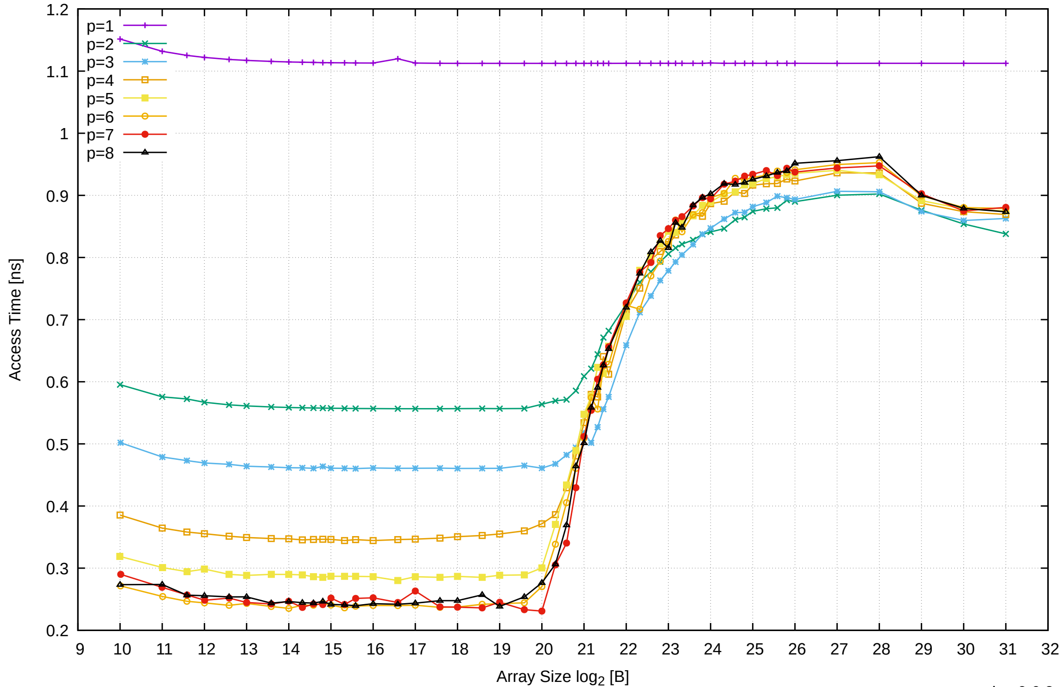
Pine64 RockPro64 Rockchip RK3399 - 4GB - Parallel Memory Access Time - ScanWrite32IndexSimpleLoop
