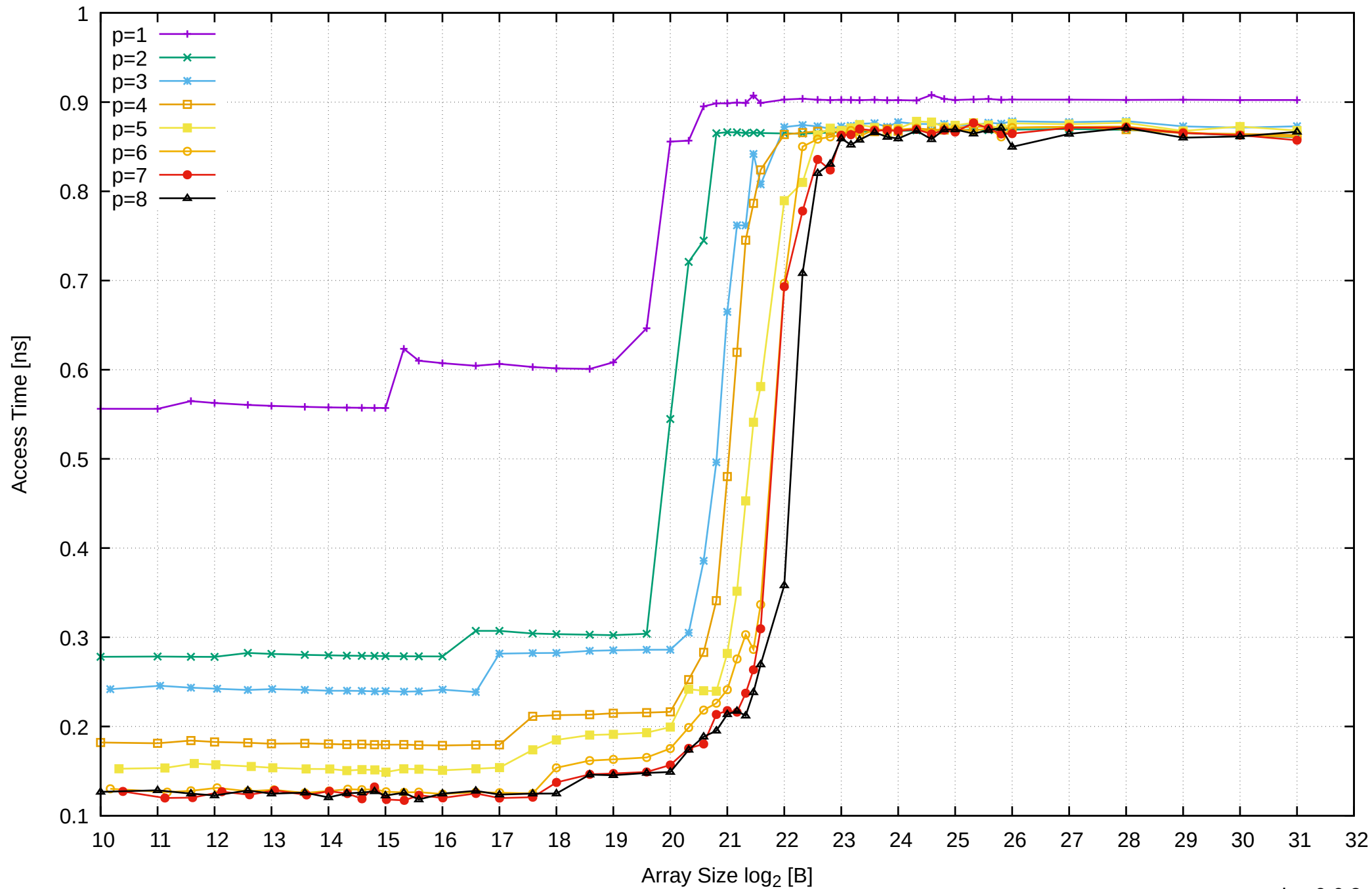
Pine64 RockPro64 Rockchip RK3399 - 4GB - Parallel Memory Access Time - ScanRead32PtrUnrollLoop
