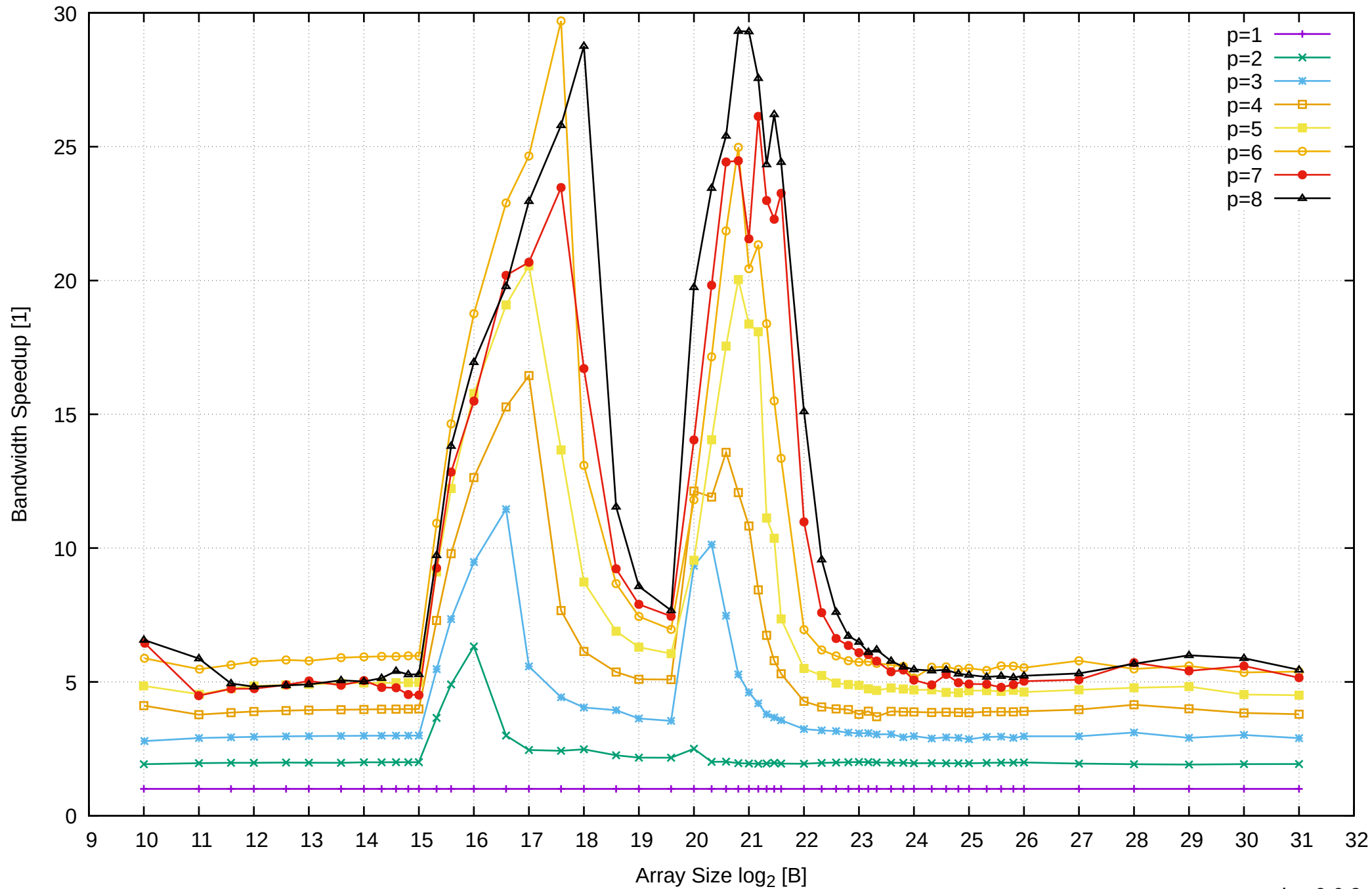
Pine64 RockPro64 Rockchip RK3399 - 4GB - Speedup of Parallel Memory Bandwidth - PermRead64SimpleLoop
