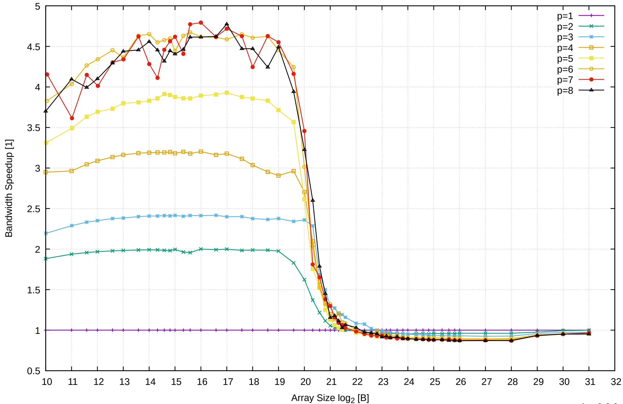
Pine64 RockPro64 Rockchip RK3399 - 4GB - Speedup of Parallel Memory Bandwidth - ScanWrite64PtrSimpleLoop
