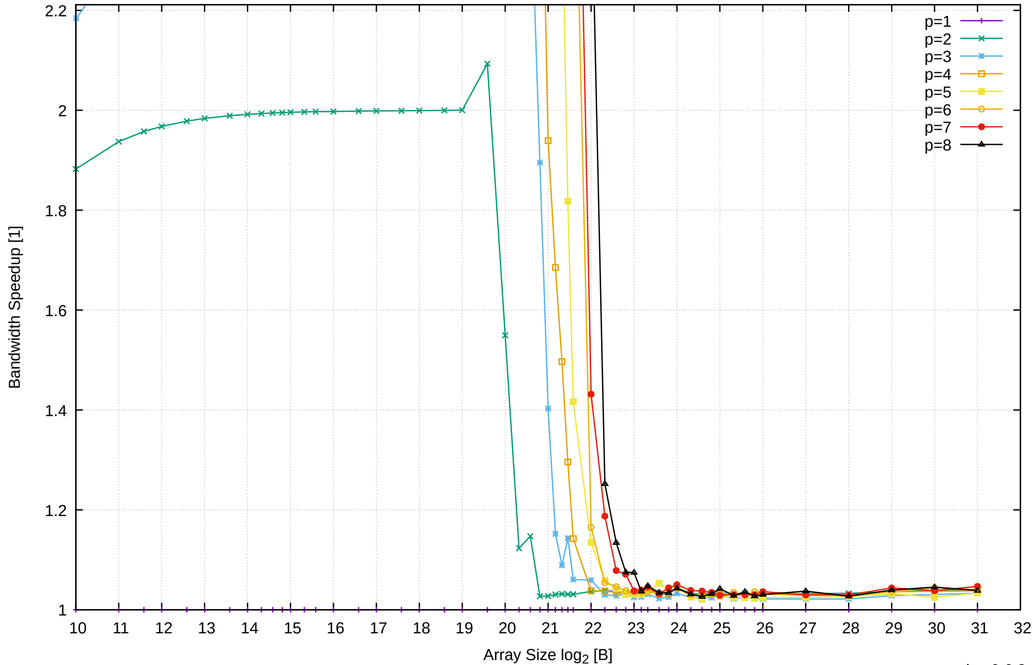
Pine64 RockPro64 Rockchip RK3399 - 4GB - Speedup of Parallel Memory Bandwidth (enlarged) - ScanRead64PtrSimpleLoop
