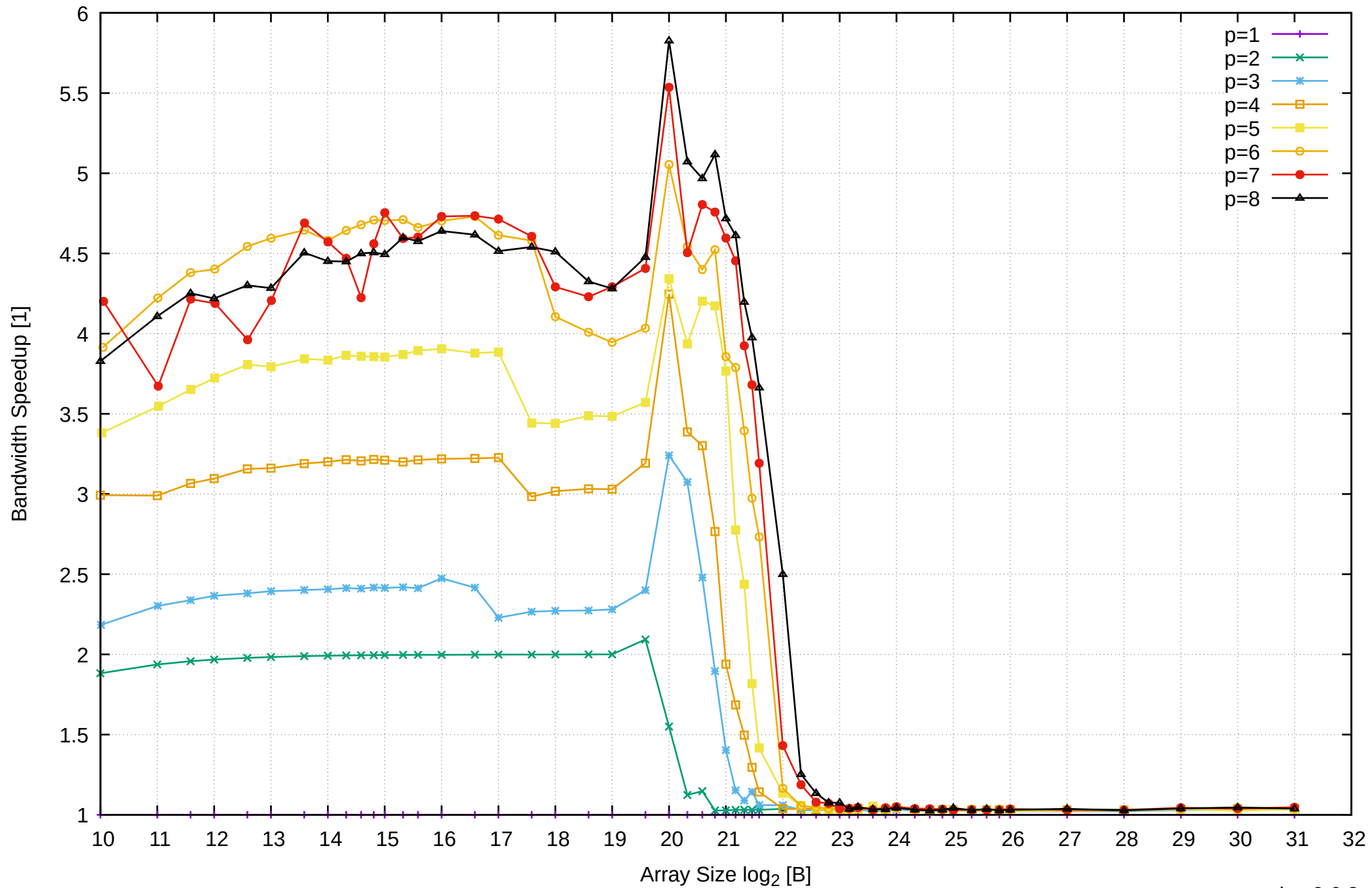
Pine64 RockPro64 Rockchip RK3399 - 4GB - Speedup of Parallel Memory Bandwidth - ScanRead64PtrSimpleLoop
