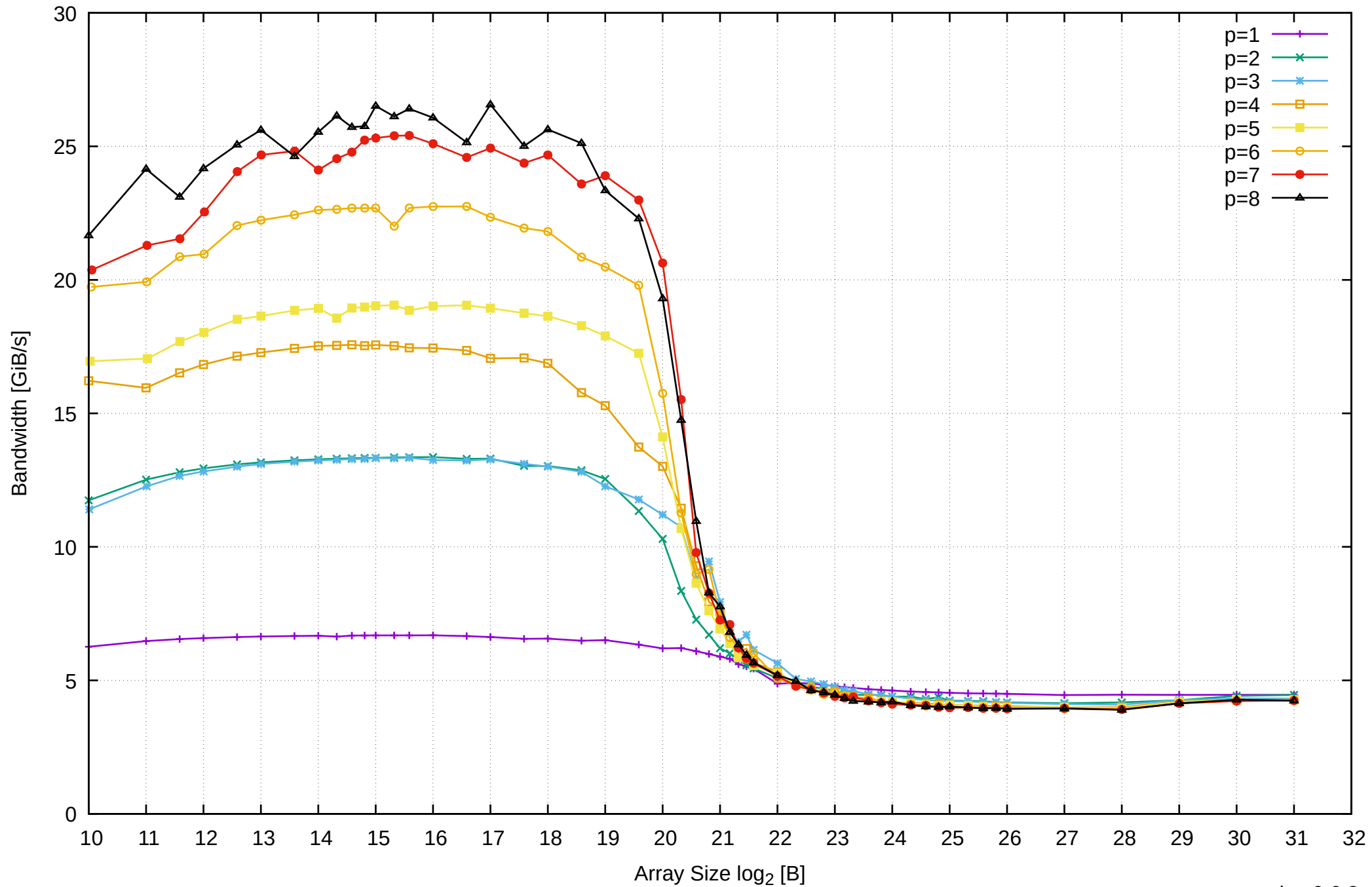
Pine64 RockPro64 Rockchip RK3399 - 4GB - Parallel Memory Bandwidth - cScanWrite64PtrSimpleLoop
