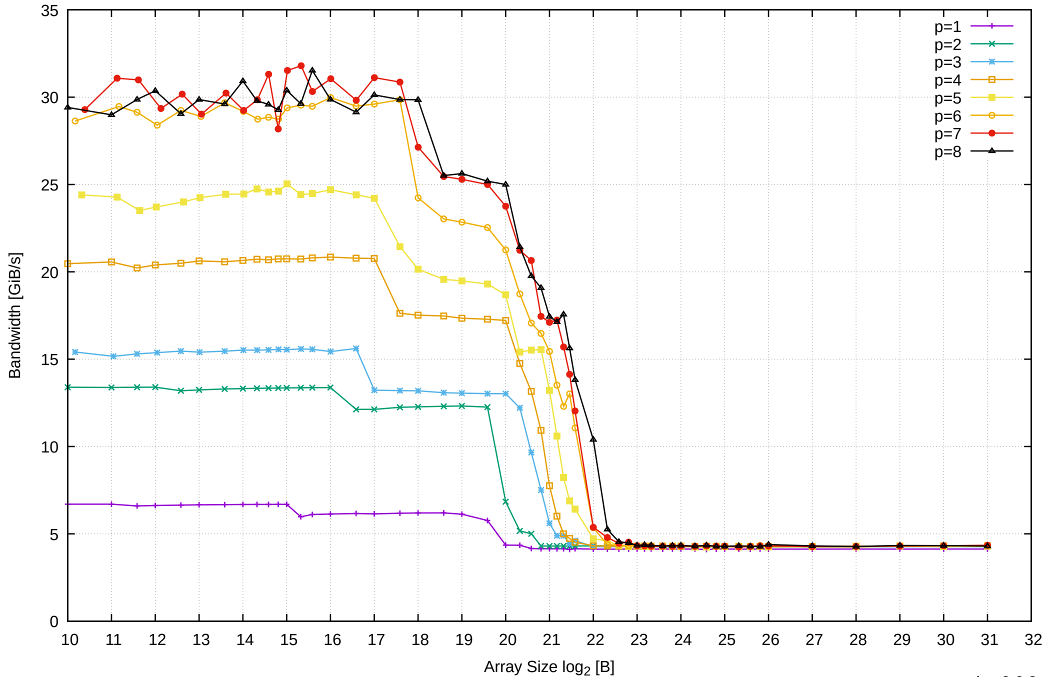
Pine64 RockPro64 Rockchip RK3399 - 4GB - Parallel Memory Bandwidth - ScanRead32PtrUnrollLoop
