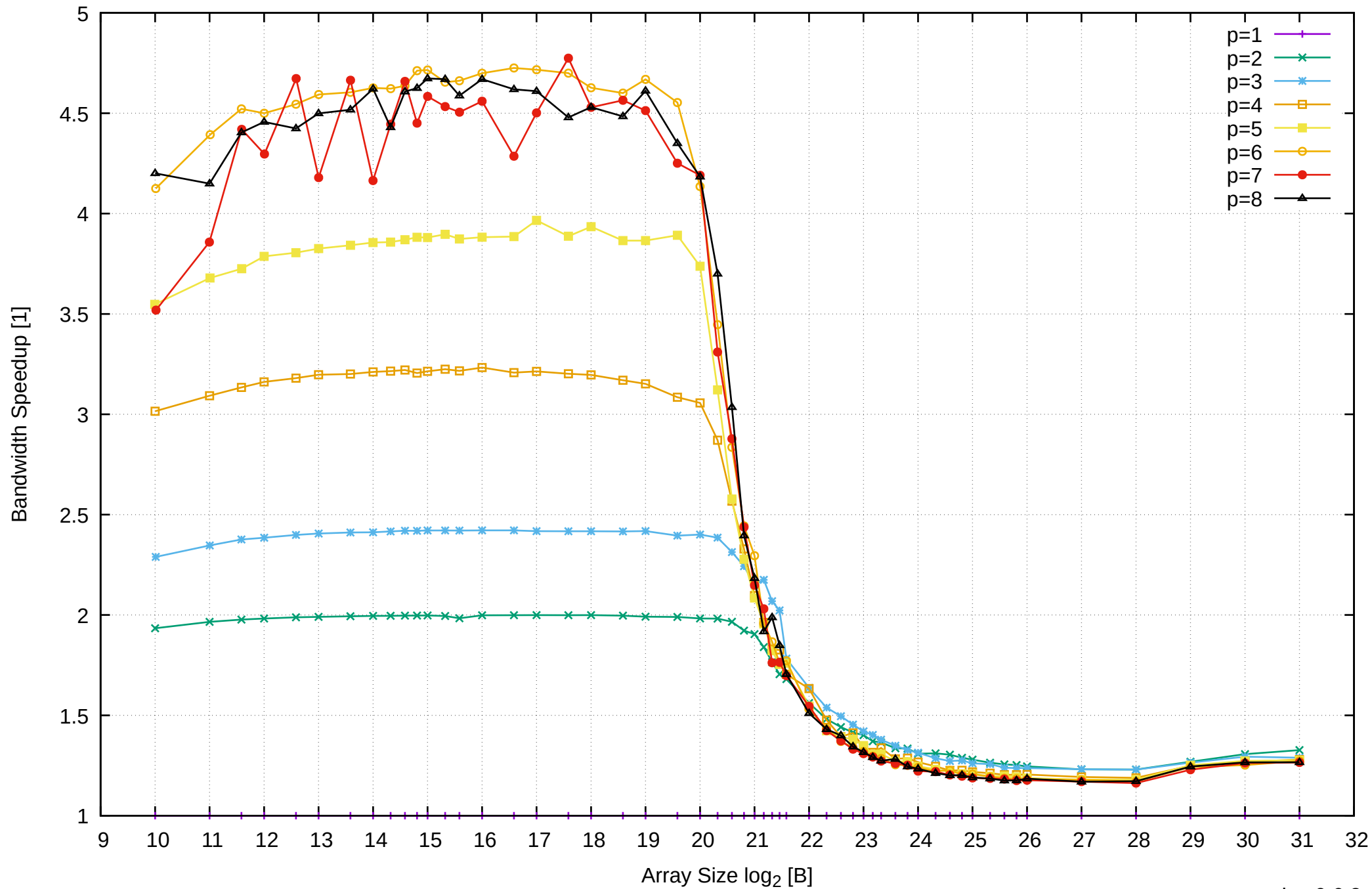
Pine64 RockPro64 Rockchip RK3399 - 4GB - Speedup of Parallel Memory Bandwidth - ScanWrite32PtrSimpleLoop
