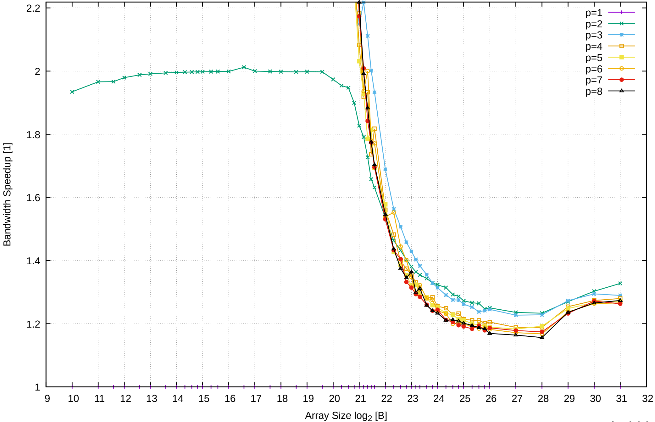
Pine64 RockPro64 Rockchip RK3399 - 4GB - Speedup of Parallel Memory Bandwidth (enlarged) - ScanWrite32IndexSimpleLoop
