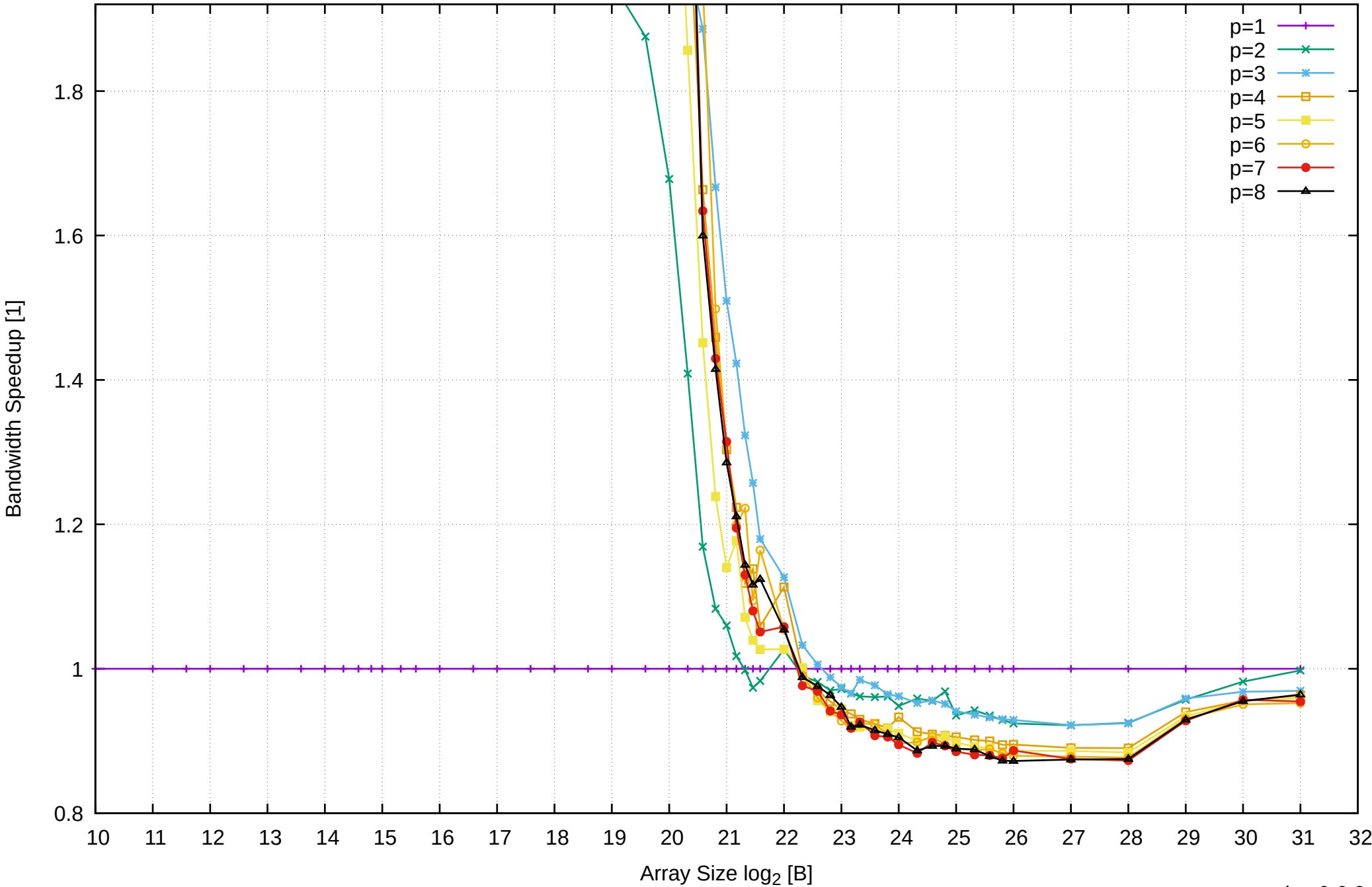
Pine64 RockPro64 Rockchip RK3399 - 4GB - Speedup of Parallel Memory Bandwidth (enlarged) - ScanWrite32PtrUnrollLoop
