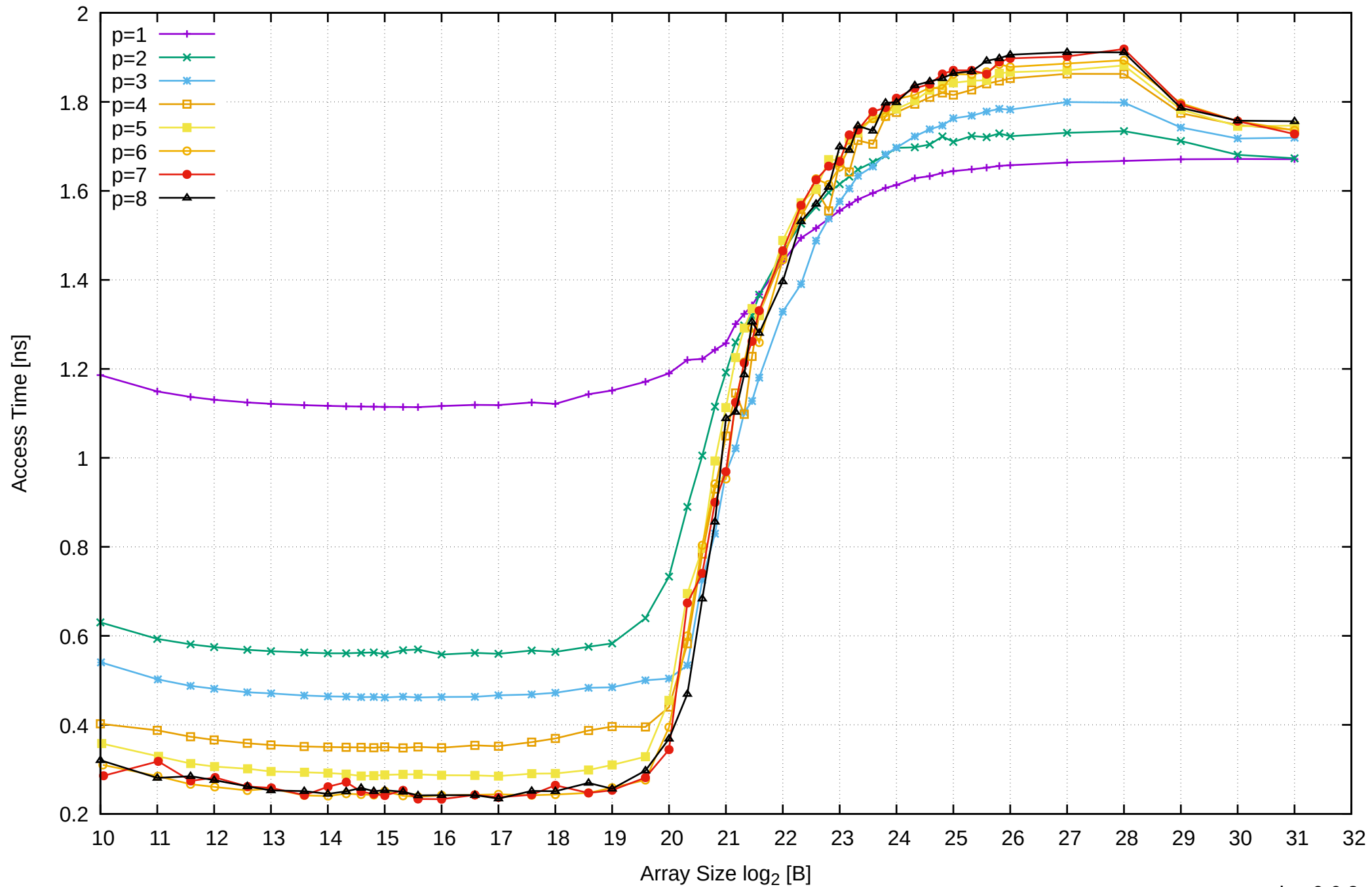
Pine64 RockPro64 Rockchip RK3399 - 4GB - Parallel Memory Access Time - ScanWrite64PtrSimpleLoop
