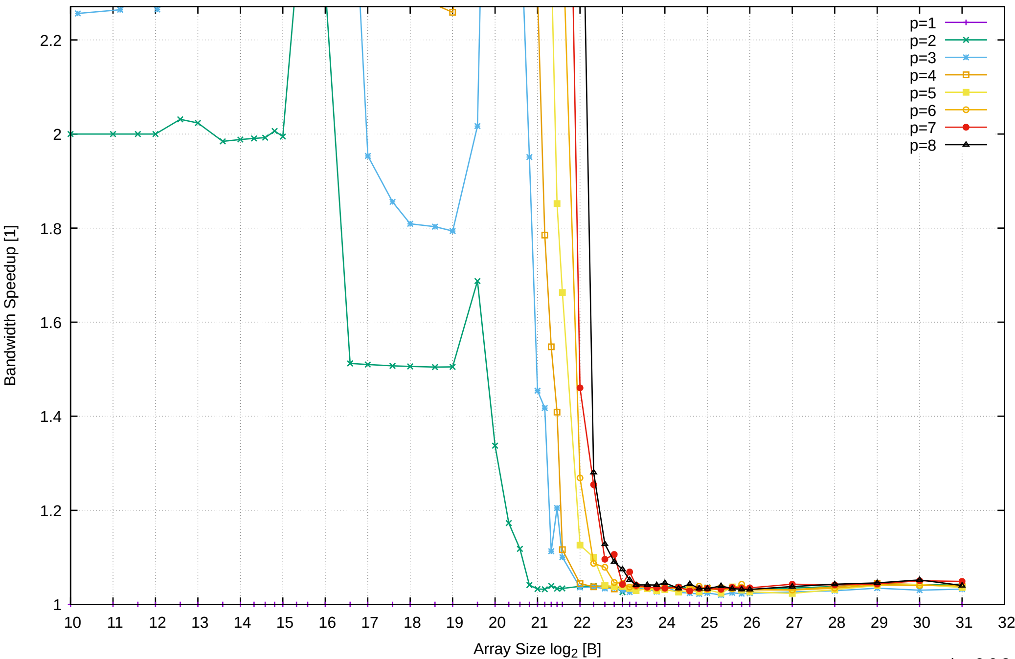
Pine64 RockPro64 Rockchip RK3399 - 4GB - Speedup of Parallel Memory Bandwidth (enlarged) - ScanRead64PtrUnrollLoop
