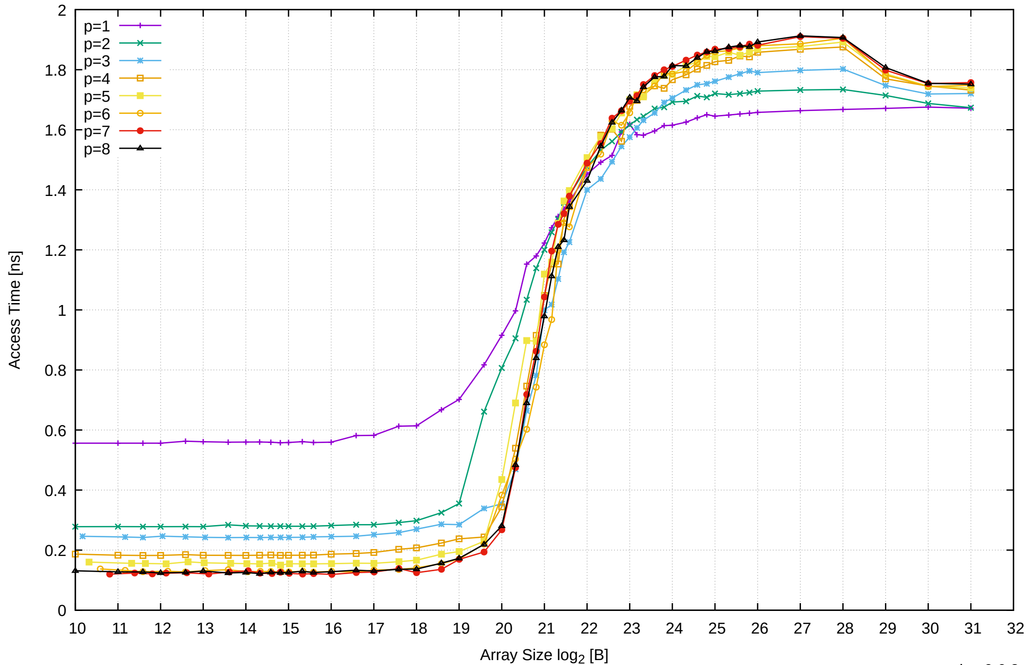
Pine64 RockPro64 Rockchip RK3399 - 4GB - Parallel Memory Access Time - ScanWrite64PtrUnrollLoop
