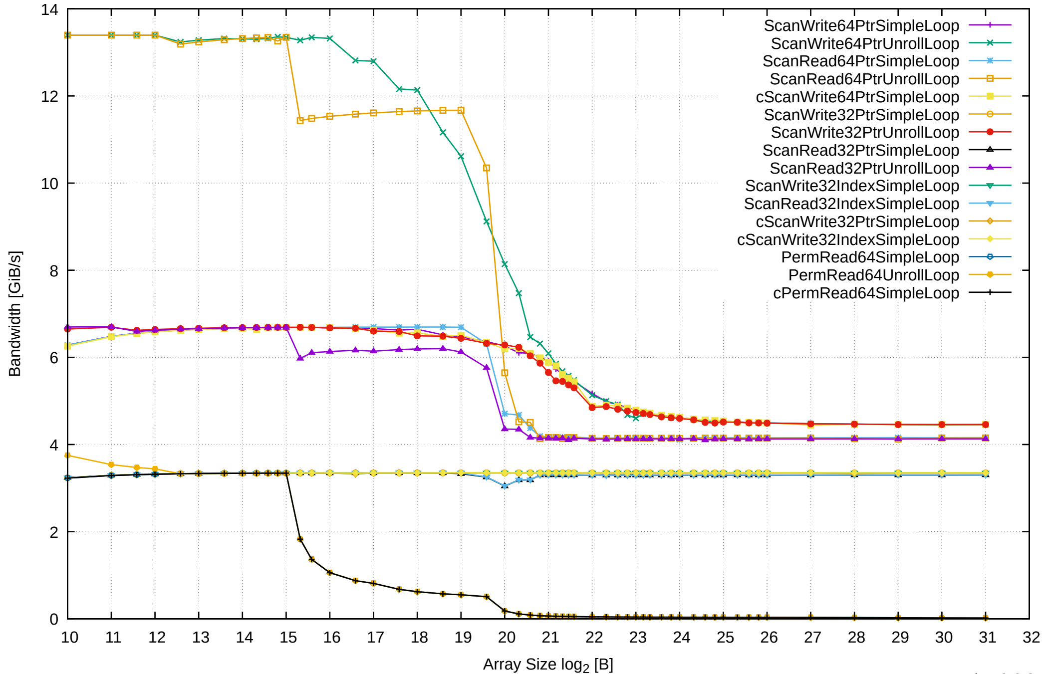
Pine64 RockPro64 Rockchip RK3399 - 4GB - One Thread Memory Bandwidth
