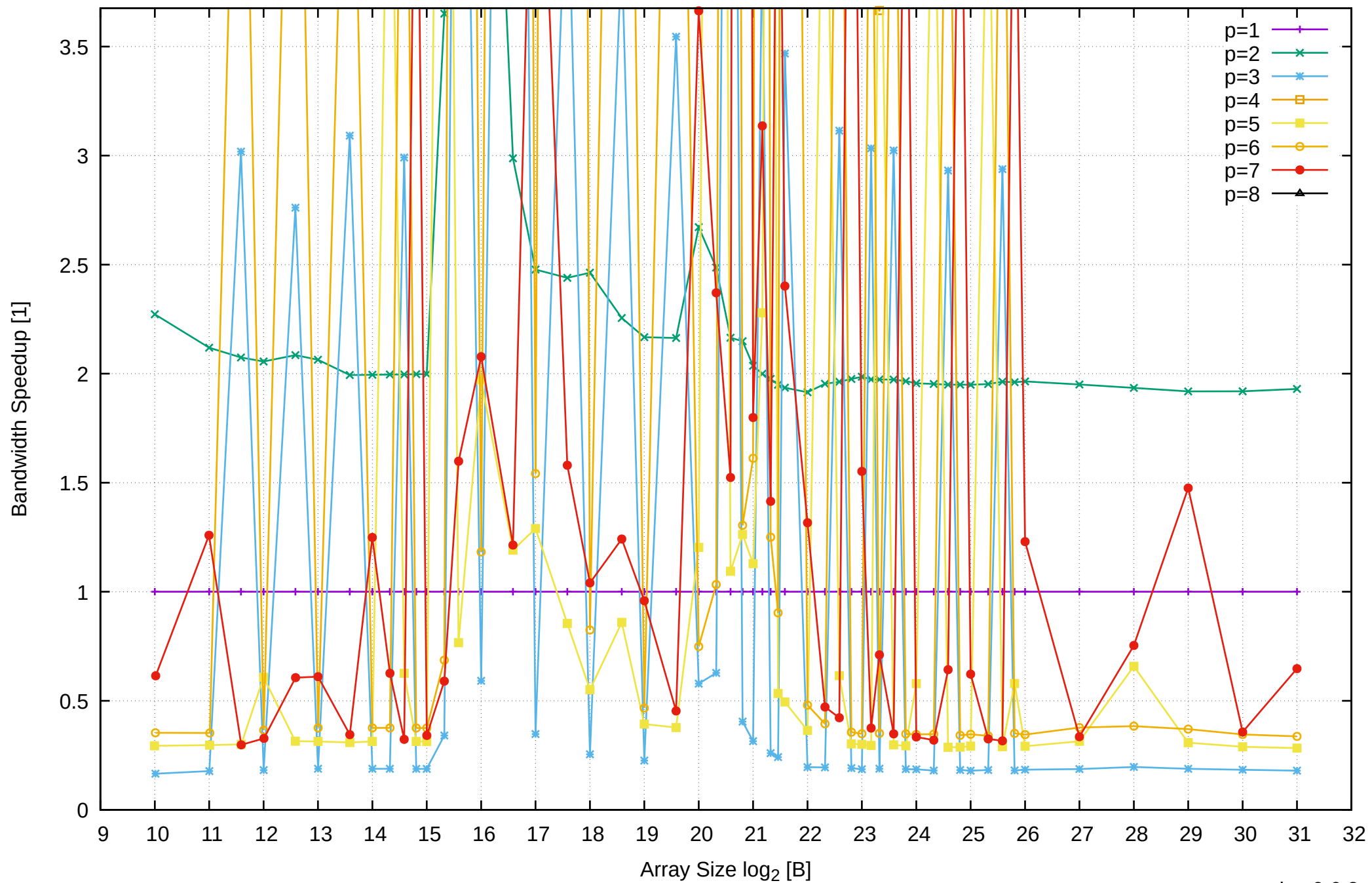
Pine64 RockPro64 Rockchip RK3399 - 4GB - Speedup of Parallel Memory Bandwidth (enlarged) - PermRead64UnrollLoop
