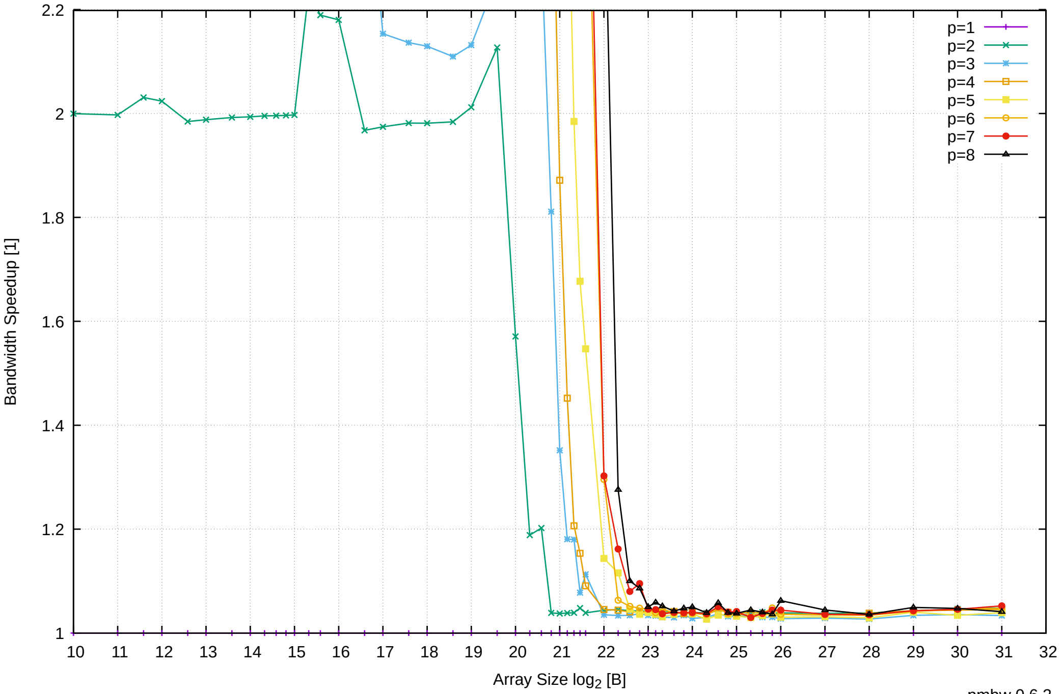
Pine64 RockPro64 Rockchip RK3399 - 4GB - Speedup of Parallel Memory Bandwidth (enlarged) - ScanRead32PtrUnrollLoop
