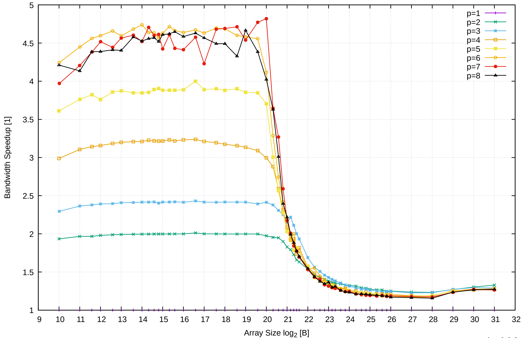
Pine64 RockPro64 Rockchip RK3399 - 4GB - Speedup of Parallel Memory Bandwidth - ScanWrite32IndexSimpleLoop
