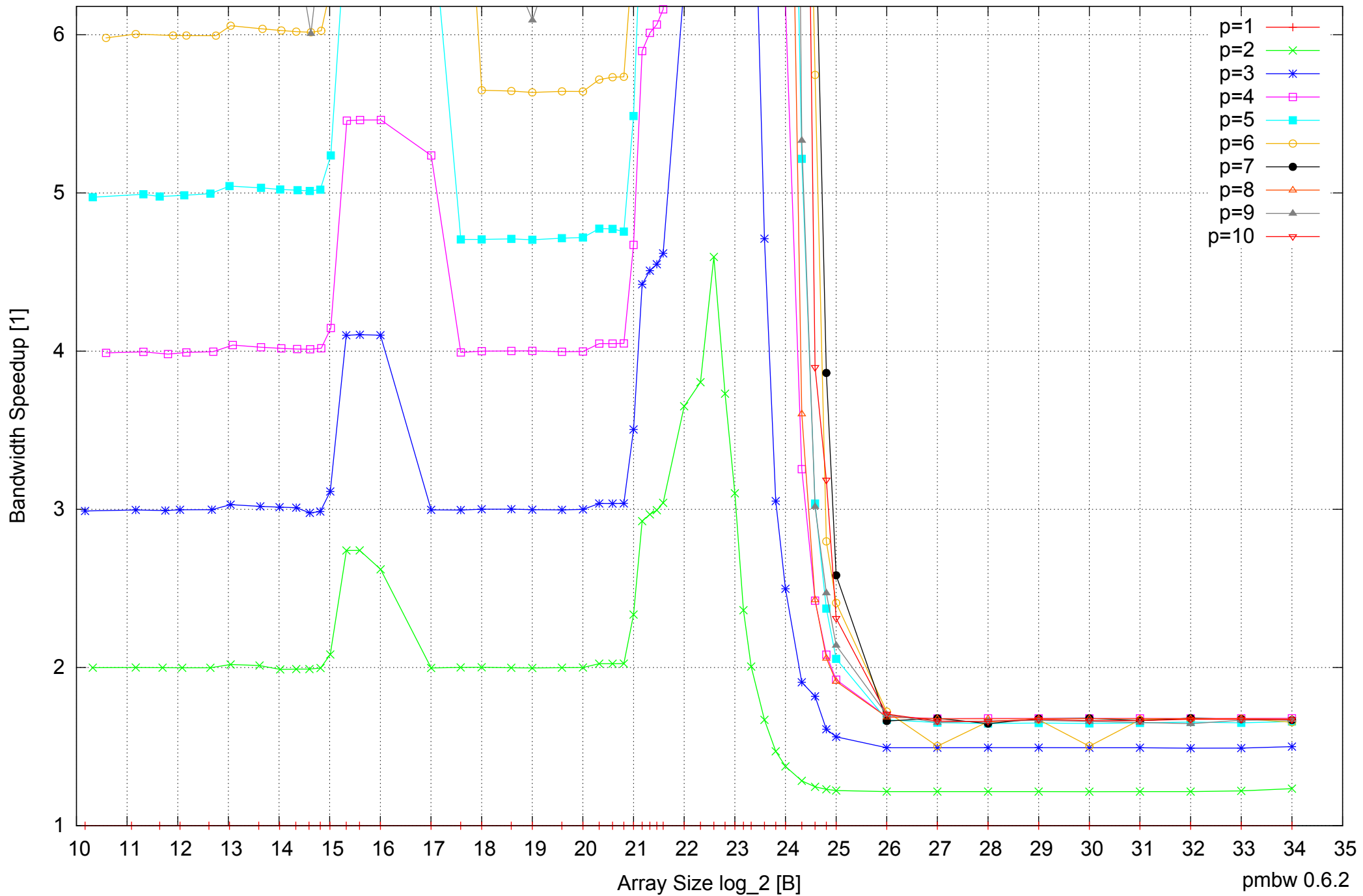
Intel Xeon X5355 24GB - Speedup of Parallel Memory Bandwidth (enlarged) - ScanRead64IndexUnrollLoop
