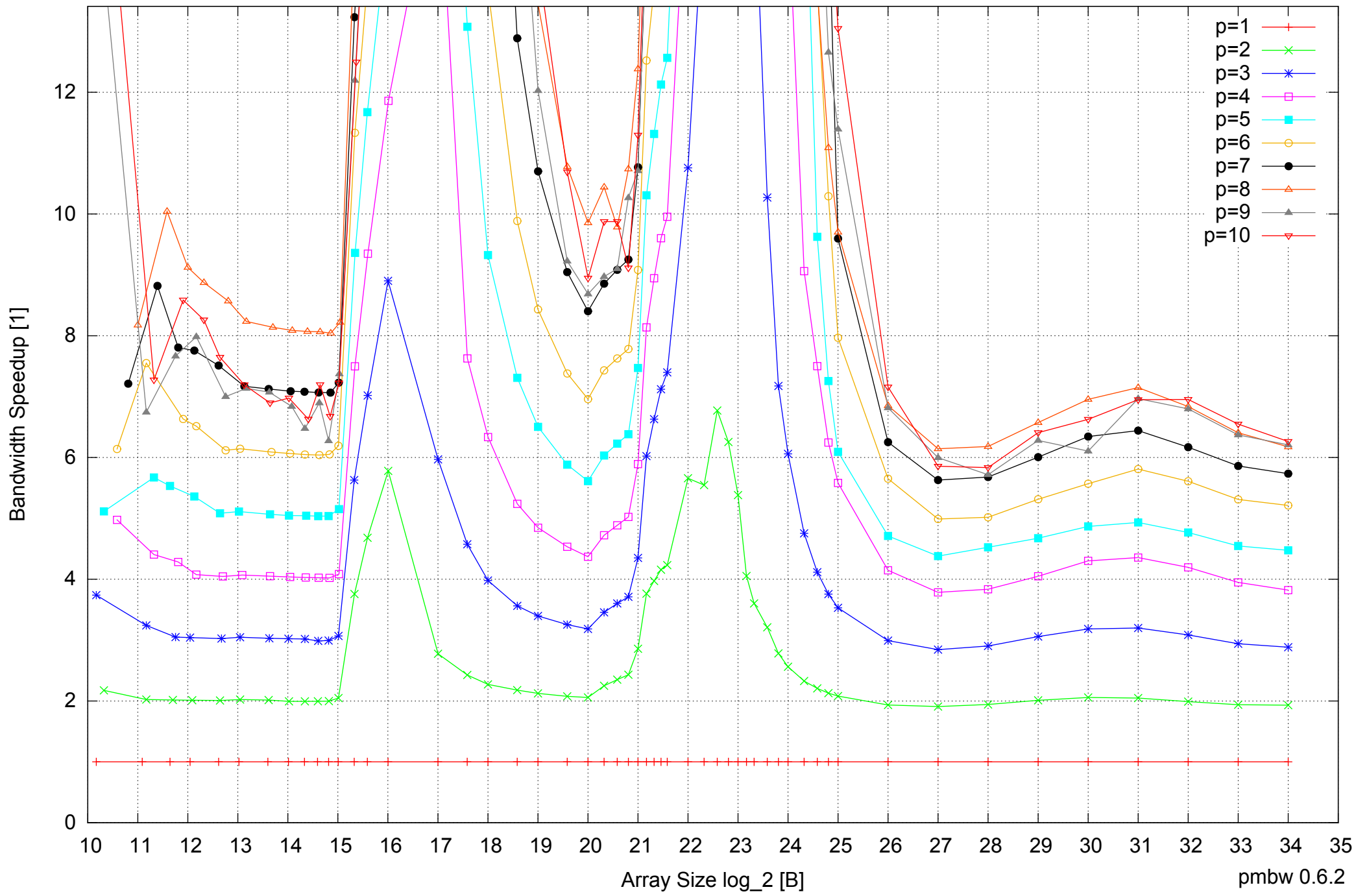
Intel Xeon X5355 24GB - Speedup of Parallel Memory Bandwidth (enlarged) - PermRead64UnrollLoop
