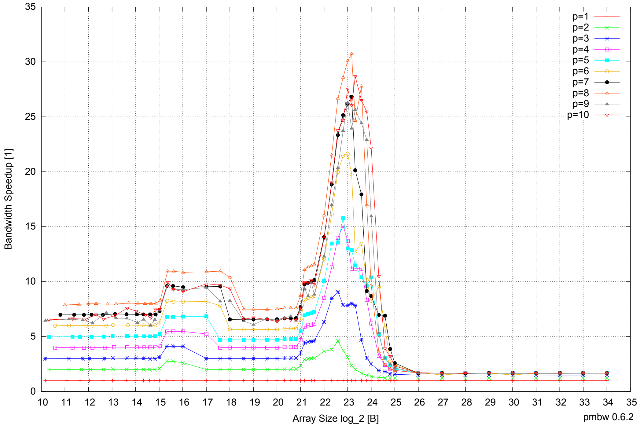
Intel Xeon X5355 24GB - Speedup of Parallel Memory Bandwidth - ScanRead64IndexUnrollLoop
