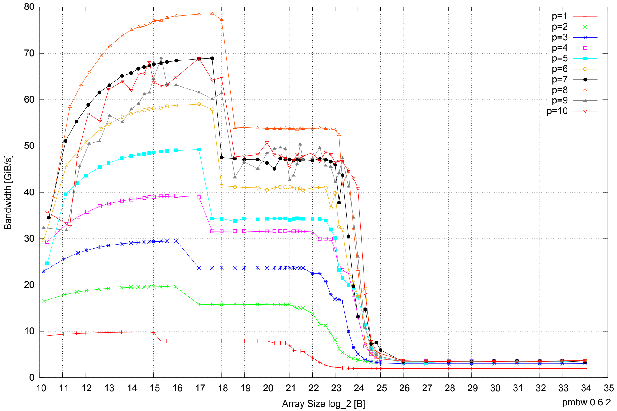
Intel Xeon X5355 24GB - Parallel Memory Bandwidth - ScanWrite32PtrSimpleLoop
