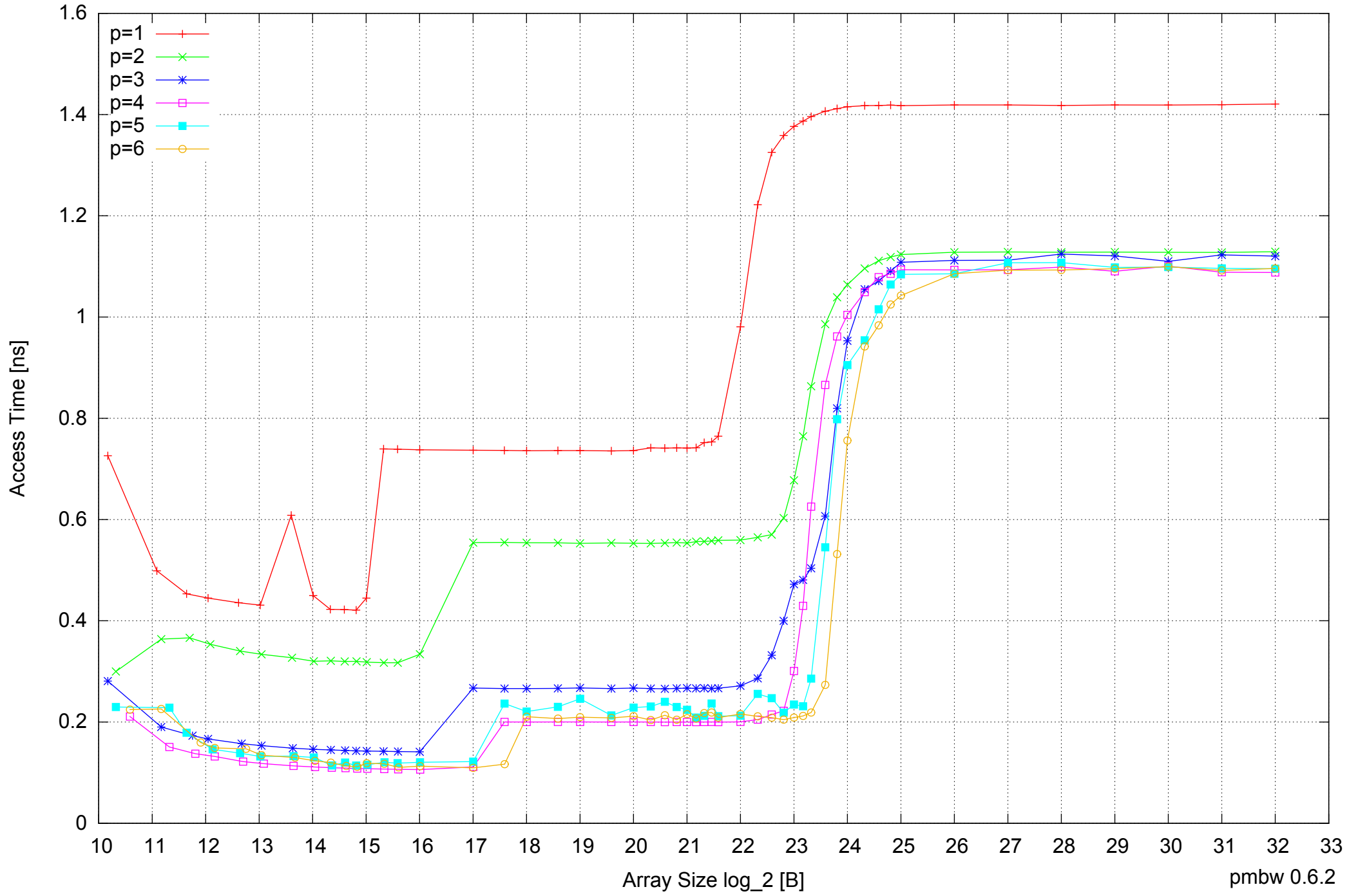
Intel Core 2 Quad Q6600 8GB - Parallel Memory Access Time - ScanRead64IndexSimpleLoop
