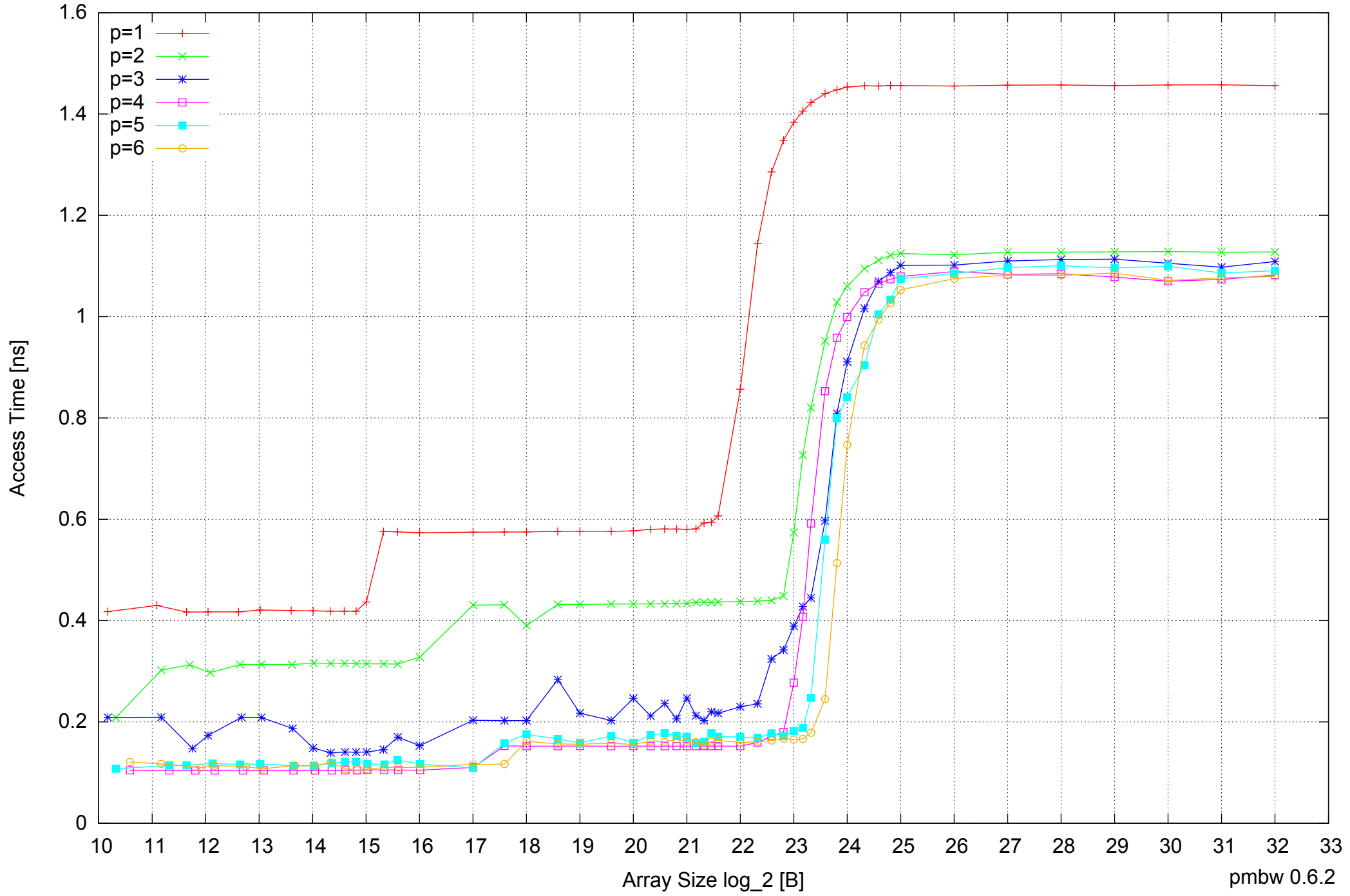
Intel Core 2 Quad Q6600 8GB - Parallel Memory Access Time - ScanRead64IndexUnrollLoop
