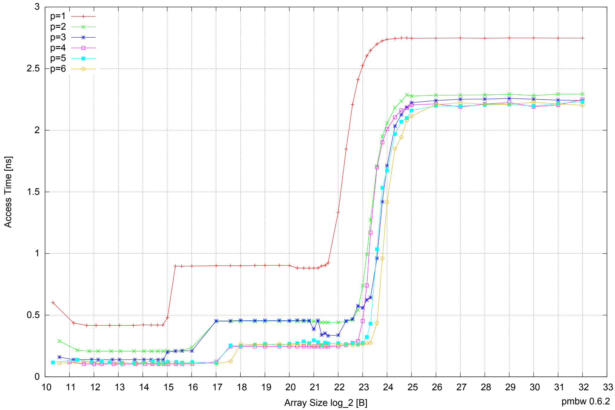
Intel Core 2 Quad Q6600 8GB - Parallel Memory Access Time - ScanRead128PtrUnrollLoop
