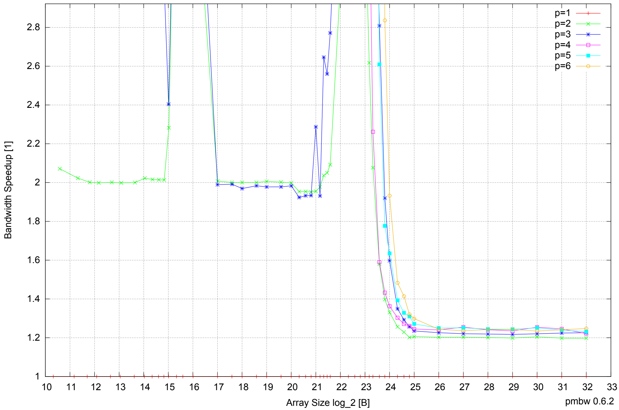
Intel Core 2 Quad Q6600 8GB - Speedup of Parallel Memory Bandwidth (enlarged) - ScanRead128PtrUnrollLoop
