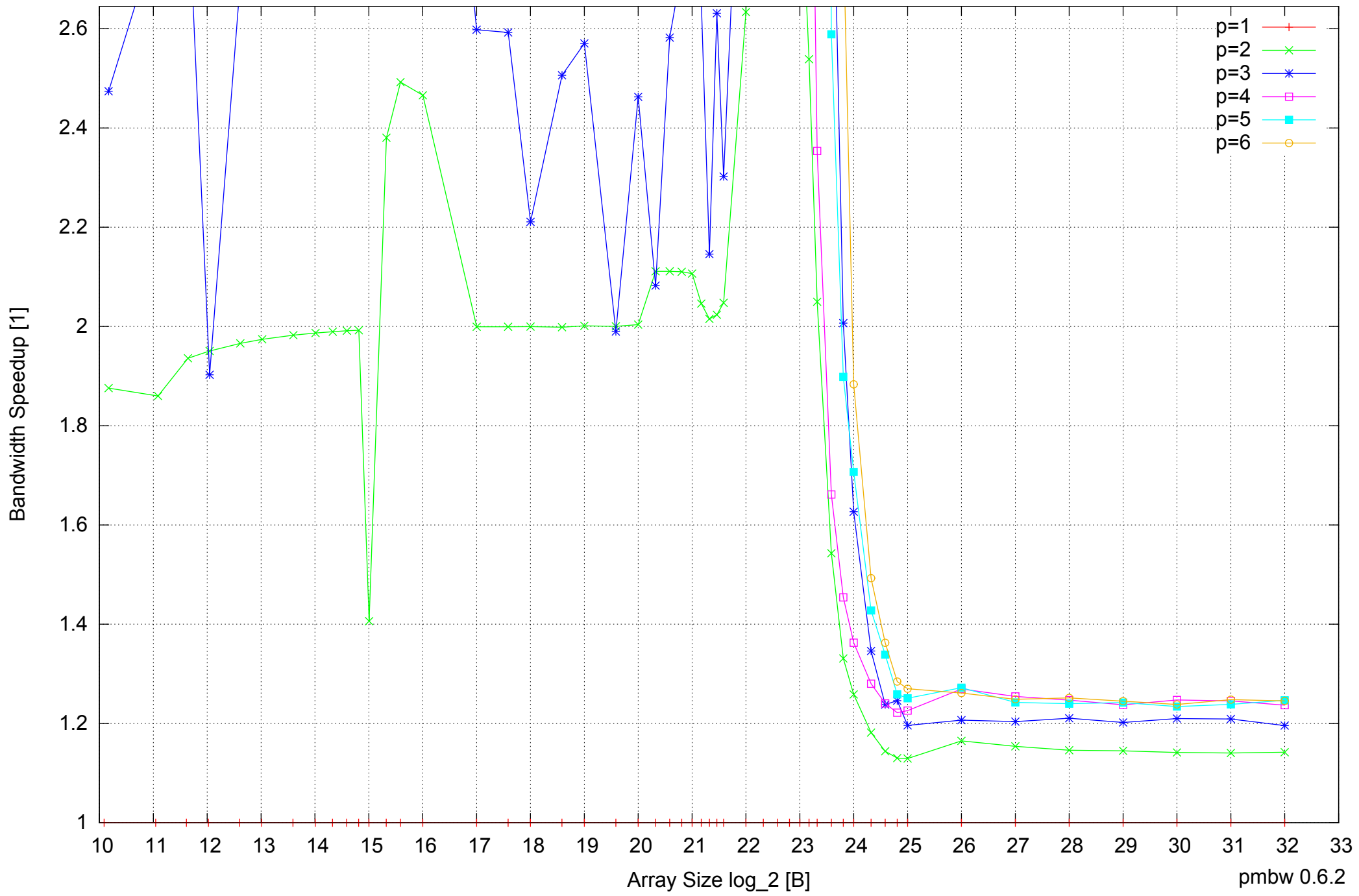
Intel Core 2 Quad Q6600 8GB - Speedup of Parallel Memory Bandwidth (enlarged) - ScanWrite32PtrSimpleLoop
