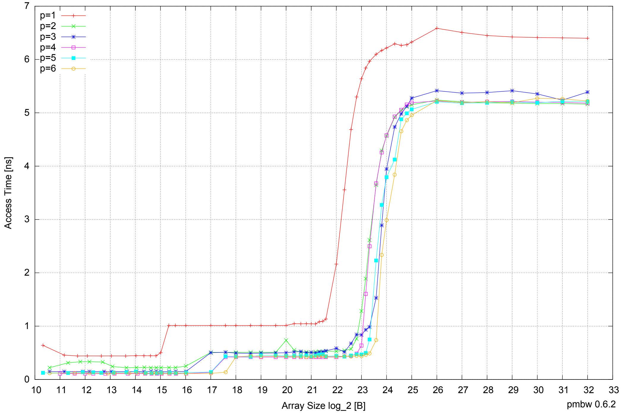
Intel Core 2 Quad Q6600 8GB - Parallel Memory Access Time - ScanWrite128PtrUnrollLoop
