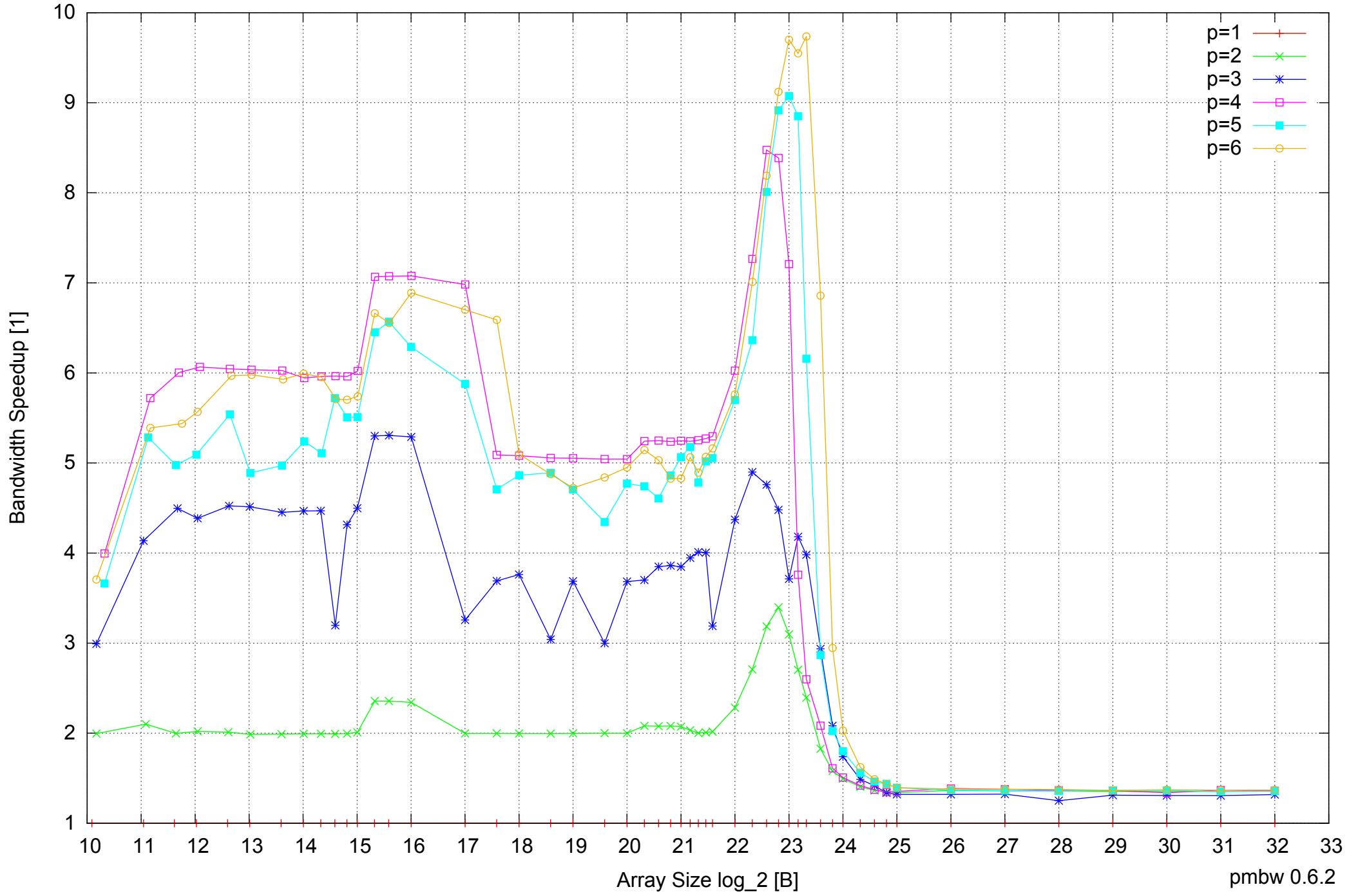
Intel Core 2 Quad Q6600 8GB - Speedup of Parallel Memory Bandwidth - ScanWrite32PtrUnrollLoop
