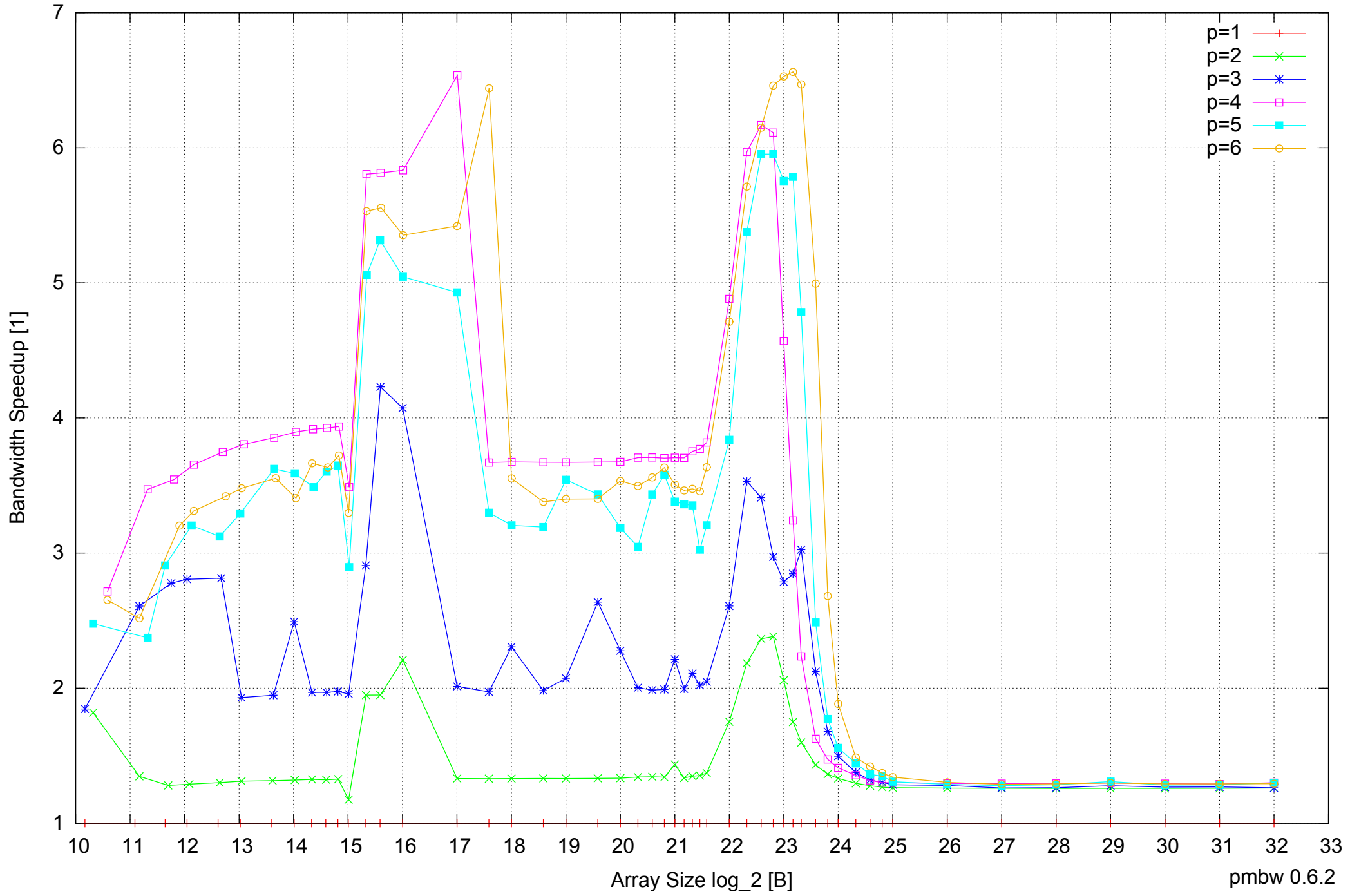
Intel Core 2 Quad Q6600 8GB - Speedup of Parallel Memory Bandwidth - ScanRead64PtrSimpleLoop
