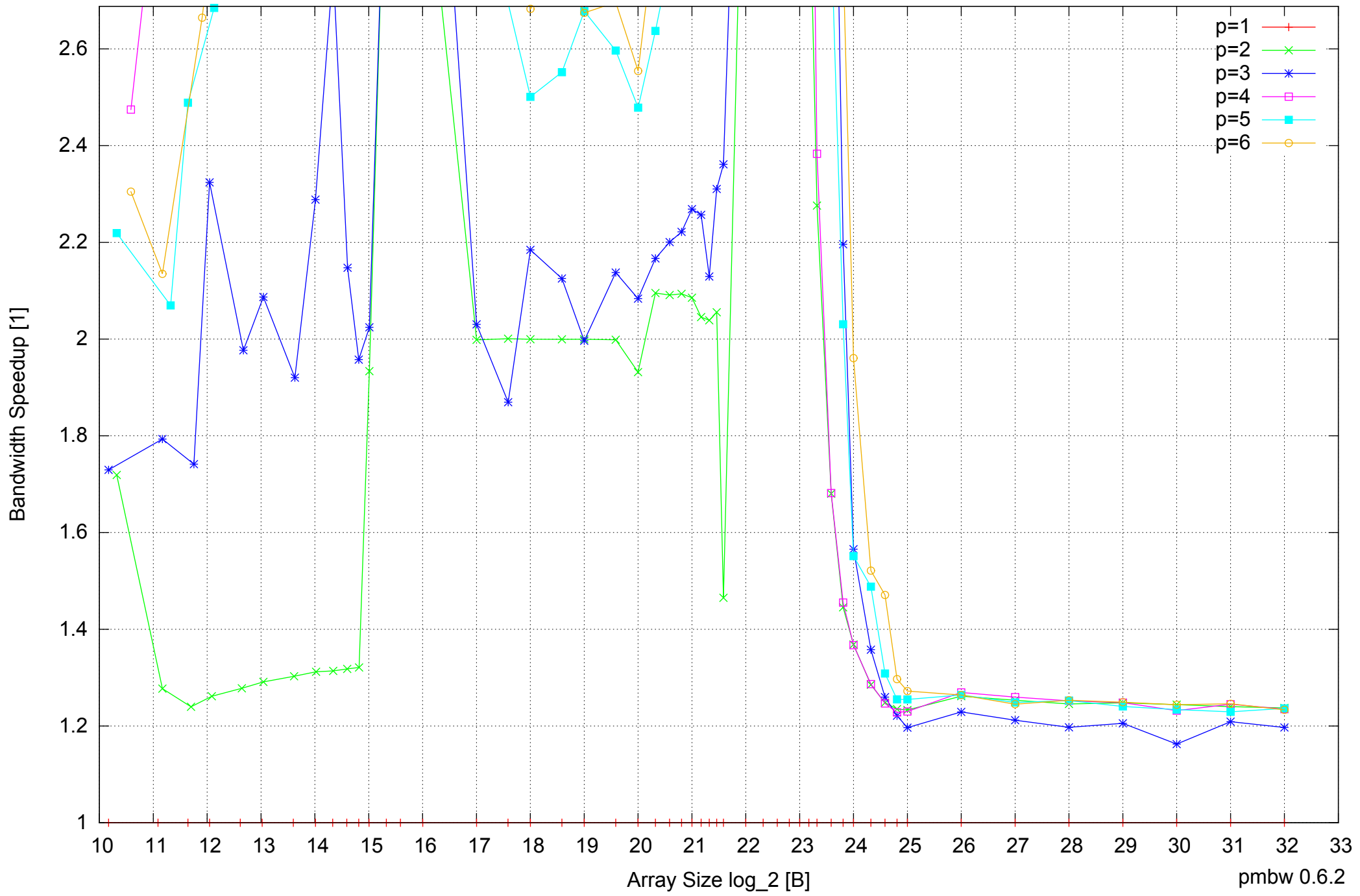
Intel Core 2 Quad Q6600 8GB - Speedup of Parallel Memory Bandwidth (enlarged) - ScanWrite64PtrSimpleLoop
