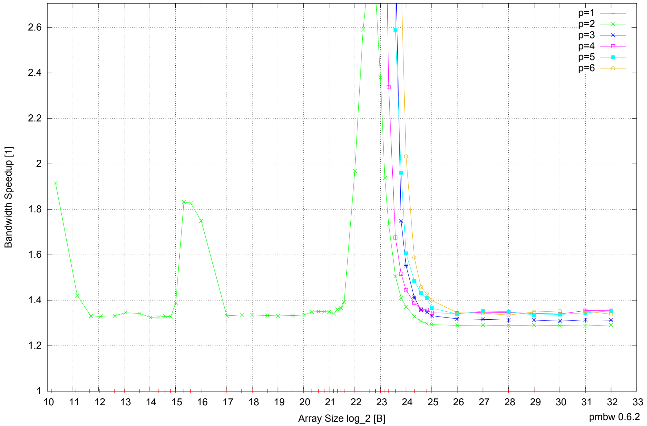
Intel Core 2 Quad Q6600 8GB - Speedup of Parallel Memory Bandwidth (enlarged) - ScanRead64PtrUnrollLoop
