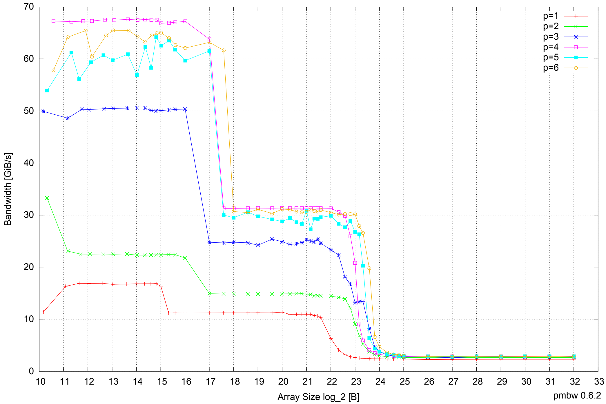
Intel Core 2 Quad Q6600 8GB - Parallel Memory Bandwidth - ScanWrite64IndexUnrollLoop
