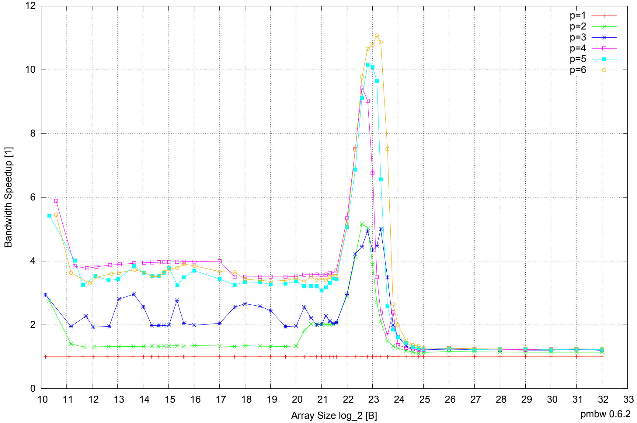
Intel Core 2 Quad Q6600 8GB - Speedup of Parallel Memory Bandwidth - ScanWrite64IndexSimpleLoop
