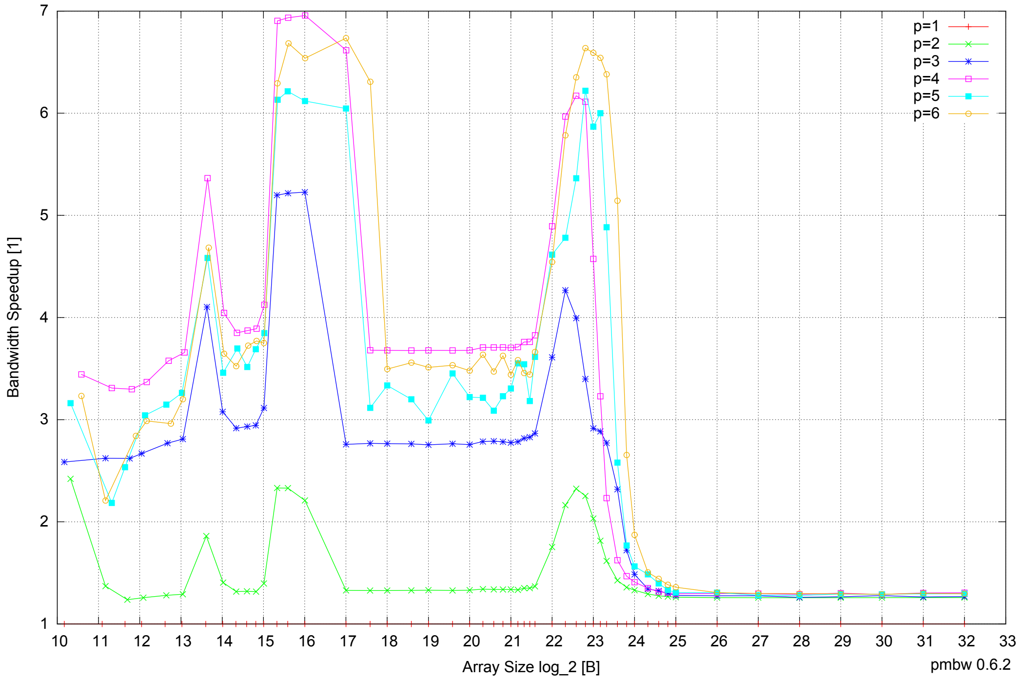
Intel Core 2 Quad Q6600 8GB - Speedup of Parallel Memory Bandwidth - ScanRead64IndexSimpleLoop
