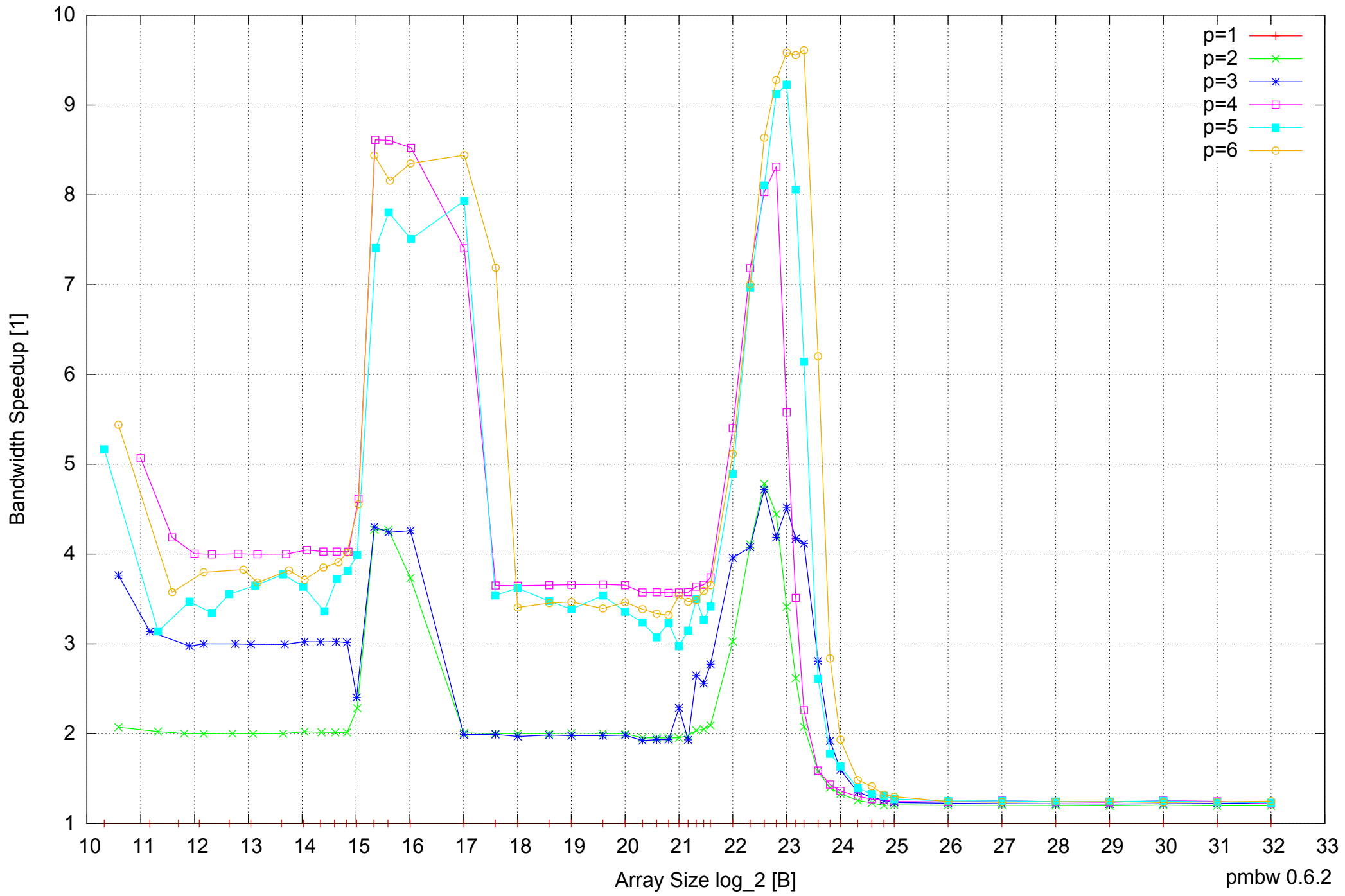
Intel Core 2 Quad Q6600 8GB - Speedup of Parallel Memory Bandwidth - ScanRead128PtrUnrollLoop
