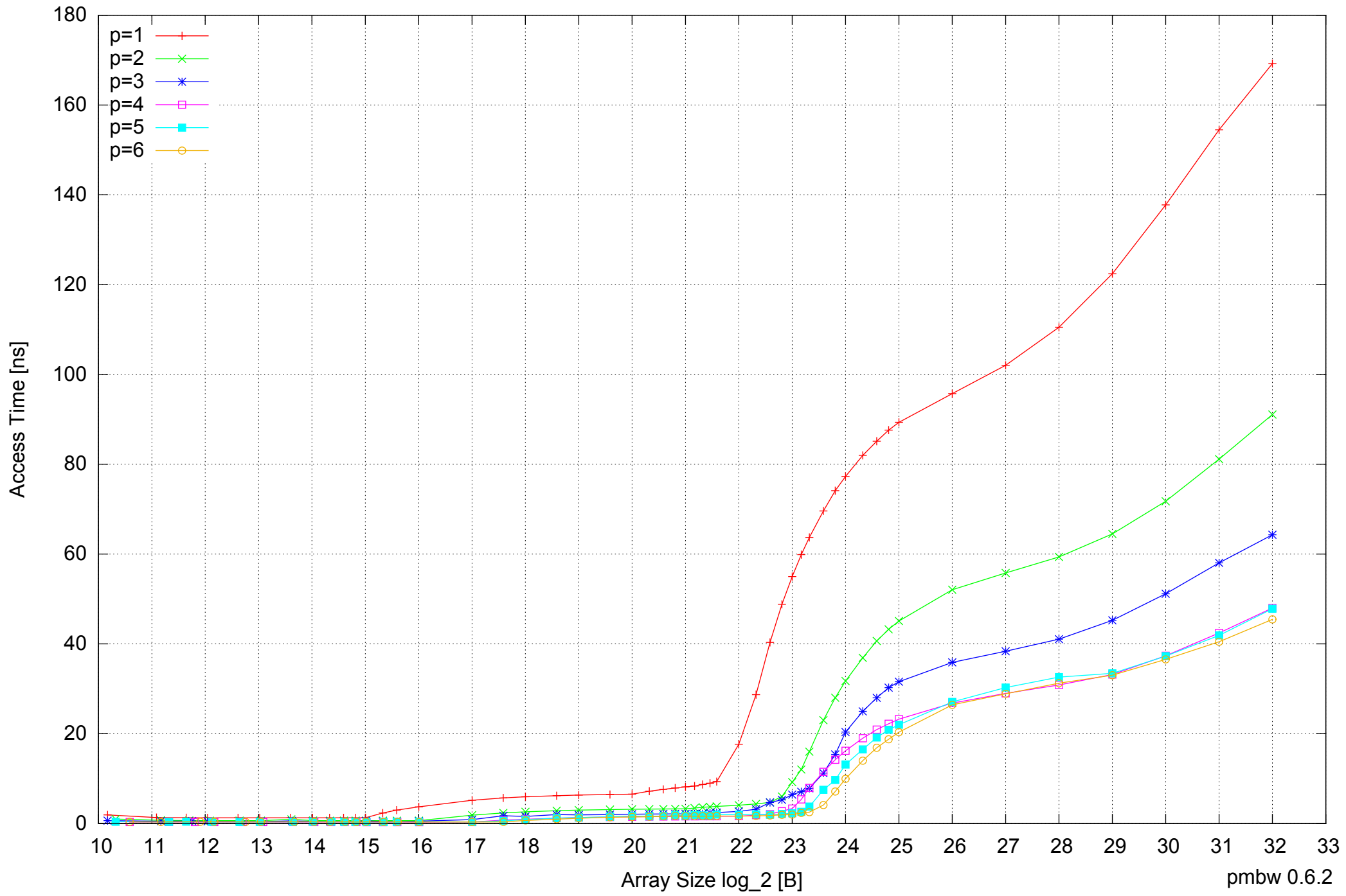
Intel Core 2 Quad Q6600 8GB - Parallel Memory Access Time - PermRead64SimpleLoop
