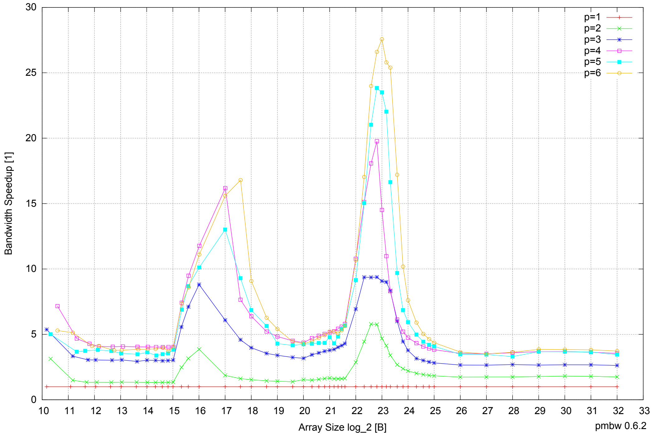
Intel Core 2 Quad Q6600 8GB - Speedup of Parallel Memory Bandwidth - PermRead64UnrollLoop
