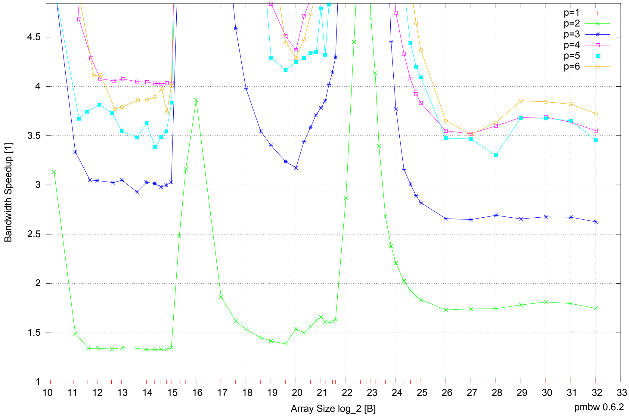
Intel Core 2 Quad Q6600 8GB - Speedup of Parallel Memory Bandwidth (enlarged) - PermRead64UnrollLoop
