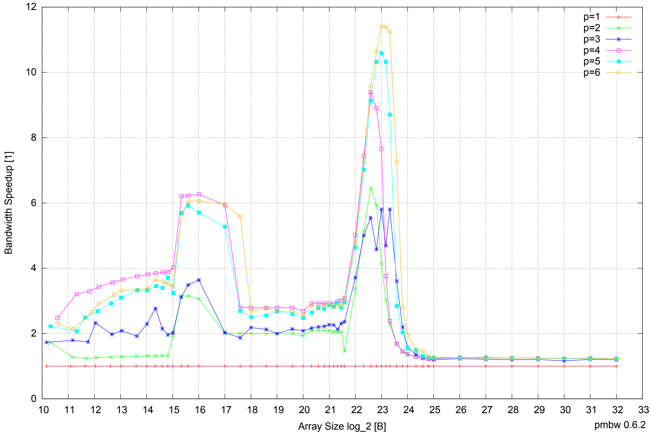
Intel Core 2 Quad Q6600 8GB - Speedup of Parallel Memory Bandwidth - ScanWrite64PtrSimpleLoop
