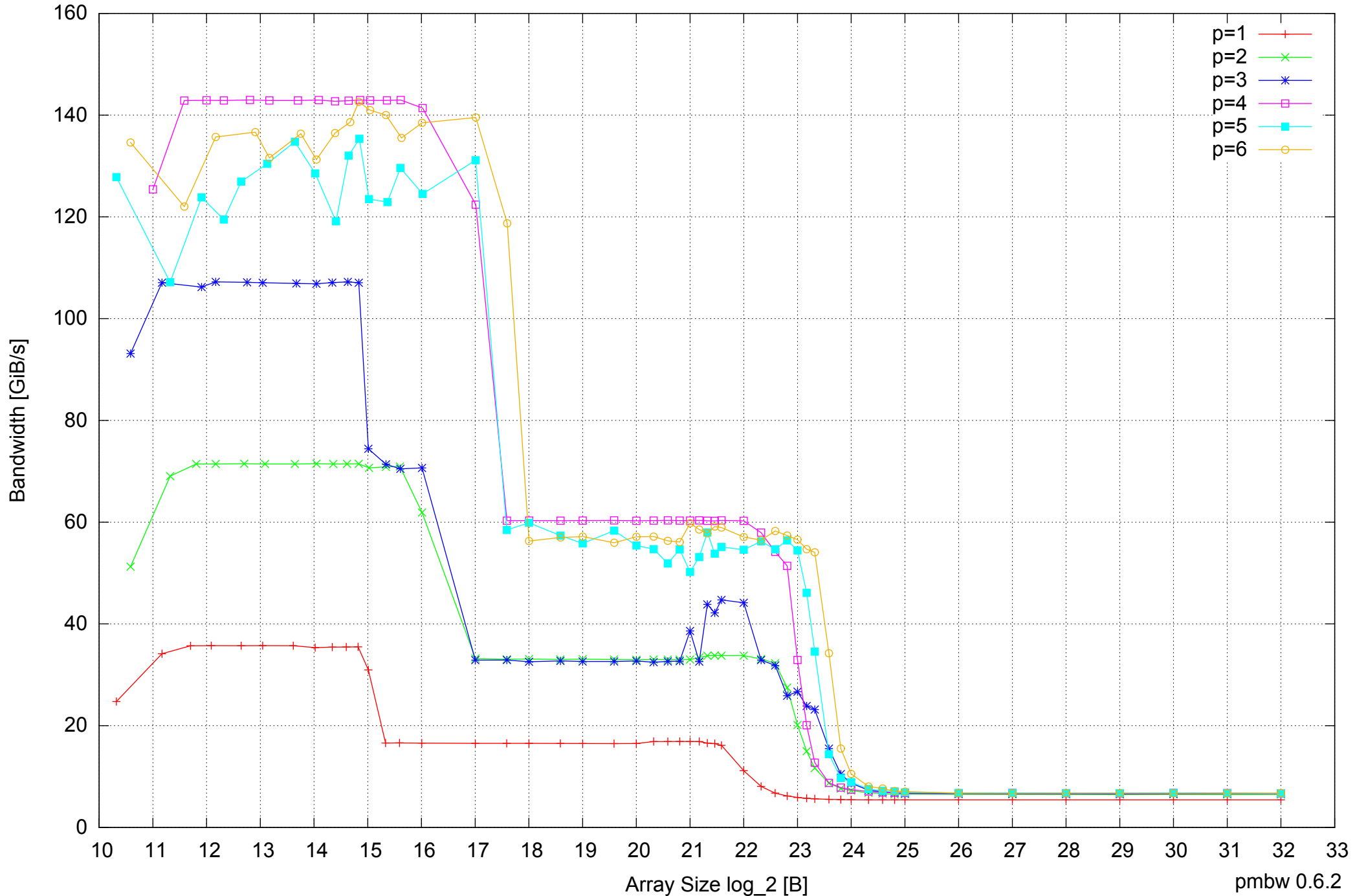
Intel Core 2 Quad Q6600 8GB - Parallel Memory Bandwidth - ScanRead128PtrUnrollLoop
