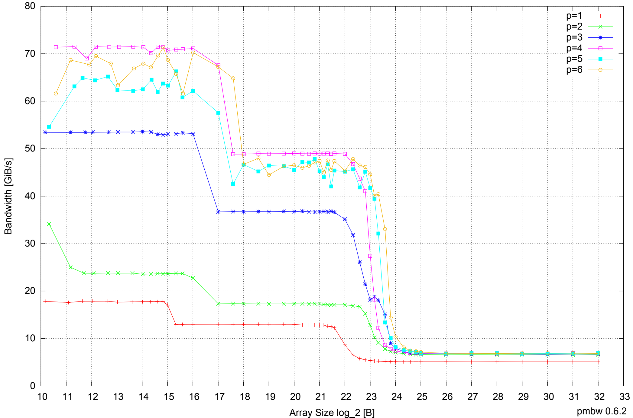
Intel Core 2 Quad Q6600 8GB - Parallel Memory Bandwidth - ScanRead64PtrUnrollLoop
