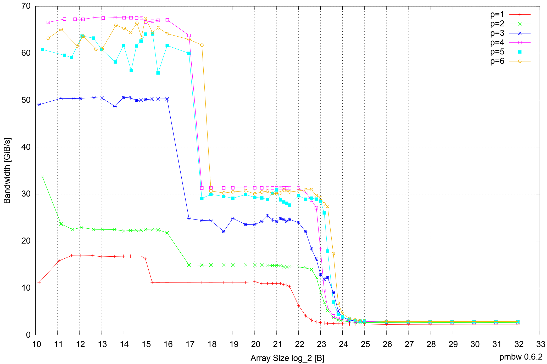
Intel Core 2 Quad Q6600 8GB - Parallel Memory Bandwidth - ScanWrite64PtrUnrollLoop
