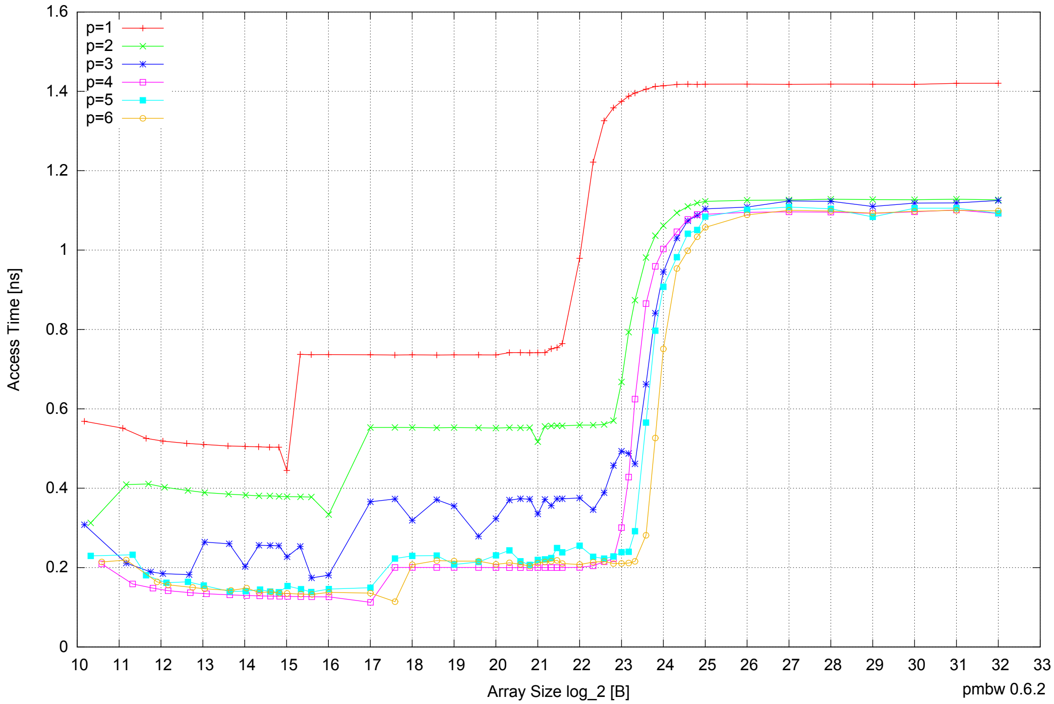
Intel Core 2 Quad Q6600 8GB - Parallel Memory Access Time - ScanRead64PtrSimpleLoop
