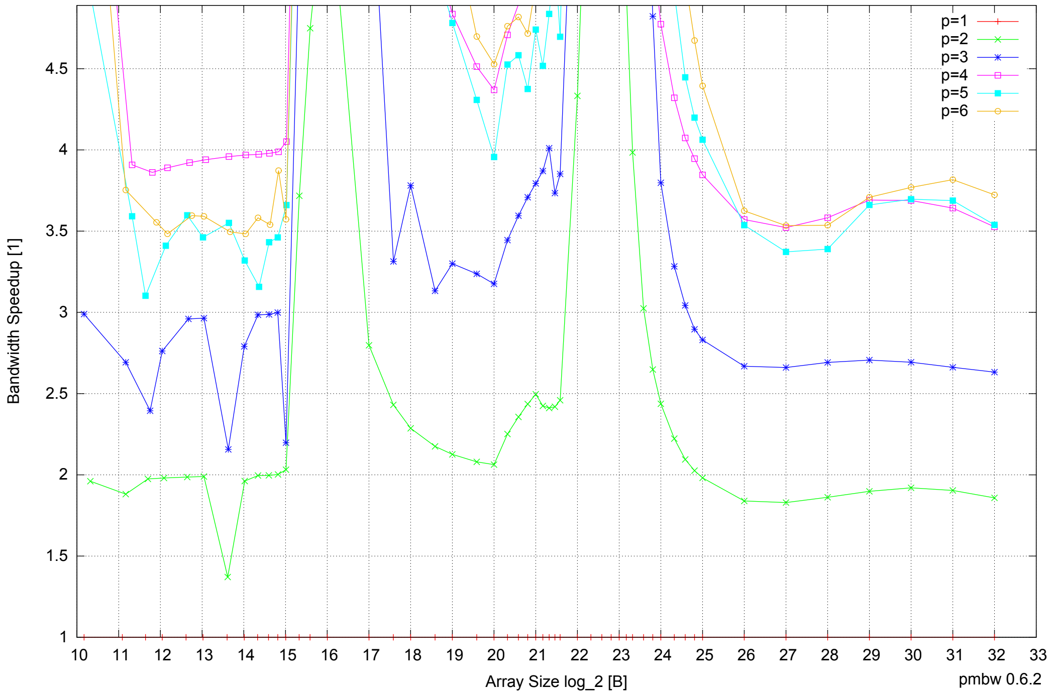
Intel Core 2 Quad Q6600 8GB - Speedup of Parallel Memory Bandwidth (enlarged) - PermRead64SimpleLoop
