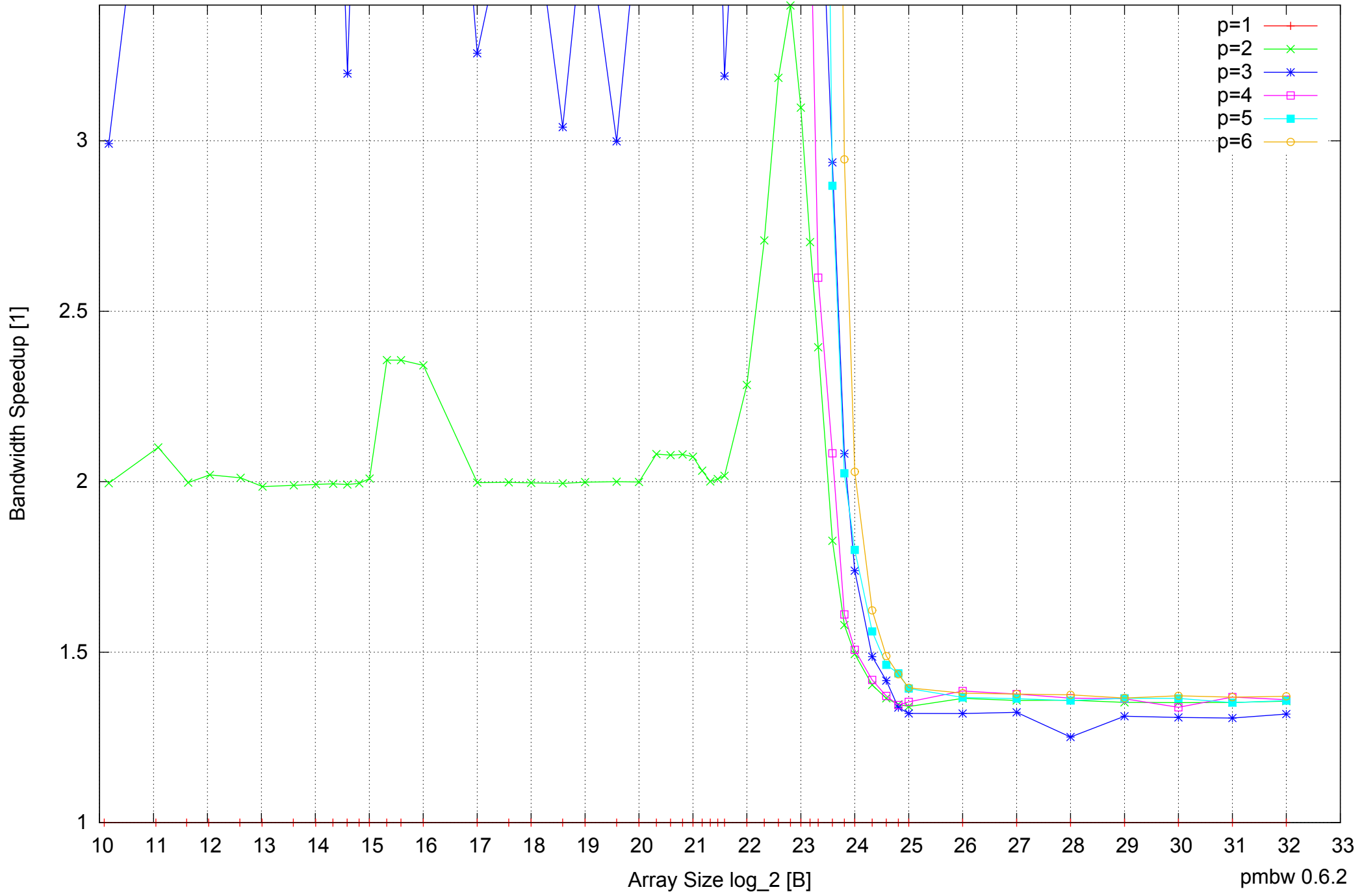
Intel Core 2 Quad Q6600 8GB - Speedup of Parallel Memory Bandwidth (enlarged) - ScanWrite32PtrUnrollLoop
