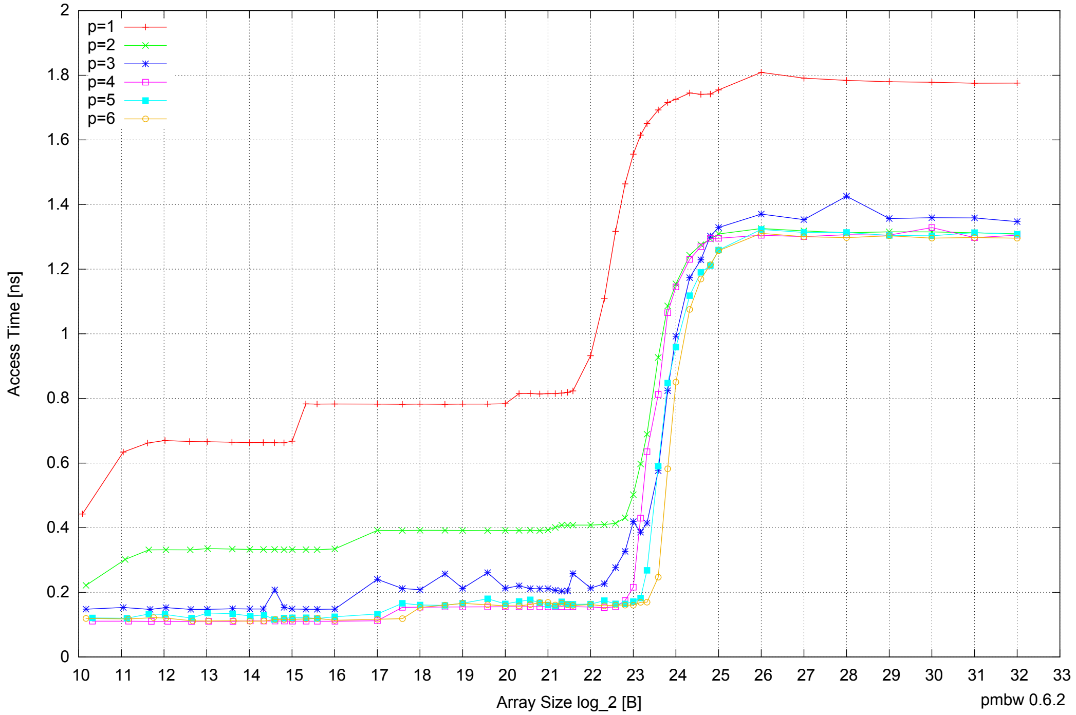
Intel Core 2 Quad Q6600 8GB - Parallel Memory Access Time - ScanWrite32PtrUnrollLoop
