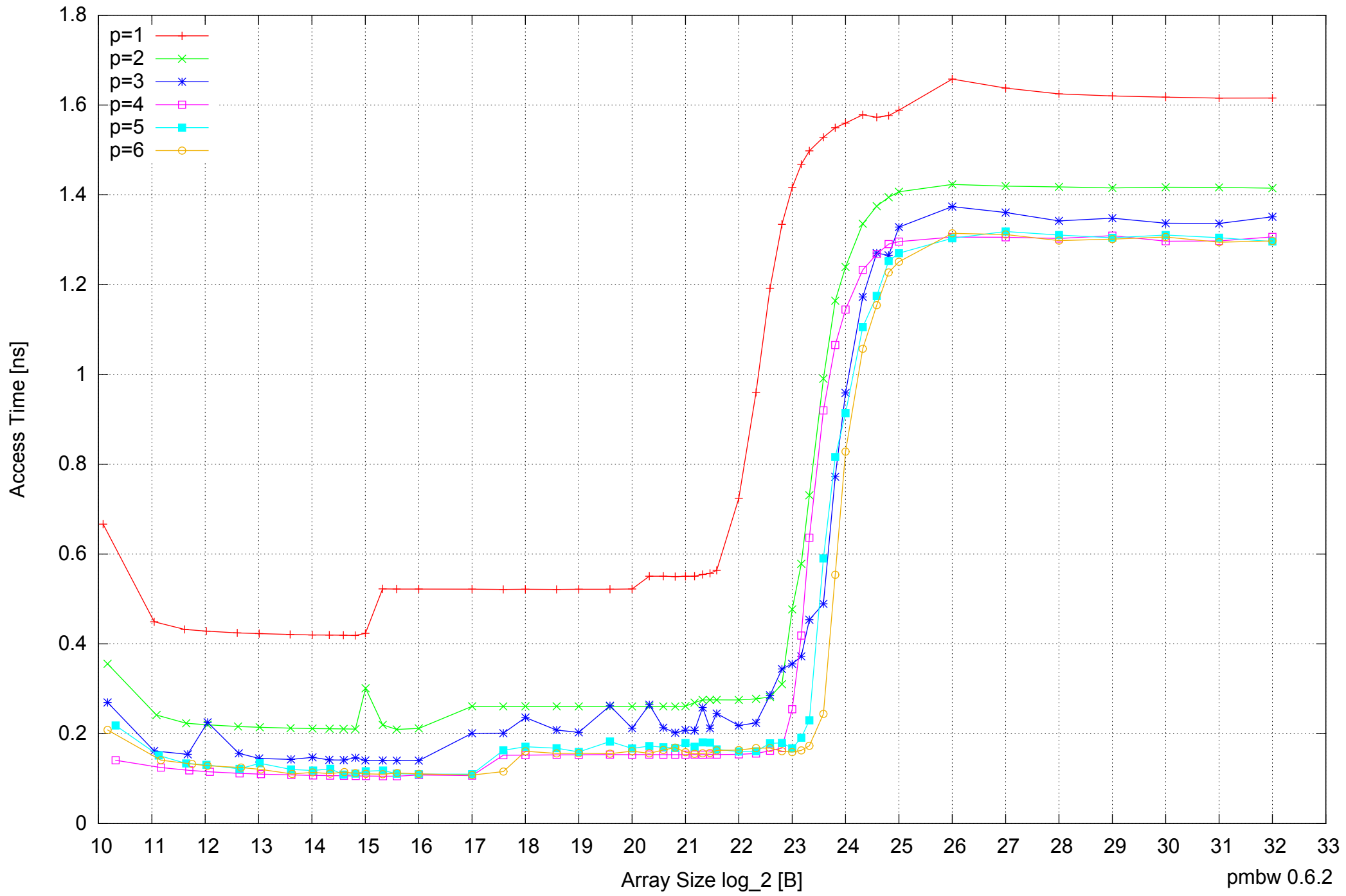
Intel Core 2 Quad Q6600 8GB - Parallel Memory Access Time - ScanWrite32PtrSimpleLoop
