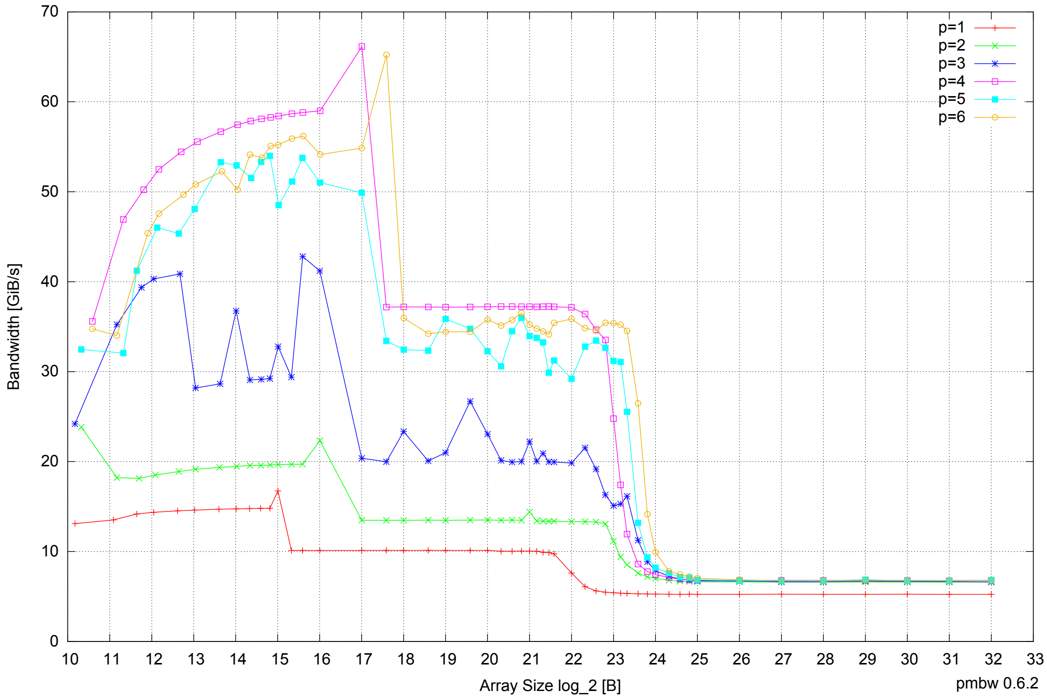
Intel Core 2 Quad Q6600 8GB - Parallel Memory Bandwidth - ScanRead64PtrSimpleLoop
