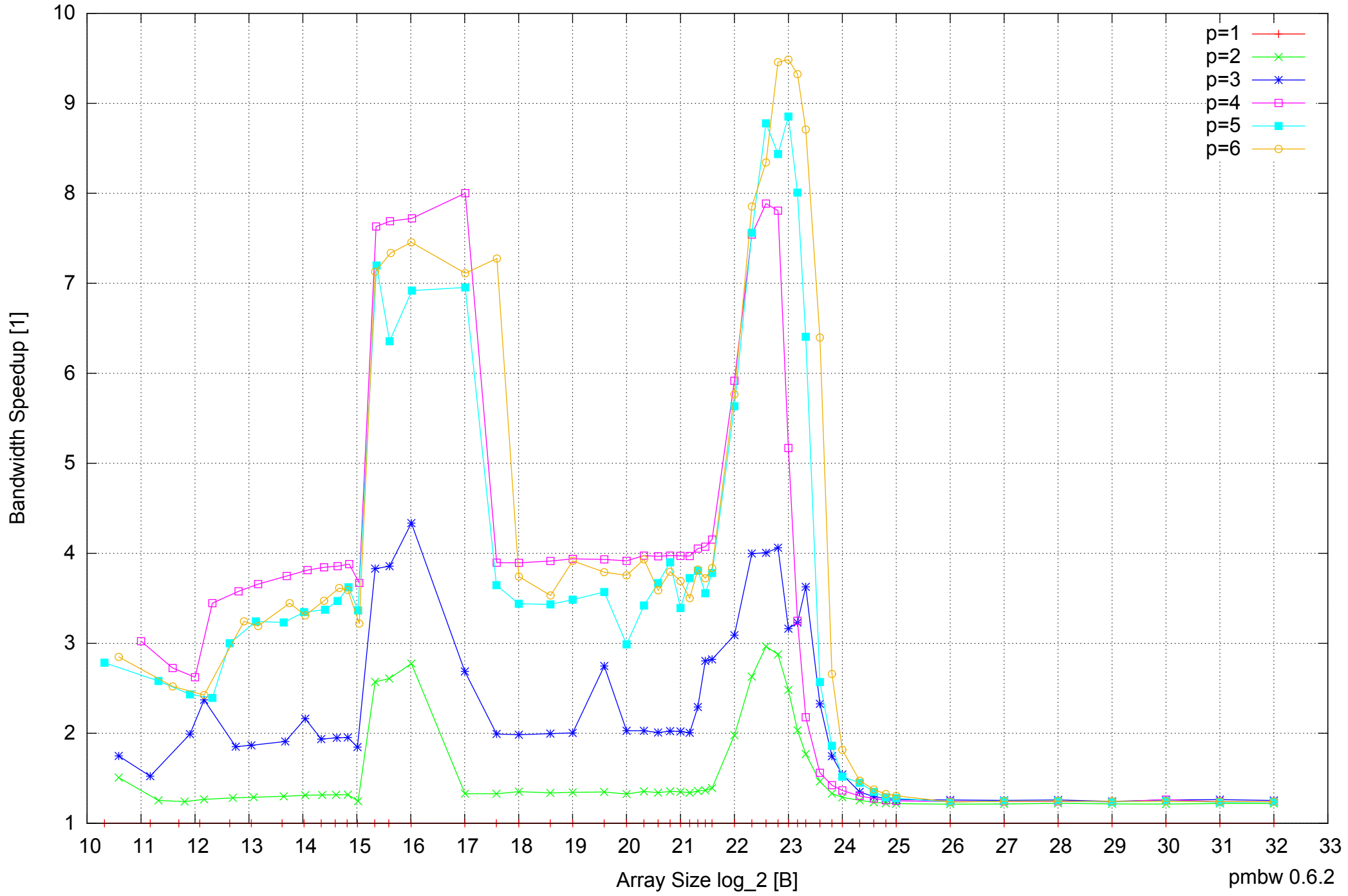
Intel Core 2 Quad Q6600 8GB - Speedup of Parallel Memory Bandwidth - ScanRead128PtrSimpleLoop
