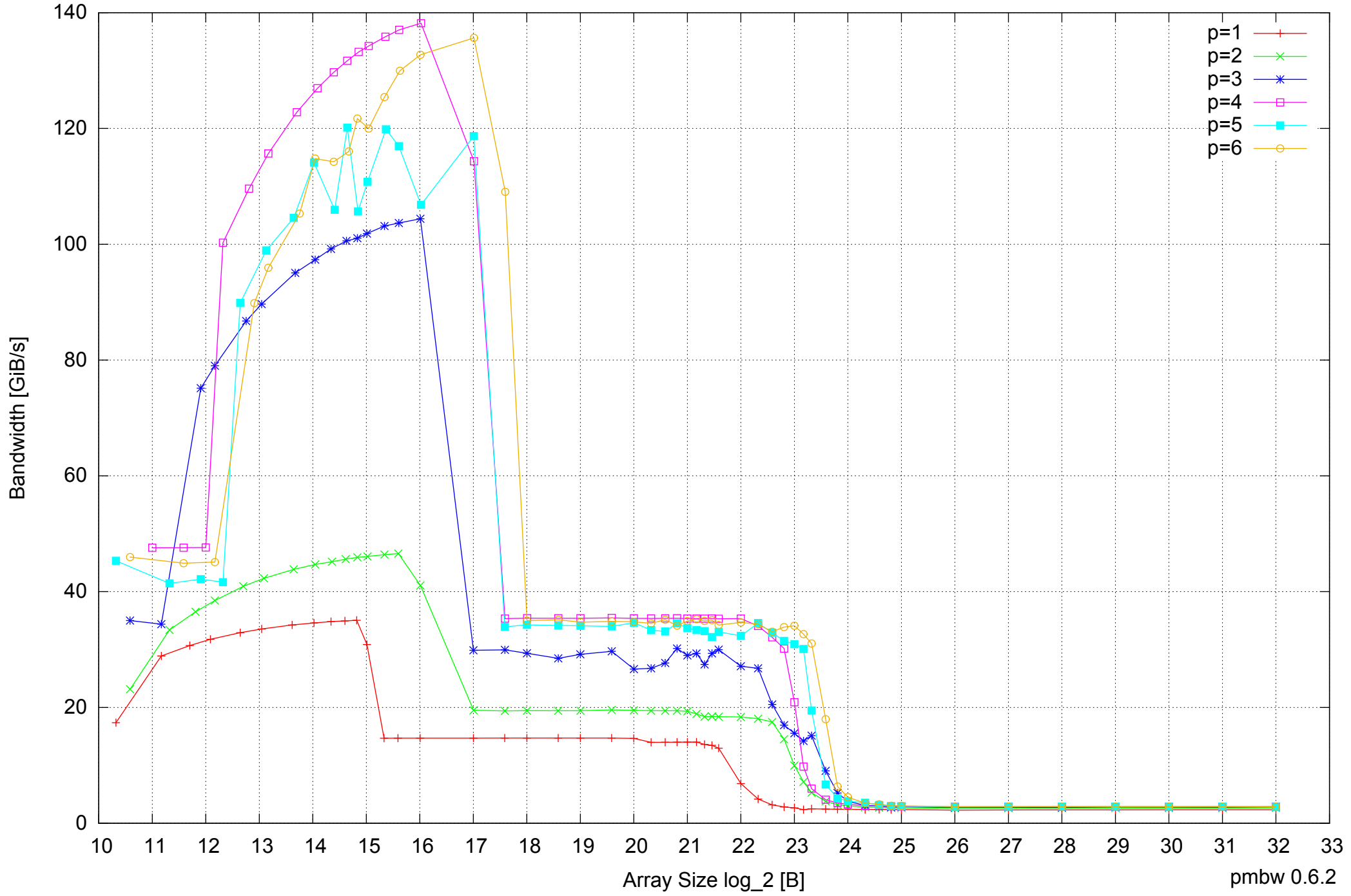
Intel Core 2 Quad Q6600 8GB - Parallel Memory Bandwidth - ScanWrite128PtrSimpleLoop
