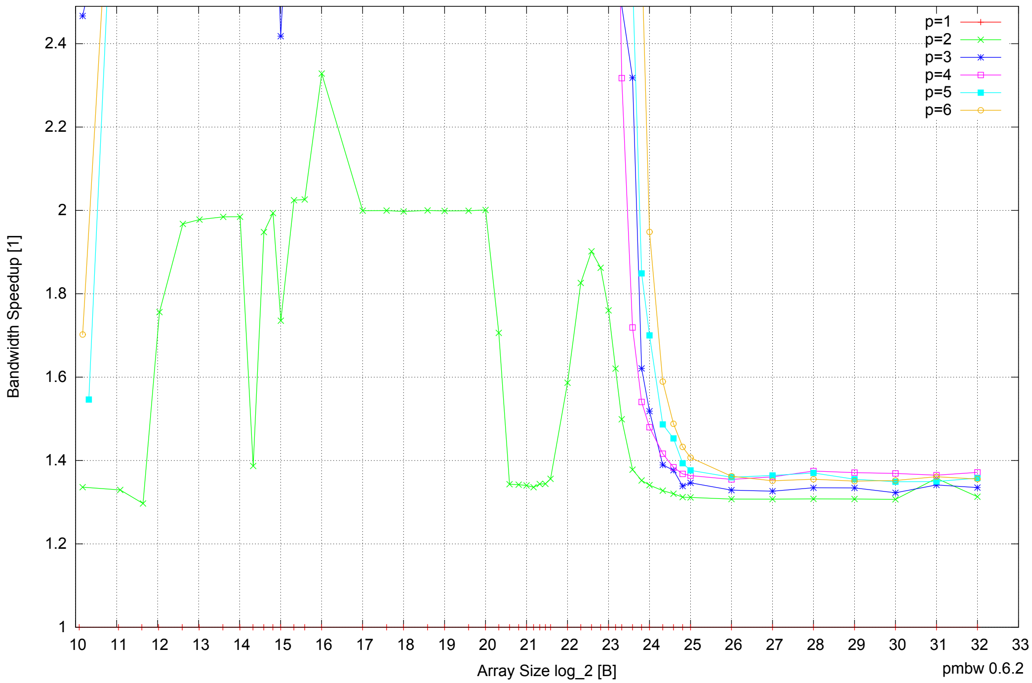
Intel Core 2 Quad Q6600 8GB - Speedup of Parallel Memory Bandwidth (enlarged) - ScanRead32PtrSimpleLoop
