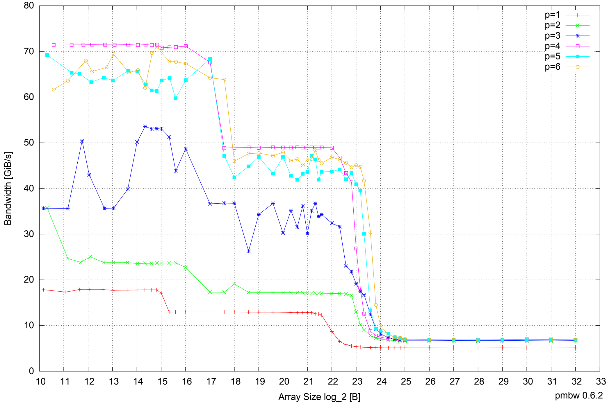
Intel Core 2 Quad Q6600 8GB - Parallel Memory Bandwidth - ScanRead64IndexUnrollLoop
