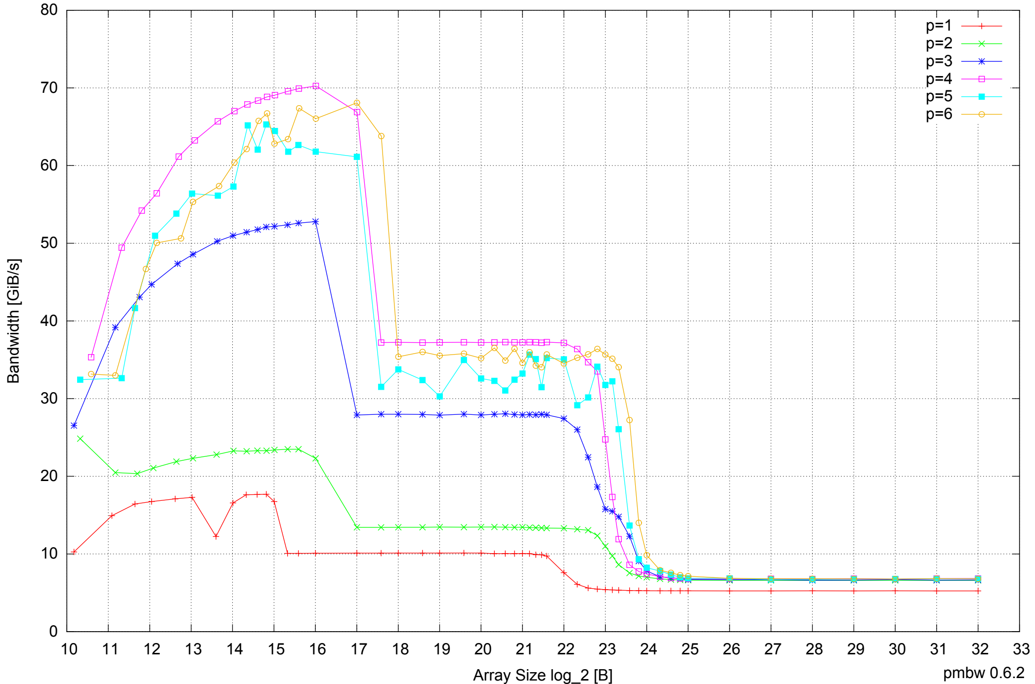
Intel Core 2 Quad Q6600 8GB - Parallel Memory Bandwidth - ScanRead64IndexSimpleLoop
