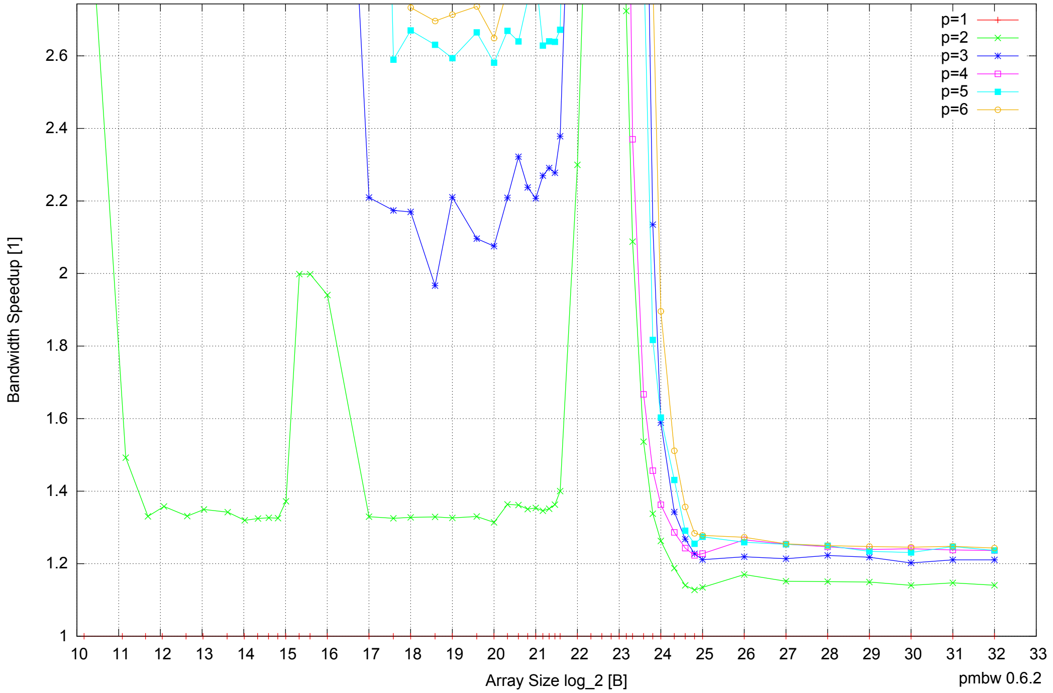
Intel Core 2 Quad Q6600 8GB - Speedup of Parallel Memory Bandwidth (enlarged) - ScanWrite64PtrUnrollLoop
