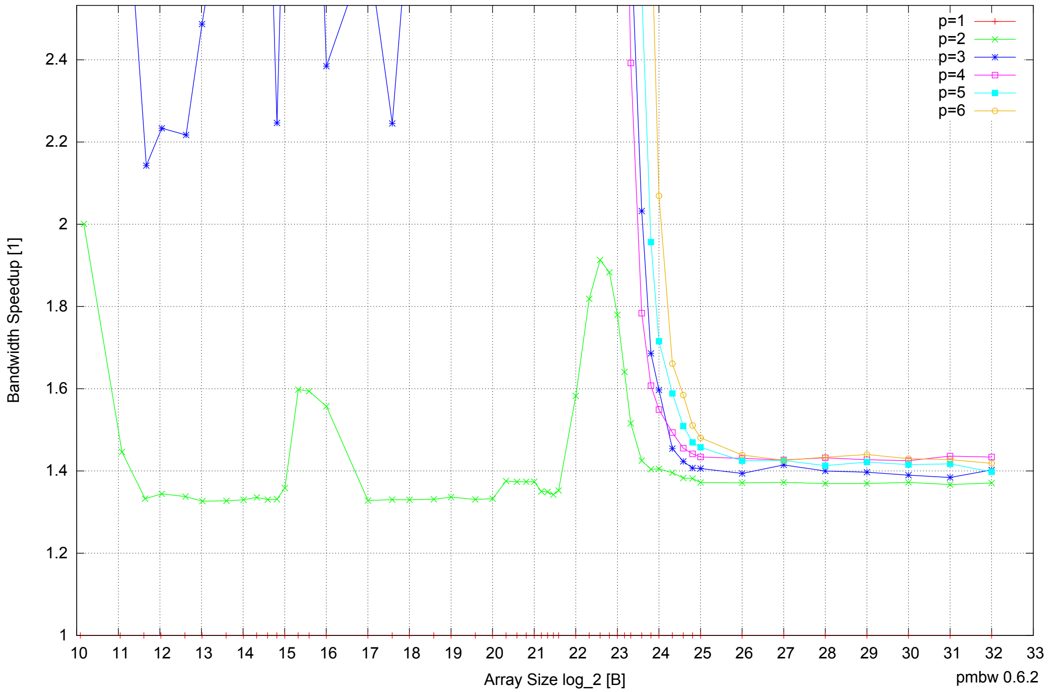
Intel Core 2 Quad Q6600 8GB - Speedup of Parallel Memory Bandwidth (enlarged) - ScanRead32PtrUnrollLoop
