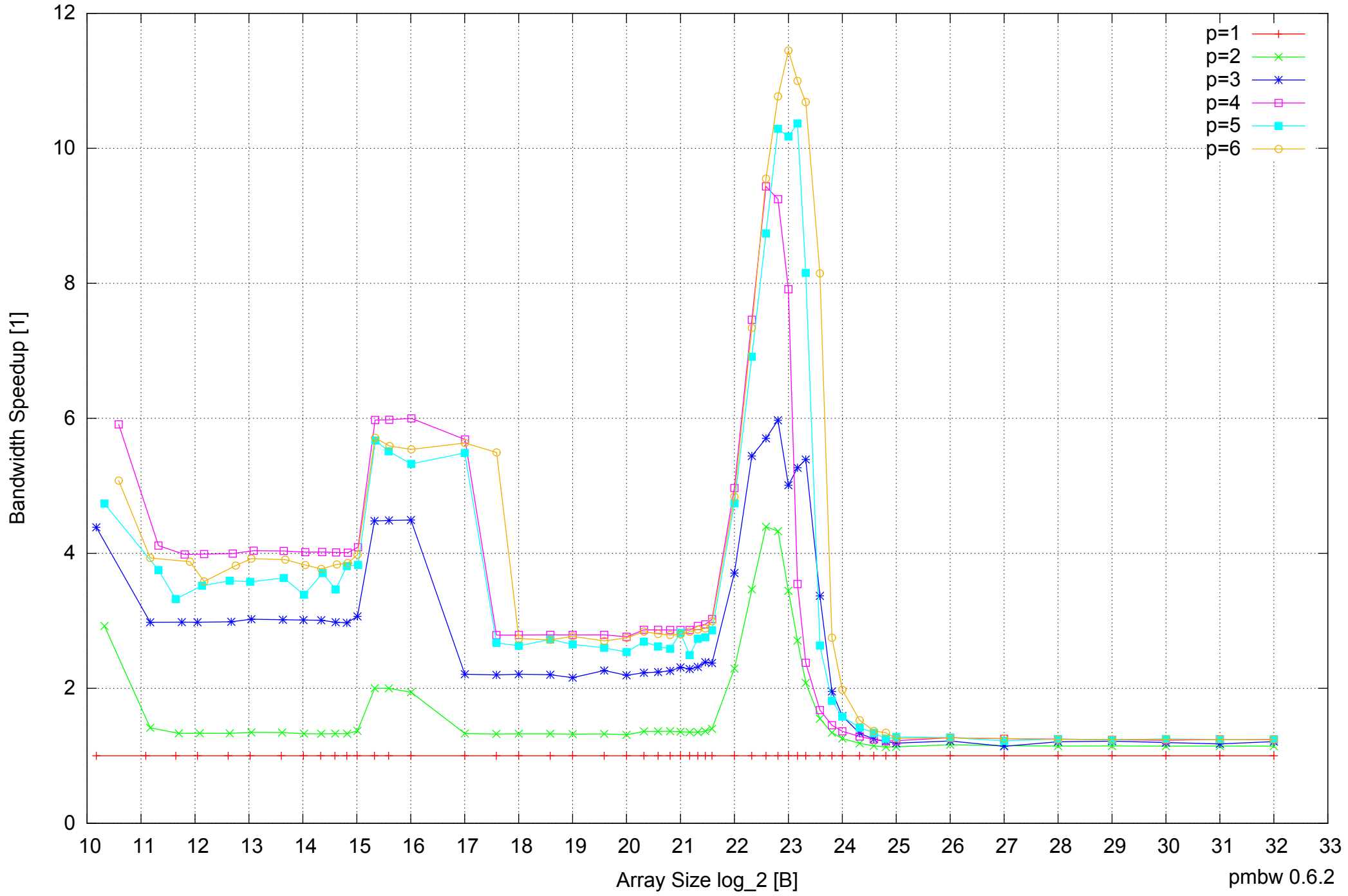
Intel Core 2 Quad Q6600 8GB - Speedup of Parallel Memory Bandwidth - ScanWrite64IndexUnrollLoop
