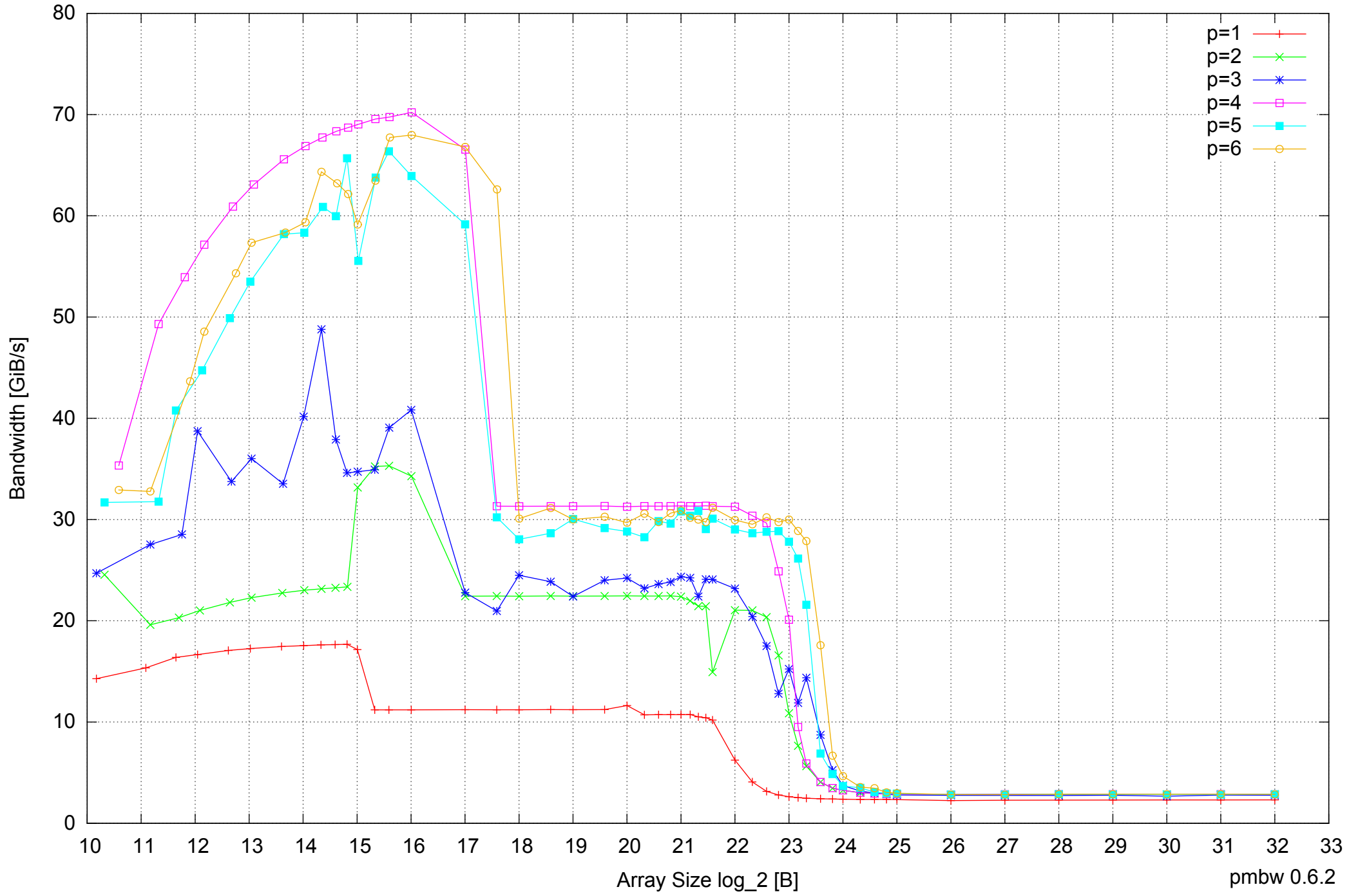
Intel Core 2 Quad Q6600 8GB - Parallel Memory Bandwidth - ScanWrite64PtrSimpleLoop
