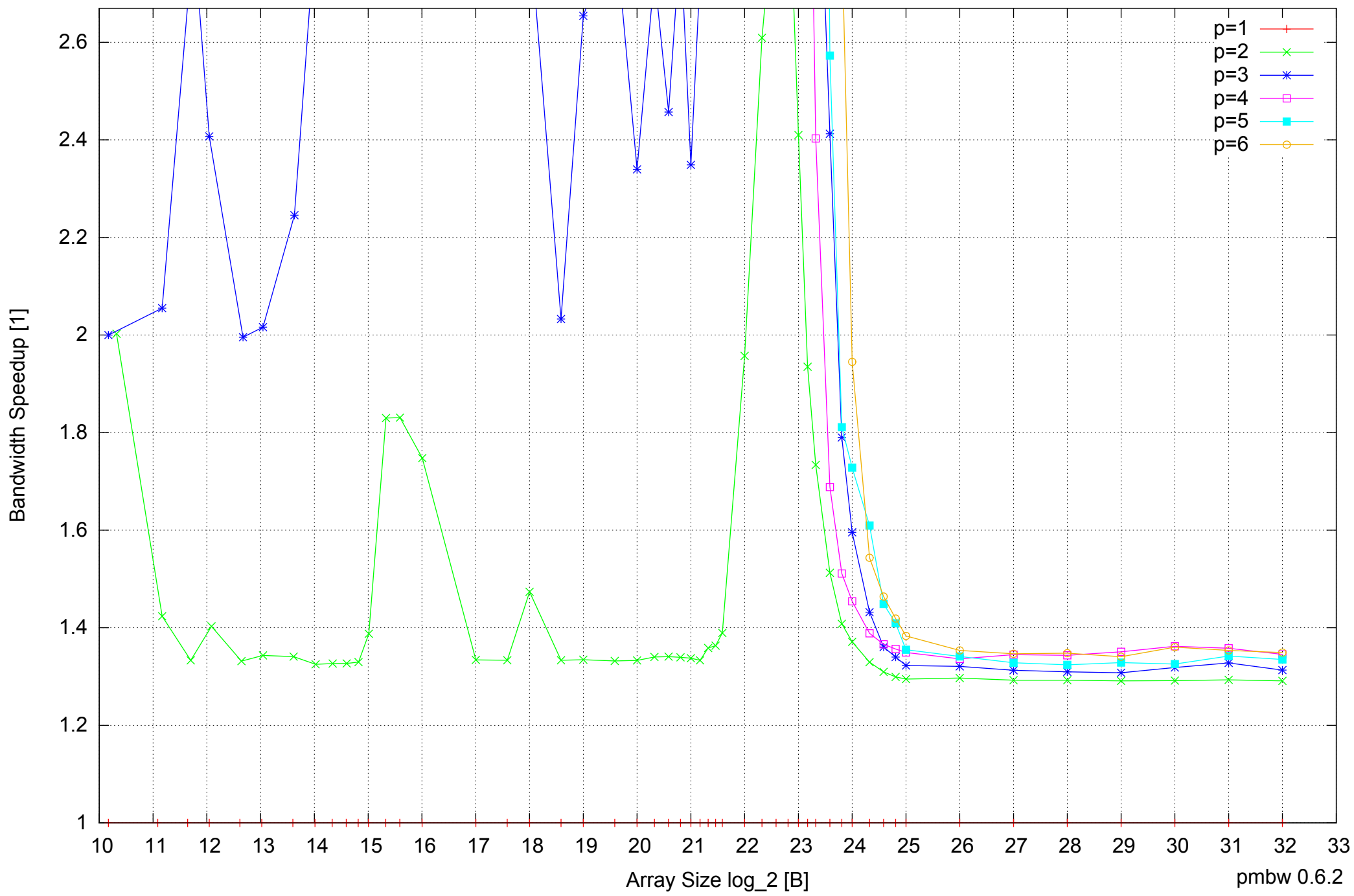
Intel Core 2 Quad Q6600 8GB - Speedup of Parallel Memory Bandwidth (enlarged) - ScanRead64IndexUnrollLoop
