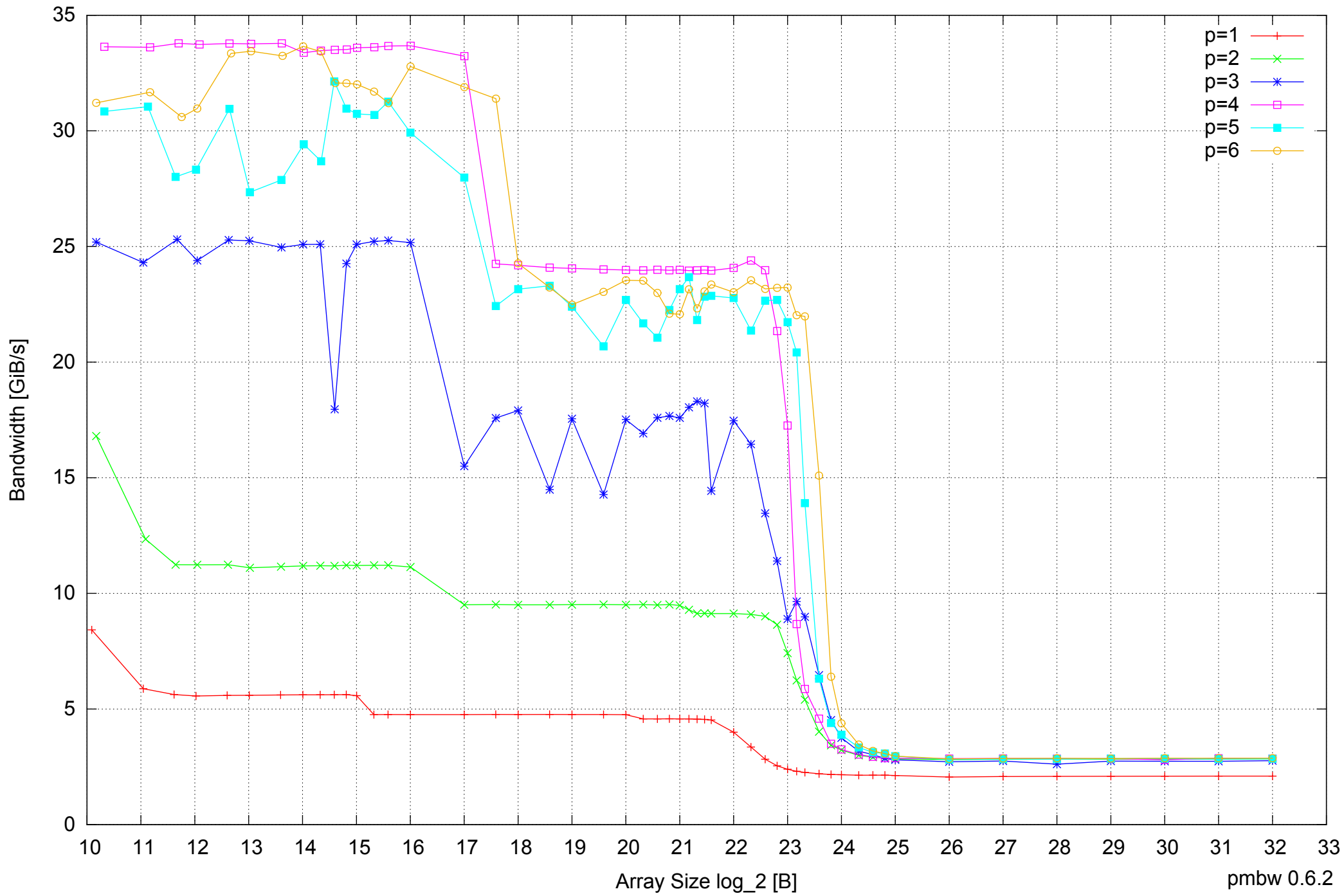
Intel Core 2 Quad Q6600 8GB - Parallel Memory Bandwidth - ScanWrite32PtrUnrollLoop
