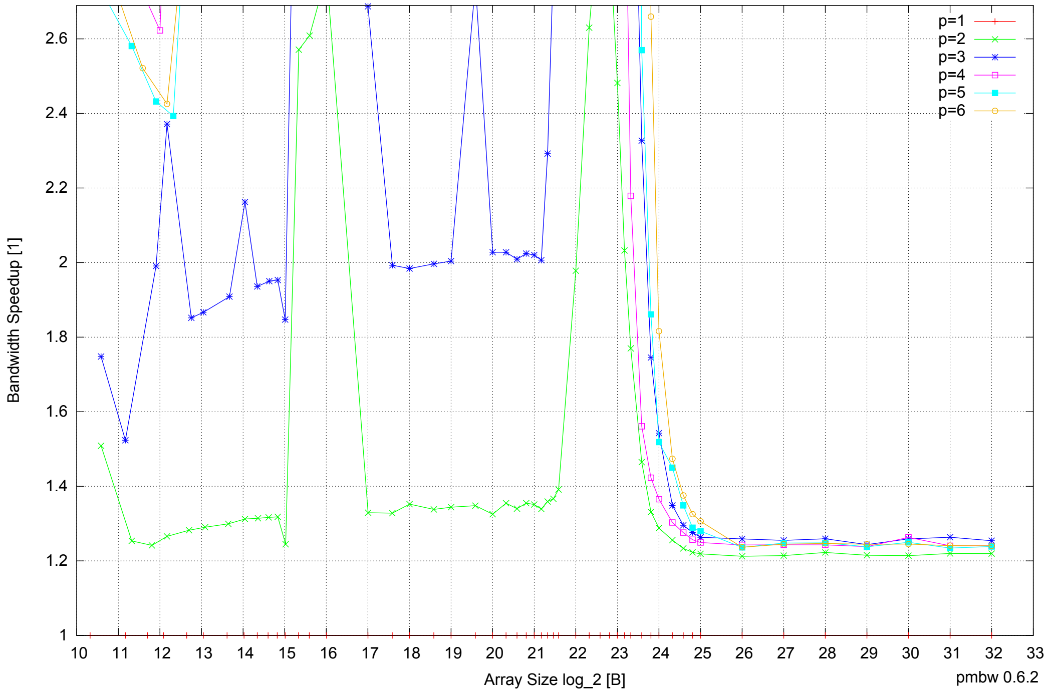
Intel Core 2 Quad Q6600 8GB - Speedup of Parallel Memory Bandwidth (enlarged) - ScanRead128PtrSimpleLoop
