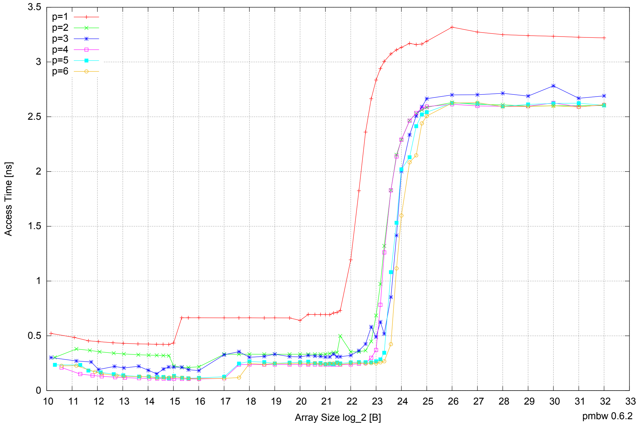
Intel Core 2 Quad Q6600 8GB - Parallel Memory Access Time - ScanWrite64PtrSimpleLoop
