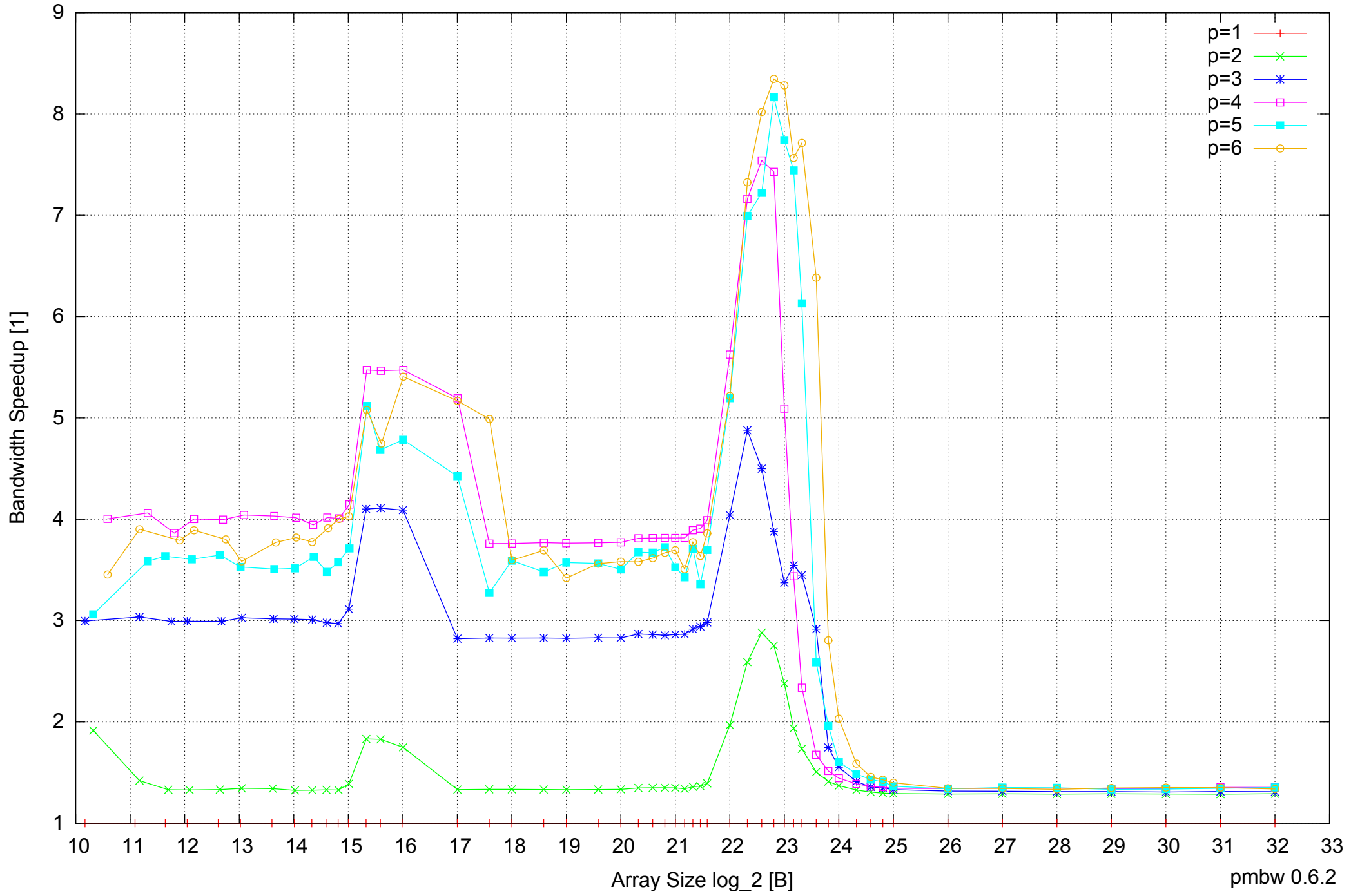
Intel Core 2 Quad Q6600 8GB - Speedup of Parallel Memory Bandwidth - ScanRead64PtrUnrollLoop
