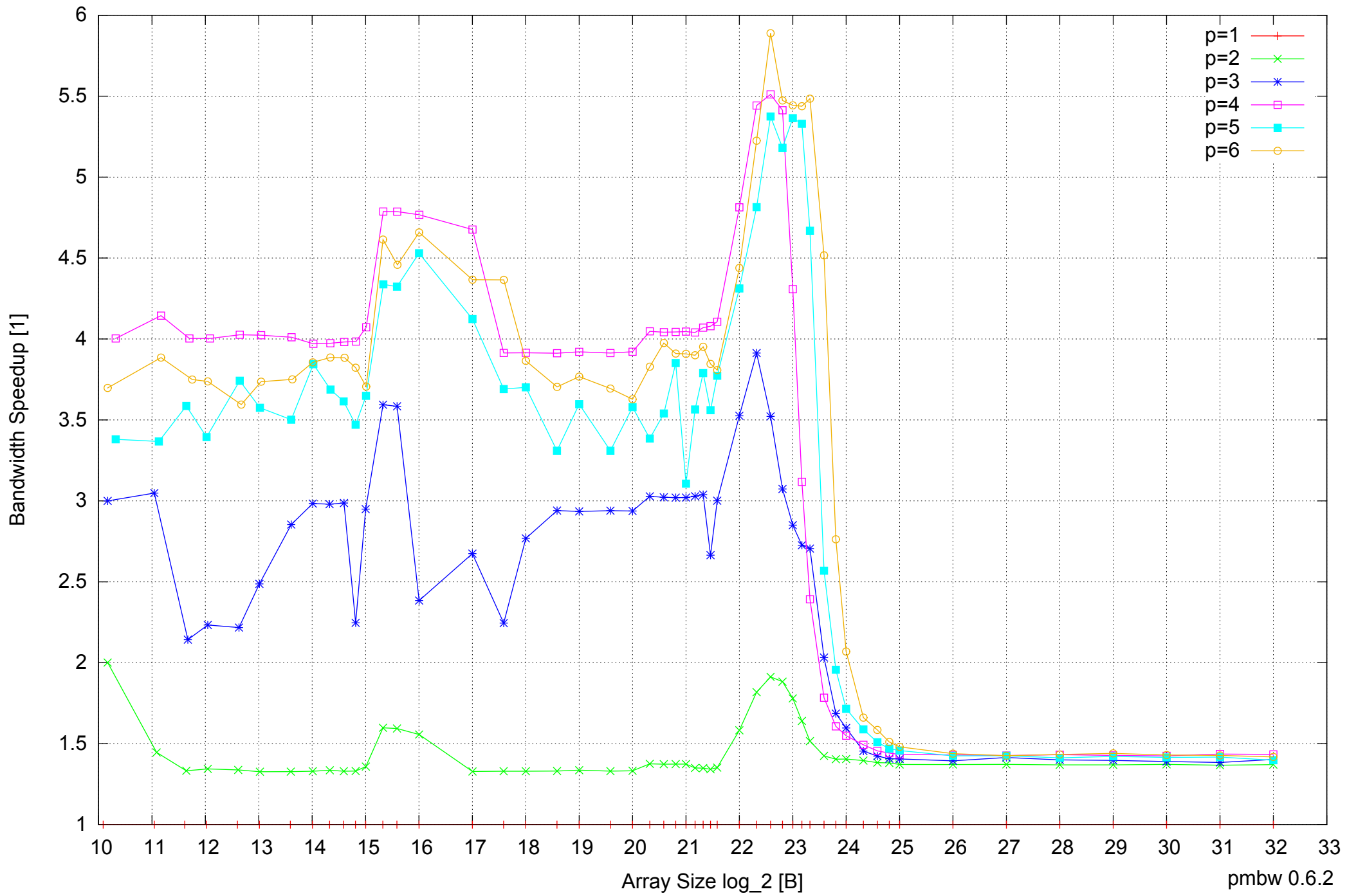
Intel Core 2 Quad Q6600 8GB - Speedup of Parallel Memory Bandwidth - ScanRead32PtrUnrollLoop
