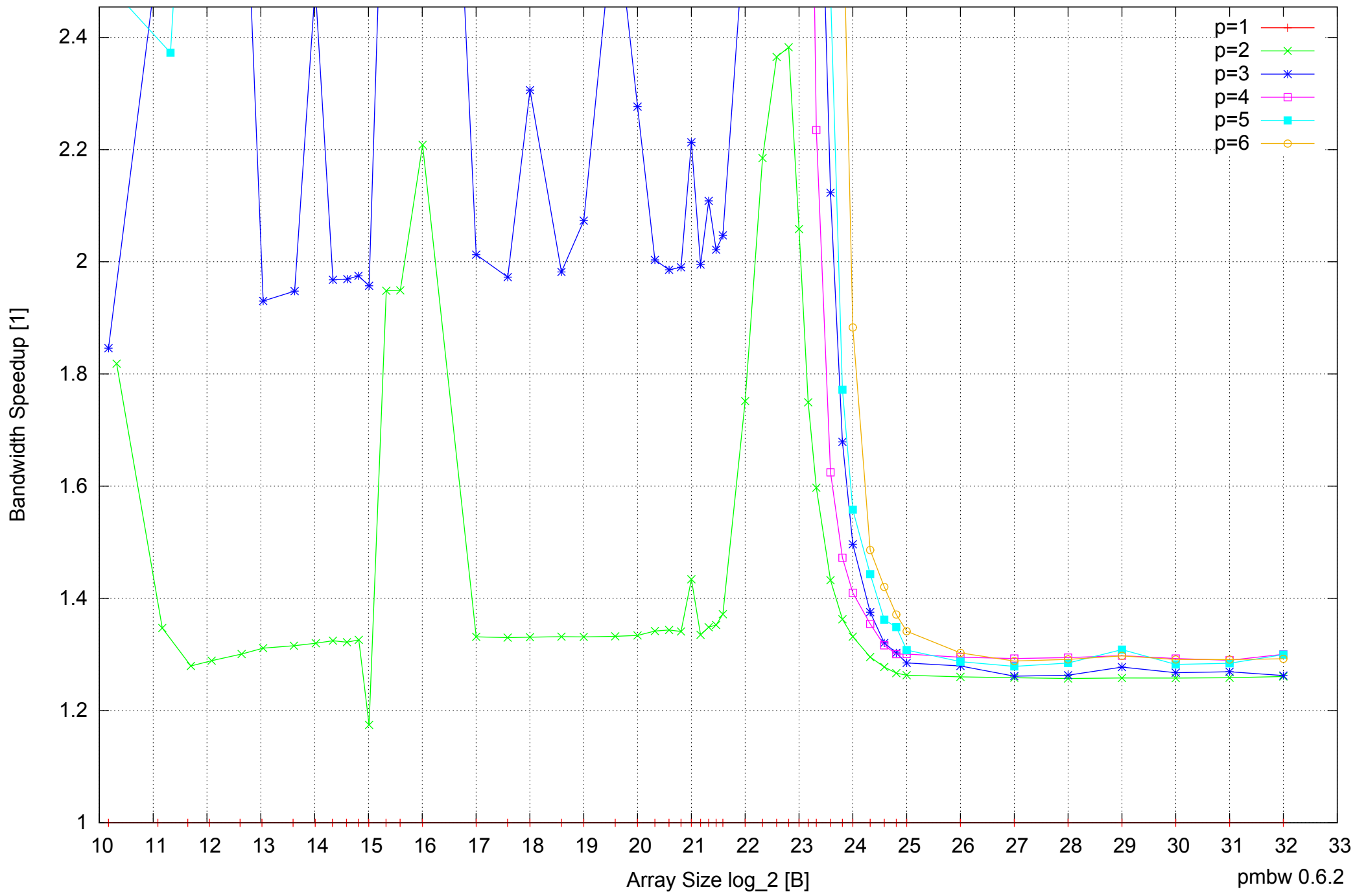
Intel Core 2 Quad Q6600 8GB - Speedup of Parallel Memory Bandwidth (enlarged) - ScanRead64PtrSimpleLoop
