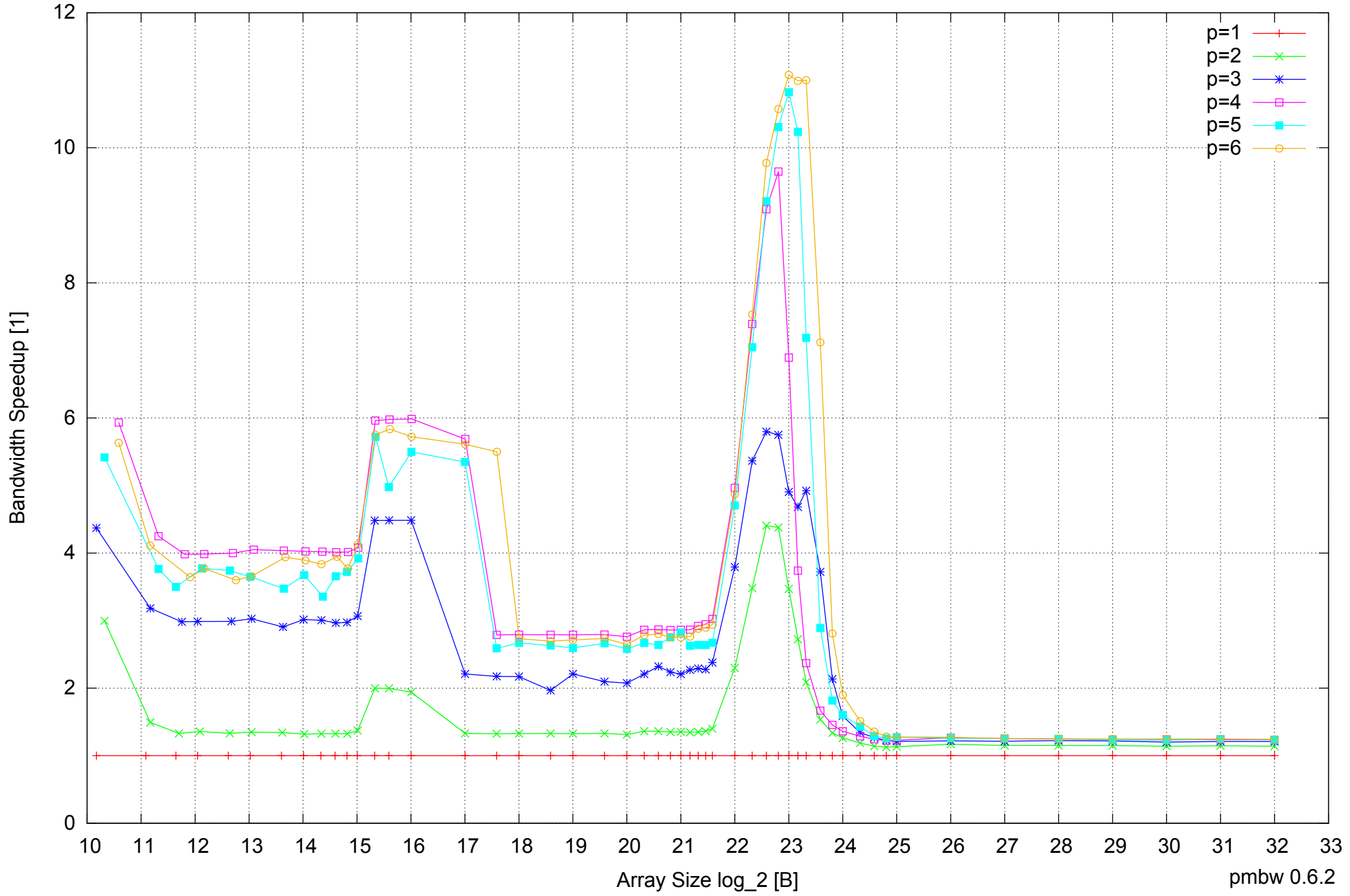
Intel Core 2 Quad Q6600 8GB - Speedup of Parallel Memory Bandwidth - ScanWrite64PtrUnrollLoop
