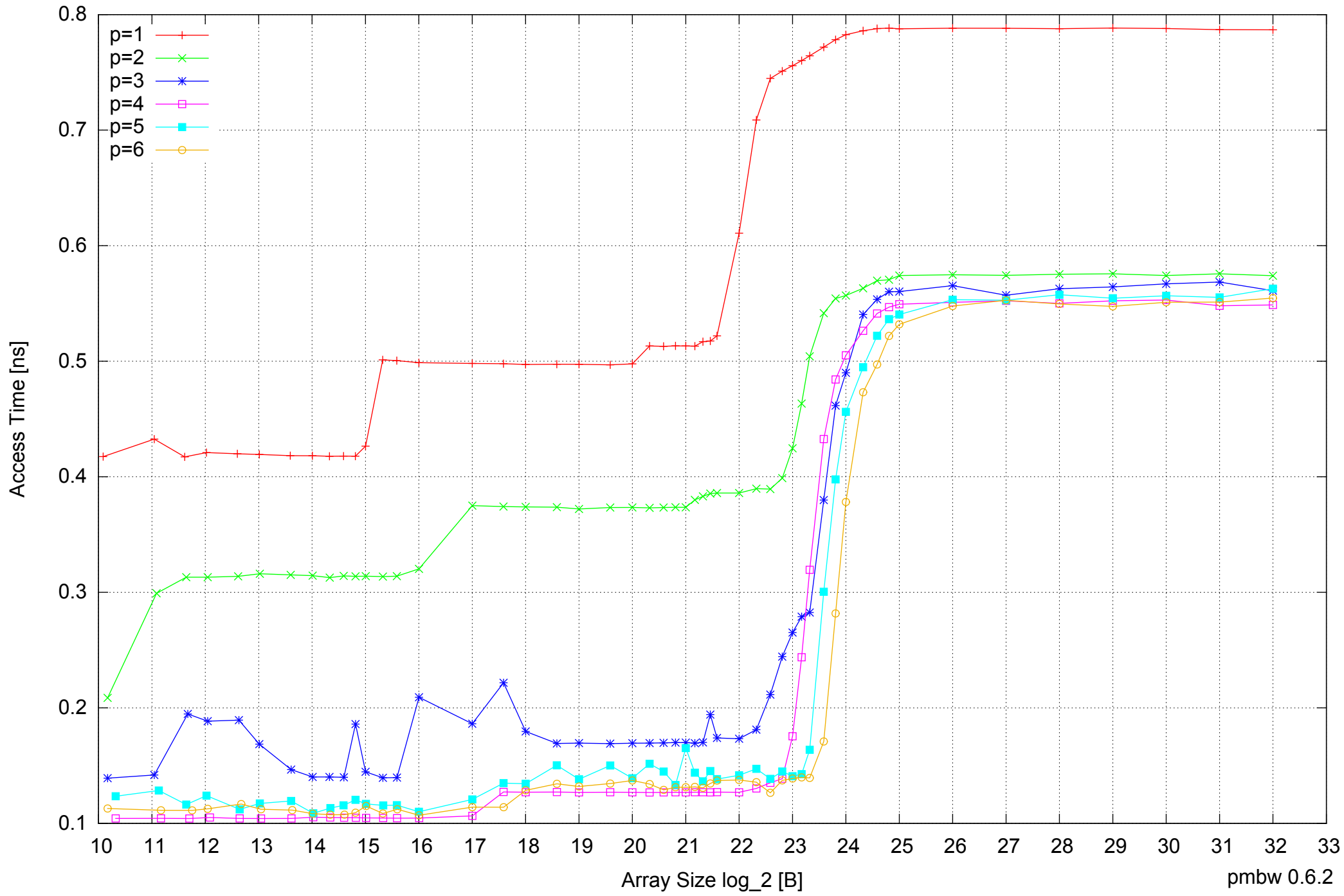
Intel Core 2 Quad Q6600 8GB - Parallel Memory Access Time - ScanRead32PtrUnrollLoop
