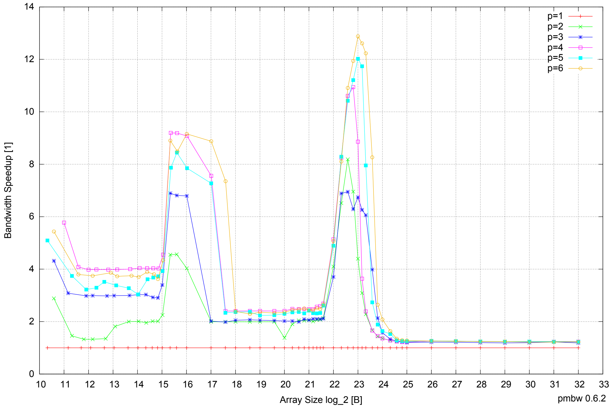
Intel Core 2 Quad Q6600 8GB - Speedup of Parallel Memory Bandwidth - ScanWrite128PtrUnrollLoop
