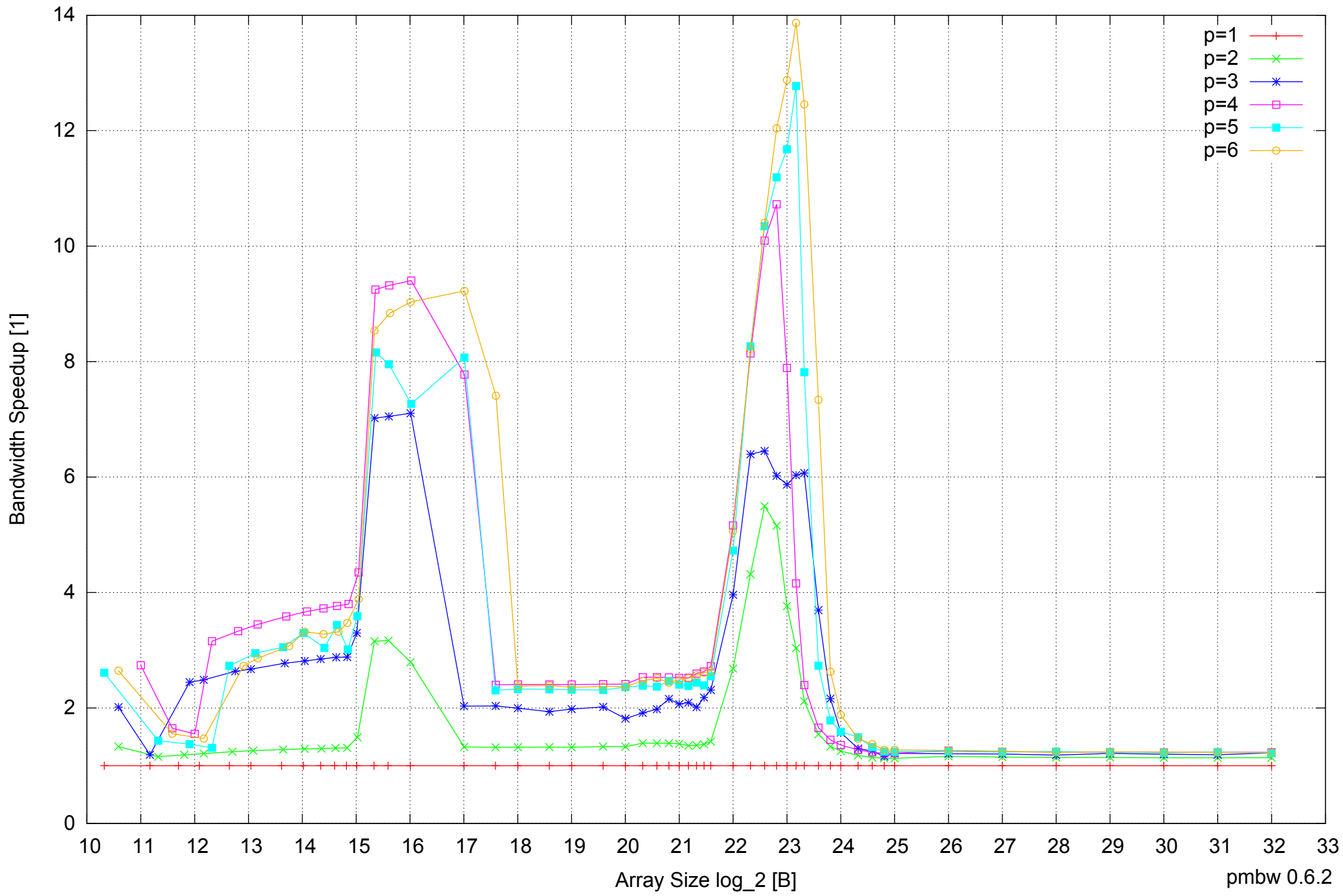
Intel Core 2 Quad Q6600 8GB - Speedup of Parallel Memory Bandwidth - ScanWrite128PtrSimpleLoop
