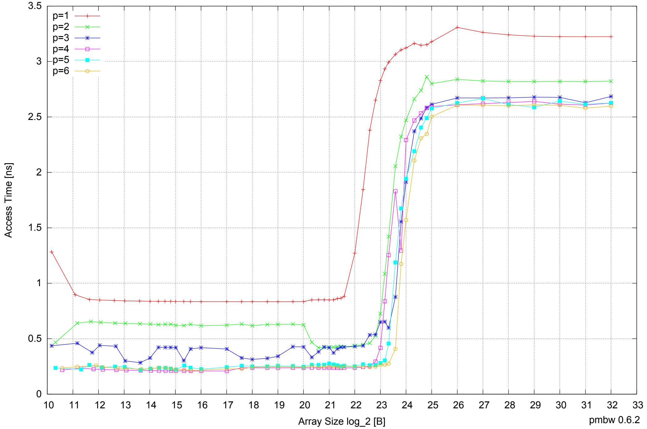
Intel Core 2 Quad Q6600 8GB - Parallel Memory Access Time - ScanWrite64IndexSimpleLoop
