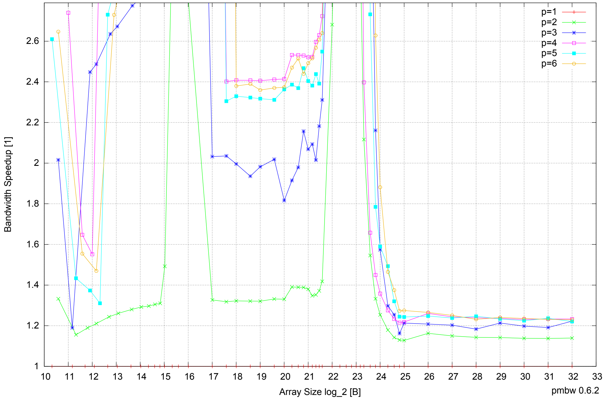
Intel Core 2 Quad Q6600 8GB - Speedup of Parallel Memory Bandwidth (enlarged) - ScanWrite128PtrSimpleLoop
