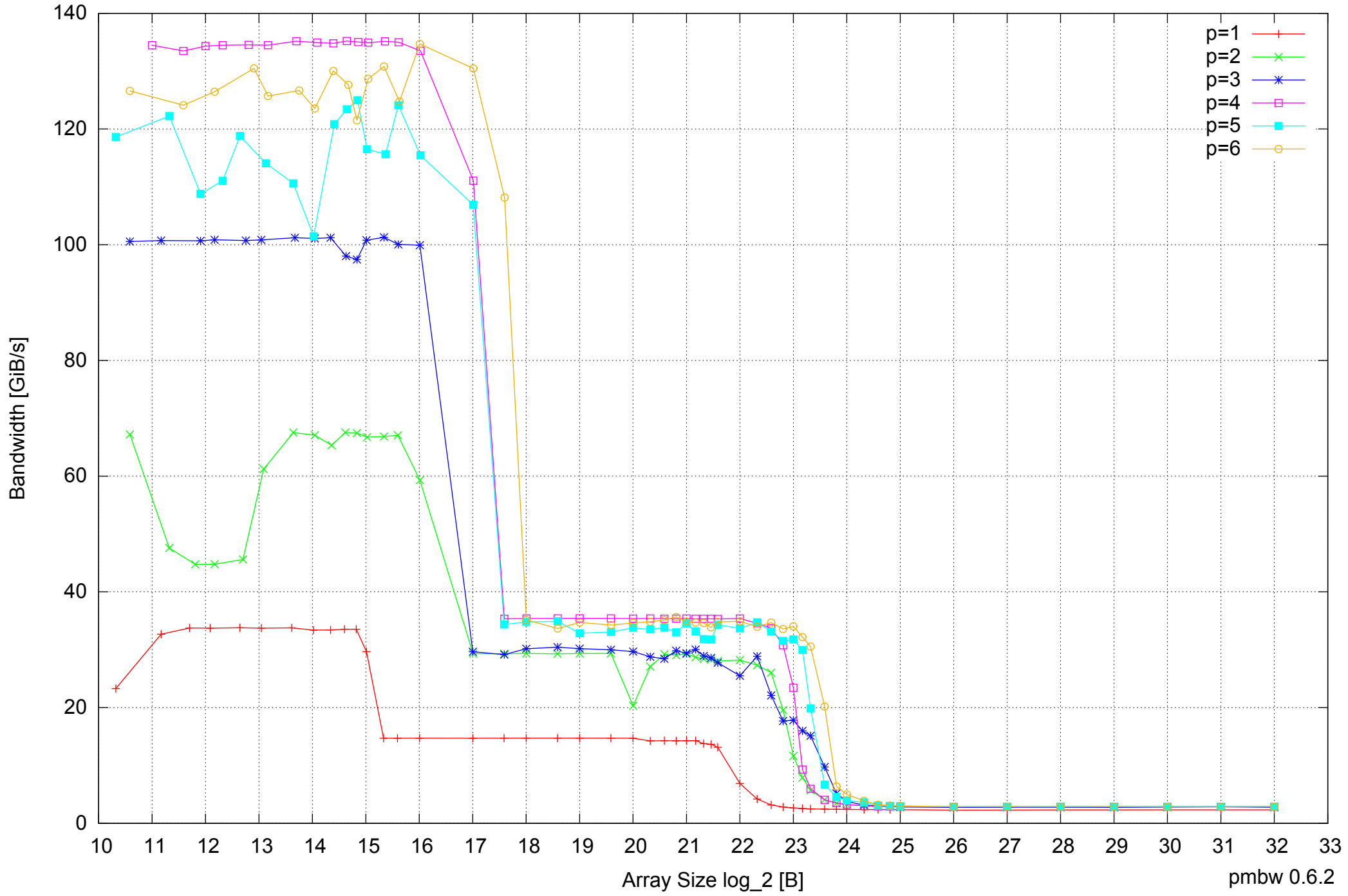
Intel Core 2 Quad Q6600 8GB - Parallel Memory Bandwidth - ScanWrite128PtrUnrollLoop
