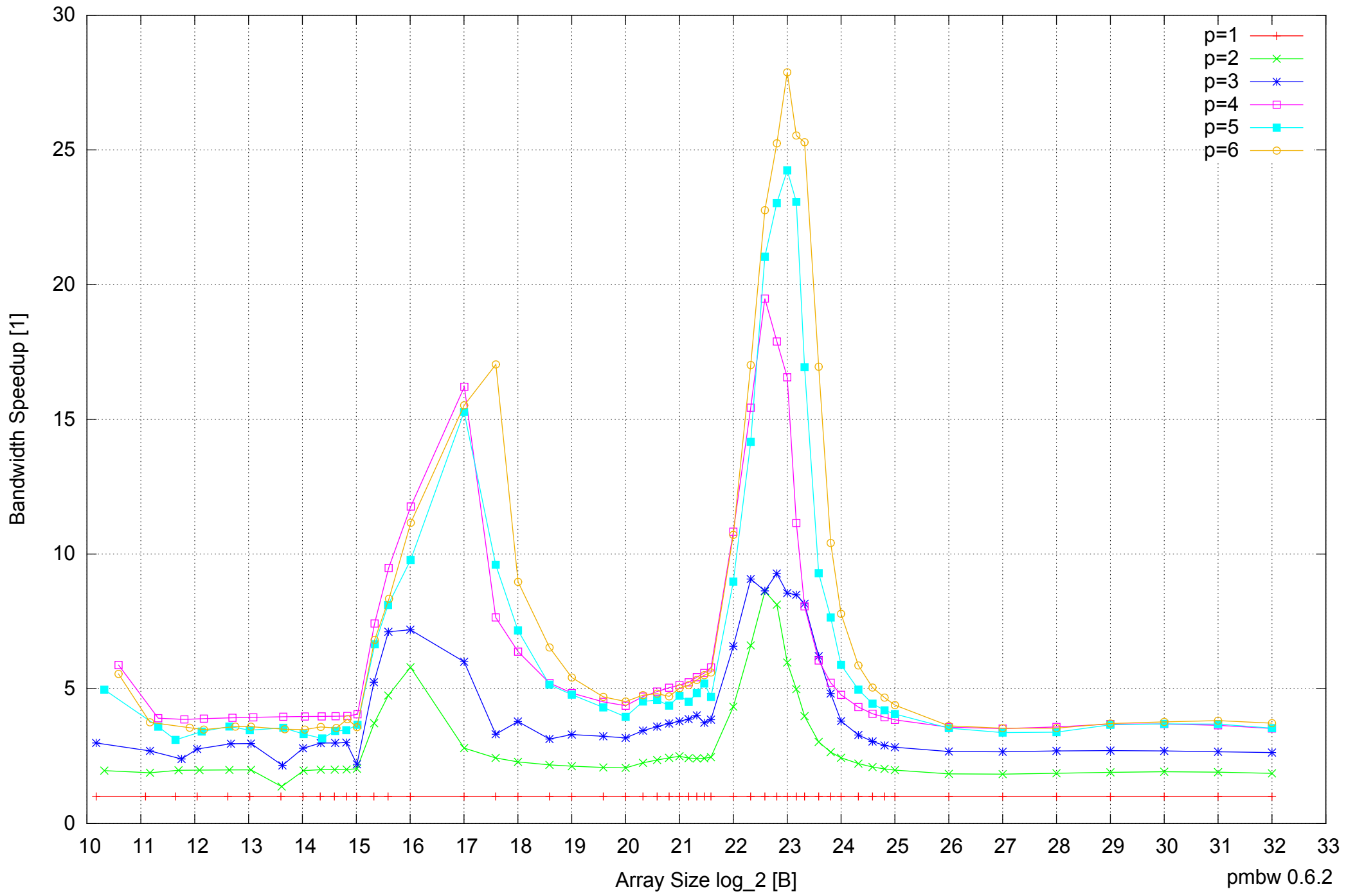
Intel Core 2 Quad Q6600 8GB - Speedup of Parallel Memory Bandwidth - PermRead64SimpleLoop
