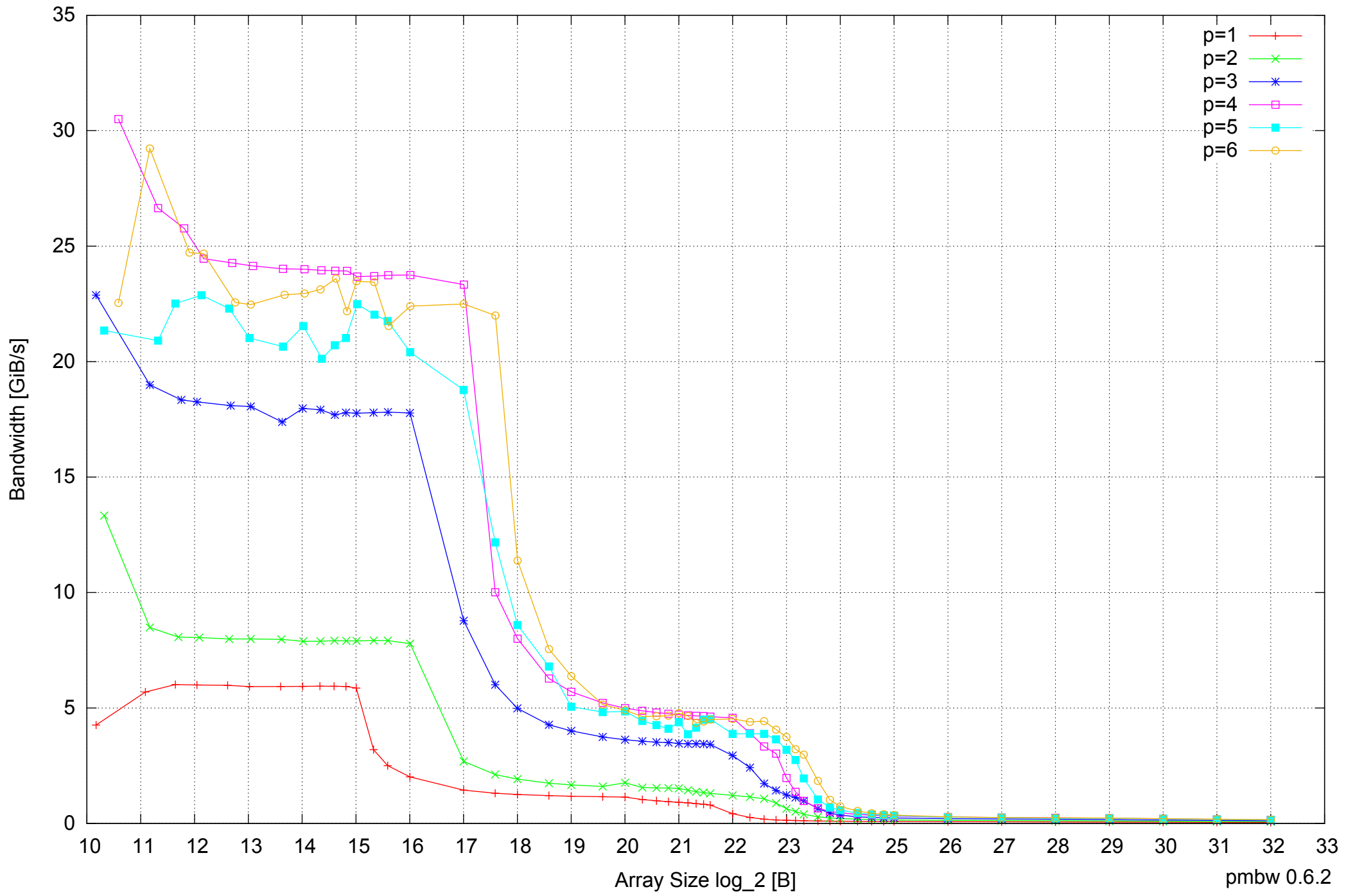
Intel Core 2 Quad Q6600 8GB - Parallel Memory Bandwidth - PermRead64UnrollLoop
