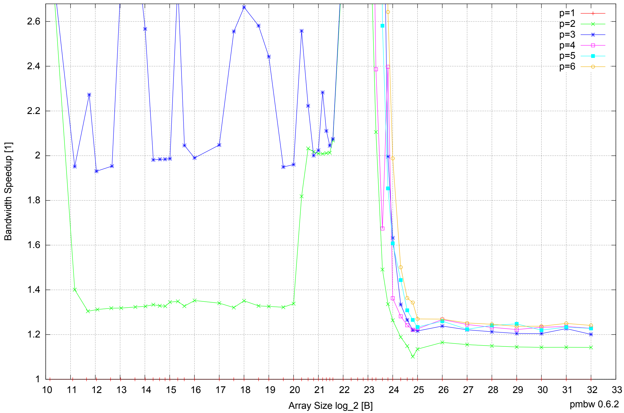
Intel Core 2 Quad Q6600 8GB - Speedup of Parallel Memory Bandwidth (enlarged) - ScanWrite64IndexSimpleLoop
