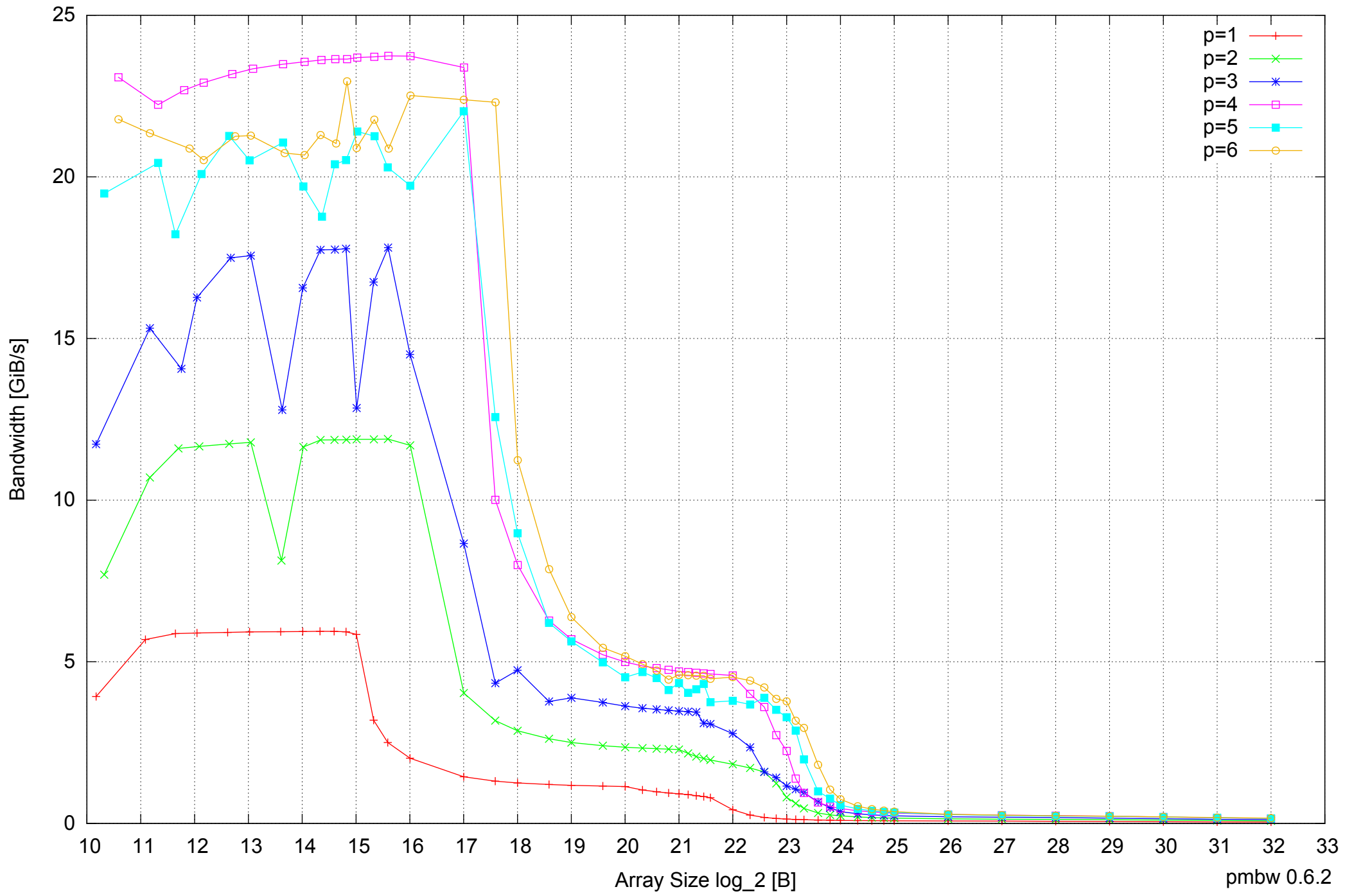
Intel Core 2 Quad Q6600 8GB - Parallel Memory Bandwidth - PermRead64SimpleLoop
