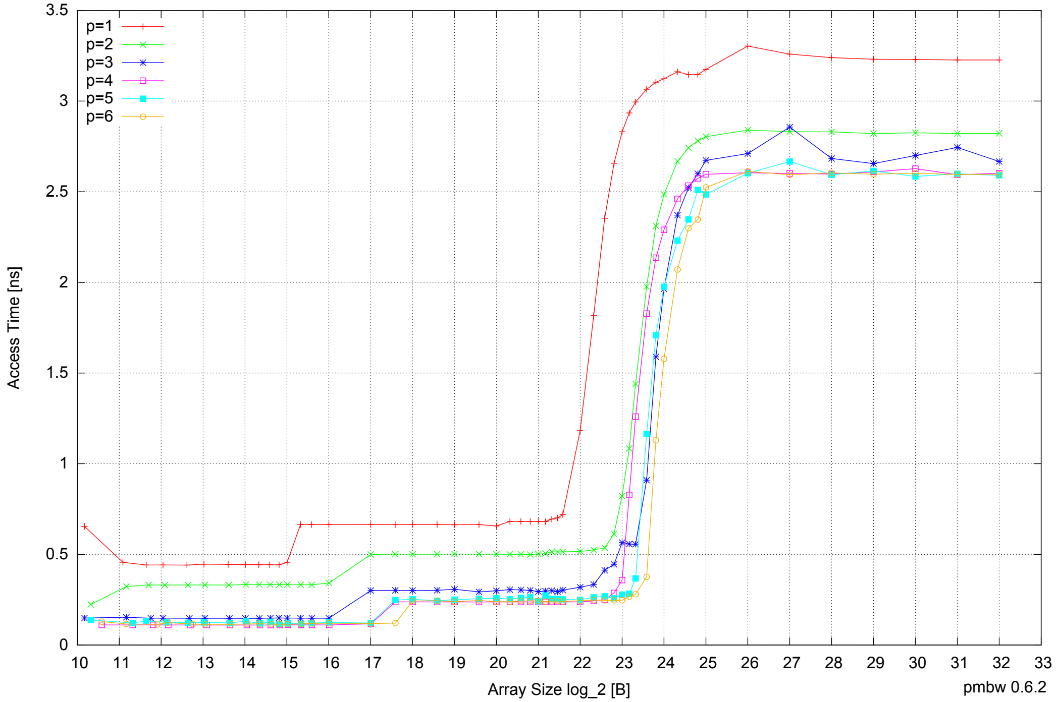
Intel Core 2 Quad Q6600 8GB - Parallel Memory Access Time - ScanWrite64IndexUnrollLoop
