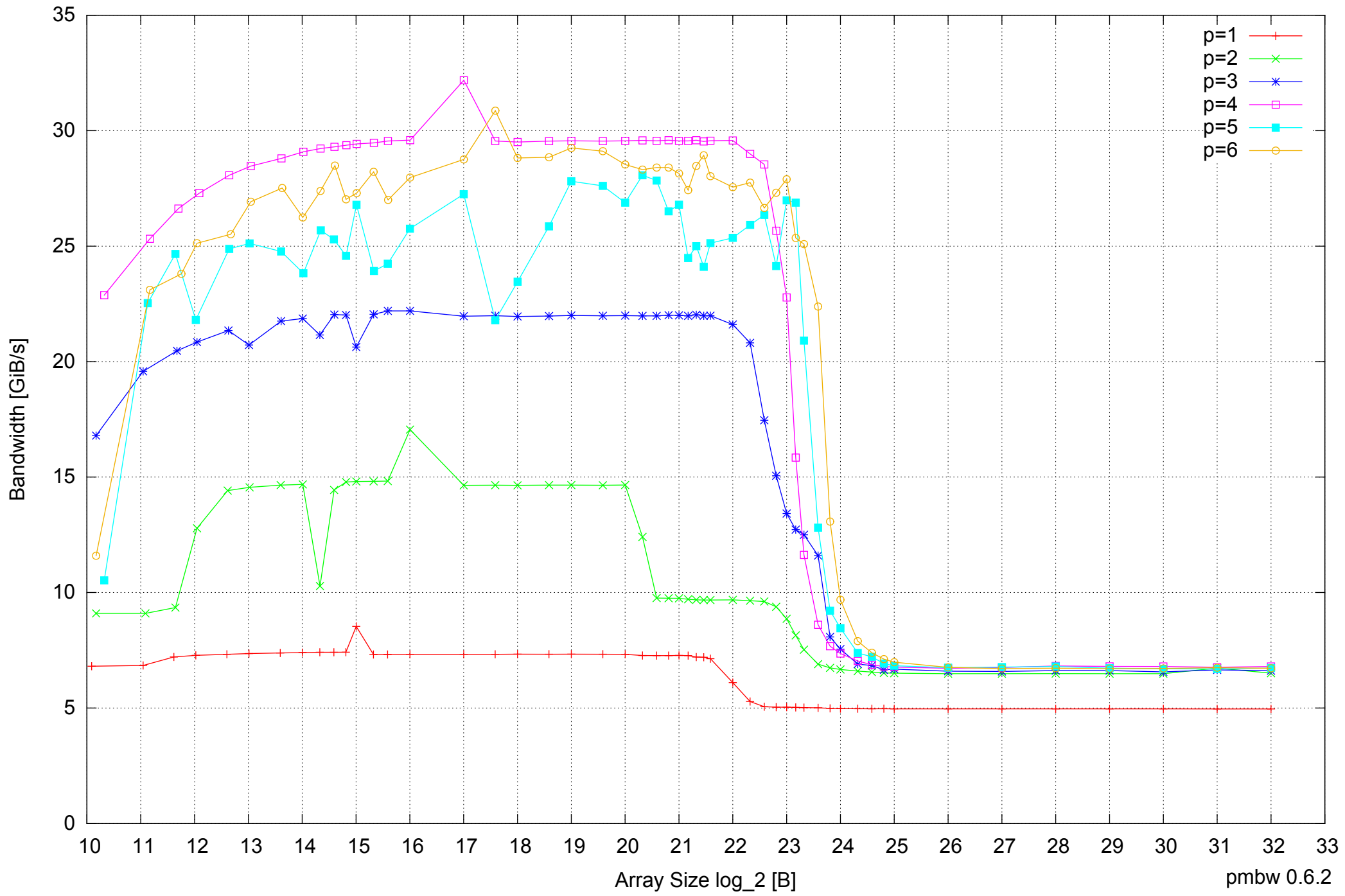
Intel Core 2 Quad Q6600 8GB - Parallel Memory Bandwidth - ScanRead32PtrSimpleLoop
