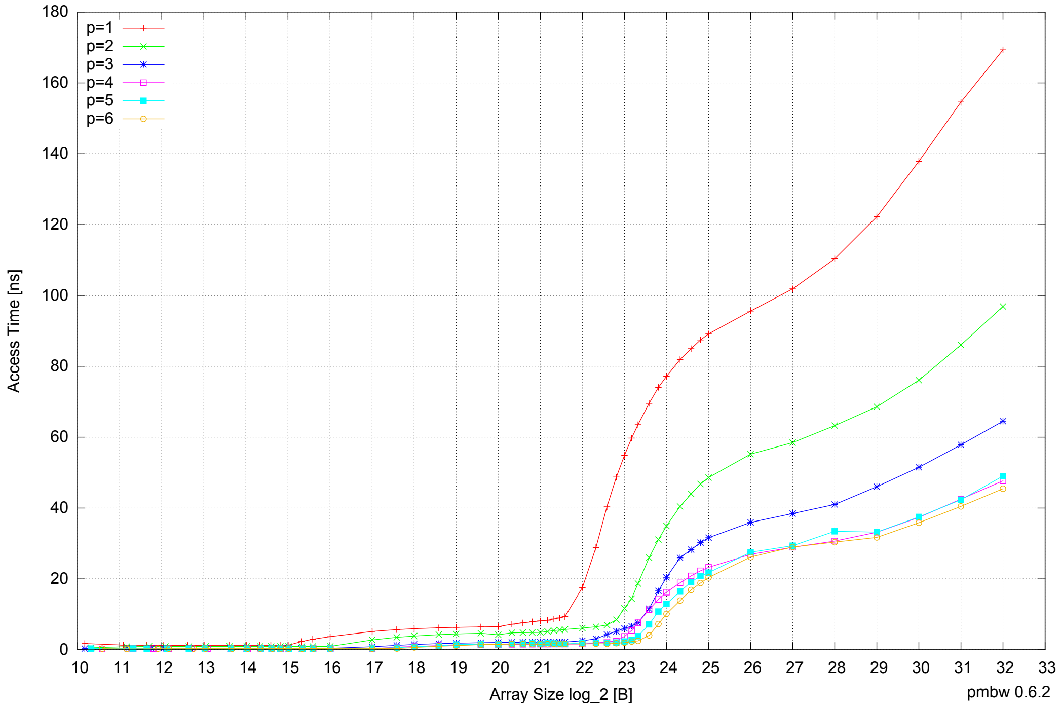
Intel Core 2 Quad Q6600 8GB - Parallel Memory Access Time - PermRead64UnrollLoop
