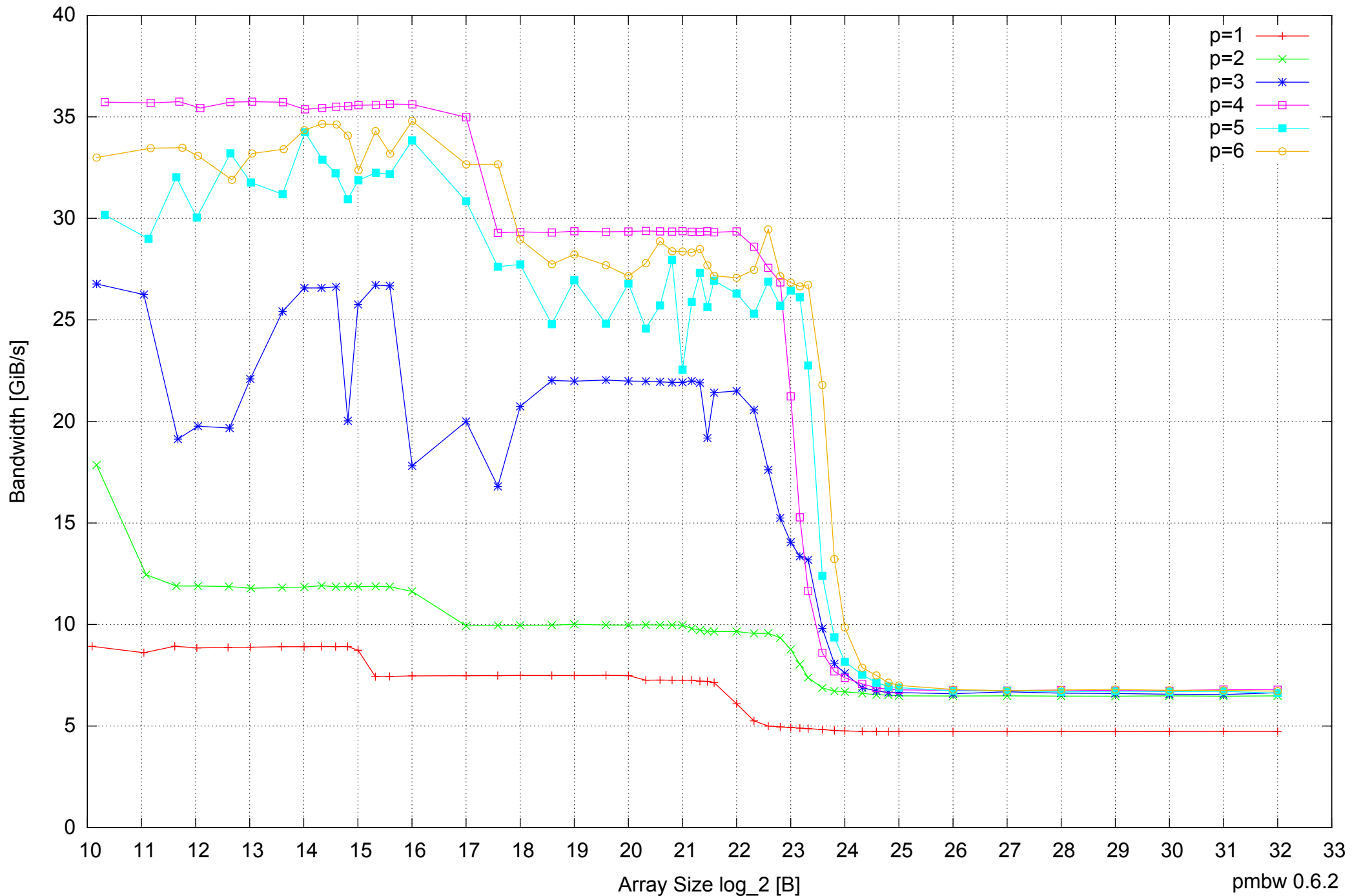
Intel Core 2 Quad Q6600 8GB - Parallel Memory Bandwidth - ScanRead32PtrUnrollLoop
