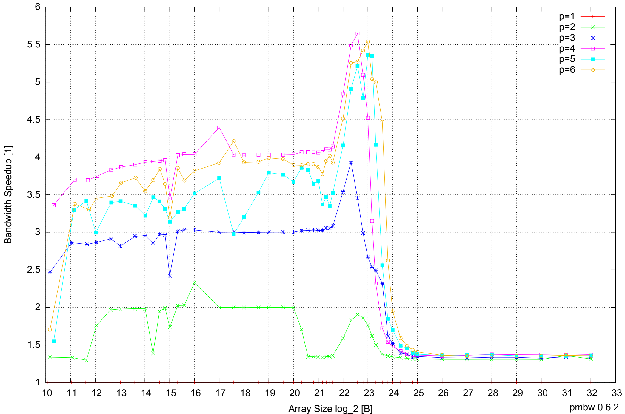
Intel Core 2 Quad Q6600 8GB - Speedup of Parallel Memory Bandwidth - ScanRead32PtrSimpleLoop
