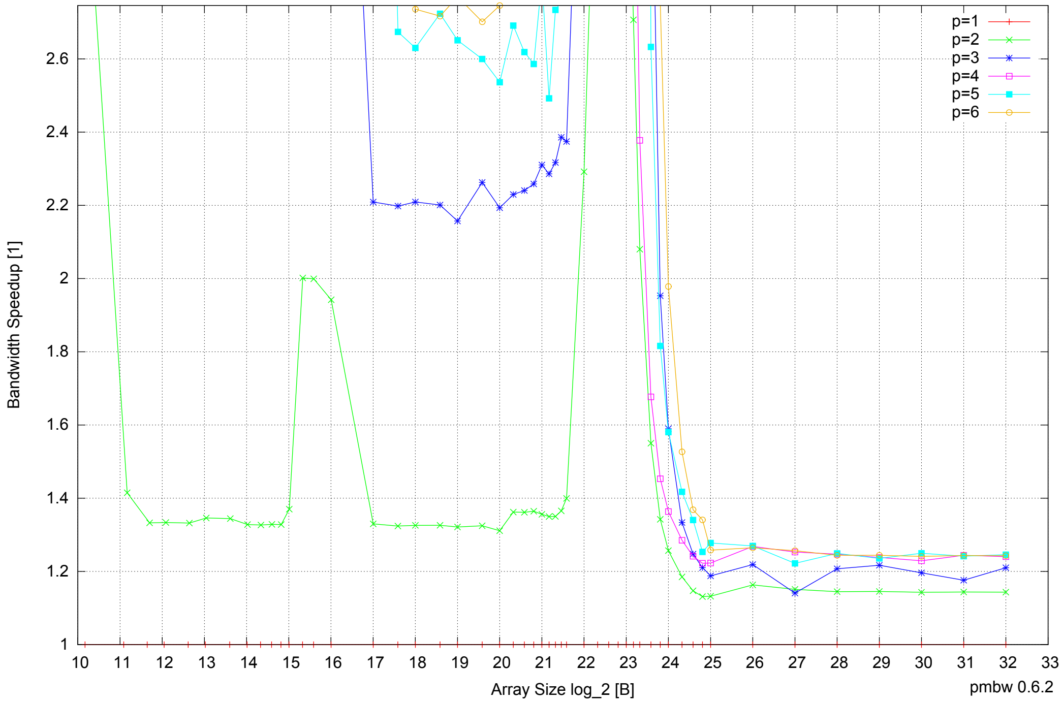
Intel Core 2 Quad Q6600 8GB - Speedup of Parallel Memory Bandwidth (enlarged) - ScanWrite64IndexUnrollLoop
