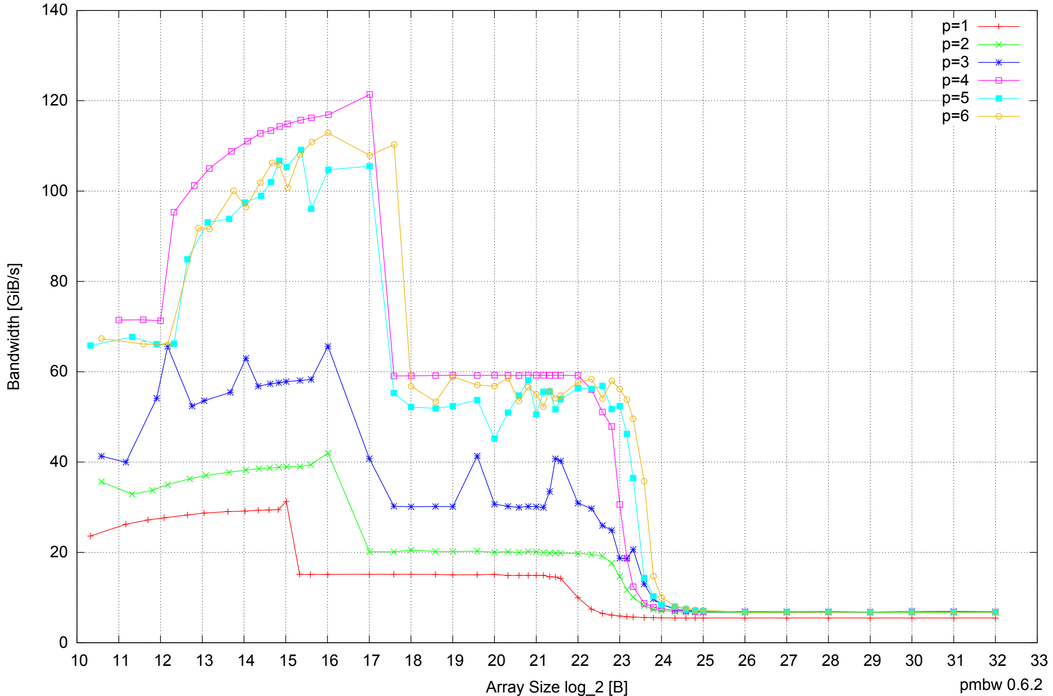
Intel Core 2 Quad Q6600 8GB - Parallel Memory Bandwidth - ScanRead128PtrSimpleLoop
