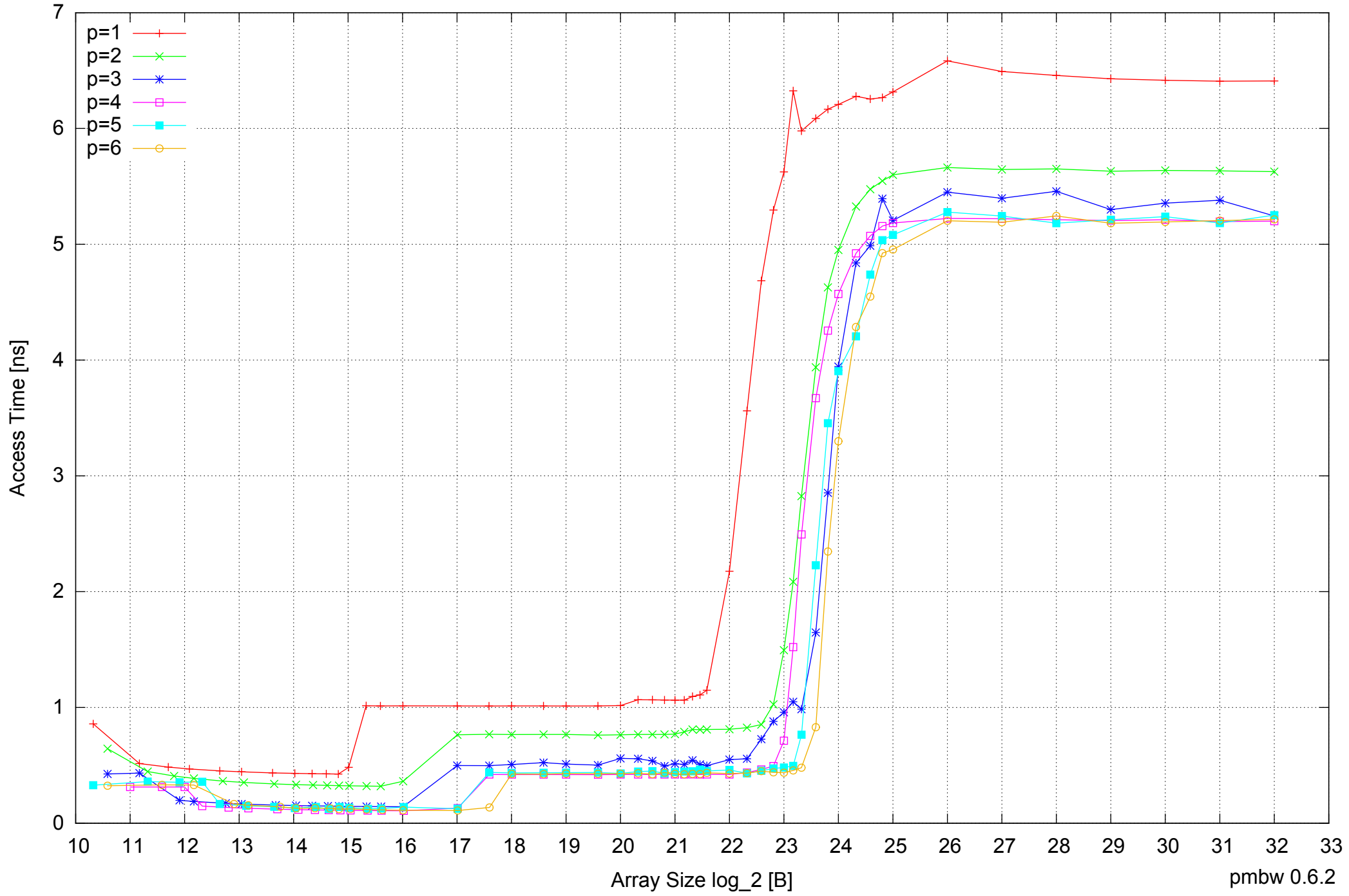
Intel Core 2 Quad Q6600 8GB - Parallel Memory Access Time - ScanWrite128PtrSimpleLoop
