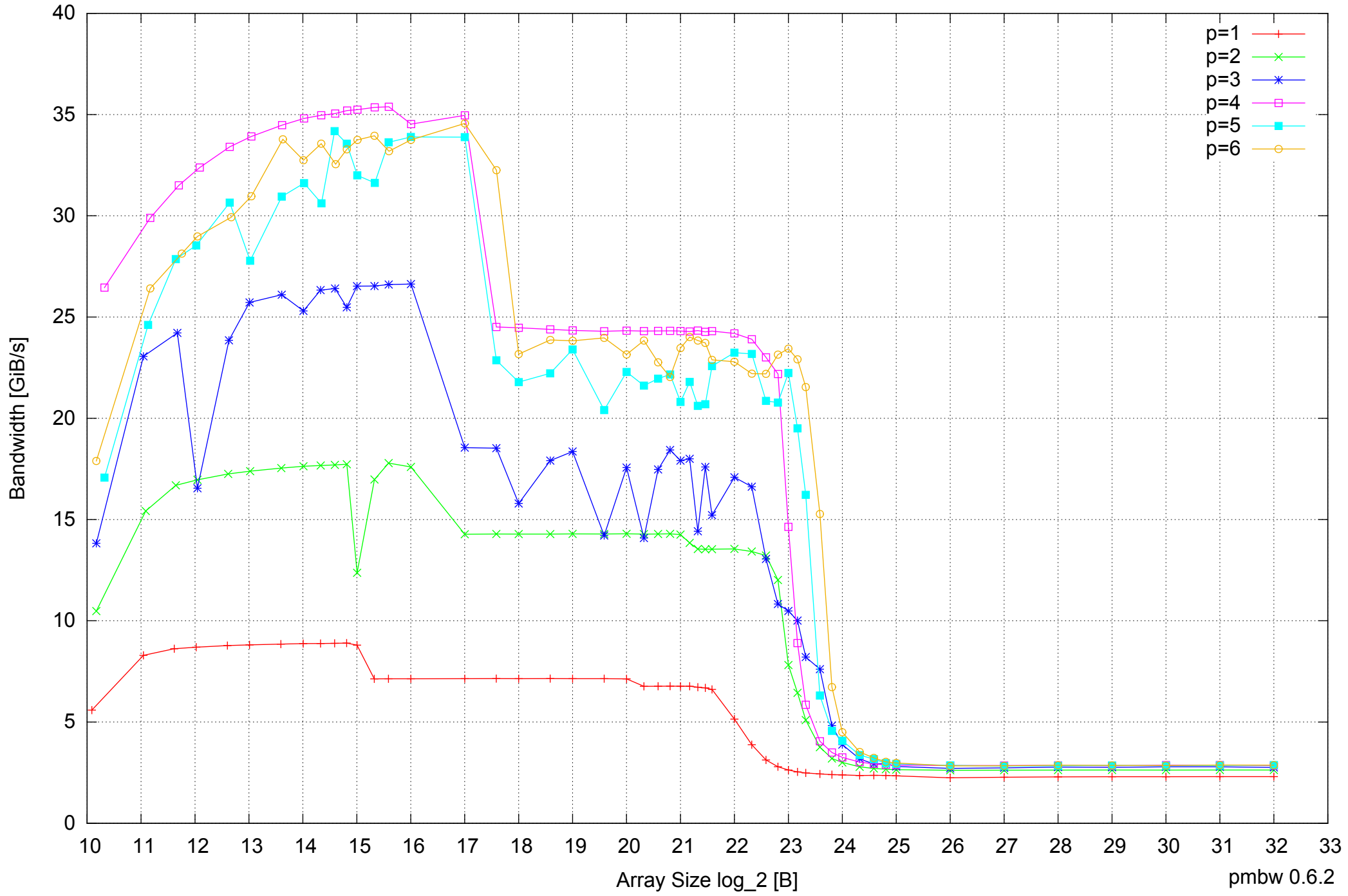
Intel Core 2 Quad Q6600 8GB - Parallel Memory Bandwidth - ScanWrite32PtrSimpleLoop
