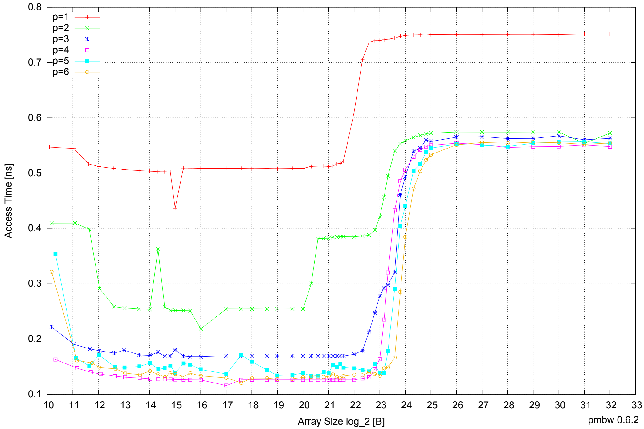
Intel Core 2 Quad Q6600 8GB - Parallel Memory Access Time - ScanRead32PtrSimpleLoop
