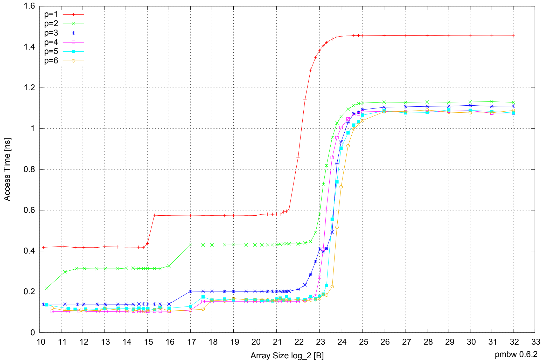
Intel Core 2 Quad Q6600 8GB - Parallel Memory Access Time - ScanRead64PtrUnrollLoop
