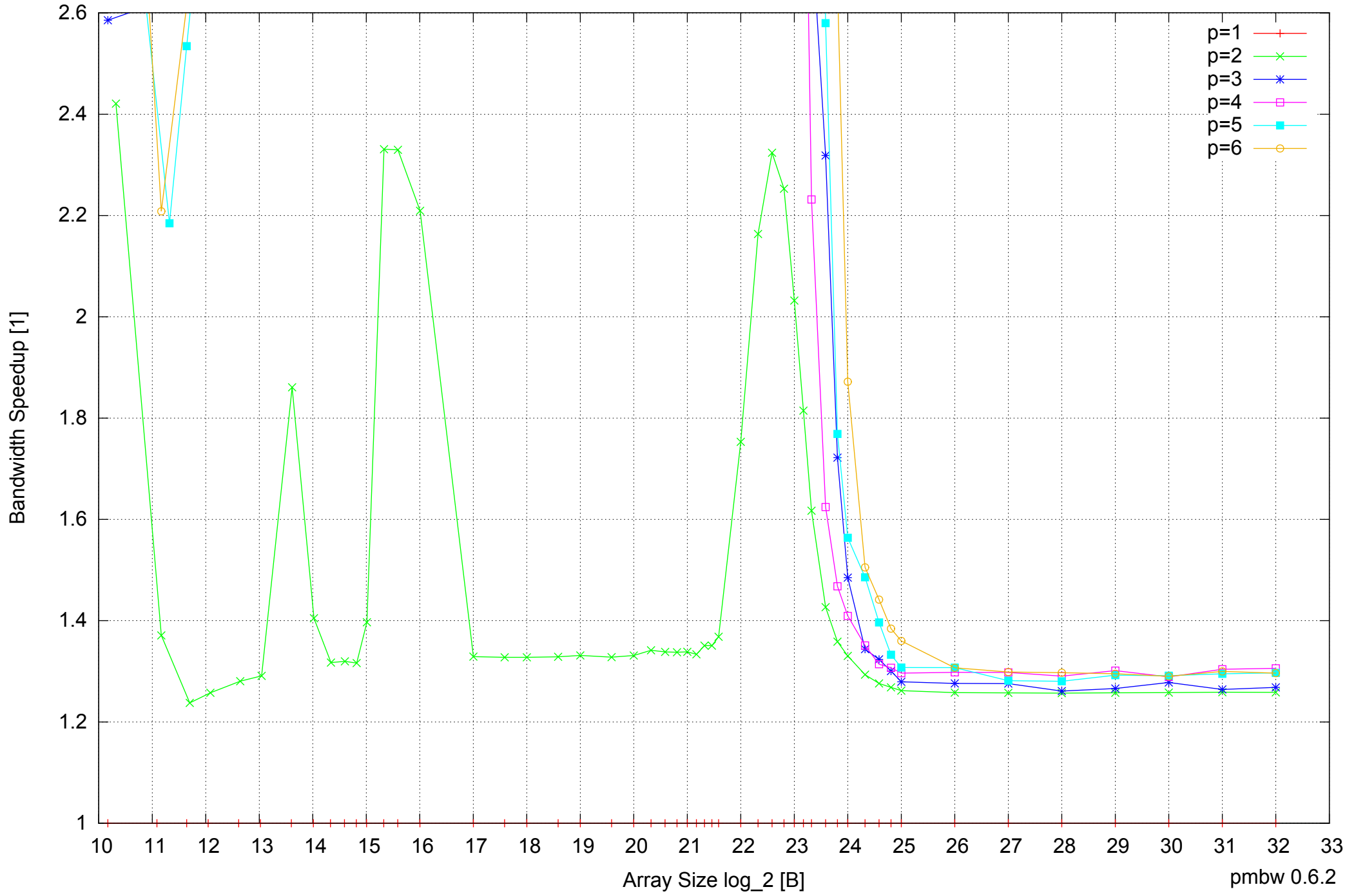
Intel Core 2 Quad Q6600 8GB - Speedup of Parallel Memory Bandwidth (enlarged) - ScanRead64IndexSimpleLoop
