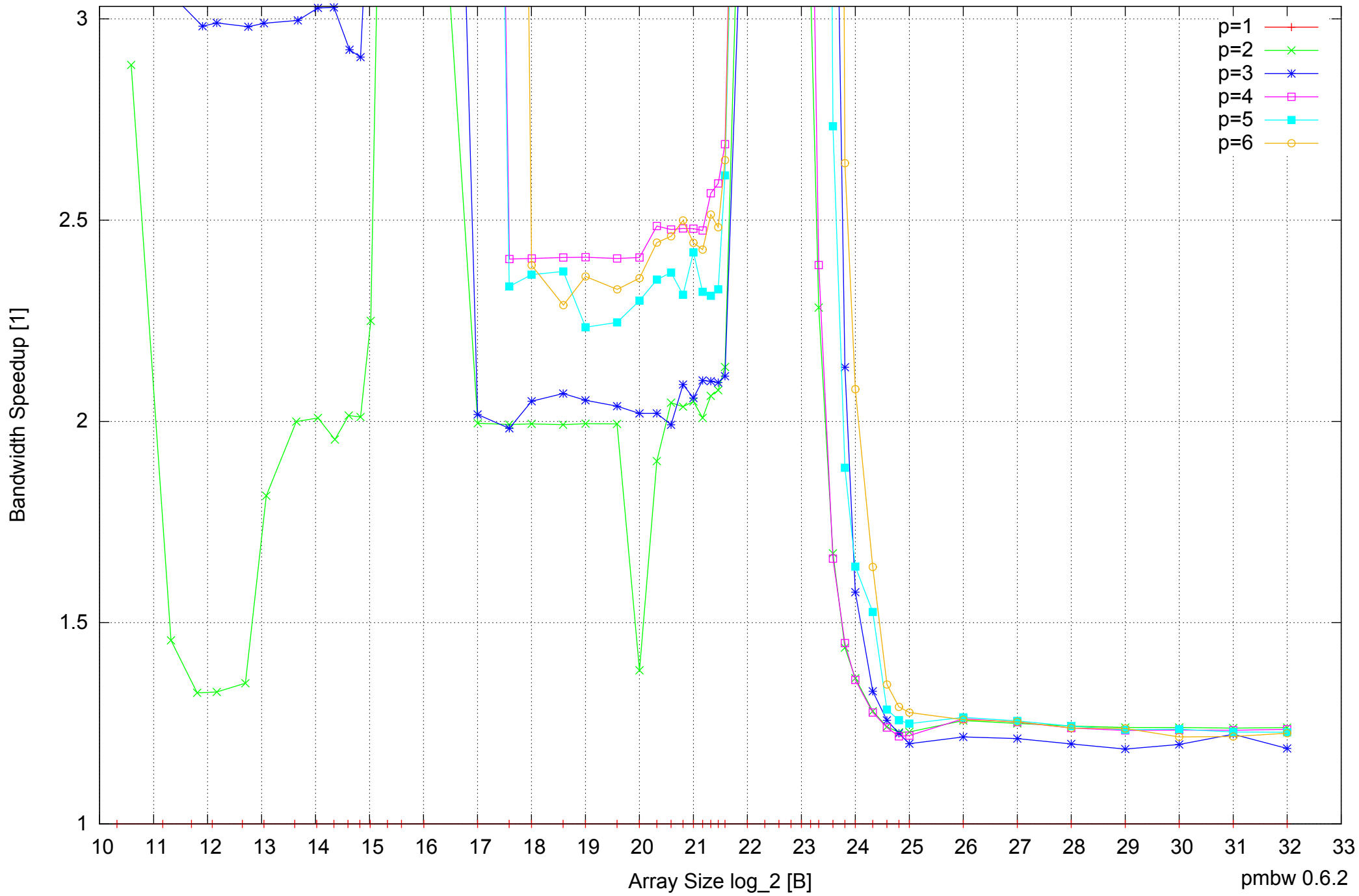
Intel Core 2 Quad Q6600 8GB - Speedup of Parallel Memory Bandwidth (enlarged) - ScanWrite128PtrUnrollLoop
