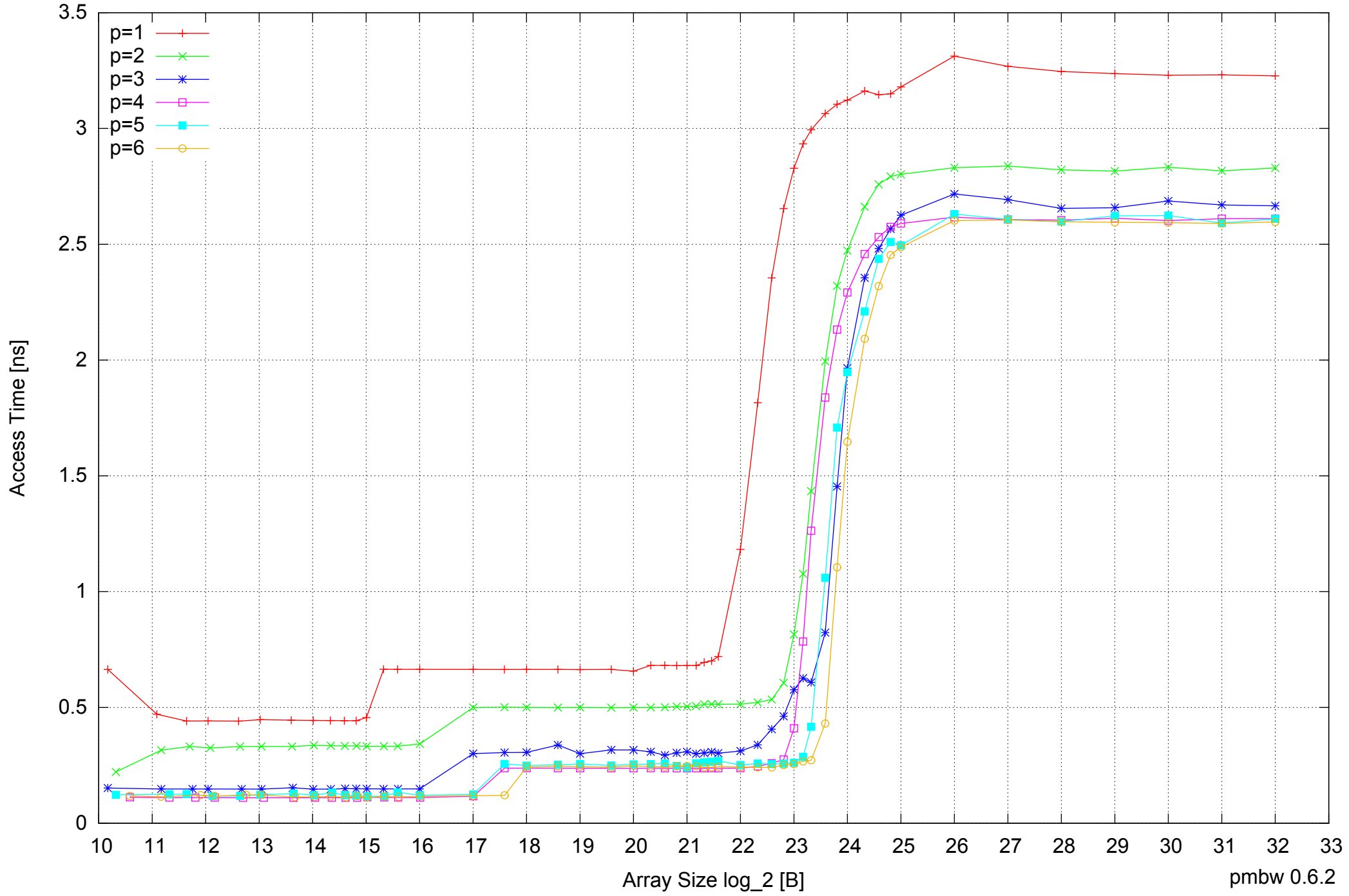
Intel Core 2 Quad Q6600 8GB - Parallel Memory Access Time - ScanWrite64PtrUnrollLoop
