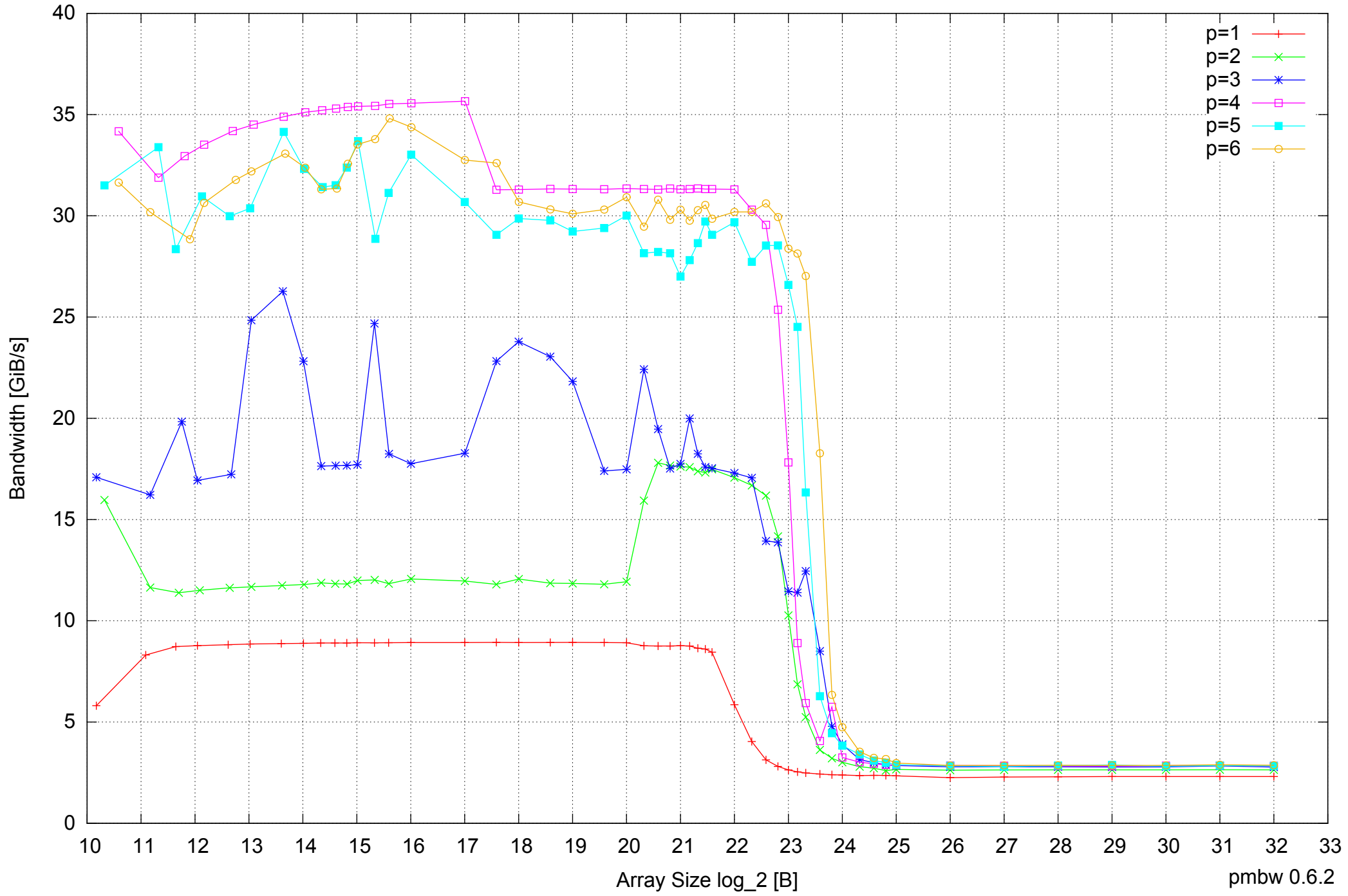
Intel Core 2 Quad Q6600 8GB - Parallel Memory Bandwidth - ScanWrite64IndexSimpleLoop
