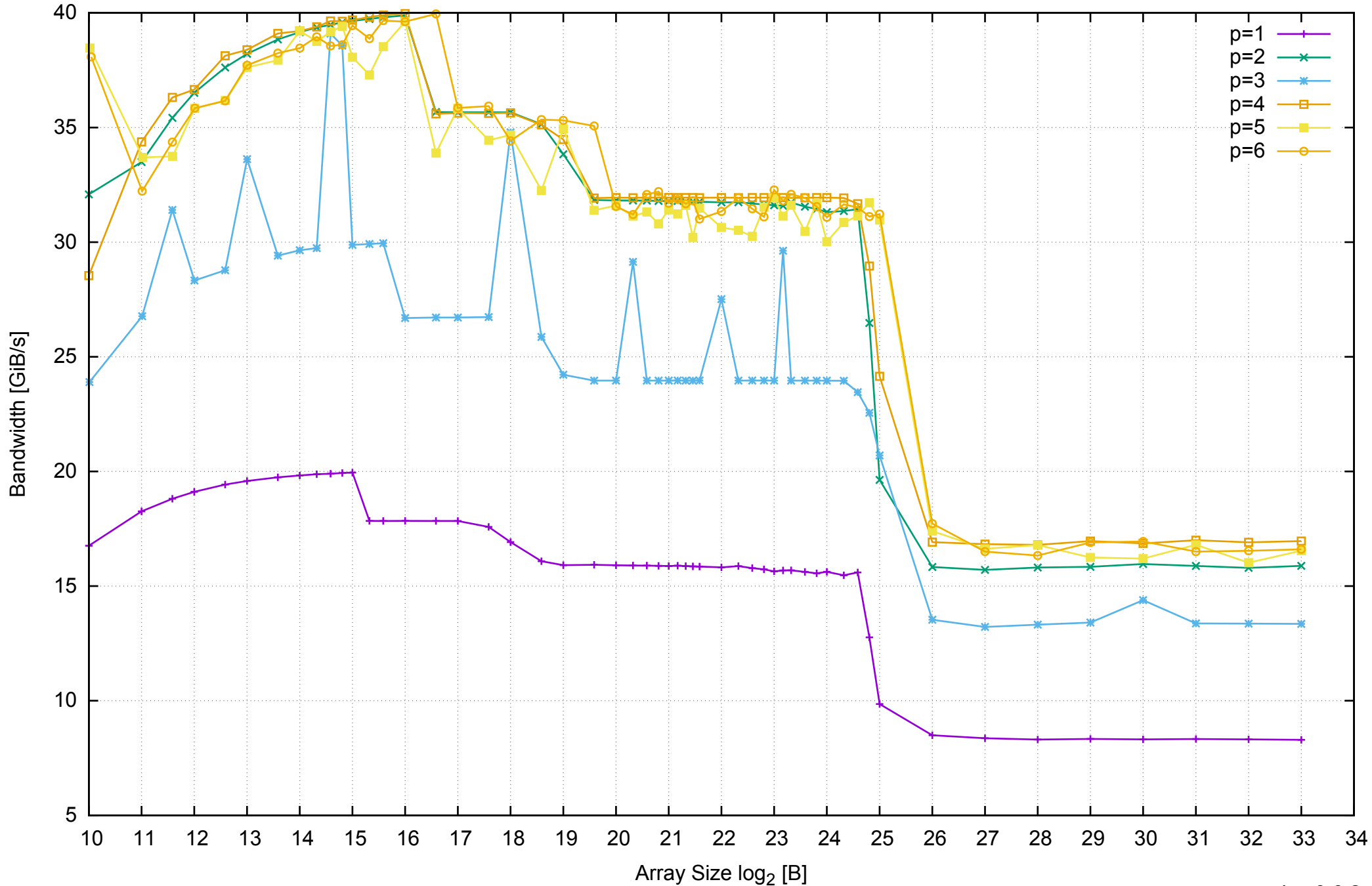
AWS m4.xlarge - Intel Xeon E5-2676 v3, 2.40 GHz 16GB - Parallel Memory Bandwidth - ScanWrite64PtrSimpleLoop
