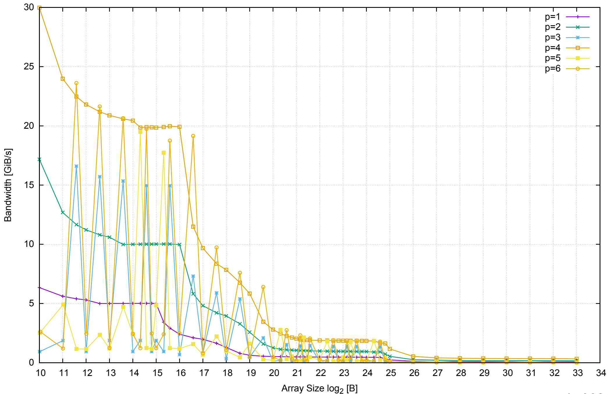
AWS m4.xlarge - Intel Xeon E5-2676 v3, 2.40 GHz 16GB - Parallel Memory Bandwidth - PermRead64UnrollLoop
