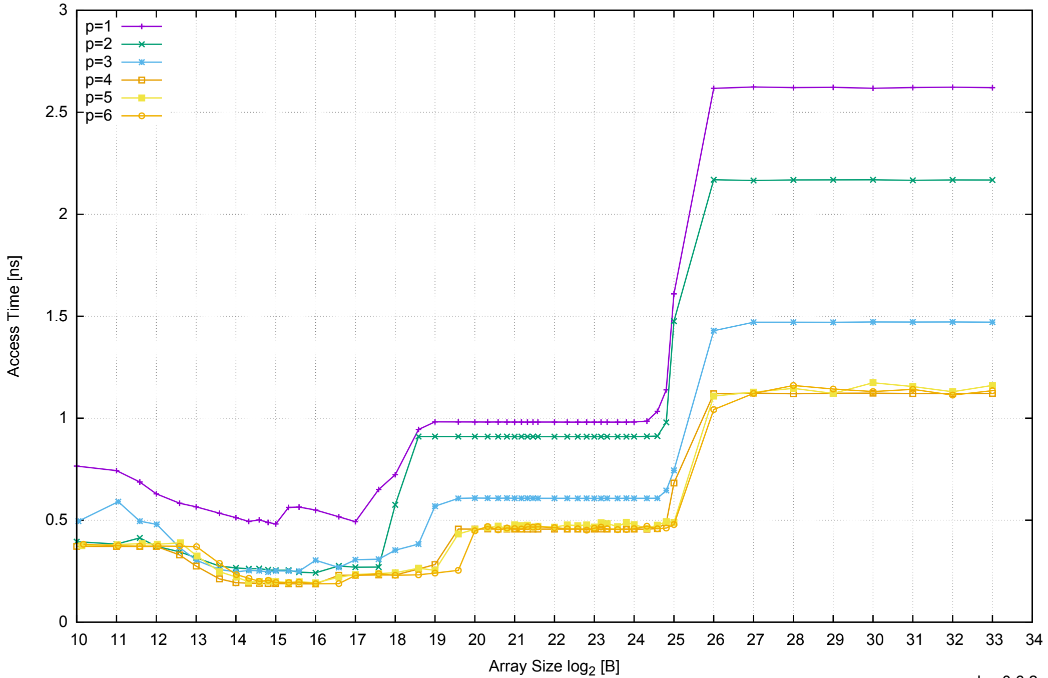
AWS m4.xlarge - Intel Xeon E5-2676 v3, 2.40 GHz 16GB - Parallel Memory Access Time - ScanRead256PtrSimpleLoop
