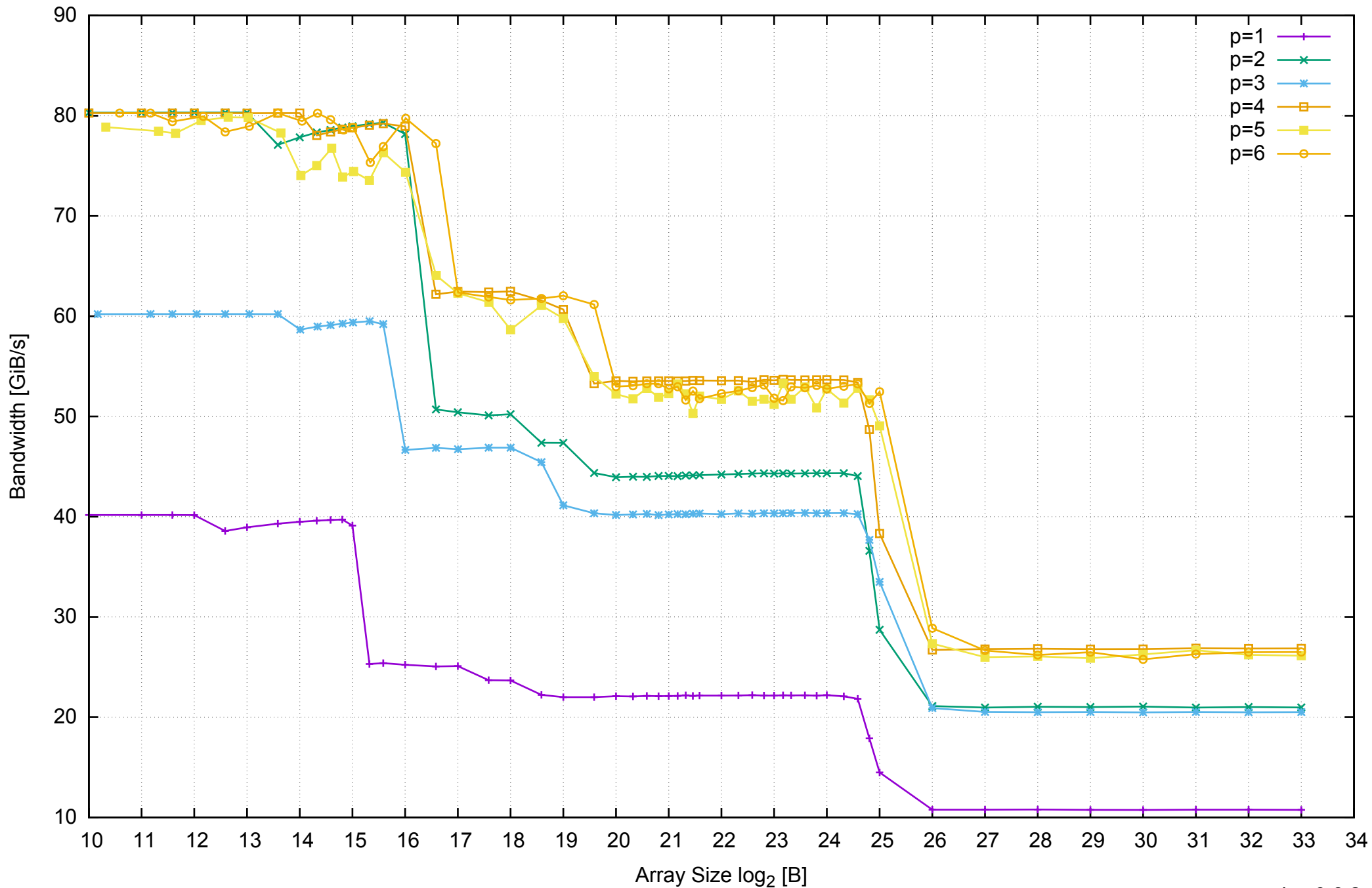
AWS m4.xlarge - Intel Xeon E5-2676 v3, 2.40 GHz 16GB - Parallel Memory Bandwidth - ScanRead64PtrUnrollLoop
