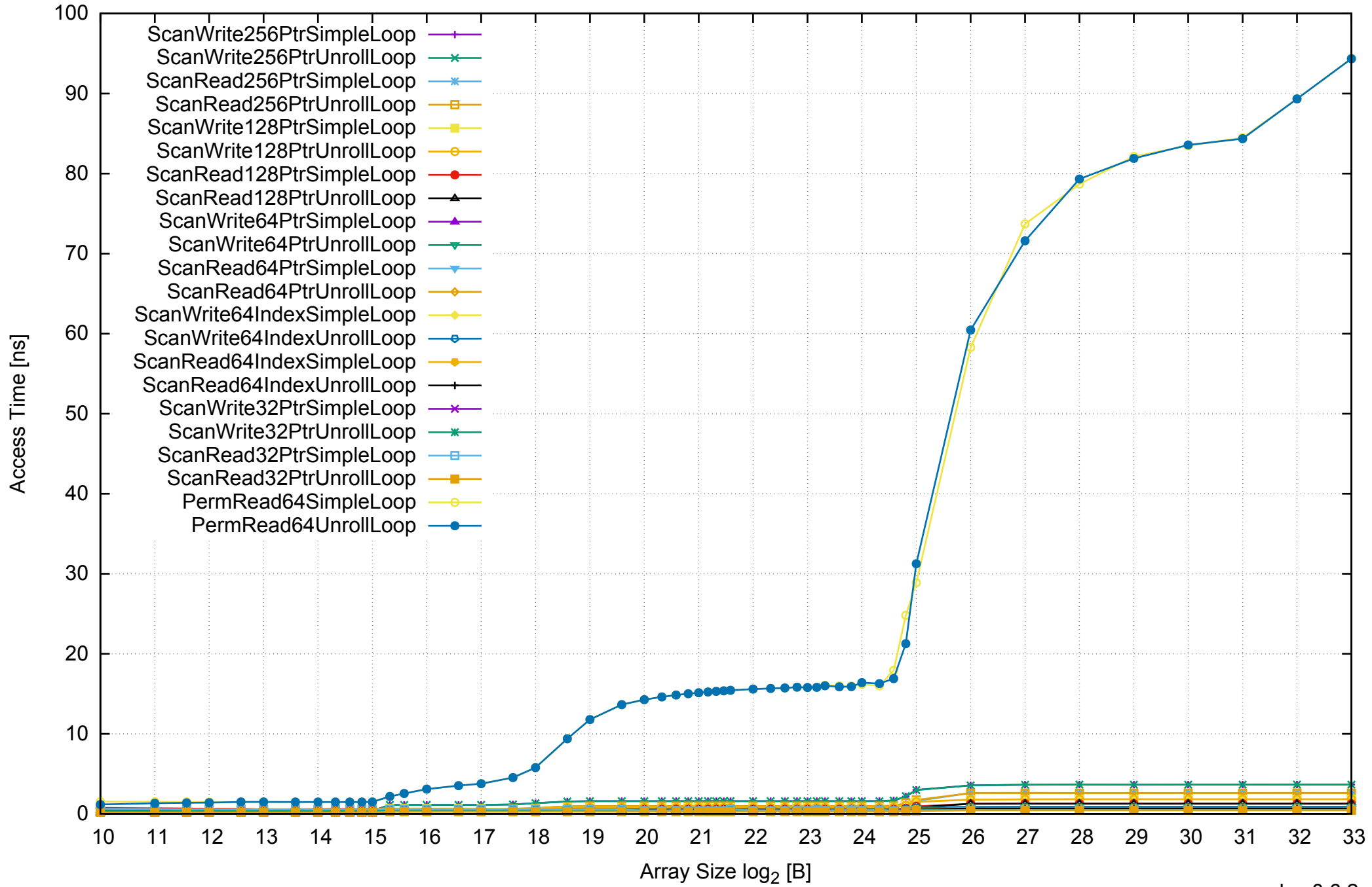
AWS m4.xlarge - Intel Xeon E5-2676 v3, 2.40 GHz 16GB - One Thread Memory Latency (Access Time)
