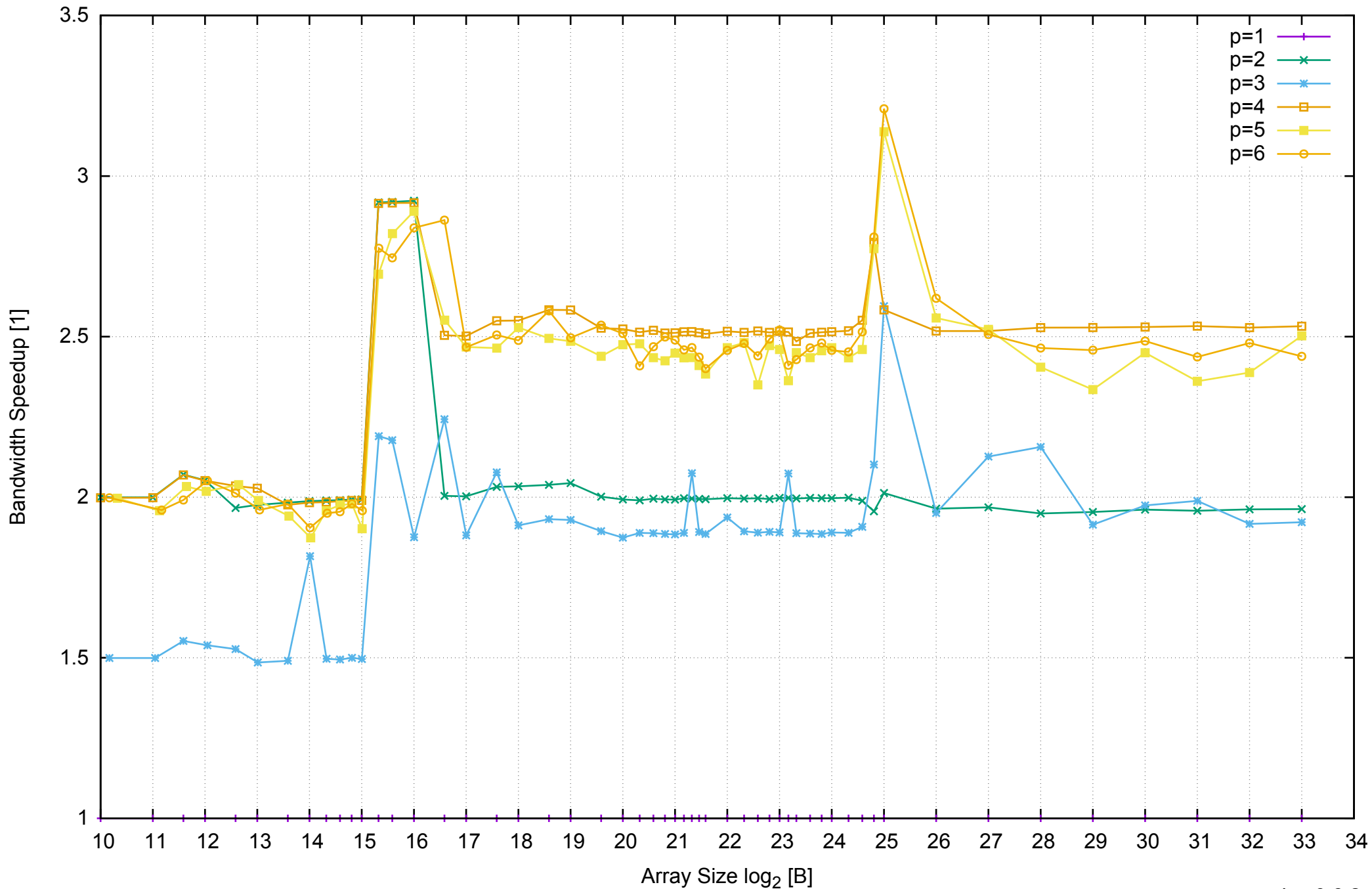
AWS m4.xlarge - Intel Xeon E5-2676 v3, 2.40 GHz 16GB - Speedup of Parallel Memory Bandwidth - ScanRead32PtrUnrollLoop
