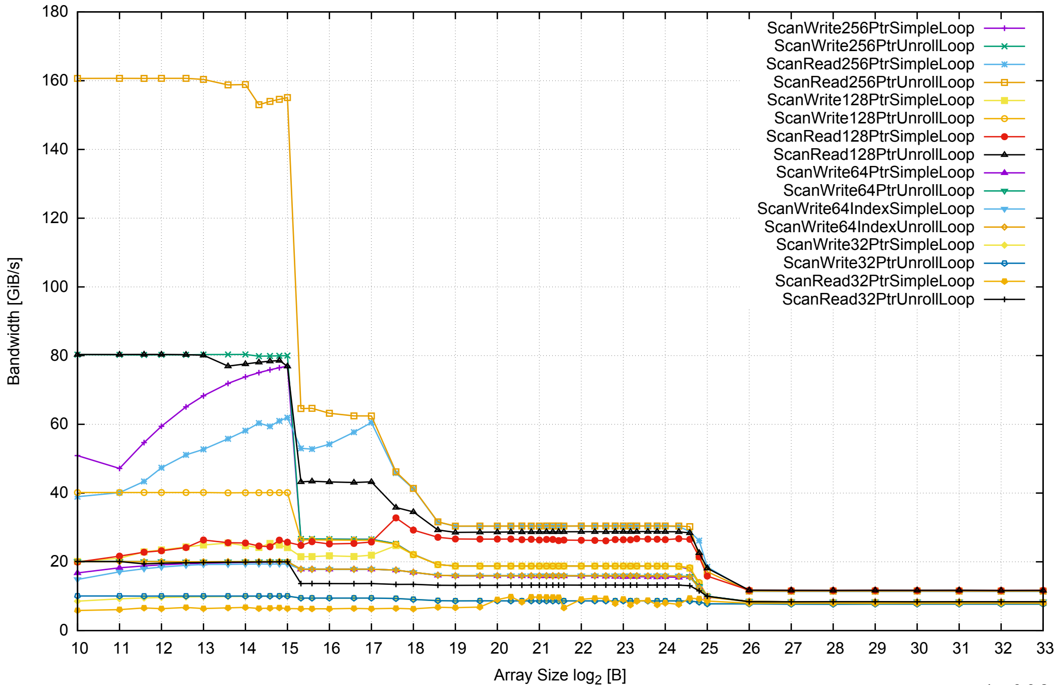
AWS m4.xlarge - Intel Xeon E5-2676 v3, 2.40 GHz 16GB - One Thread Memory Bandwidth (only 64-bit Reads)
