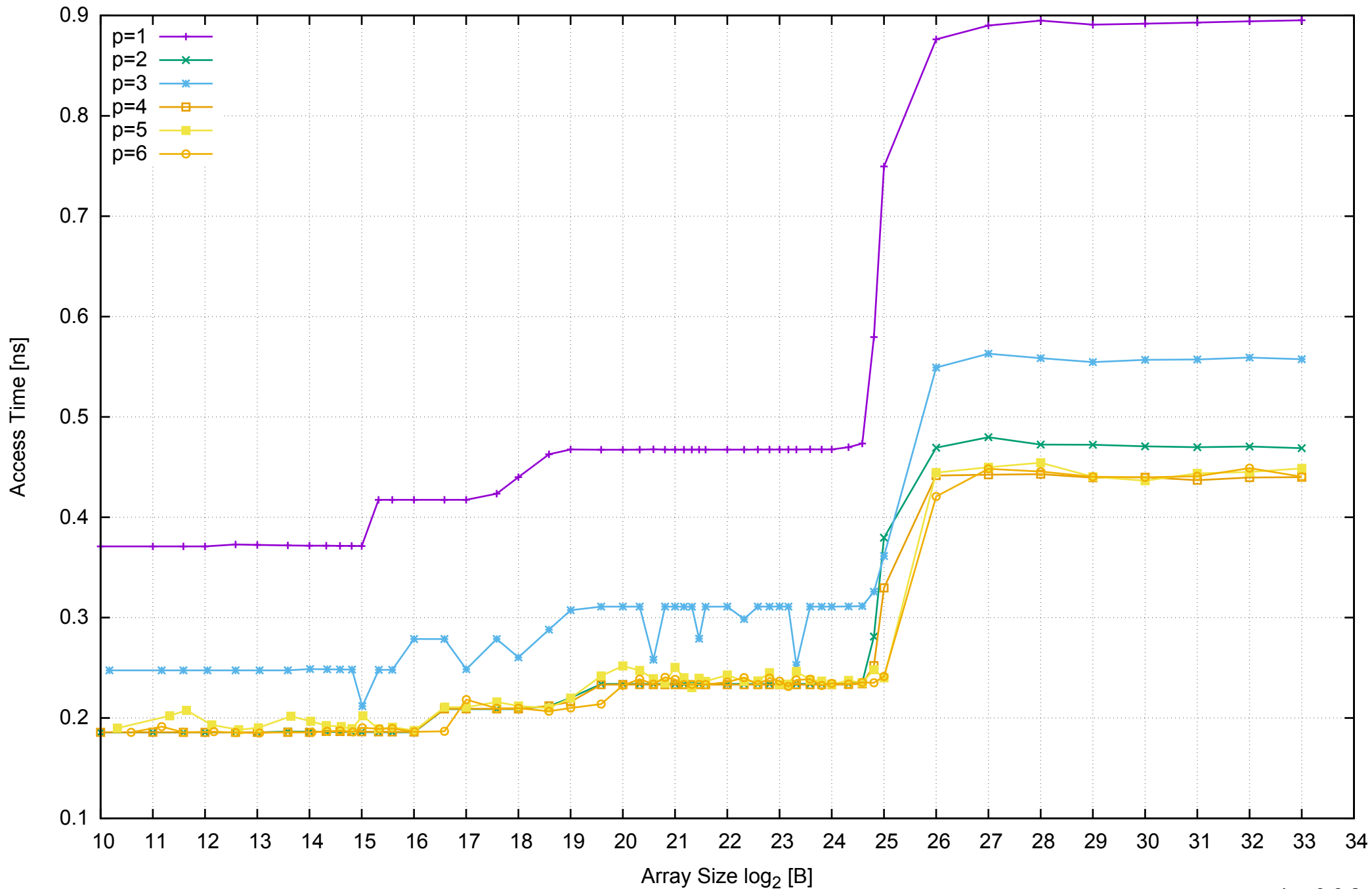
AWS m4.xlarge - Intel Xeon E5-2676 v3, 2.40 GHz 16GB - Parallel Memory Access Time - ScanWrite64PtrUnrollLoop
