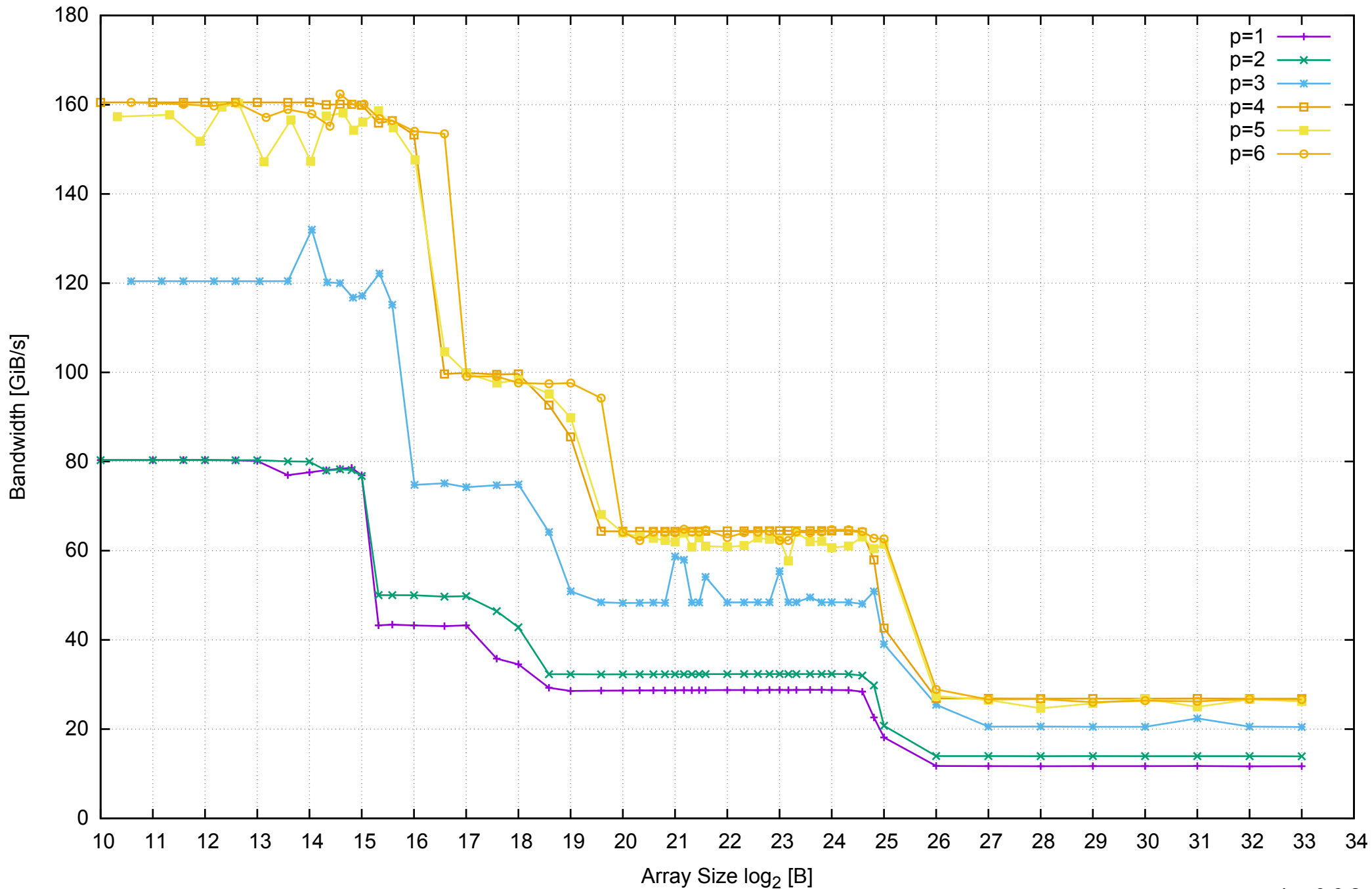
AWS m4.xlarge - Intel Xeon E5-2676 v3, 2.40 GHz 16GB - Parallel Memory Bandwidth - ScanRead128PtrUnrollLoop
