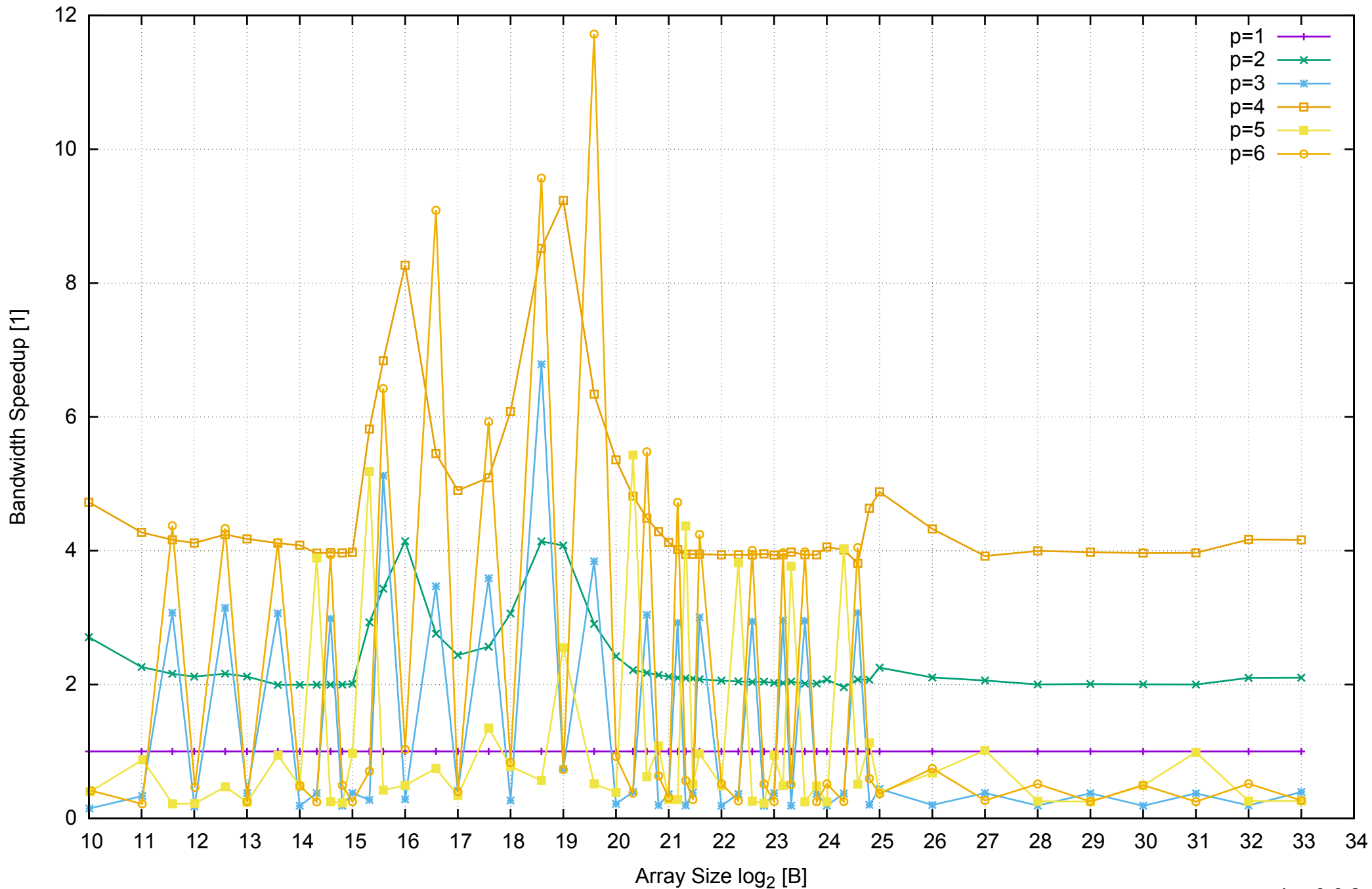
AWS m4.xlarge - Intel Xeon E5-2676 v3, 2.40 GHz 16GB - Speedup of Parallel Memory Bandwidth - PermRead64UnrollLoop
