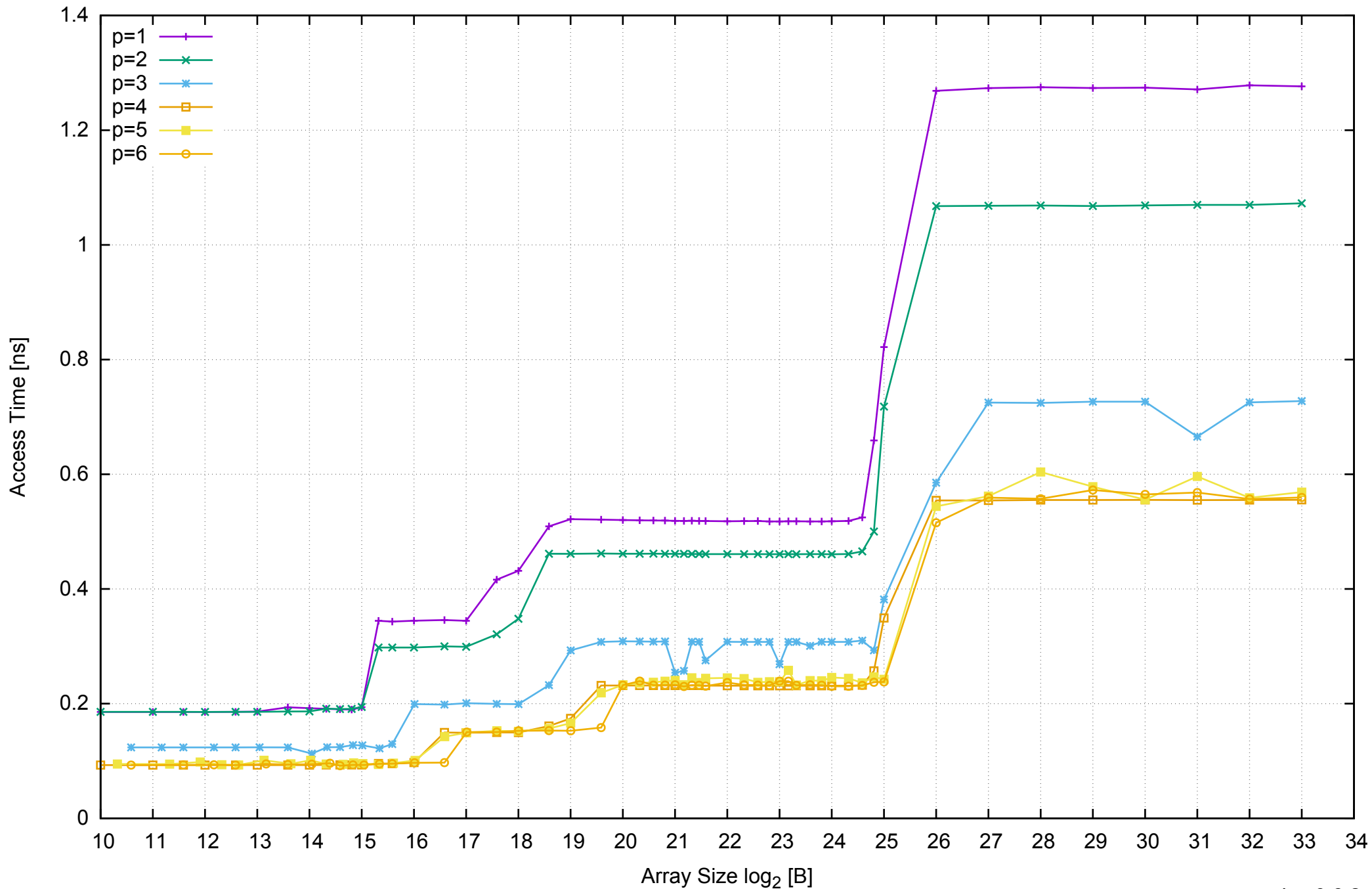
AWS m4.xlarge - Intel Xeon E5-2676 v3, 2.40 GHz 16GB - Parallel Memory Access Time - ScanRead128PtrUnrollLoop
