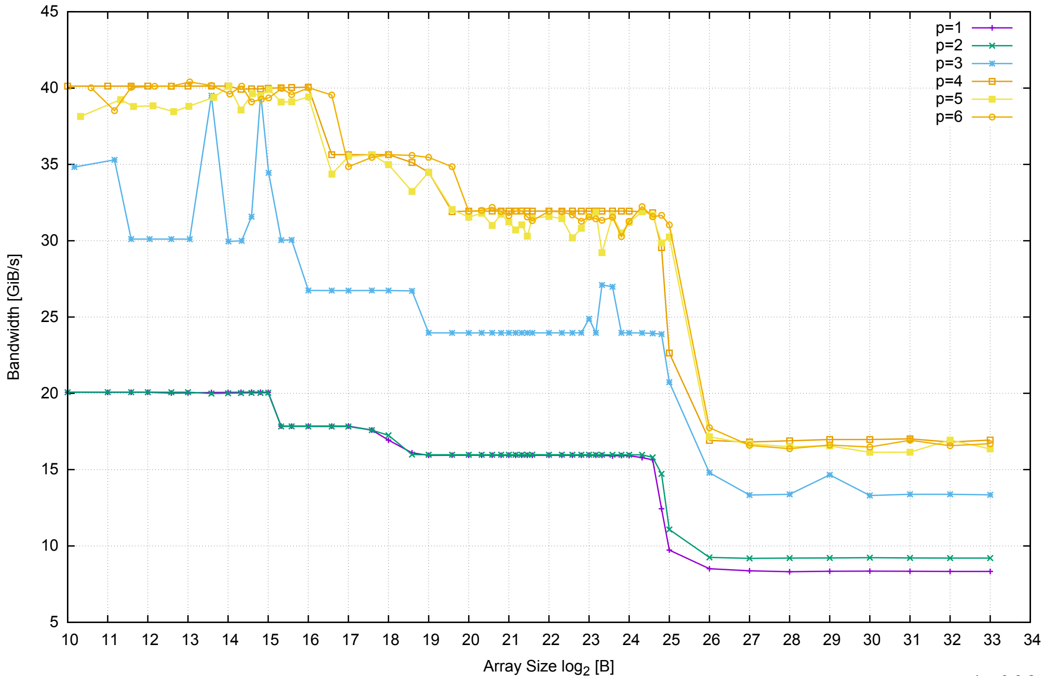
AWS m4.xlarge - Intel Xeon E5-2676 v3, 2.40 GHz 16GB - Parallel Memory Bandwidth - ScanWrite64IndexUnrollLoop
