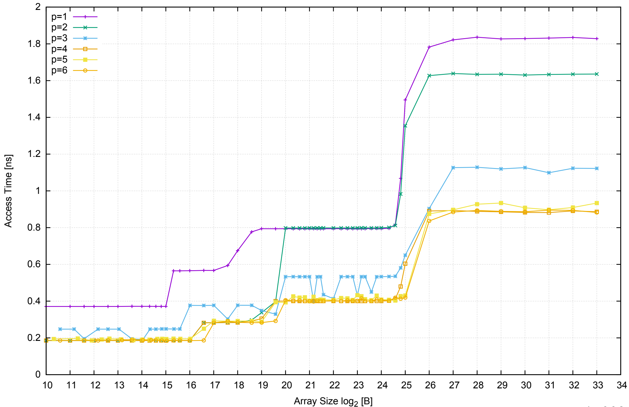
AWS m4.xlarge - Intel Xeon E5-2676 v3, 2.40 GHz 16GB - Parallel Memory Access Time - ScanWrite128PtrUnrollLoop
