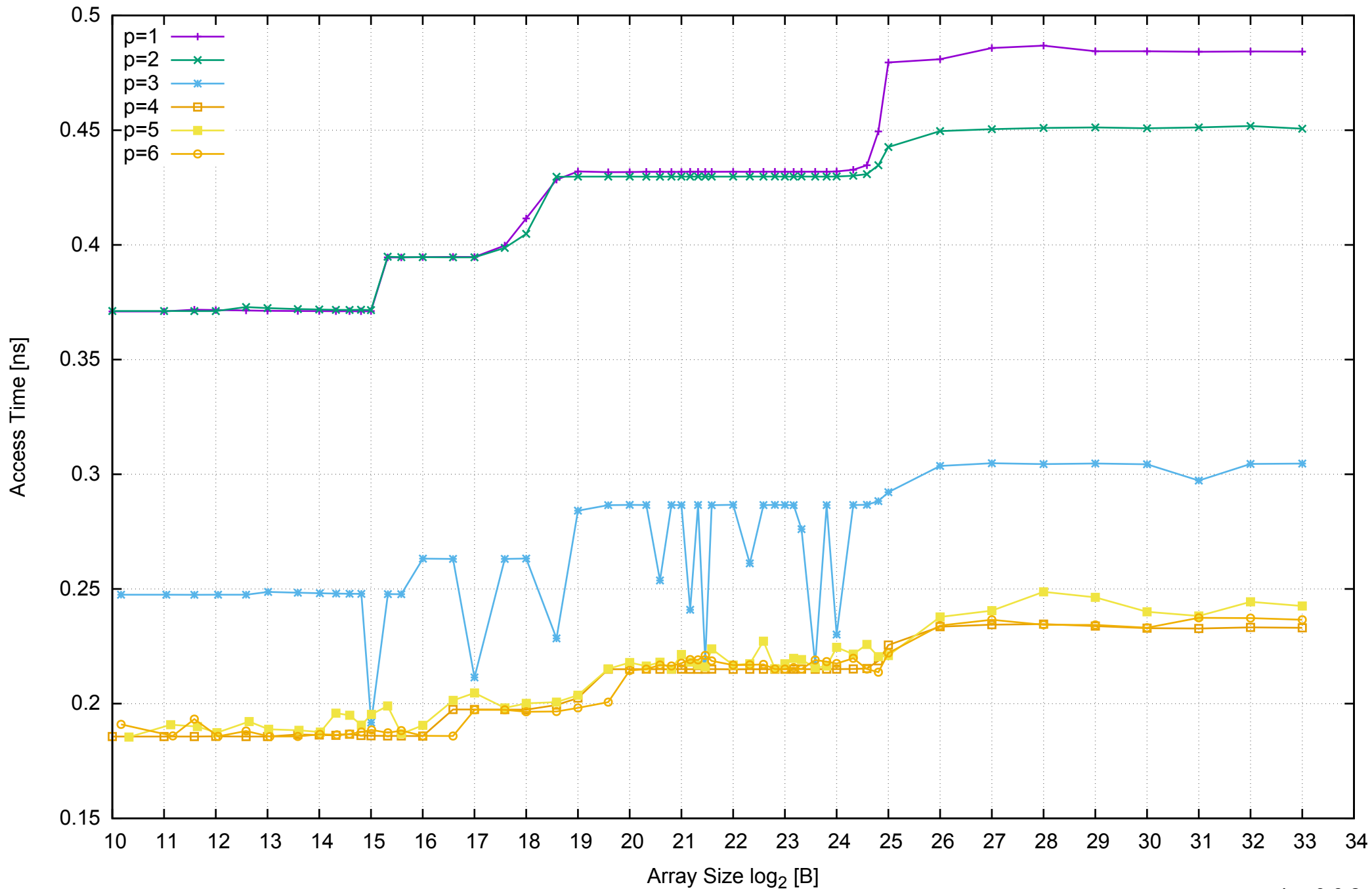
AWS m4.xlarge - Intel Xeon E5-2676 v3, 2.40 GHz 16GB - Parallel Memory Access Time - ScanWrite32PtrUnrollLoop
