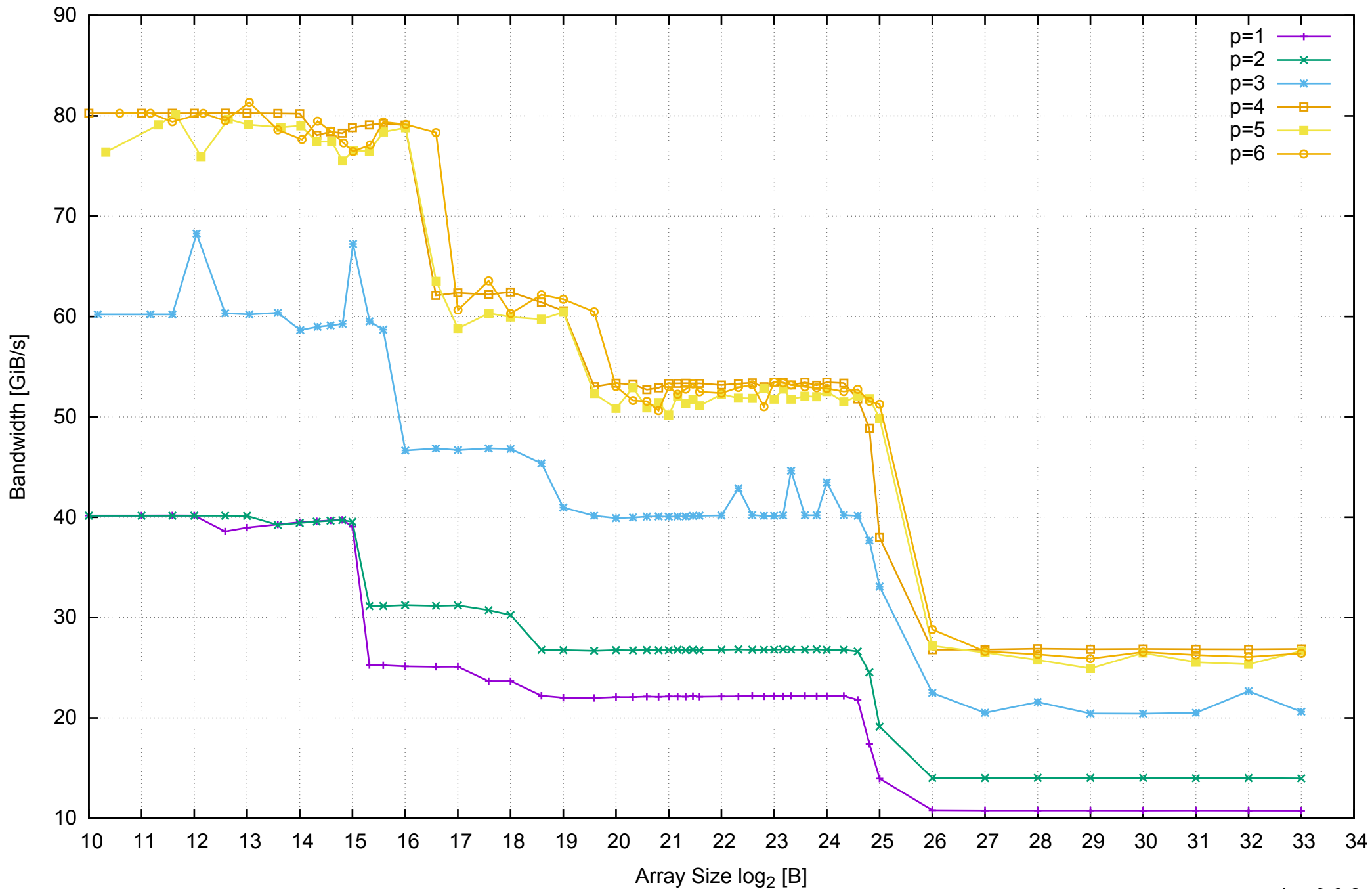
AWS m4.xlarge - Intel Xeon E5-2676 v3, 2.40 GHz 16GB - Parallel Memory Bandwidth - ScanRead64IndexUnrollLoop
