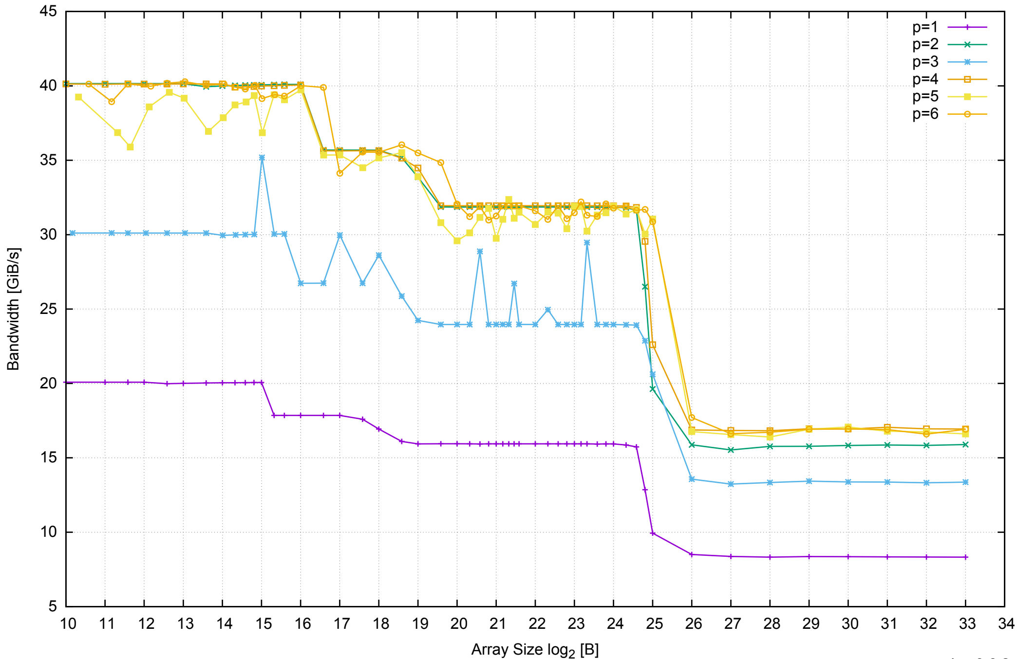
AWS m4.xlarge - Intel Xeon E5-2676 v3, 2.40 GHz 16GB - Parallel Memory Bandwidth - ScanWrite64PtrUnrollLoop
