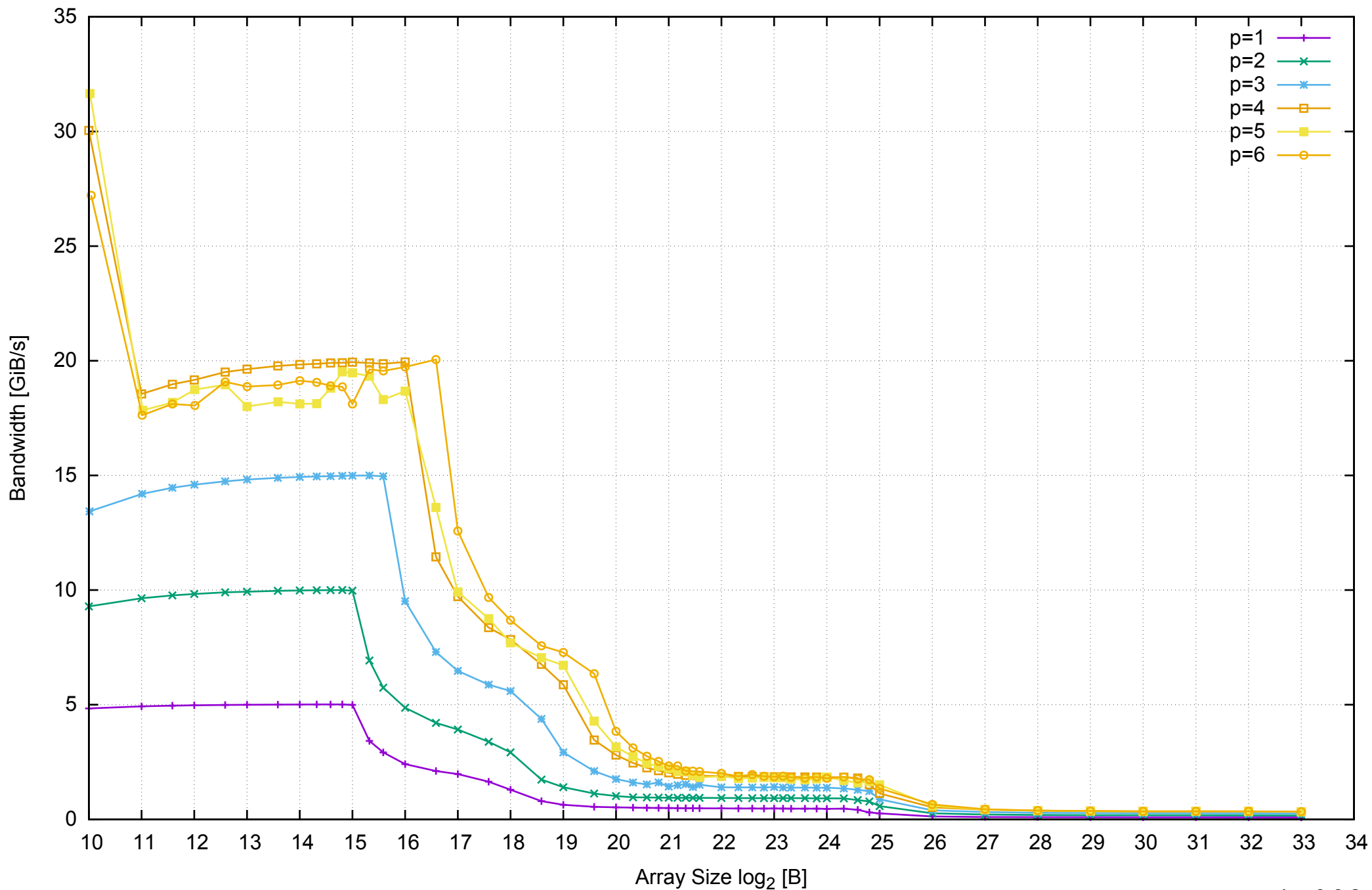
AWS m4.xlarge - Intel Xeon E5-2676 v3, 2.40 GHz 16GB - Parallel Memory Bandwidth - PermRead64SimpleLoop
