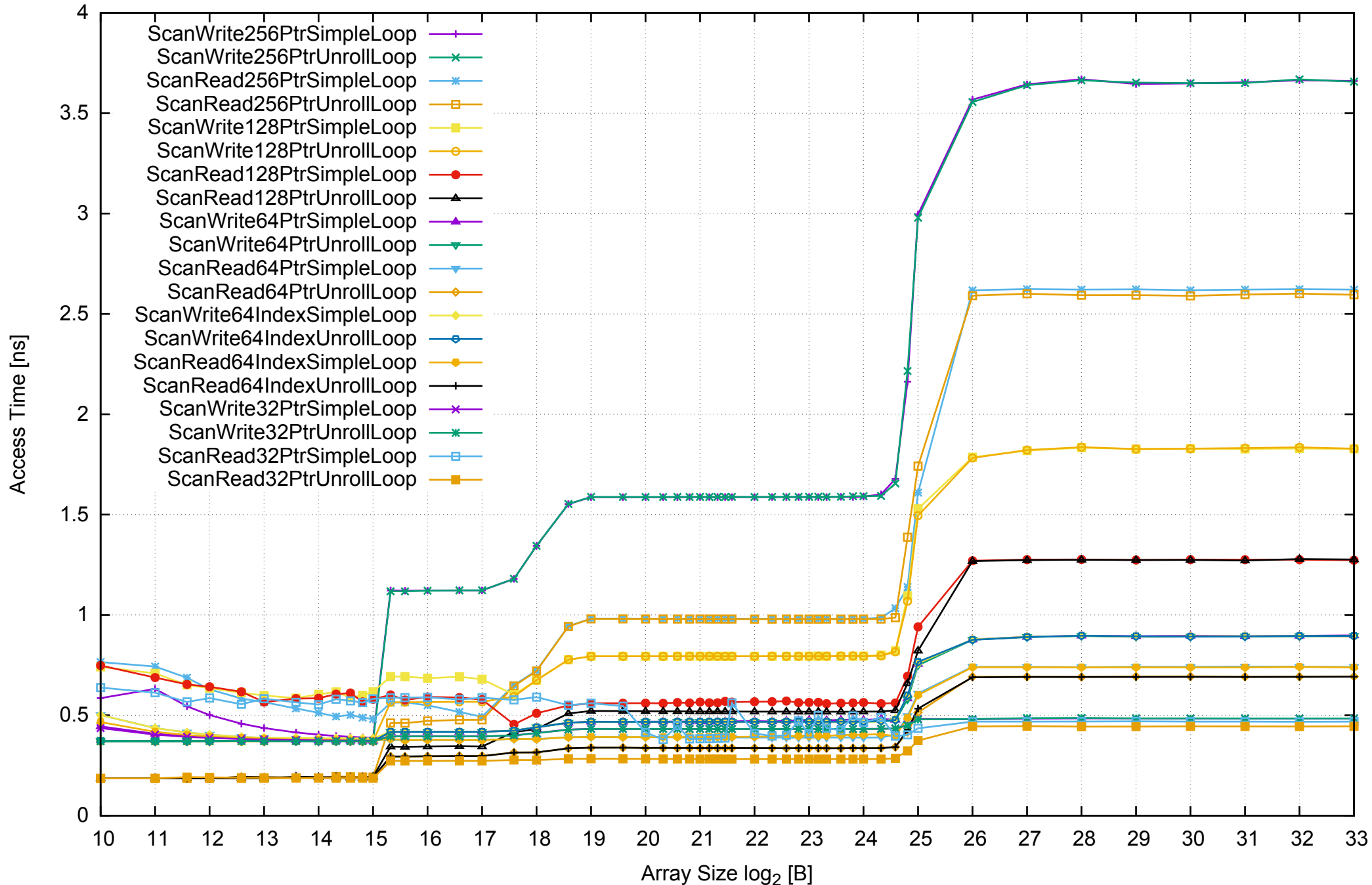
AWS m4.xlarge - Intel Xeon E5-2676 v3, 2.40 GHz 16GB - One Thread Memory Latency (excluding Permutation)
