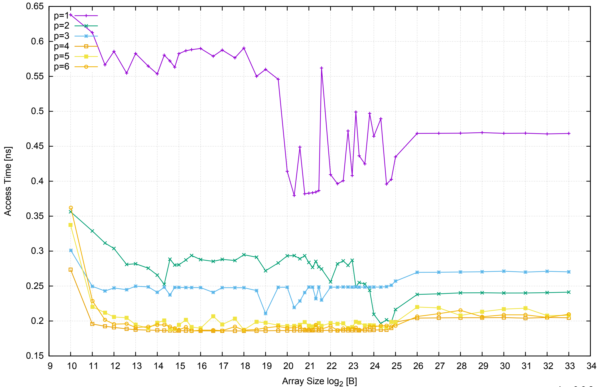
AWS m4.xlarge - Intel Xeon E5-2676 v3, 2.40 GHz 16GB - Parallel Memory Access Time - ScanRead32PtrSimpleLoop
