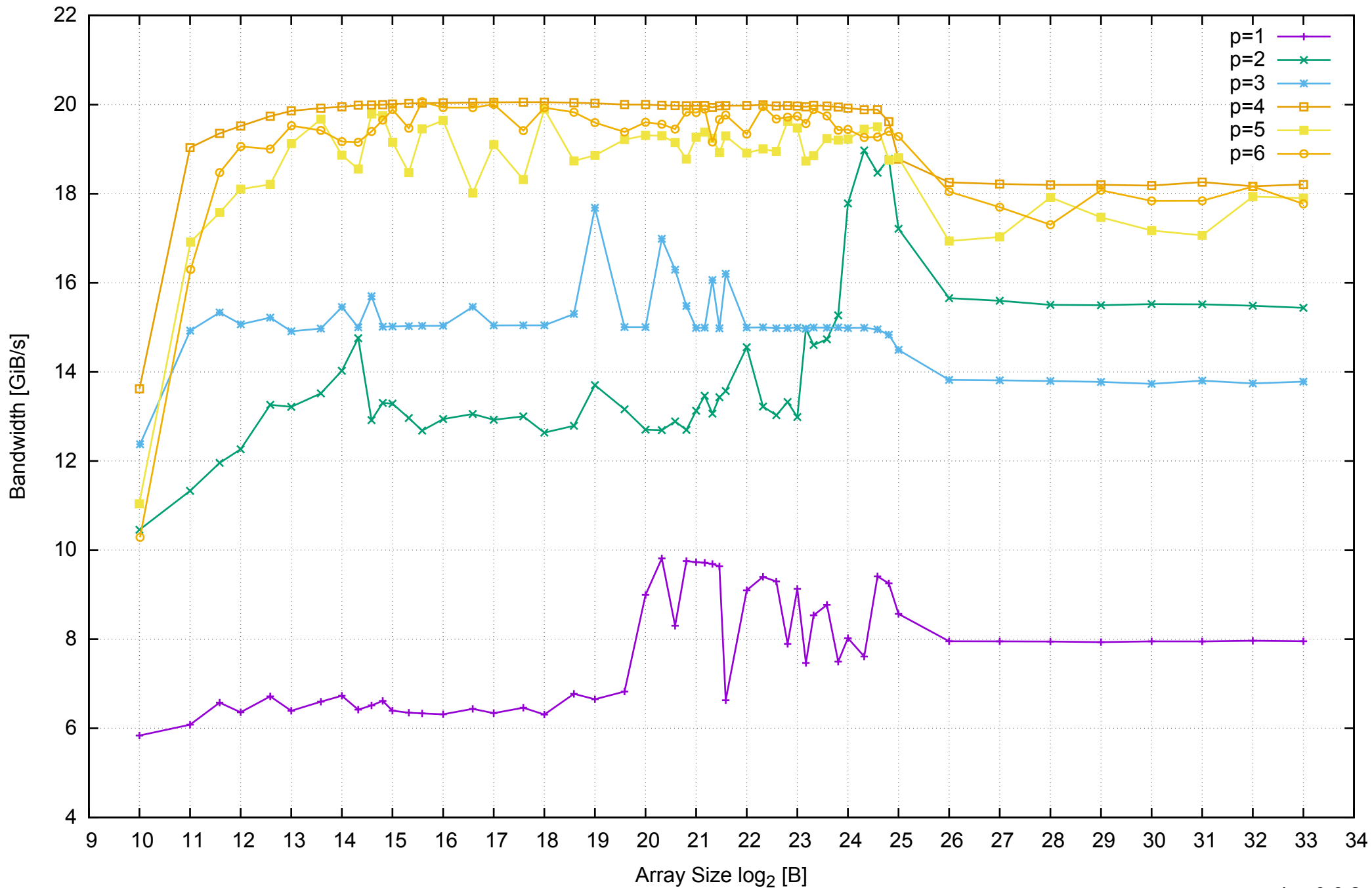
AWS m4.xlarge - Intel Xeon E5-2676 v3, 2.40 GHz 16GB - Parallel Memory Bandwidth - ScanRead32PtrSimpleLoop
