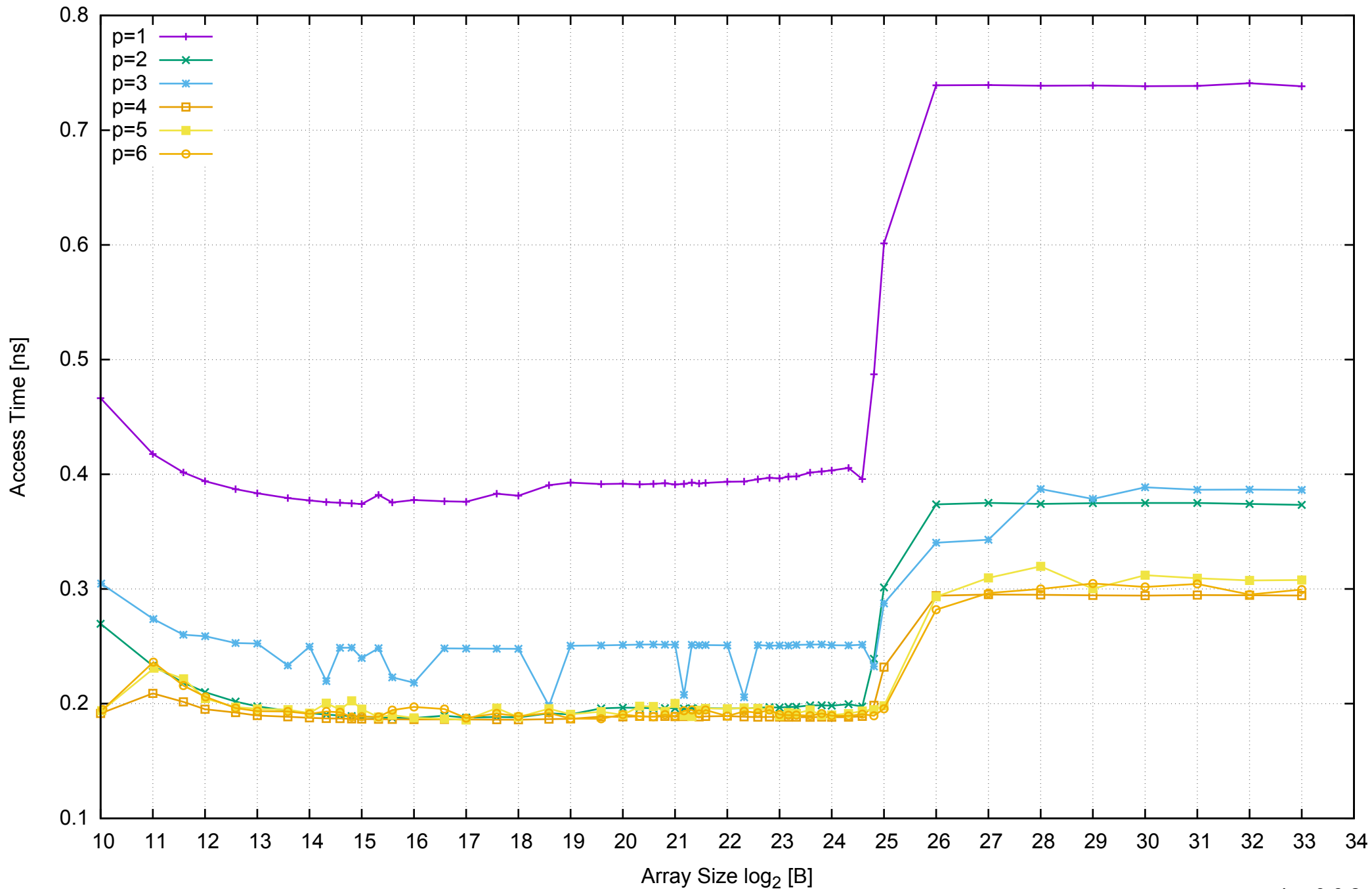
AWS m4.xlarge - Intel Xeon E5-2676 v3, 2.40 GHz 16GB - Parallel Memory Access Time - ScanRead64IndexSimpleLoop
