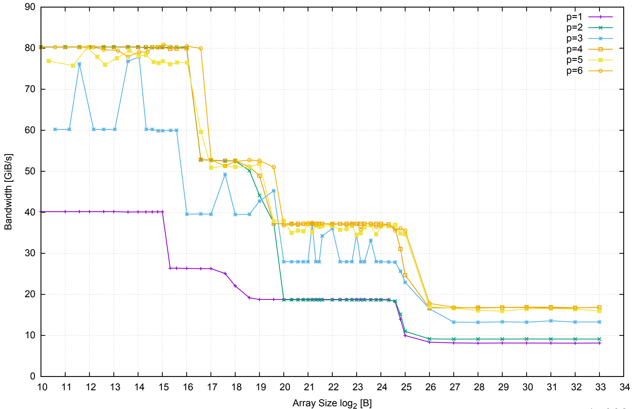
AWS m4.xlarge - Intel Xeon E5-2676 v3, 2.40 GHz 16GB - Parallel Memory Bandwidth - ScanWrite128PtrUnrollLoop
