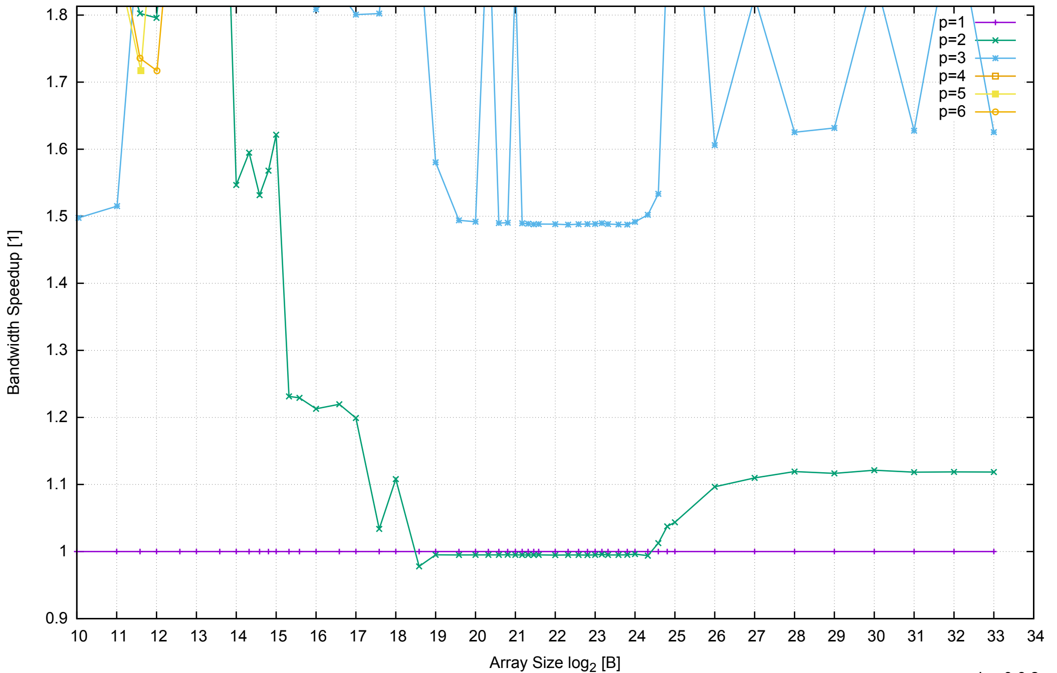
AWS m4.xlarge - Intel Xeon E5-2676 v3, 2.40 GHz 16GB - Speedup of Parallel Memory Bandwidth (enlarged) - ScanWrite128PtrSimpleLoop
