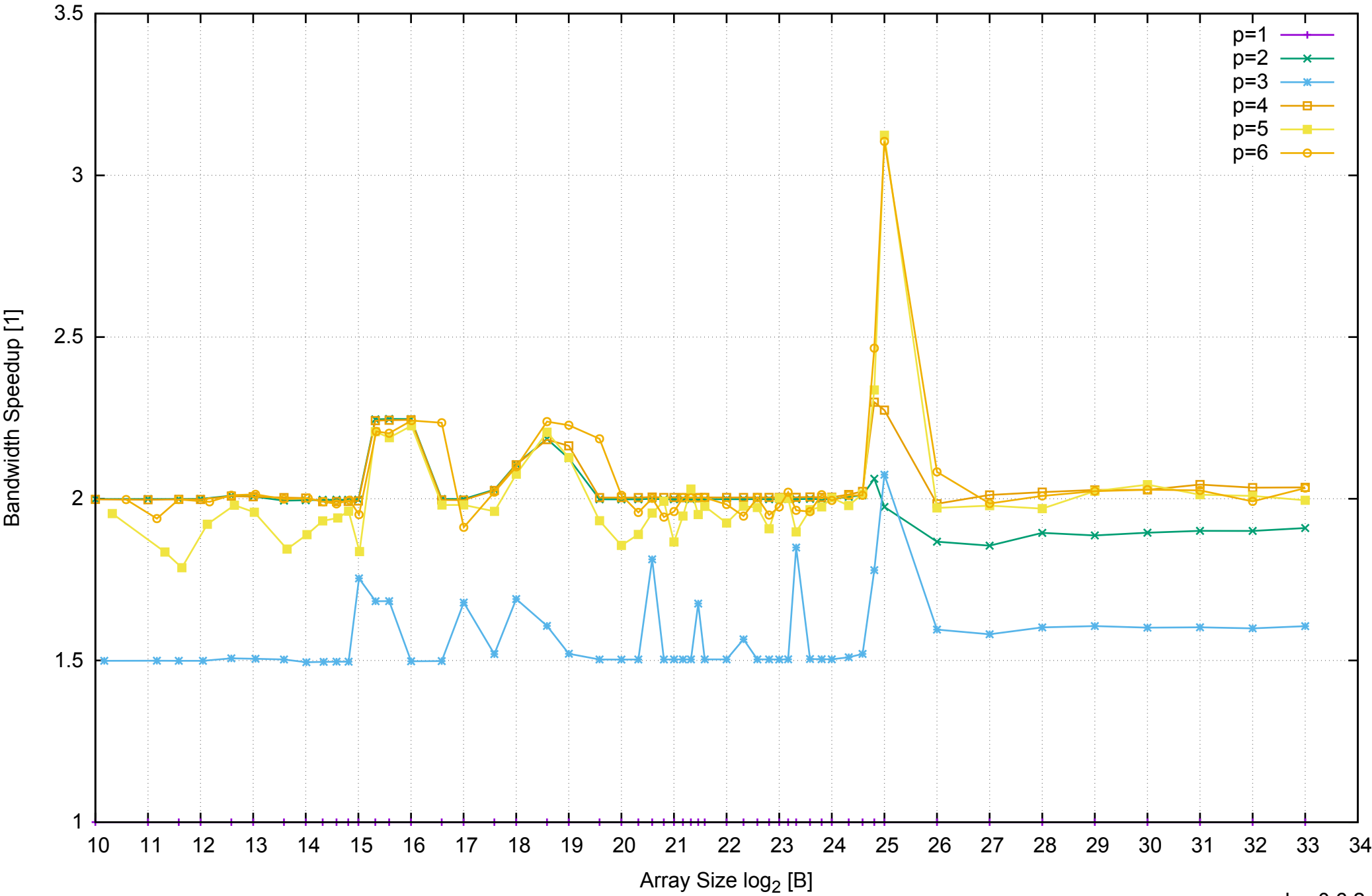
AWS m4.xlarge - Intel Xeon E5-2676 v3, 2.40 GHz 16GB - Speedup of Parallel Memory Bandwidth - ScanWrite64PtrUnrollLoop
