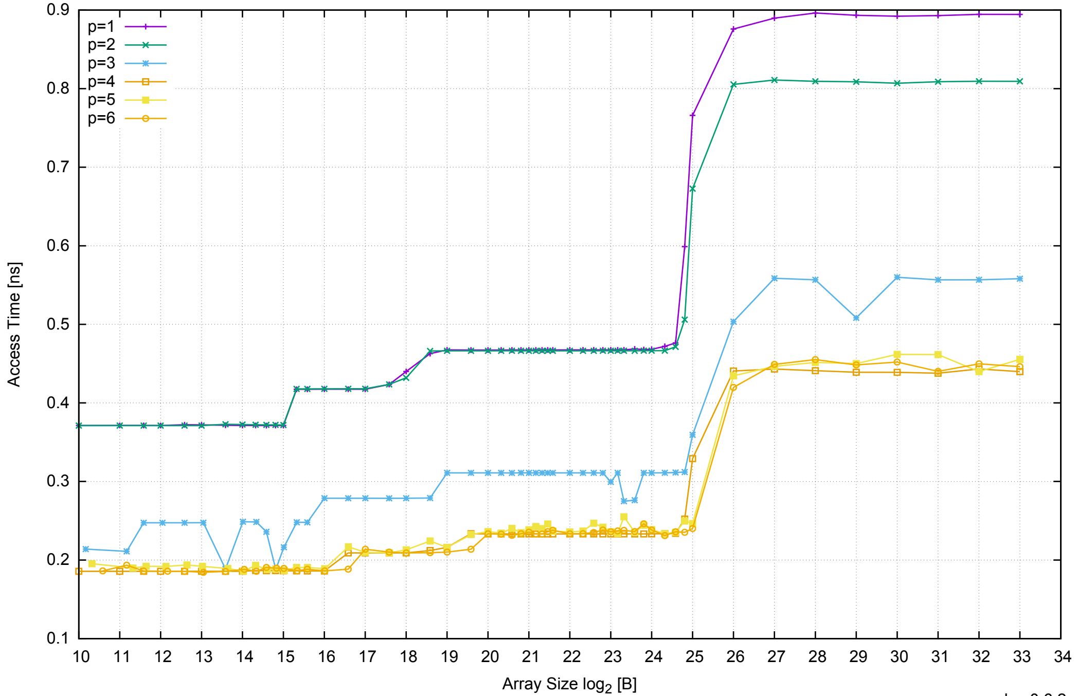
AWS m4.xlarge - Intel Xeon E5-2676 v3, 2.40 GHz 16GB - Parallel Memory Access Time - ScanWrite64IndexUnrollLoop
