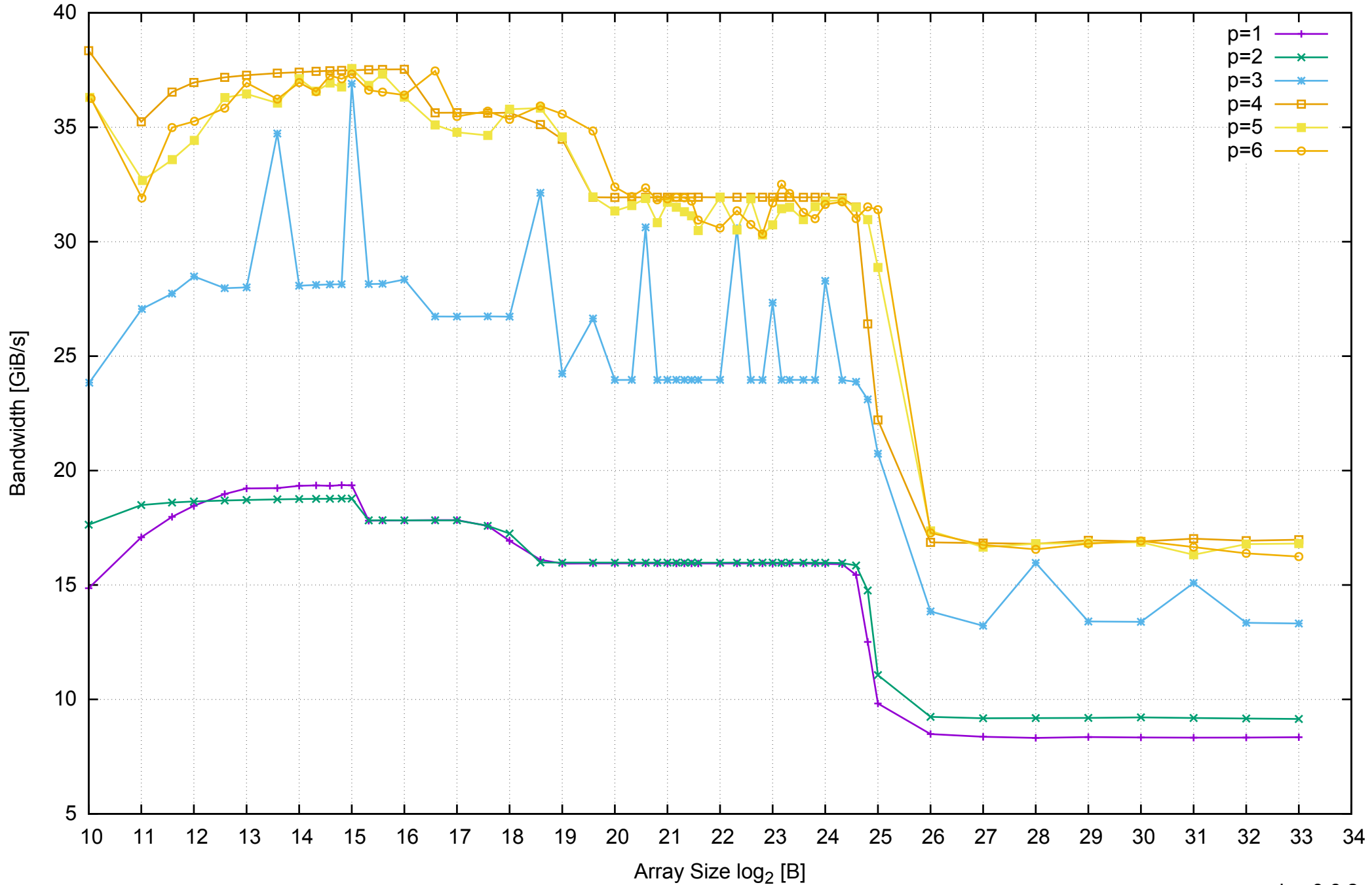
AWS m4.xlarge - Intel Xeon E5-2676 v3, 2.40 GHz 16GB - Parallel Memory Bandwidth - ScanWrite64IndexSimpleLoop
