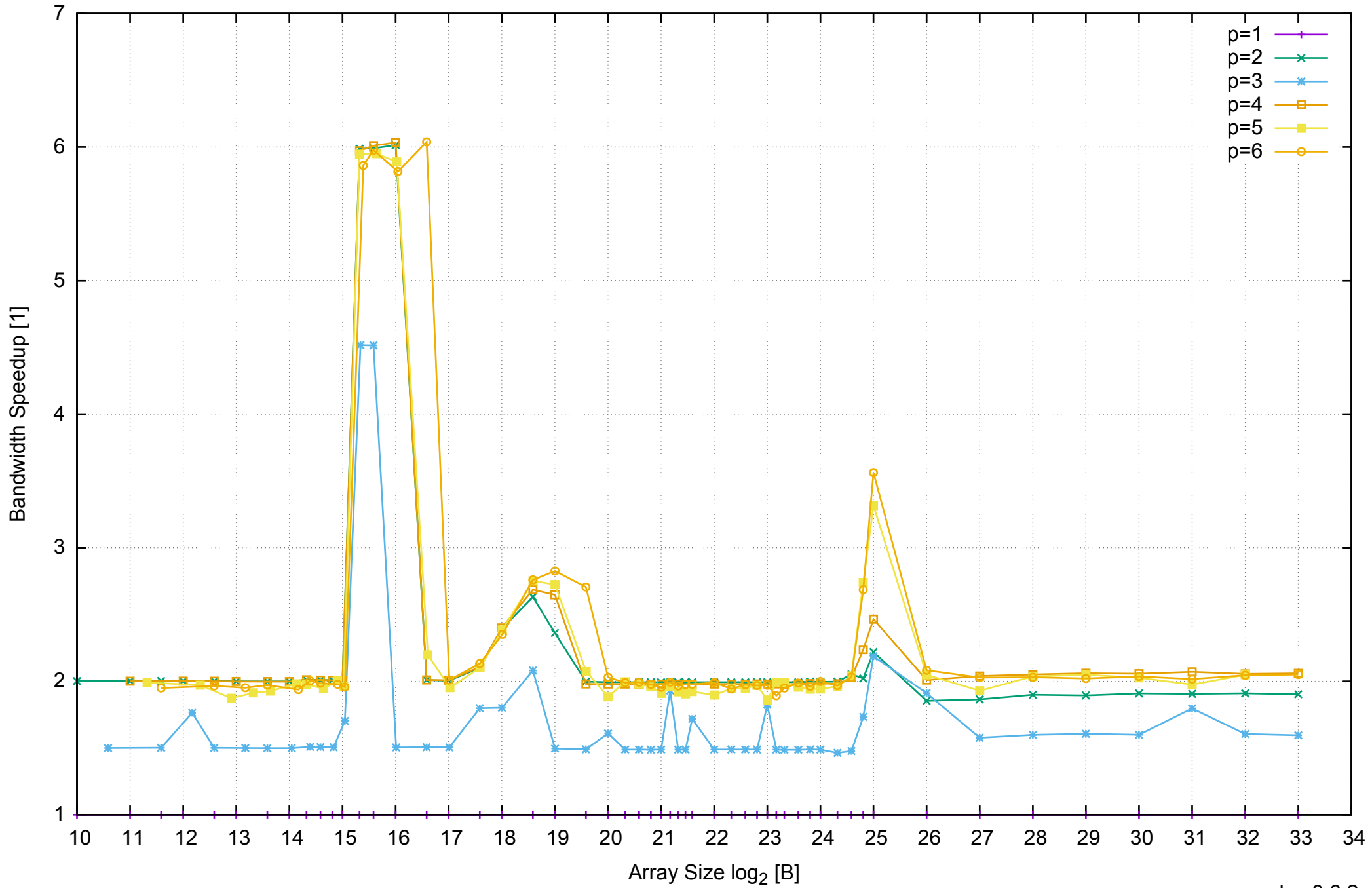
AWS m4.xlarge - Intel Xeon E5-2676 v3, 2.40 GHz 16GB - Speedup of Parallel Memory Bandwidth - ScanWrite256PtrUnrollLoop
