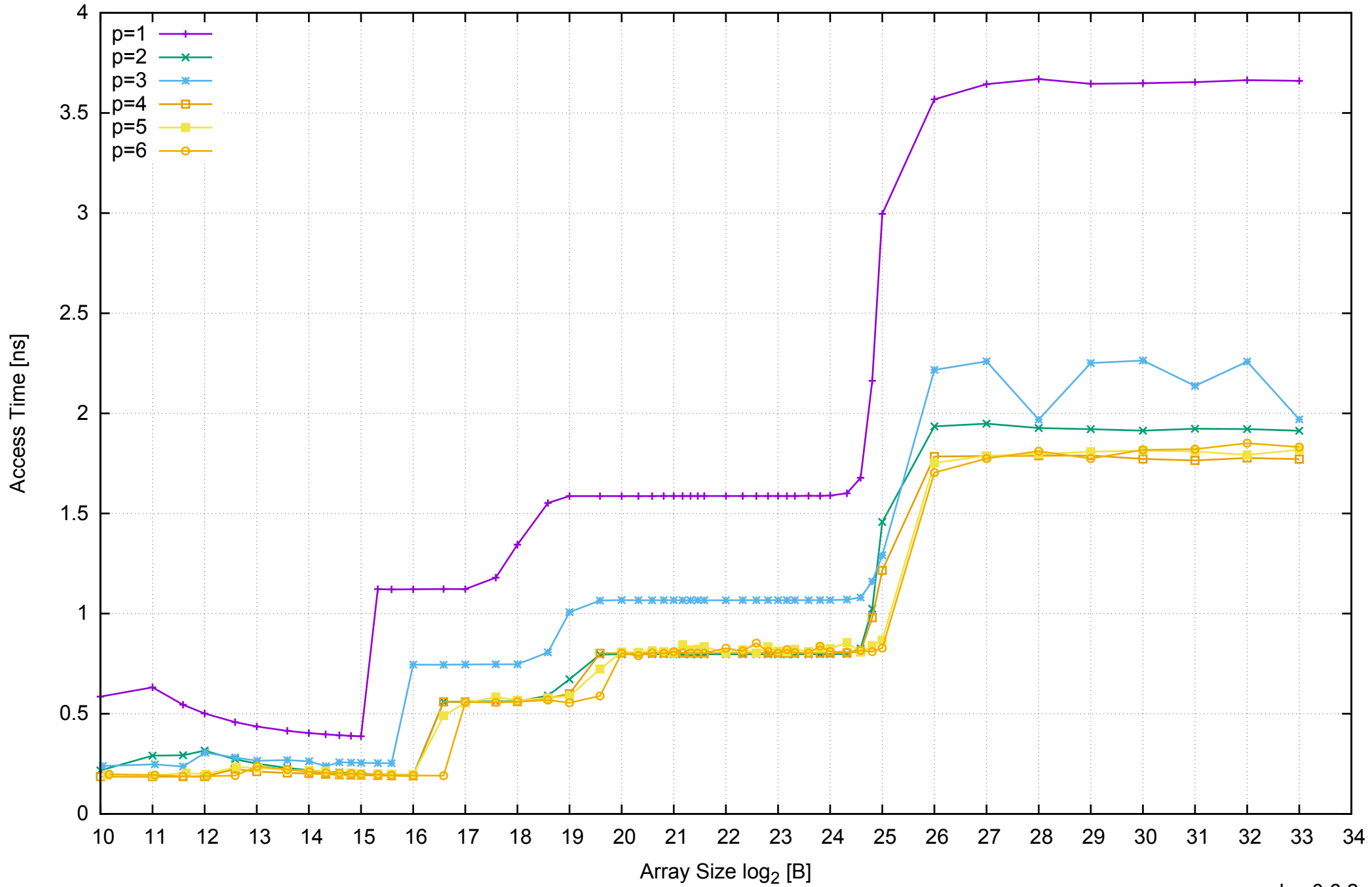
AWS m4.xlarge - Intel Xeon E5-2676 v3, 2.40 GHz 16GB - Parallel Memory Access Time - ScanWrite256PtrSimpleLoop
