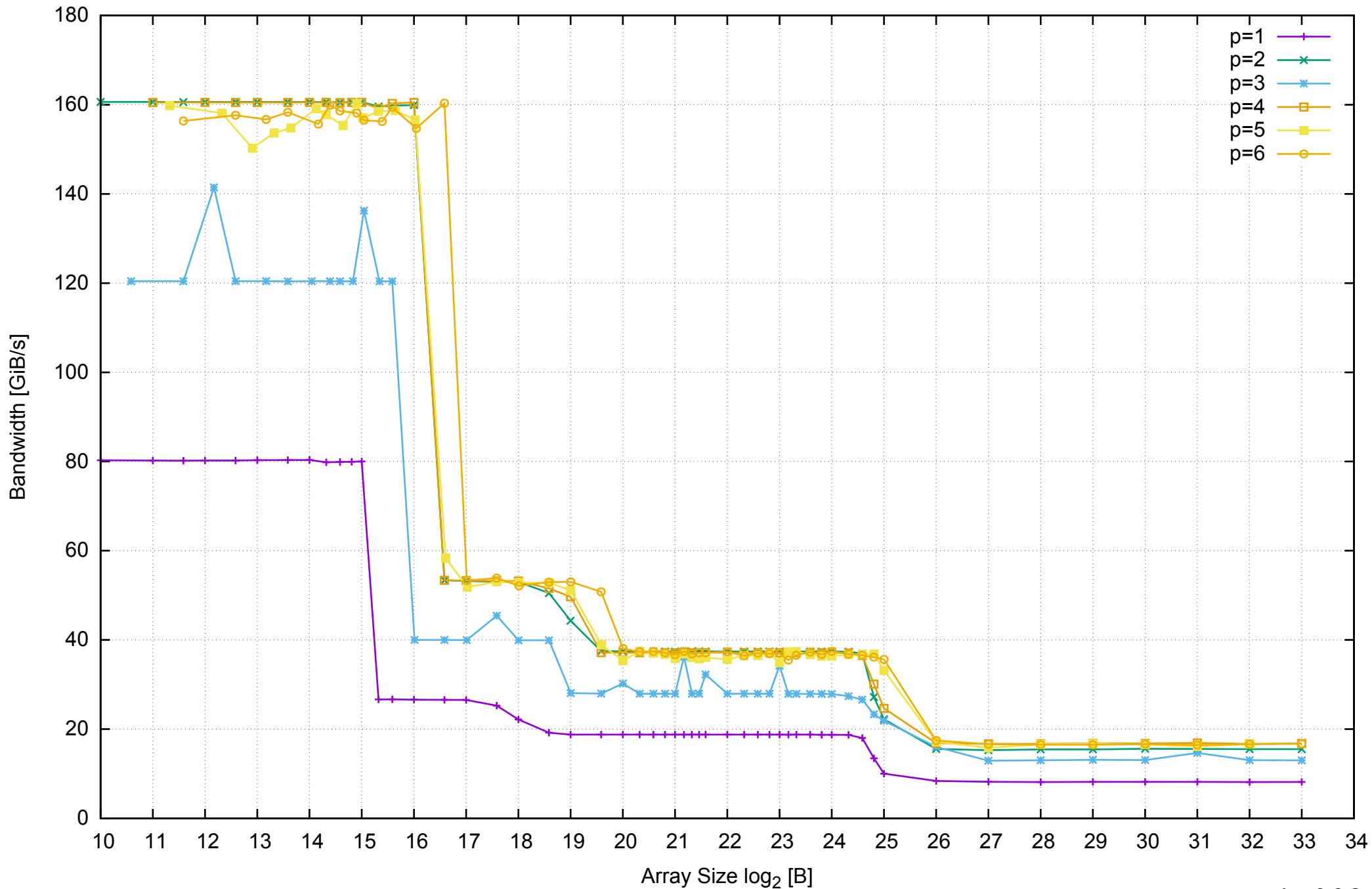
AWS m4.xlarge - Intel Xeon E5-2676 v3, 2.40 GHz 16GB - Parallel Memory Bandwidth - ScanWrite256PtrUnrollLoop
