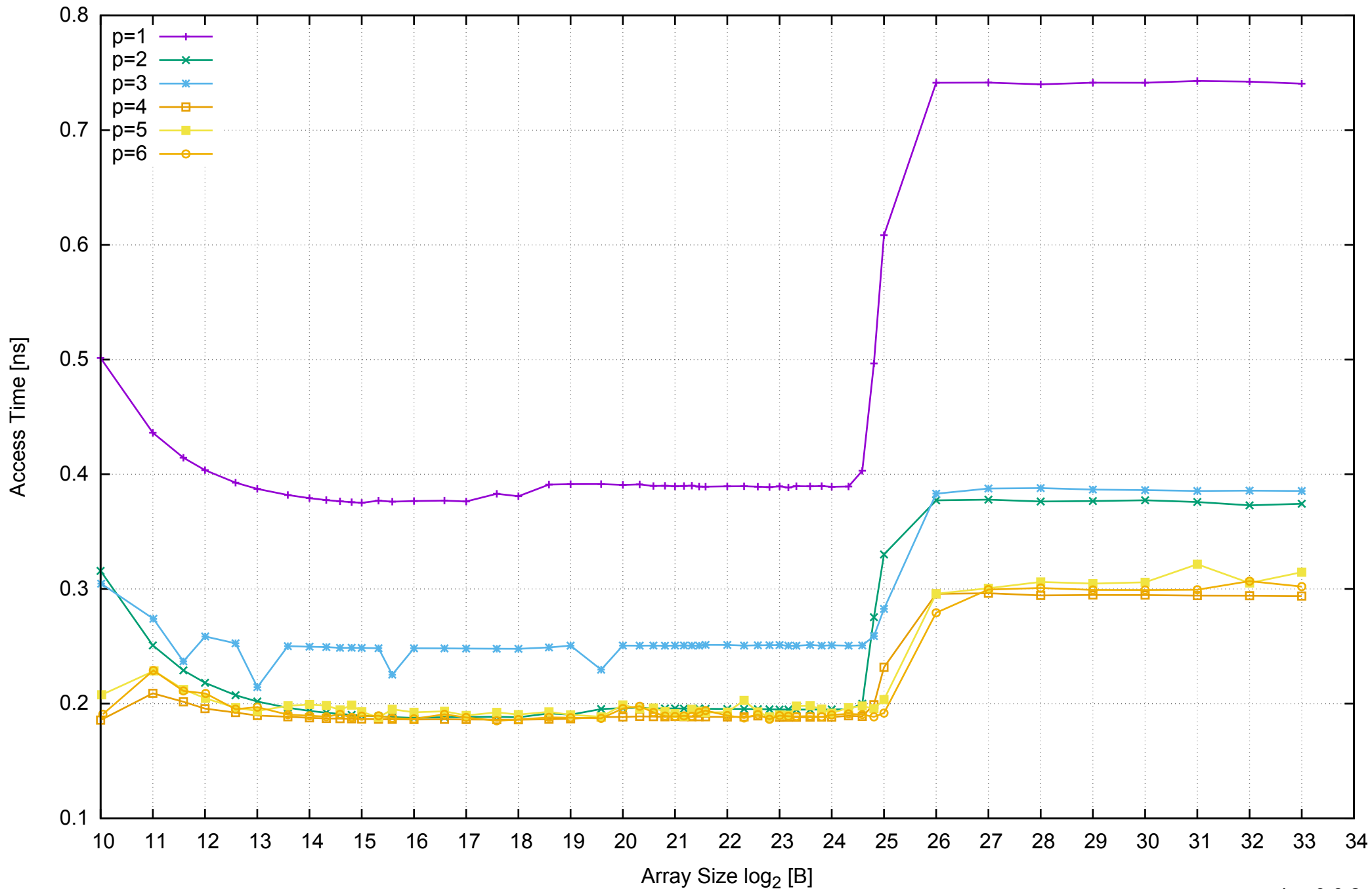
AWS m4.xlarge - Intel Xeon E5-2676 v3, 2.40 GHz 16GB - Parallel Memory Access Time - ScanRead64PtrSimpleLoop
