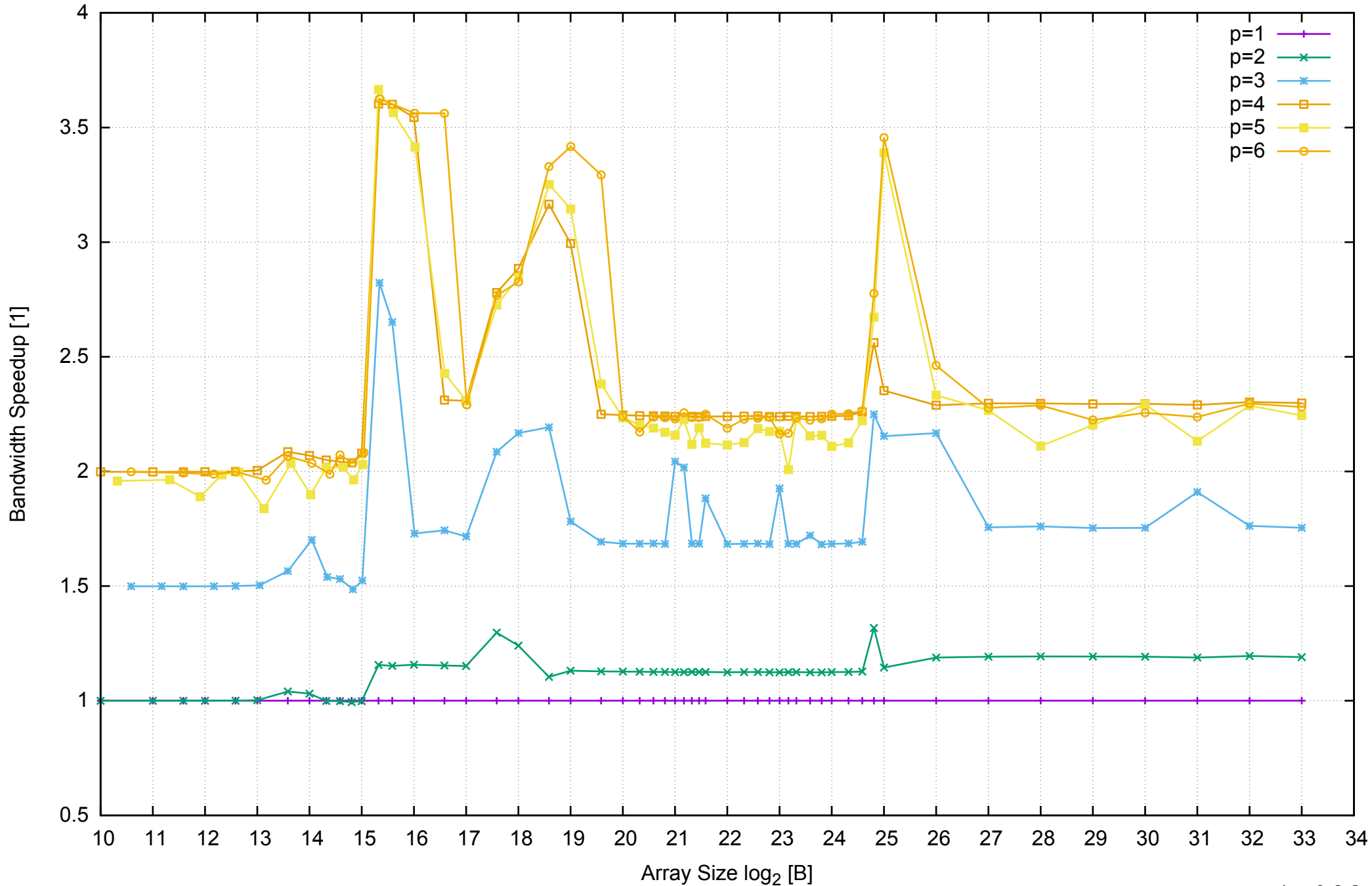
AWS m4.xlarge - Intel Xeon E5-2676 v3, 2.40 GHz 16GB - Speedup of Parallel Memory Bandwidth - ScanRead128PtrUnrollLoop
