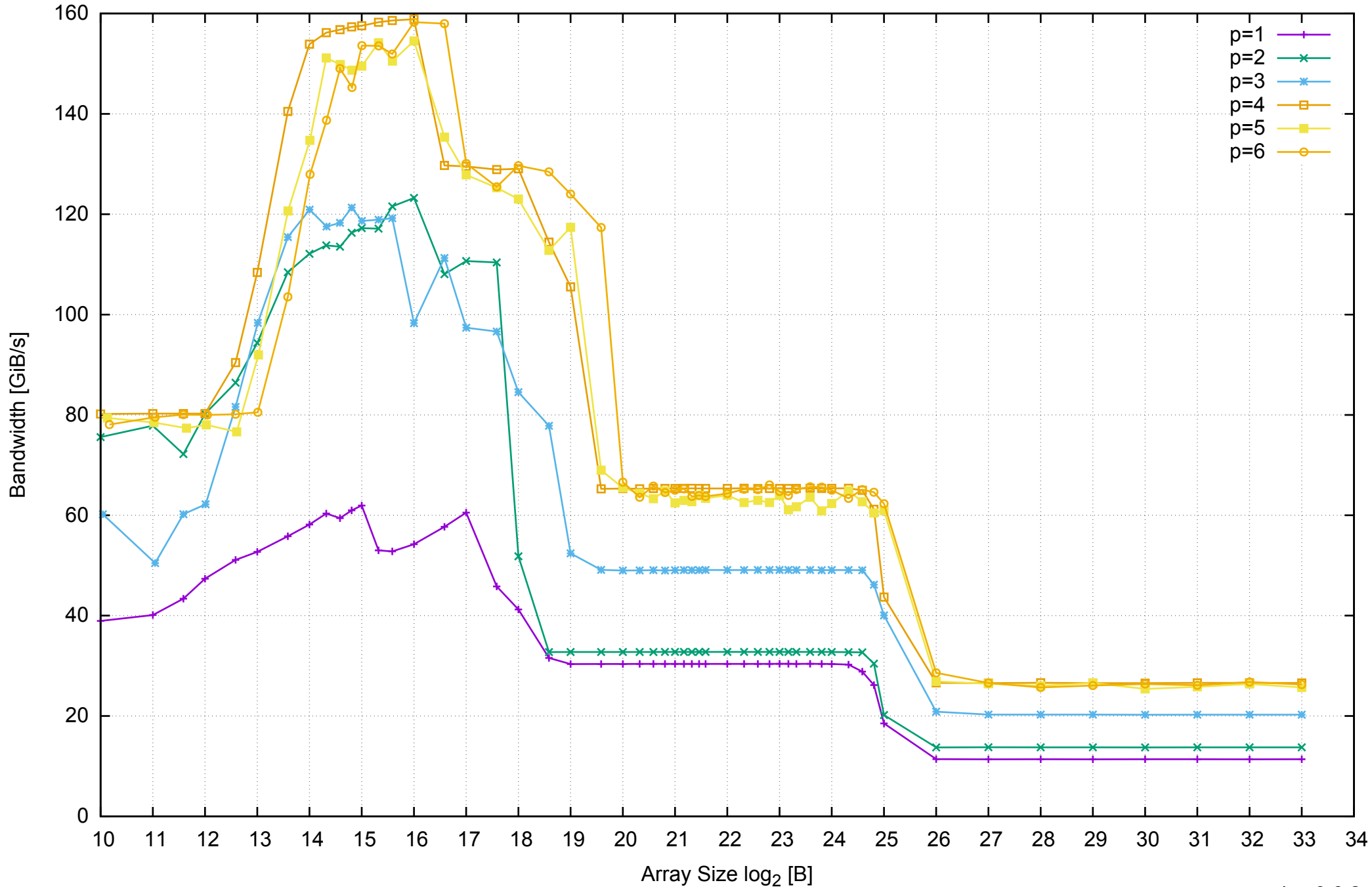
AWS m4.xlarge - Intel Xeon E5-2676 v3, 2.40 GHz 16GB - Parallel Memory Bandwidth - ScanRead256PtrSimpleLoop
