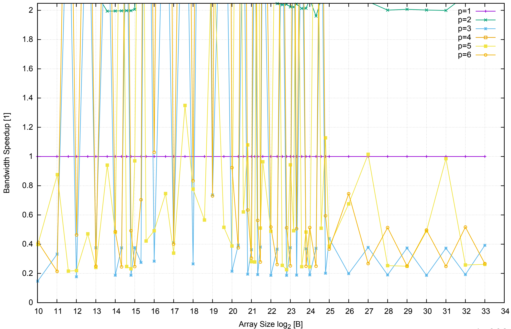
AWS m4.xlarge - Intel Xeon E5-2676 v3, 2.40 GHz 16GB - Speedup of Parallel Memory Bandwidth (enlarged) - PermRead64UnrollLoop
