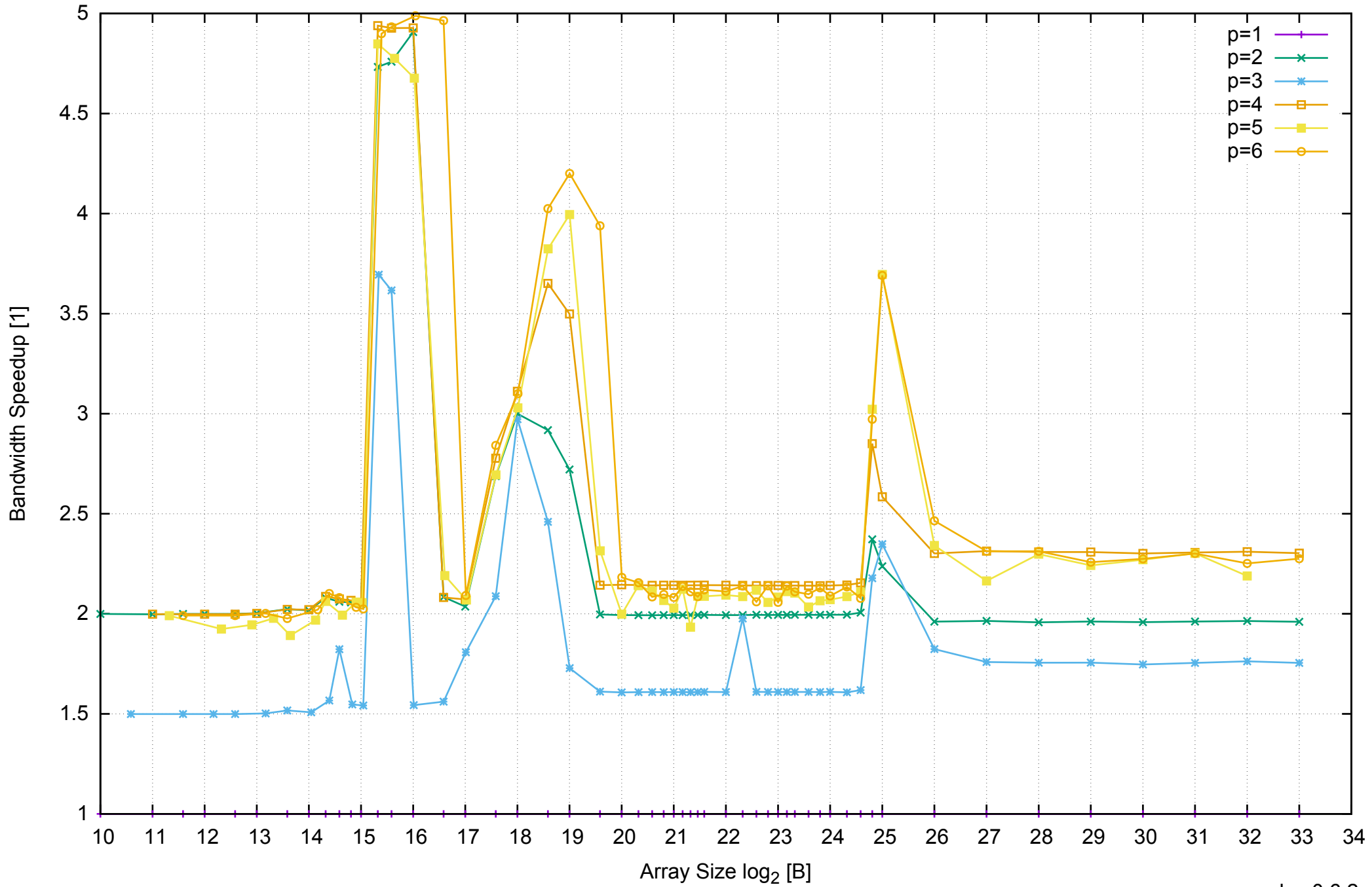
AWS m4.xlarge - Intel Xeon E5-2676 v3, 2.40 GHz 16GB - Speedup of Parallel Memory Bandwidth - ScanRead256PtrUnrollLoop
