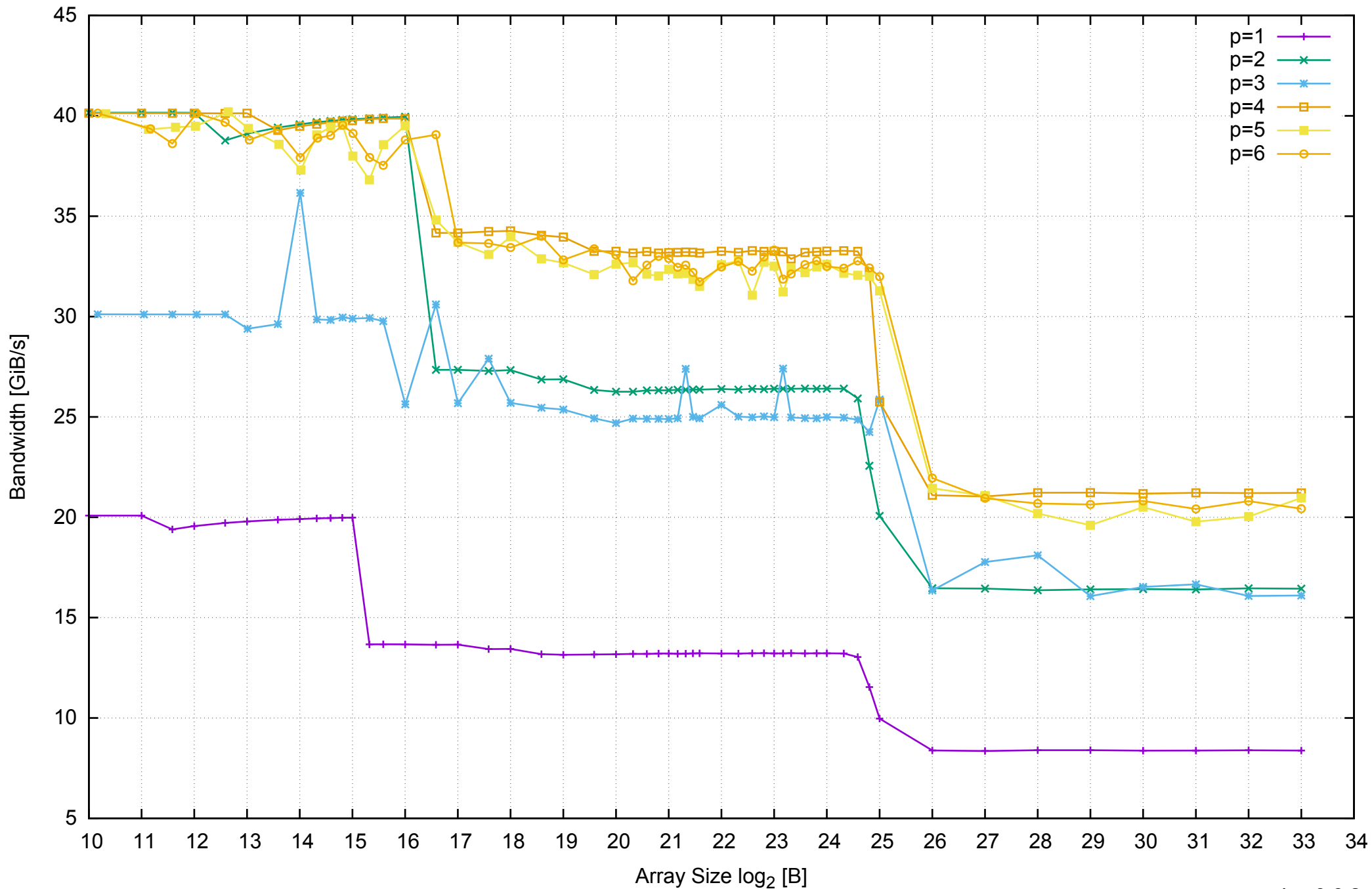
AWS m4.xlarge - Intel Xeon E5-2676 v3, 2.40 GHz 16GB - Parallel Memory Bandwidth - ScanRead32PtrUnrollLoop
