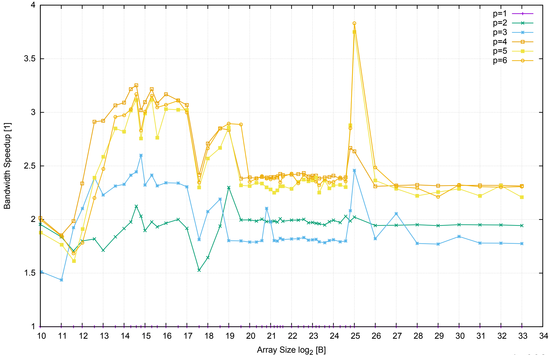
AWS m4.xlarge - Intel Xeon E5-2676 v3, 2.40 GHz 16GB - Speedup of Parallel Memory Bandwidth - ScanRead128PtrSimpleLoop
