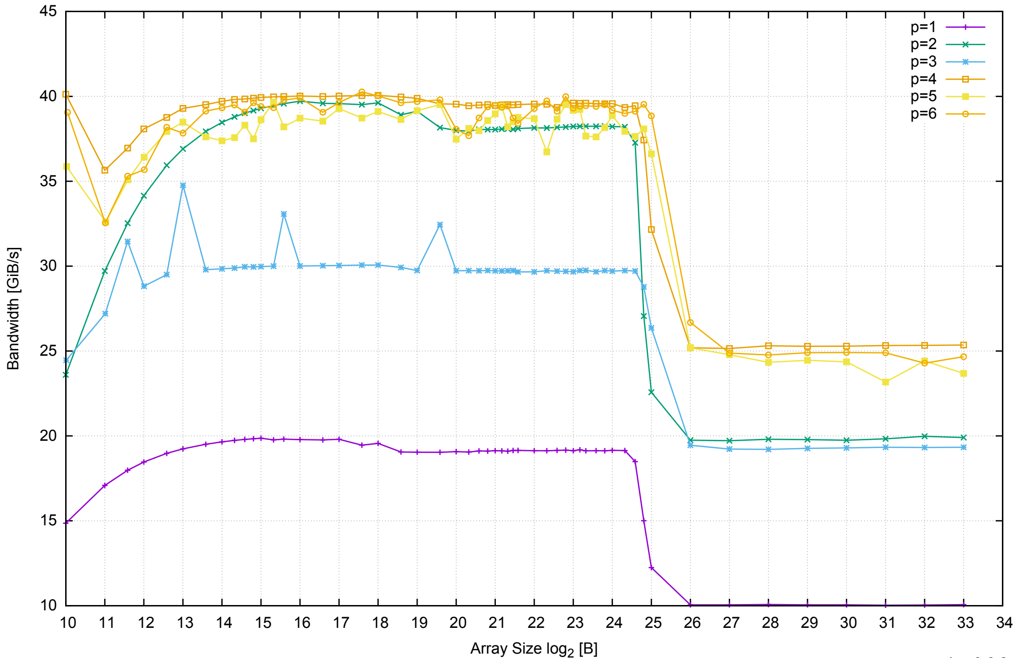
AWS m4.xlarge - Intel Xeon E5-2676 v3, 2.40 GHz 16GB - Parallel Memory Bandwidth - ScanRead64PtrSimpleLoop
