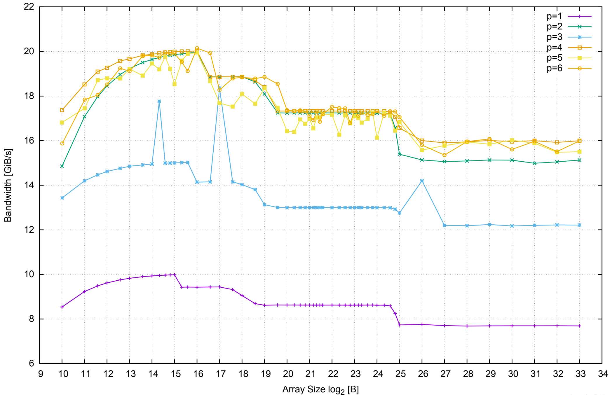
AWS m4.xlarge - Intel Xeon E5-2676 v3, 2.40 GHz 16GB - Parallel Memory Bandwidth - ScanWrite32PtrSimpleLoop
