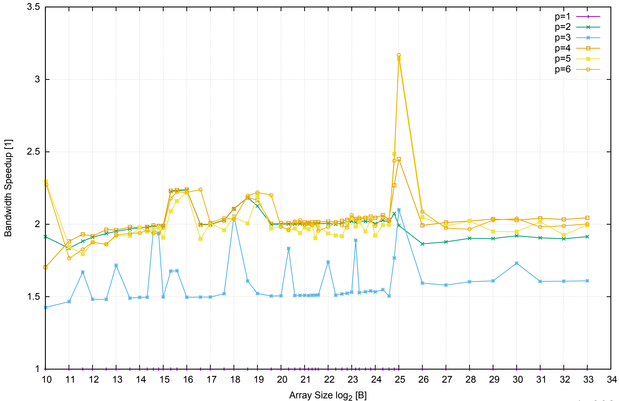
AWS m4.xlarge - Intel Xeon E5-2676 v3, 2.40 GHz 16GB - Speedup of Parallel Memory Bandwidth - ScanWrite64PtrSimpleLoop
