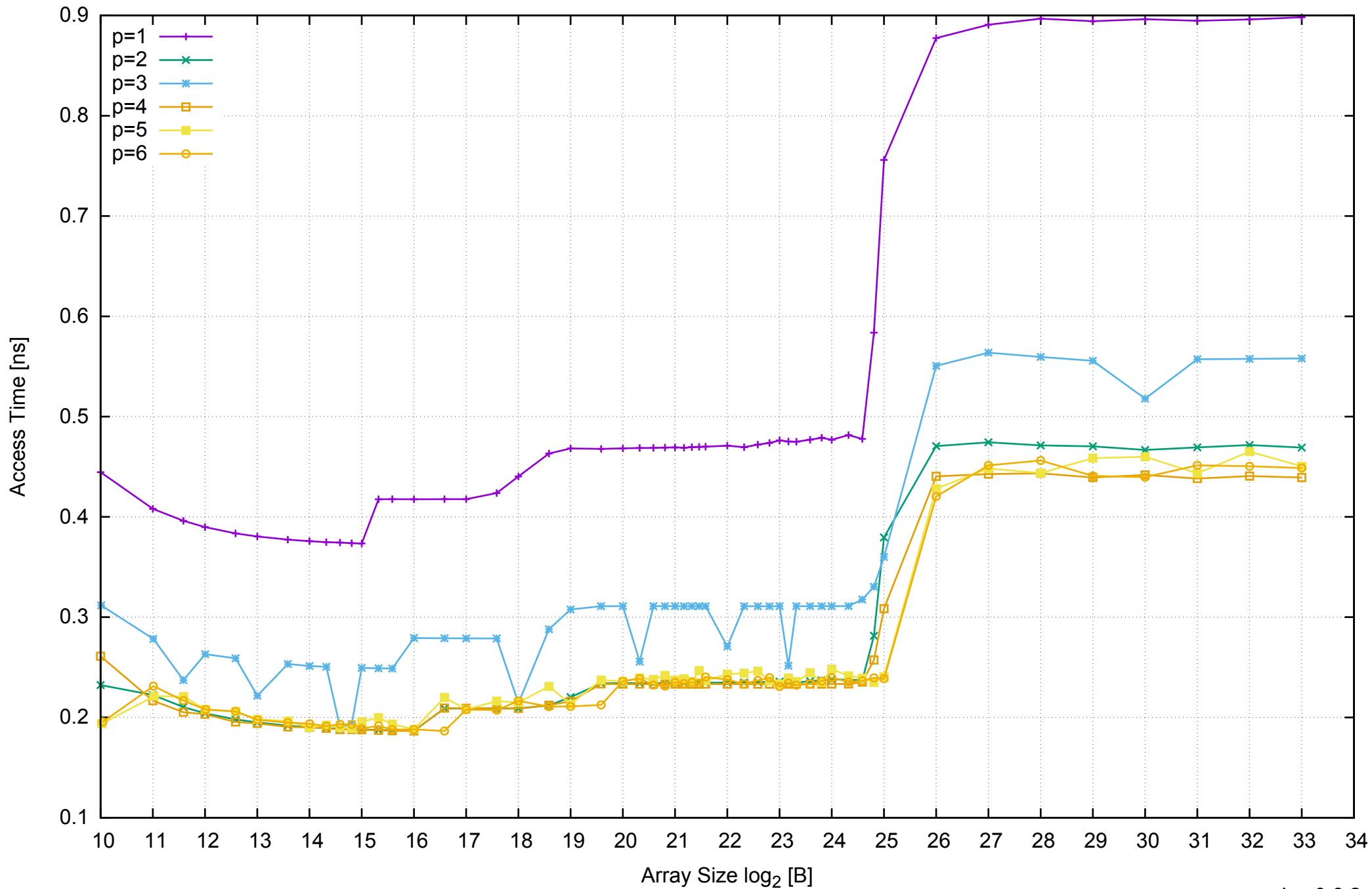
AWS m4.xlarge - Intel Xeon E5-2676 v3, 2.40 GHz 16GB - Parallel Memory Access Time - ScanWrite64PtrSimpleLoop
