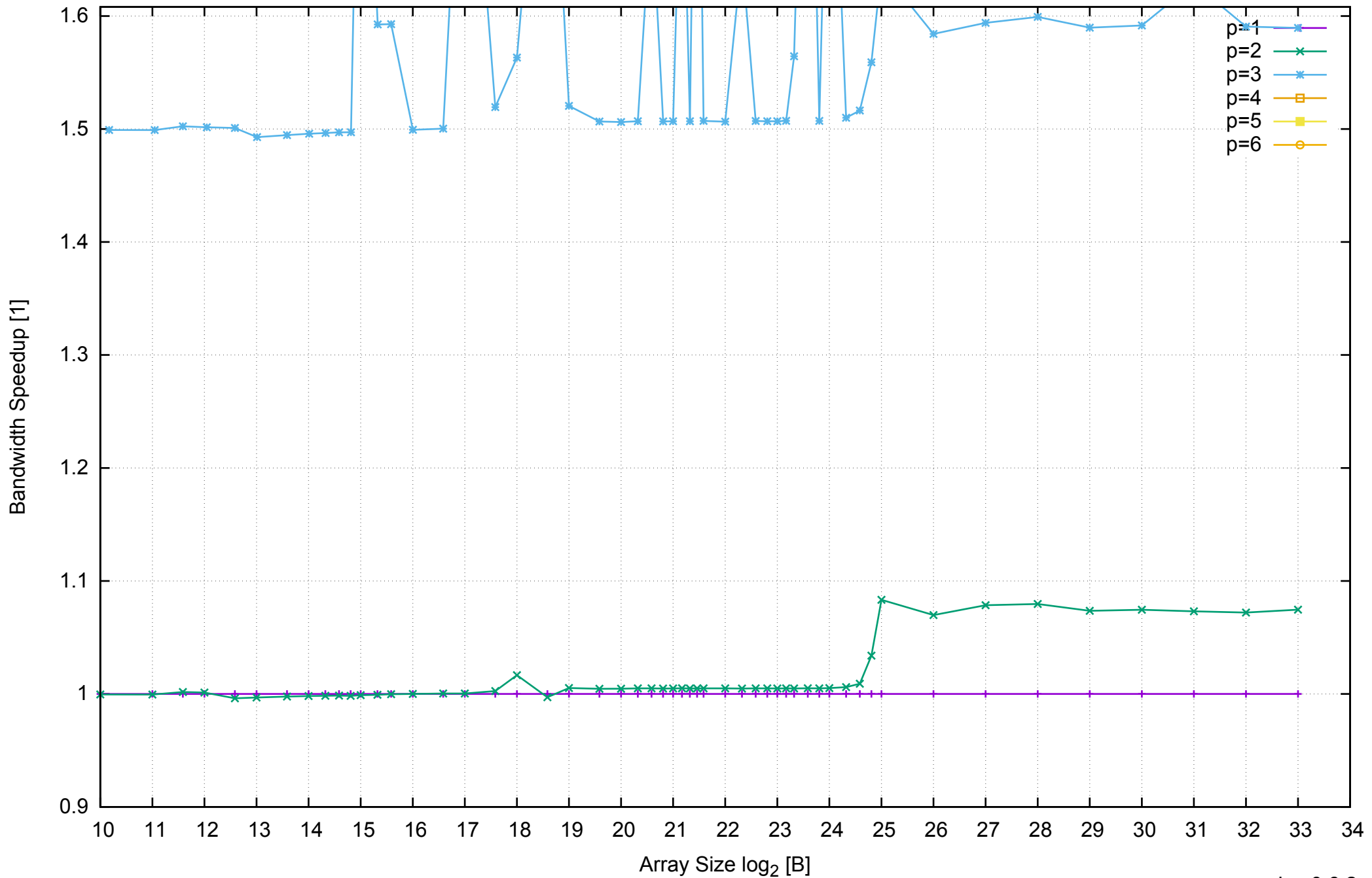
AWS m4.xlarge - Intel Xeon E5-2676 v3, 2.40 GHz 16GB - Speedup of Parallel Memory Bandwidth (enlarged) - ScanWrite32PtrUnrollLoop
