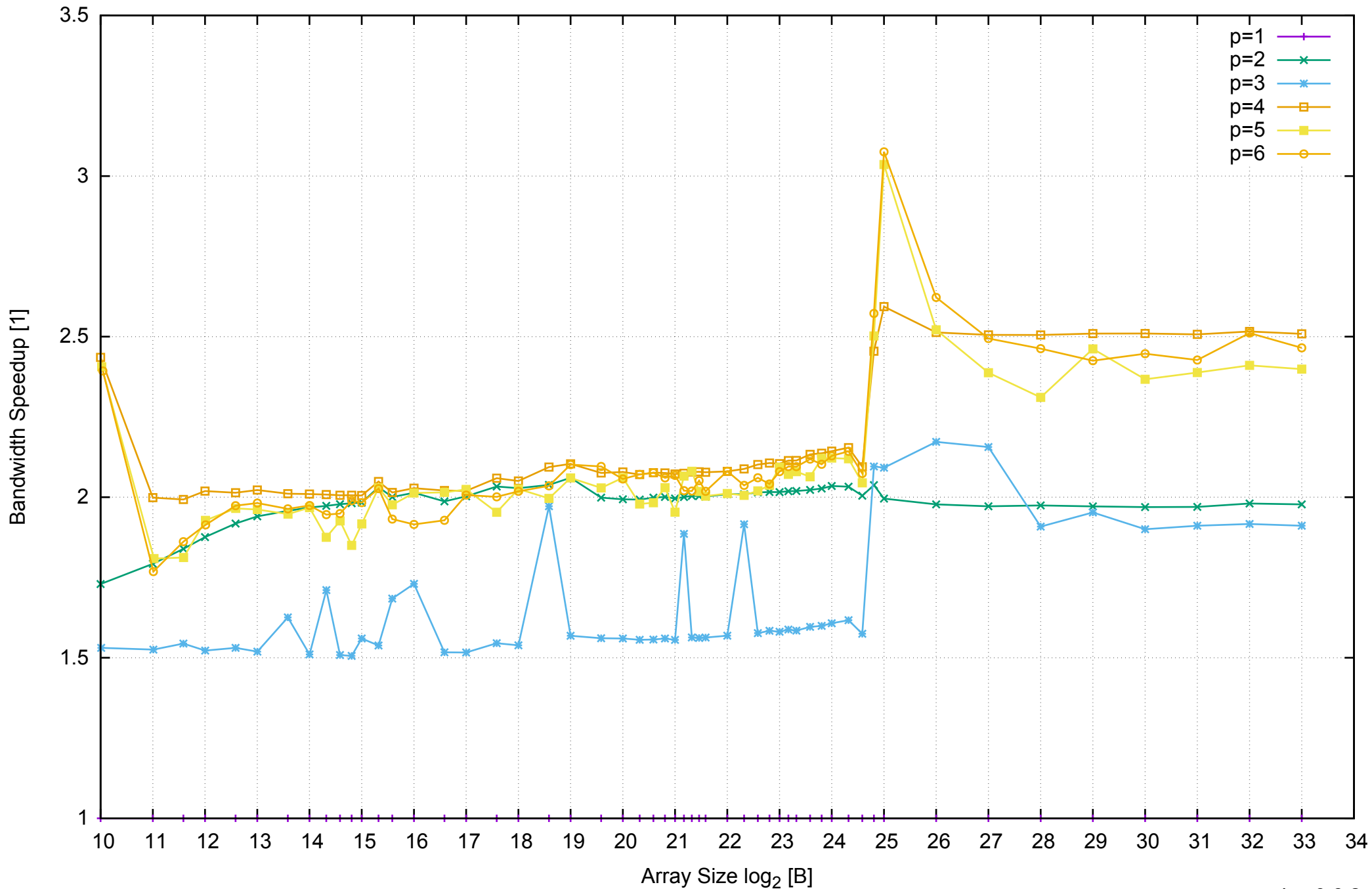
AWS m4.xlarge - Intel Xeon E5-2676 v3, 2.40 GHz 16GB - Speedup of Parallel Memory Bandwidth - ScanRead64IndexSimpleLoop
