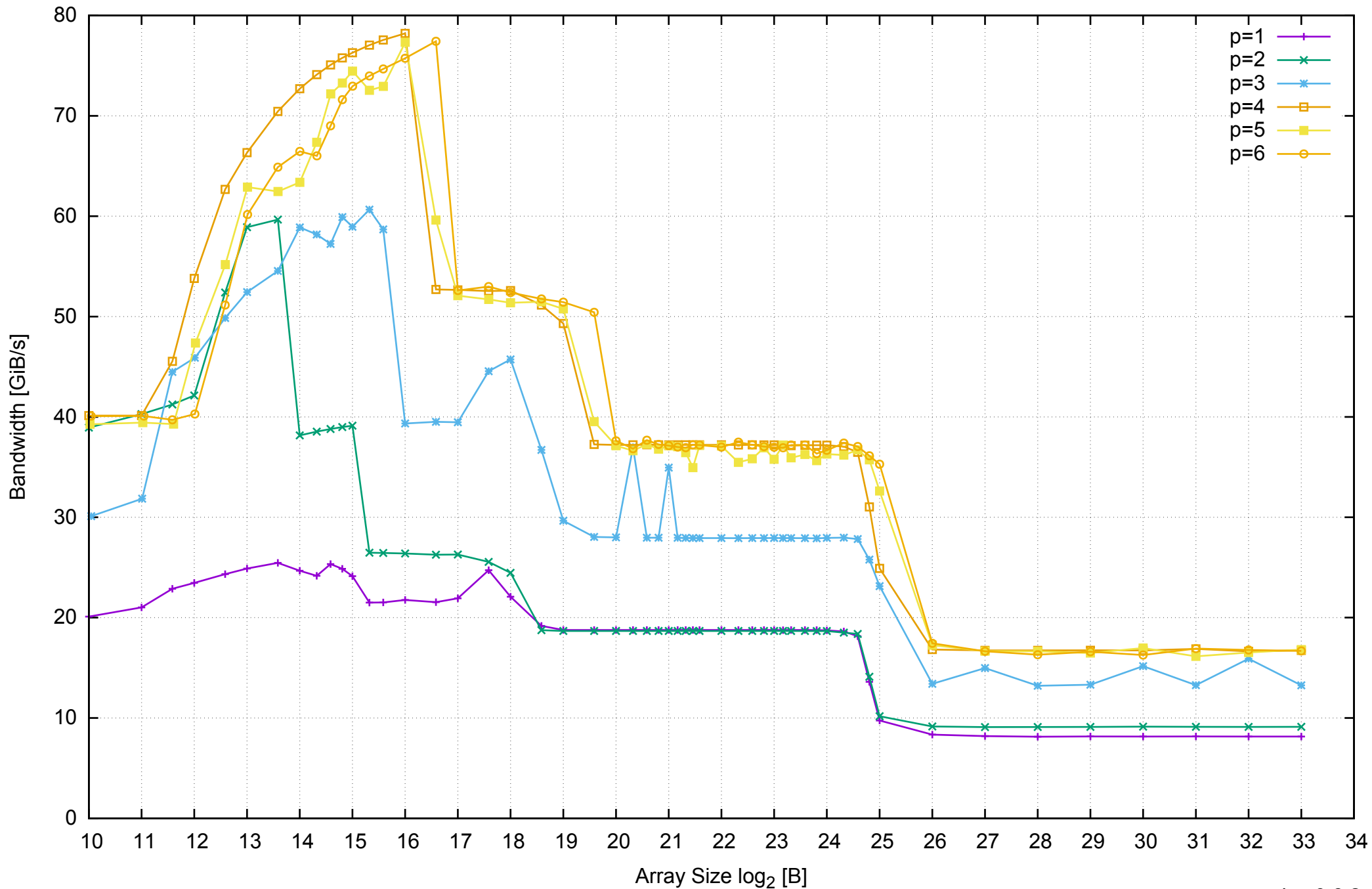
AWS m4.xlarge - Intel Xeon E5-2676 v3, 2.40 GHz 16GB - Parallel Memory Bandwidth - ScanWrite128PtrSimpleLoop
