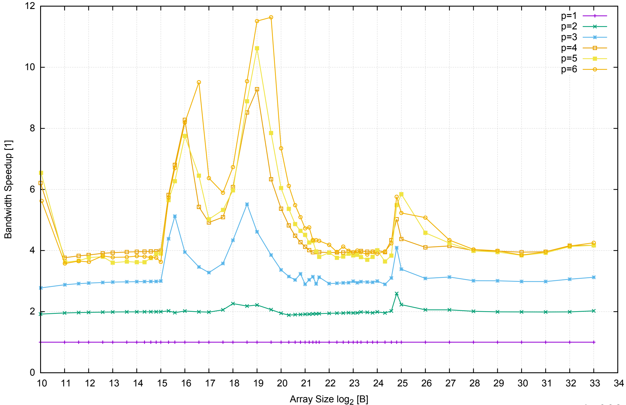
AWS m4.xlarge - Intel Xeon E5-2676 v3, 2.40 GHz 16GB - Speedup of Parallel Memory Bandwidth - PermRead64SimpleLoop
