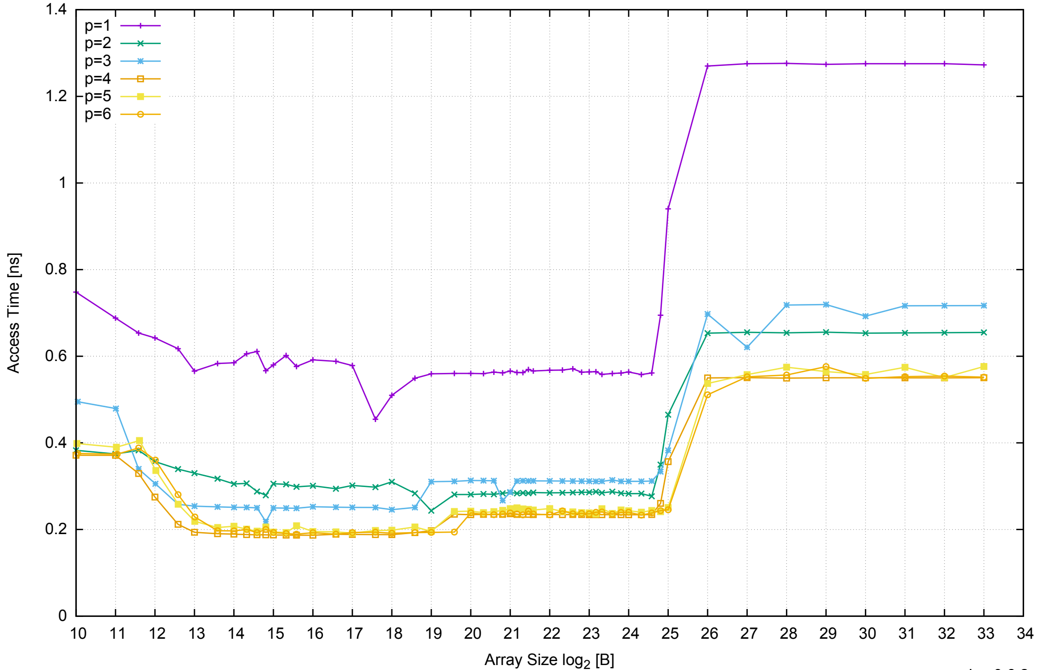
AWS m4.xlarge - Intel Xeon E5-2676 v3, 2.40 GHz 16GB - Parallel Memory Access Time - ScanRead128PtrSimpleLoop
