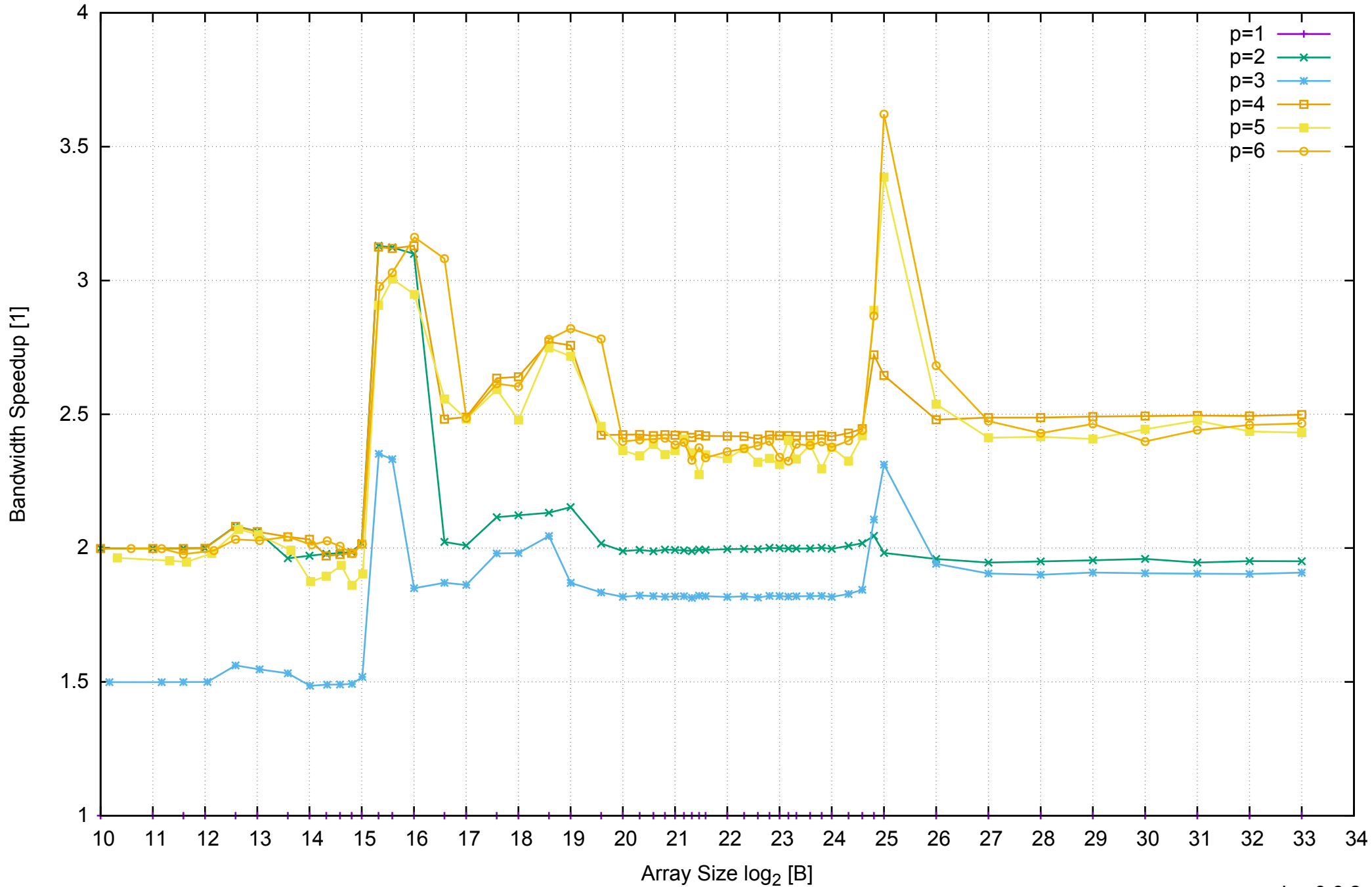
AWS m4.xlarge - Intel Xeon E5-2676 v3, 2.40 GHz 16GB - Speedup of Parallel Memory Bandwidth - ScanRead64PtrUnrollLoop
