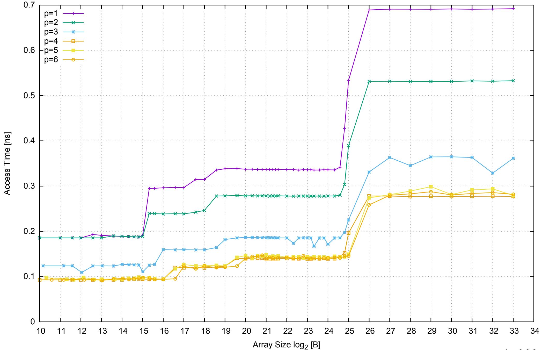
AWS m4.xlarge - Intel Xeon E5-2676 v3, 2.40 GHz 16GB - Parallel Memory Access Time - ScanRead64IndexUnrollLoop
