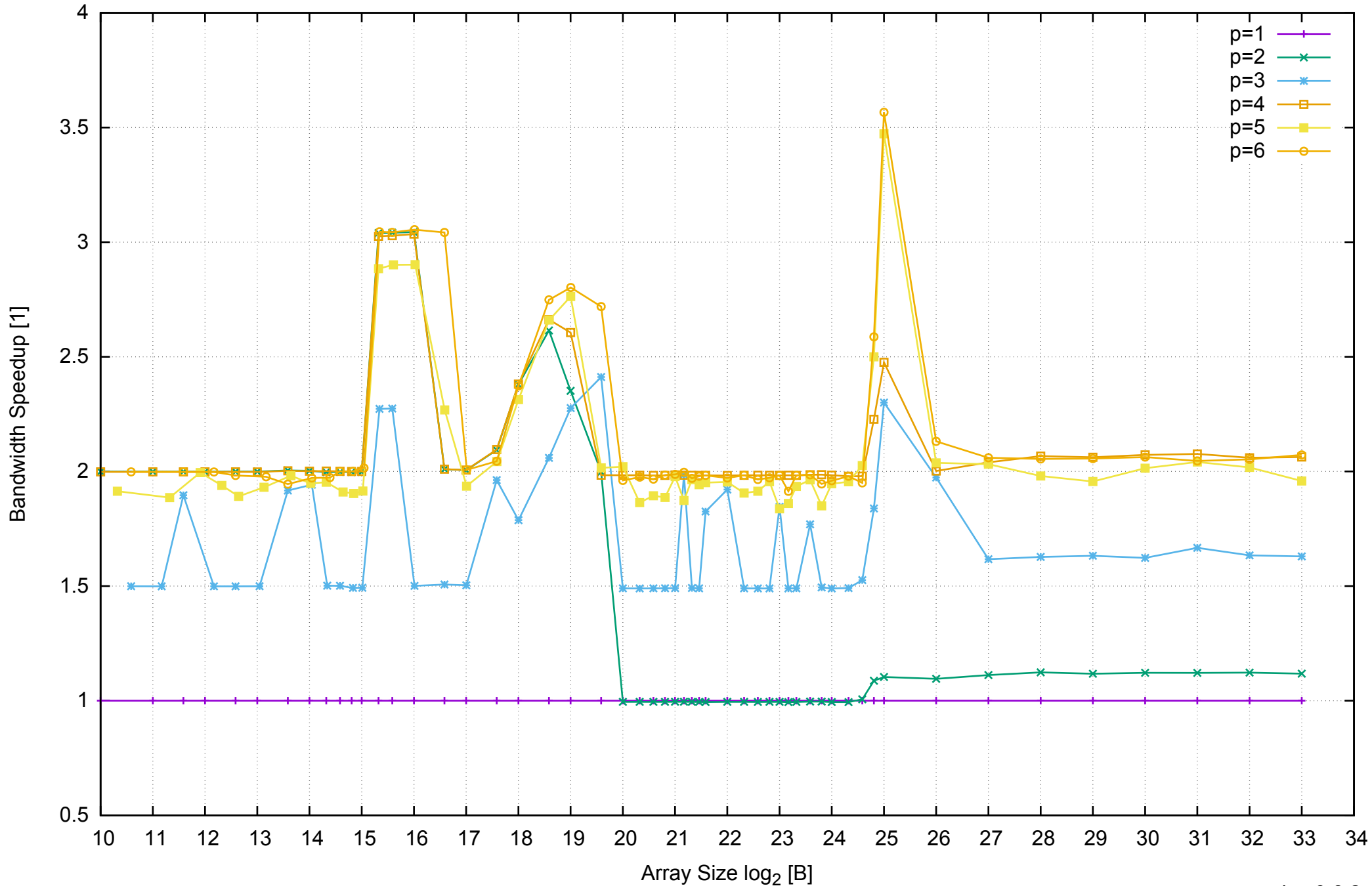
AWS m4.xlarge - Intel Xeon E5-2676 v3, 2.40 GHz 16GB - Speedup of Parallel Memory Bandwidth - ScanWrite128PtrUnrollLoop
