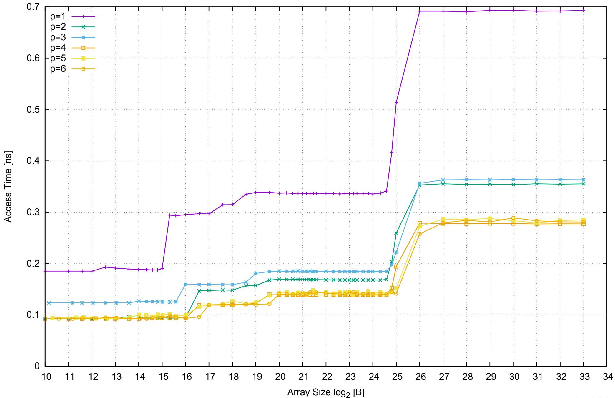
AWS m4.xlarge - Intel Xeon E5-2676 v3, 2.40 GHz 16GB - Parallel Memory Access Time - ScanRead64PtrUnrollLoop
