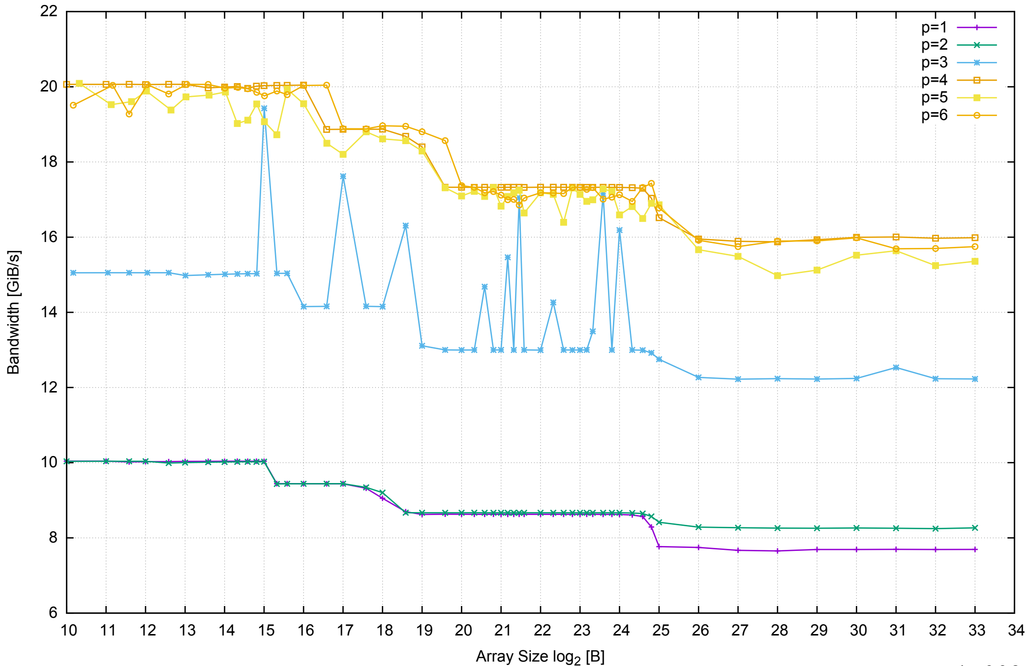
AWS m4.xlarge - Intel Xeon E5-2676 v3, 2.40 GHz 16GB - Parallel Memory Bandwidth - ScanWrite32PtrUnrollLoop
