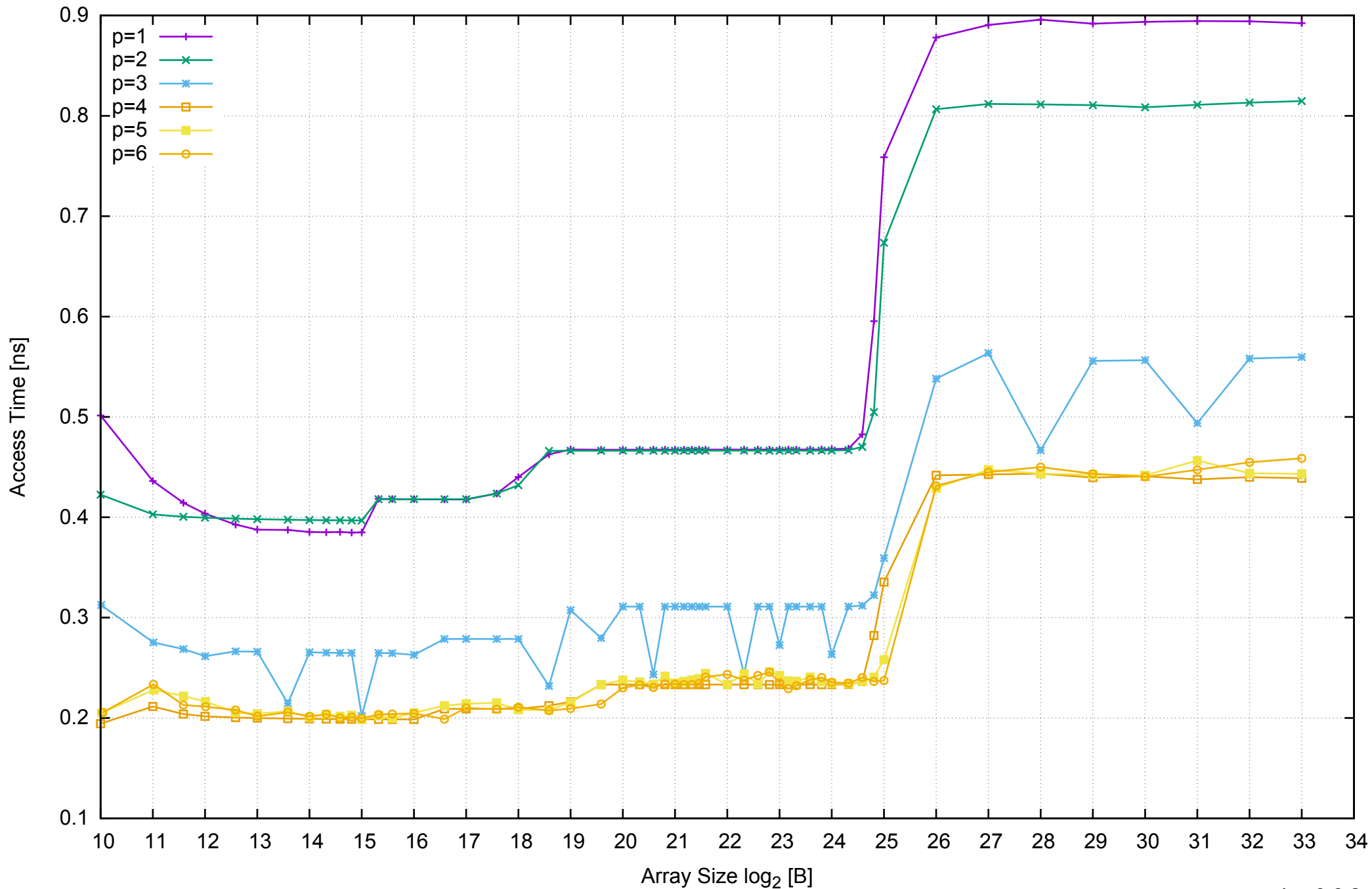
AWS m4.xlarge - Intel Xeon E5-2676 v3, 2.40 GHz 16GB - Parallel Memory Access Time - ScanWrite64IndexSimpleLoop
