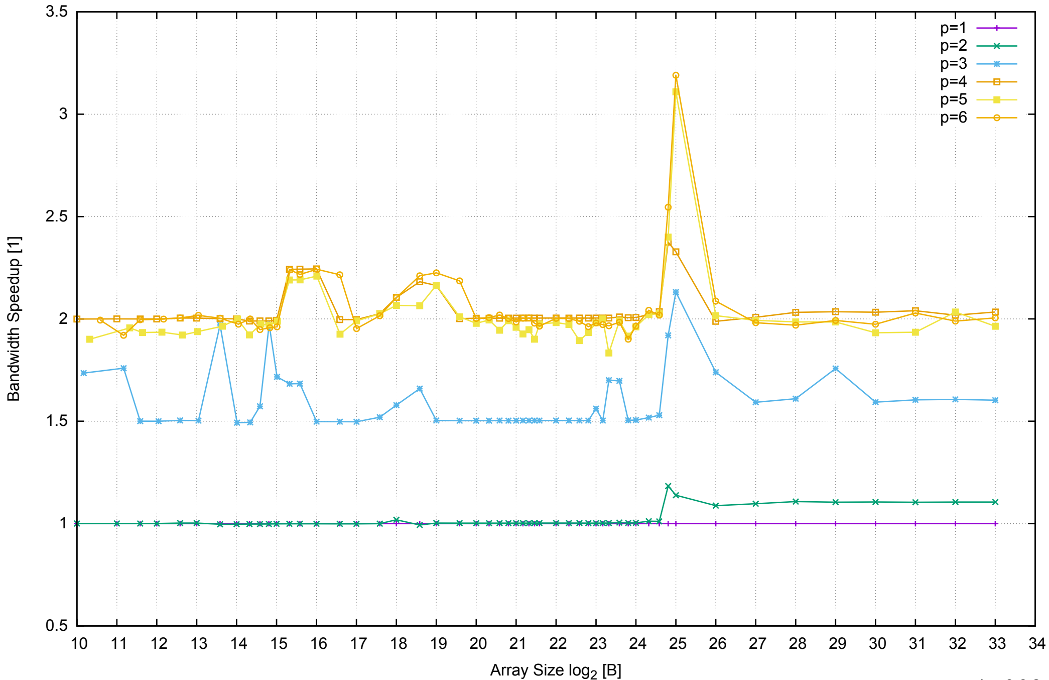
AWS m4.xlarge - Intel Xeon E5-2676 v3, 2.40 GHz 16GB - Speedup of Parallel Memory Bandwidth - ScanWrite64IndexUnrollLoop
