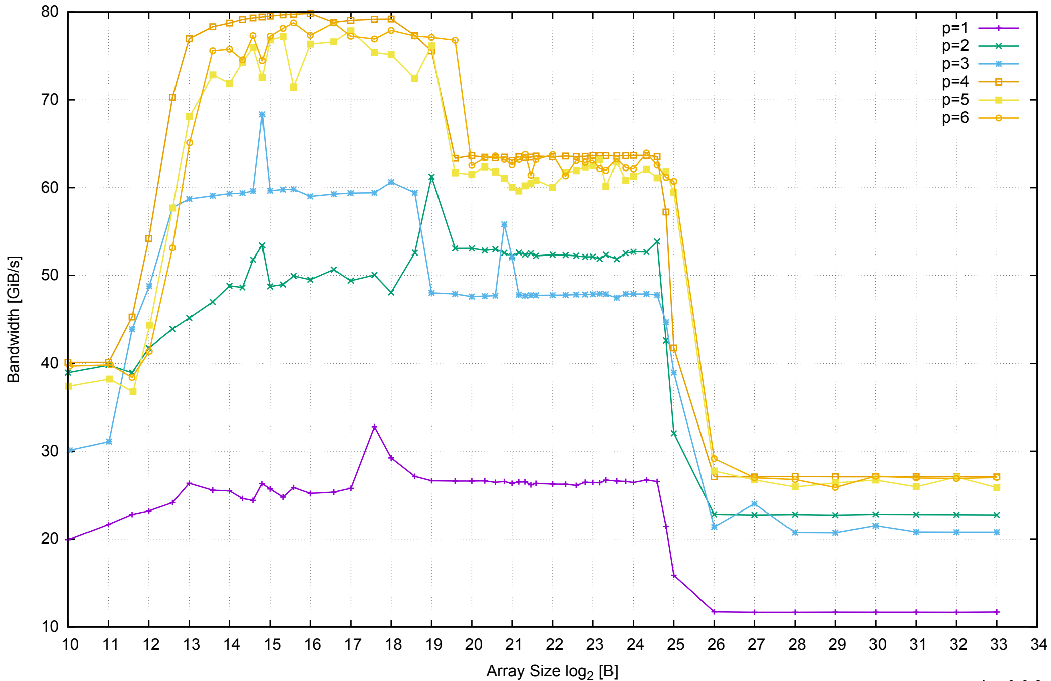
AWS m4.xlarge - Intel Xeon E5-2676 v3, 2.40 GHz 16GB - Parallel Memory Bandwidth - ScanRead128PtrSimpleLoop
