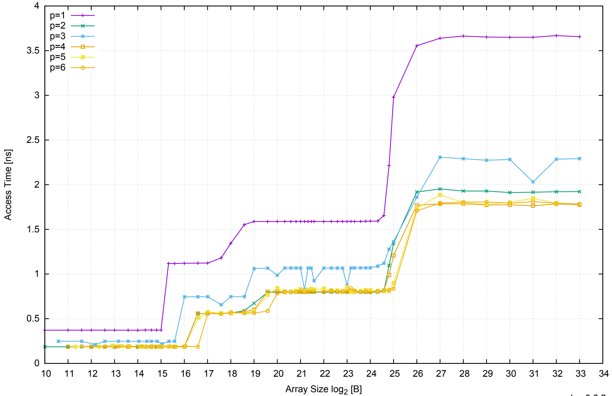
AWS m4.xlarge - Intel Xeon E5-2676 v3, 2.40 GHz 16GB - Parallel Memory Access Time - ScanWrite256PtrUnrollLoop
