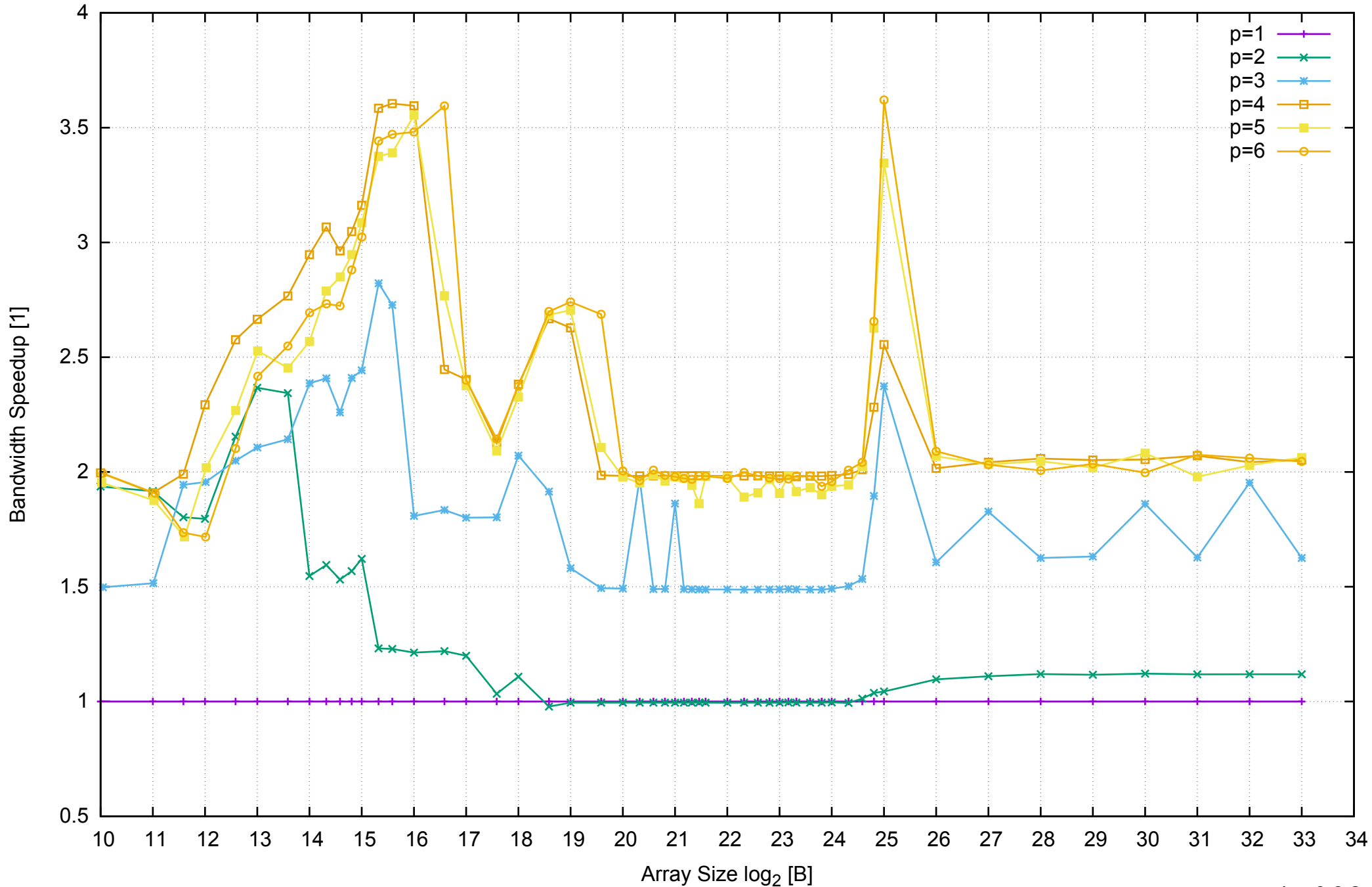
AWS m4.xlarge - Intel Xeon E5-2676 v3, 2.40 GHz 16GB - Speedup of Parallel Memory Bandwidth - ScanWrite128PtrSimpleLoop
