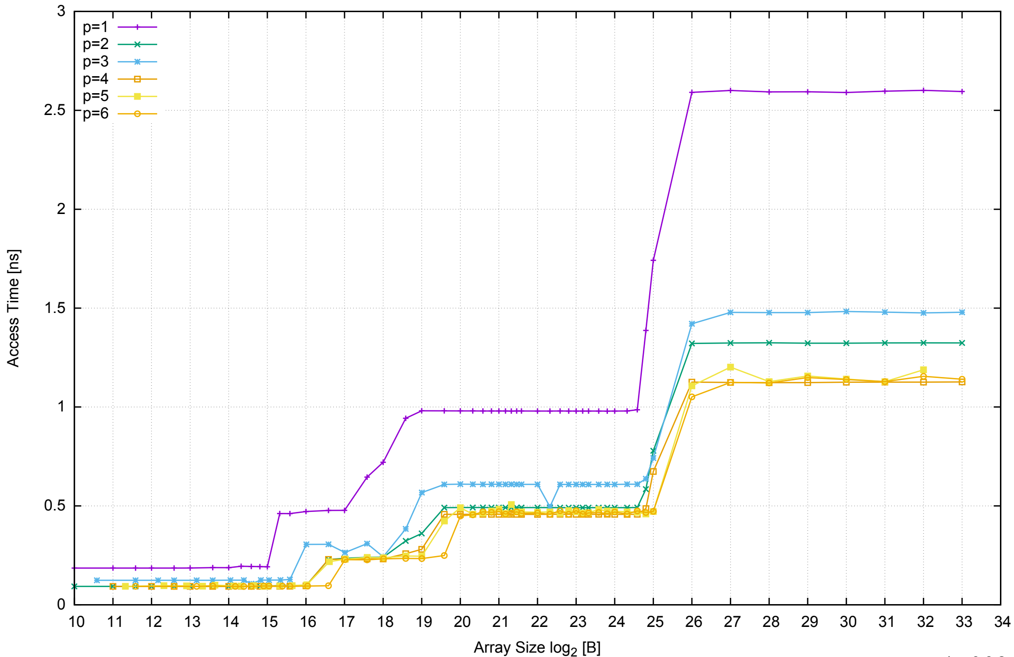
AWS m4.xlarge - Intel Xeon E5-2676 v3, 2.40 GHz 16GB - Parallel Memory Access Time - ScanRead256PtrUnrollLoop
