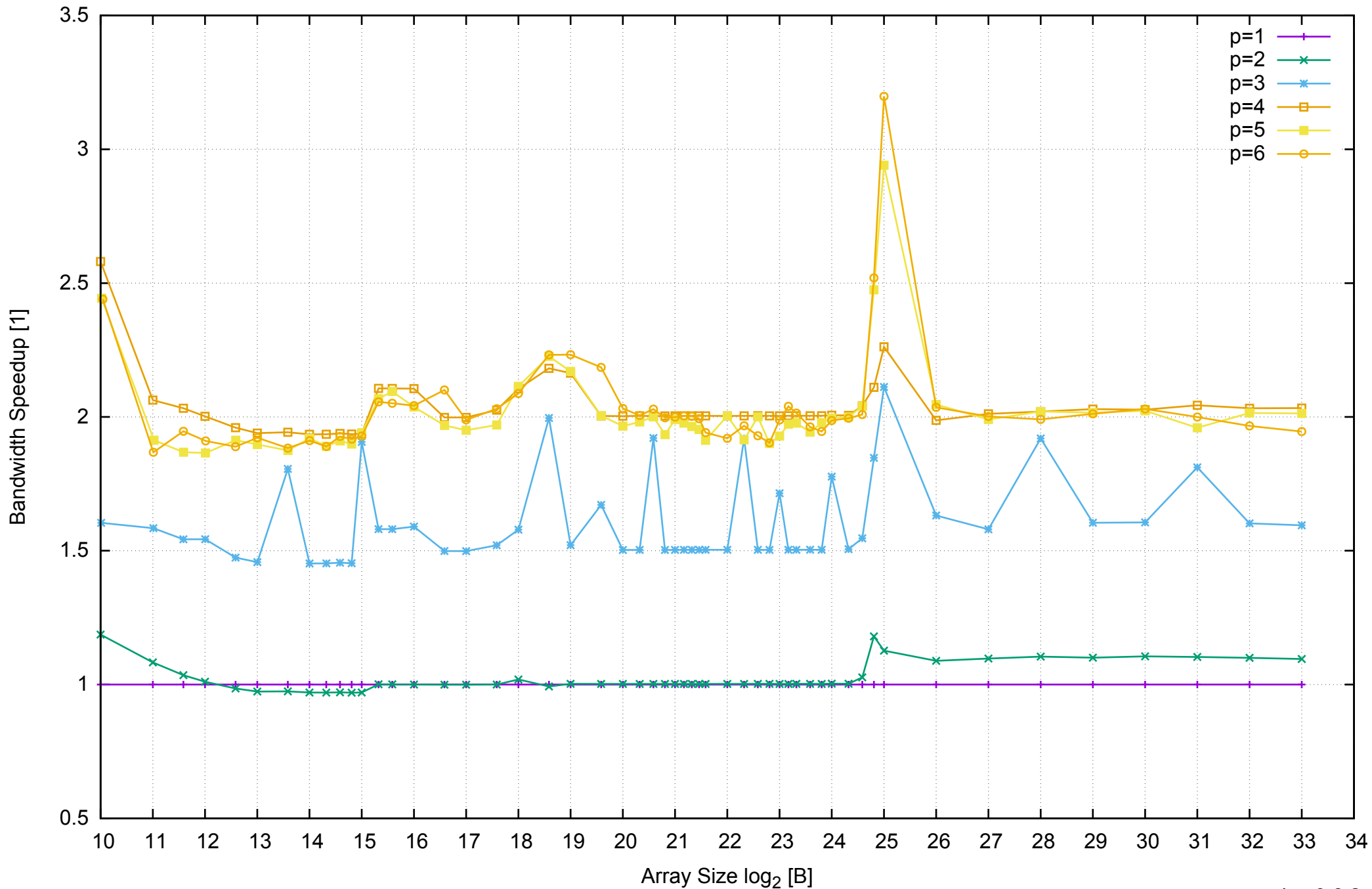
AWS m4.xlarge - Intel Xeon E5-2676 v3, 2.40 GHz 16GB - Speedup of Parallel Memory Bandwidth - ScanWrite64IndexSimpleLoop
