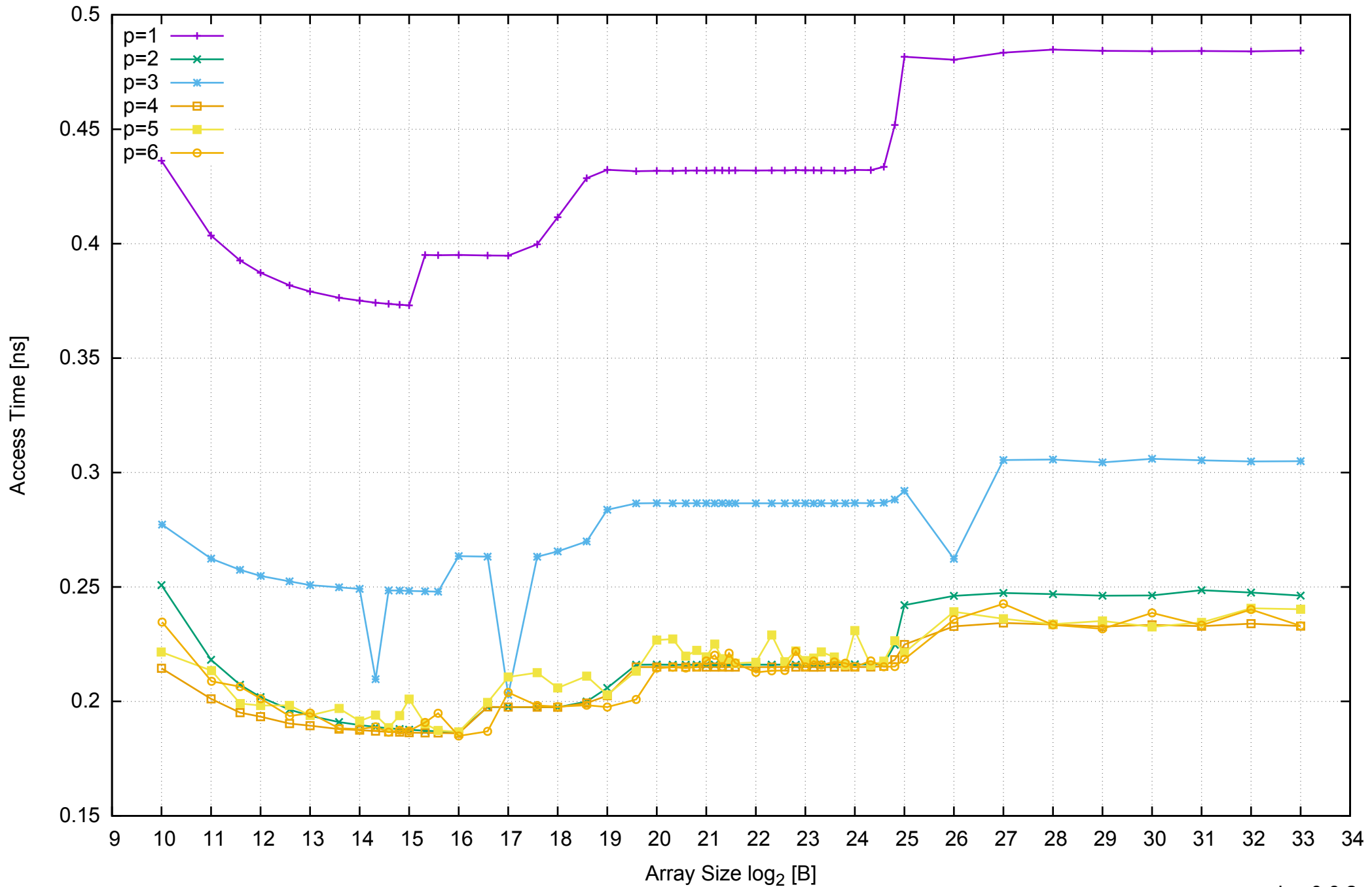
AWS m4.xlarge - Intel Xeon E5-2676 v3, 2.40 GHz 16GB - Parallel Memory Access Time - ScanWrite32PtrSimpleLoop
