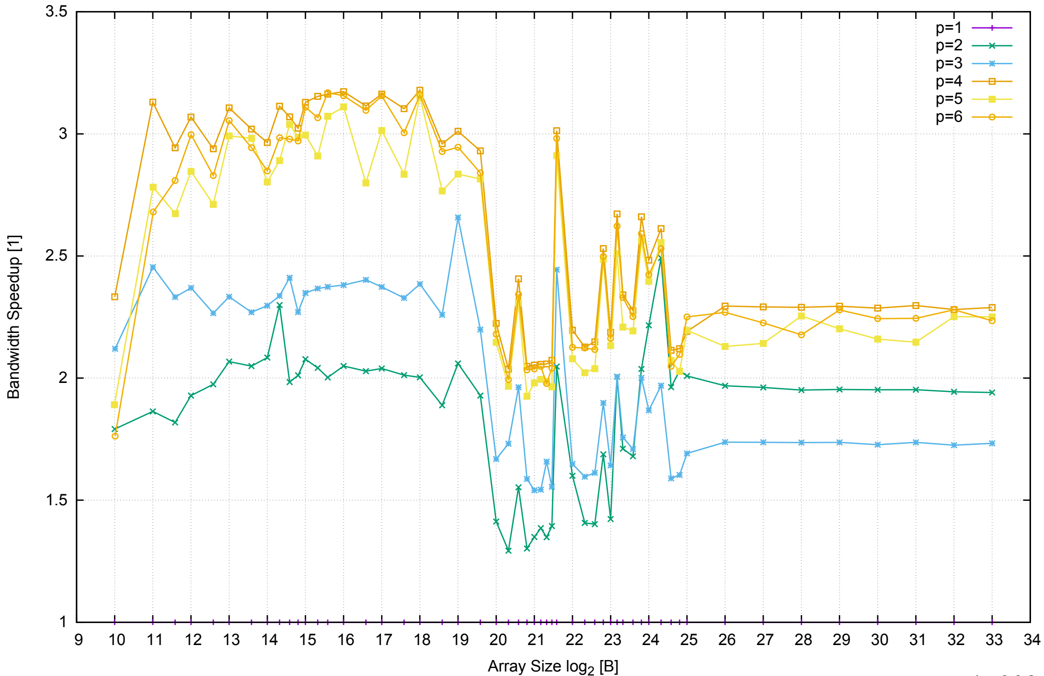
AWS m4.xlarge - Intel Xeon E5-2676 v3, 2.40 GHz 16GB - Speedup of Parallel Memory Bandwidth - ScanRead32PtrSimpleLoop
