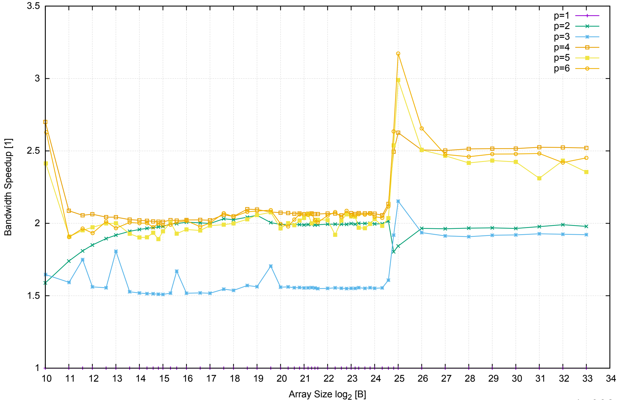
AWS m4.xlarge - Intel Xeon E5-2676 v3, 2.40 GHz 16GB - Speedup of Parallel Memory Bandwidth - ScanRead64PtrSimpleLoop
