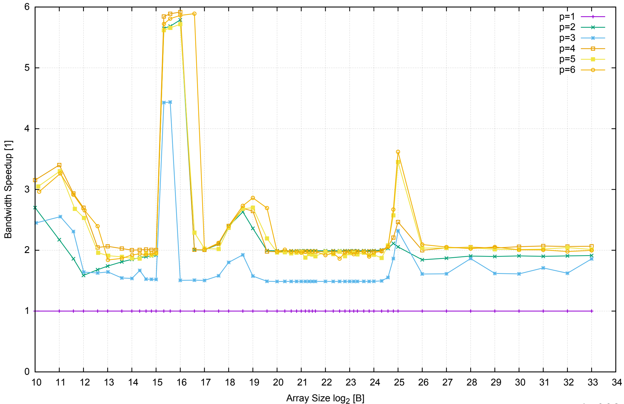
AWS m4.xlarge - Intel Xeon E5-2676 v3, 2.40 GHz 16GB - Speedup of Parallel Memory Bandwidth - ScanWrite256PtrSimpleLoop
