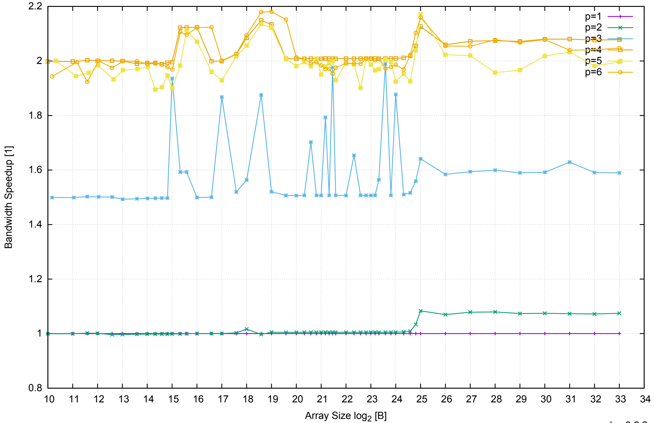
AWS m4.xlarge - Intel Xeon E5-2676 v3, 2.40 GHz 16GB - Speedup of Parallel Memory Bandwidth - ScanWrite32PtrUnrollLoop
