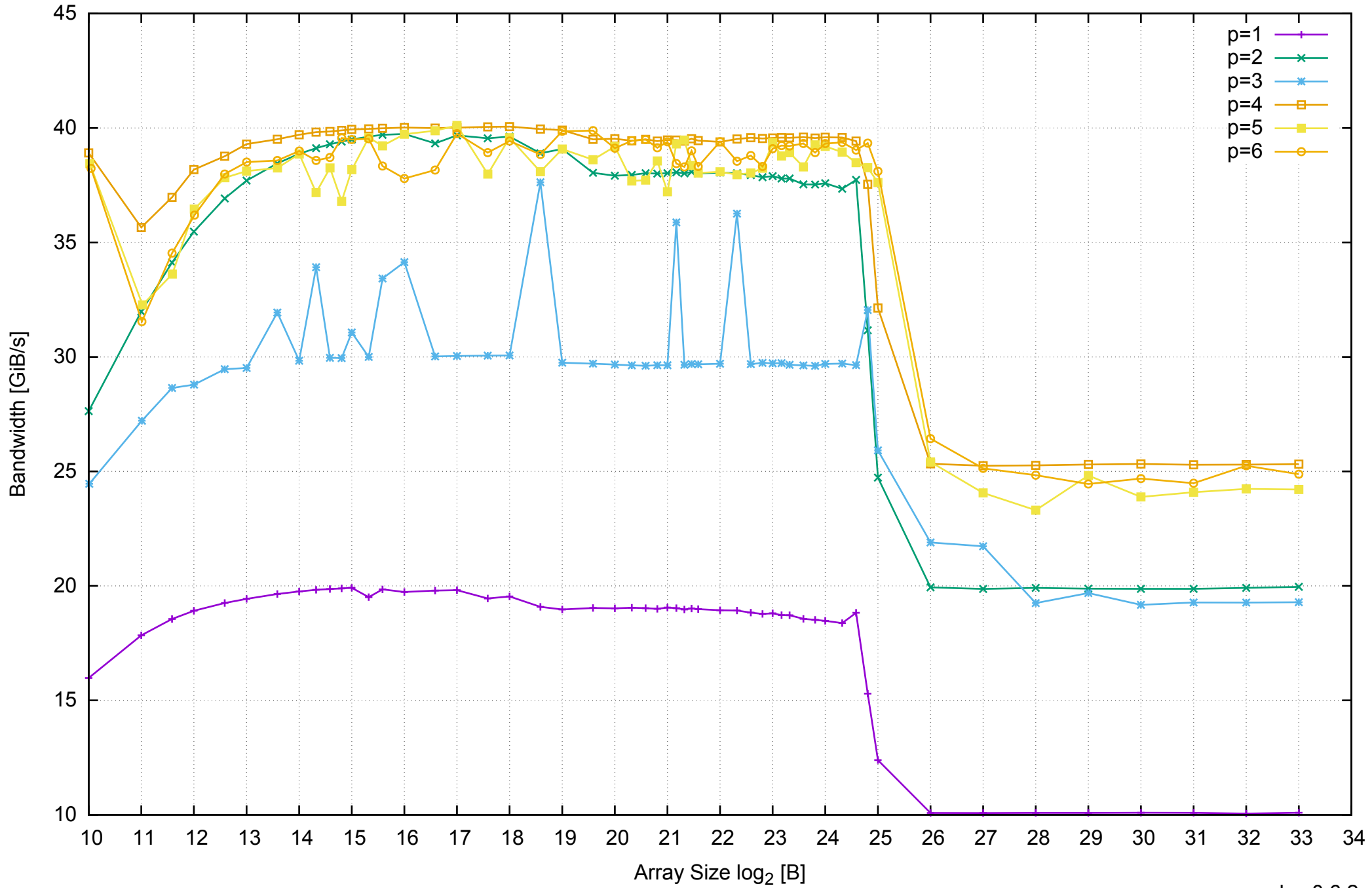
AWS m4.xlarge - Intel Xeon E5-2676 v3, 2.40 GHz 16GB - Parallel Memory Bandwidth - ScanRead64IndexSimpleLoop
