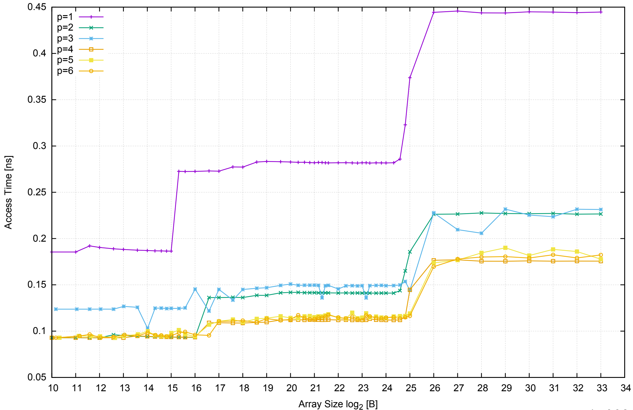
AWS m4.xlarge - Intel Xeon E5-2676 v3, 2.40 GHz 16GB - Parallel Memory Access Time - ScanRead32PtrUnrollLoop
