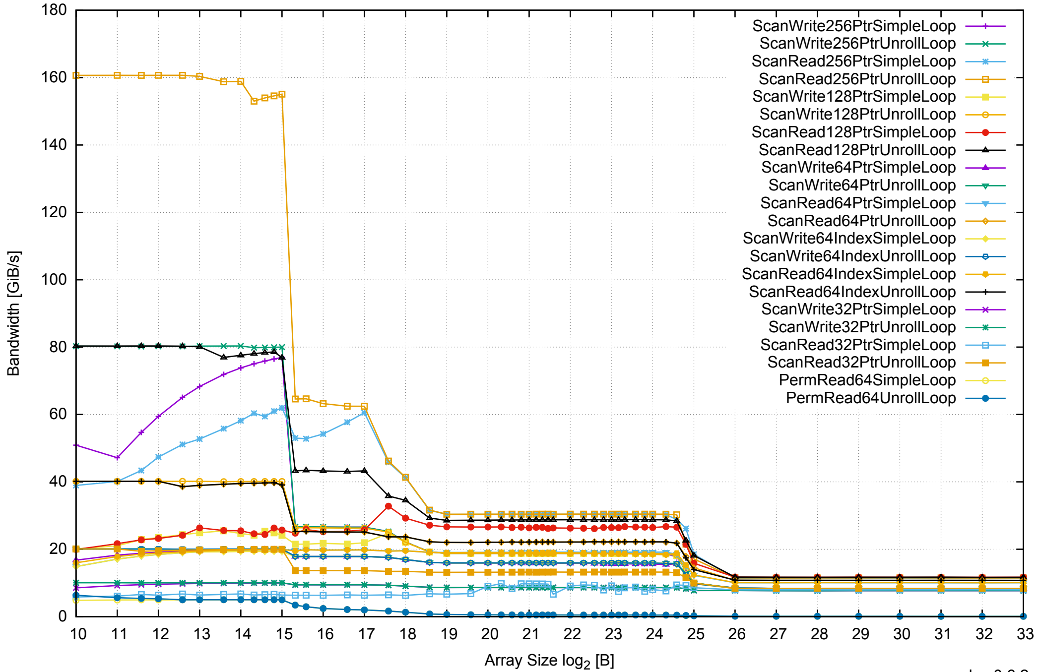
AWS m4.xlarge - Intel Xeon E5-2676 v3, 2.40 GHz 16GB - One Thread Memory Bandwidth
