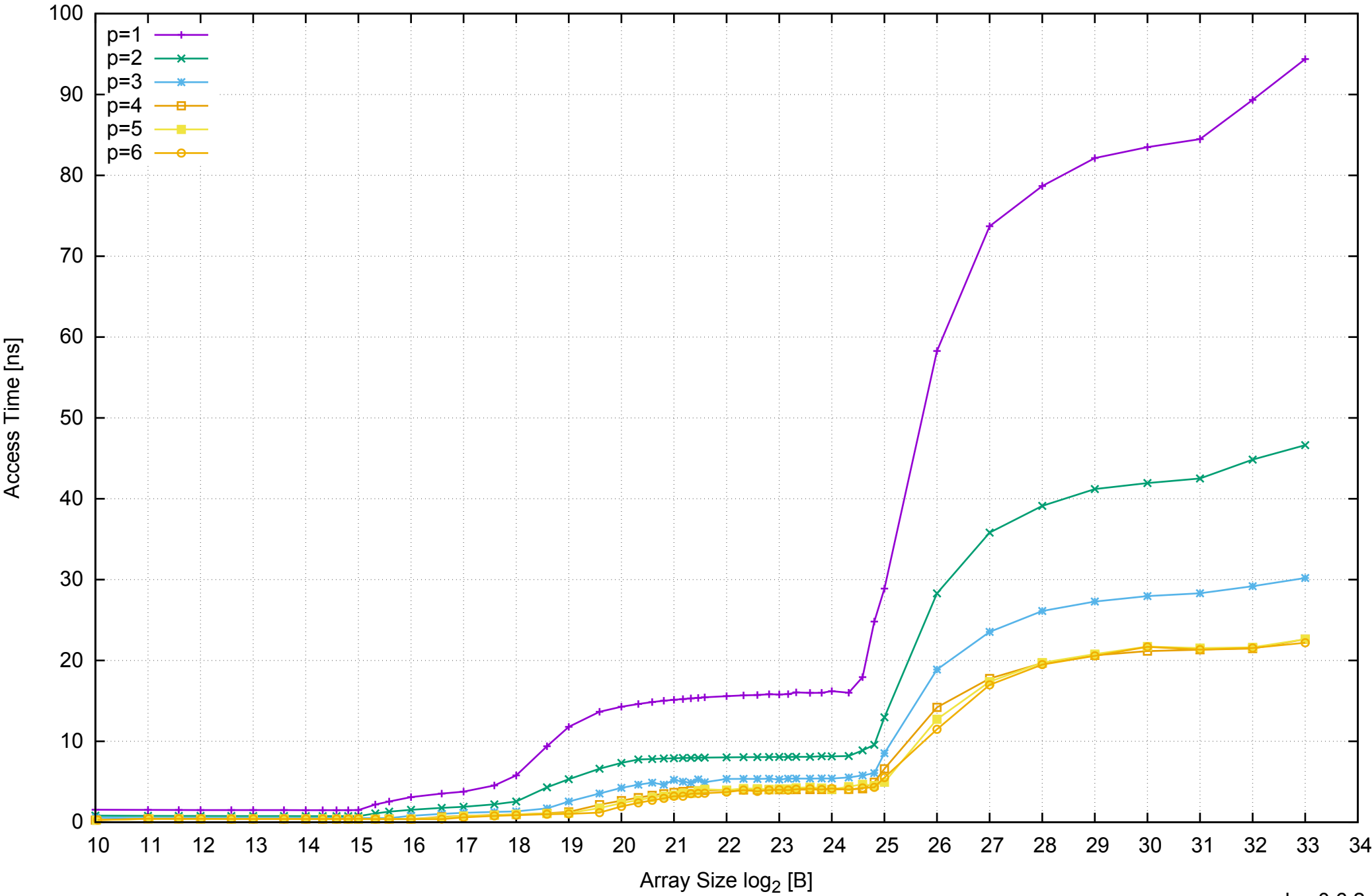
AWS m4.xlarge - Intel Xeon E5-2676 v3, 2.40 GHz 16GB - Parallel Memory Access Time - PermRead64SimpleLoop
