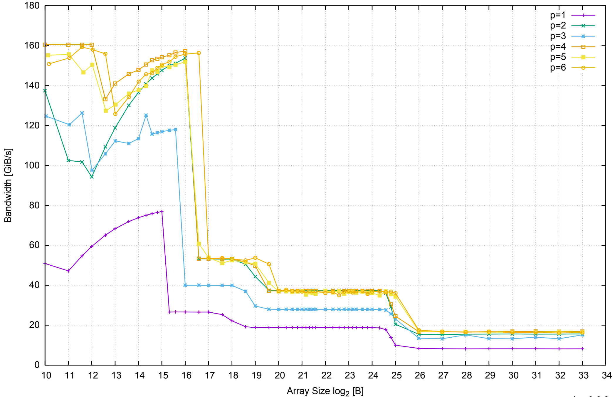
AWS m4.xlarge - Intel Xeon E5-2676 v3, 2.40 GHz 16GB - Parallel Memory Bandwidth - ScanWrite256PtrSimpleLoop
