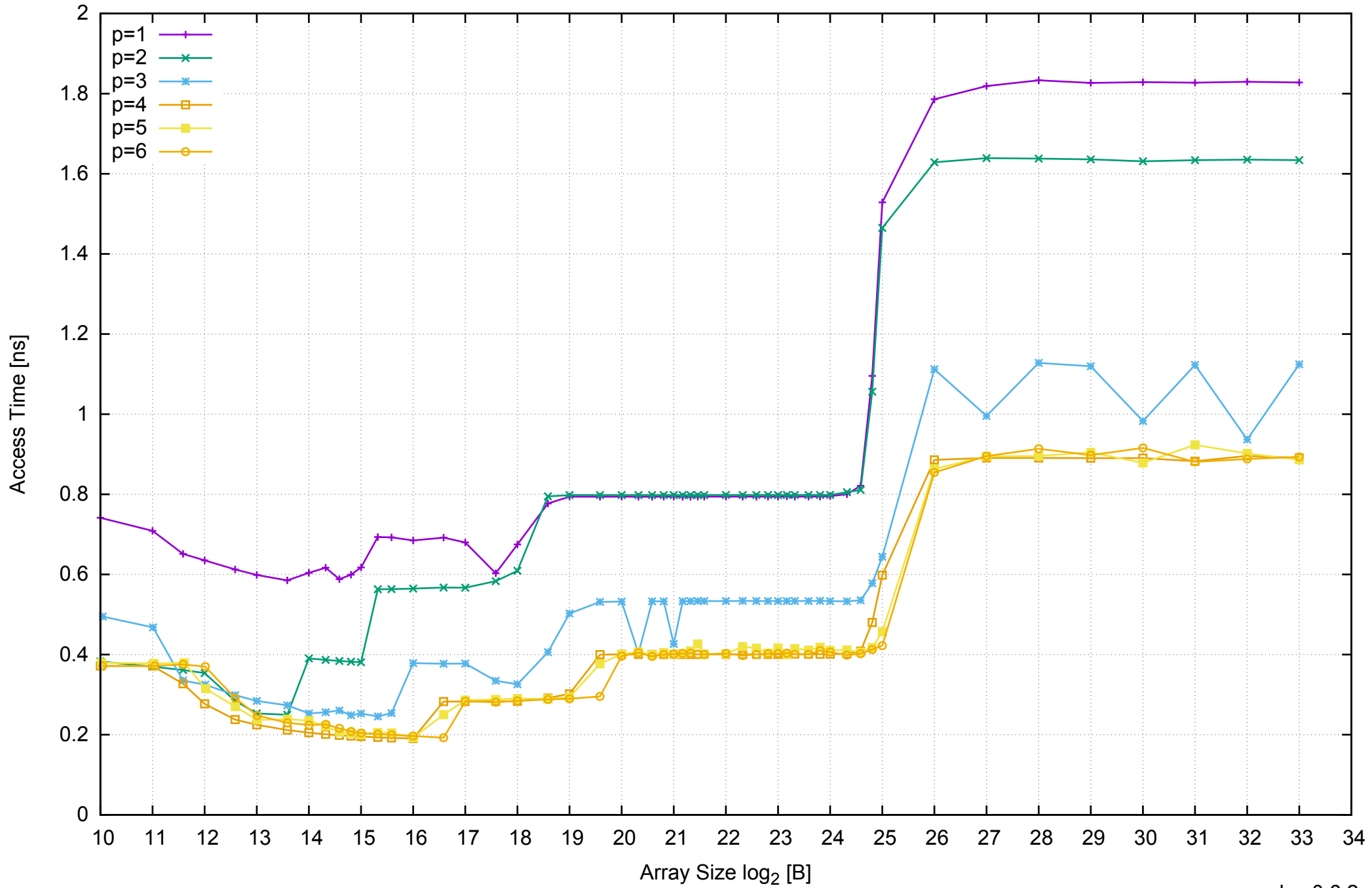
AWS m4.xlarge - Intel Xeon E5-2676 v3, 2.40 GHz 16GB - Parallel Memory Access Time - ScanWrite128PtrSimpleLoop
