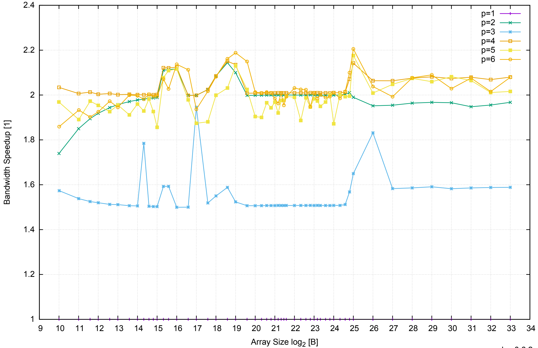
AWS m4.xlarge - Intel Xeon E5-2676 v3, 2.40 GHz 16GB - Speedup of Parallel Memory Bandwidth - ScanWrite32PtrSimpleLoop
