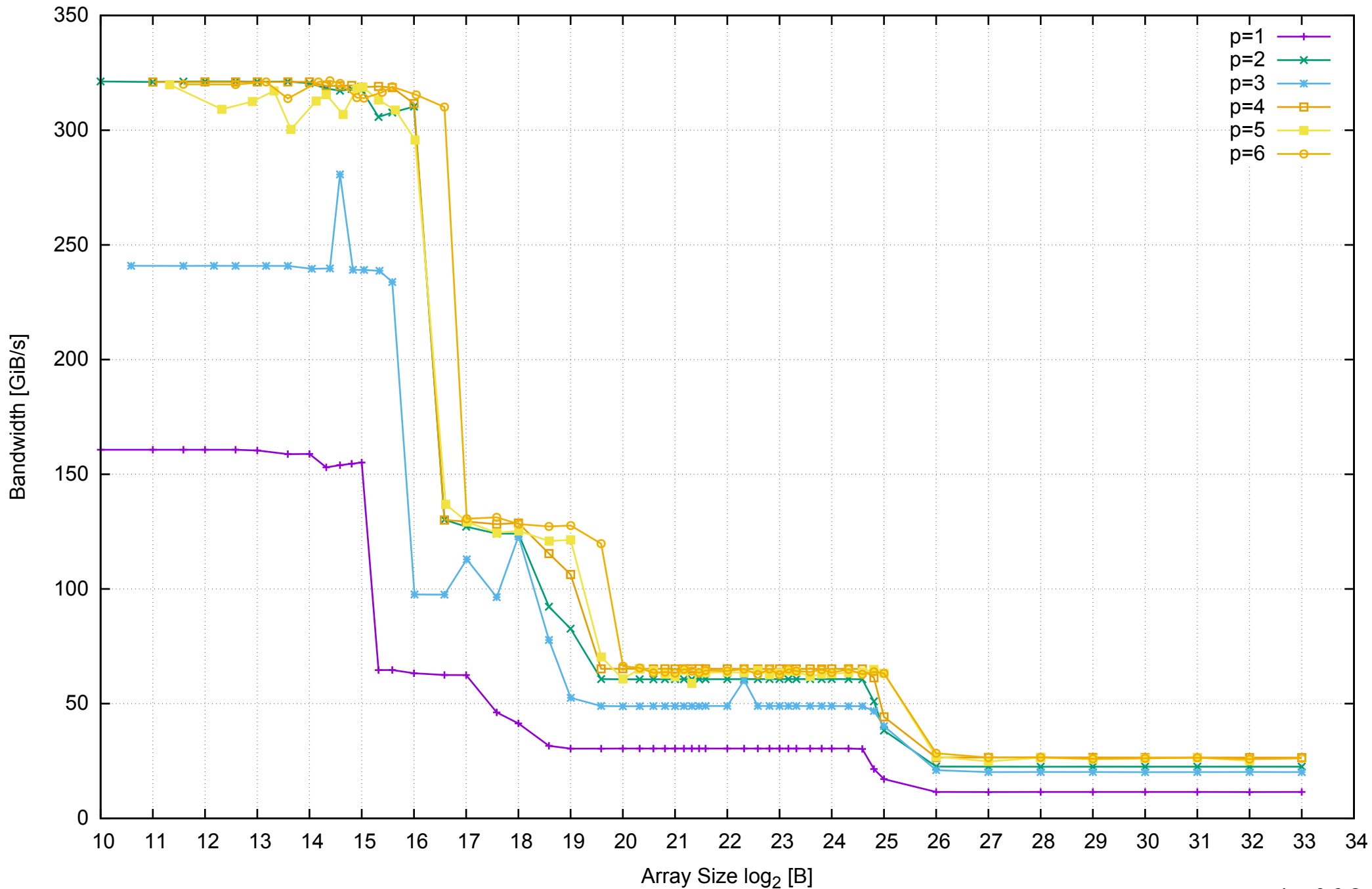
AWS m4.xlarge - Intel Xeon E5-2676 v3, 2.40 GHz 16GB - Parallel Memory Bandwidth - ScanRead256PtrUnrollLoop
