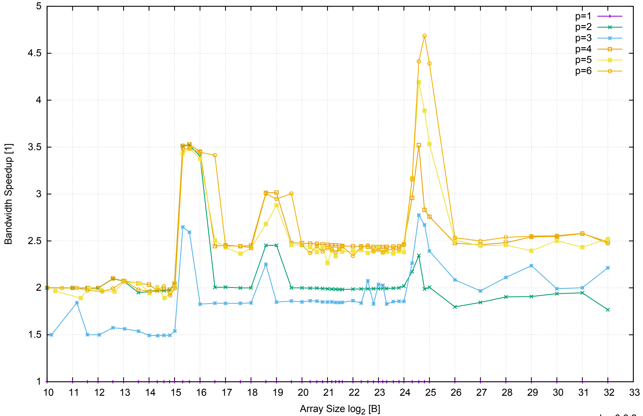
AWS c3.xlarge - Intel Xeon E5-2680 v2 2.80 GHz 7.5GB - Speedup of Parallel Memory Bandwidth - ScanRead64IndexUnrollLoop
