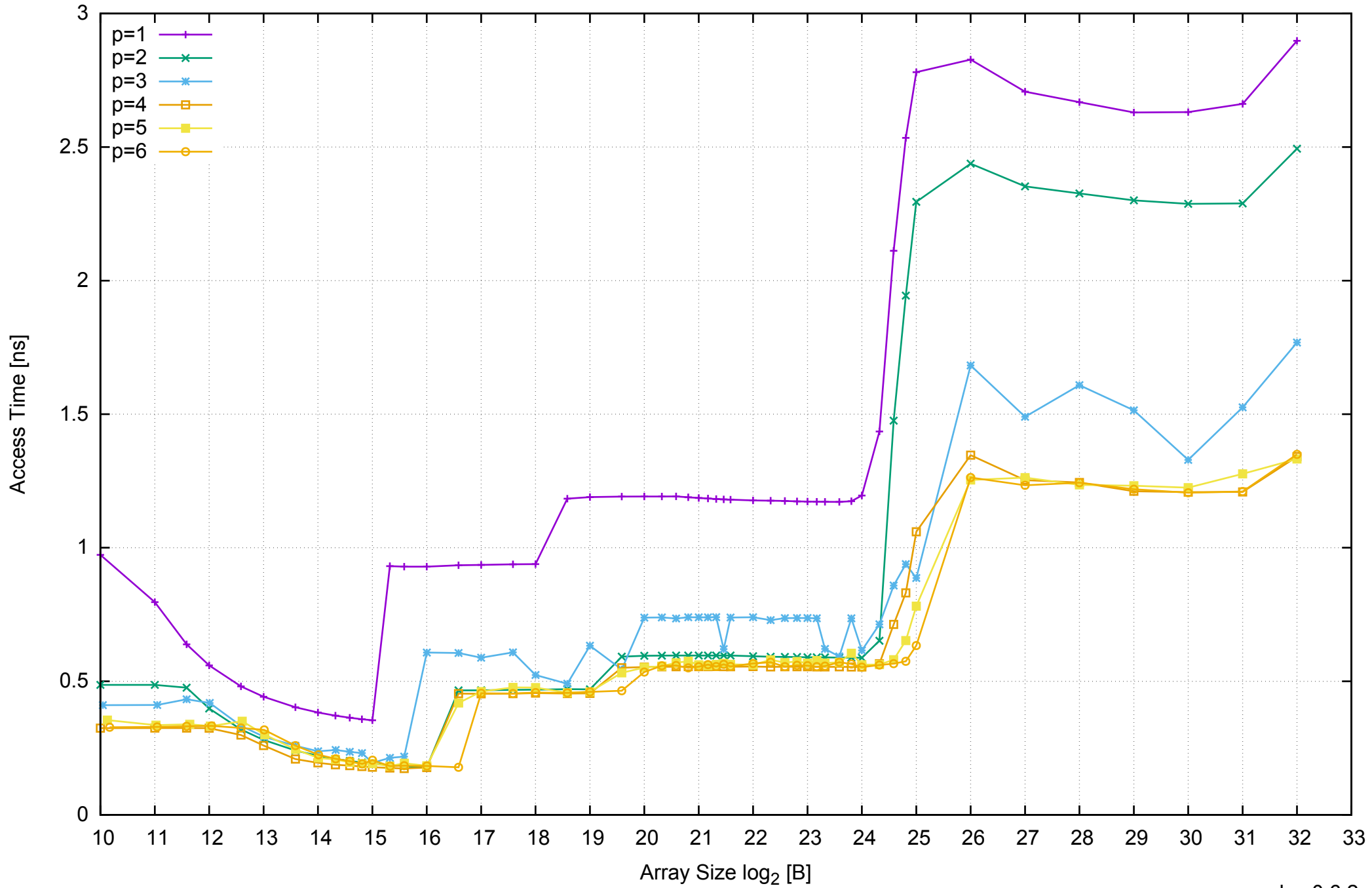
AWS c3.xlarge - Intel Xeon E5-2680 v2 2.80 GHz 7.5GB - Parallel Memory Access Time - ScanRead256PtrSimpleLoop
