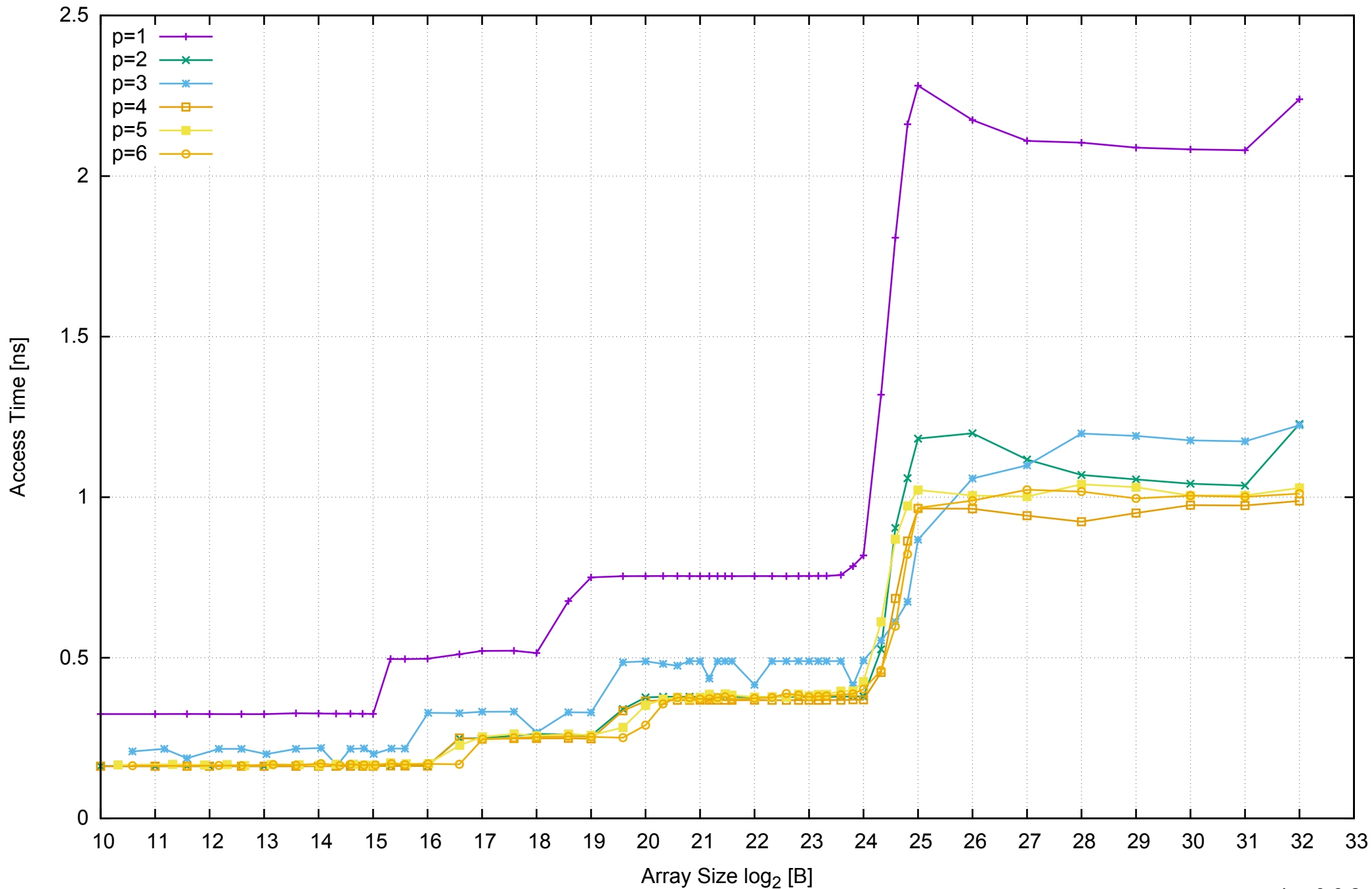
AWS c3.xlarge - Intel Xeon E5-2680 v2 2.80 GHz 7.5GB - Parallel Memory Access Time - ScanWrite128PtrUnrollLoop
