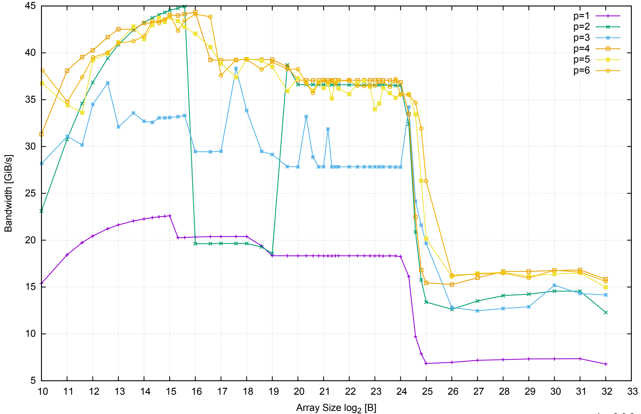
AWS c3.xlarge - Intel Xeon E5-2680 v2 2.80 GHz 7.5GB - Parallel Memory Bandwidth - ScanWrite64PtrSimpleLoop
