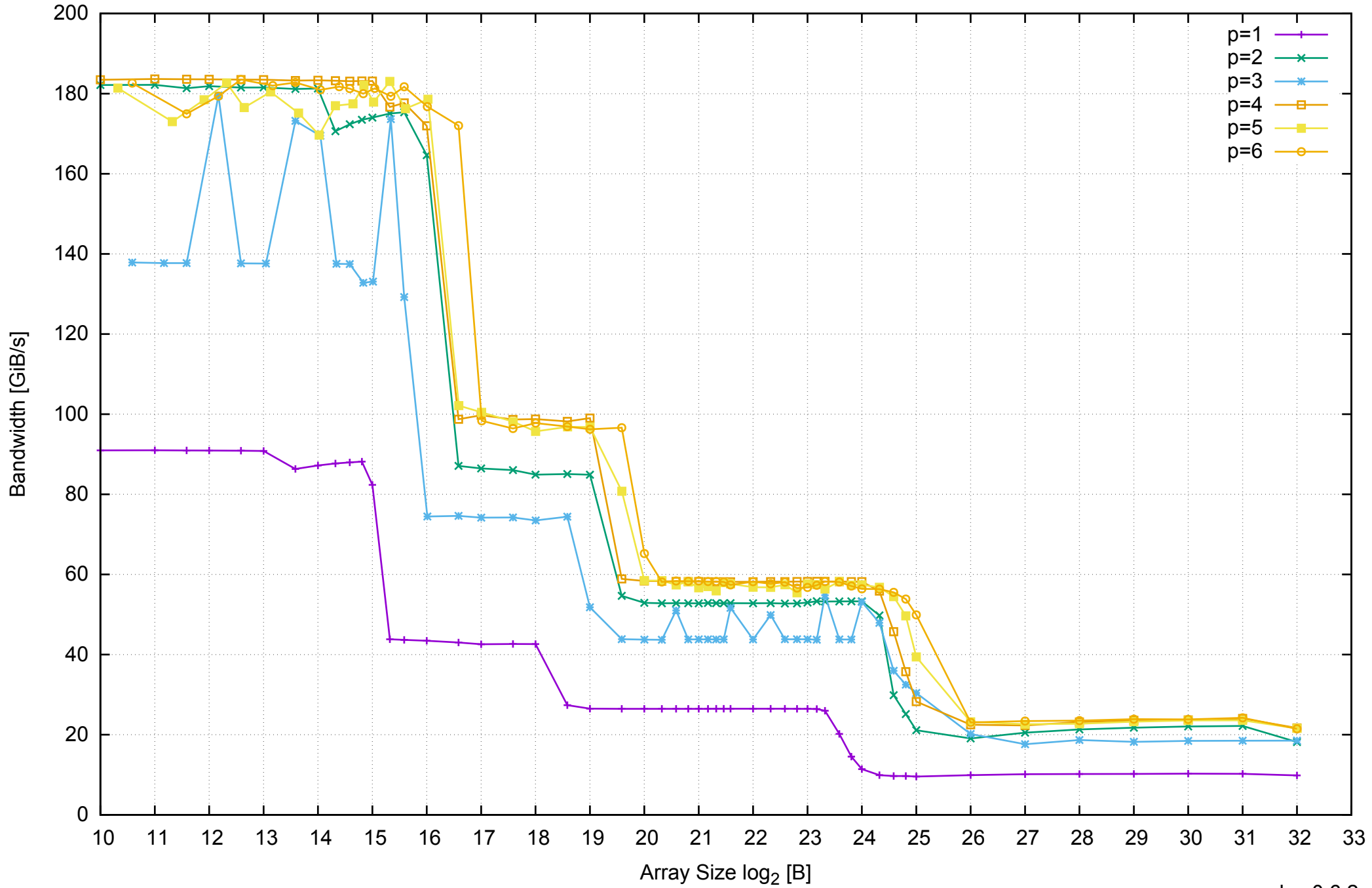
AWS c3.xlarge - Intel Xeon E5-2680 v2 2.80 GHz 7.5GB - Parallel Memory Bandwidth - ScanRead128PtrUnrollLoop
