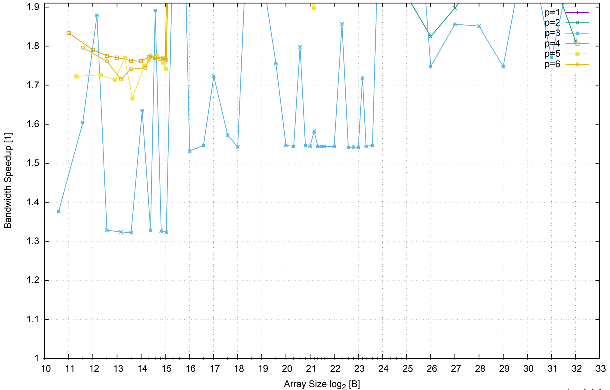
AWS c3.xlarge - Intel Xeon E5-2680 v2 2.80 GHz 7.5GB - Speedup of Parallel Memory Bandwidth (enlarged) - ScanWrite256PtrUnrollLoop
