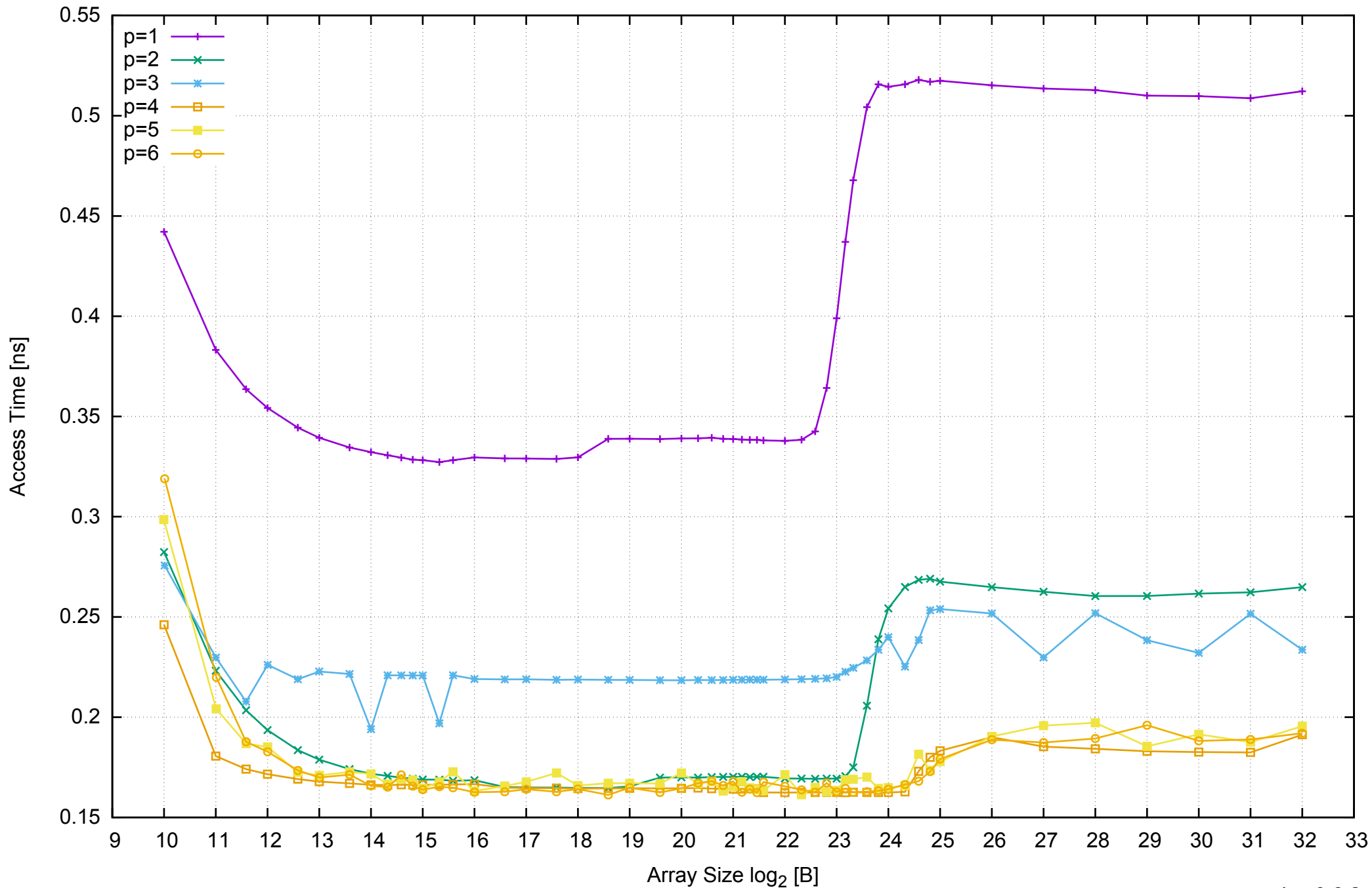
AWS c3.xlarge - Intel Xeon E5-2680 v2 2.80 GHz 7.5GB - Parallel Memory Access Time - ScanRead32PtrSimpleLoop
