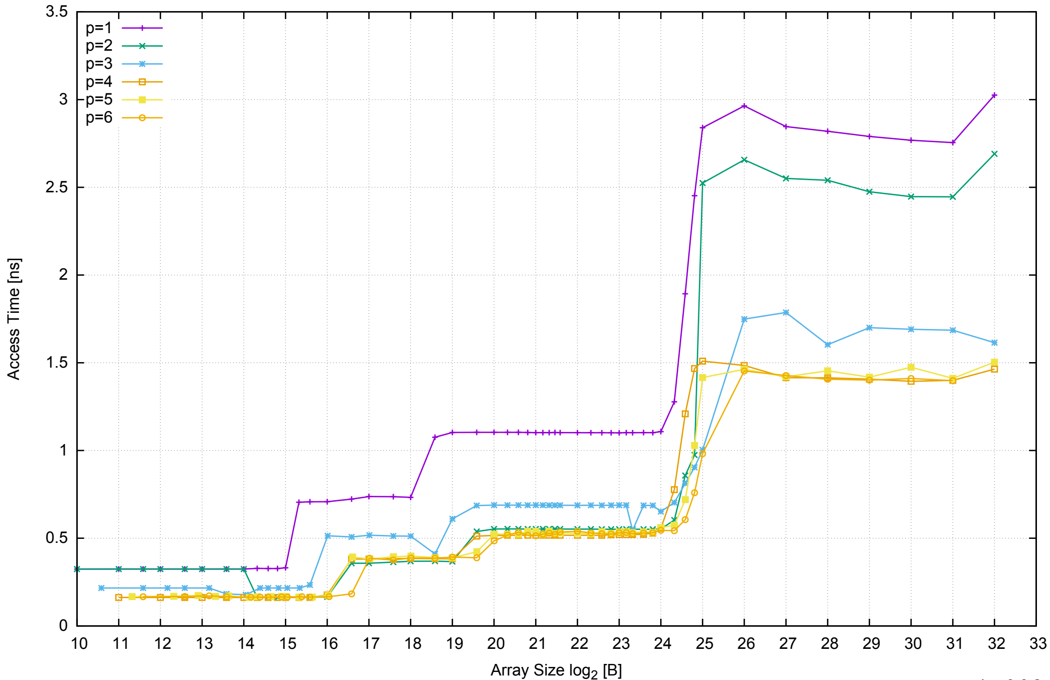
AWS c3.xlarge - Intel Xeon E5-2680 v2 2.80 GHz 7.5GB - Parallel Memory Access Time - ScanRead256PtrUnrollLoop
