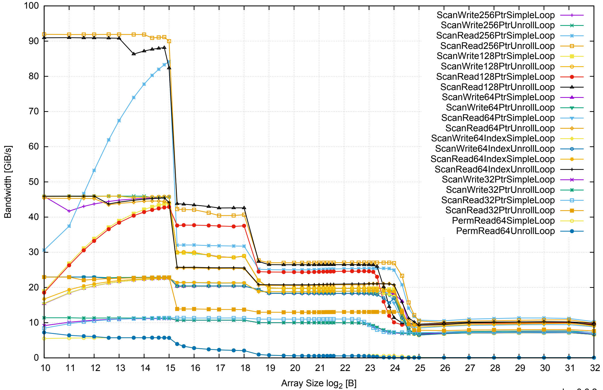
AWS c3.xlarge - Intel Xeon E5-2680 v2 2.80 GHz 7.5GB - One Thread Memory Bandwidth
