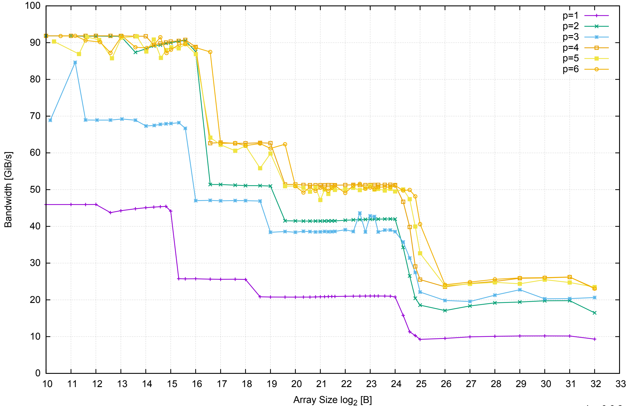
AWS c3.xlarge - Intel Xeon E5-2680 v2 2.80 GHz 7.5GB - Parallel Memory Bandwidth - ScanRead64IndexUnrollLoop
