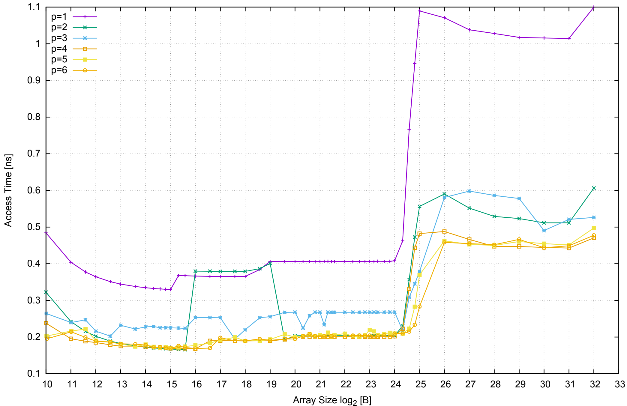
AWS c3.xlarge - Intel Xeon E5-2680 v2 2.80 GHz 7.5GB - Parallel Memory Access Time - ScanWrite64PtrSimpleLoop
