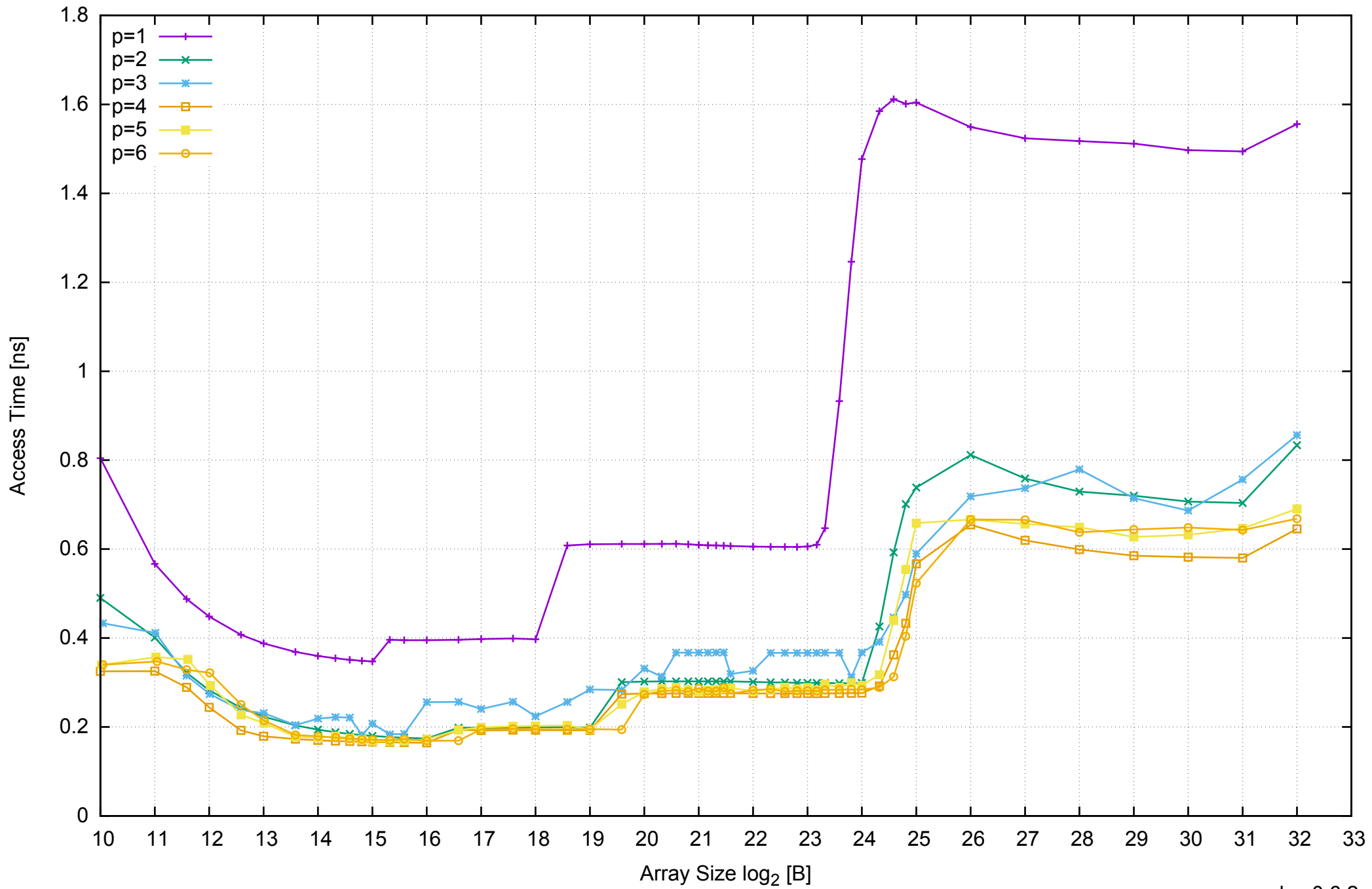
AWS c3.xlarge - Intel Xeon E5-2680 v2 2.80 GHz 7.5GB - Parallel Memory Access Time - ScanRead128PtrSimpleLoop
