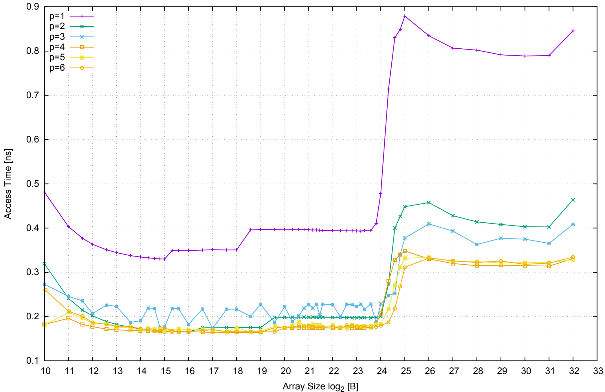
AWS c3.xlarge - Intel Xeon E5-2680 v2 2.80 GHz 7.5GB - Parallel Memory Access Time - ScanRead64PtrSimpleLoop
