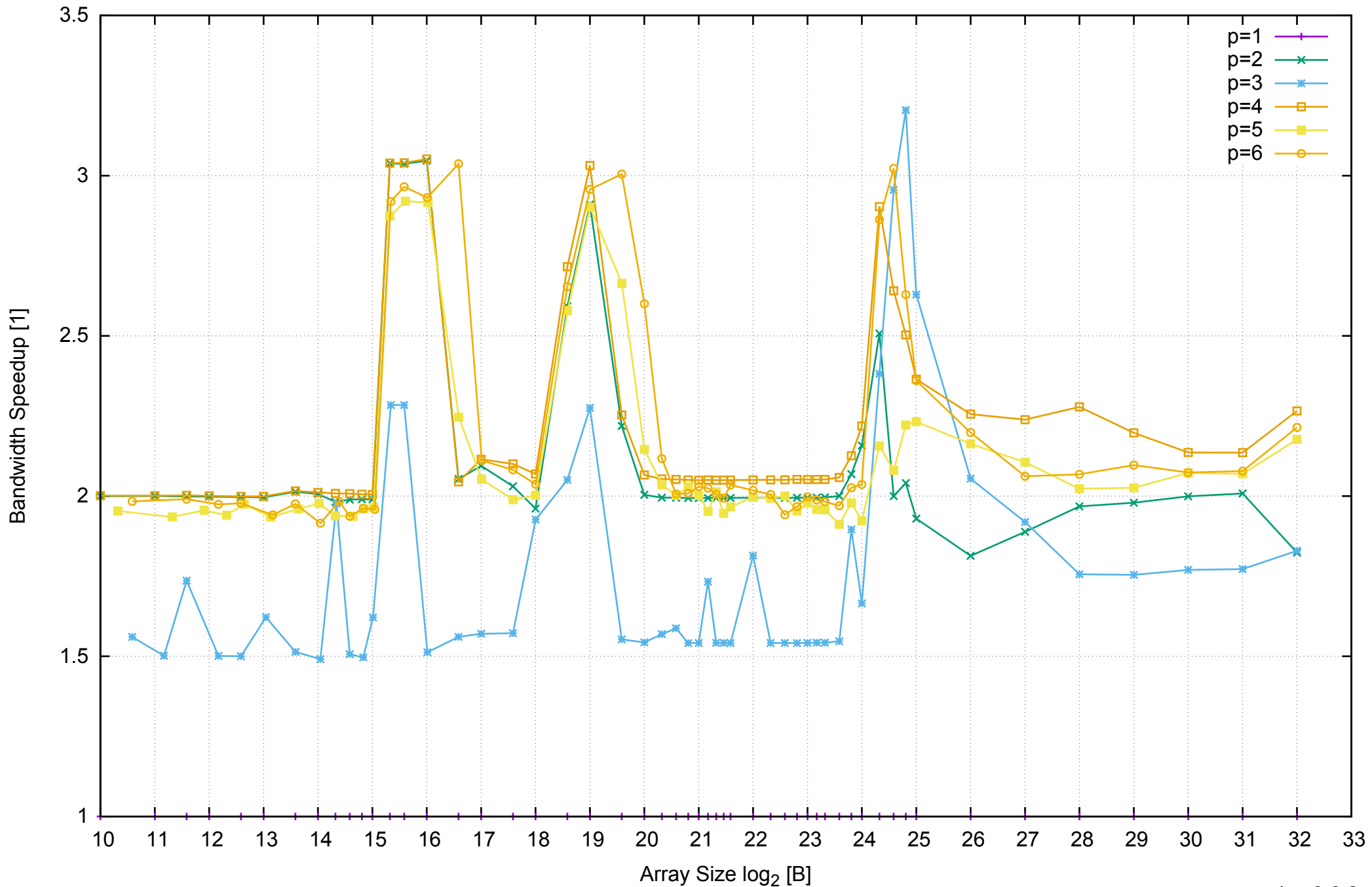
AWS c3.xlarge - Intel Xeon E5-2680 v2 2.80 GHz 7.5GB - Speedup of Parallel Memory Bandwidth - ScanWrite128PtrUnrollLoop
