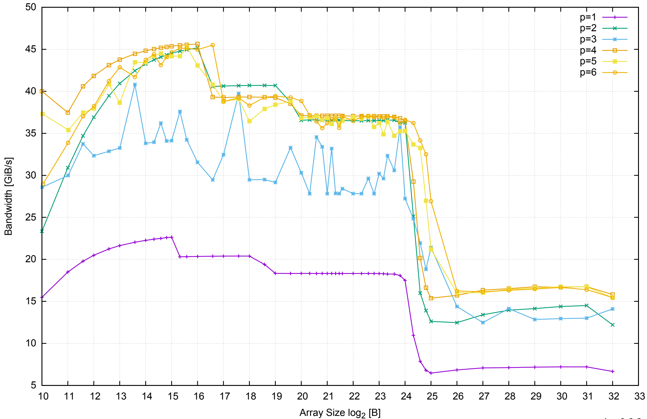
AWS c3.xlarge - Intel Xeon E5-2680 v2 2.80 GHz 7.5GB - Parallel Memory Bandwidth - ScanWrite64IndexSimpleLoop
