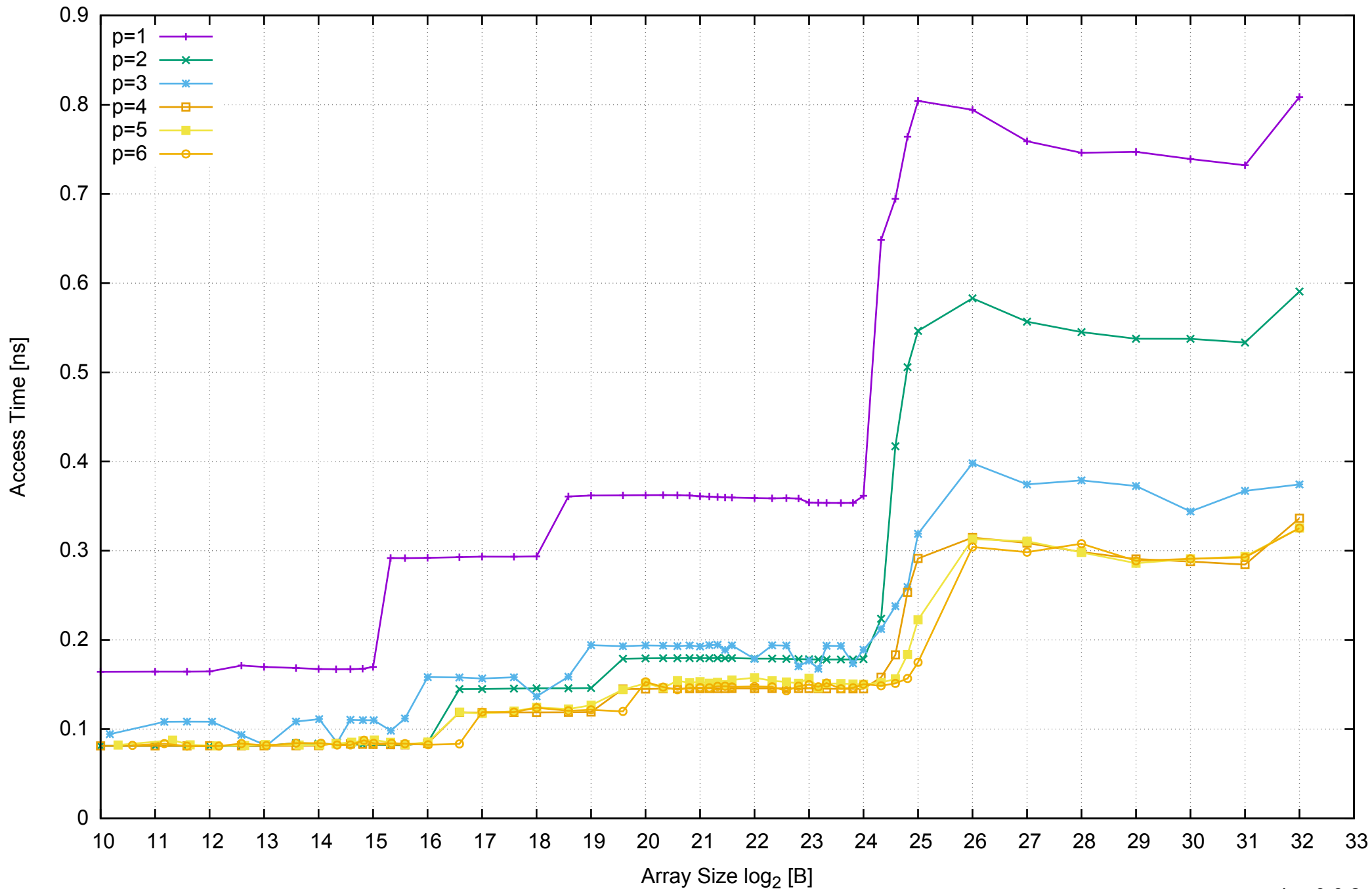
AWS c3.xlarge - Intel Xeon E5-2680 v2 2.80 GHz 7.5GB - Parallel Memory Access Time - ScanRead64PtrUnrollLoop
