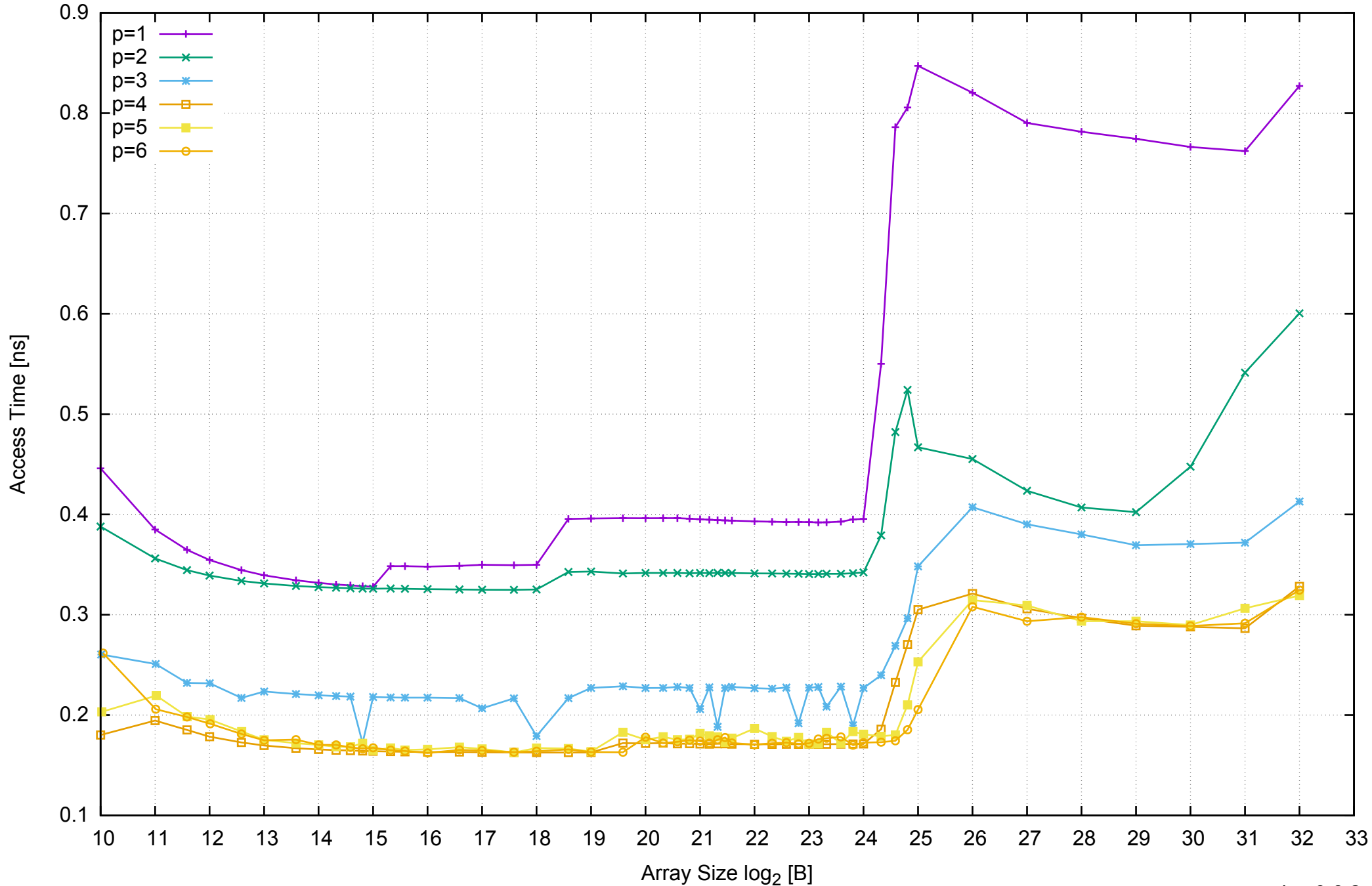
AWS c3.xlarge - Intel Xeon E5-2680 v2 2.80 GHz 7.5GB - Parallel Memory Access Time - ScanRead64IndexSimpleLoop
