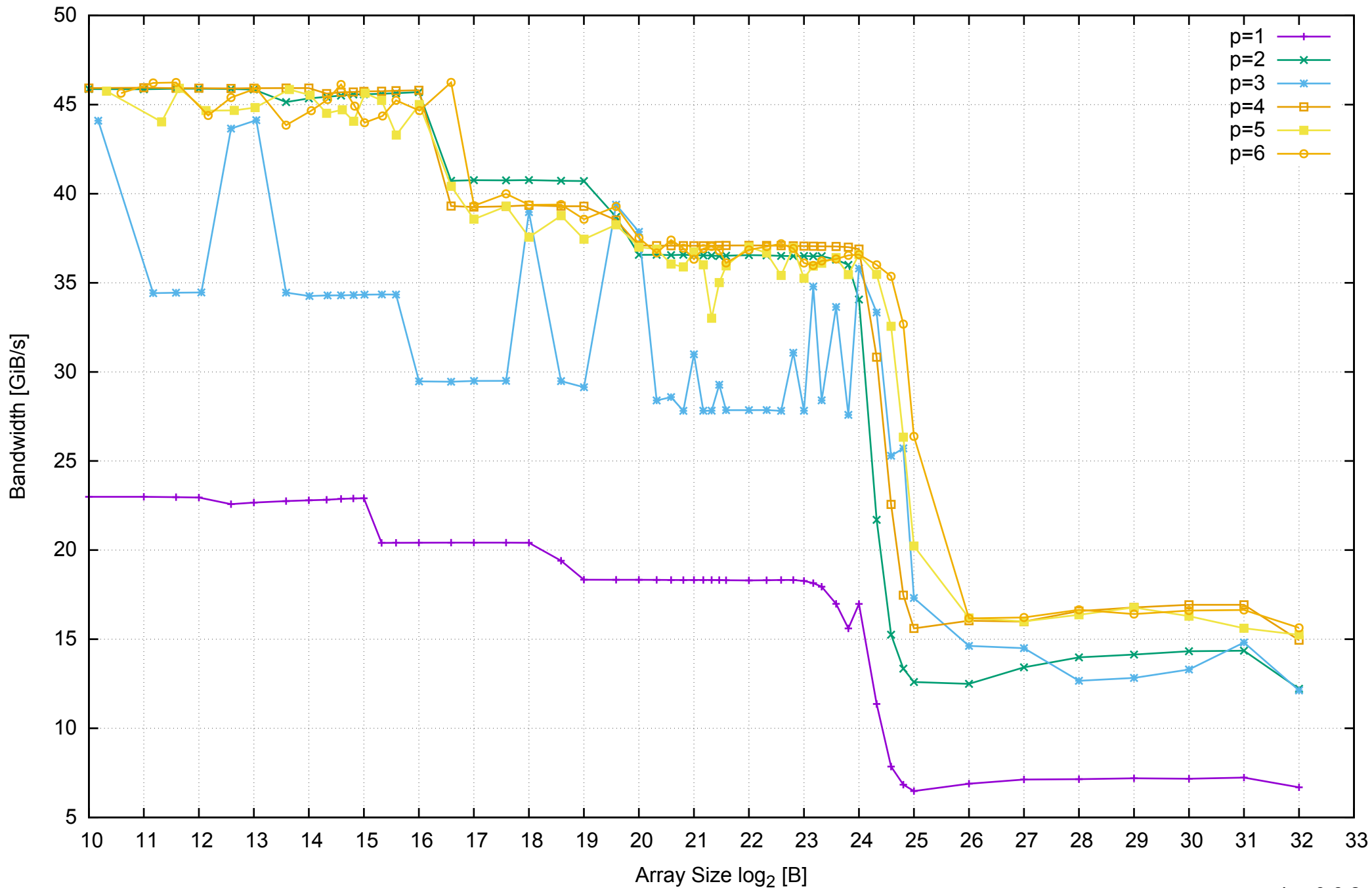
AWS c3.xlarge - Intel Xeon E5-2680 v2 2.80 GHz 7.5GB - Parallel Memory Bandwidth - ScanWrite64IndexUnrollLoop
