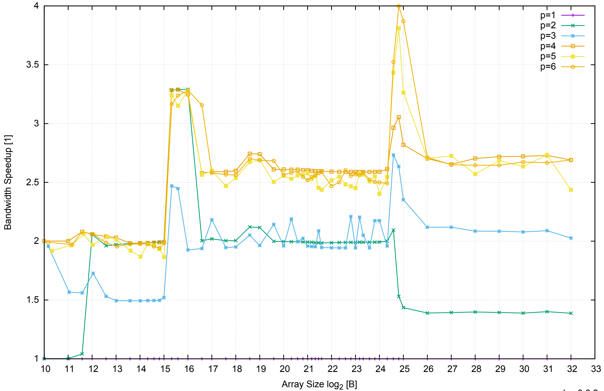
AWS c3.xlarge - Intel Xeon E5-2680 v2 2.80 GHz 7.5GB - Speedup of Parallel Memory Bandwidth - ScanRead32PtrUnrollLoop
