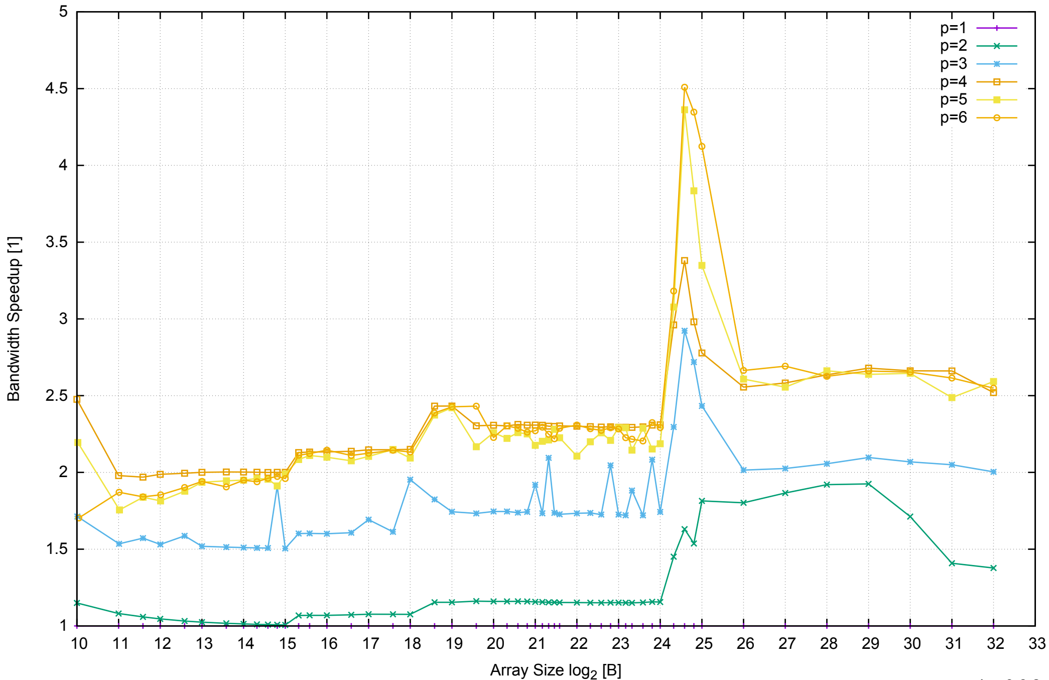
AWS c3.xlarge - Intel Xeon E5-2680 v2 2.80 GHz 7.5GB - Speedup of Parallel Memory Bandwidth - ScanRead64IndexSimpleLoop
