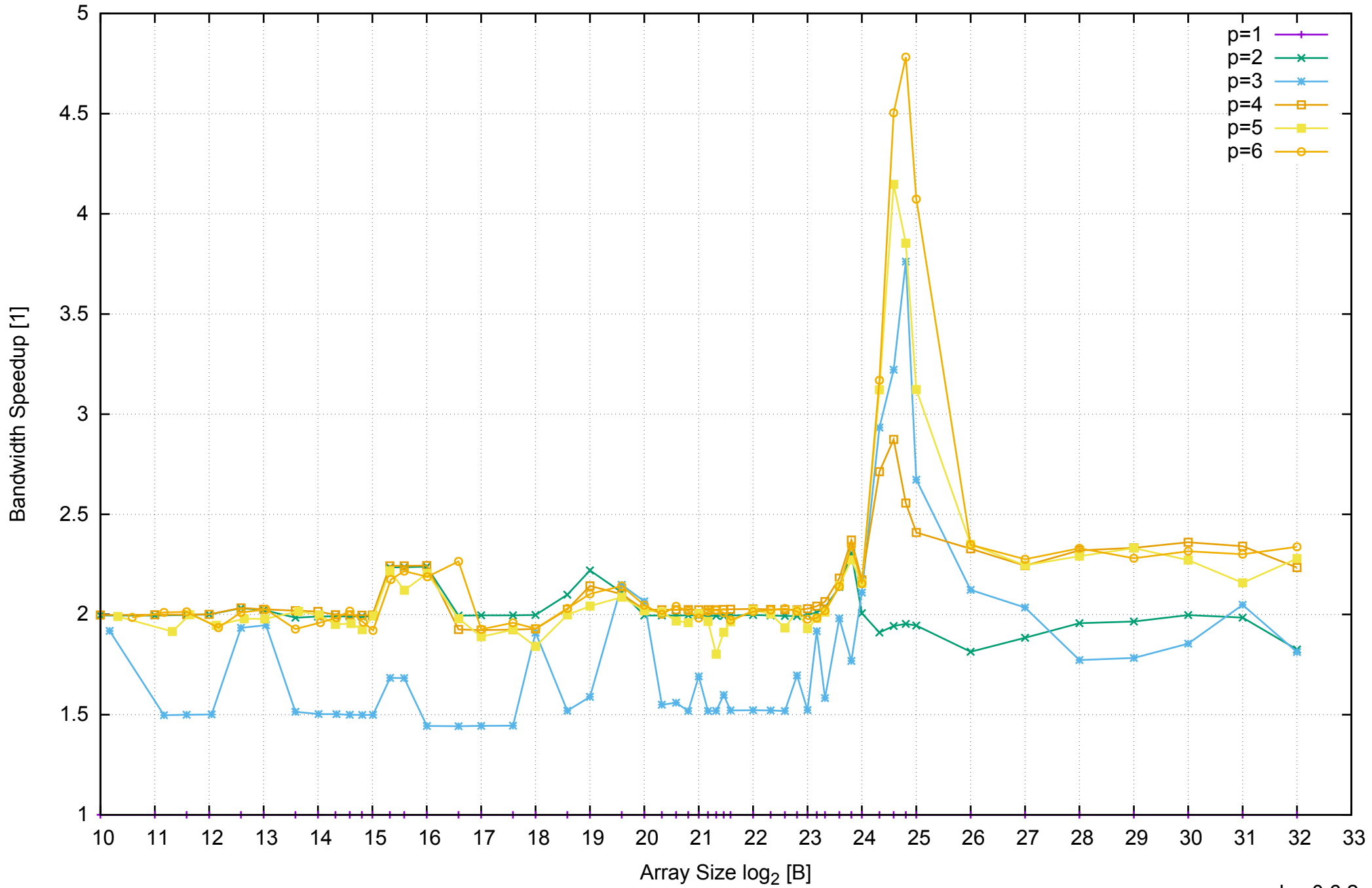
AWS c3.xlarge - Intel Xeon E5-2680 v2 2.80 GHz 7.5GB - Speedup of Parallel Memory Bandwidth - ScanWrite64IndexUnrollLoop
