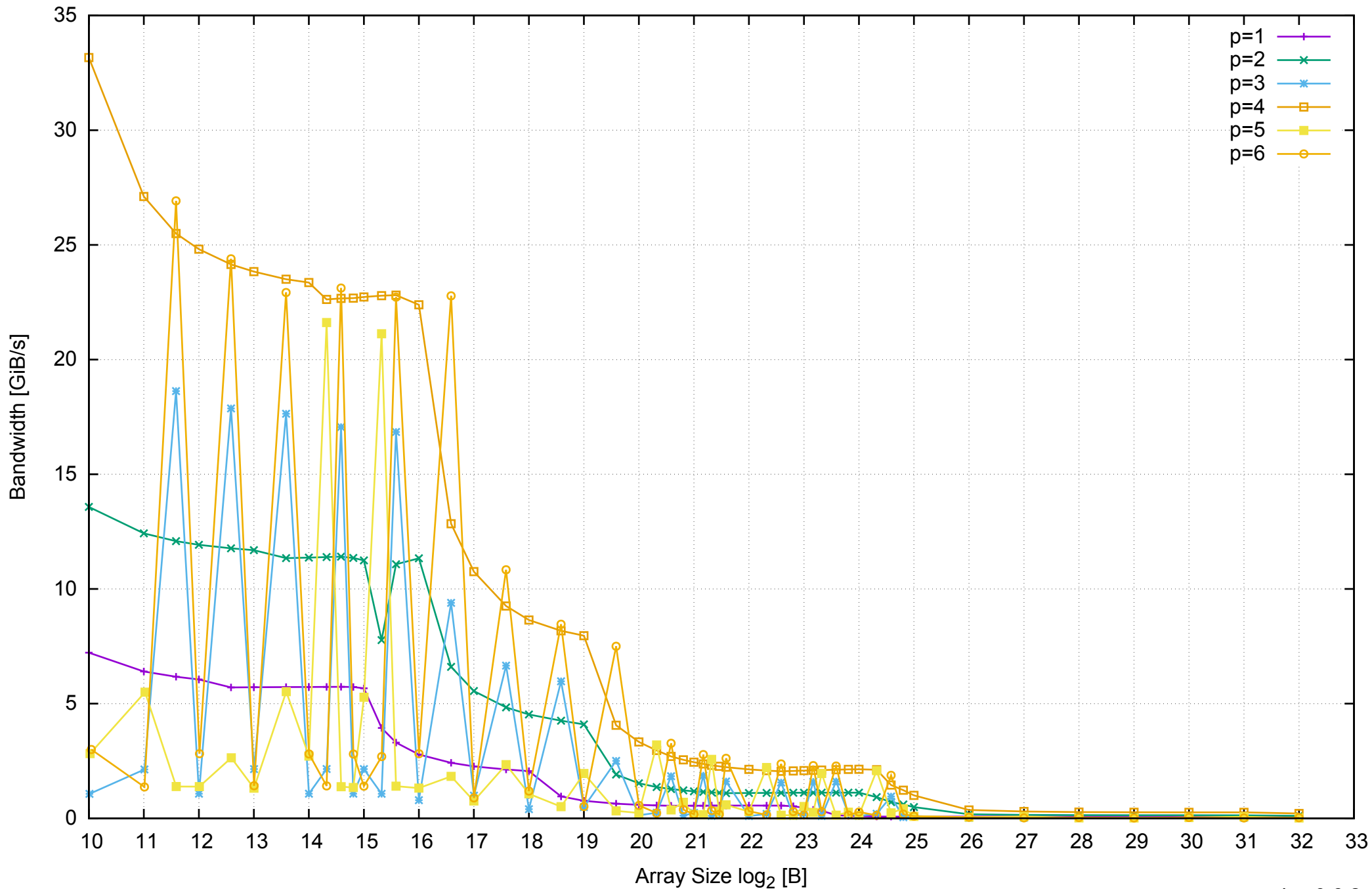
AWS c3.xlarge - Intel Xeon E5-2680 v2 2.80 GHz 7.5GB - Parallel Memory Bandwidth - PermRead64UnrollLoop
