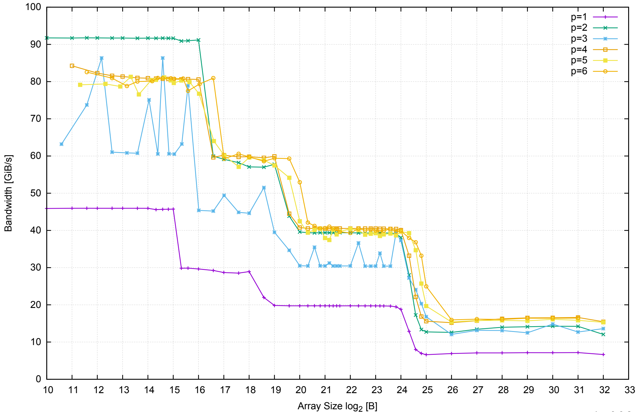
AWS c3.xlarge - Intel Xeon E5-2680 v2 2.80 GHz 7.5GB - Parallel Memory Bandwidth - ScanWrite256PtrUnrollLoop
