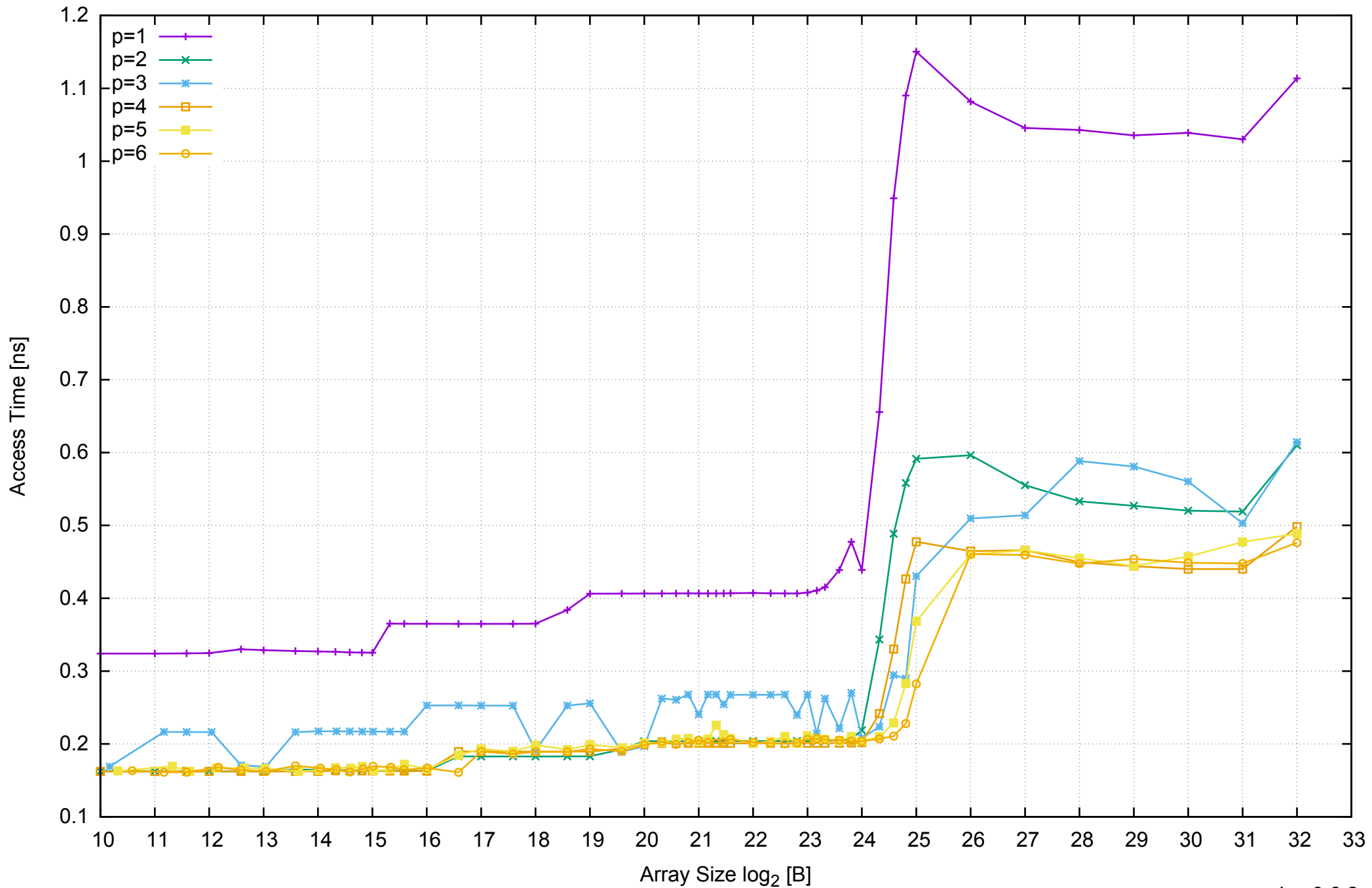
AWS c3.xlarge - Intel Xeon E5-2680 v2 2.80 GHz 7.5GB - Parallel Memory Access Time - ScanWrite64IndexUnrollLoop
