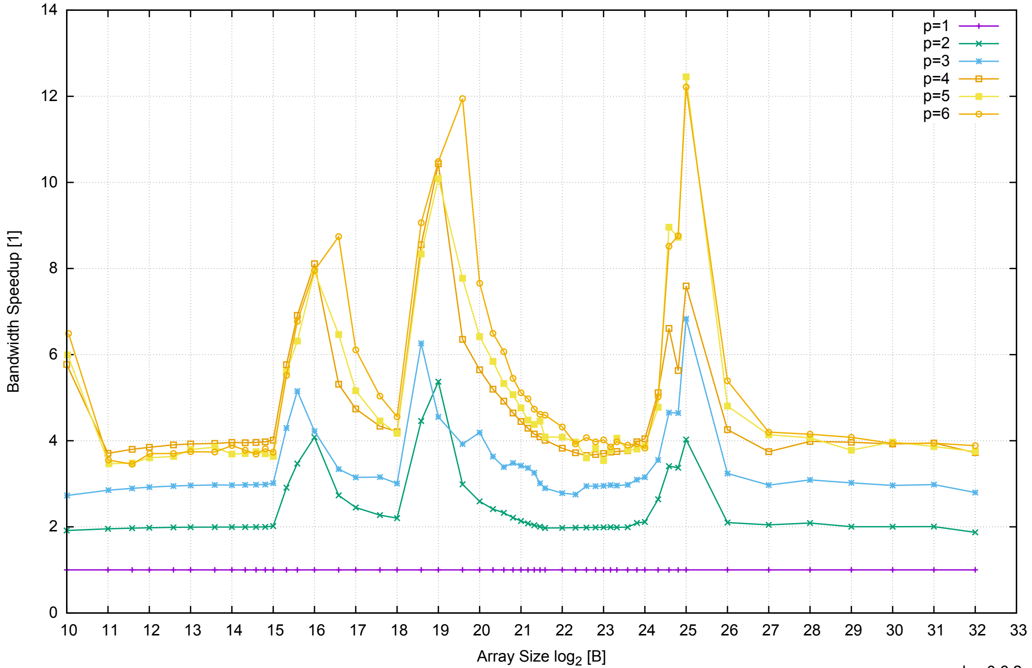
AWS c3.xlarge - Intel Xeon E5-2680 v2 2.80 GHz 7.5GB - Speedup of Parallel Memory Bandwidth - PermRead64SimpleLoop
