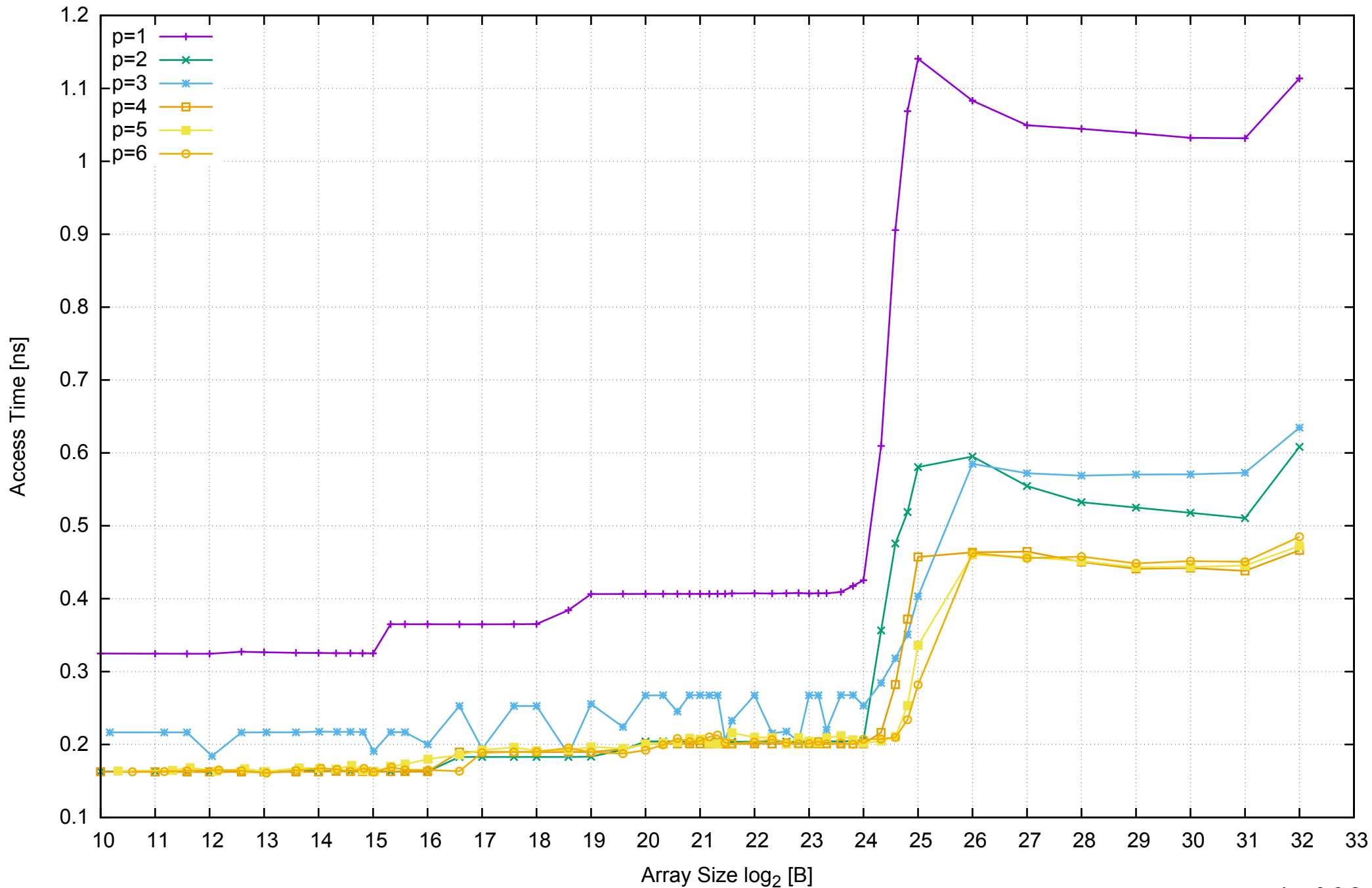
AWS c3.xlarge - Intel Xeon E5-2680 v2 2.80 GHz 7.5GB - Parallel Memory Access Time - ScanWrite64PtrUnrollLoop
