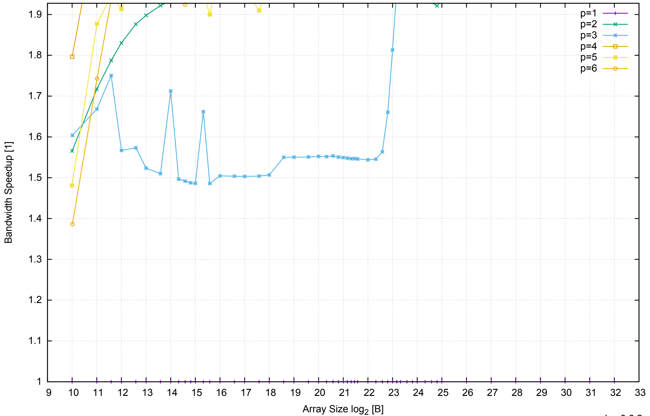
AWS c3.xlarge - Intel Xeon E5-2680 v2 2.80 GHz 7.5GB - Speedup of Parallel Memory Bandwidth (enlarged) - ScanRead32PtrSimpleLoop
