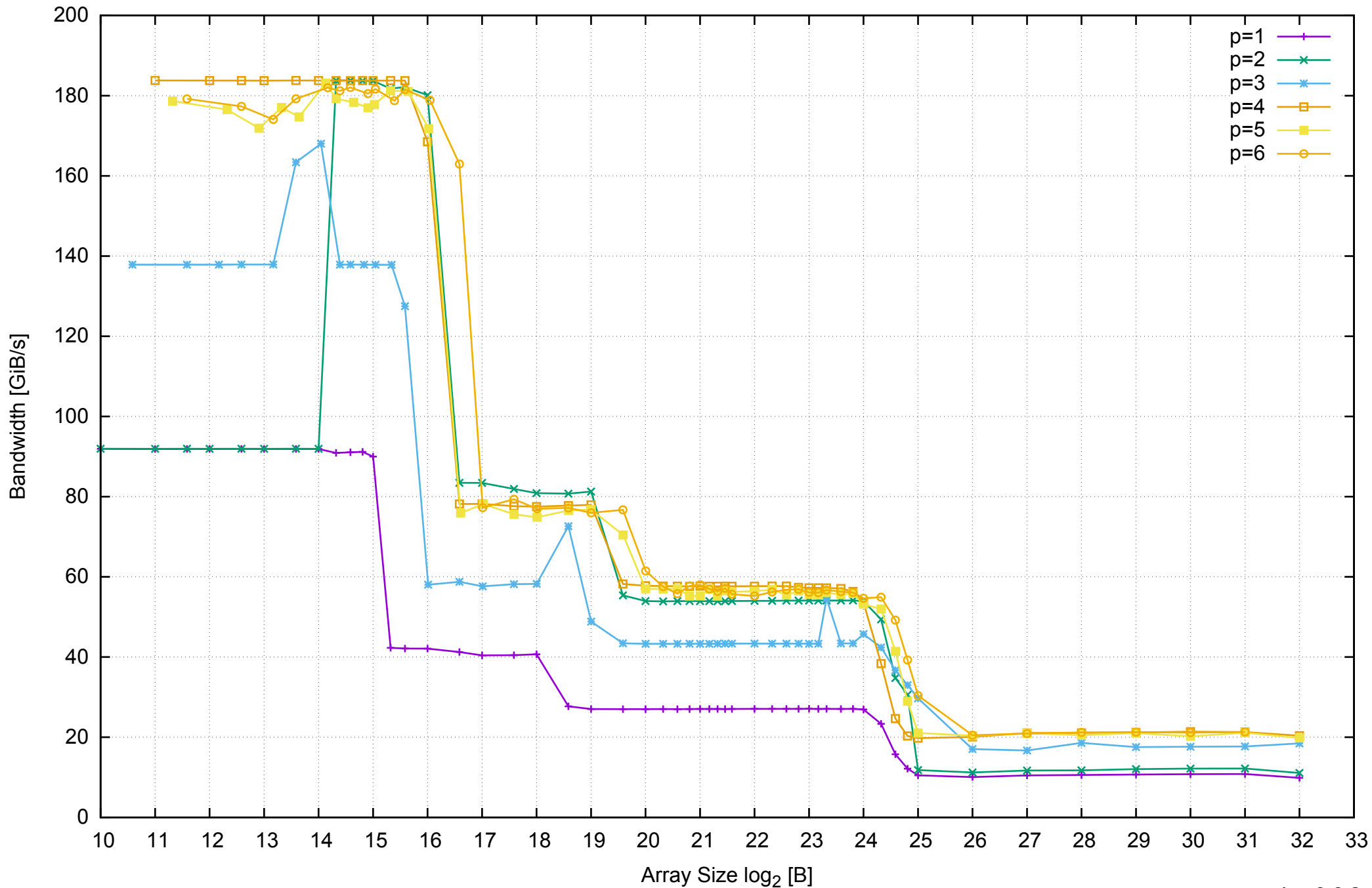
AWS c3.xlarge - Intel Xeon E5-2680 v2 2.80 GHz 7.5GB - Parallel Memory Bandwidth - ScanRead256PtrUnrollLoop
