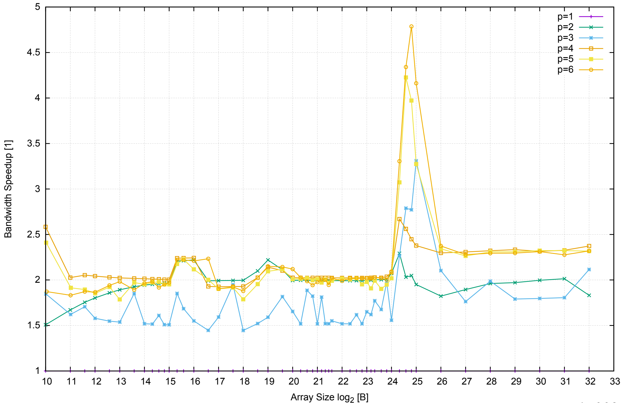
AWS c3.xlarge - Intel Xeon E5-2680 v2 2.80 GHz 7.5GB - Speedup of Parallel Memory Bandwidth - ScanWrite64IndexSimpleLoop
