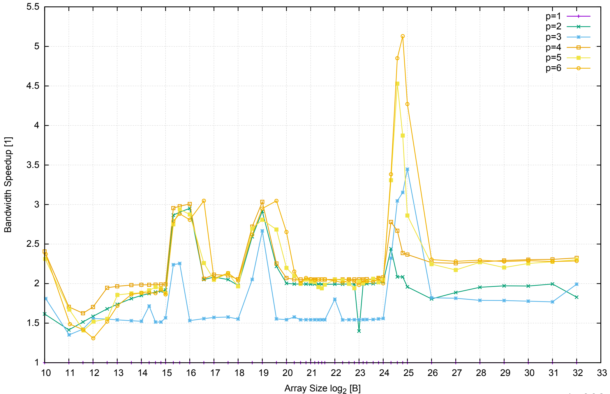
AWS c3.xlarge - Intel Xeon E5-2680 v2 2.80 GHz 7.5GB - Speedup of Parallel Memory Bandwidth - ScanWrite128PtrSimpleLoop
