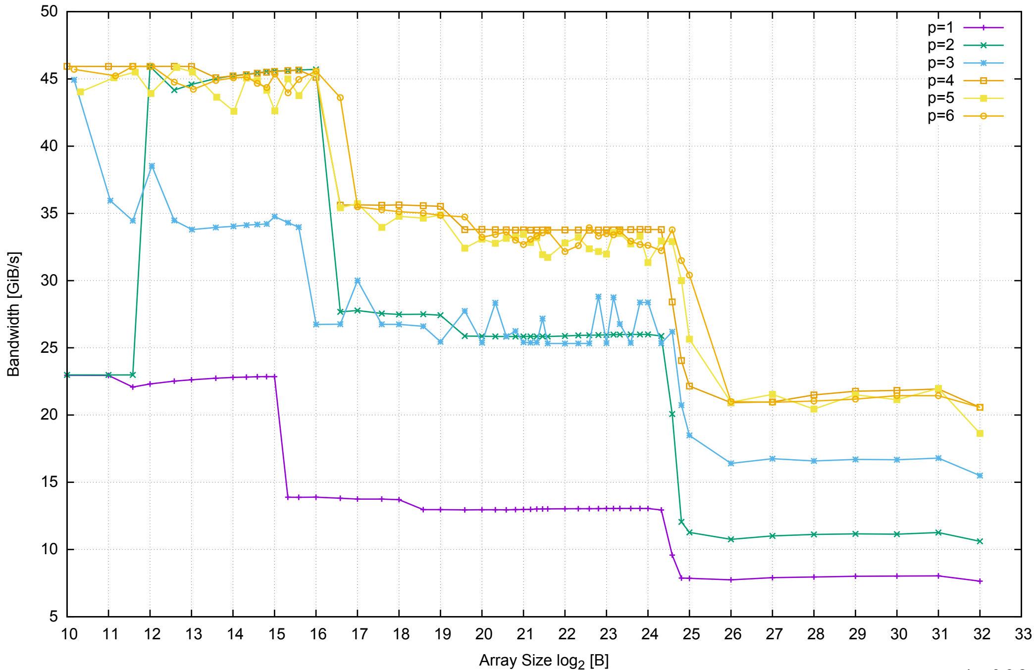
AWS c3.xlarge - Intel Xeon E5-2680 v2 2.80 GHz 7.5GB - Parallel Memory Bandwidth - ScanRead32PtrUnrollLoop
