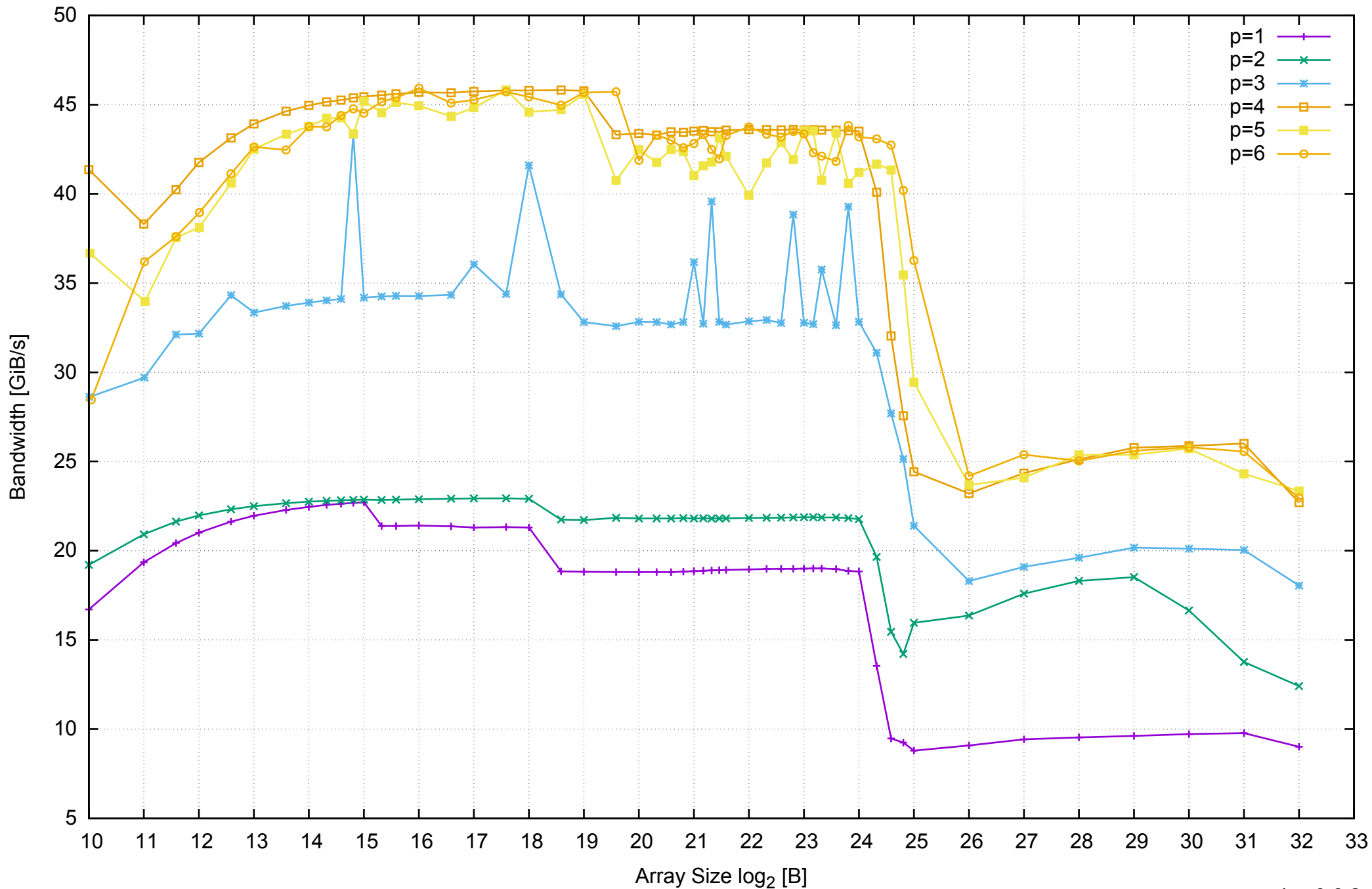
AWS c3.xlarge - Intel Xeon E5-2680 v2 2.80 GHz 7.5GB - Parallel Memory Bandwidth - ScanRead64IndexSimpleLoop
