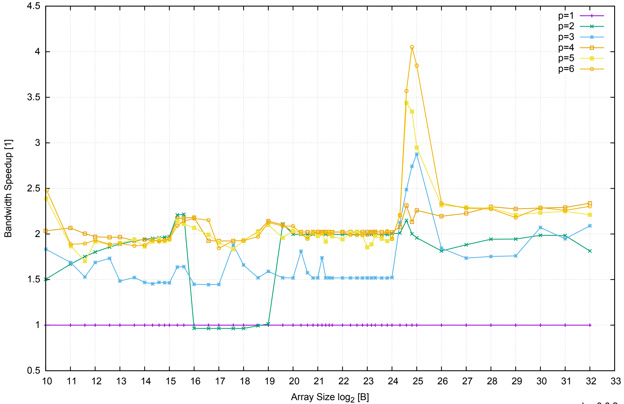
AWS c3.xlarge - Intel Xeon E5-2680 v2 2.80 GHz 7.5GB - Speedup of Parallel Memory Bandwidth - ScanWrite64PtrSimpleLoop
