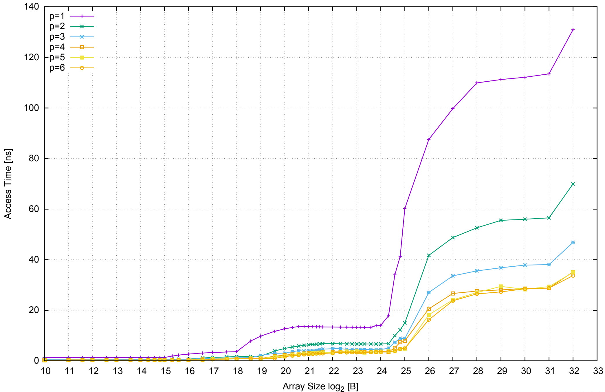
AWS c3.xlarge - Intel Xeon E5-2680 v2 2.80 GHz 7.5GB - Parallel Memory Access Time - PermRead64SimpleLoop
