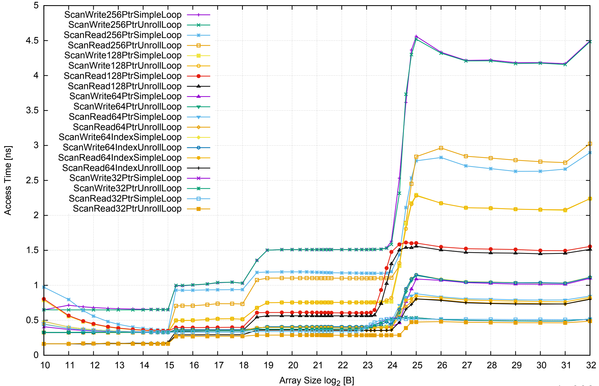
AWS c3.xlarge - Intel Xeon E5-2680 v2 2.80 GHz 7.5GB - One Thread Memory Latency (excluding Permutation)
