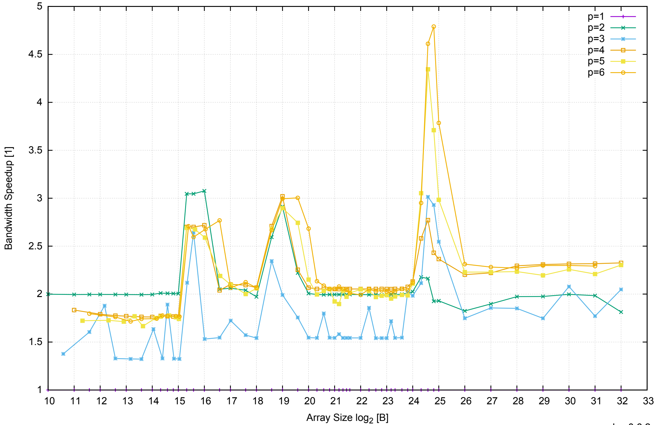
AWS c3.xlarge - Intel Xeon E5-2680 v2 2.80 GHz 7.5GB - Speedup of Parallel Memory Bandwidth - ScanWrite256PtrUnrollLoop
