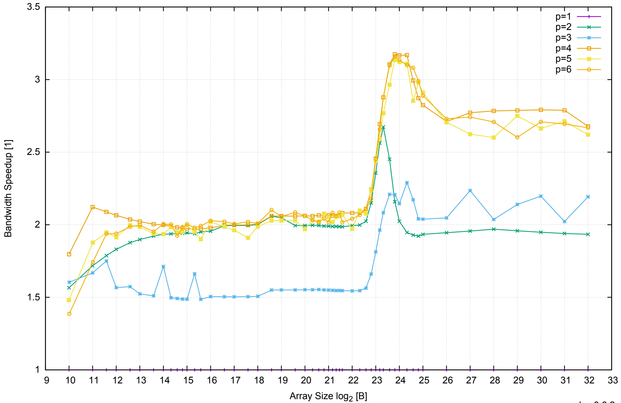
AWS c3.xlarge - Intel Xeon E5-2680 v2 2.80 GHz 7.5GB - Speedup of Parallel Memory Bandwidth - ScanRead32PtrSimpleLoop
