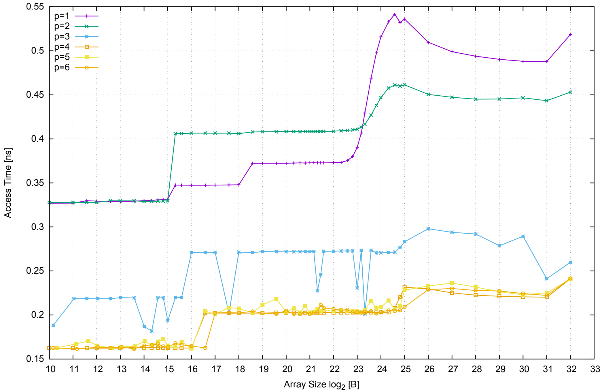
AWS c3.xlarge - Intel Xeon E5-2680 v2 2.80 GHz 7.5GB - Parallel Memory Access Time - ScanWrite32PtrUnrollLoop
