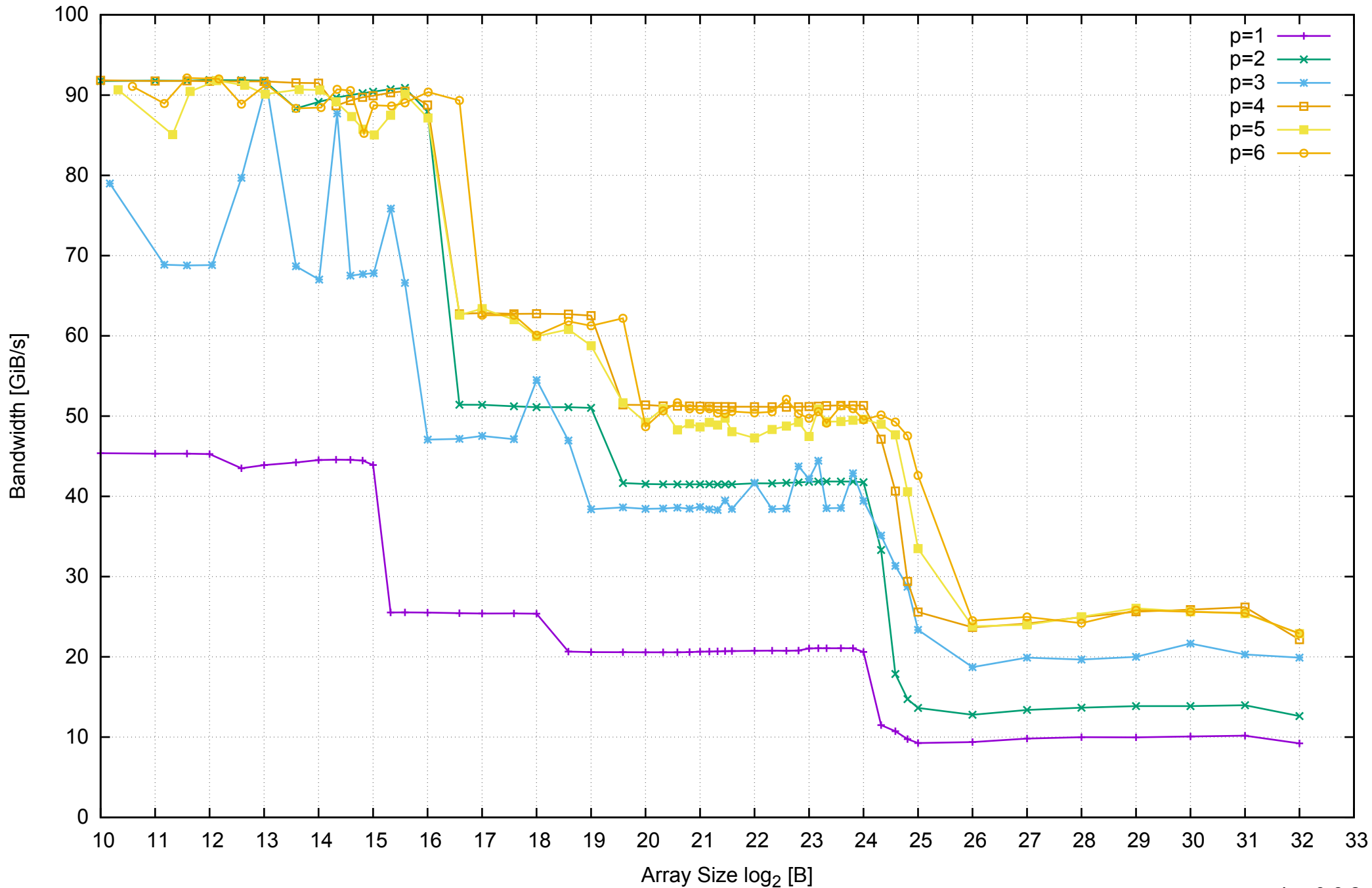
AWS c3.xlarge - Intel Xeon E5-2680 v2 2.80 GHz 7.5GB - Parallel Memory Bandwidth - ScanRead64PtrUnrollLoop
