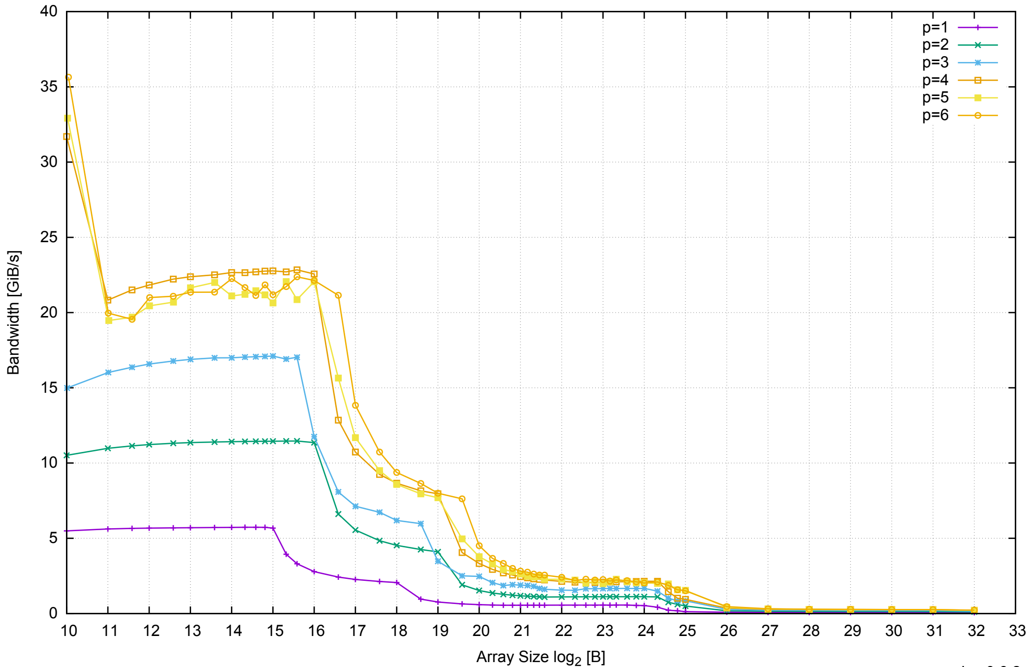
AWS c3.xlarge - Intel Xeon E5-2680 v2 2.80 GHz 7.5GB - Parallel Memory Bandwidth - PermRead64SimpleLoop
