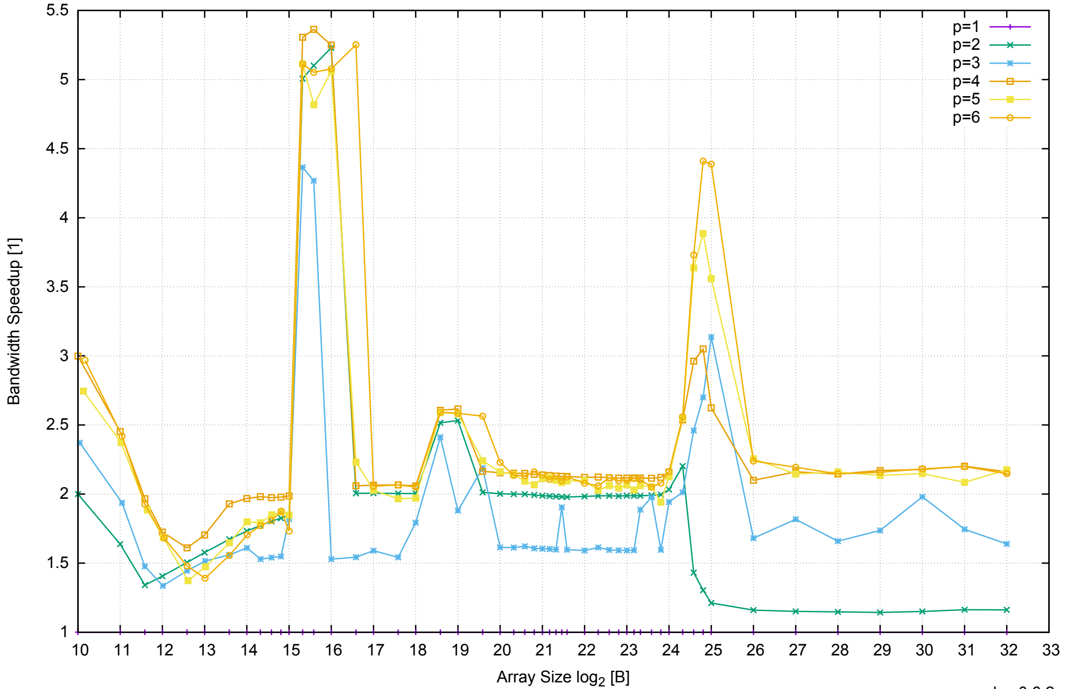
AWS c3.xlarge - Intel Xeon E5-2680 v2 2.80 GHz 7.5GB - Speedup of Parallel Memory Bandwidth - ScanRead256PtrSimpleLoop
