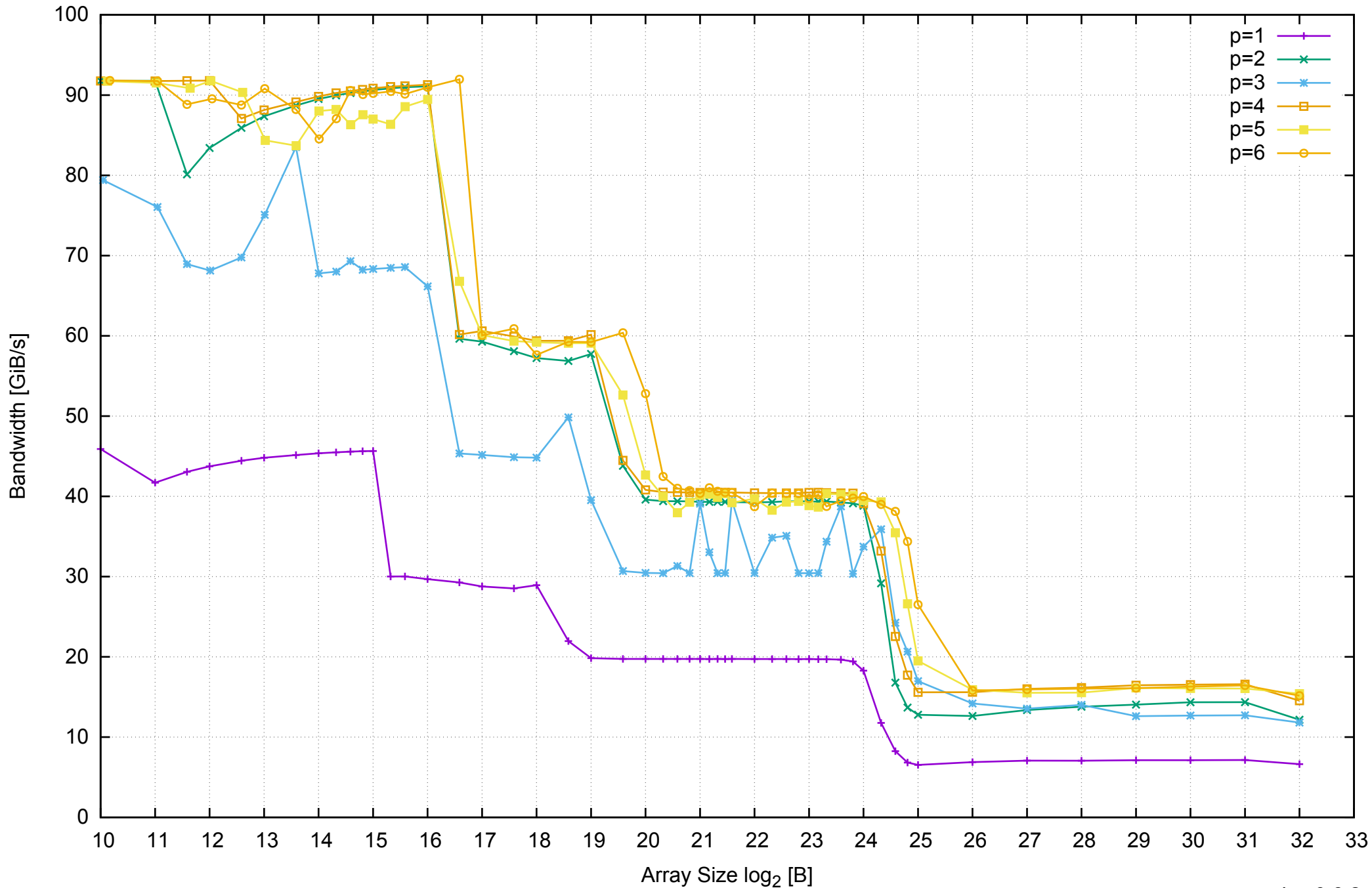
AWS c3.xlarge - Intel Xeon E5-2680 v2 2.80 GHz 7.5GB - Parallel Memory Bandwidth - ScanWrite256PtrSimpleLoop
