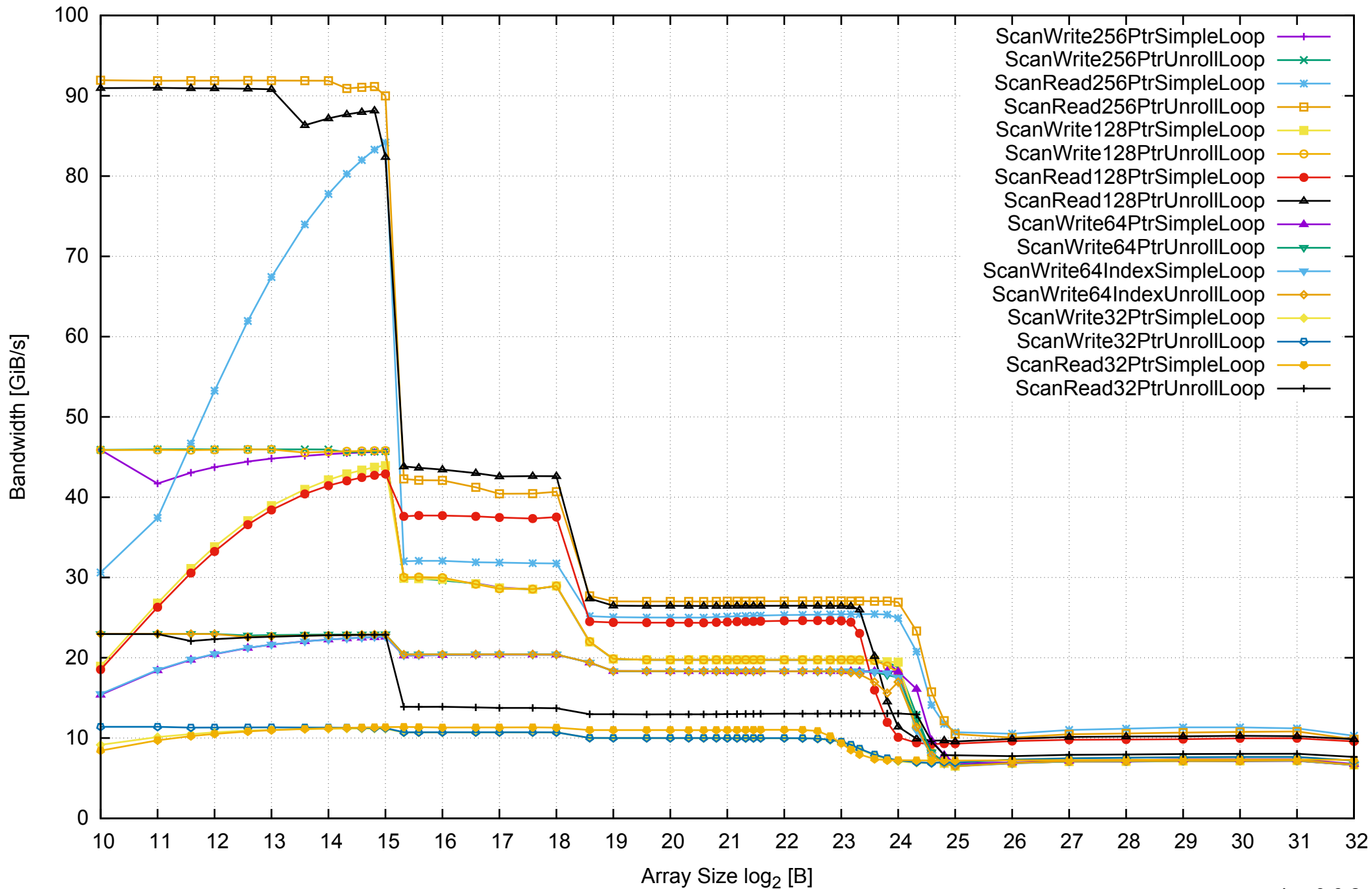
AWS c3.xlarge - Intel Xeon E5-2680 v2 2.80 GHz 7.5GB - One Thread Memory Bandwidth (only 64-bit Reads)
