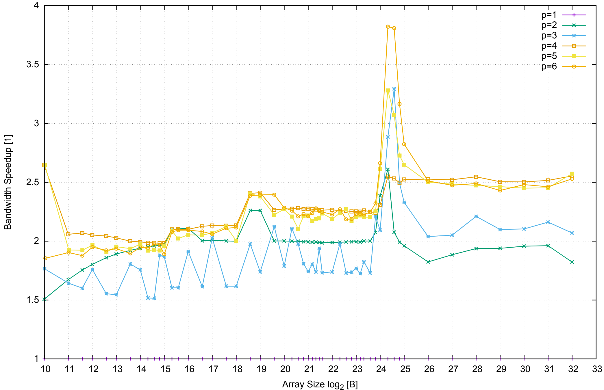
AWS c3.xlarge - Intel Xeon E5-2680 v2 2.80 GHz 7.5GB - Speedup of Parallel Memory Bandwidth - ScanRead64PtrSimpleLoop
