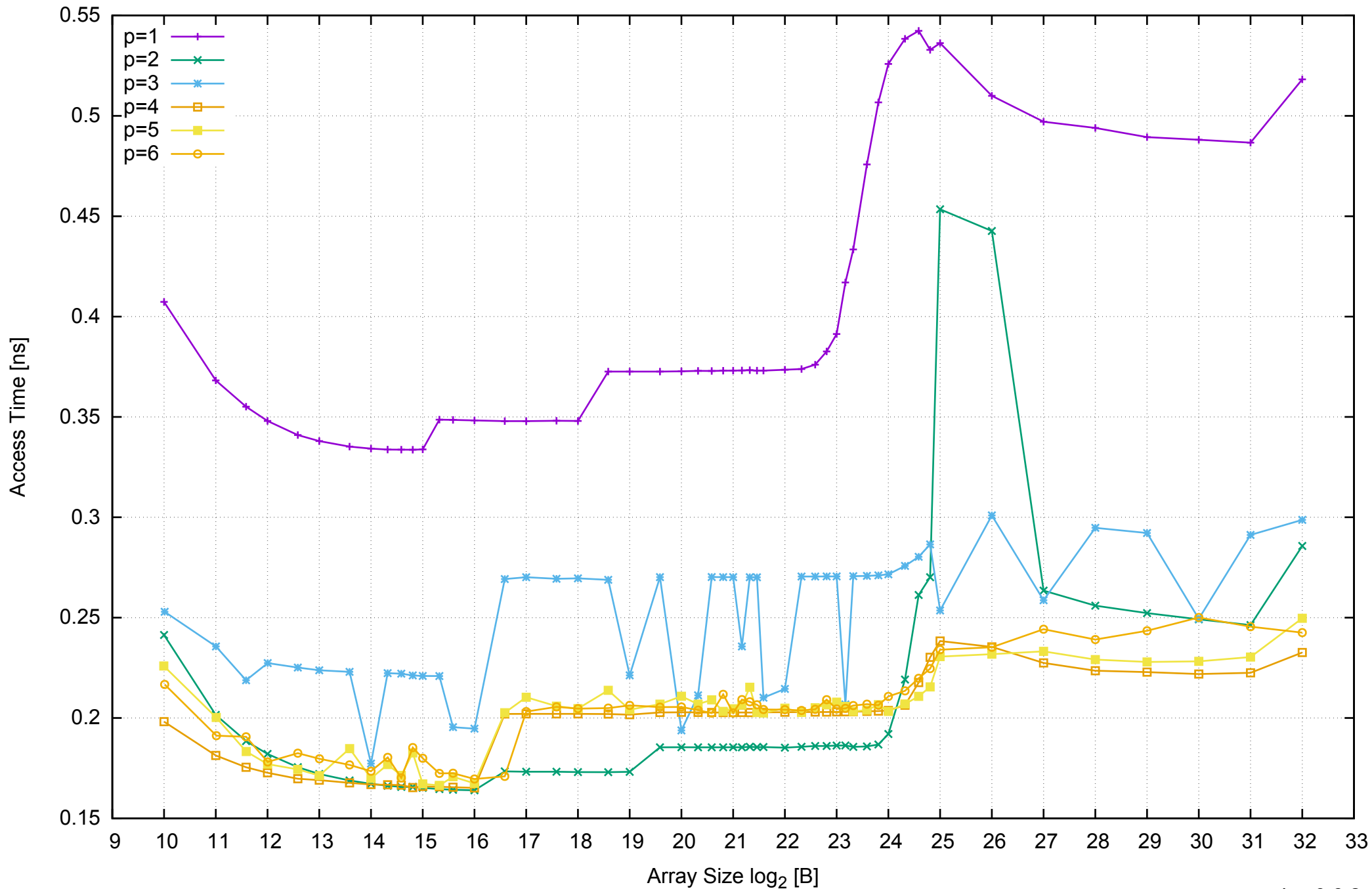
AWS c3.xlarge - Intel Xeon E5-2680 v2 2.80 GHz 7.5GB - Parallel Memory Access Time - ScanWrite32PtrSimpleLoop
