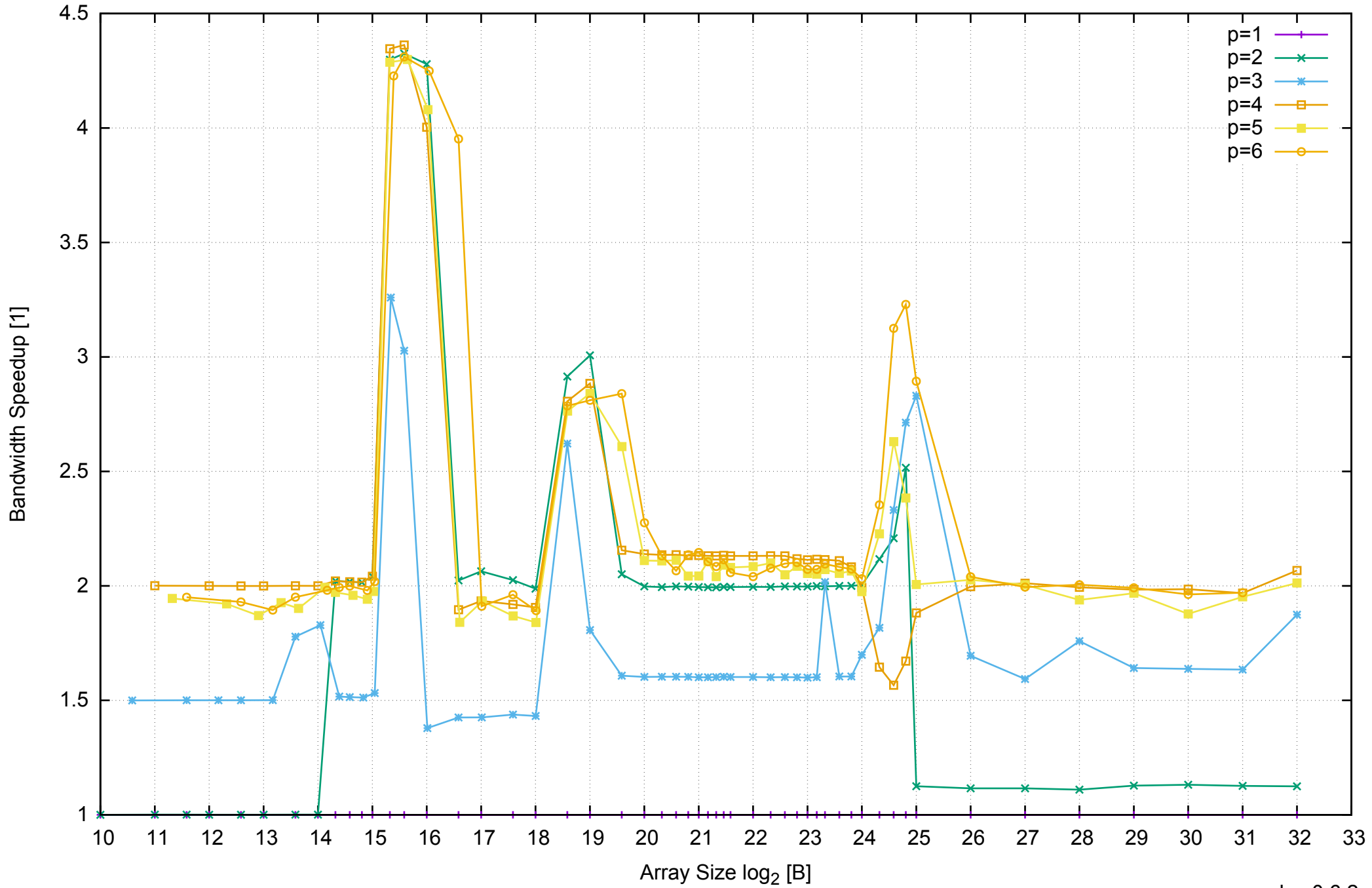
AWS c3.xlarge - Intel Xeon E5-2680 v2 2.80 GHz 7.5GB - Speedup of Parallel Memory Bandwidth - ScanRead256PtrUnrollLoop
