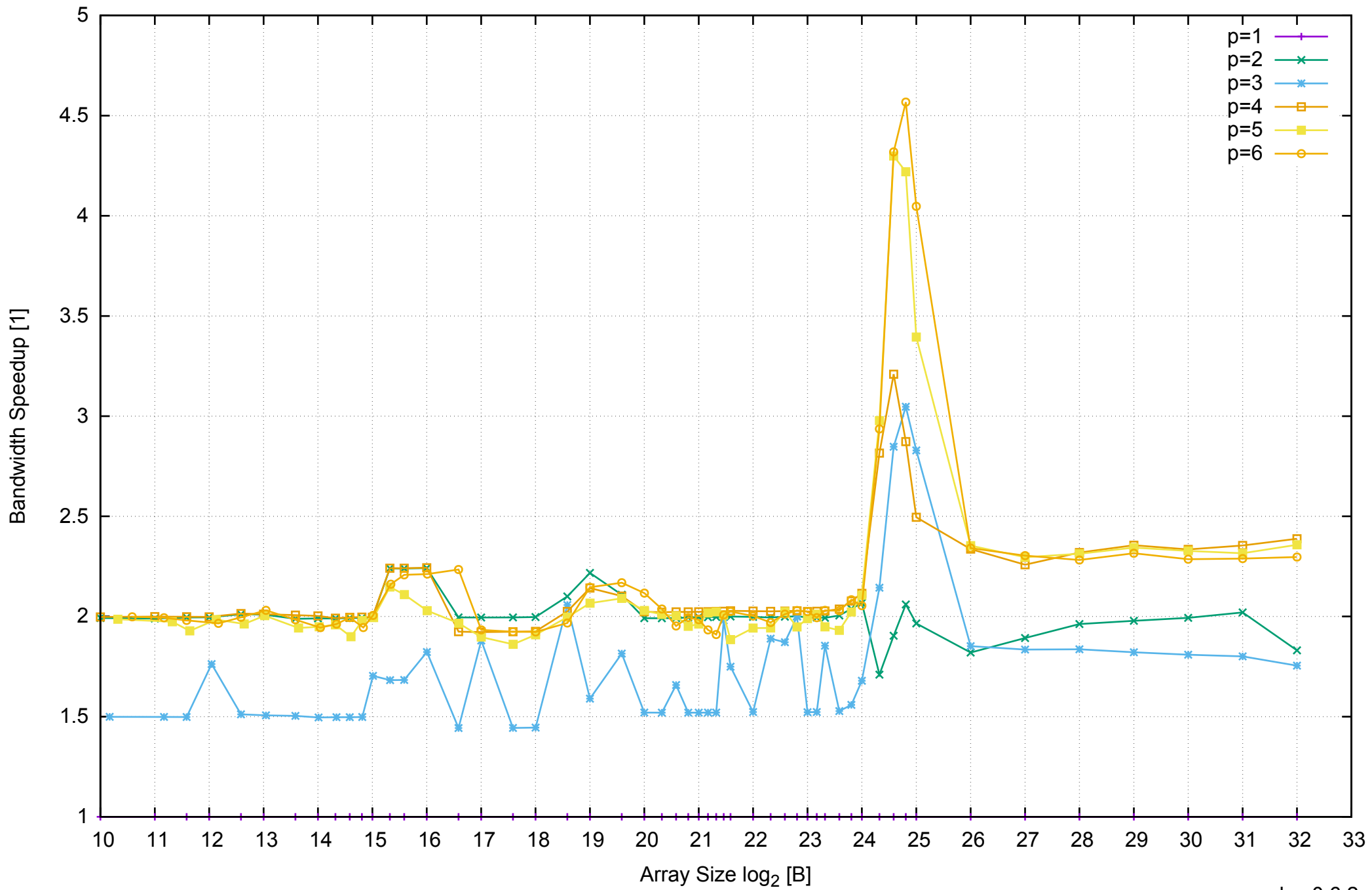
AWS c3.xlarge - Intel Xeon E5-2680 v2 2.80 GHz 7.5GB - Speedup of Parallel Memory Bandwidth - ScanWrite64PtrUnrollLoop
