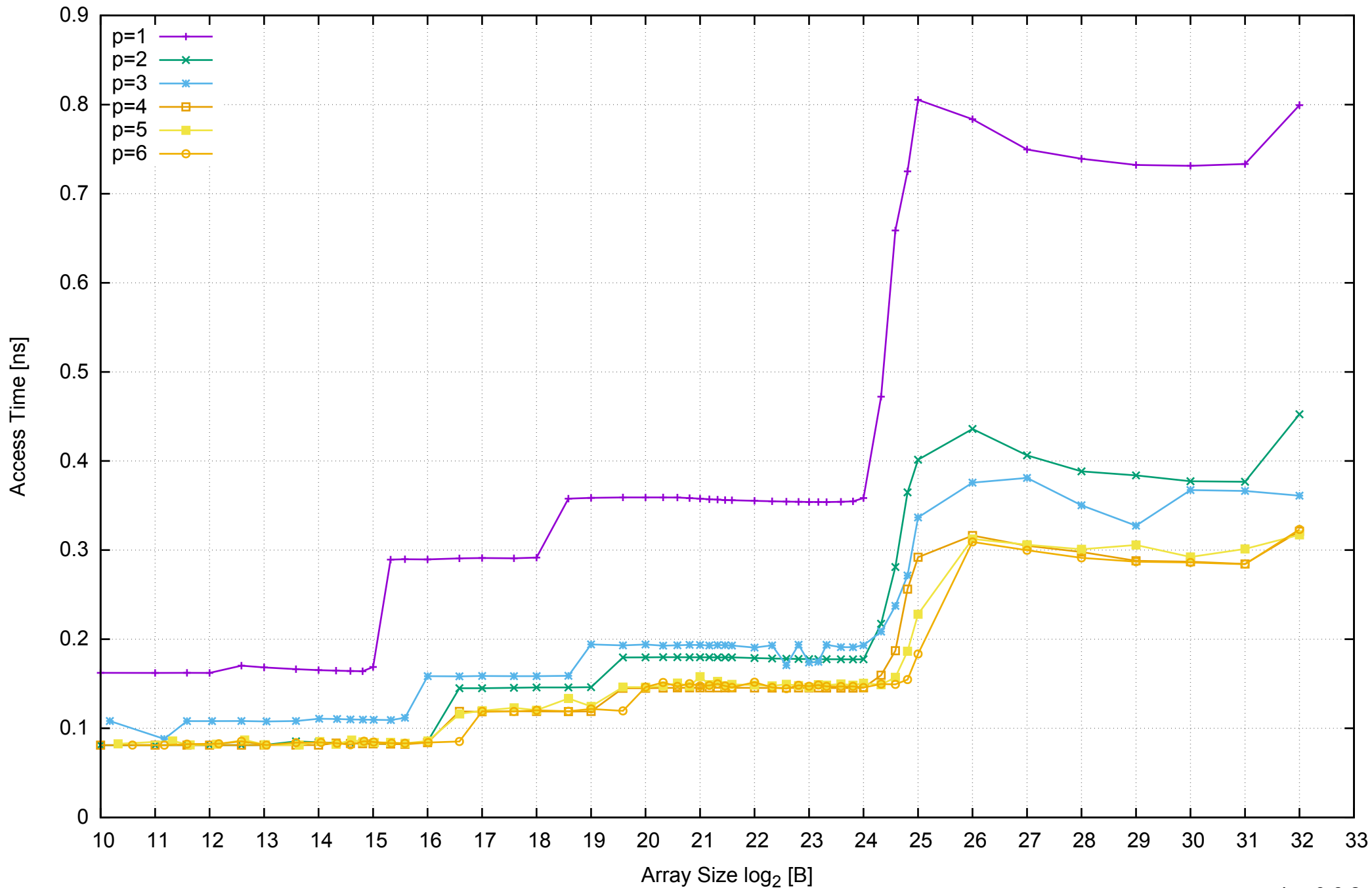
AWS c3.xlarge - Intel Xeon E5-2680 v2 2.80 GHz 7.5GB - Parallel Memory Access Time - ScanRead64IndexUnrollLoop
