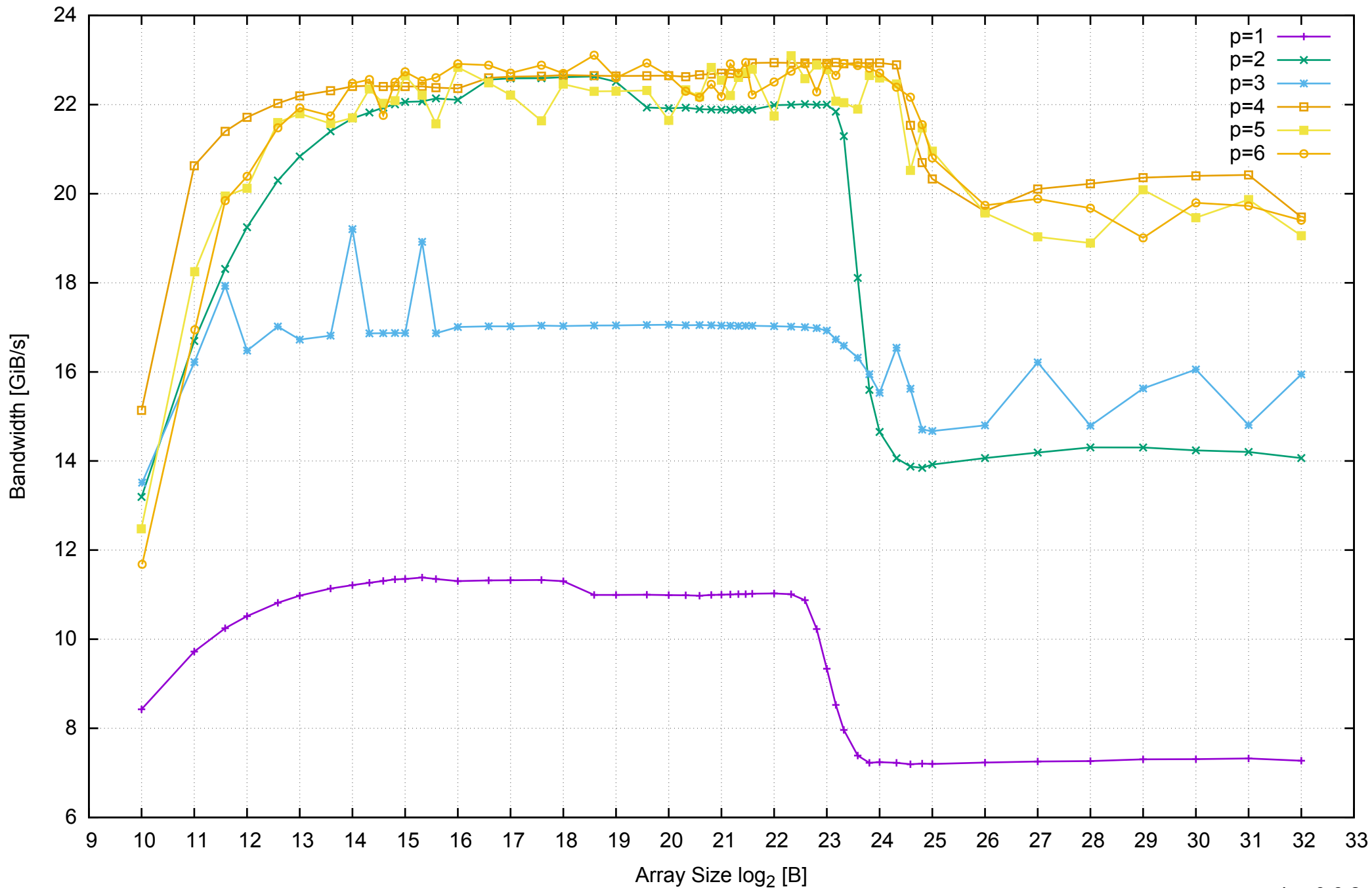
AWS c3.xlarge - Intel Xeon E5-2680 v2 2.80 GHz 7.5GB - Parallel Memory Bandwidth - ScanRead32PtrSimpleLoop
