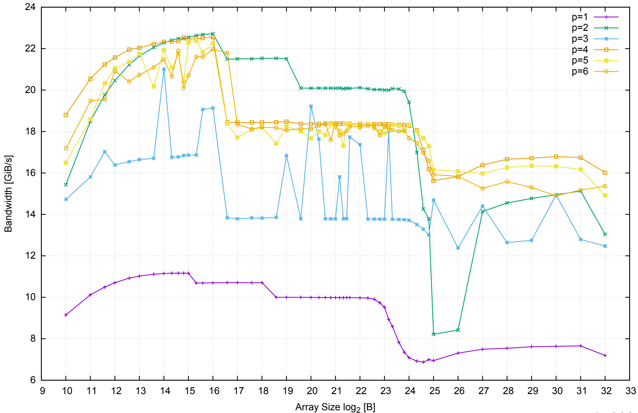
AWS c3.xlarge - Intel Xeon E5-2680 v2 2.80 GHz 7.5GB - Parallel Memory Bandwidth - ScanWrite32PtrSimpleLoop
