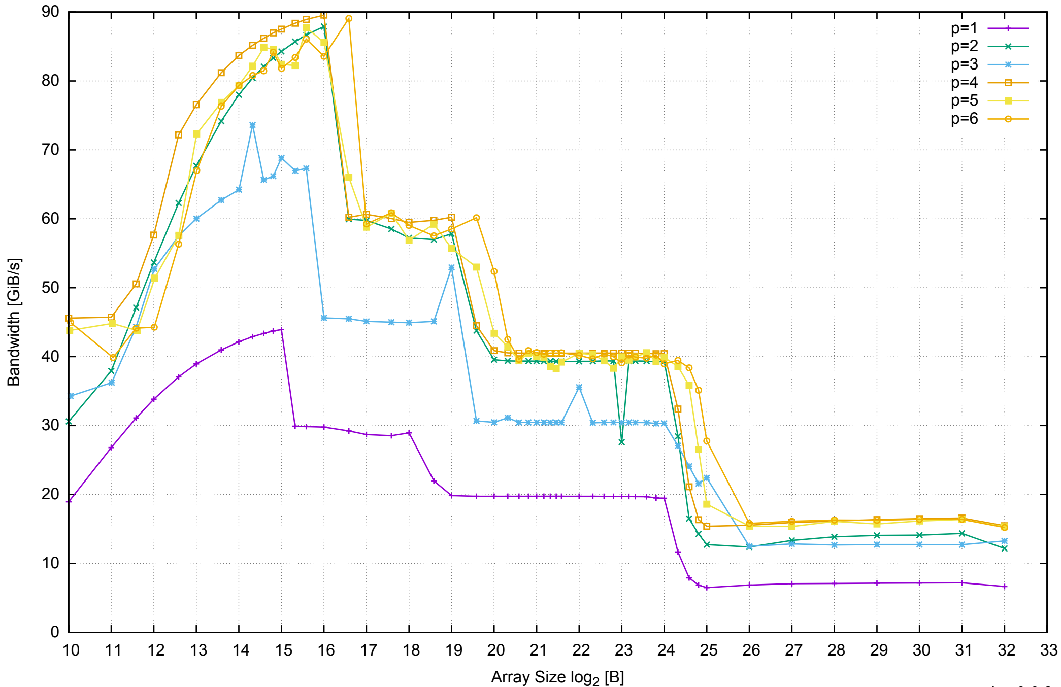
AWS c3.xlarge - Intel Xeon E5-2680 v2 2.80 GHz 7.5GB - Parallel Memory Bandwidth - ScanWrite128PtrSimpleLoop
