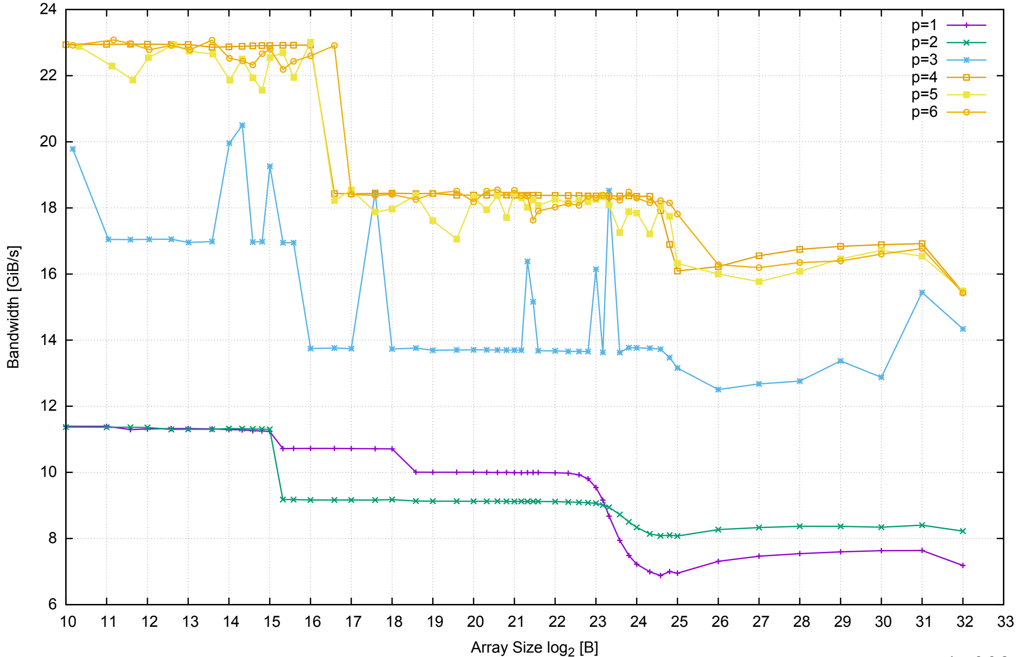
AWS c3.xlarge - Intel Xeon E5-2680 v2 2.80 GHz 7.5GB - Parallel Memory Bandwidth - ScanWrite32PtrUnrollLoop
