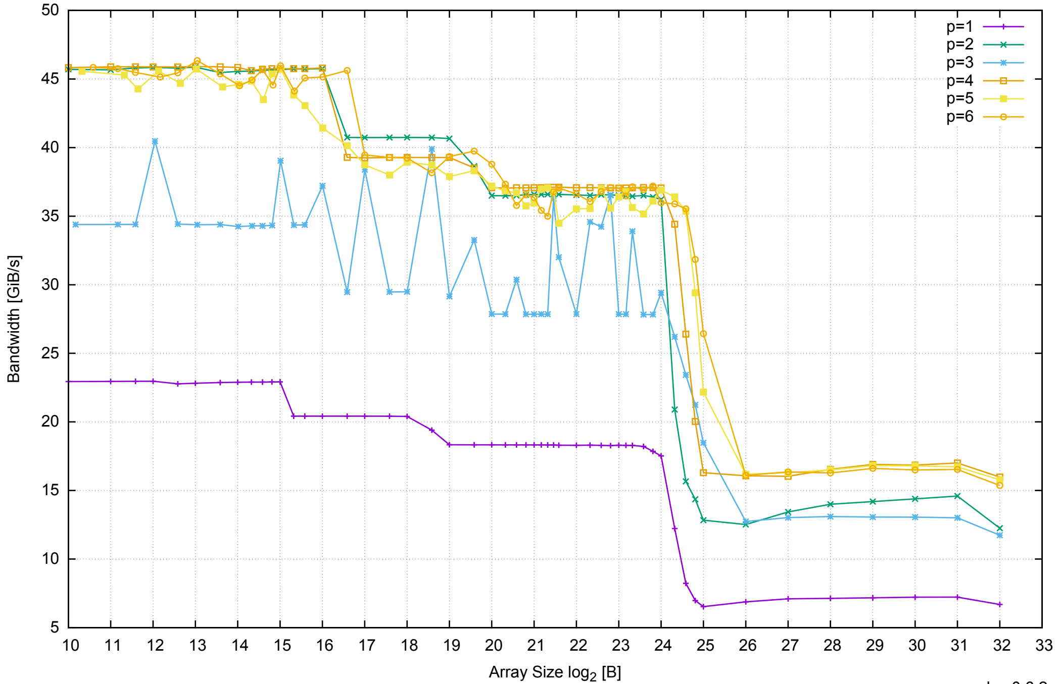
AWS c3.xlarge - Intel Xeon E5-2680 v2 2.80 GHz 7.5GB - Parallel Memory Bandwidth - ScanWrite64PtrUnrollLoop
