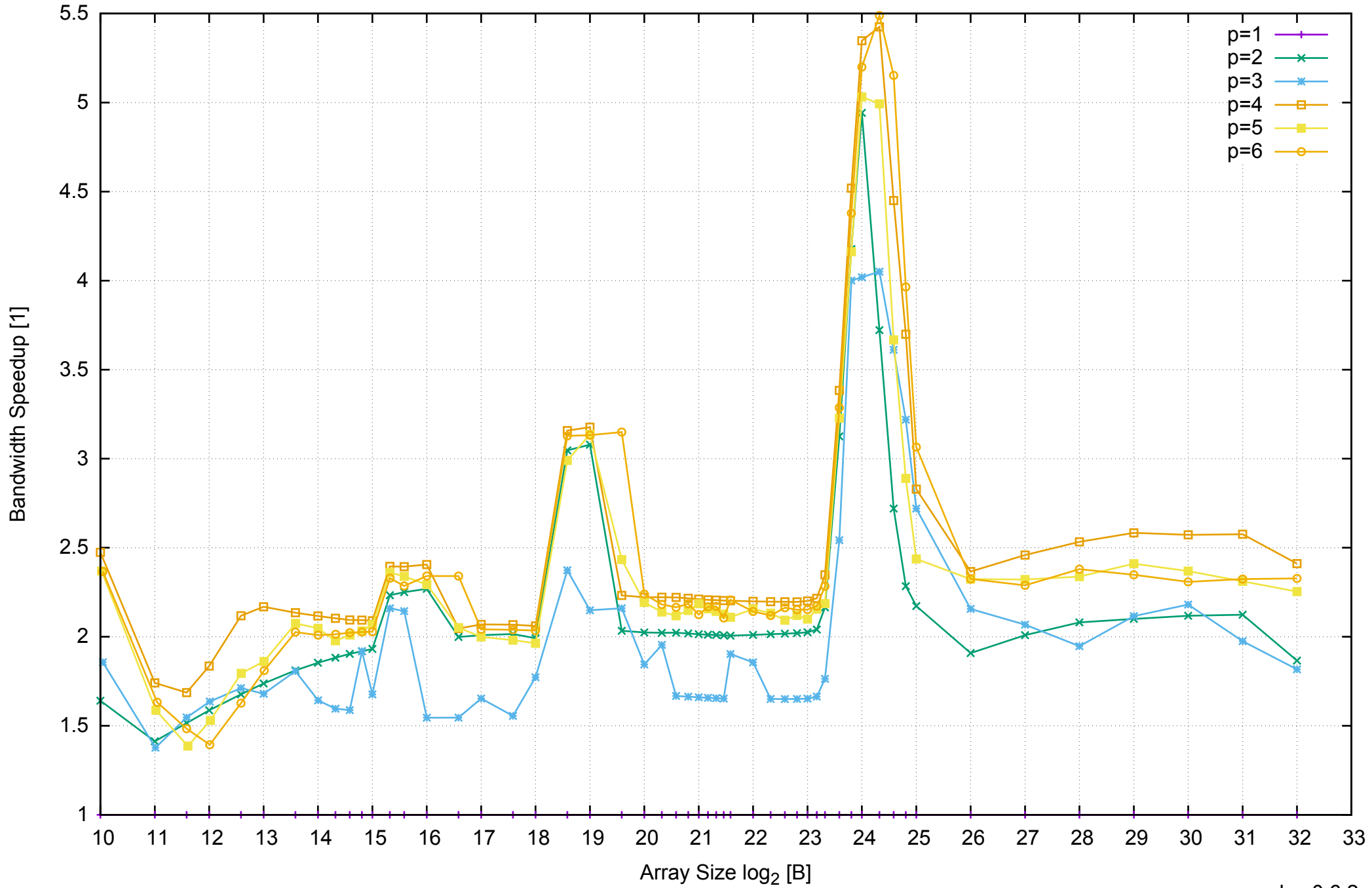
AWS c3.xlarge - Intel Xeon E5-2680 v2 2.80 GHz 7.5GB - Speedup of Parallel Memory Bandwidth - ScanRead128PtrSimpleLoop
