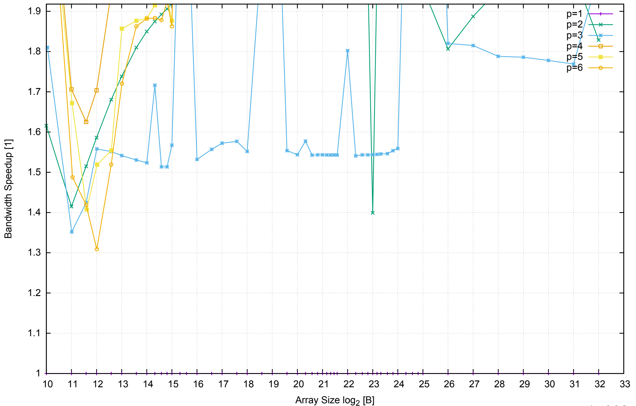
AWS c3.xlarge - Intel Xeon E5-2680 v2 2.80 GHz 7.5GB - Speedup of Parallel Memory Bandwidth (enlarged) - ScanWrite128PtrSimpleLoop
