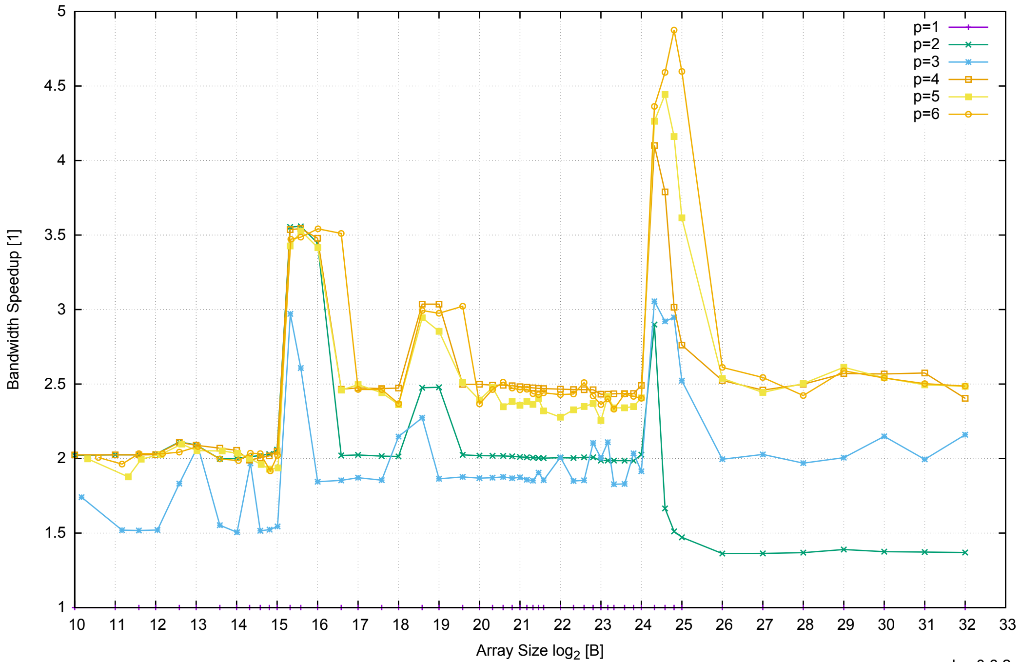
AWS c3.xlarge - Intel Xeon E5-2680 v2 2.80 GHz 7.5GB - Speedup of Parallel Memory Bandwidth - ScanRead64PtrUnrollLoop
