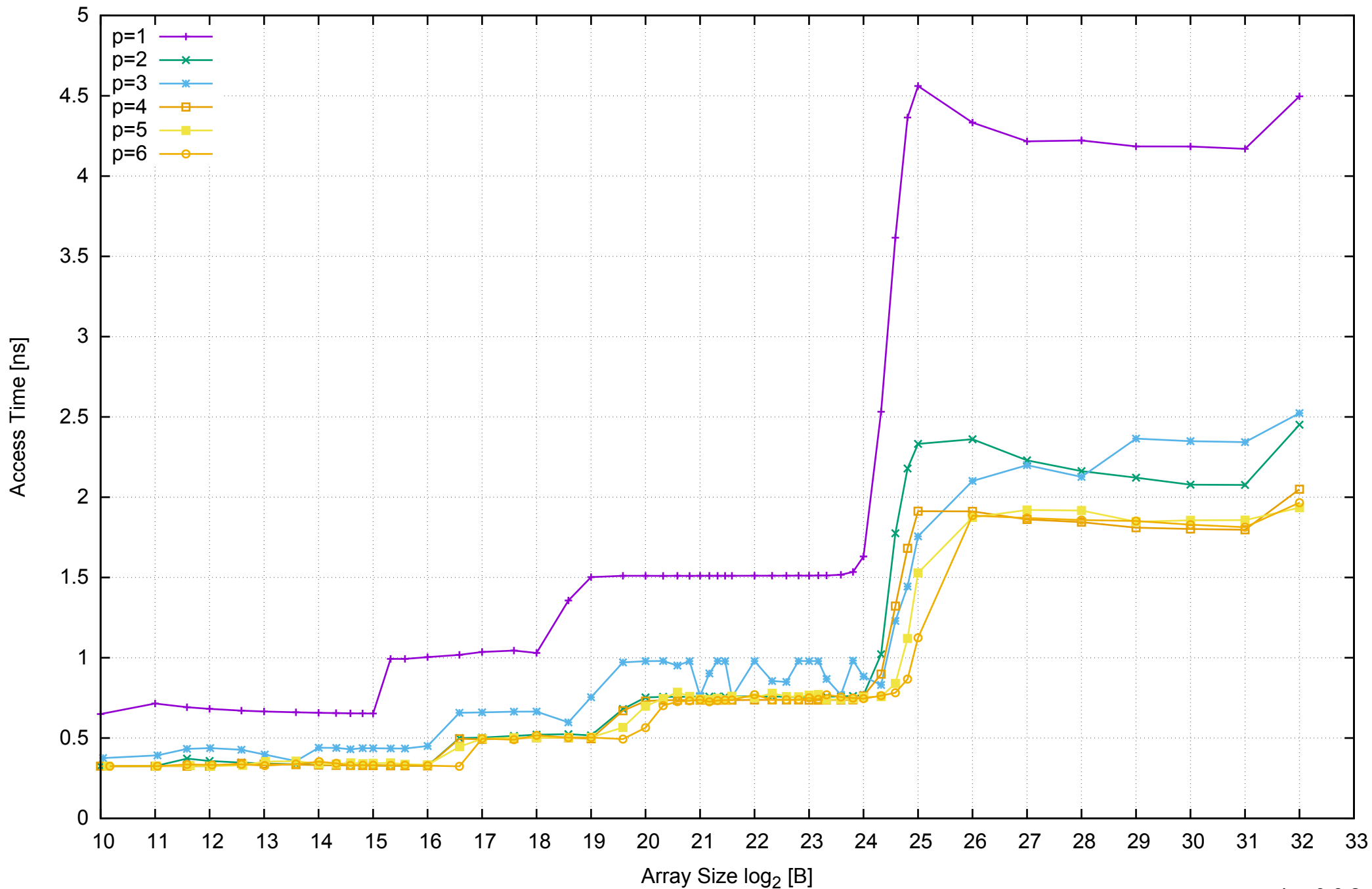
AWS c3.xlarge - Intel Xeon E5-2680 v2 2.80 GHz 7.5GB - Parallel Memory Access Time - ScanWrite256PtrSimpleLoop
