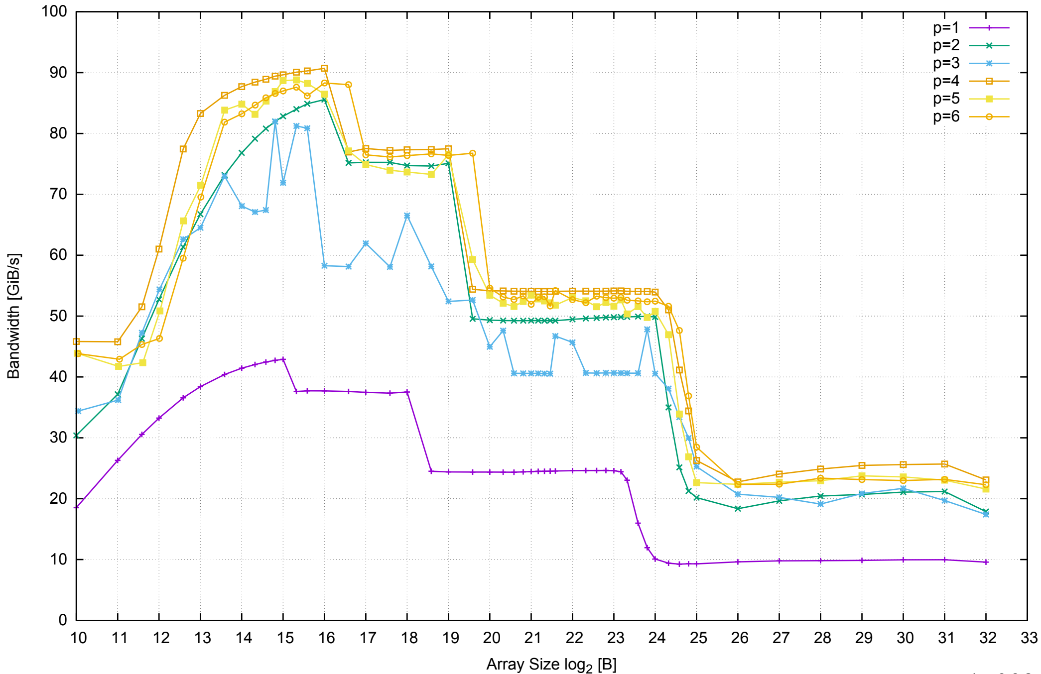
AWS c3.xlarge - Intel Xeon E5-2680 v2 2.80 GHz 7.5GB - Parallel Memory Bandwidth - ScanRead128PtrSimpleLoop
