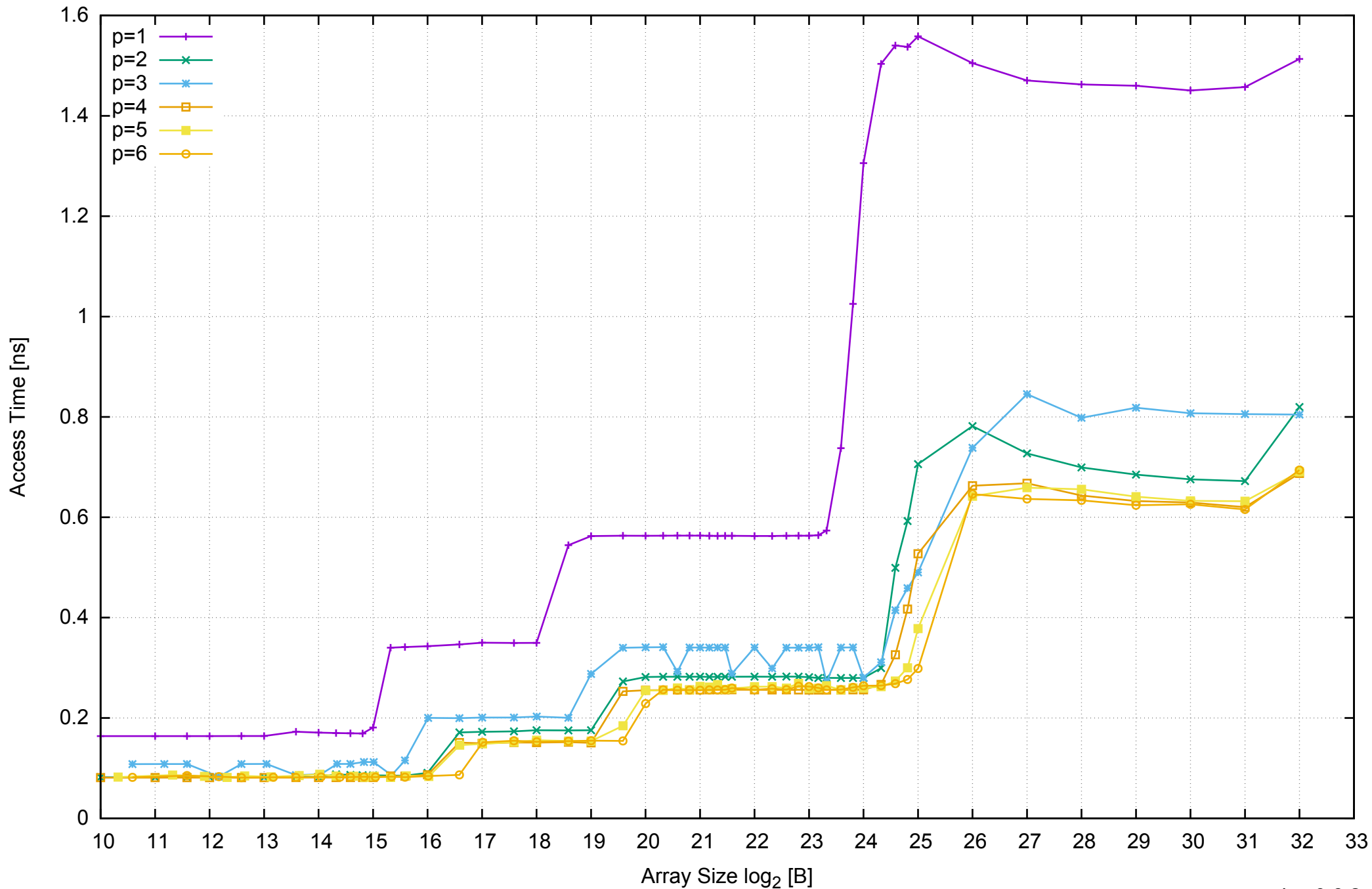
AWS c3.xlarge - Intel Xeon E5-2680 v2 2.80 GHz 7.5GB - Parallel Memory Access Time - ScanRead128PtrUnrollLoop
