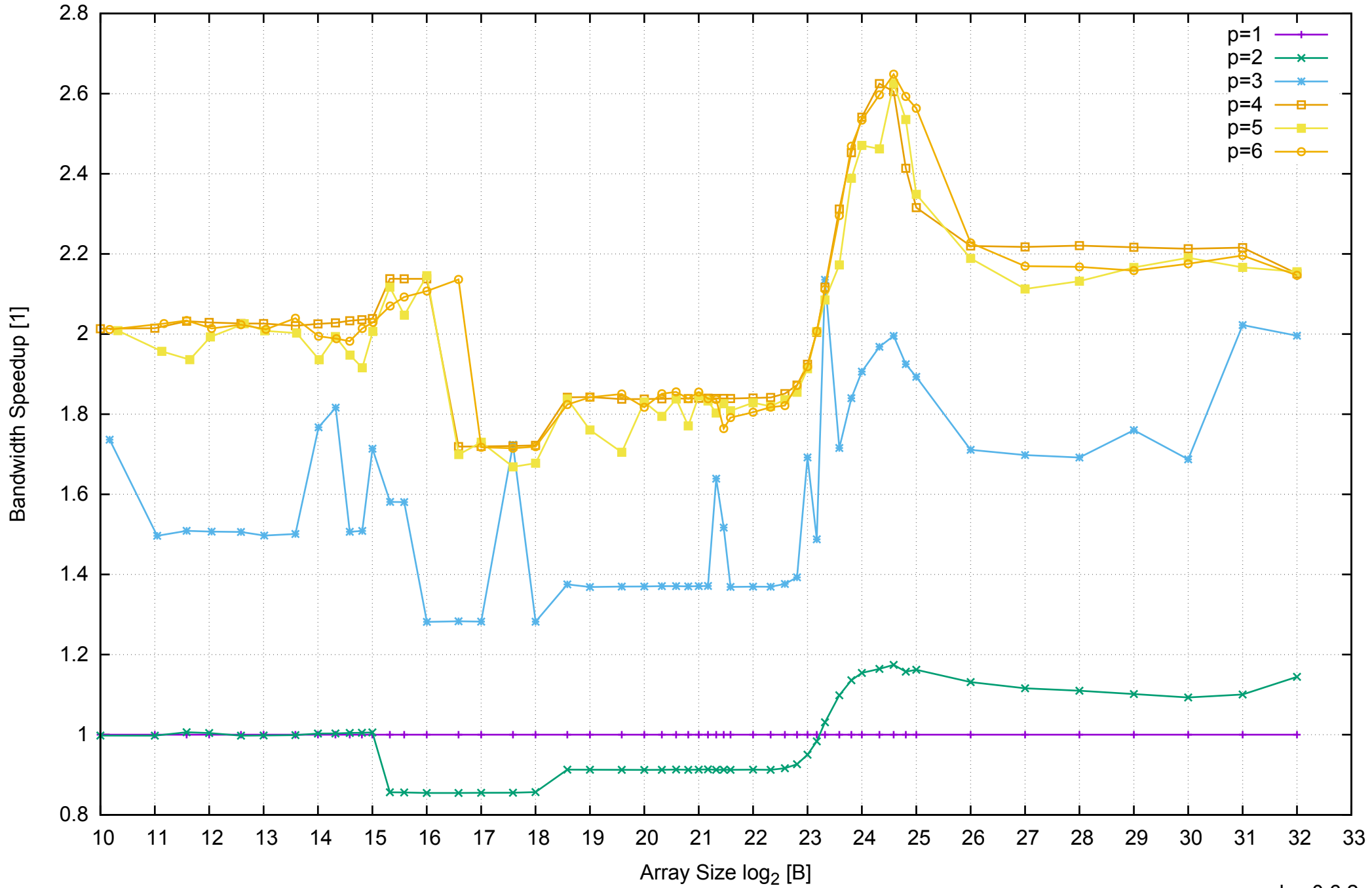
AWS c3.xlarge - Intel Xeon E5-2680 v2 2.80 GHz 7.5GB - Speedup of Parallel Memory Bandwidth - ScanWrite32PtrUnrollLoop
