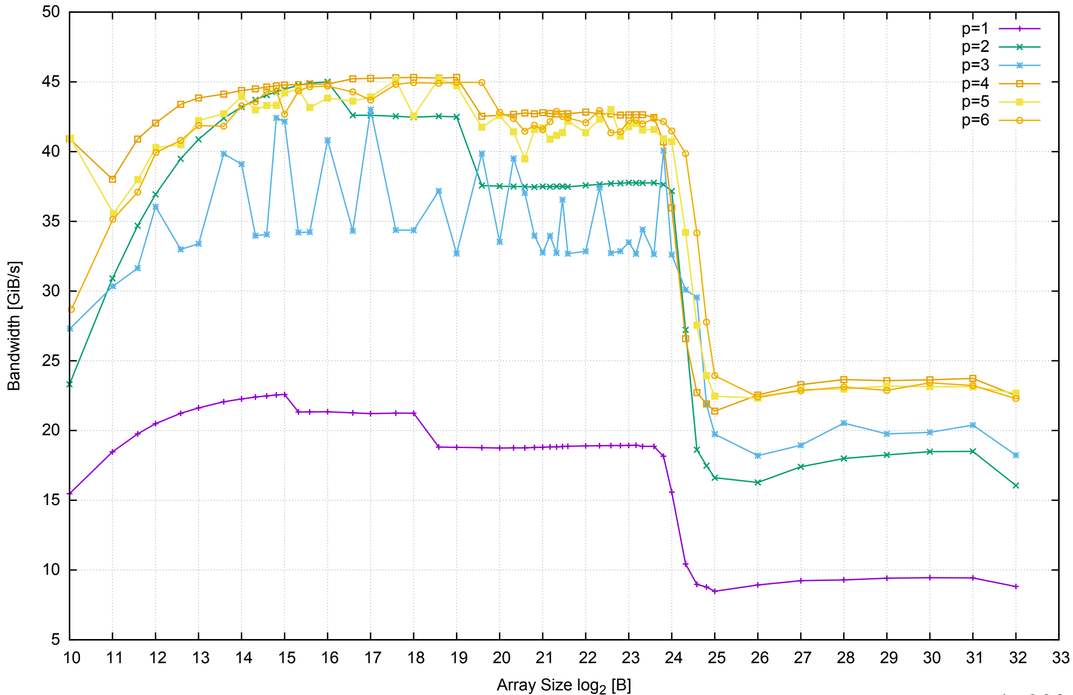
AWS c3.xlarge - Intel Xeon E5-2680 v2 2.80 GHz 7.5GB - Parallel Memory Bandwidth - ScanRead64PtrSimpleLoop
