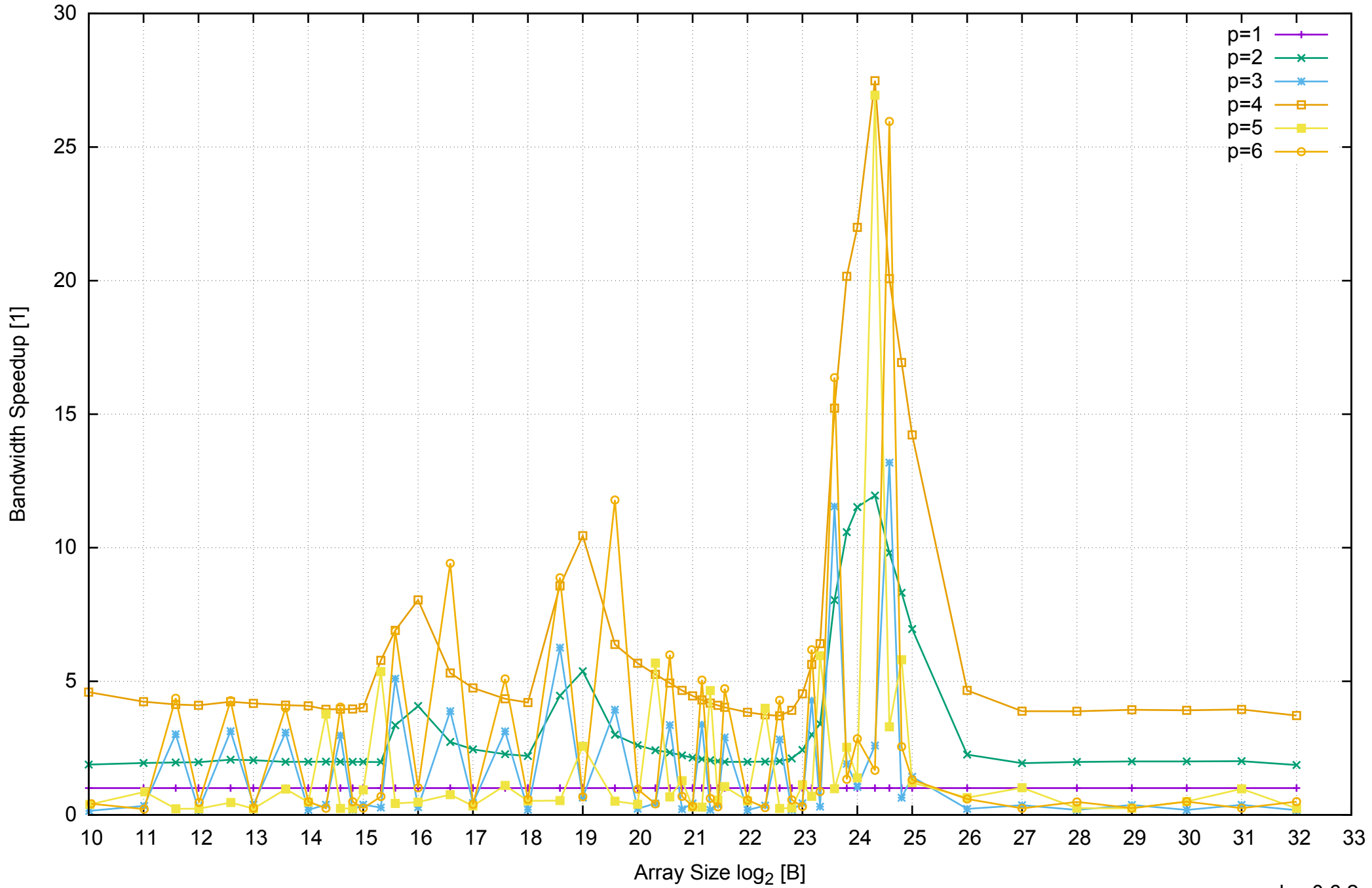
AWS c3.xlarge - Intel Xeon E5-2680 v2 2.80 GHz 7.5GB - Speedup of Parallel Memory Bandwidth - PermRead64UnrollLoop
