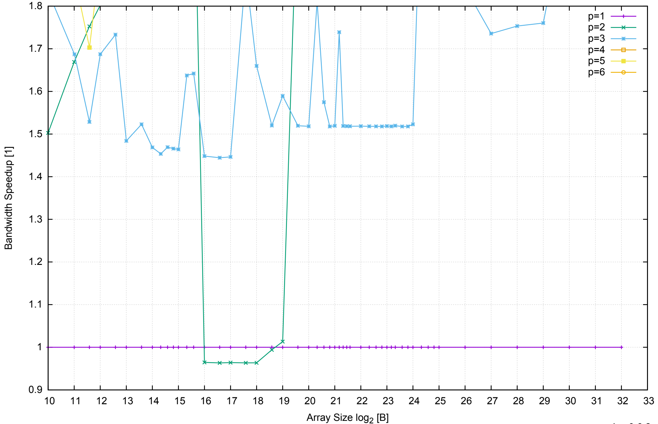
AWS c3.xlarge - Intel Xeon E5-2680 v2 2.80 GHz 7.5GB - Speedup of Parallel Memory Bandwidth (enlarged) - ScanWrite64PtrSimpleLoop
