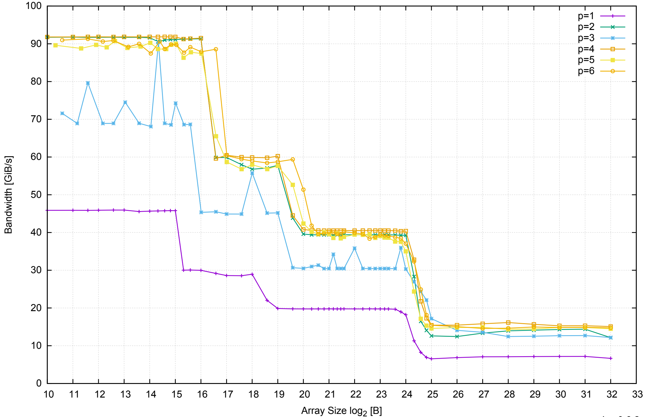
AWS c3.xlarge - Intel Xeon E5-2680 v2 2.80 GHz 7.5GB - Parallel Memory Bandwidth - ScanWrite128PtrUnrollLoop
