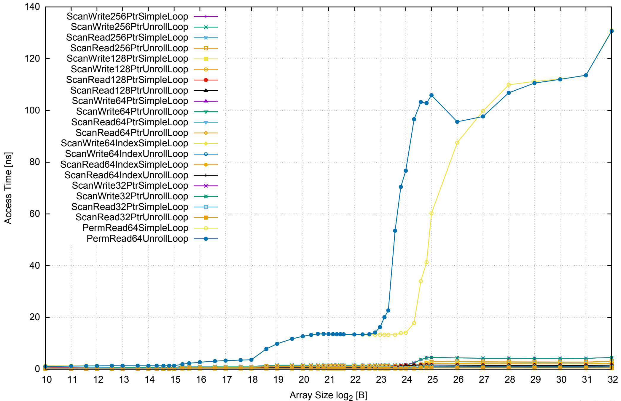
AWS c3.xlarge - Intel Xeon E5-2680 v2 2.80 GHz 7.5GB - One Thread Memory Latency (Access Time)
