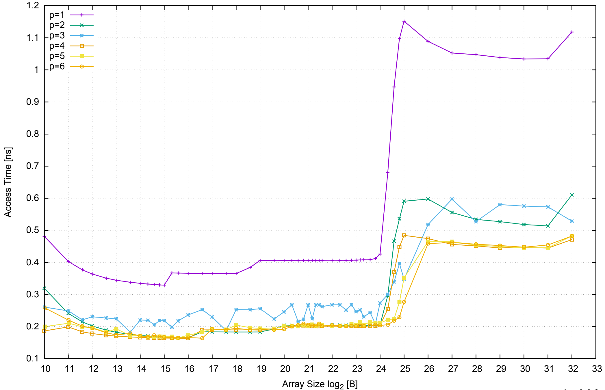
AWS c3.xlarge - Intel Xeon E5-2680 v2 2.80 GHz 7.5GB - Parallel Memory Access Time - ScanWrite64IndexSimpleLoop
