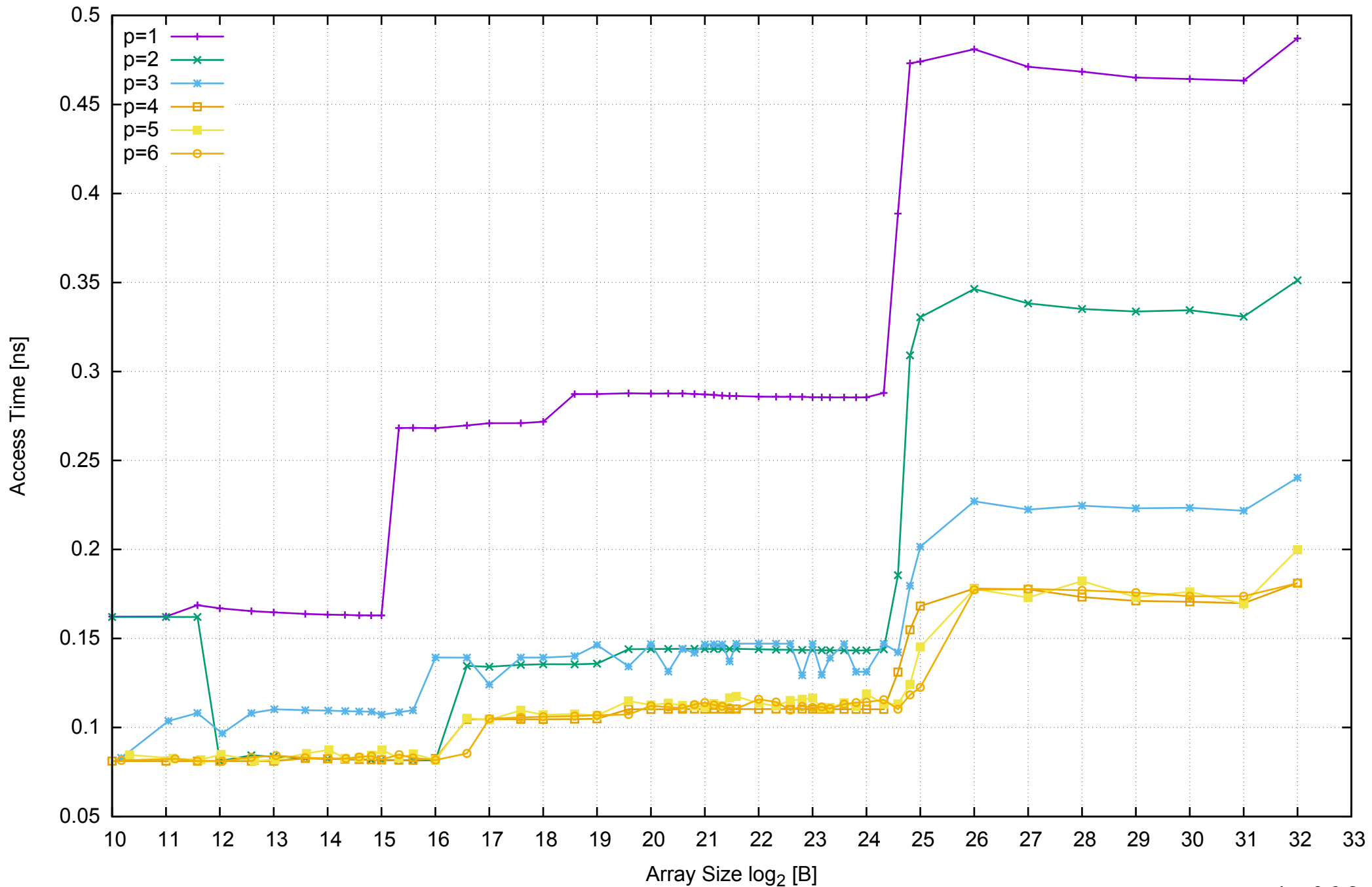
AWS c3.xlarge - Intel Xeon E5-2680 v2 2.80 GHz 7.5GB - Parallel Memory Access Time - ScanRead32PtrUnrollLoop
