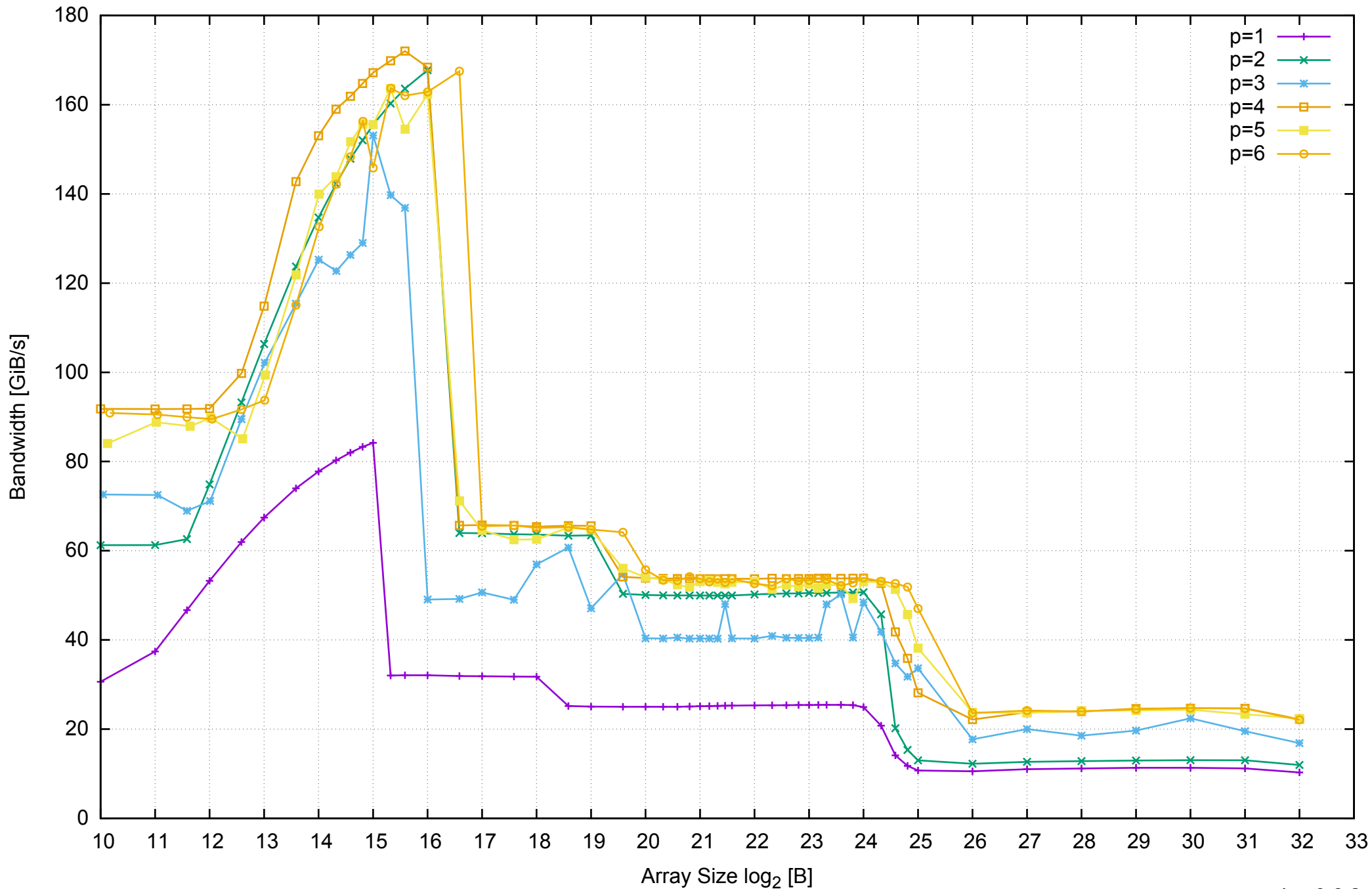
AWS c3.xlarge - Intel Xeon E5-2680 v2 2.80 GHz 7.5GB - Parallel Memory Bandwidth - ScanRead256PtrSimpleLoop
