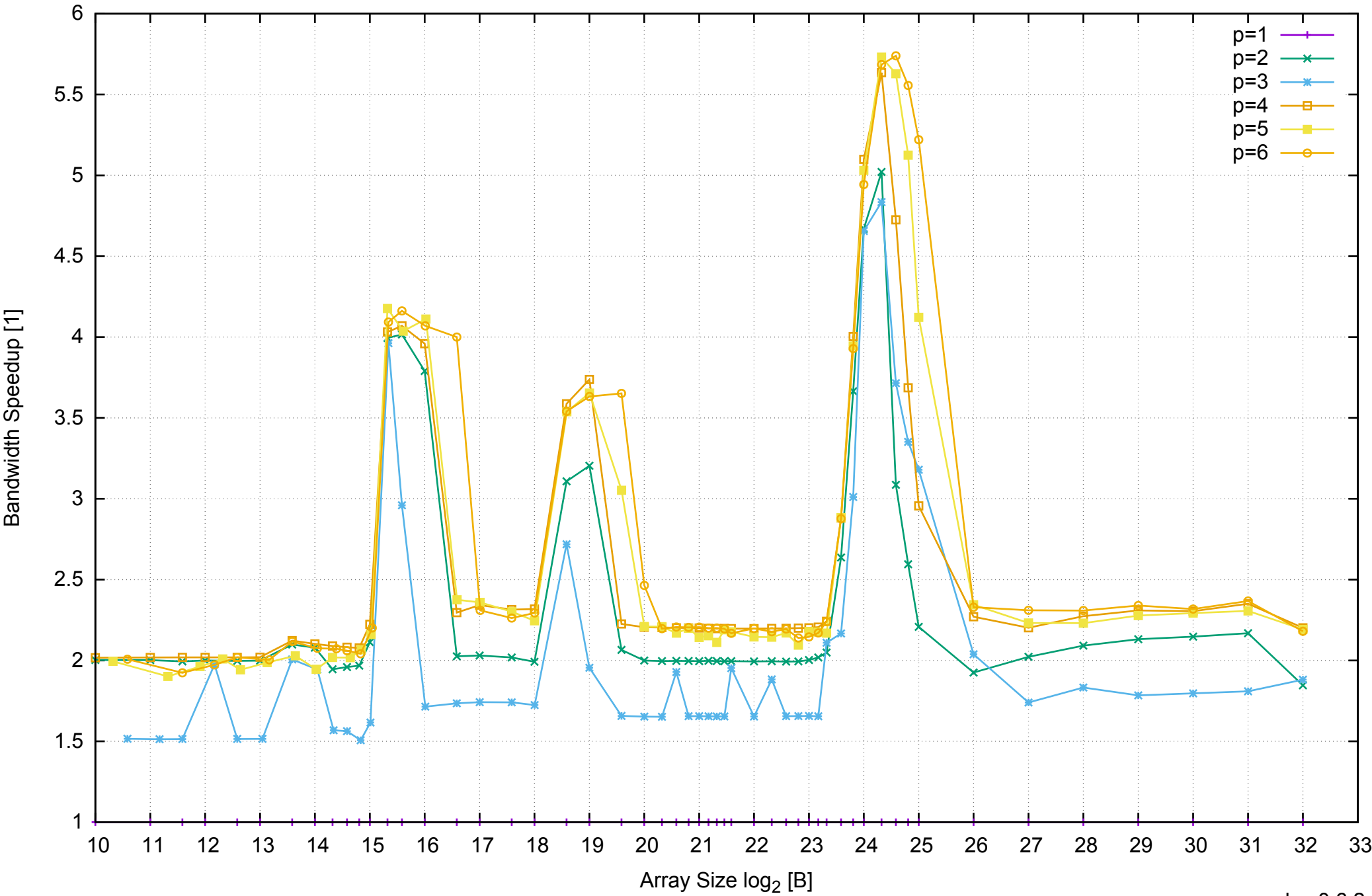
AWS c3.xlarge - Intel Xeon E5-2680 v2 2.80 GHz 7.5GB - Speedup of Parallel Memory Bandwidth - ScanRead128PtrUnrollLoop
