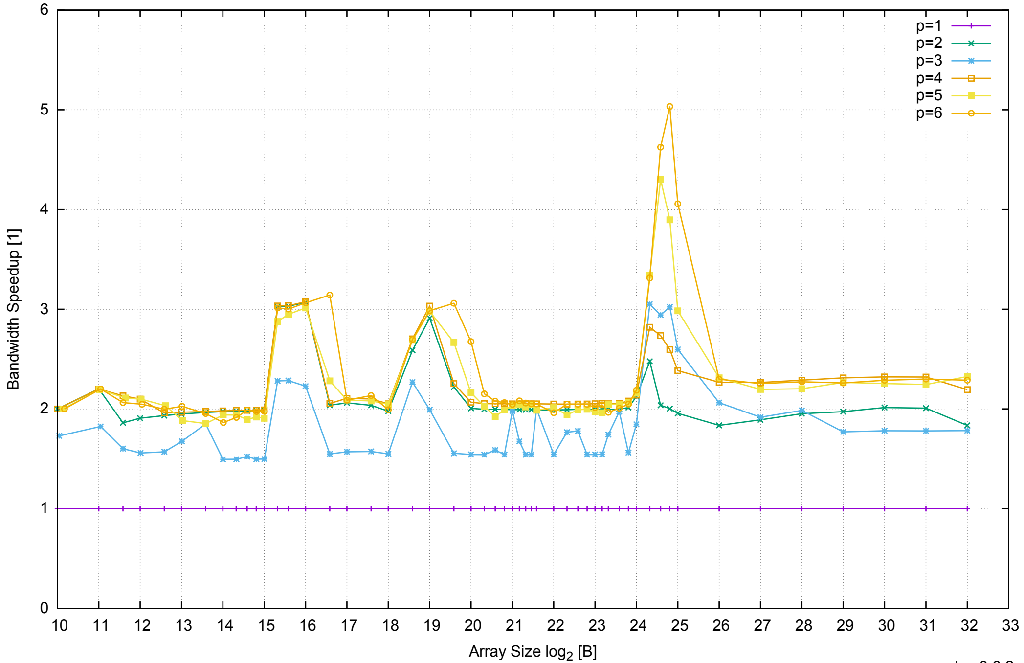
AWS c3.xlarge - Intel Xeon E5-2680 v2 2.80 GHz 7.5GB - Speedup of Parallel Memory Bandwidth - ScanWrite256PtrSimpleLoop
