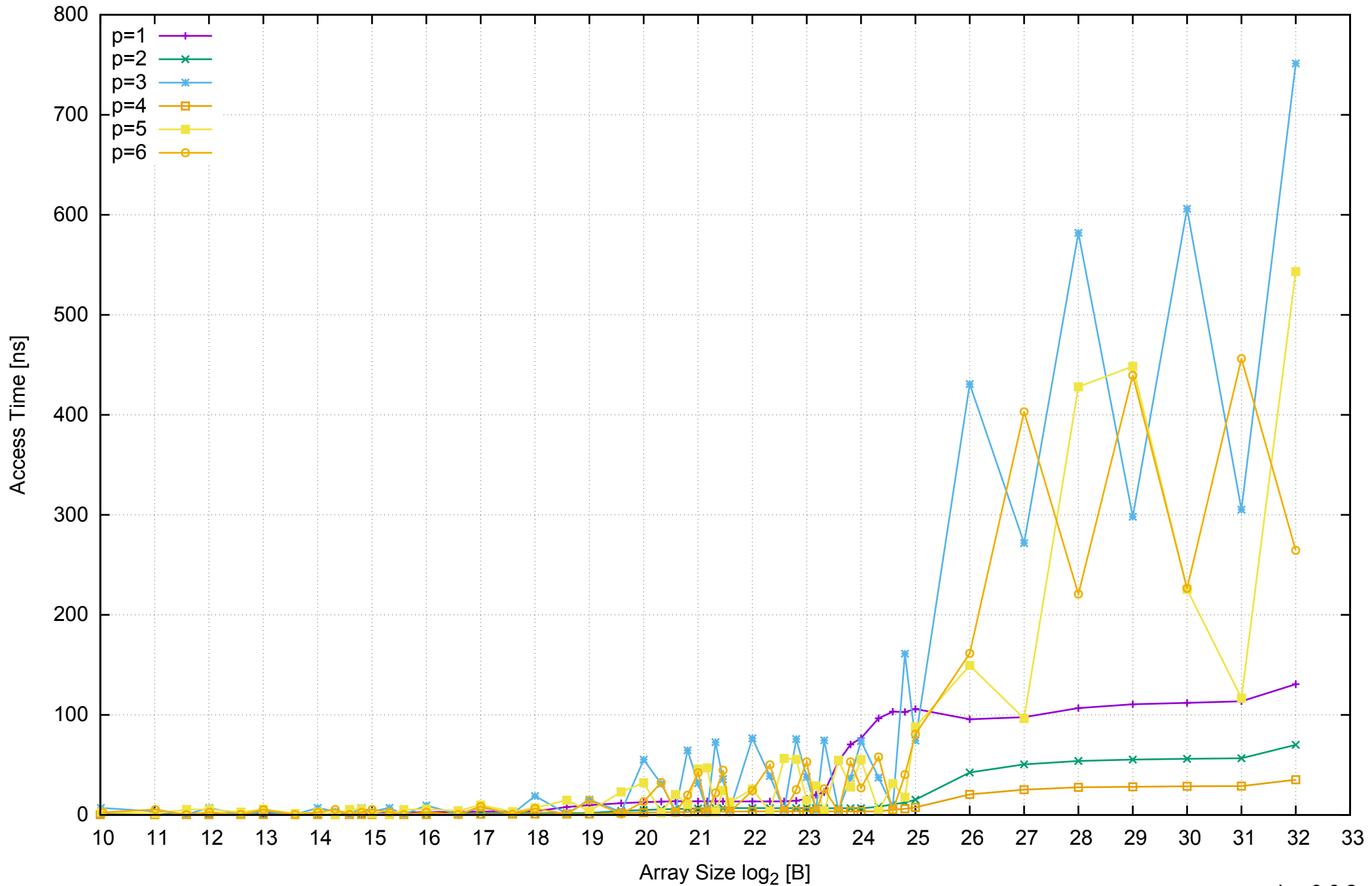
AWS c3.xlarge - Intel Xeon E5-2680 v2 2.80 GHz 7.5GB - Parallel Memory Access Time - PermRead64UnrollLoop
