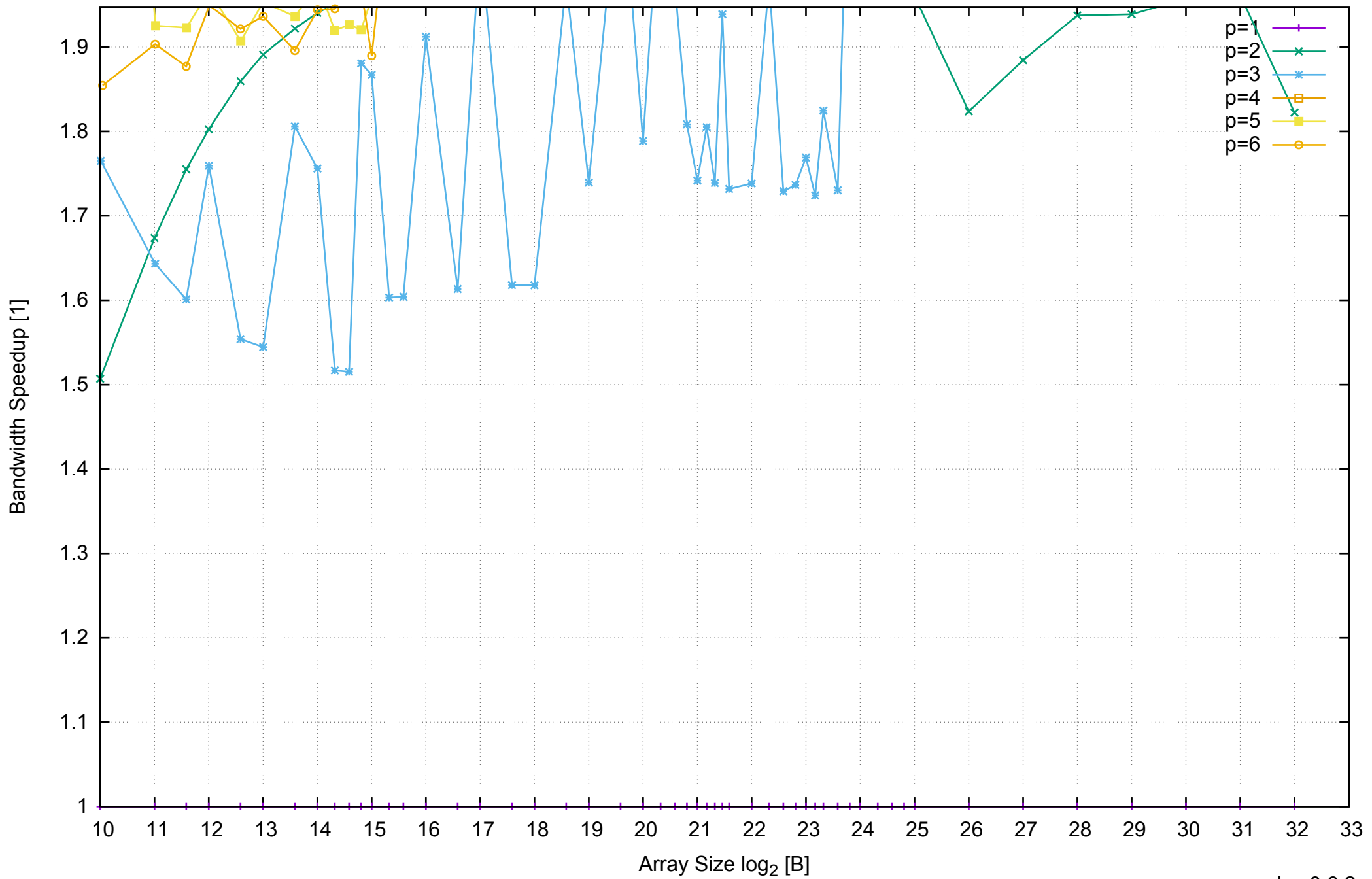
AWS c3.xlarge - Intel Xeon E5-2680 v2 2.80 GHz 7.5GB - Speedup of Parallel Memory Bandwidth (enlarged) - ScanRead64PtrSimpleLoop
