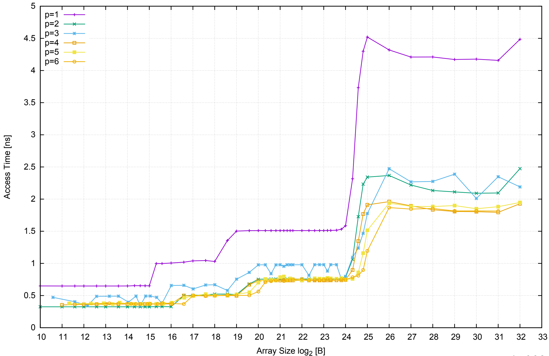
AWS c3.xlarge - Intel Xeon E5-2680 v2 2.80 GHz 7.5GB - Parallel Memory Access Time - ScanWrite256PtrUnrollLoop
