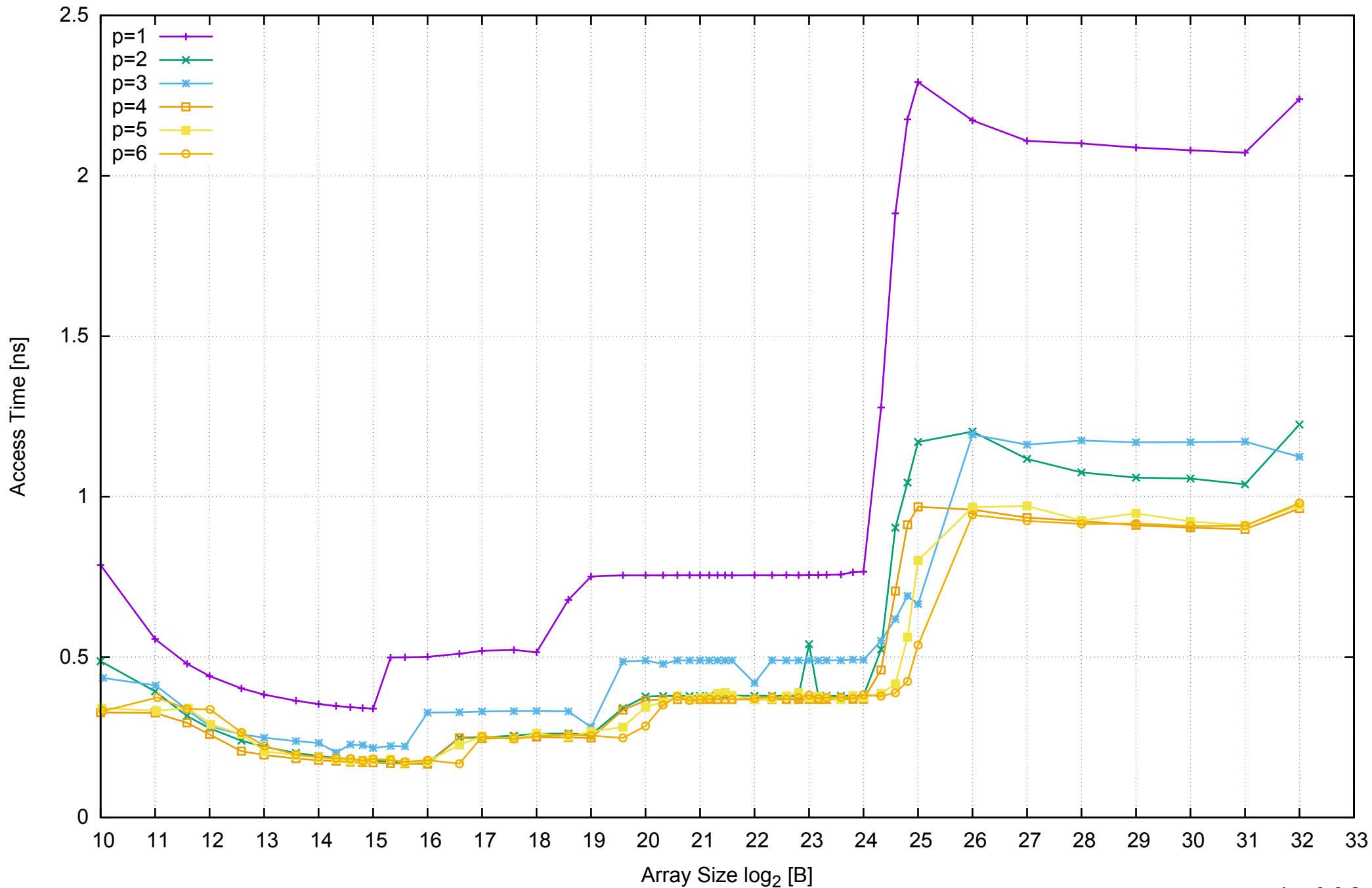
AWS c3.xlarge - Intel Xeon E5-2680 v2 2.80 GHz 7.5GB - Parallel Memory Access Time - ScanWrite128PtrSimpleLoop
