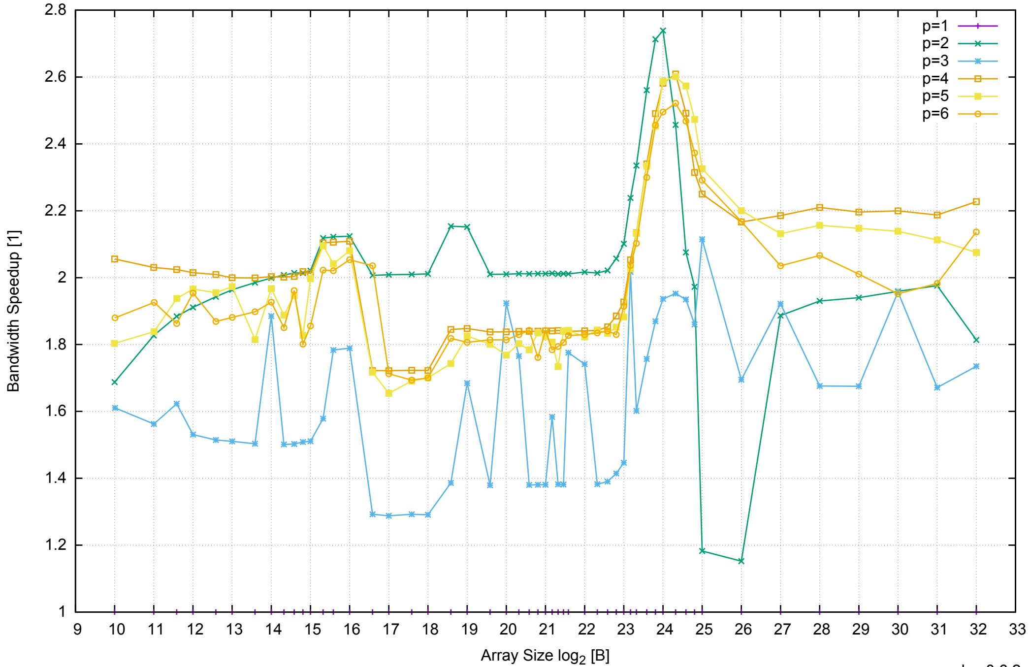
AWS c3.xlarge - Intel Xeon E5-2680 v2 2.80 GHz 7.5GB - Speedup of Parallel Memory Bandwidth - ScanWrite32PtrSimpleLoop
