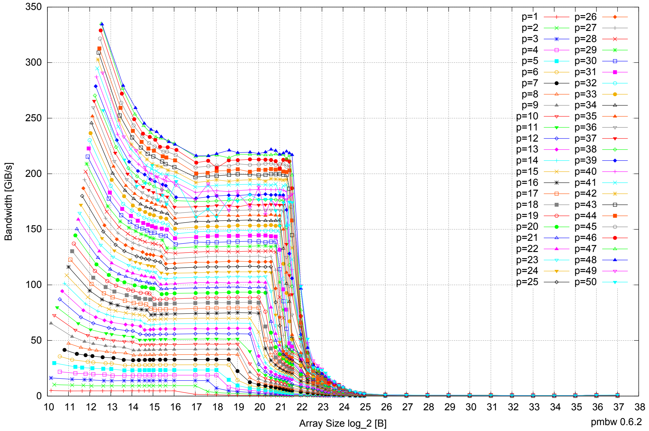
AMD Opteron 6168 256GB - Parallel Memory Bandwidth - PermRead64UnrollLoop
