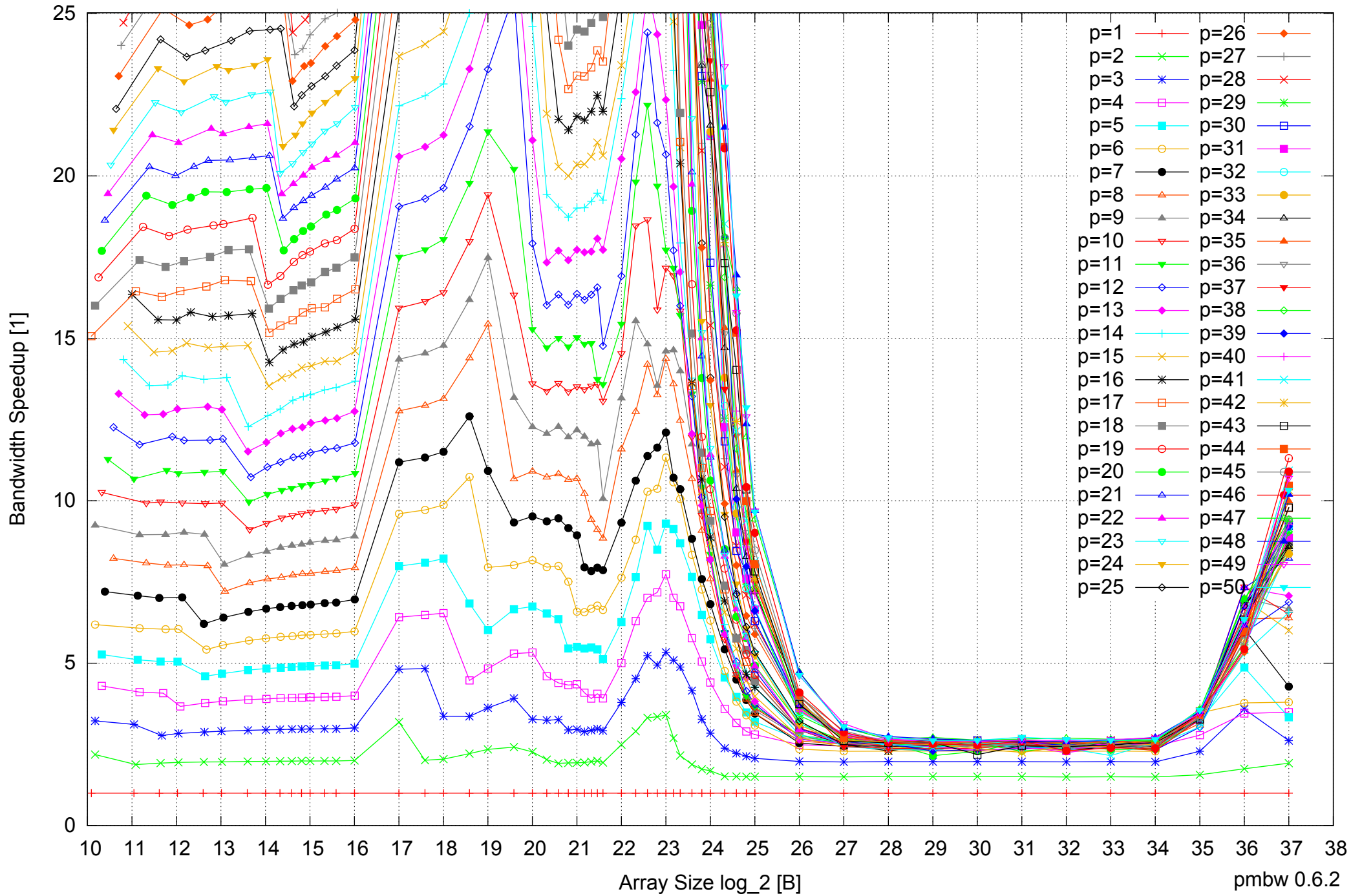
AMD Opteron 6168 256GB - Speedup of Parallel Memory Bandwidth (enlarged) - ScanRead32PtrUnrollLoop
