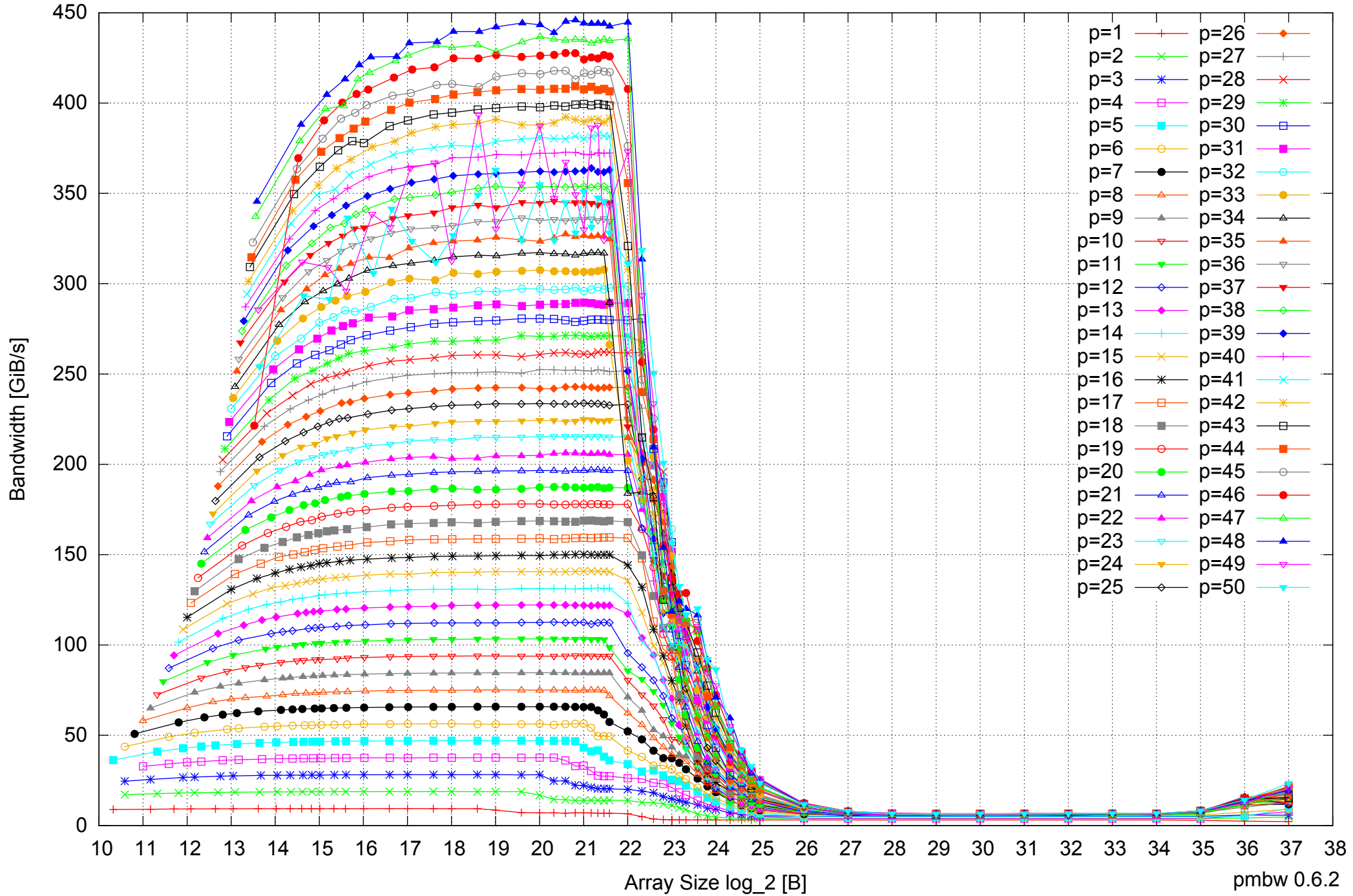
AMD Opteron 6168 256GB - Parallel Memory Bandwidth - ScanRead128PtrSimpleLoop
