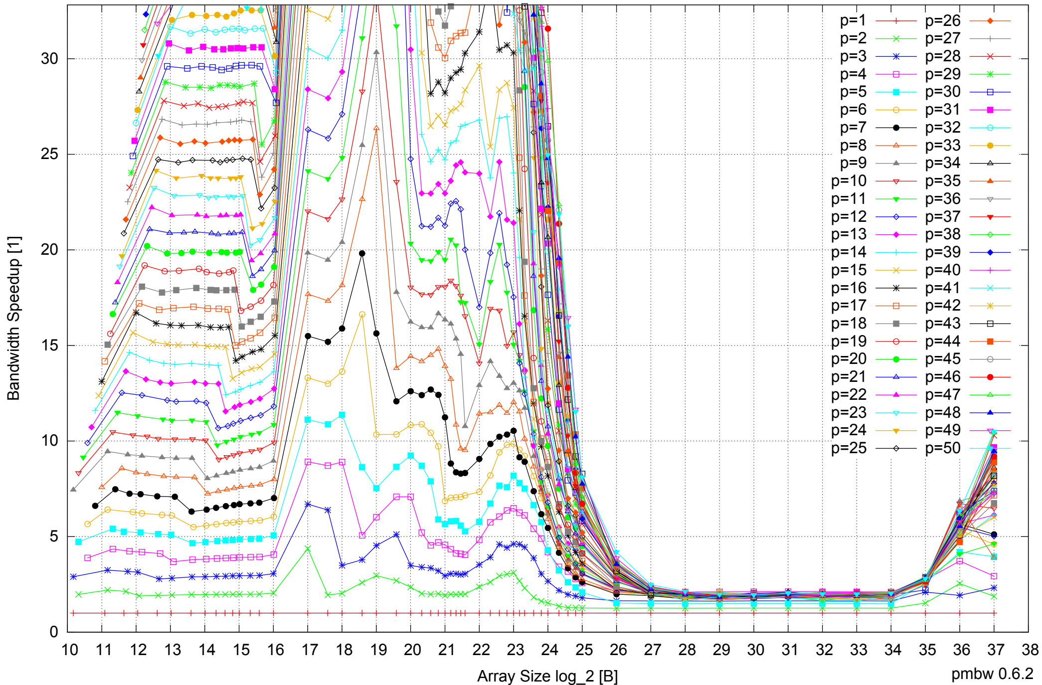
AMD Opteron 6168 256GB - Speedup of Parallel Memory Bandwidth (enlarged) - ScanRead64PtrUnrollLoop
