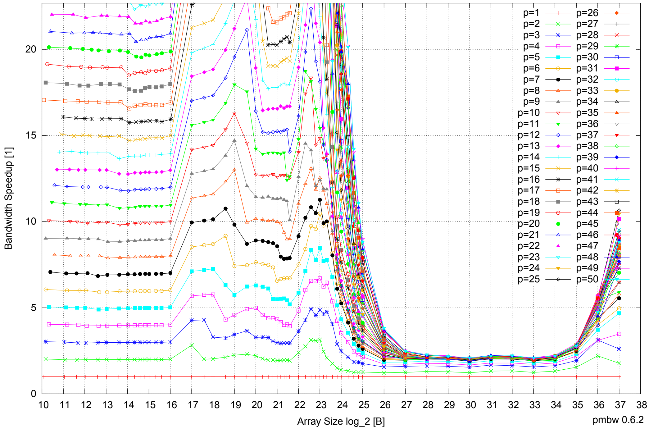
AMD Opteron 6168 256GB - Speedup of Parallel Memory Bandwidth (enlarged) - ScanWrite32PtrUnrollLoop
