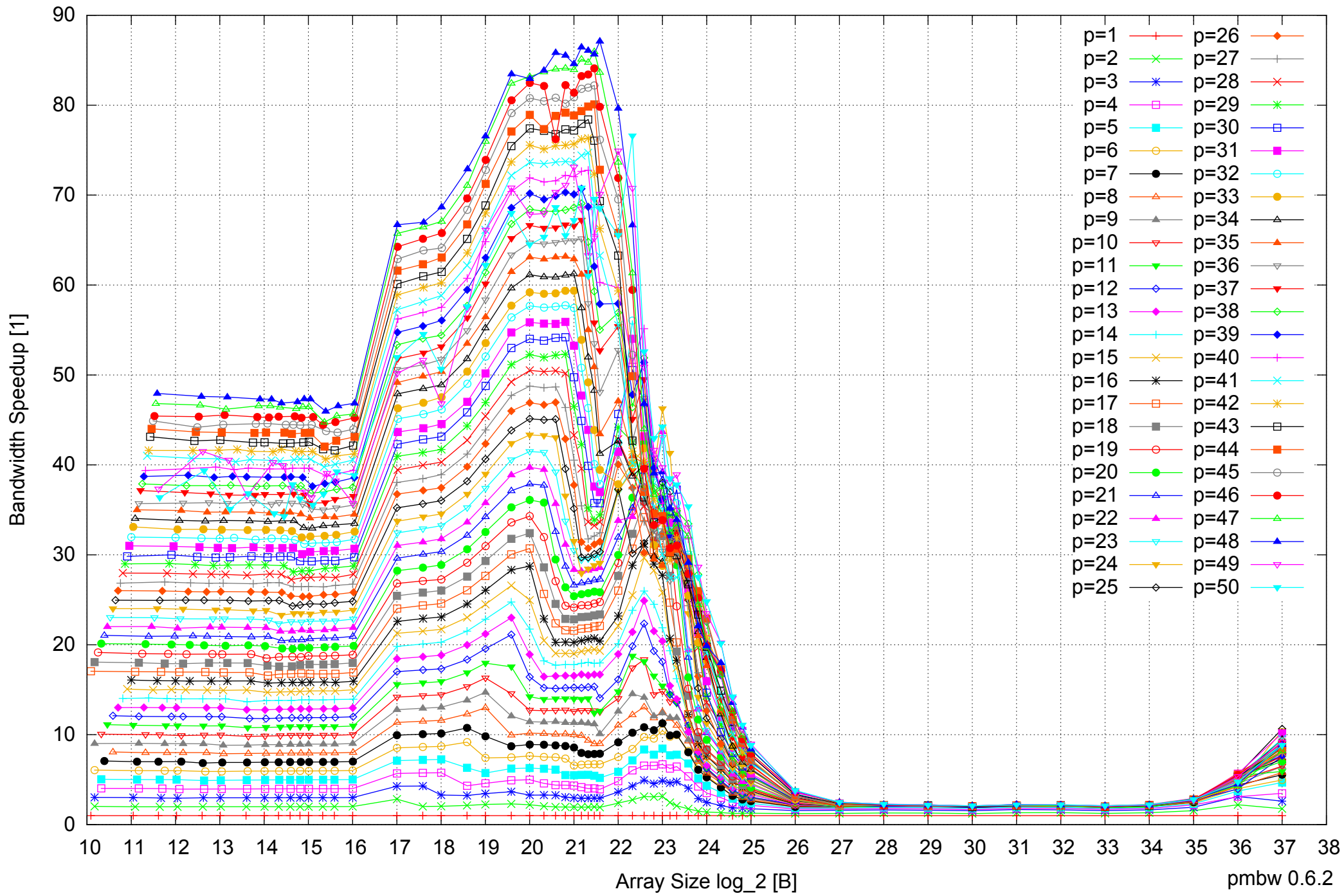
AMD Opteron 6168 256GB - Speedup of Parallel Memory Bandwidth - ScanWrite32PtrUnrollLoop
