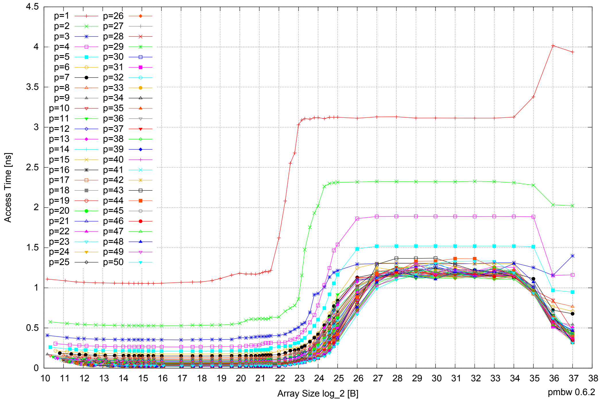
AMD Opteron 6168 256GB - Parallel Memory Access Time - ScanRead64PtrSimpleLoop
