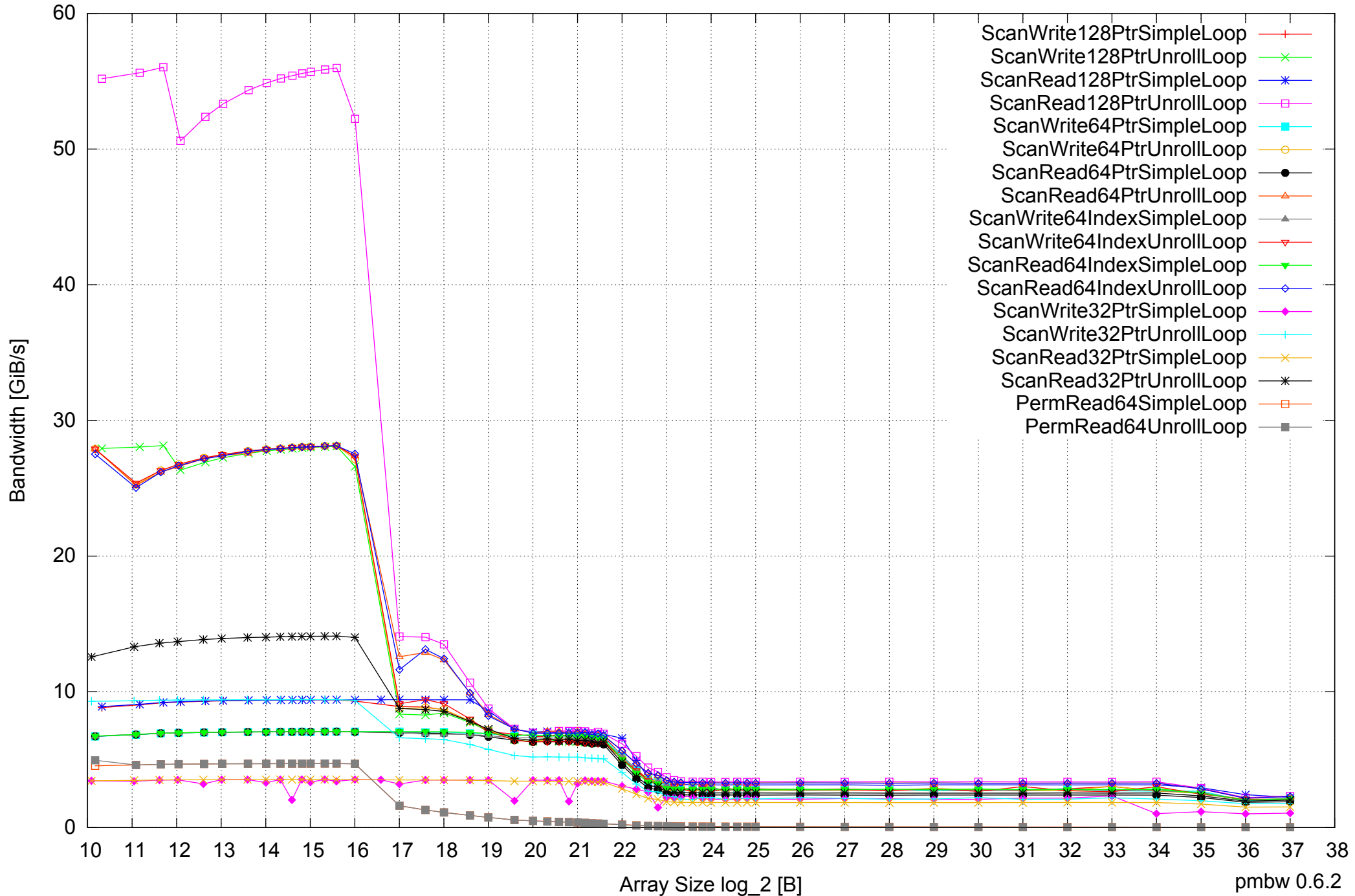
AMD Opteron 6168 256GB - One Thread Memory Bandwidth
