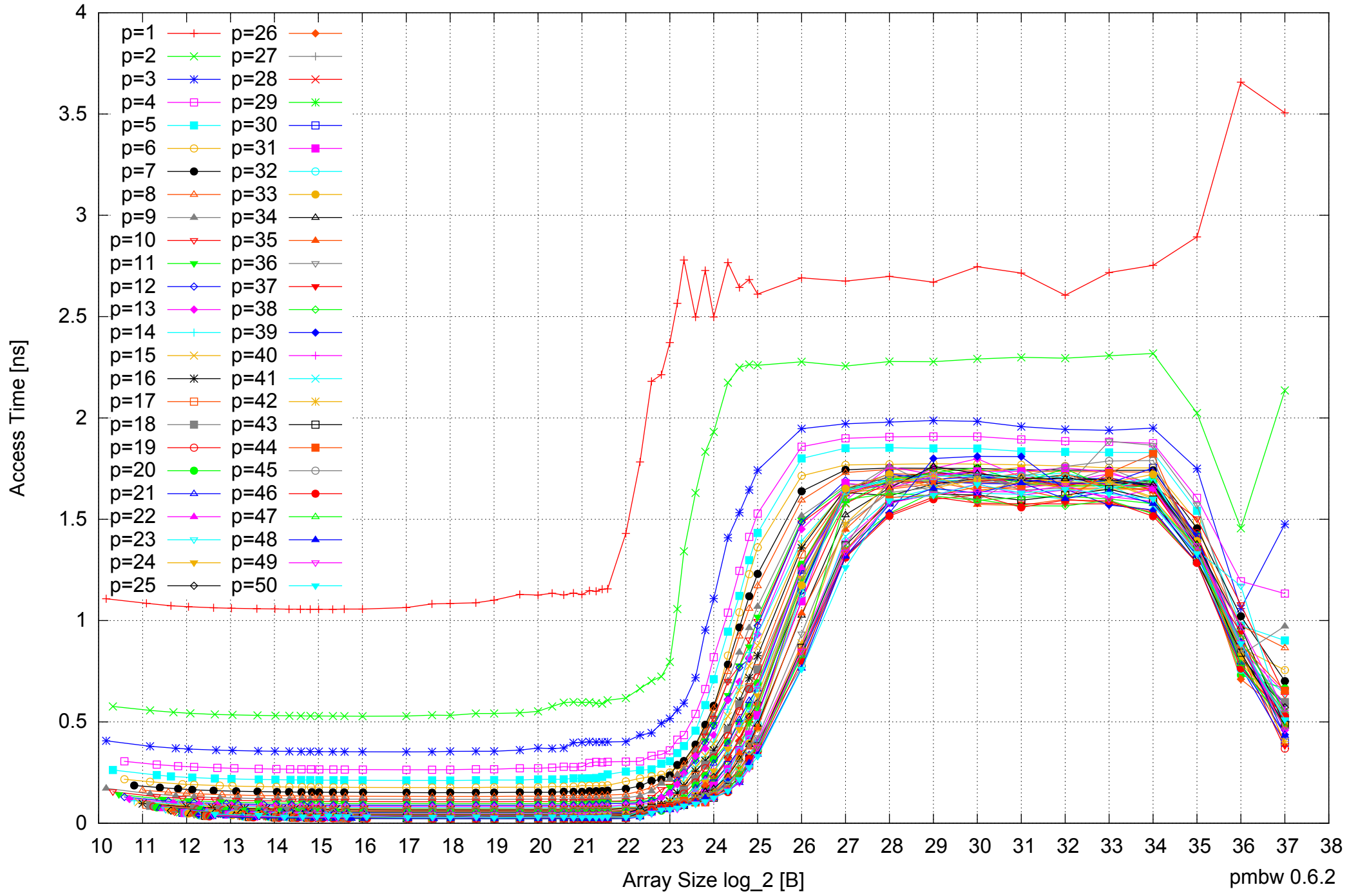
AMD Opteron 6168 256GB - Parallel Memory Access Time - ScanWrite64IndexSimpleLoop
