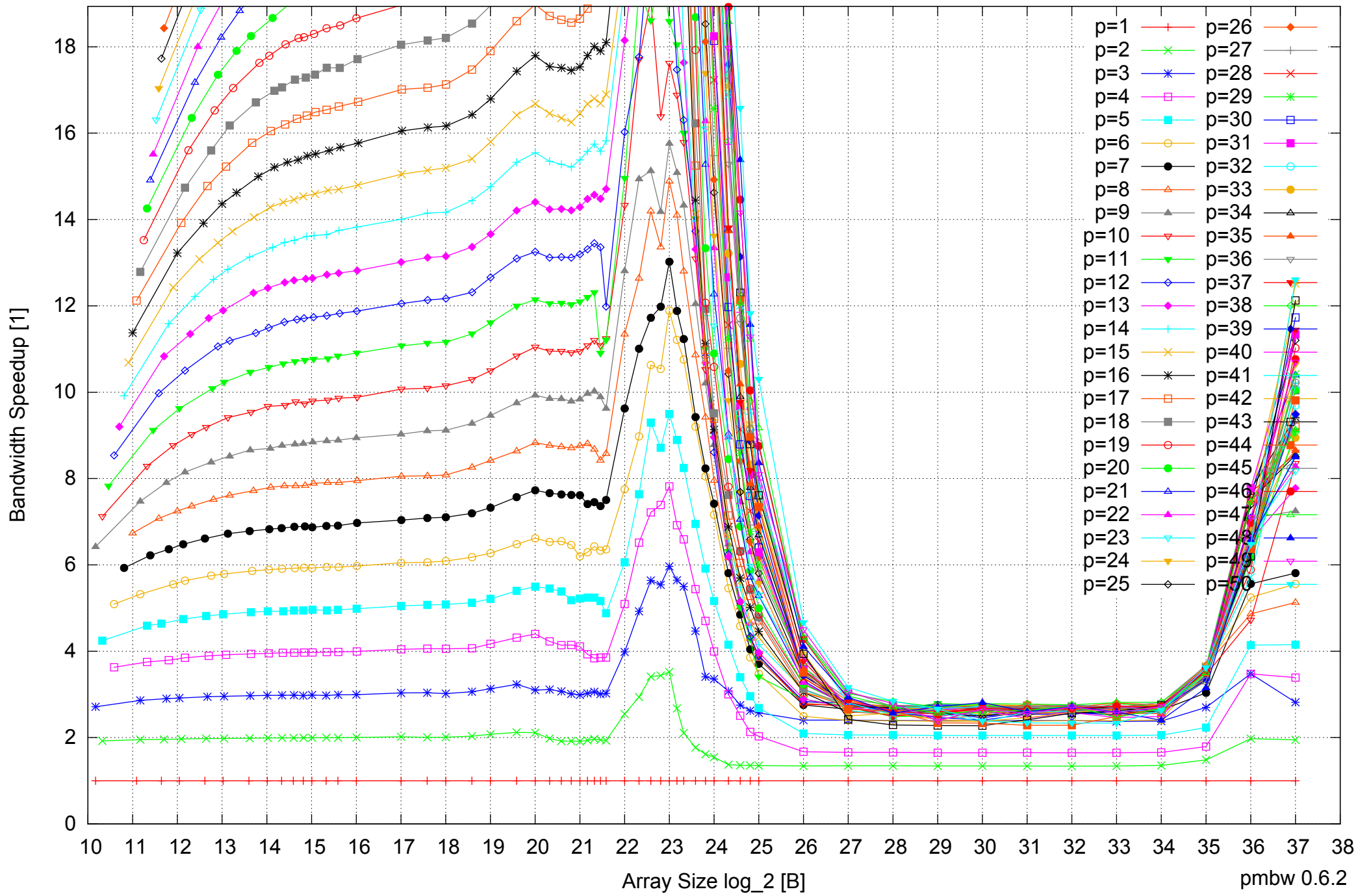
AMD Opteron 6168 256GB - Speedup of Parallel Memory Bandwidth (enlarged) - ScanRead64PtrSimpleLoop
