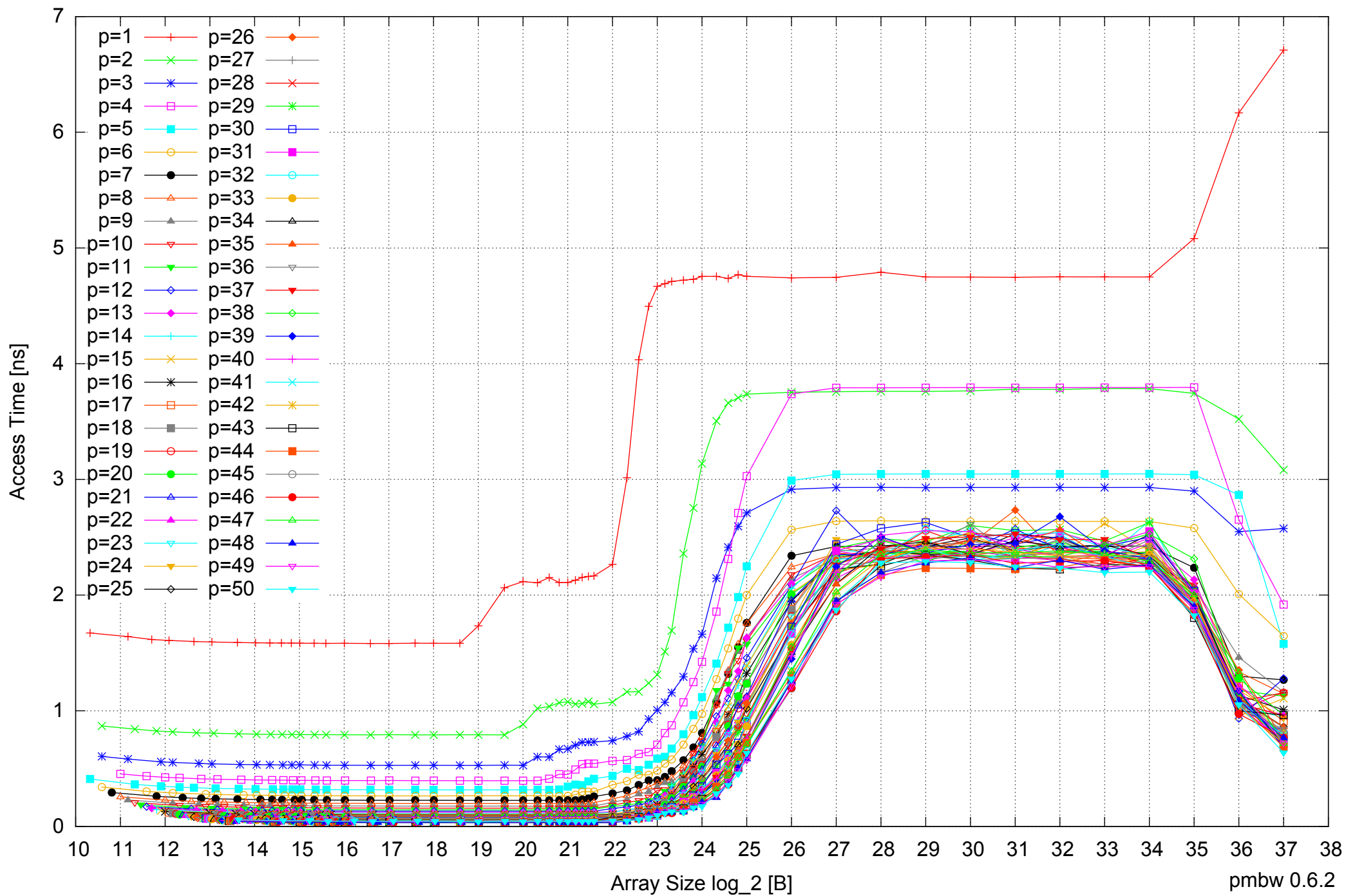
AMD Opteron 6168 256GB - Parallel Memory Access Time - ScanRead128PtrSimpleLoop
