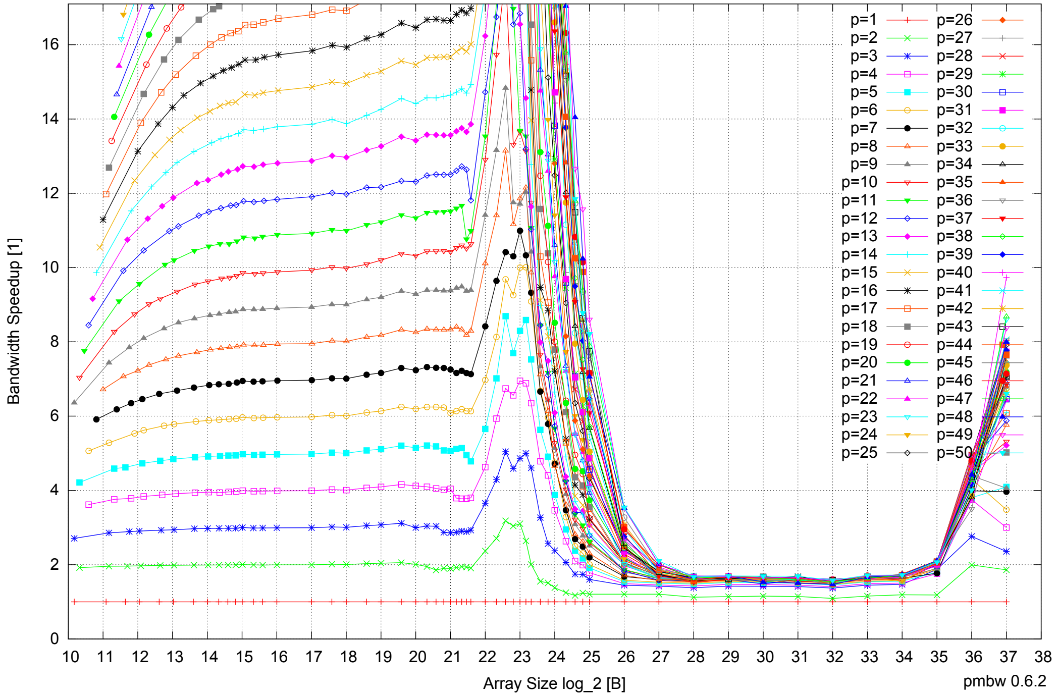
AMD Opteron 6168 256GB - Speedup of Parallel Memory Bandwidth (enlarged) - ScanWrite64PtrSimpleLoop
