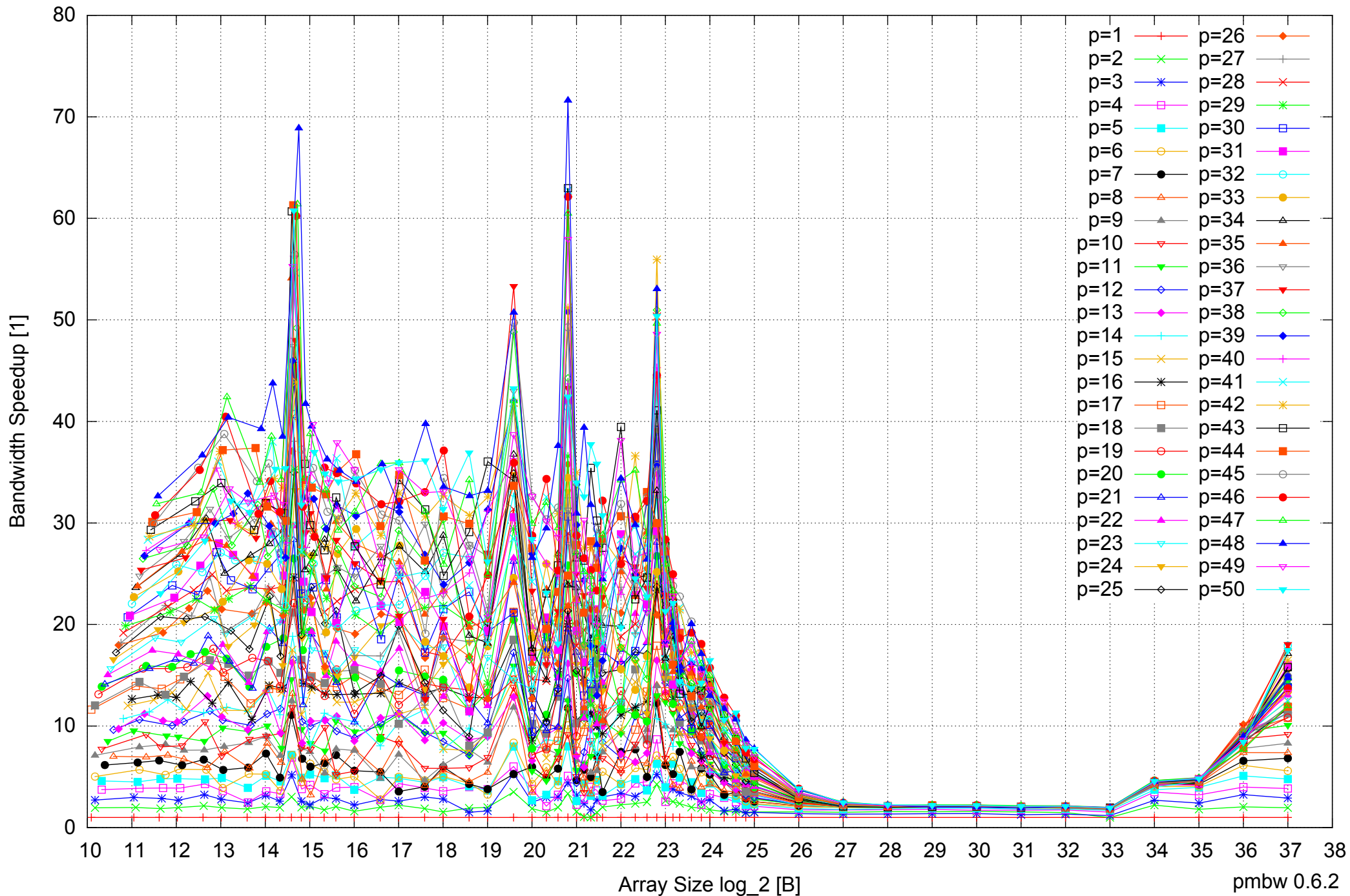
AMD Opteron 6168 256GB - Speedup of Parallel Memory Bandwidth - ScanWrite32PtrSimpleLoop
