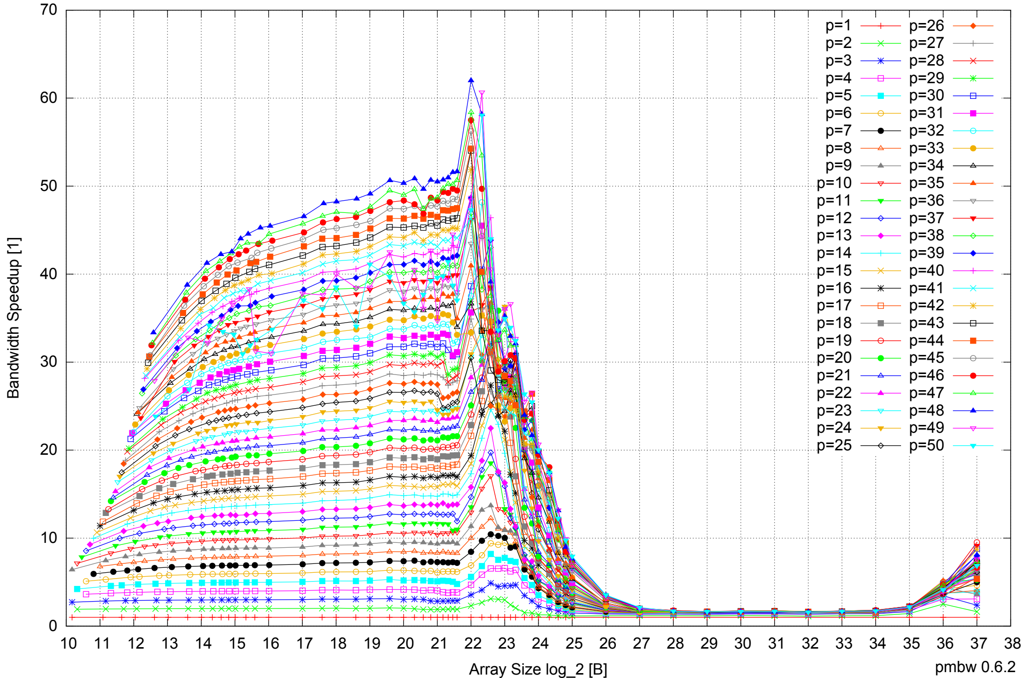
AMD Opteron 6168 256GB - Speedup of Parallel Memory Bandwidth - ScanWrite64IndexSimpleLoop
