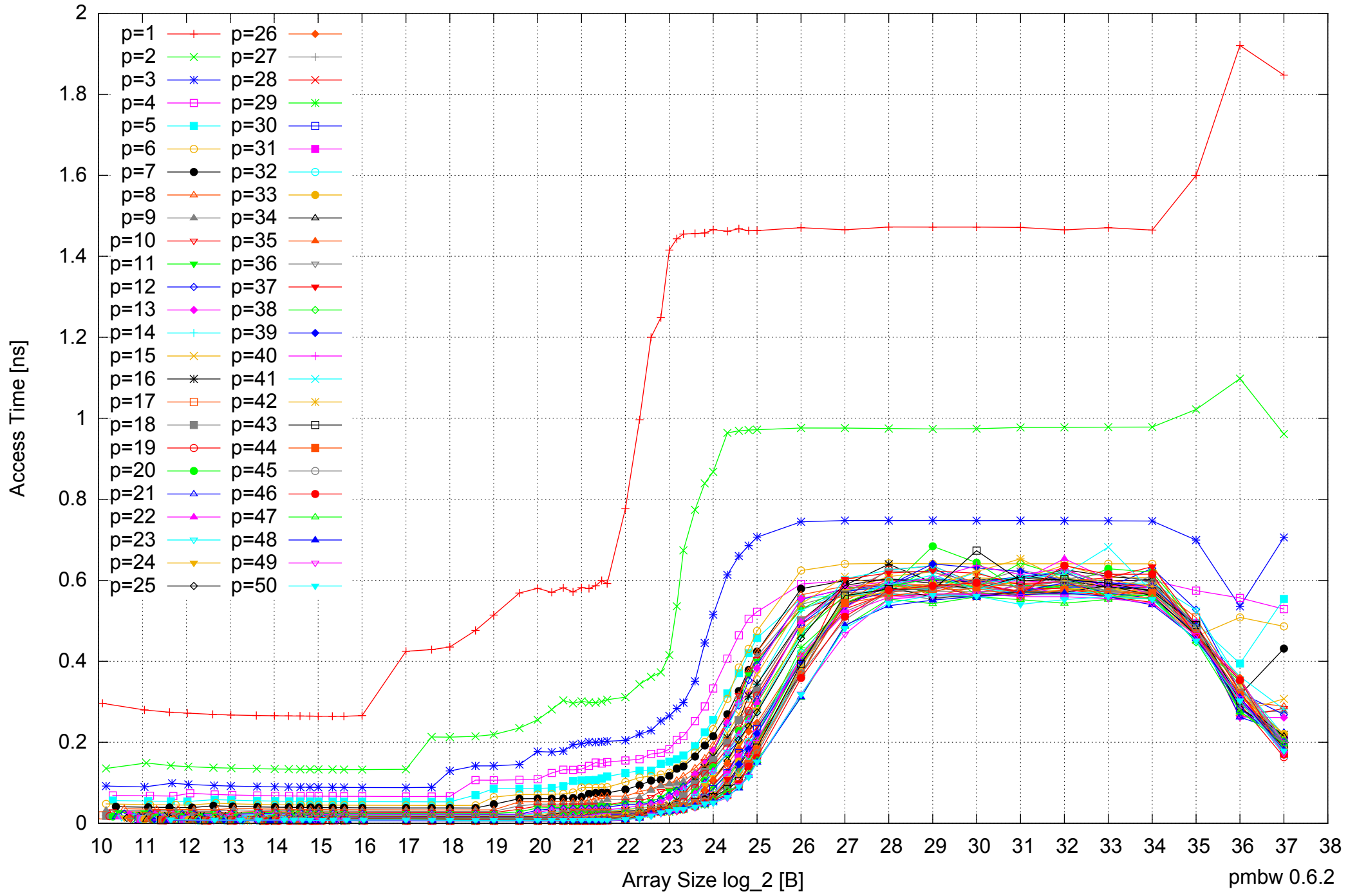
AMD Opteron 6168 256GB - Parallel Memory Access Time - ScanRead32PtrUnrollLoop
