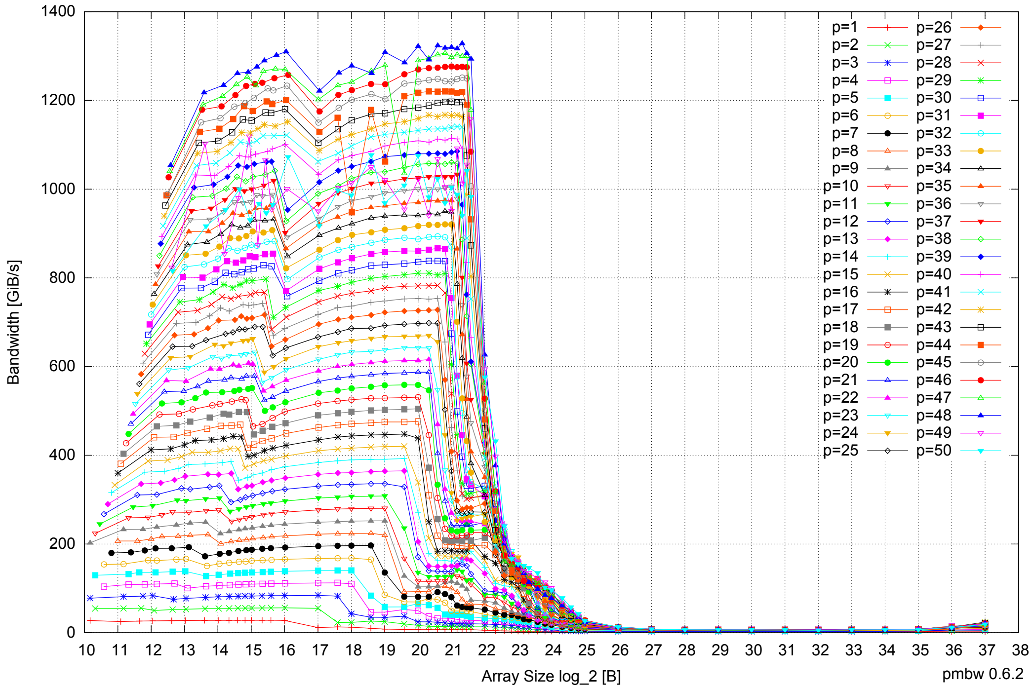
AMD Opteron 6168 256GB - Parallel Memory Bandwidth - ScanRead64IndexUnrollLoop
