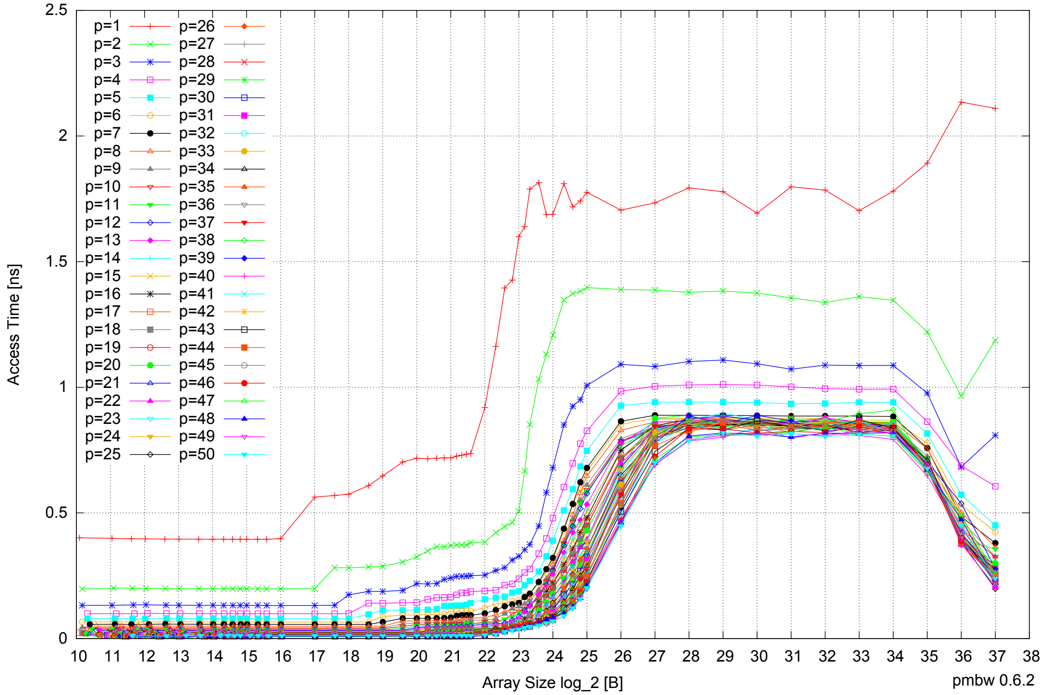
AMD Opteron 6168 256GB - Parallel Memory Access Time - ScanWrite32PtrUnrollLoop
