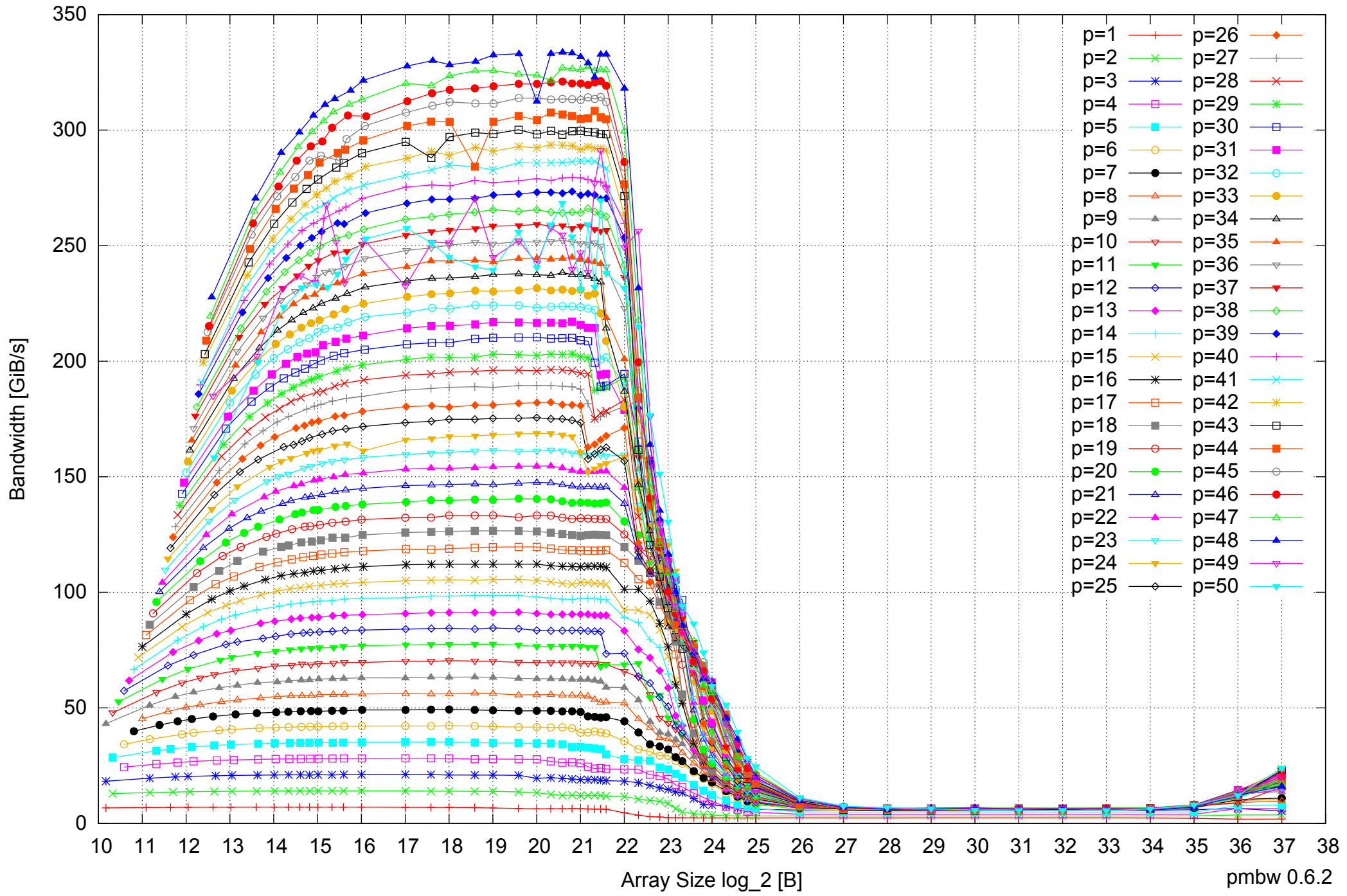
AMD Opteron 6168 256GB - Parallel Memory Bandwidth - ScanRead64PtrSimpleLoop
