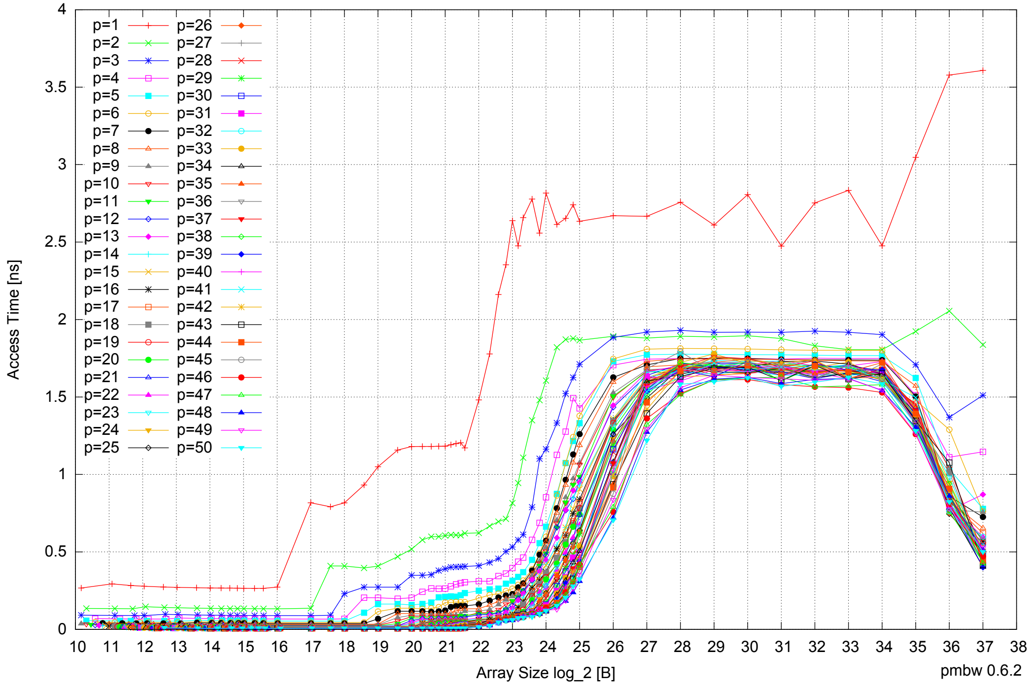
AMD Opteron 6168 256GB - Parallel Memory Access Time - ScanWrite64IndexUnrollLoop
