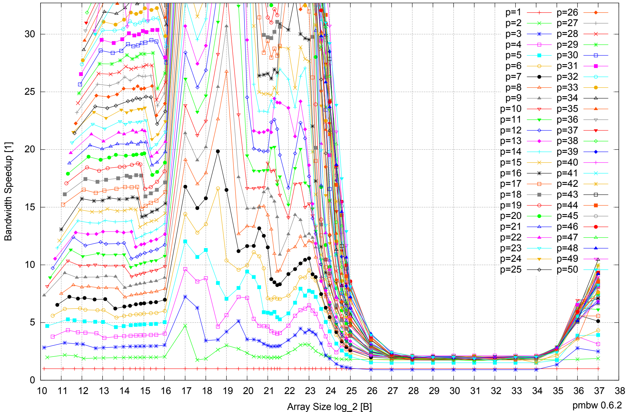
AMD Opteron 6168 256GB - Speedup of Parallel Memory Bandwidth (enlarged) - ScanRead64IndexUnrollLoop
