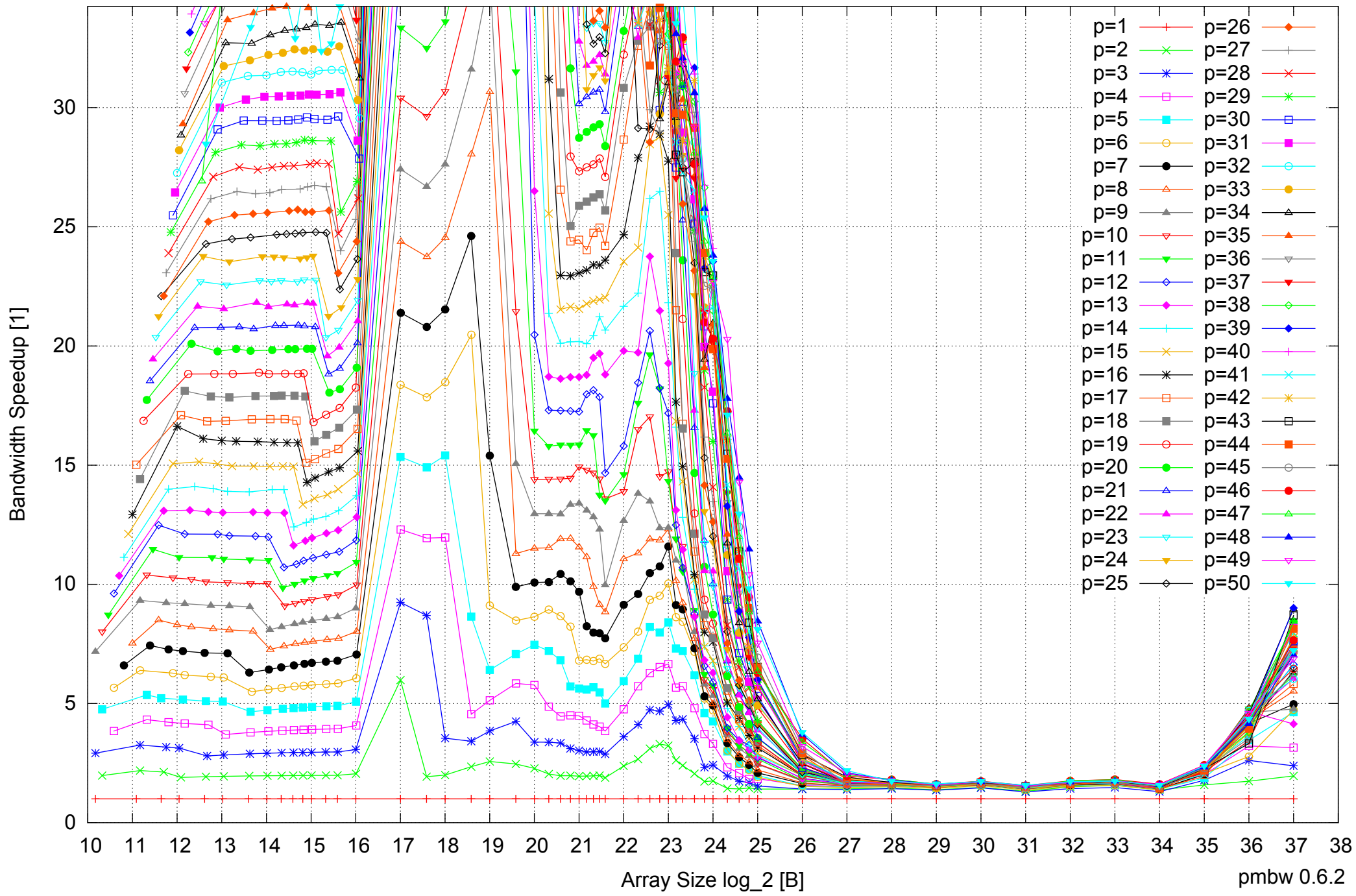
AMD Opteron 6168 256GB - Speedup of Parallel Memory Bandwidth (enlarged) - ScanWrite64IndexUnrollLoop
