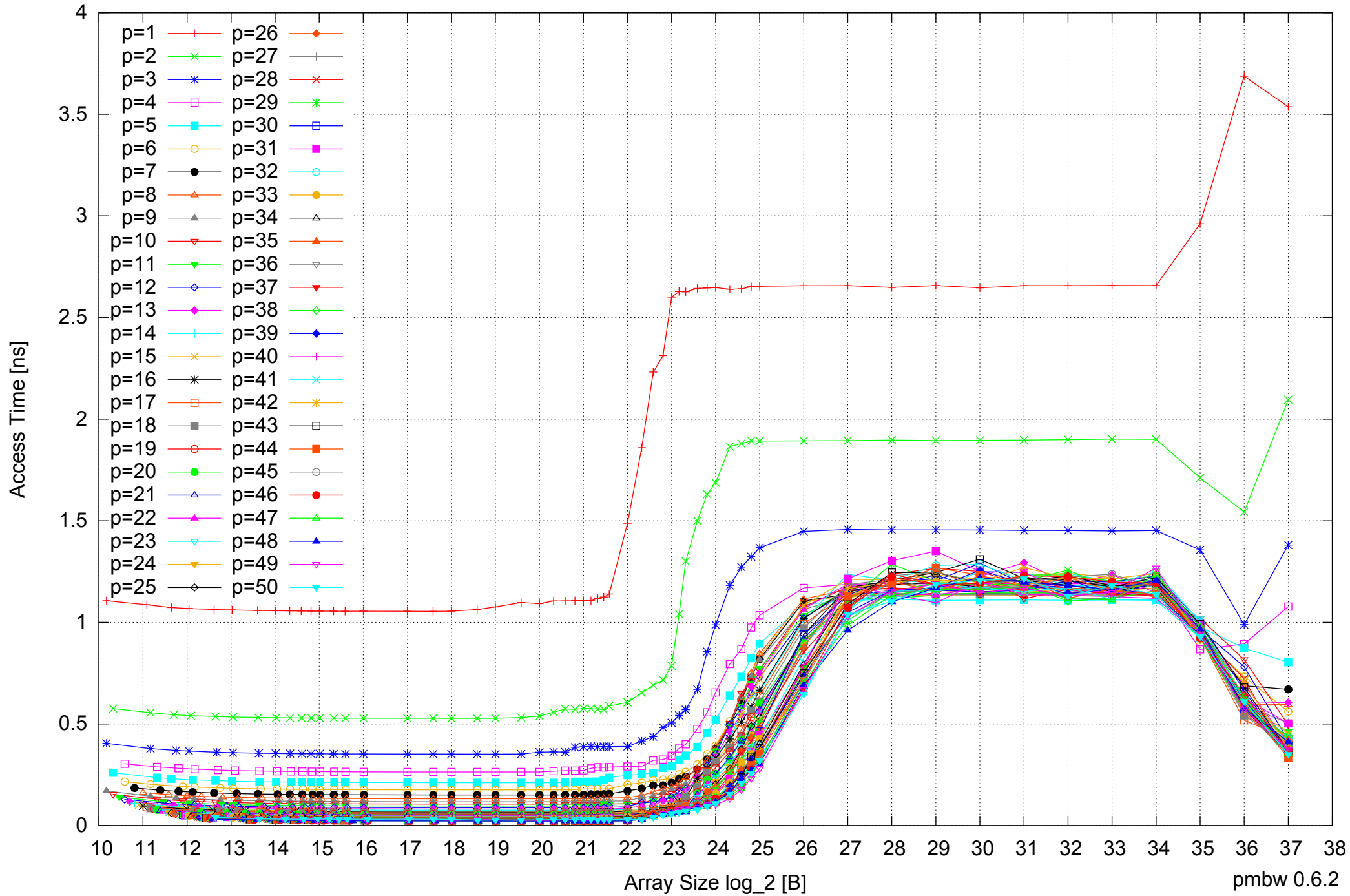
AMD Opteron 6168 256GB - Parallel Memory Access Time - ScanRead64IndexSimpleLoop
