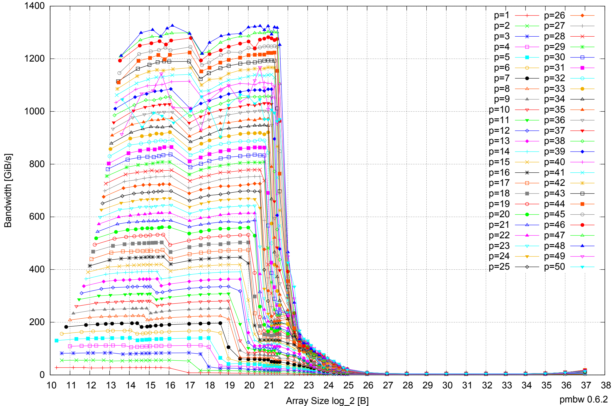
AMD Opteron 6168 256GB - Parallel Memory Bandwidth - ScanWrite128PtrUnrollLoop
