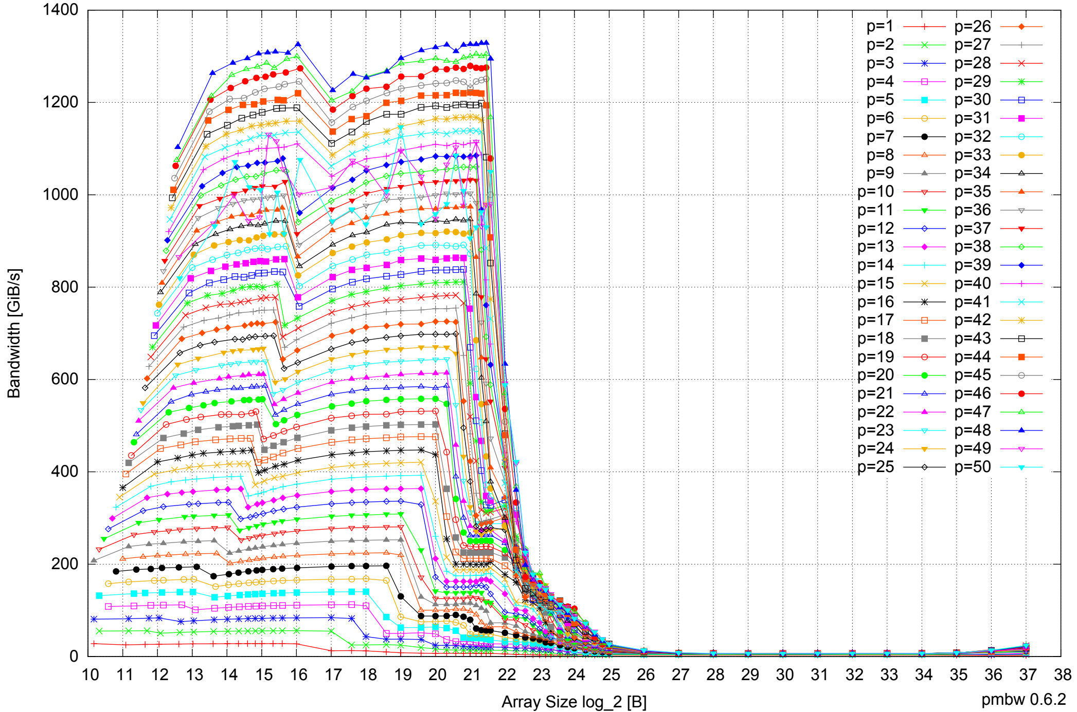
AMD Opteron 6168 256GB - Parallel Memory Bandwidth - ScanRead64PtrUnrollLoop
