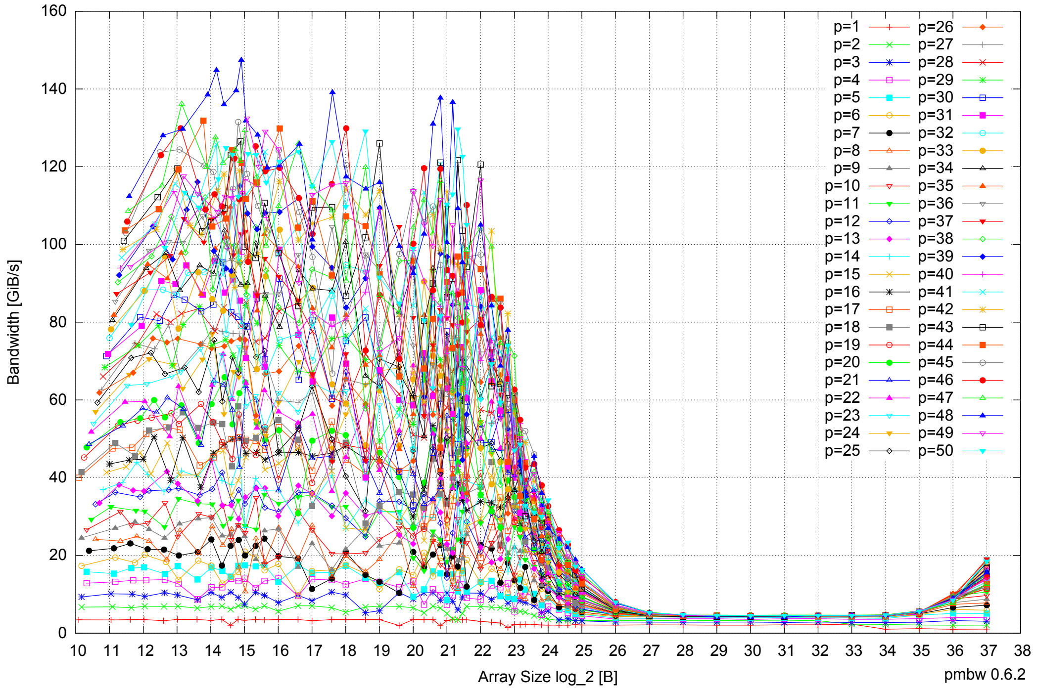
AMD Opteron 6168 256GB - Parallel Memory Bandwidth - ScanWrite32PtrSimpleLoop
