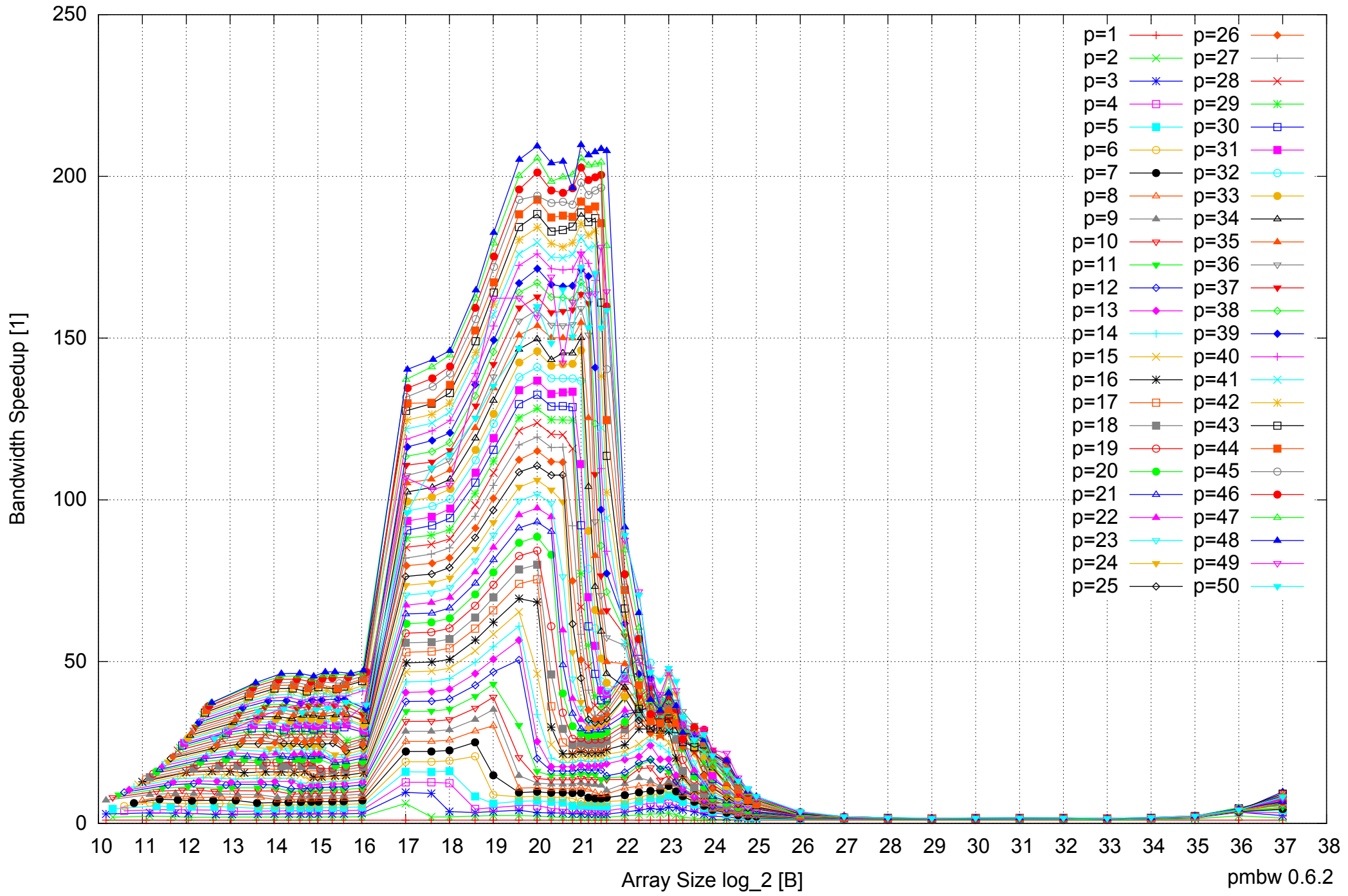
AMD Opteron 6168 256GB - Speedup of Parallel Memory Bandwidth - ScanWrite64PtrUnrollLoop
