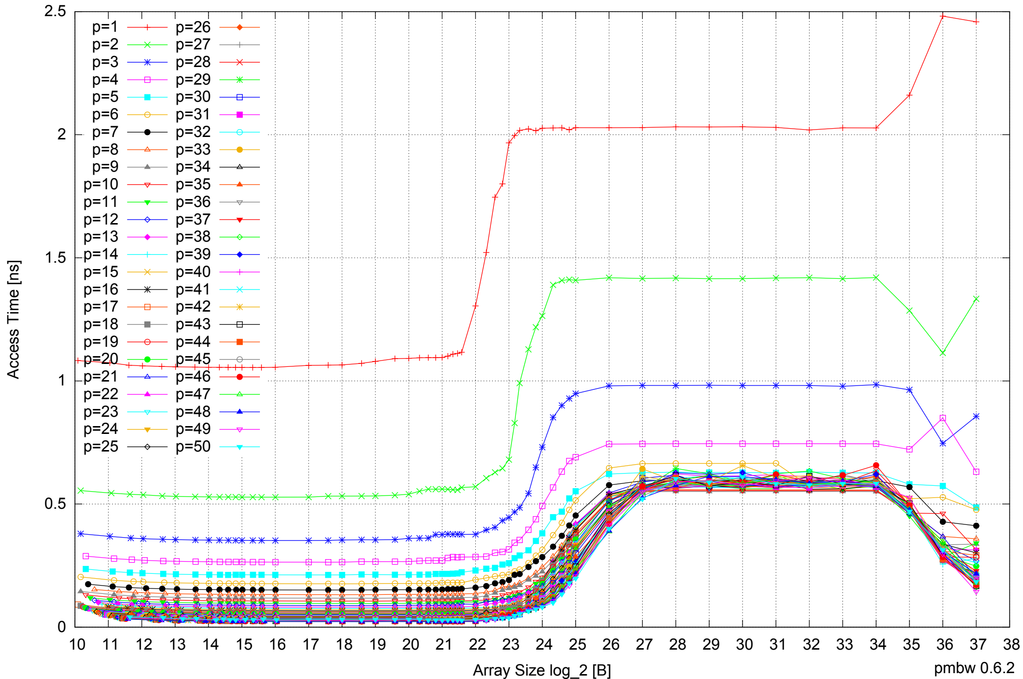
AMD Opteron 6168 256GB - Parallel Memory Access Time - ScanRead32PtrSimpleLoop
