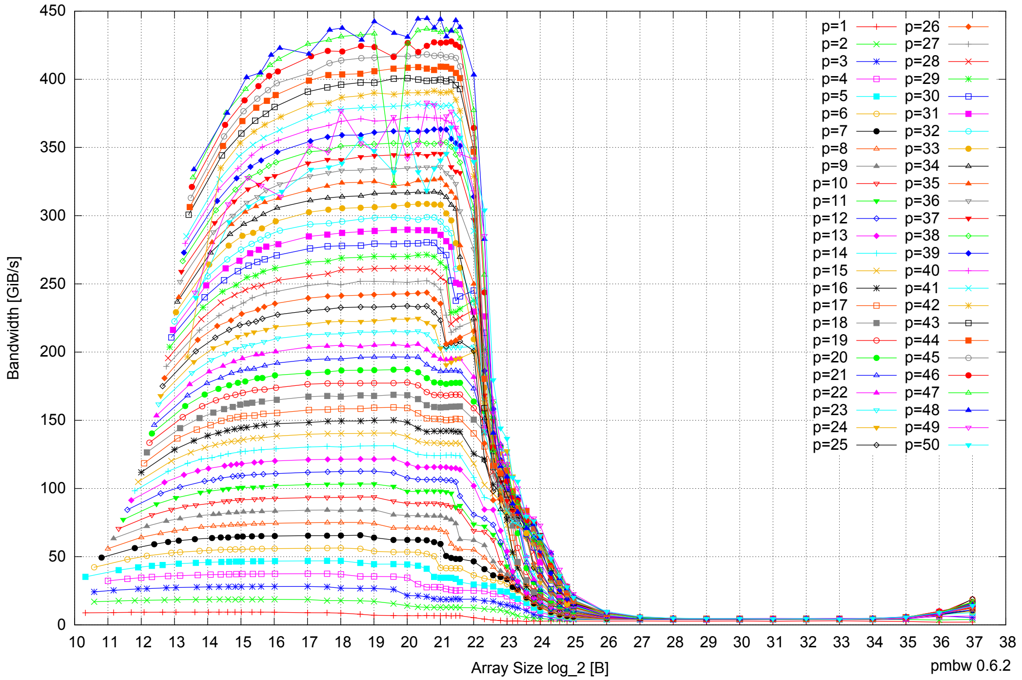
AMD Opteron 6168 256GB - Parallel Memory Bandwidth - ScanWrite128PtrSimpleLoop
