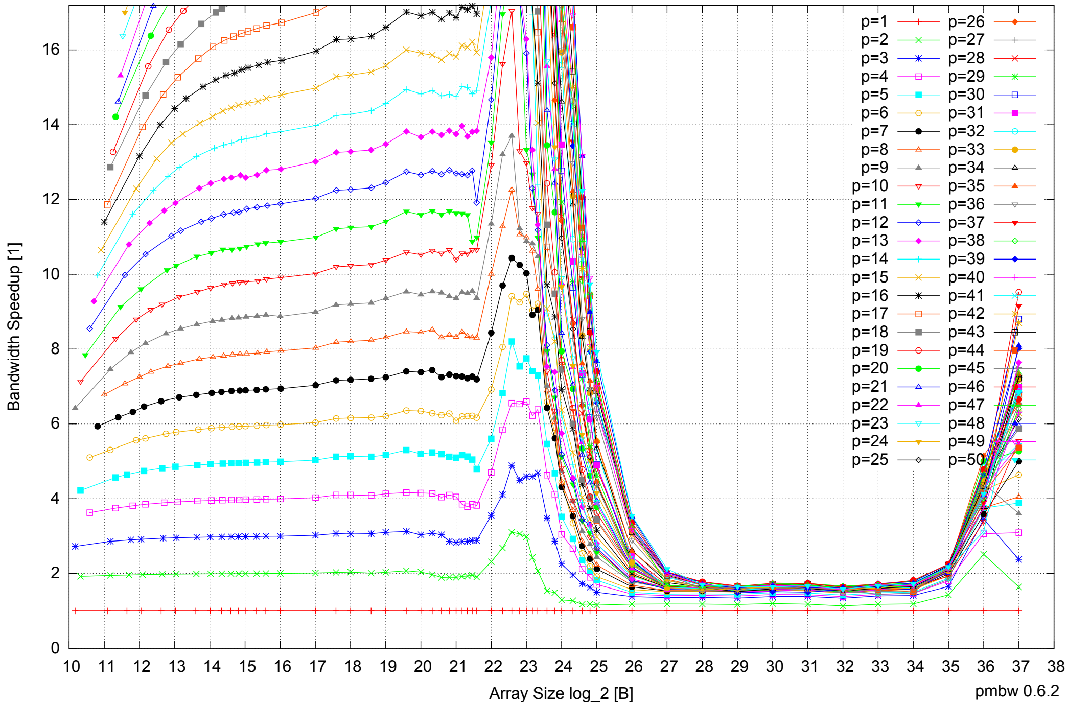
AMD Opteron 6168 256GB - Speedup of Parallel Memory Bandwidth (enlarged) - ScanWrite64IndexSimpleLoop
