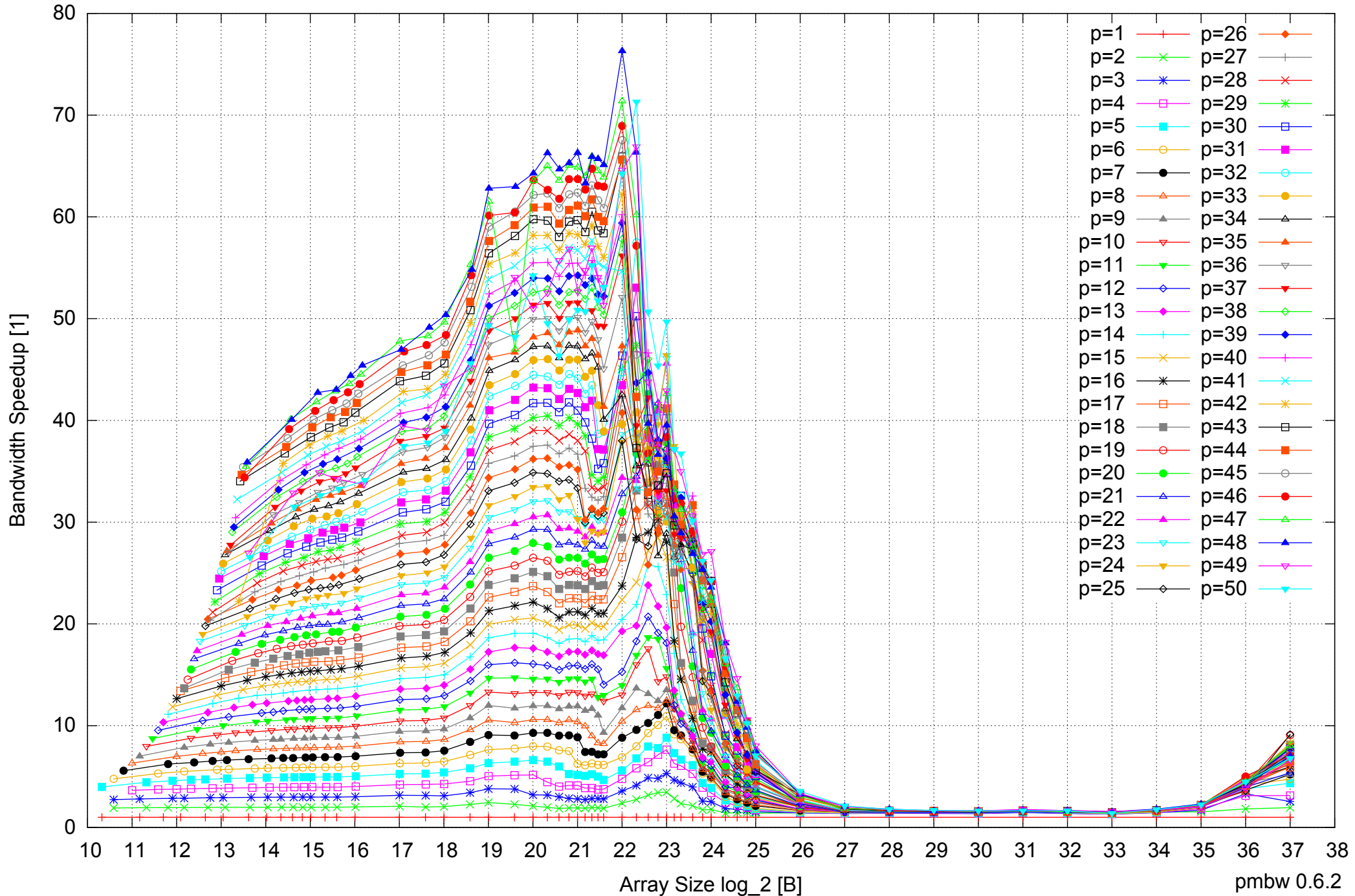
AMD Opteron 6168 256GB - Speedup of Parallel Memory Bandwidth - ScanWrite128PtrSimpleLoop
