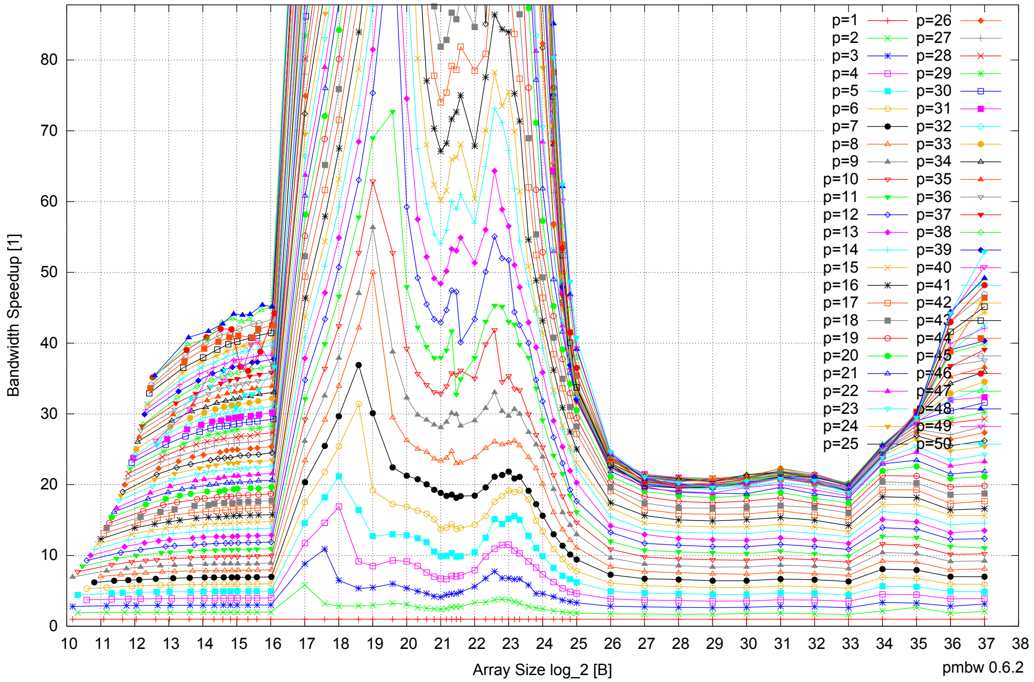
AMD Opteron 6168 256GB - Speedup of Parallel Memory Bandwidth (enlarged) - PermRead64SimpleLoop
