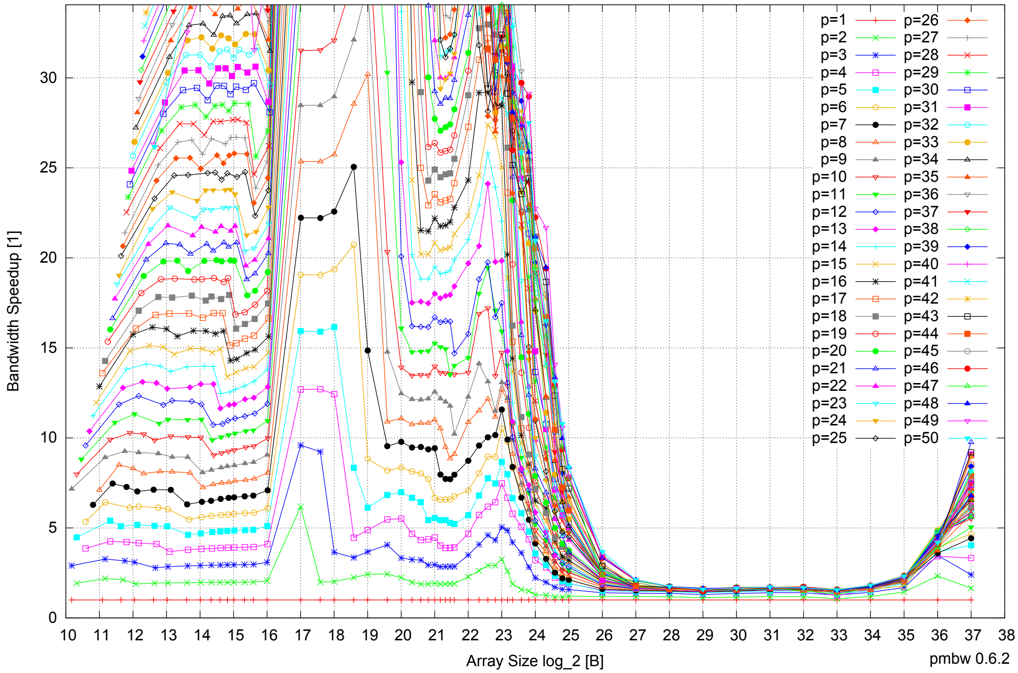
AMD Opteron 6168 256GB - Speedup of Parallel Memory Bandwidth (enlarged) - ScanWrite64PtrUnrollLoop
