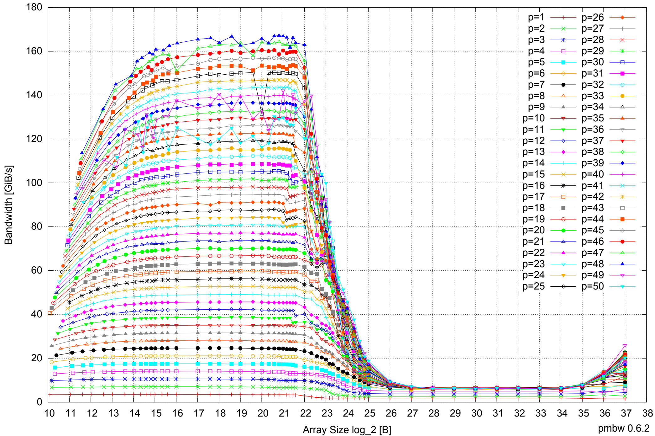
AMD Opteron 6168 256GB - Parallel Memory Bandwidth - ScanRead32PtrSimpleLoop
