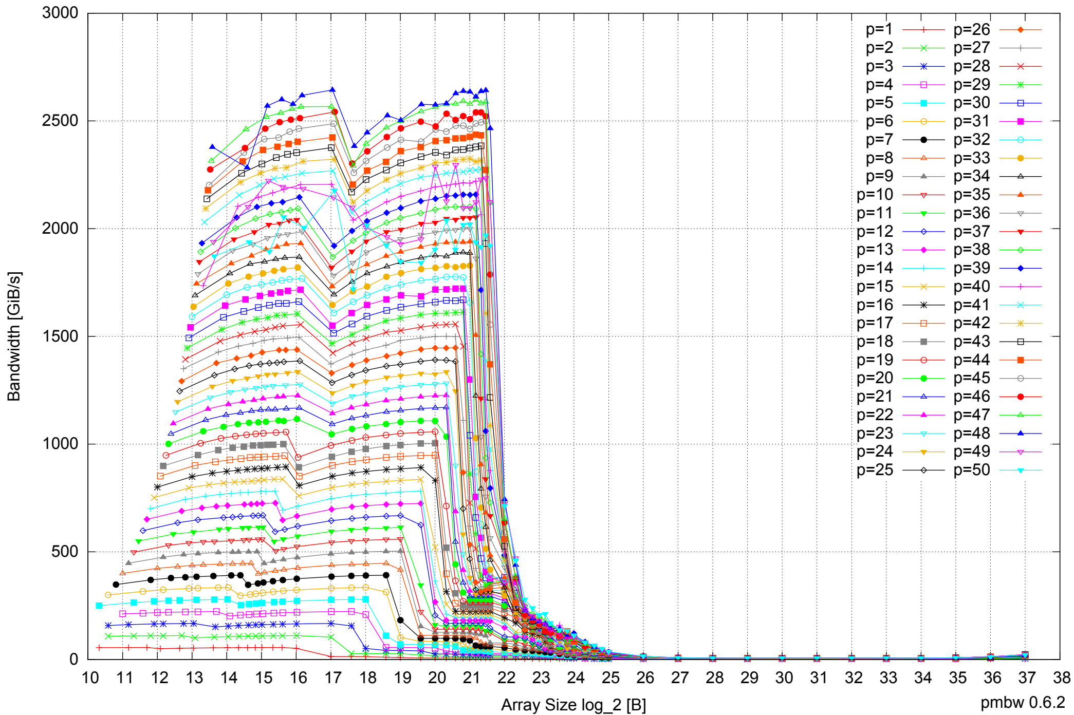
AMD Opteron 6168 256GB - Parallel Memory Bandwidth - ScanRead128PtrUnrollLoop
