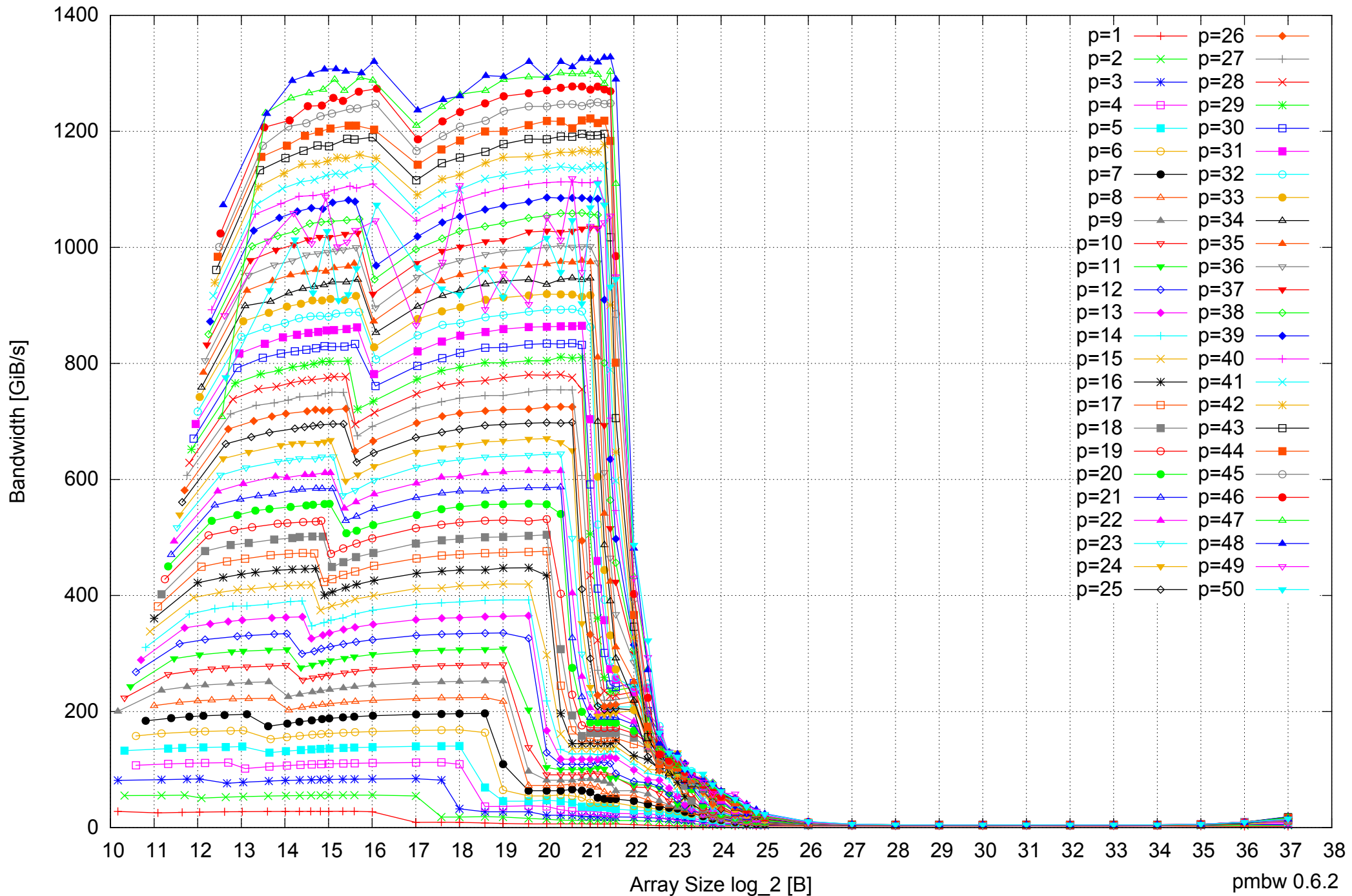
AMD Opteron 6168 256GB - Parallel Memory Bandwidth - ScanWrite64IndexUnrollLoop
