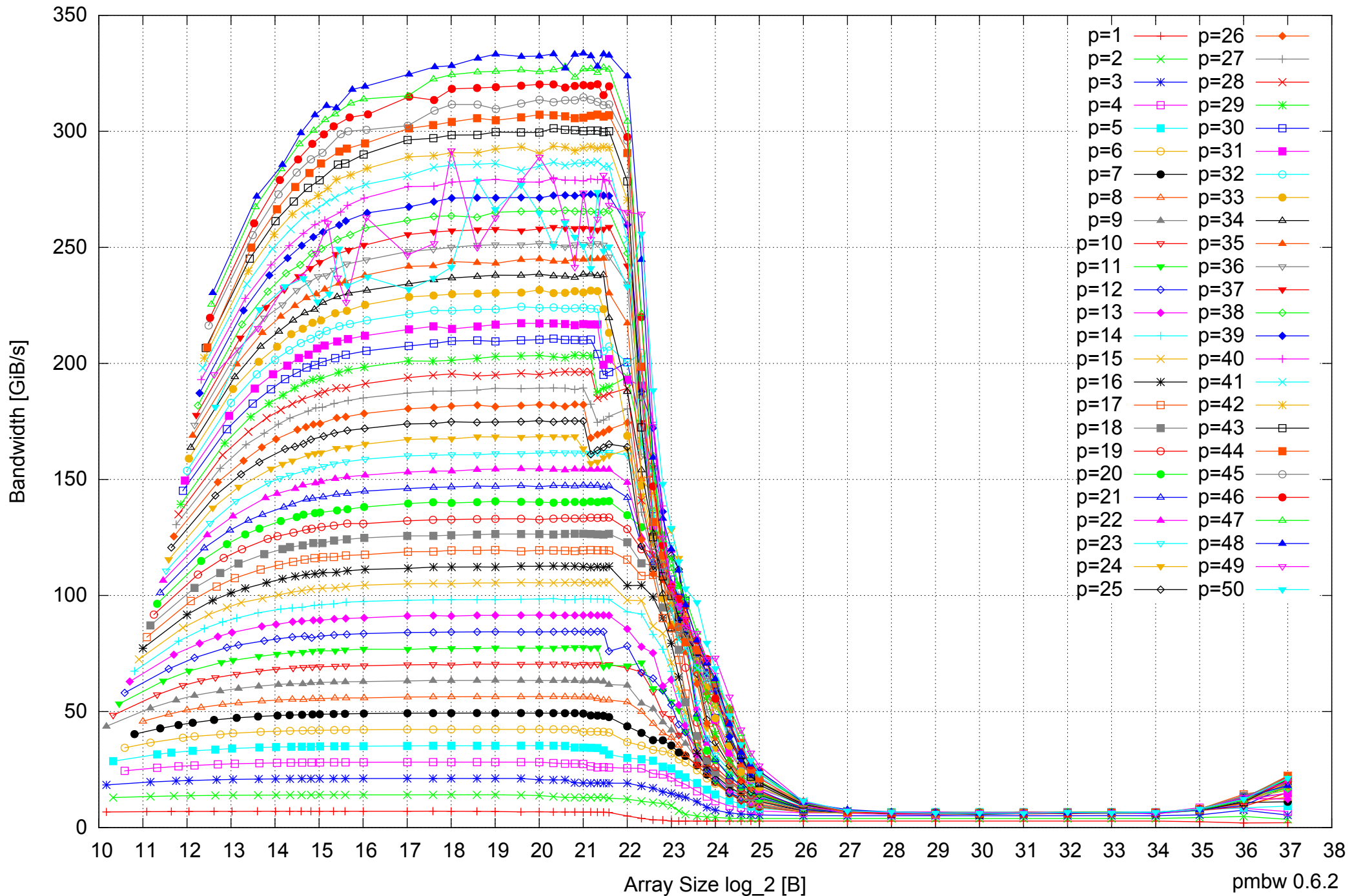
AMD Opteron 6168 256GB - Parallel Memory Bandwidth - ScanRead64IndexSimpleLoop
