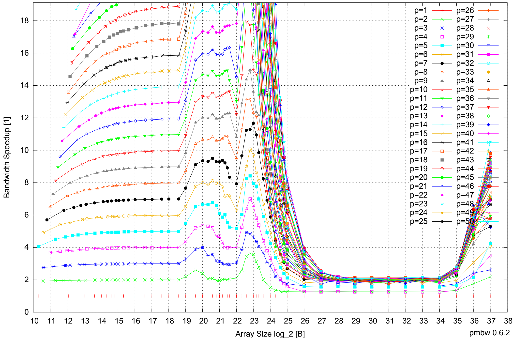
AMD Opteron 6168 256GB - Speedup of Parallel Memory Bandwidth (enlarged) - ScanRead128PtrSimpleLoop
