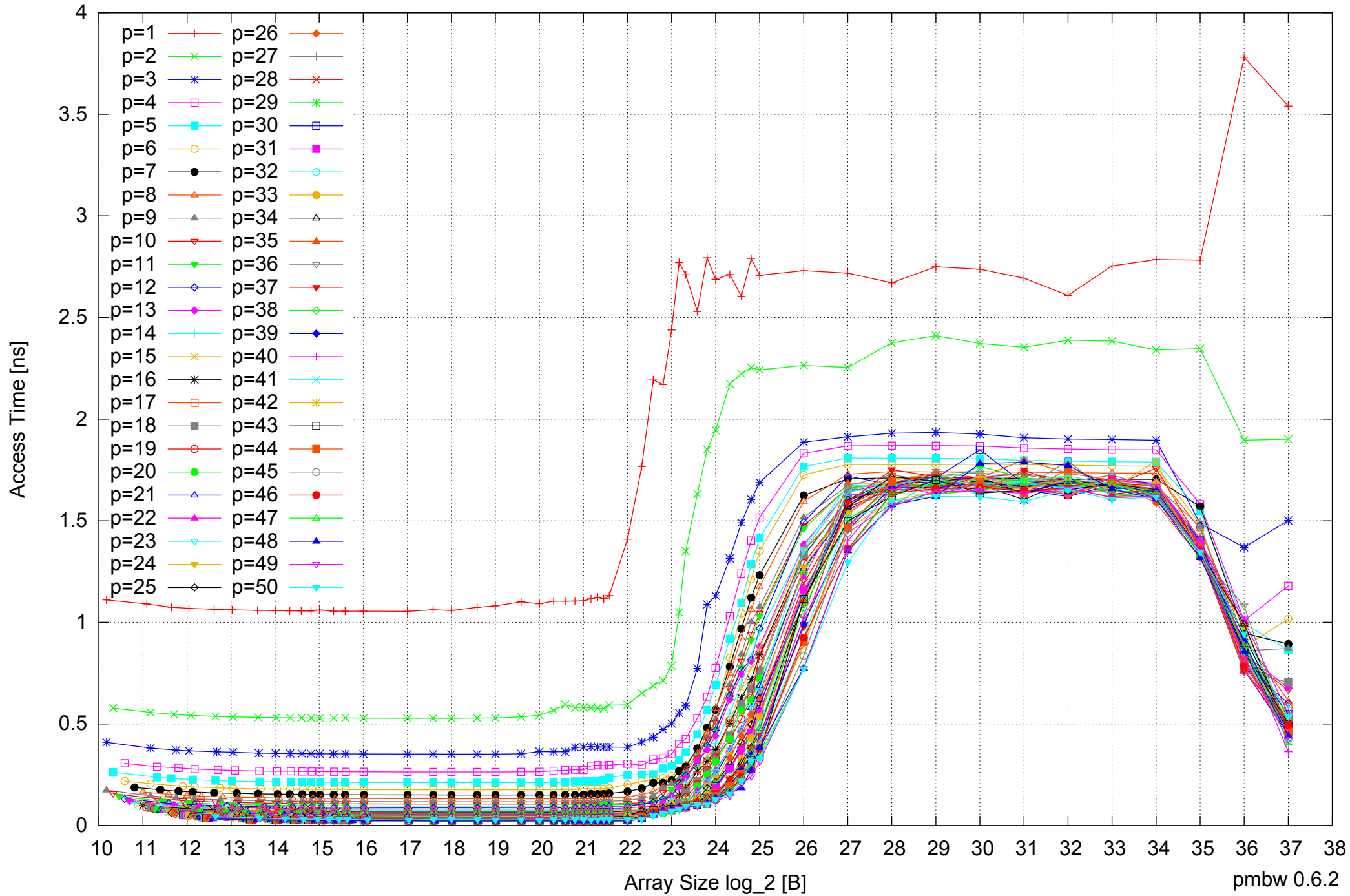
AMD Opteron 6168 256GB - Parallel Memory Access Time - ScanWrite64PtrSimpleLoop
