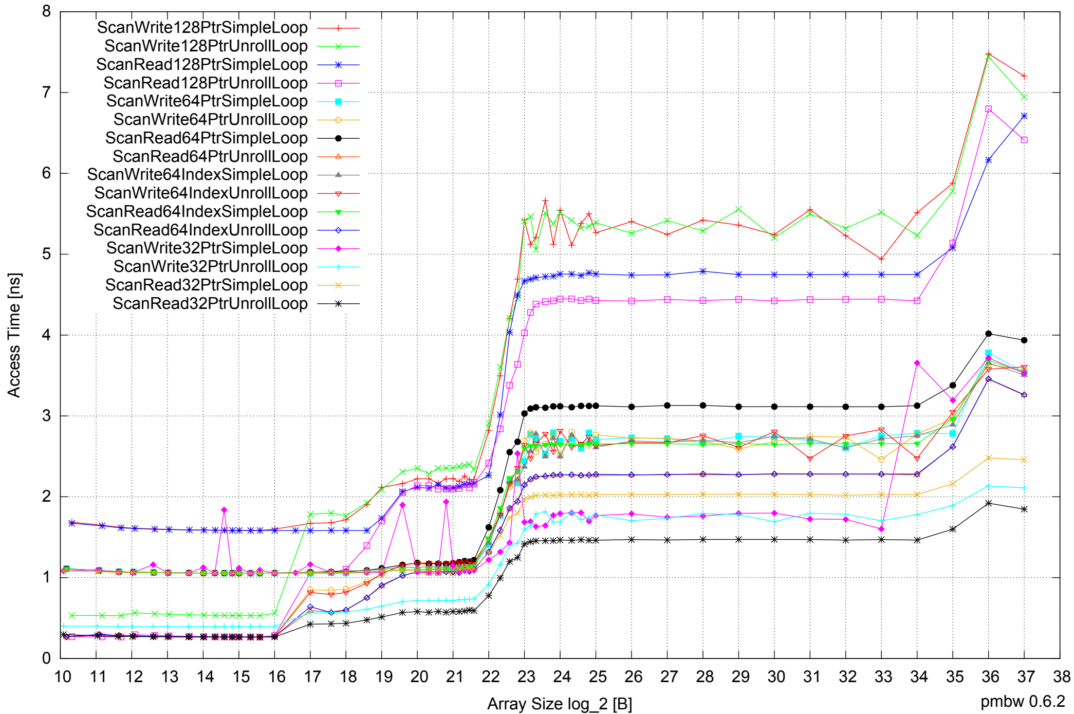
AMD Optron 6168 256GB - One Thread Memory Latency (excluding Permutation)
