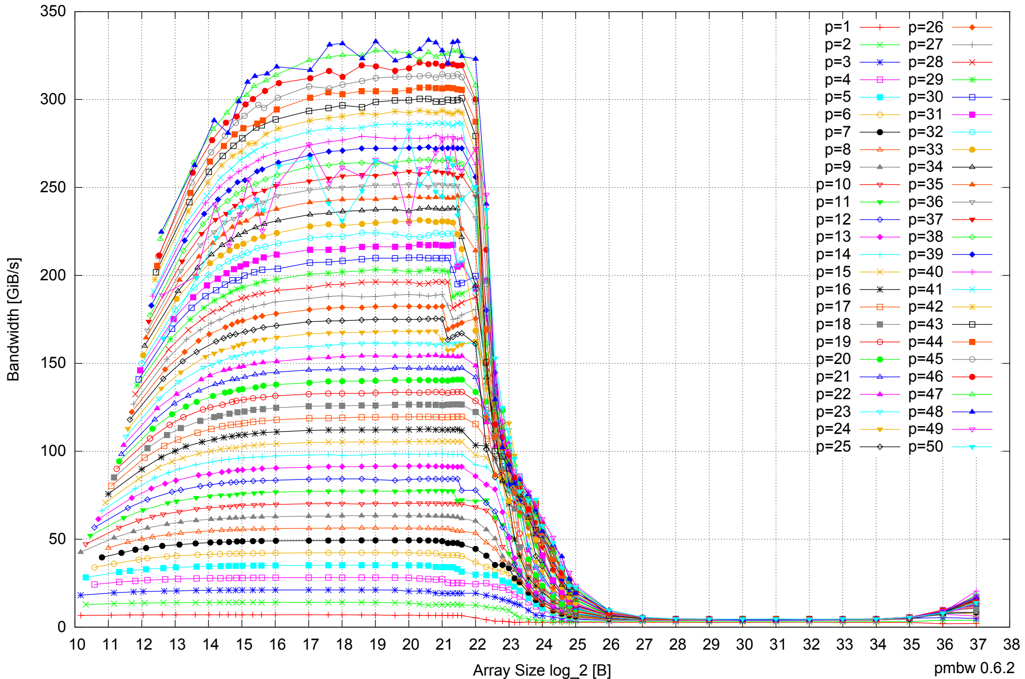
AMD Opteron 6168 256GB - Parallel Memory Bandwidth - ScanWrite64PtrSimpleLoop
