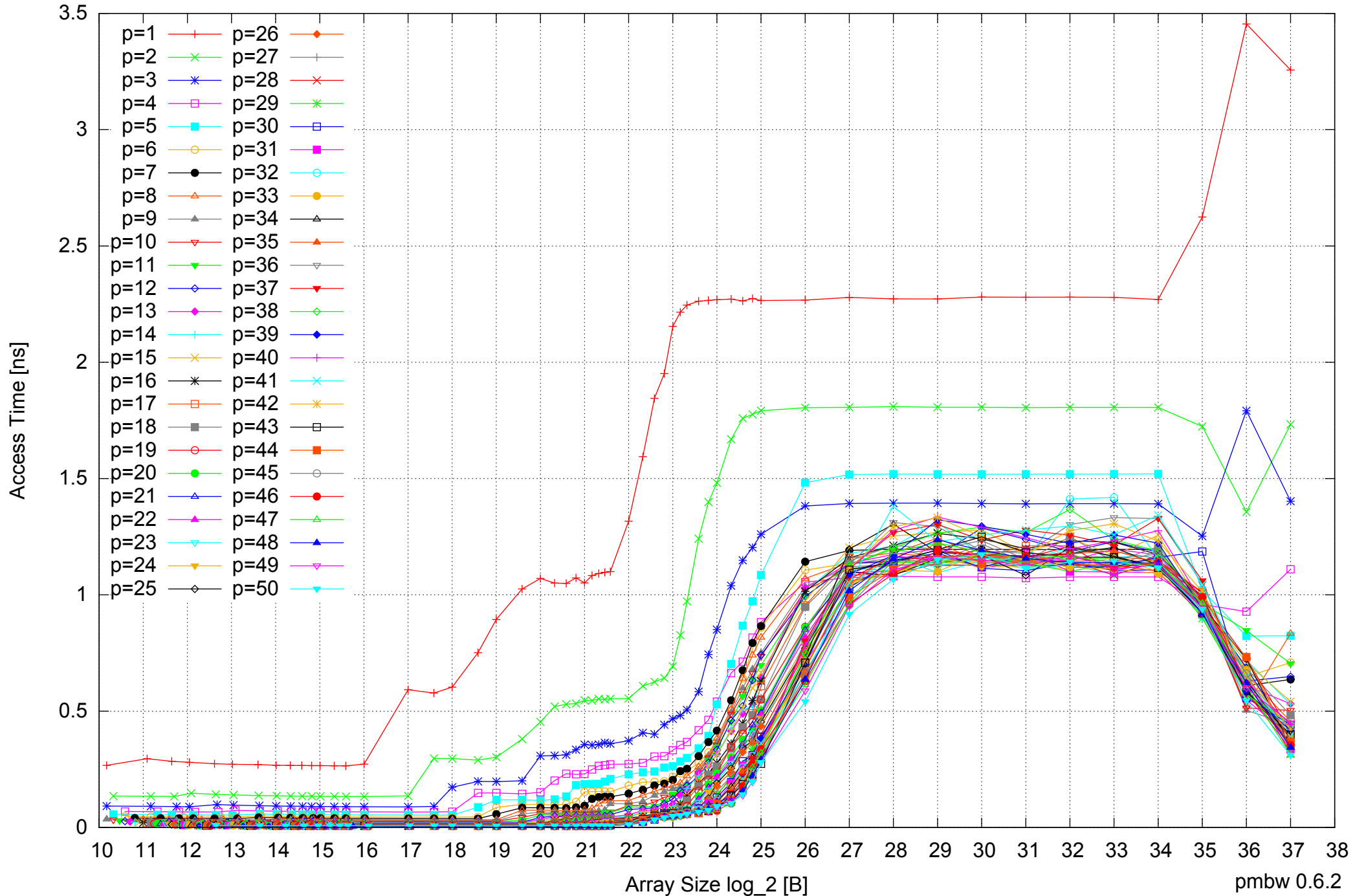
AMD Opteron 6168 256GB - Parallel Memory Access Time - ScanRead64PtrUnrollLoop
