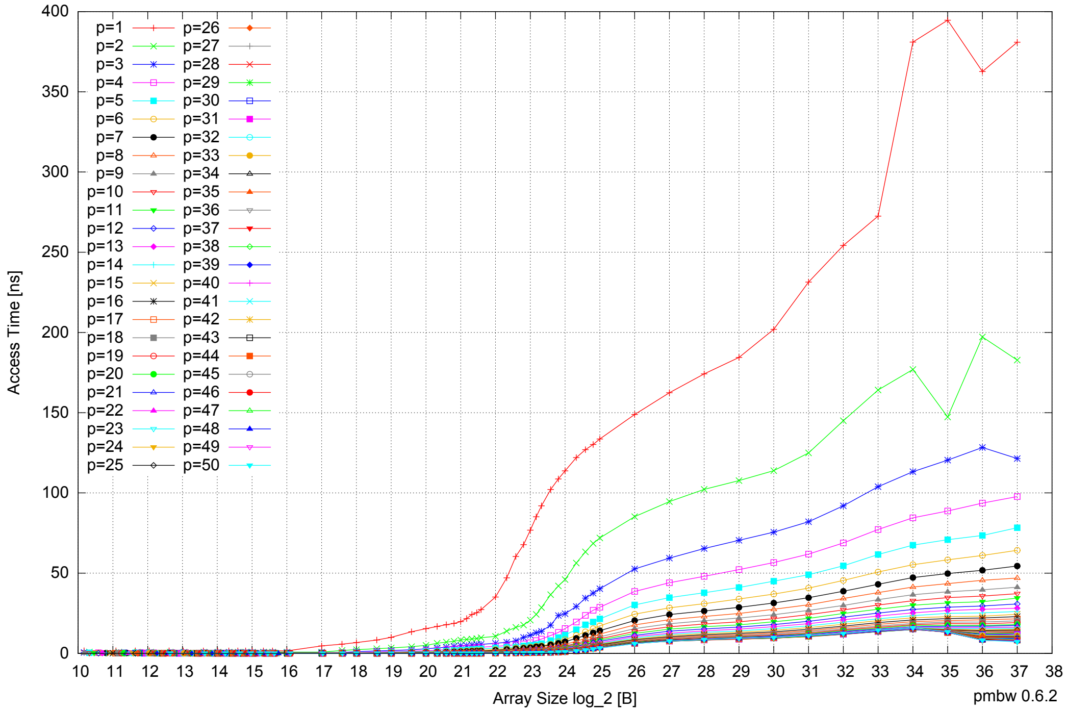
AMD Opteron 6168 256GB - Parallel Memory Access Time - PermRead64SimpleLoop
