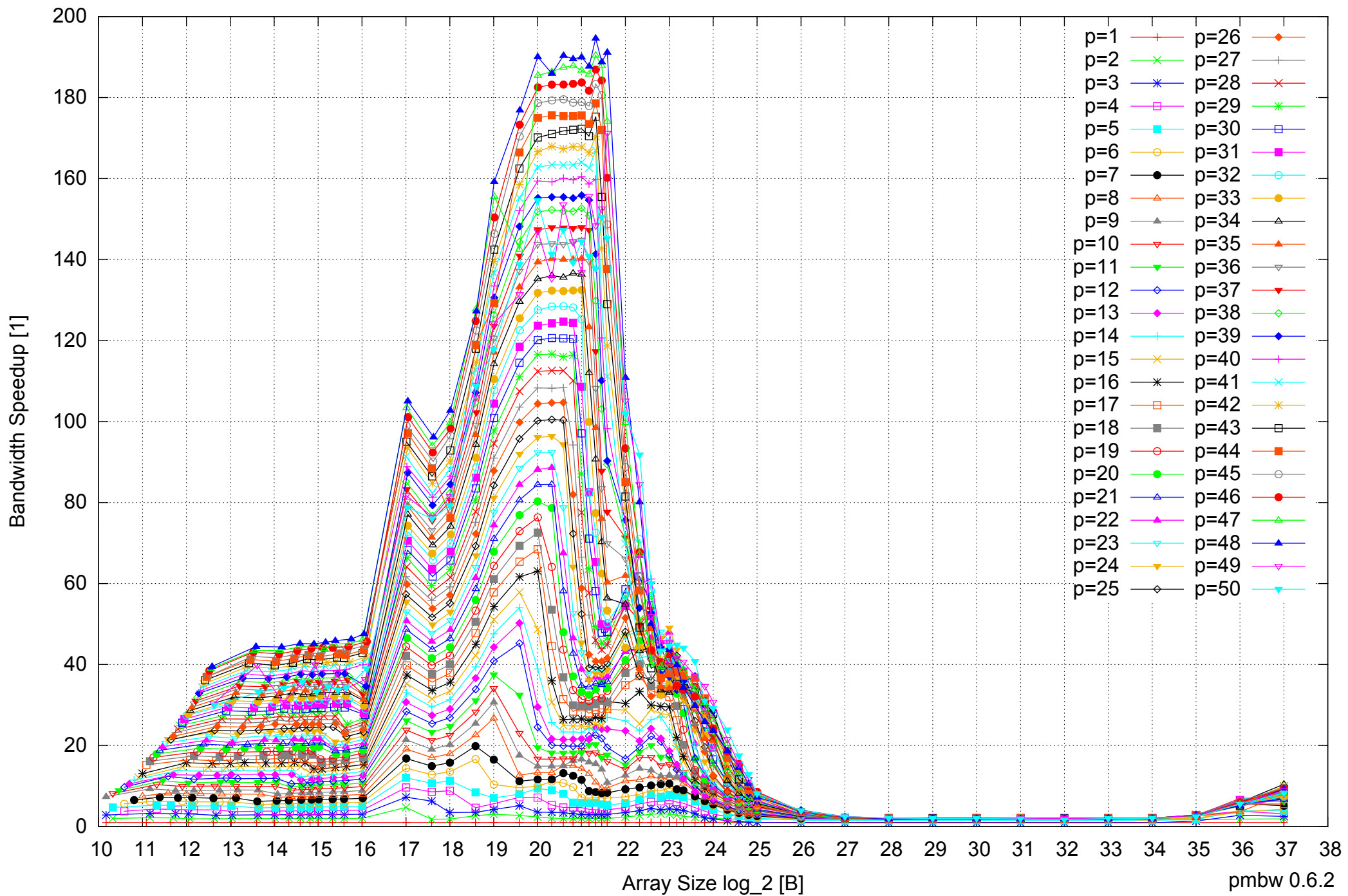
AMD Opteron 6168 256GB - Speedup of Parallel Memory Bandwidth - ScanRead64IndexUnrollLoop
