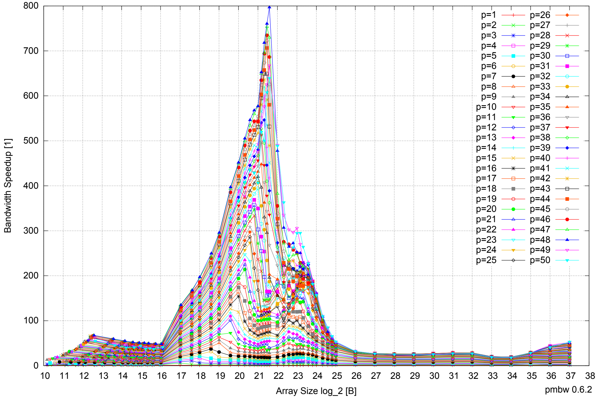
AMD Opteron 6168 256GB - Speedup of Parallel Memory Bandwidth - PermRead64UnrollLoop
