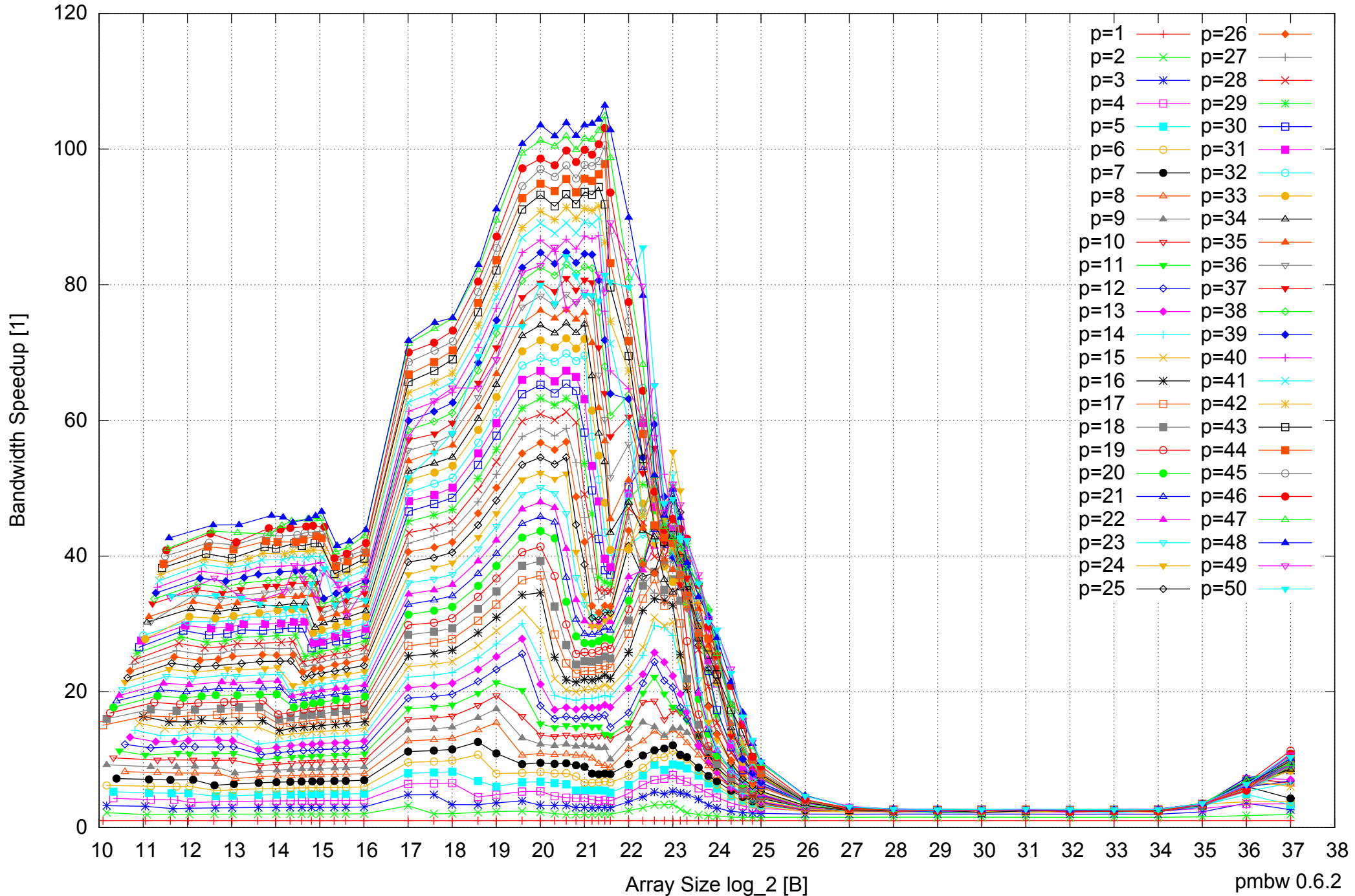
AMD Opteron 6168 256GB - Speedup of Parallel Memory Bandwidth - ScanRead32PtrUnrollLoop
