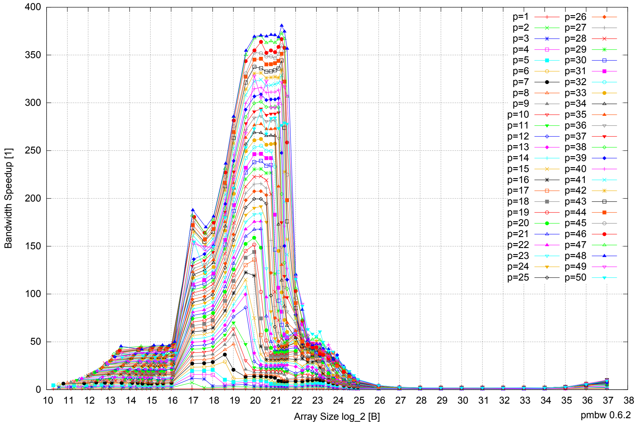
AMD Opteron 6168 256GB - Speedup of Parallel Memory Bandwidth - ScanRead128PtrUnrollLoop
