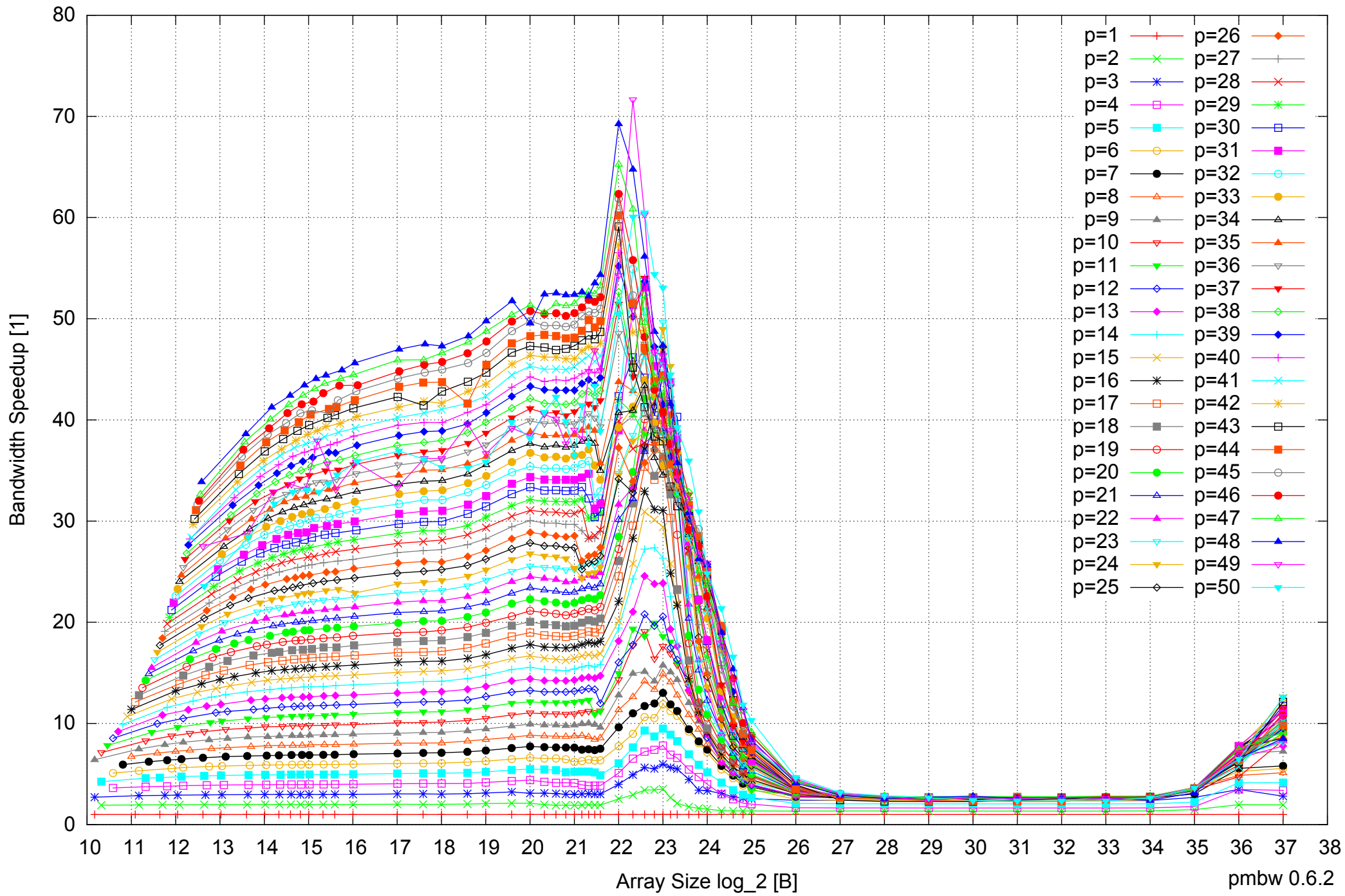
AMD Opteron 6168 256GB - Speedup of Parallel Memory Bandwidth - ScanRead64PtrSimpleLoop
