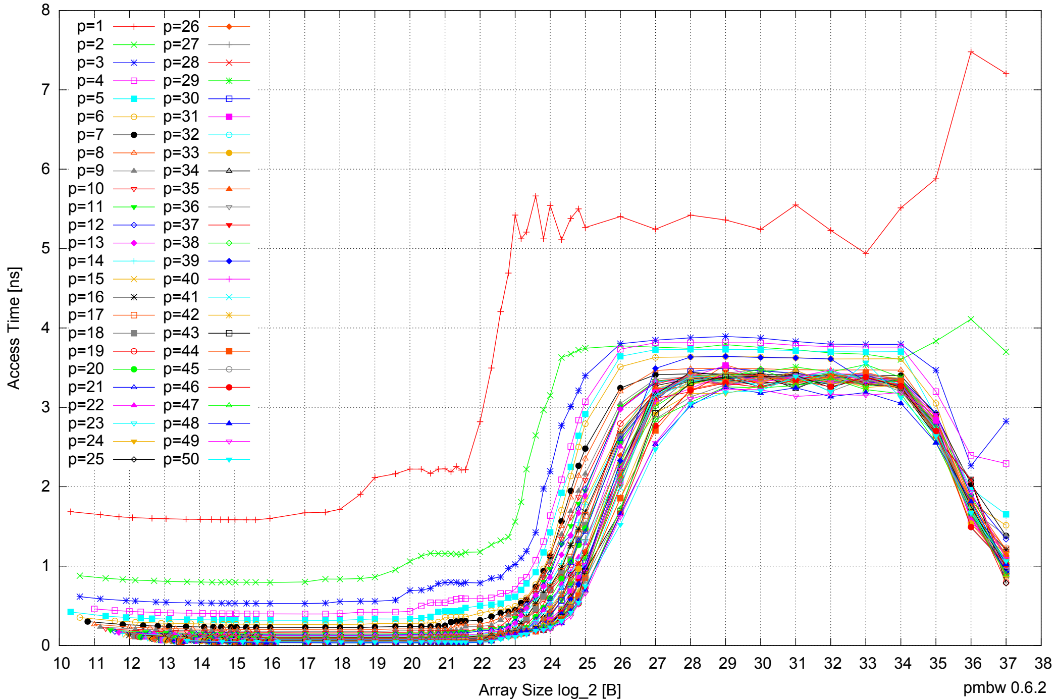
AMD Opteron 6168 256GB - Parallel Memory Access Time - ScanWrite128PtrSimpleLoop
