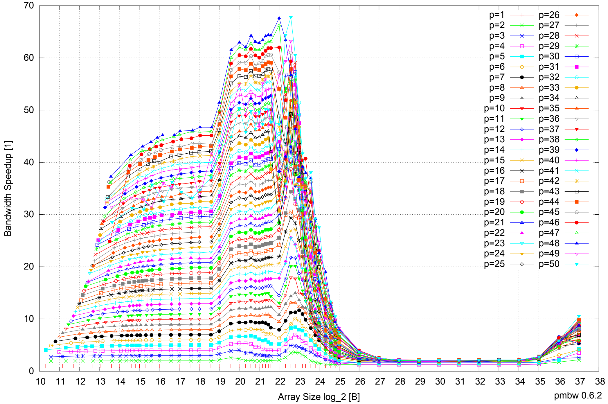
AMD Opteron 6168 256GB - Speedup of Parallel Memory Bandwidth - ScanRead128PtrSimpleLoop
