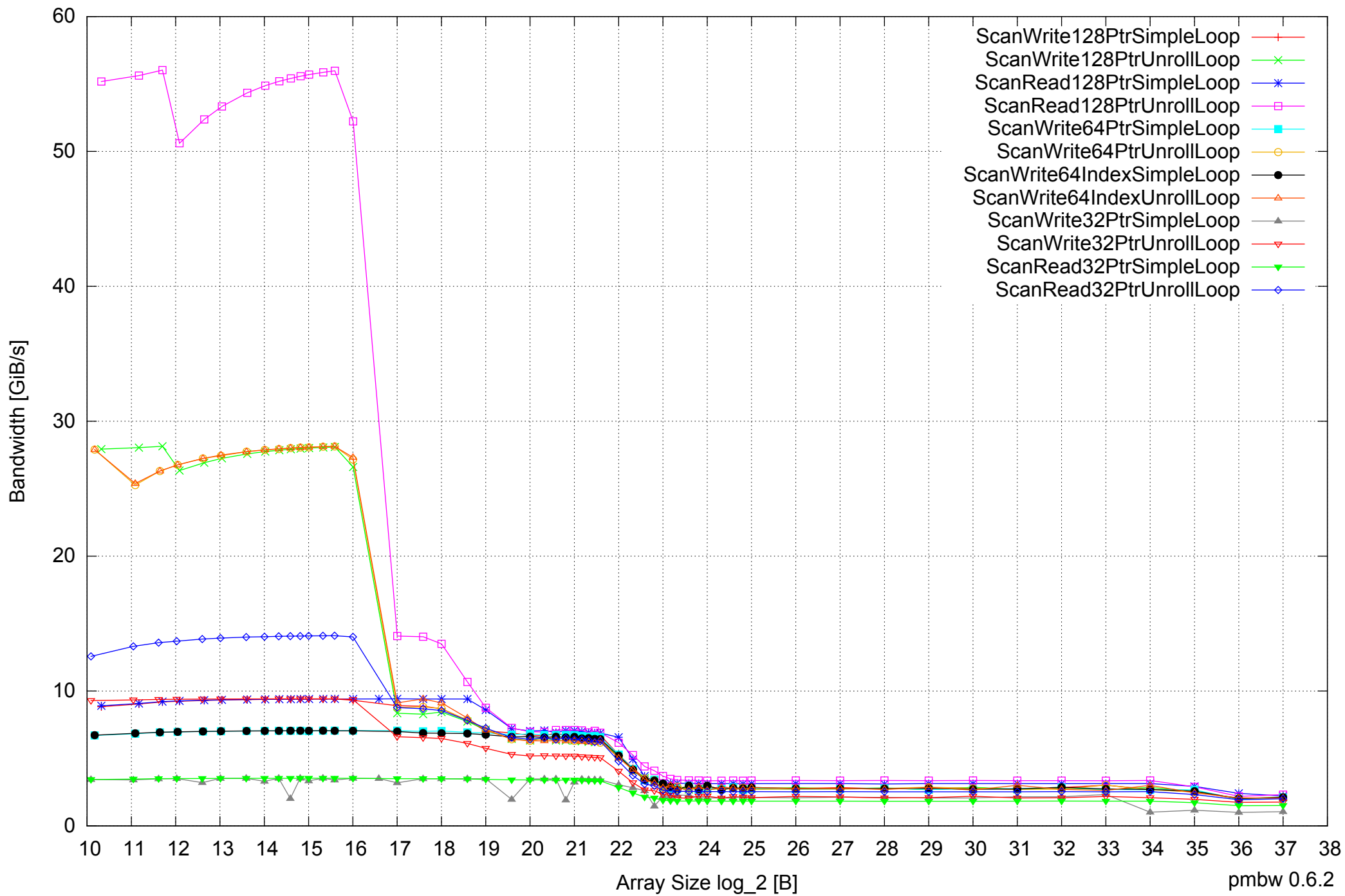
AMD Opteron 6168 256GB - One Thread Memory Bandwidth (only 64-bit Reads)
