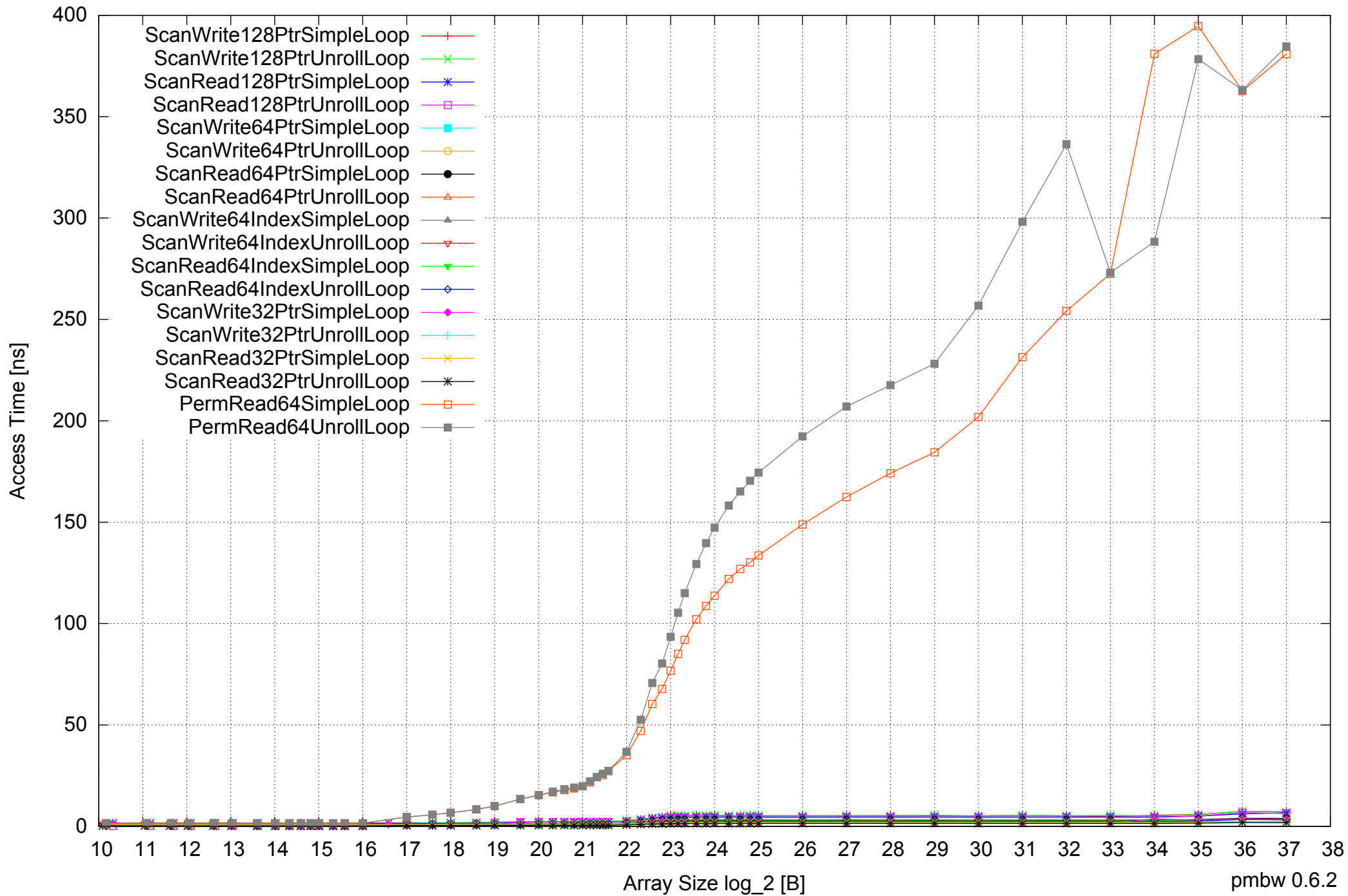
AMD Opteron 6168 256GB - One Thread Memory Latency (Access Time)
