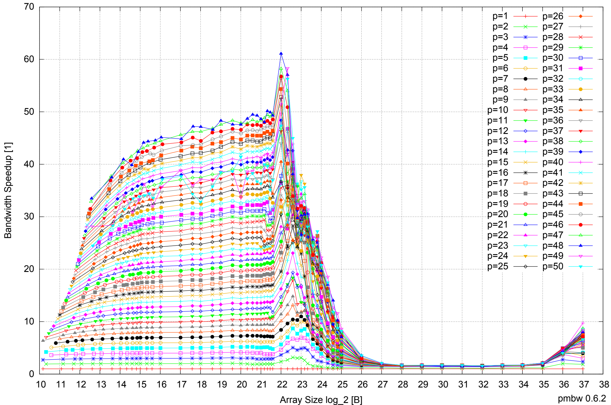
AMD Opteron 6168 256GB - Speedup of Parallel Memory Bandwidth - ScanWrite64PtrSimpleLoop
