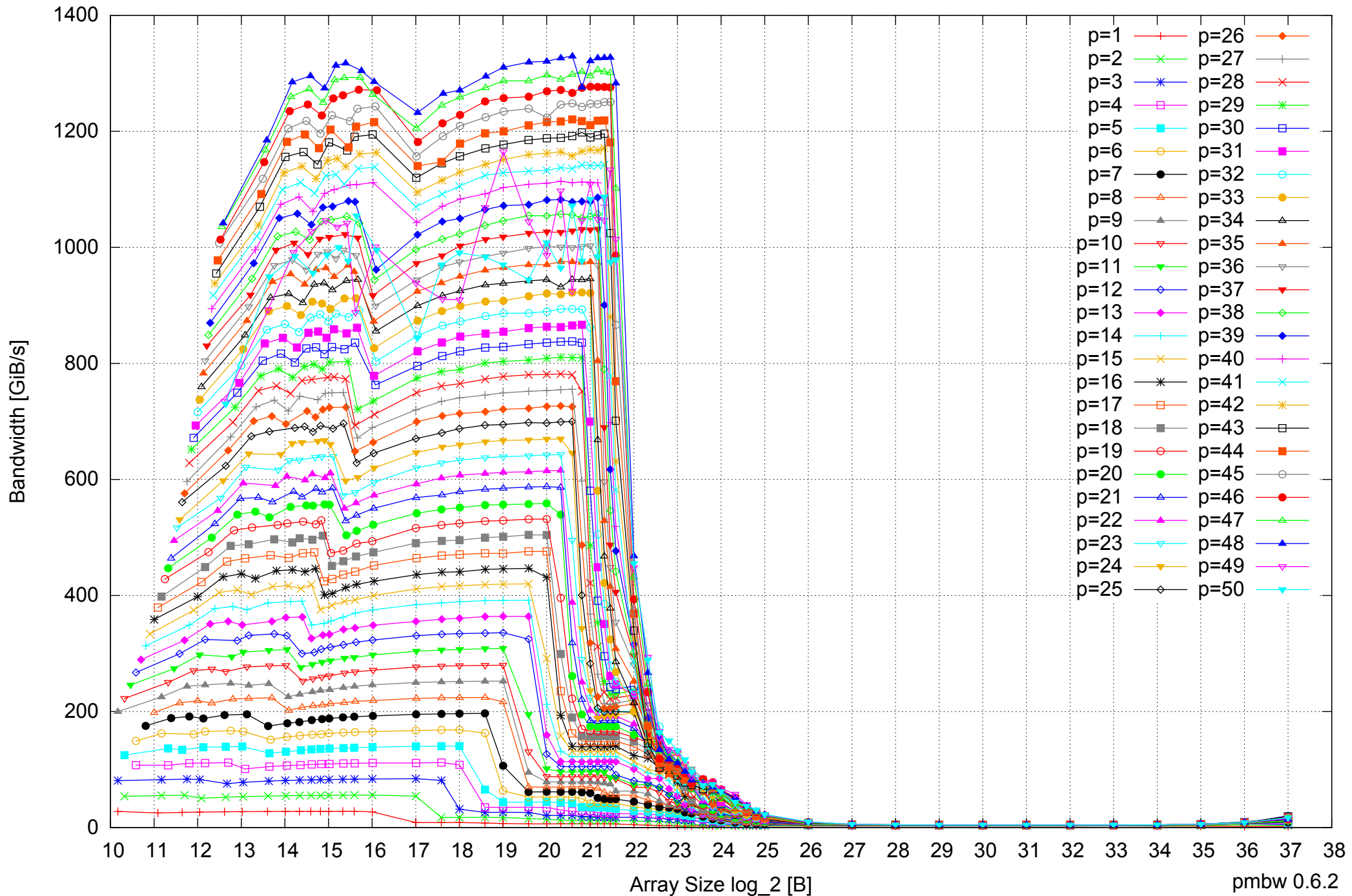
AMD Opteron 6168 256GB - Parallel Memory Bandwidth - ScanWrite64PtrUnrollLoop
