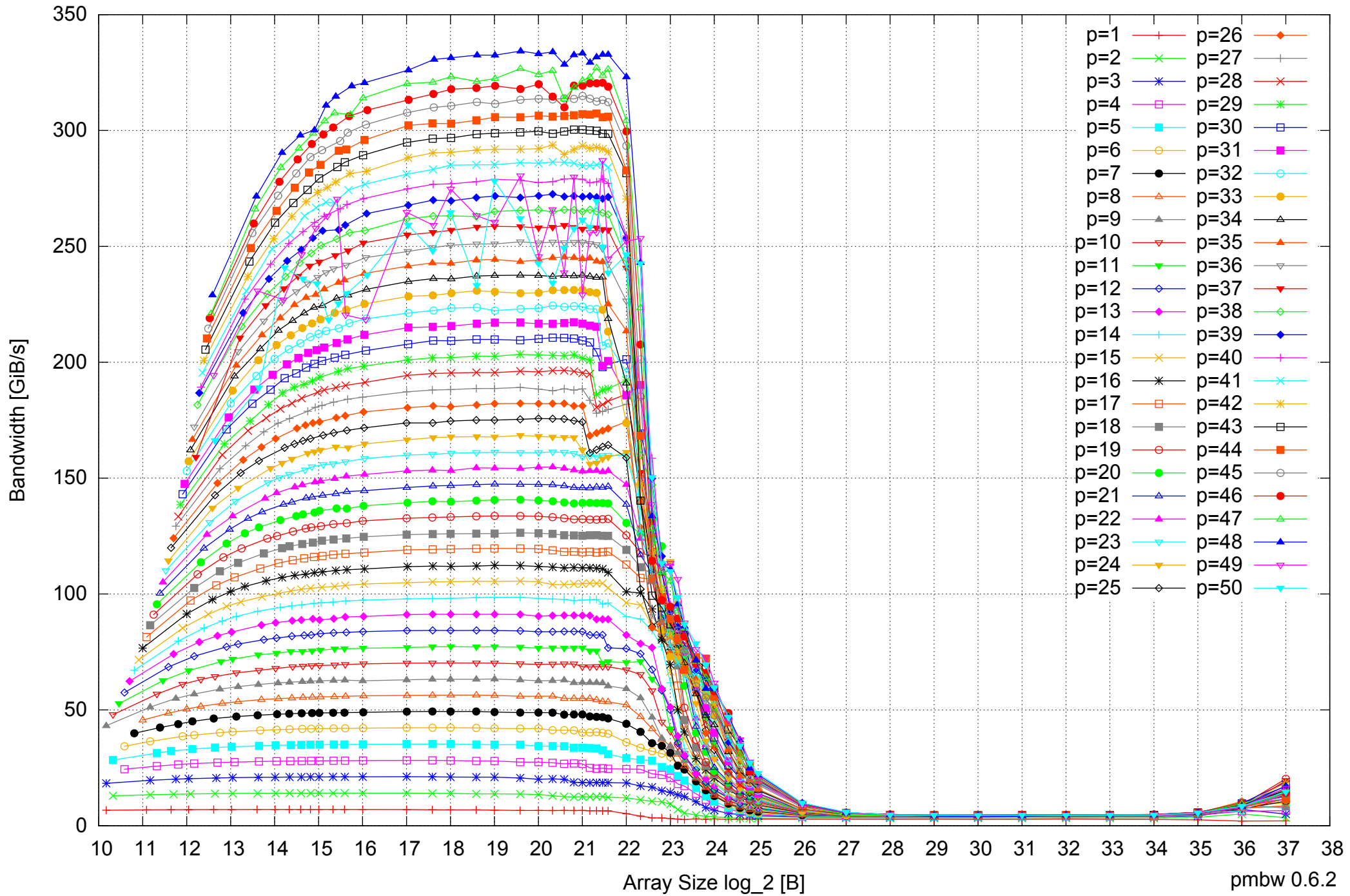
AMD Opteron 6168 256GB - Parallel Memory Bandwidth - ScanWrite64IndexSimpleLoop
