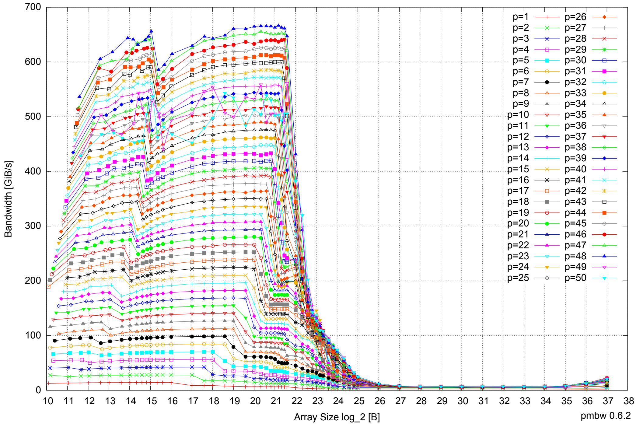
AMD Opteron 6168 256GB - Parallel Memory Bandwidth - ScanRead32PtrUnrollLoop
