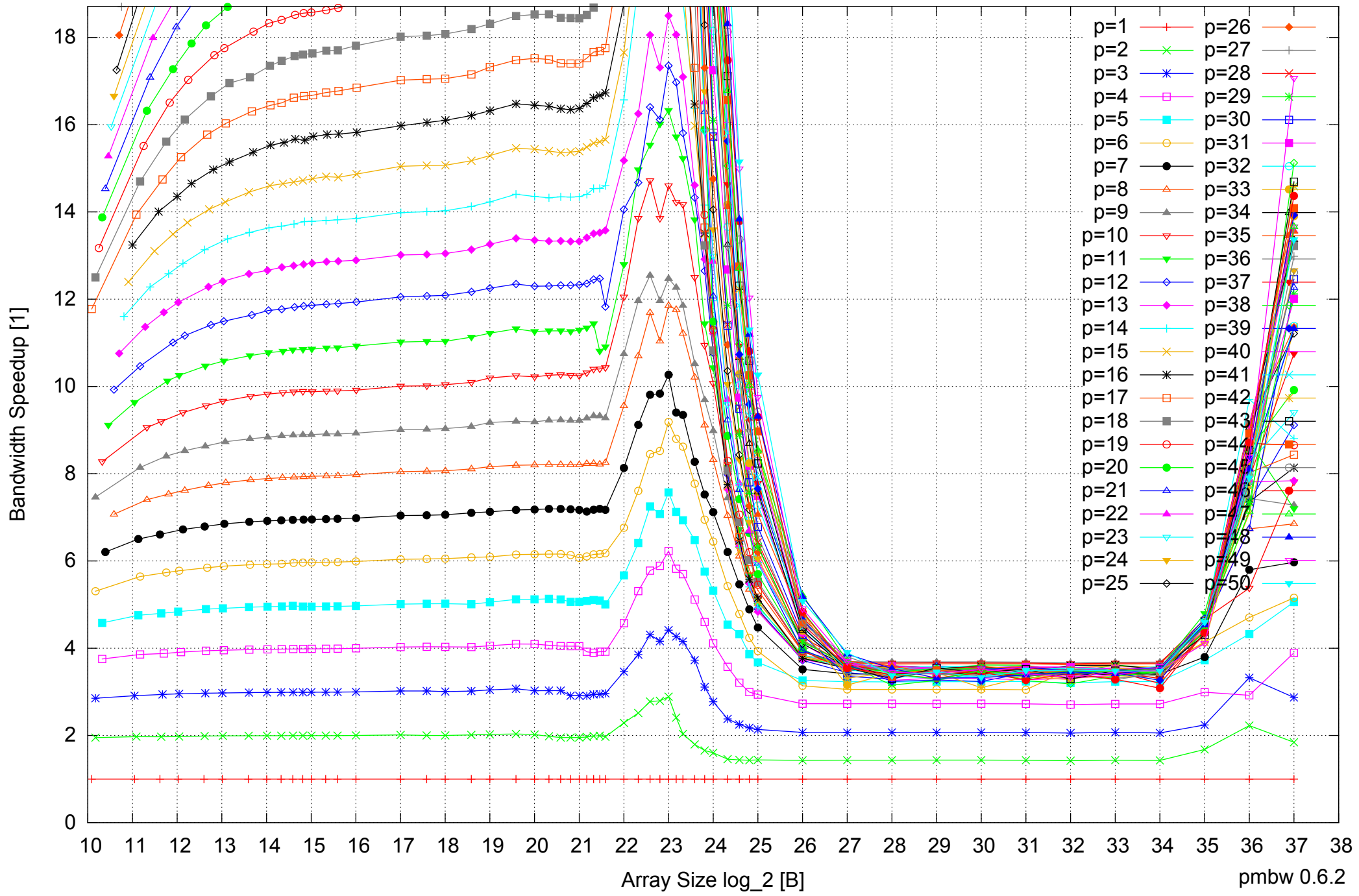
AMD Opteron 6168 256GB - Speedup of Parallel Memory Bandwidth (enlarged) - ScanRead32PtrSimpleLoop
