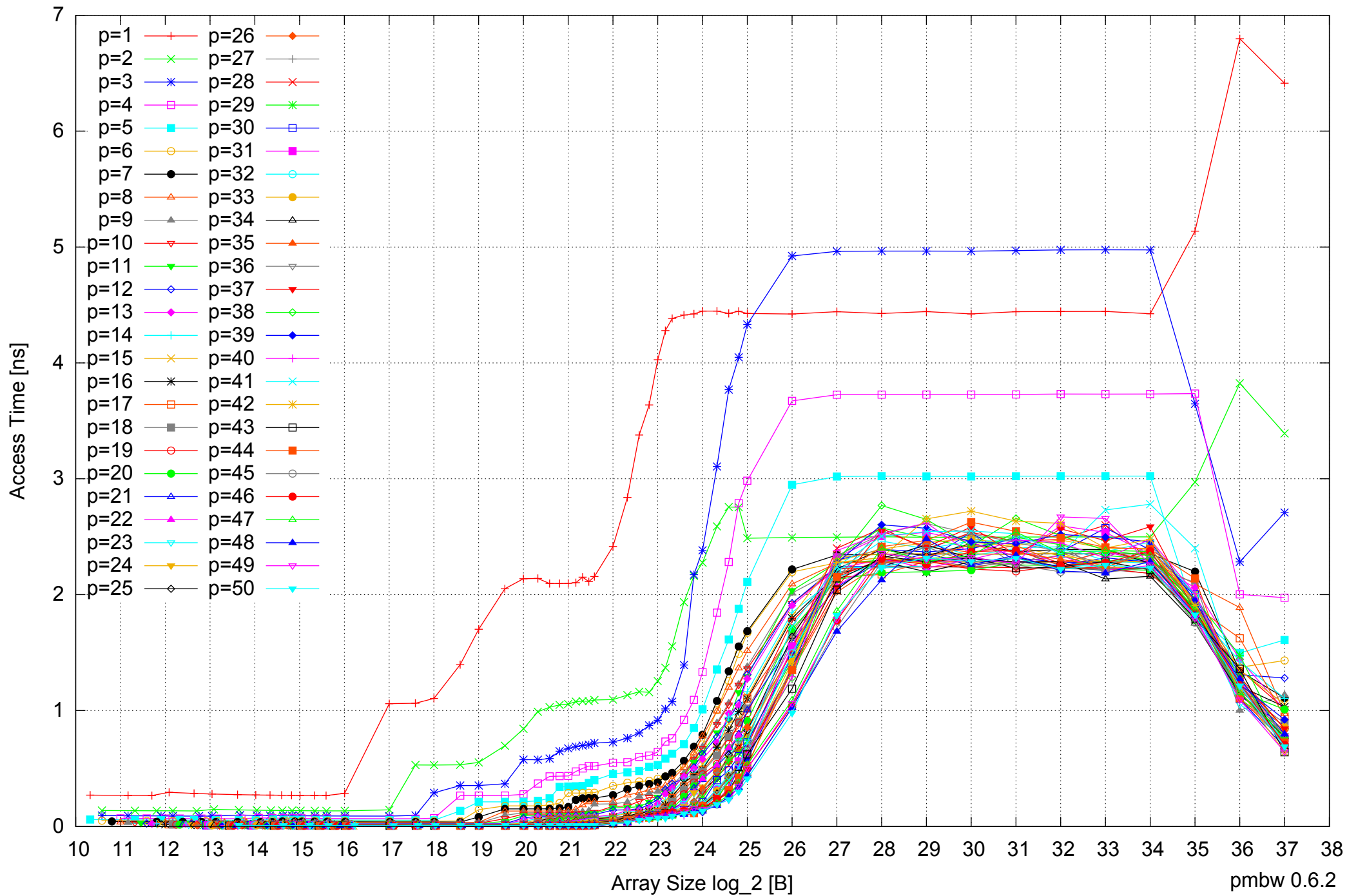
AMD Opteron 6168 256GB - Parallel Memory Access Time - ScanRead128PtrUnrollLoop
