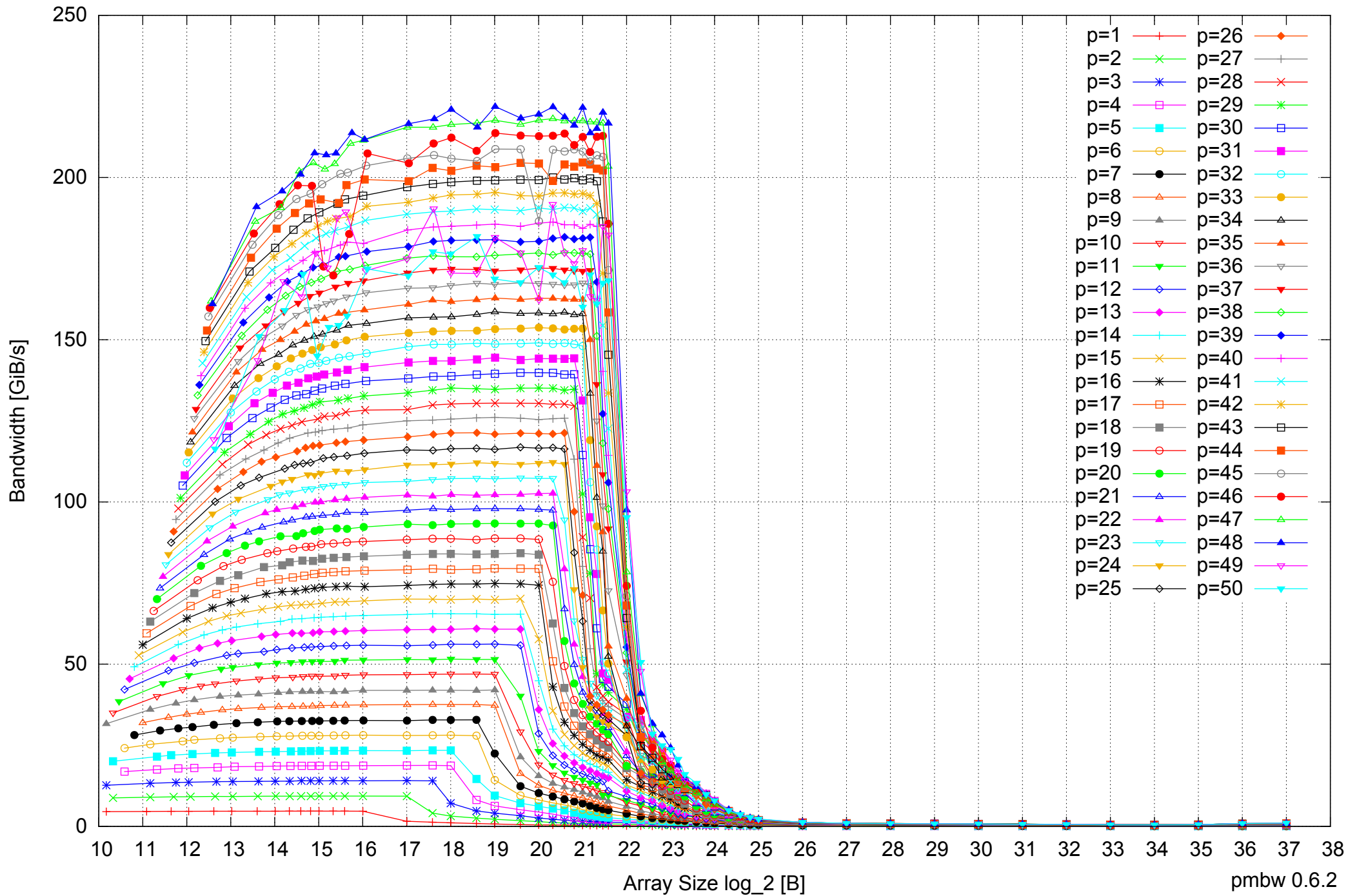
AMD Opteron 6168 256GB - Parallel Memory Bandwidth - PermRead64SimpleLoop
