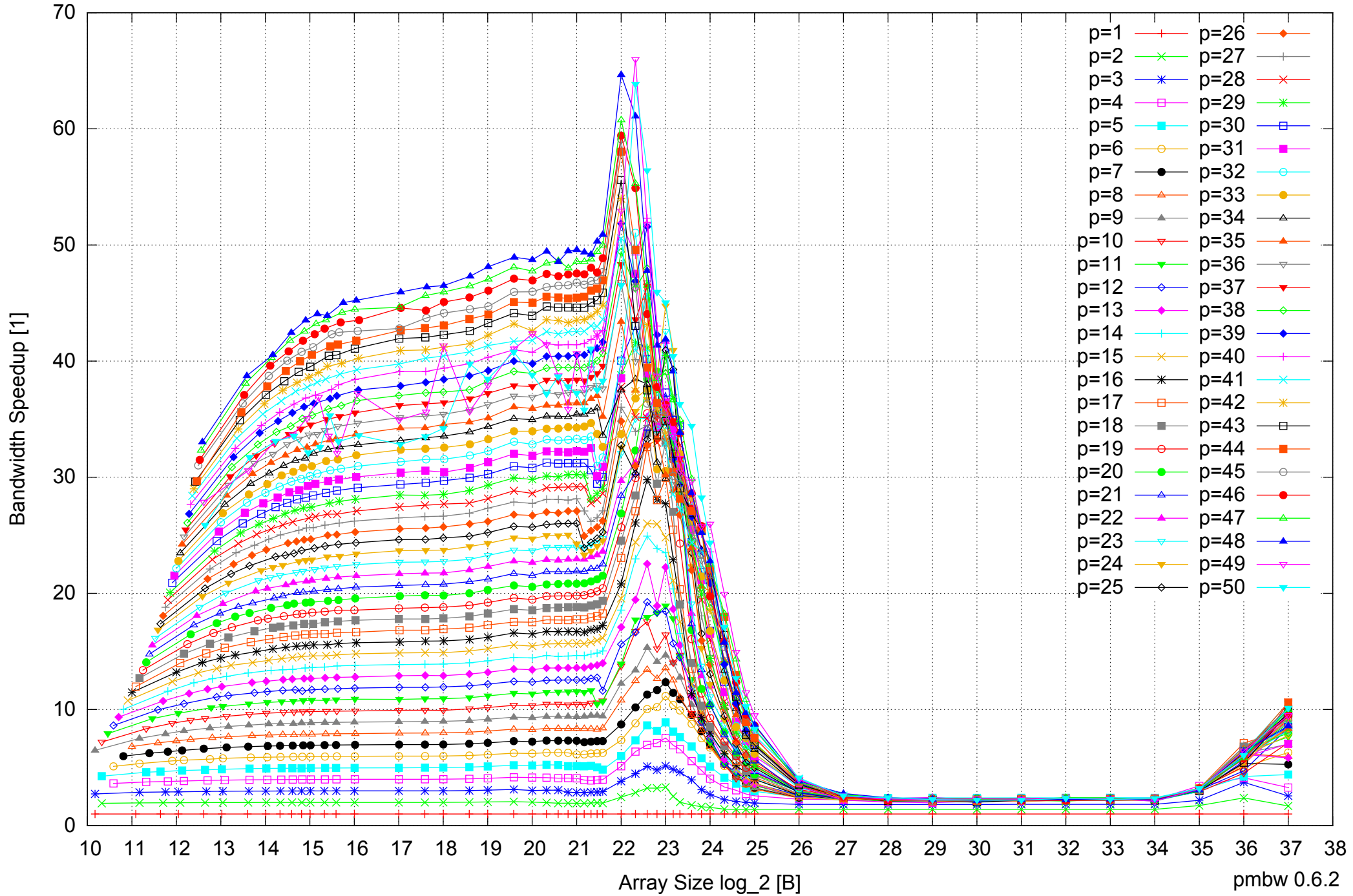
AMD Opteron 6168 256GB - Speedup of Parallel Memory Bandwidth - ScanRead64IndexSimpleLoop
