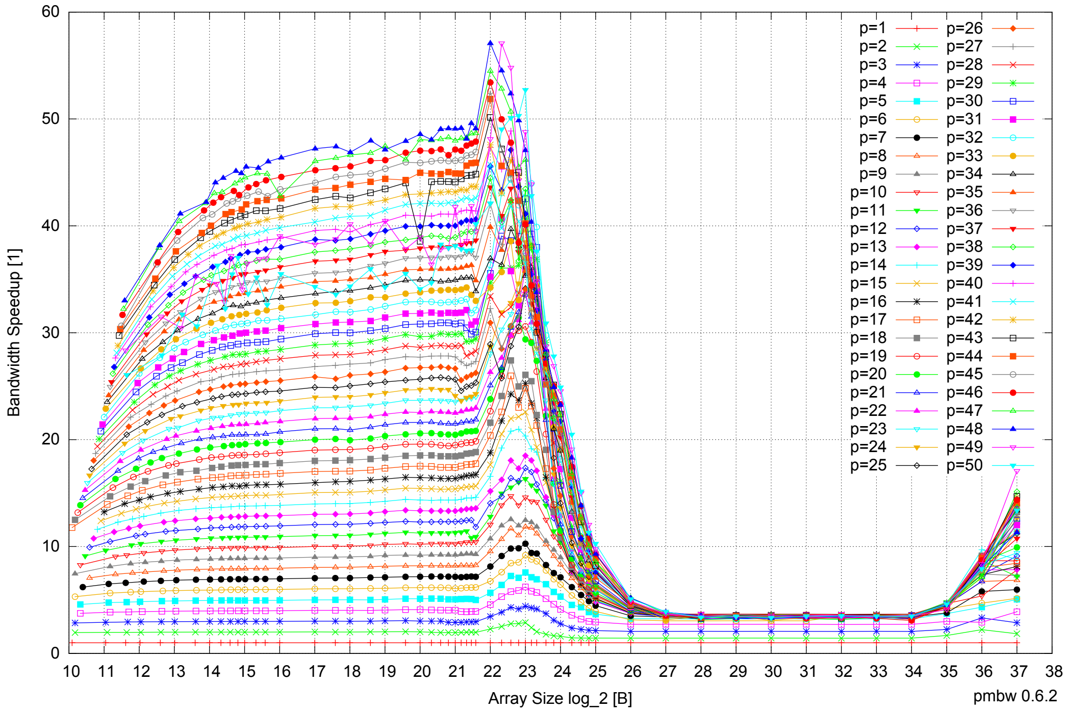
AMD Opteron 6168 256GB - Speedup of Parallel Memory Bandwidth - ScanRead32PtrSimpleLoop
