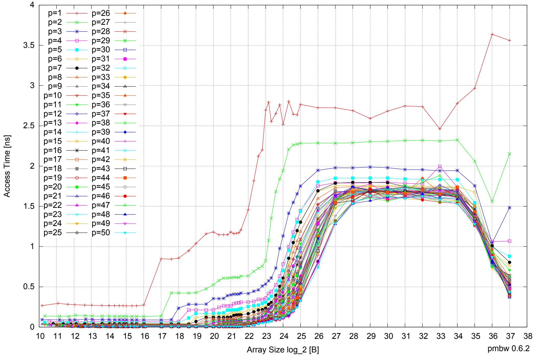
AMD Opteron 6168 256GB - Parallel Memory Access Time - ScanWrite64PtrUnrollLoop
