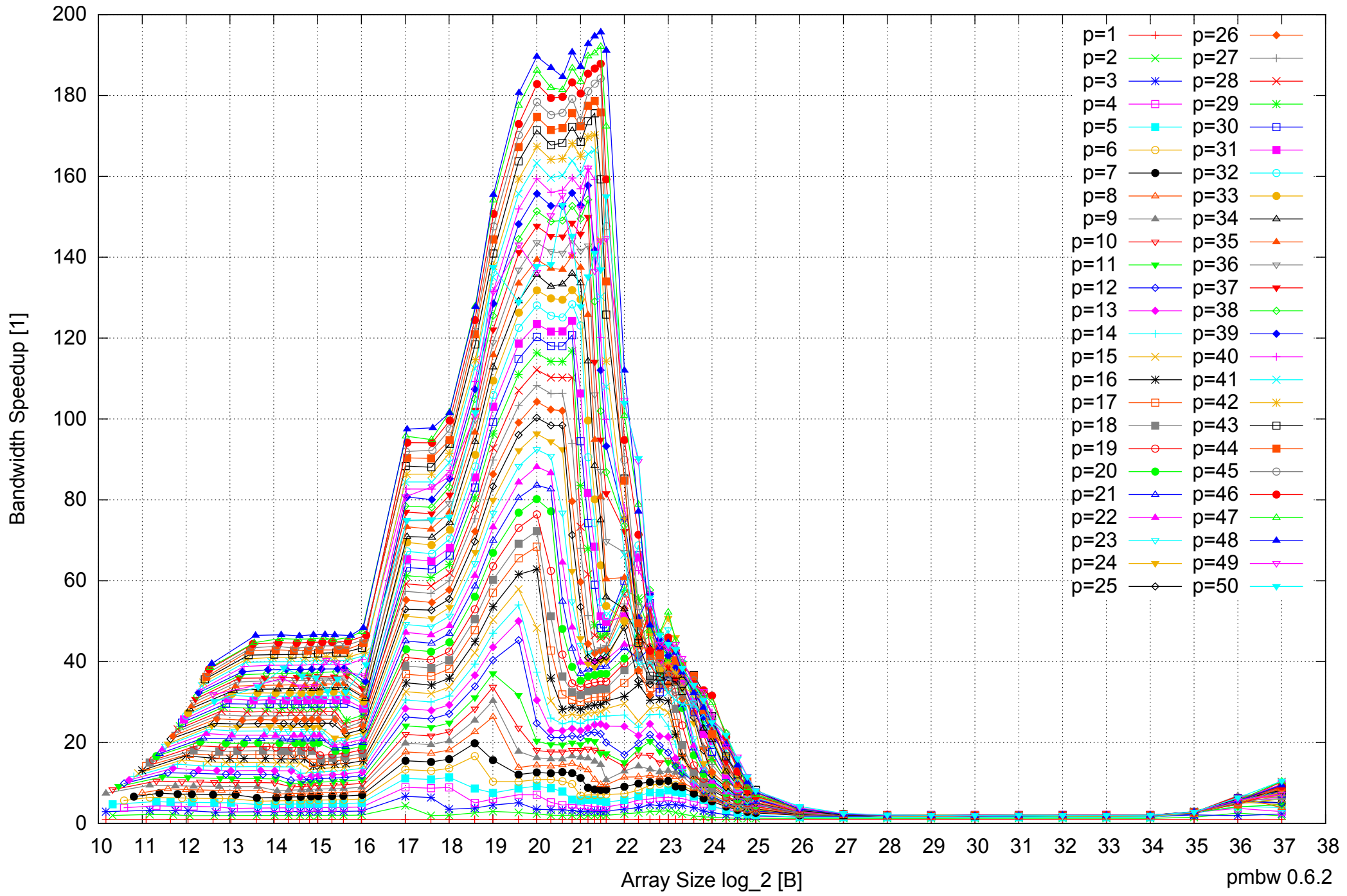
AMD Opteron 6168 256GB - Speedup of Parallel Memory Bandwidth - ScanRead64PtrUnrollLoop
