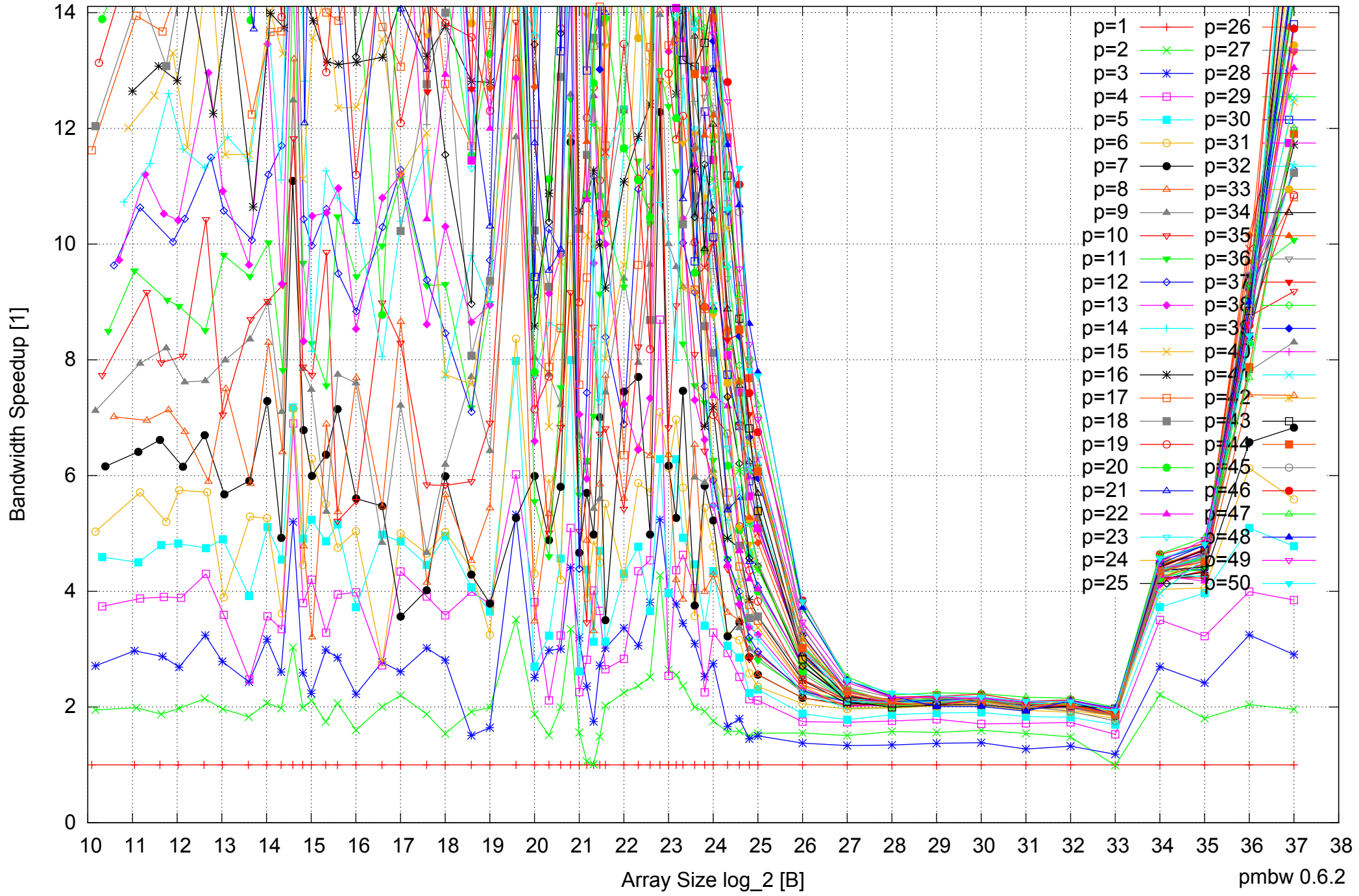
AMD Opteron 6168 256GB - Speedup of Parallel Memory Bandwidth (enlarged) - ScanWrite32PtrSimpleLoop
