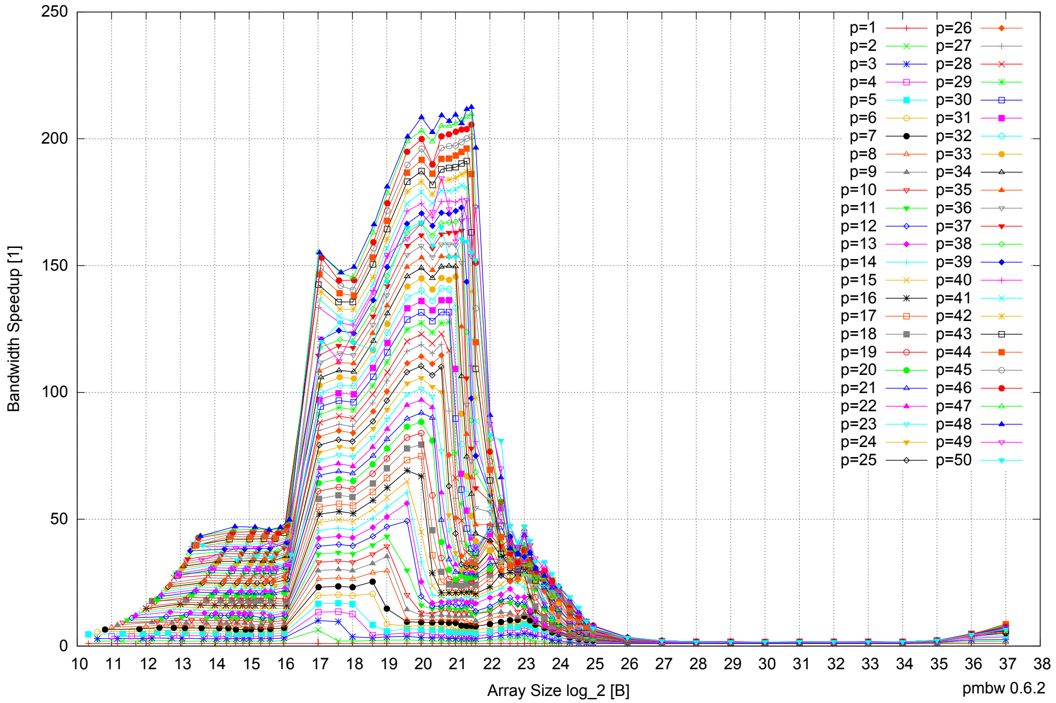
AMD Opteron 6168 256GB - Speedup of Parallel Memory Bandwidth - ScanWrite128PtrUnrollLoop
