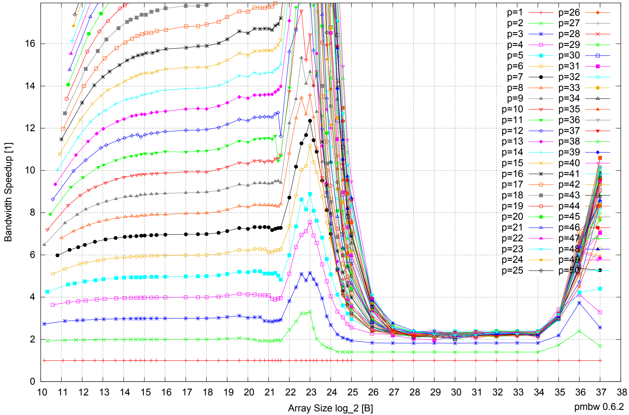
AMD Opteron 6168 256GB - Speedup of Parallel Memory Bandwidth (enlarged) - ScanRead64IndexSimpleLoop
