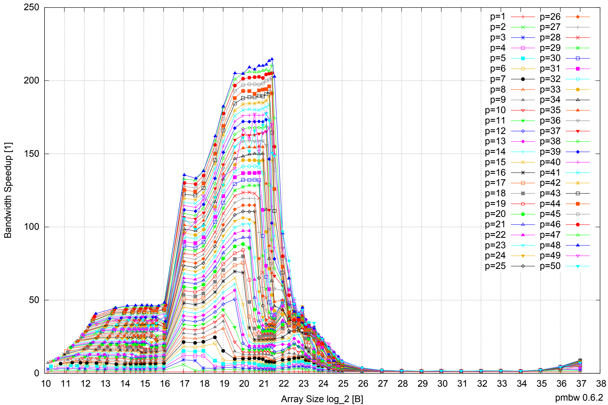
AMD Opteron 6168 256GB - Speedup of Parallel Memory Bandwidth - ScanWrite64IndexUnrollLoop
