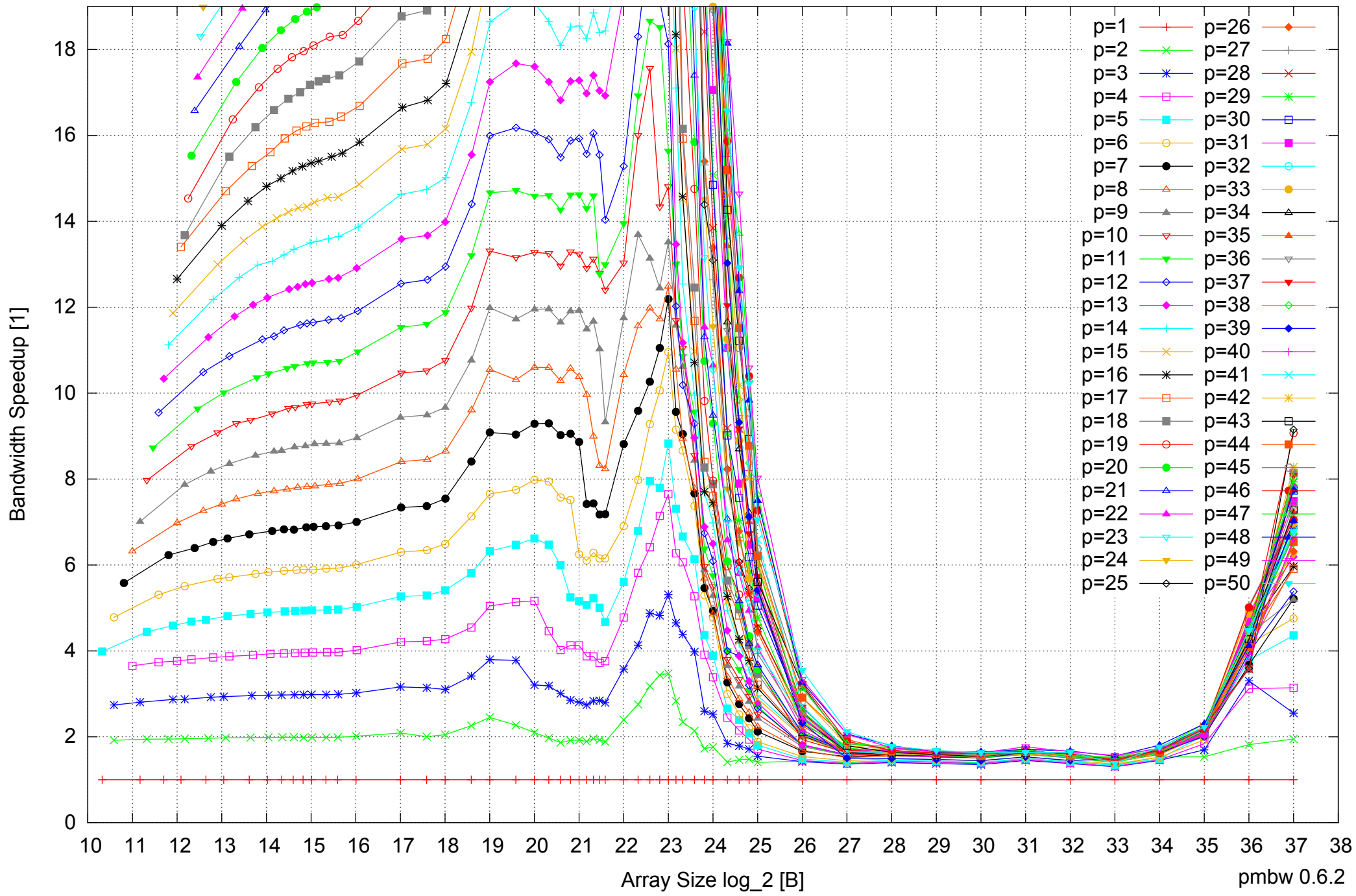
AMD Opteron 6168 256GB - Speedup of Parallel Memory Bandwidth (enlarged) - ScanWrite128PtrSimpleLoop
