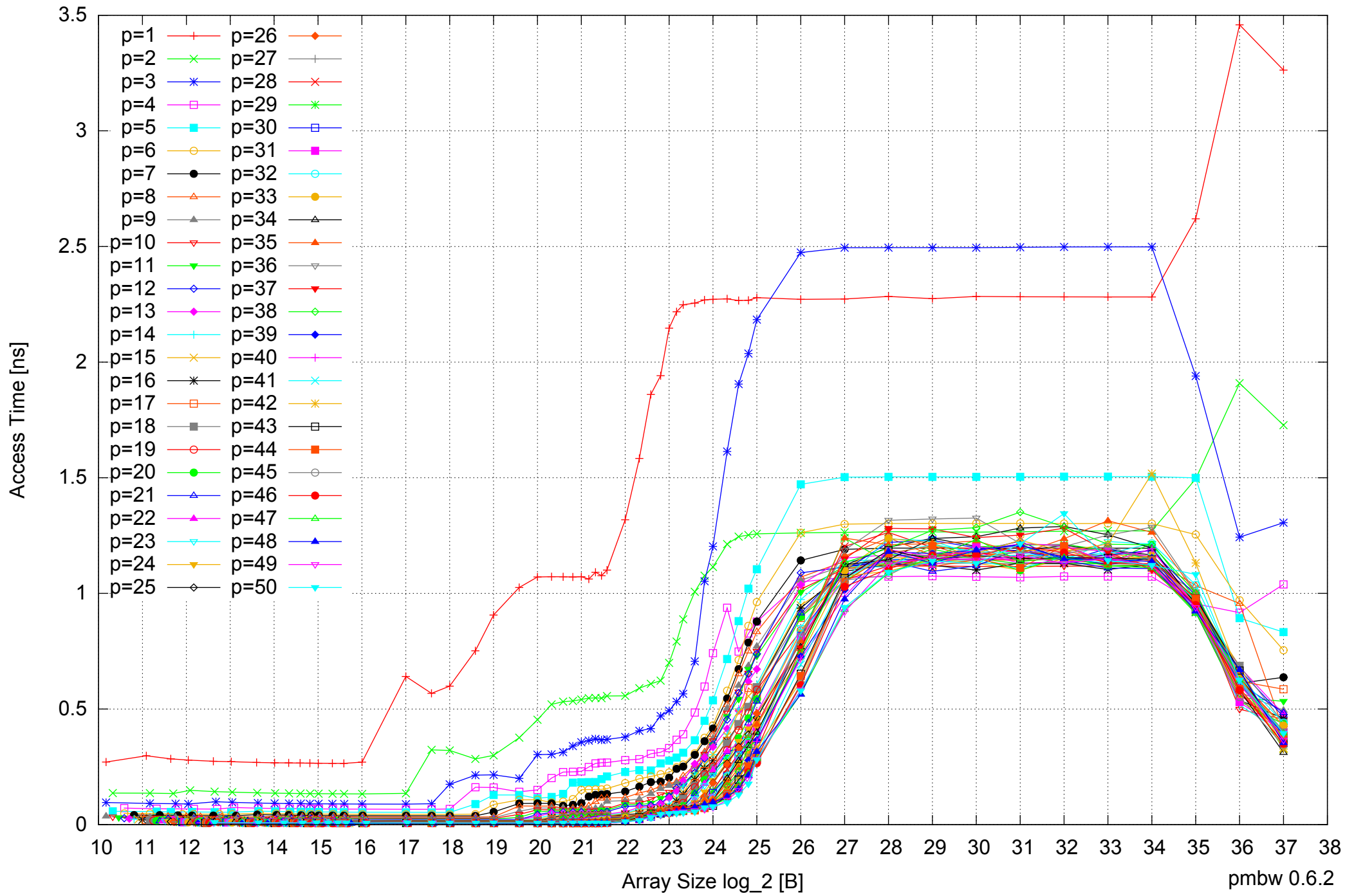
AMD Optreron 6168 256GB - Parallel Memory Access Time - ScanRead64IndexUnrollLoop
