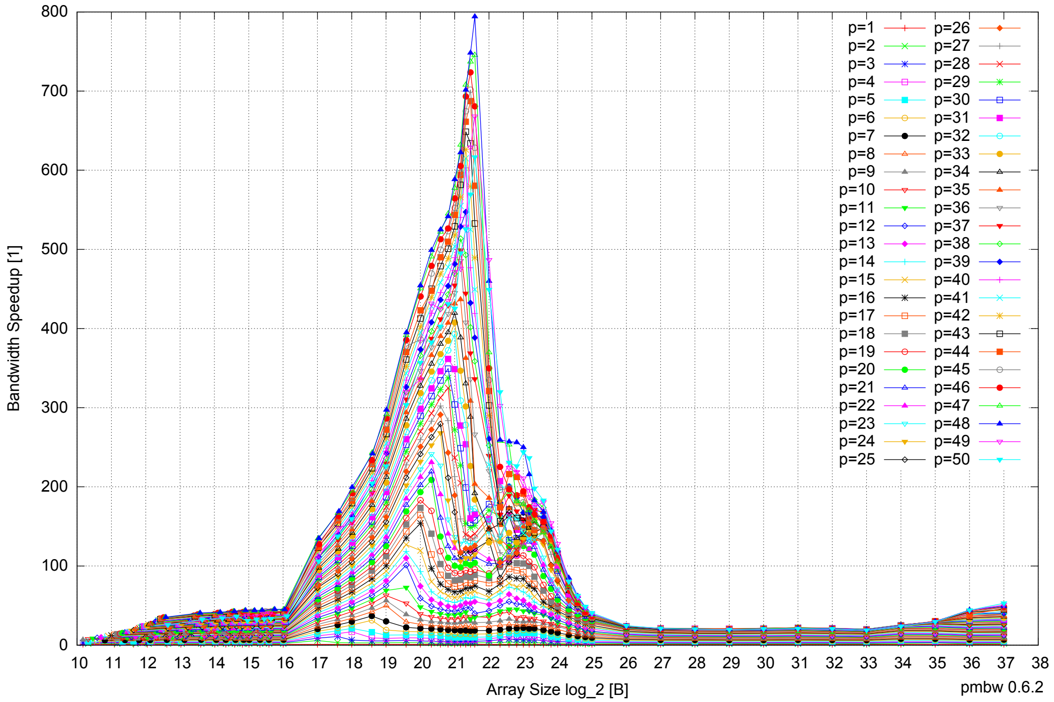
AMD Opteron 6168 256GB - Speedup of Parallel Memory Bandwidth - PermRead64SimpleLoop
