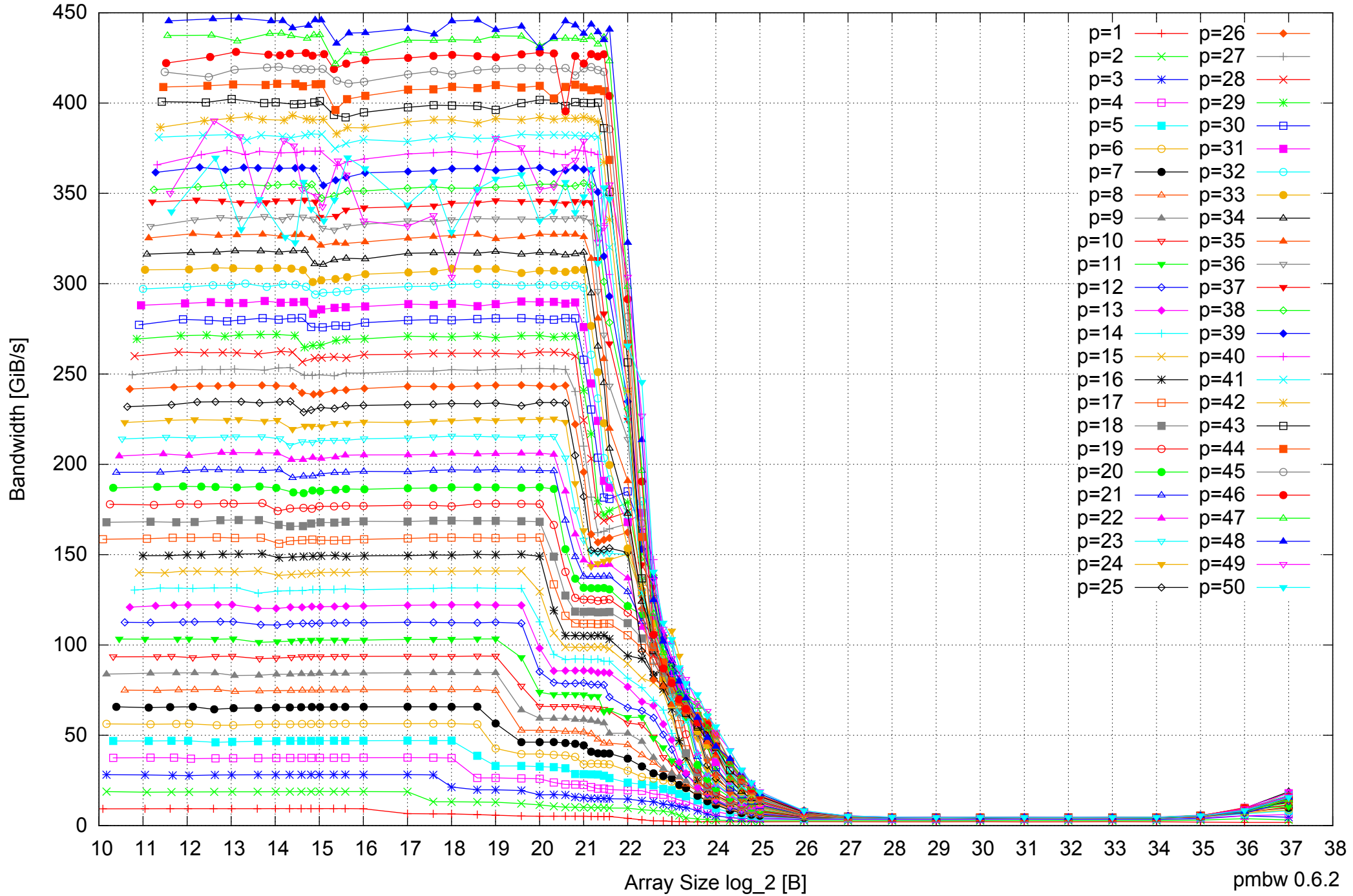
AMD Opteron 6168 256GB - Parallel Memory Bandwidth - ScanWrite32PtrUnrollLoop
