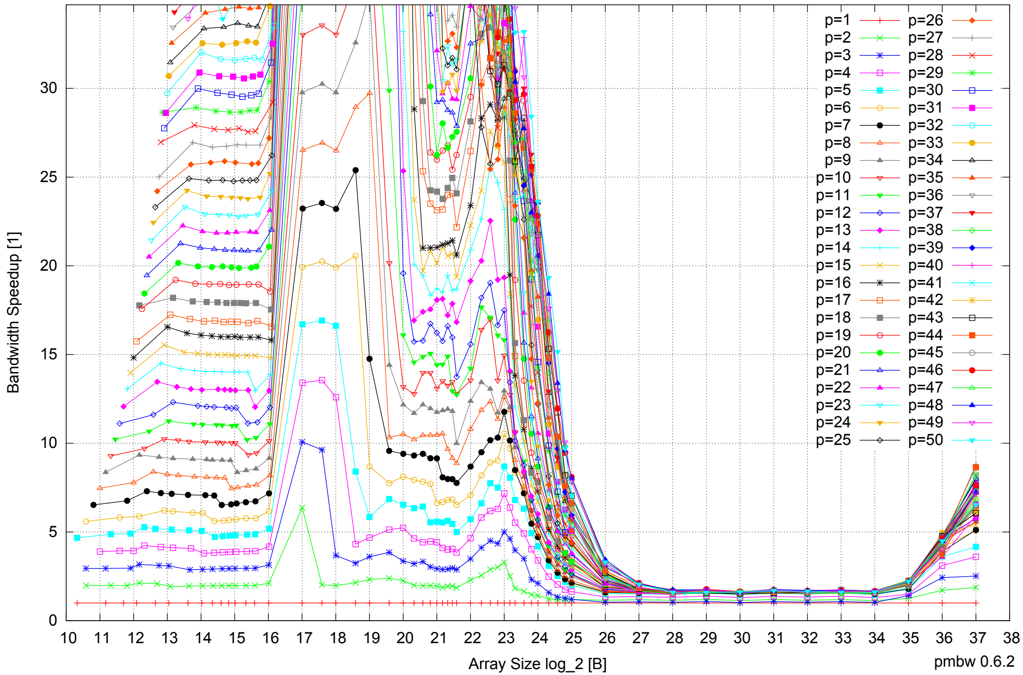
AMD Opteron 6168 256GB - Speedup of Parallel Memory Bandwidth (enlarged) - ScanWrite128PtrUnrollLoop
