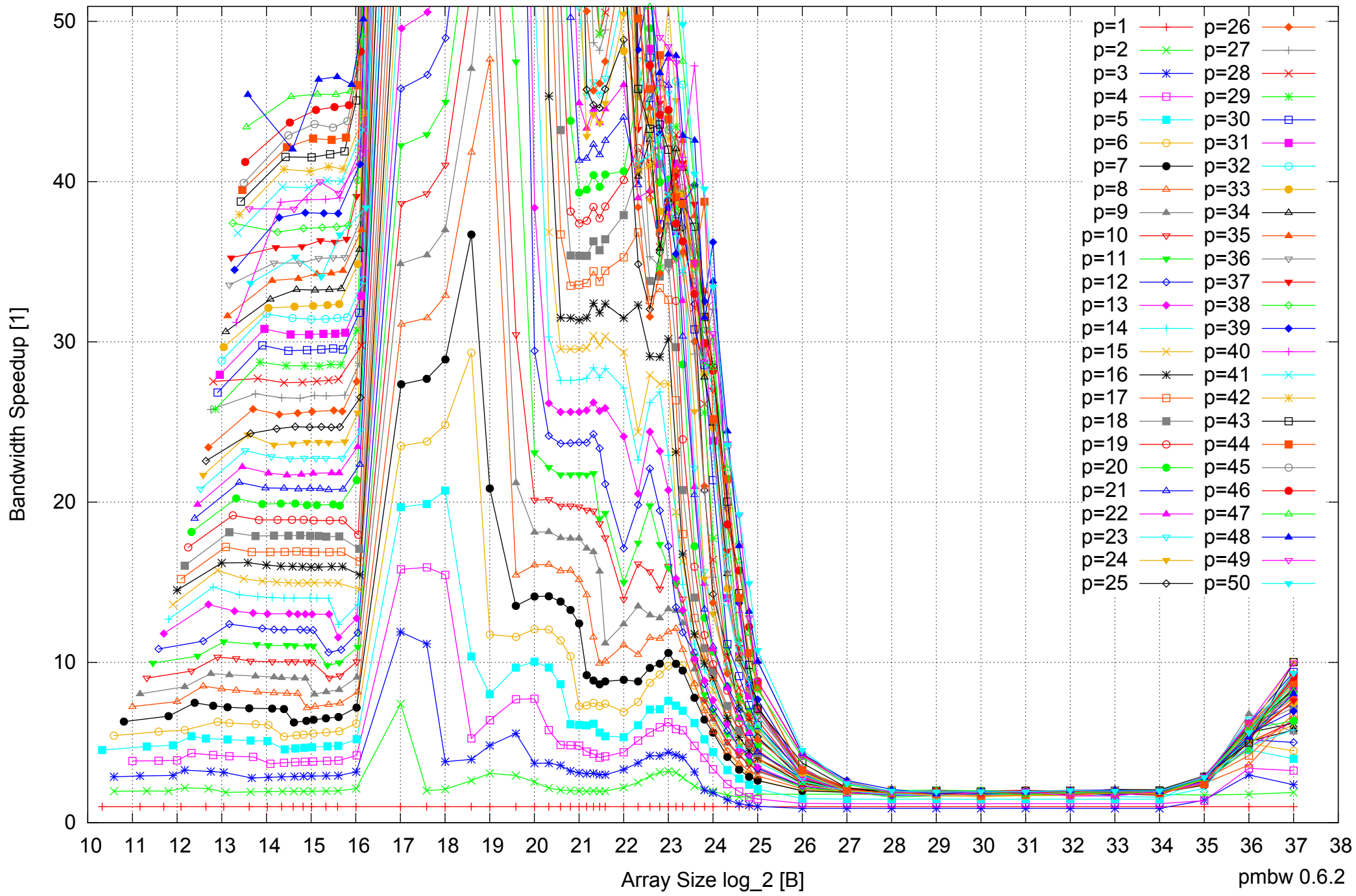
AMD Opteron 6168 256GB - Speedup of Parallel Memory Bandwidth (enlarged) - ScanRead128PtrUnrollLoop
