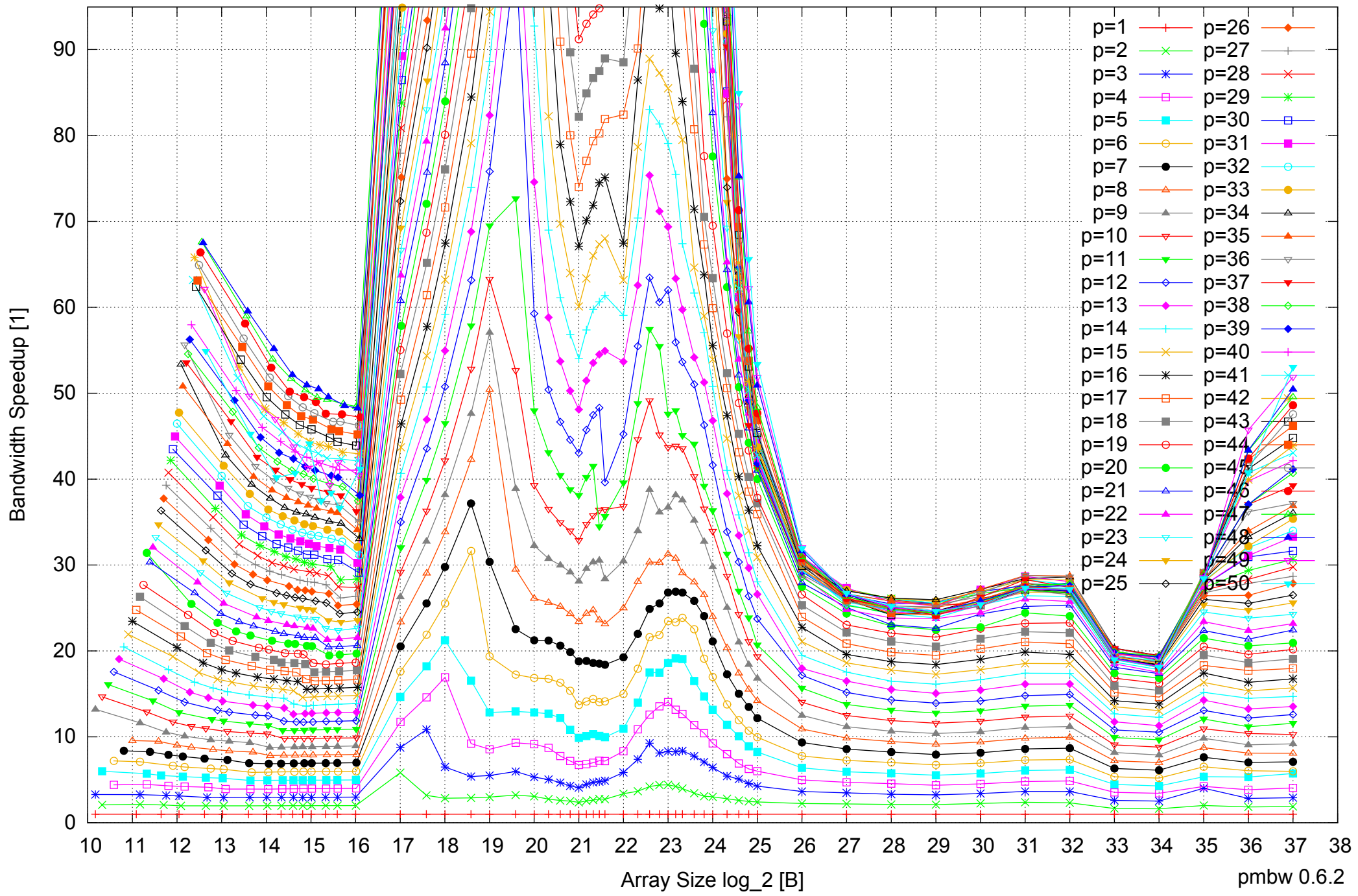
AMD Opteron 6168 256GB - Speedup of Parallel Memory Bandwidth (enlarged) - PermRead64UnrollLoop
