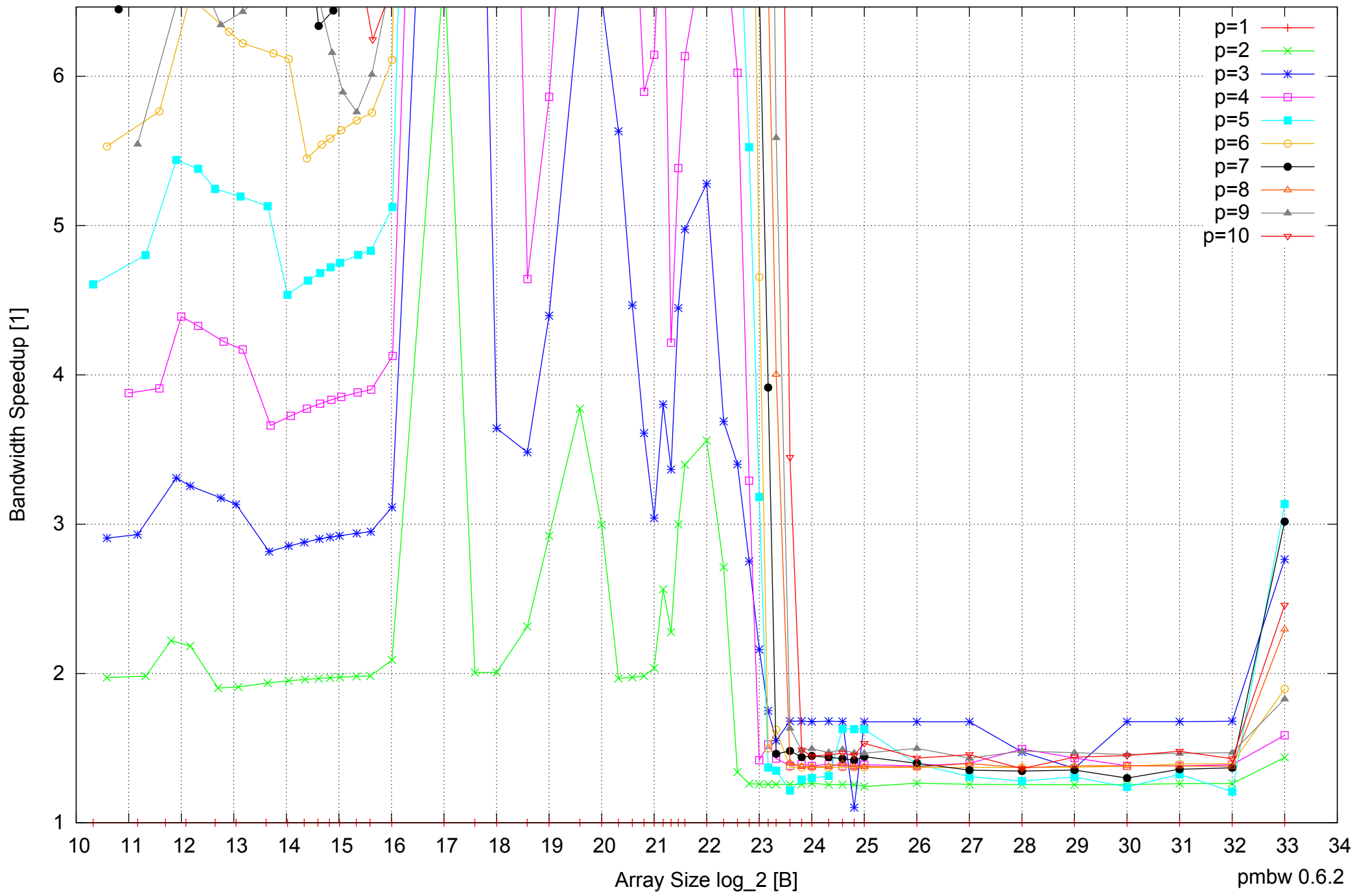
AMD Opteron 2350 16GB - Speedup of Parallel Memory Bandwidth (enlarged) - ScanRead128PtrUnrollLoop
