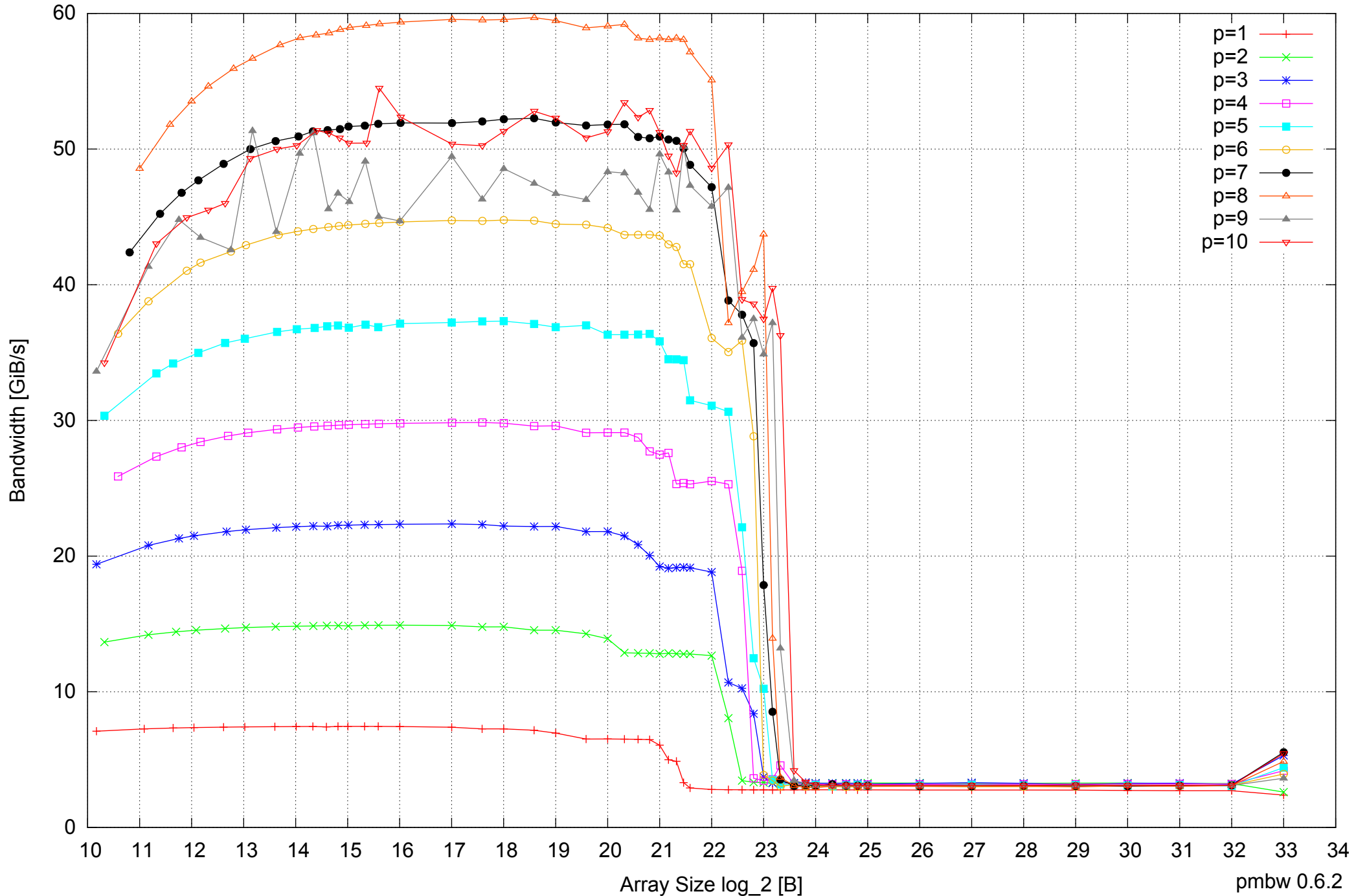
AMD Opteron 2350 16GB - Parallel Memory Bandwidth - ScanWrite64IndexSimpleLoop
