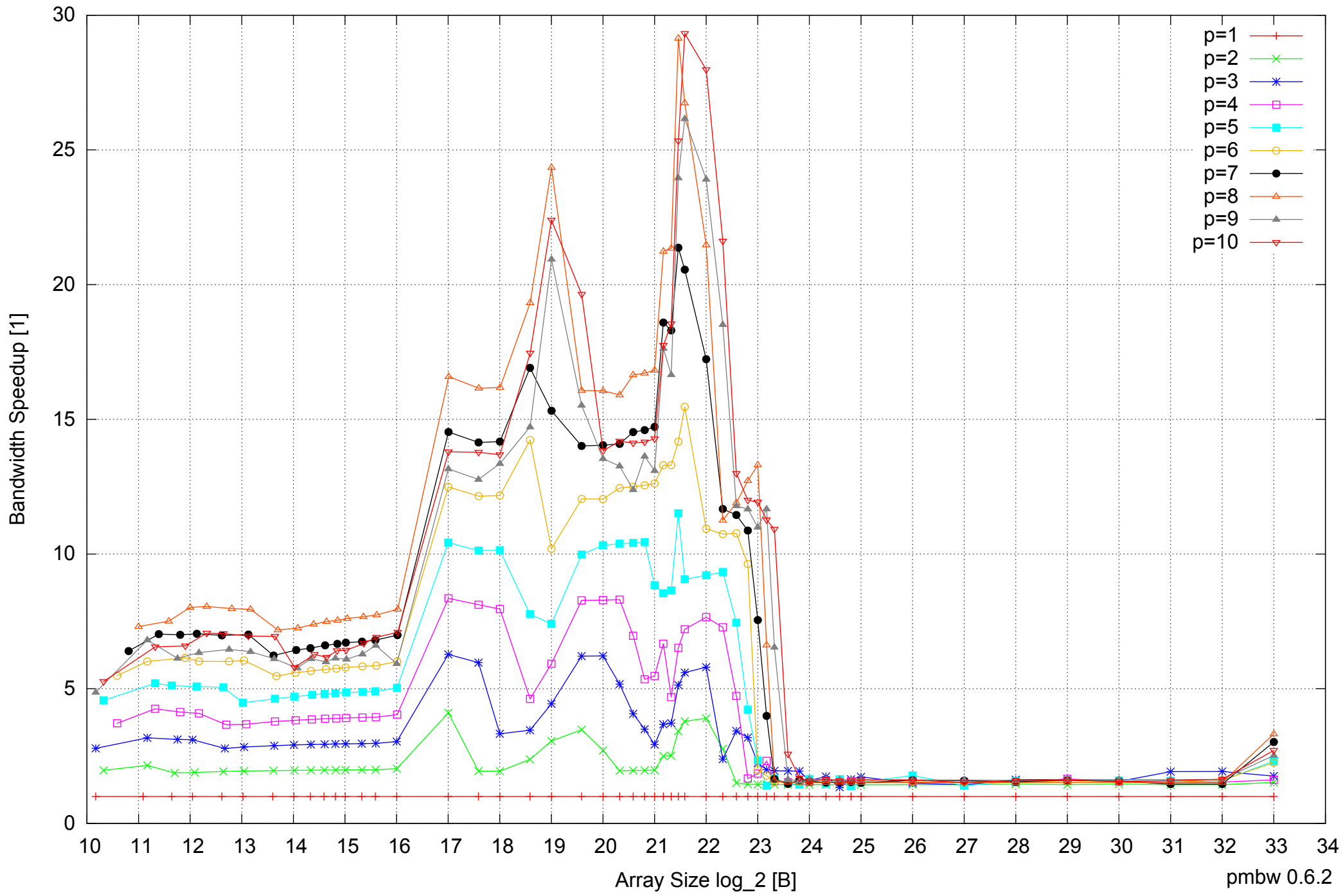
AMD Opteron 2350 16GB - Speedup of Parallel Memory Bandwidth - ScanRead64IndexUnrollLoop
