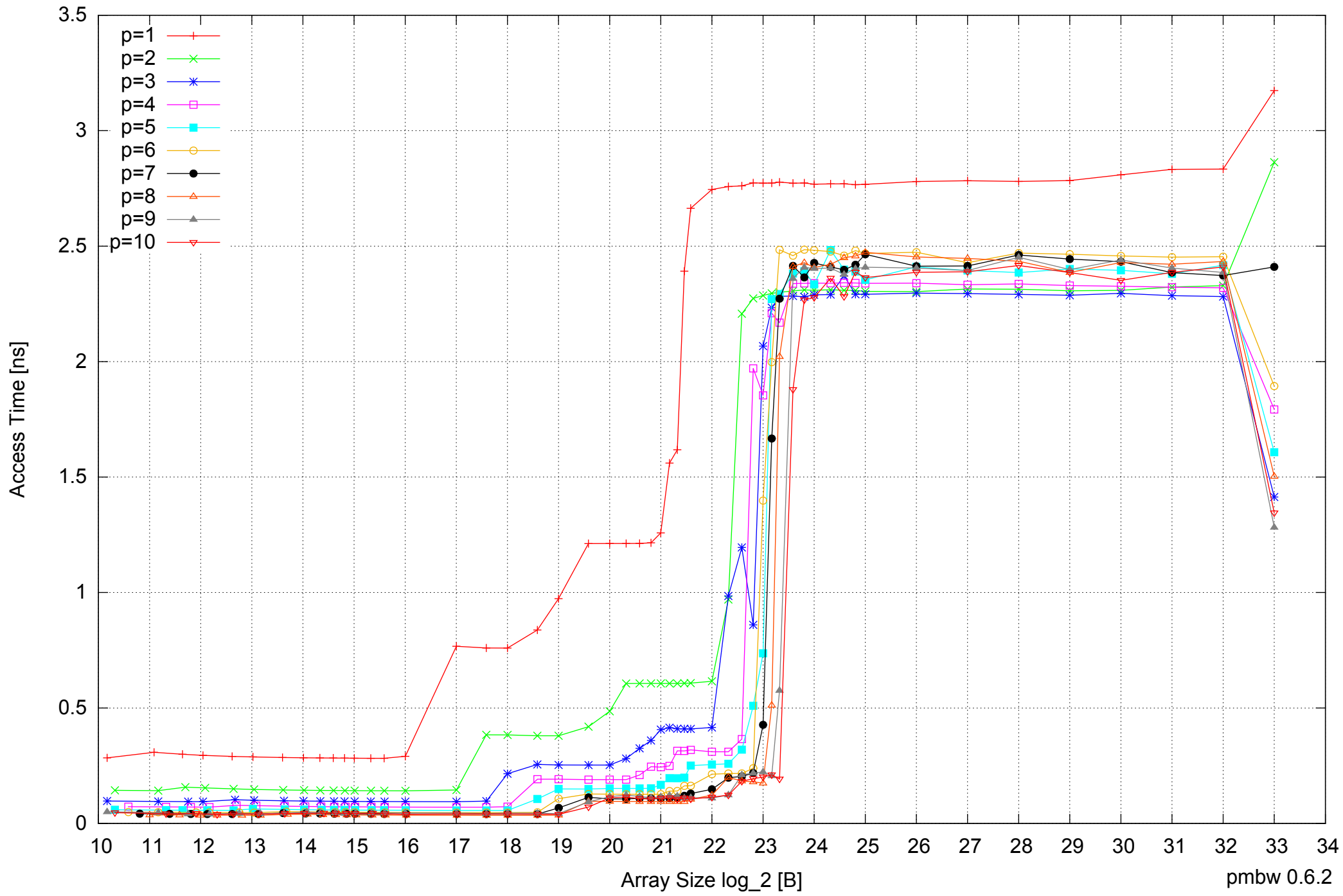
AMD Opteron 2350 16GB - Parallel Memory Access Time - ScanWrite64IndexUnrollLoop
