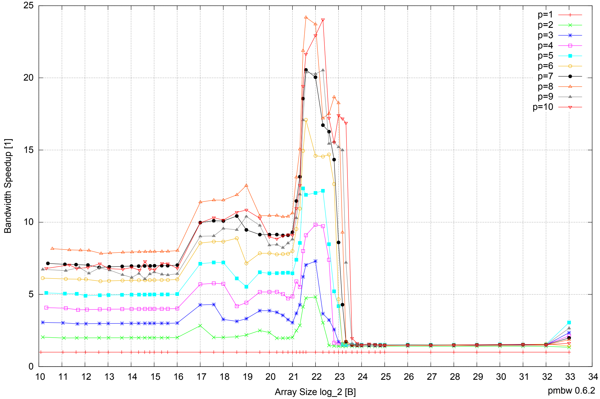
AMD Opteron 2350 16GB - Speedup of Parallel Memory Bandwidth - ScanWrite32PtrUnrollLoop
