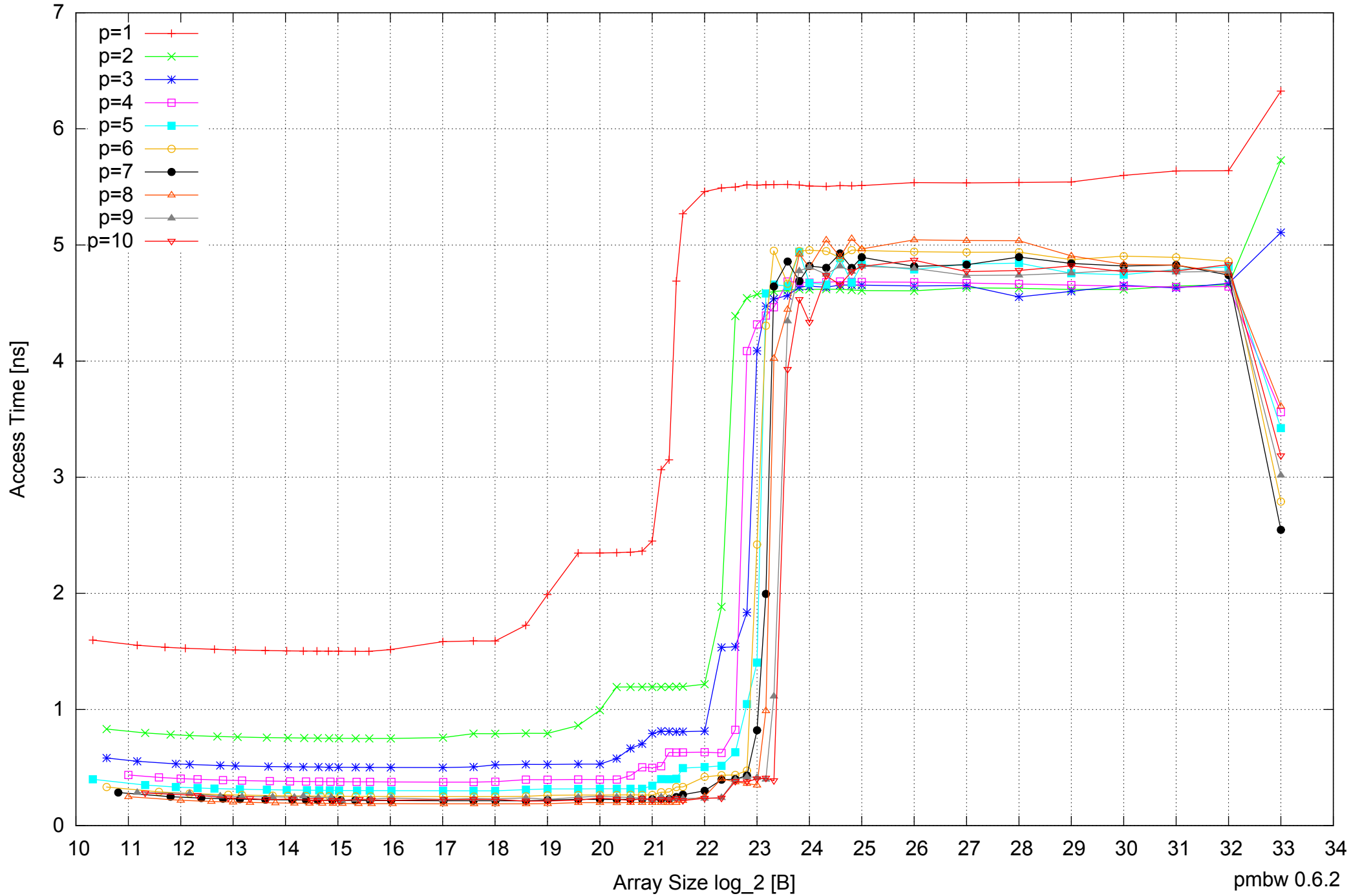
AMD Opteron 2350 16GB - Parallel Memory Access Time - ScanWrite128PtrSimpleLoop
