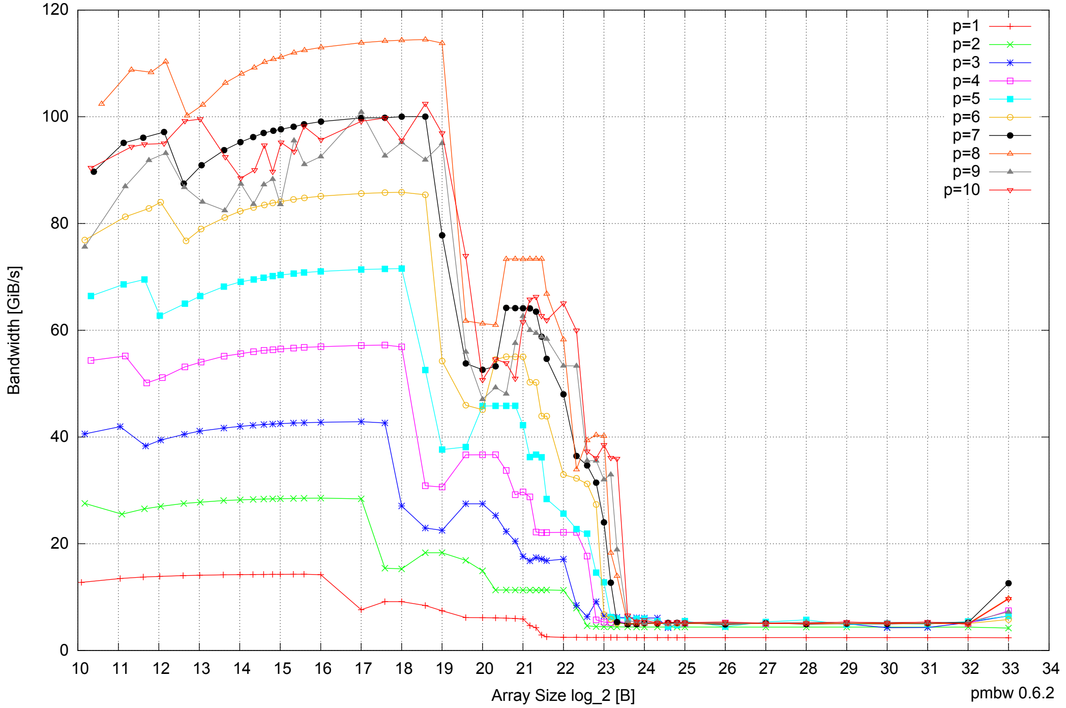
AMD Opteron 2350 16GB - Parallel Memory Bandwidth - ScanRead32PtrUnrollLoop
