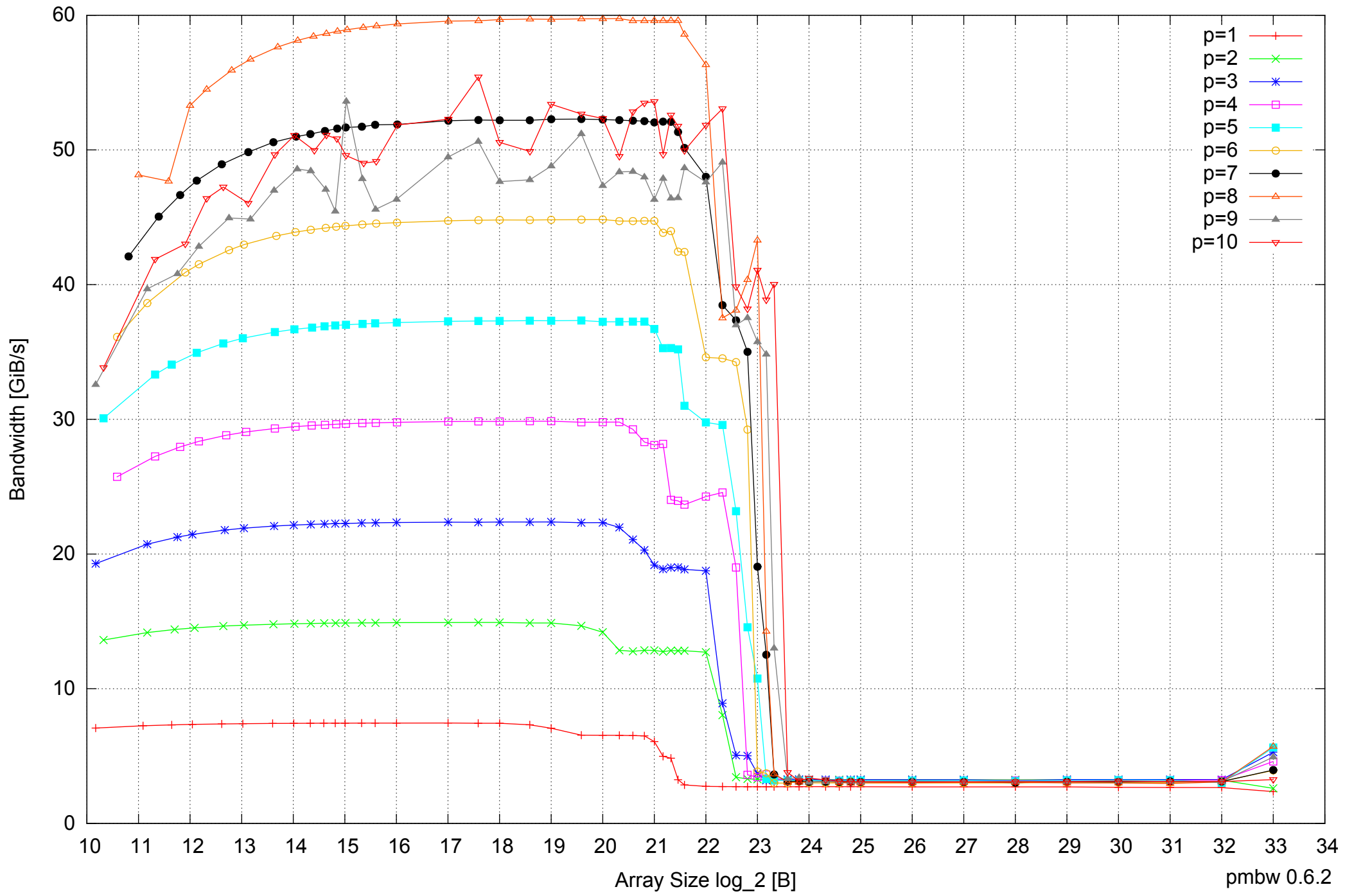
AMD Opteron 2350 16GB - Parallel Memory Bandwidth - ScanWrite64PtrSimpleLoop
