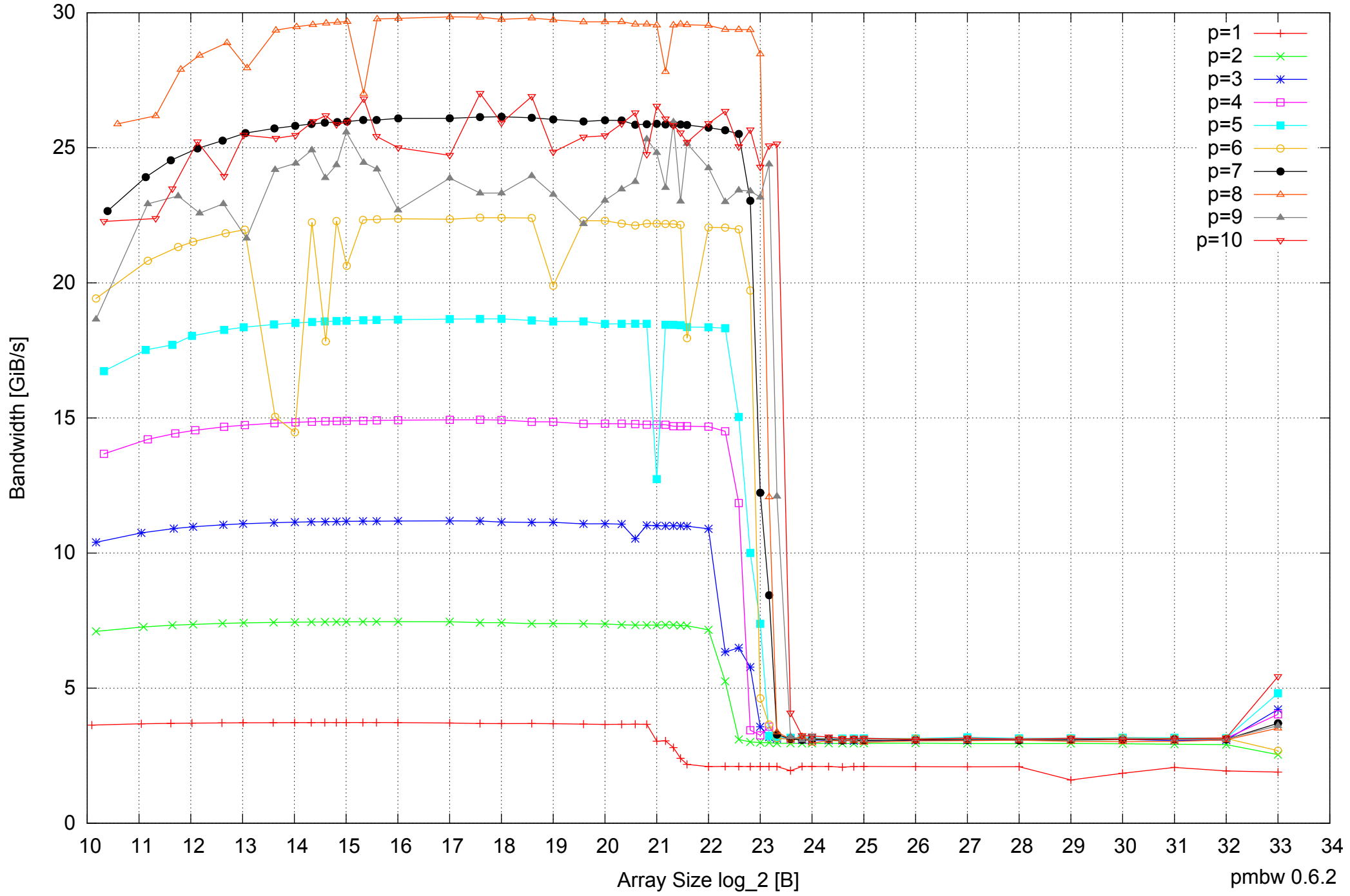
AMD Opteron 2350 16GB - Parallel Memory Bandwidth - ScanWrite32PtrSimpleLoop
