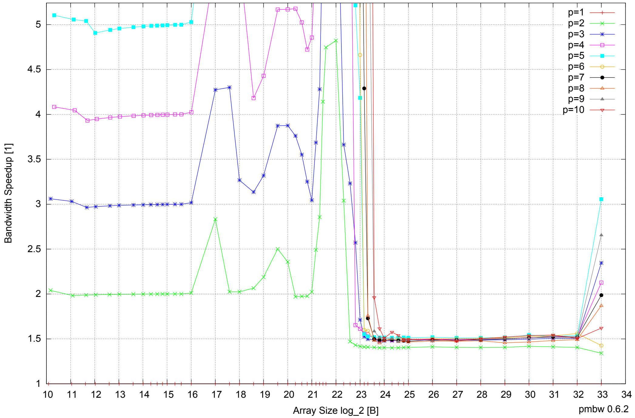
AMD Opteron 2350 16GB - Speedup of Parallel Memory Bandwidth (enlarged) - ScanWrite32PtrUnrollLoop
