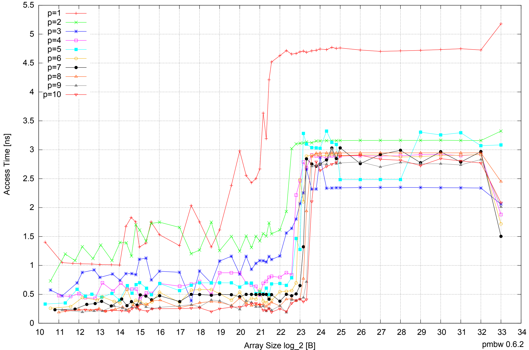
AMD Opteron 2350 16GB - Parallel Memory Access Time - ScanRead128PtrSimpleLoop
