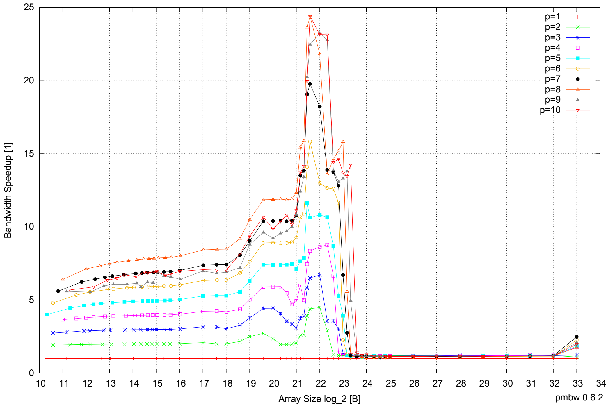
AMD Opteron 2350 16GB - Speedup of Parallel Memory Bandwidth - ScanWrite128PtrSimpleLoop
