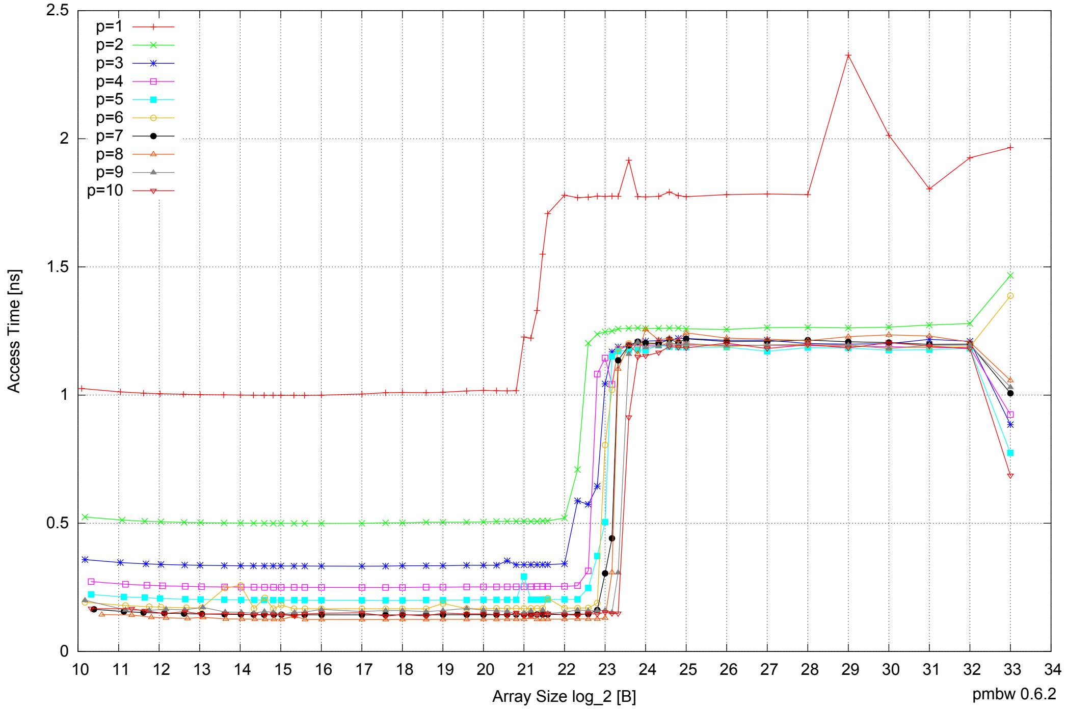
AMD Opteron 2350 16GB - Parallel Memory Access Time - ScanWrite32PtrSimpleLoop
