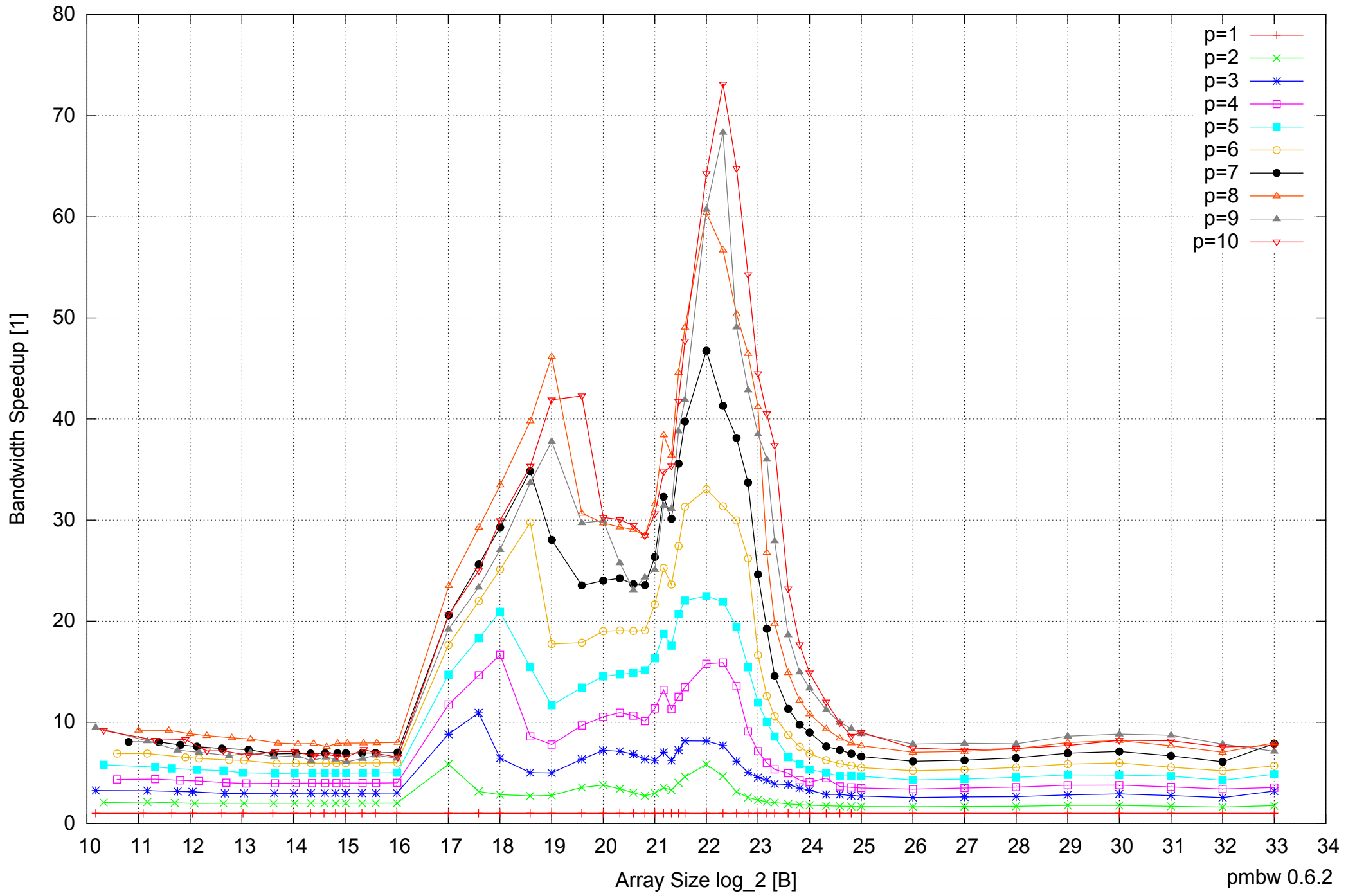
AMD Opteron 2350 16GB - Speedup of Parallel Memory Bandwidth - PermRead64UnrollLoop
