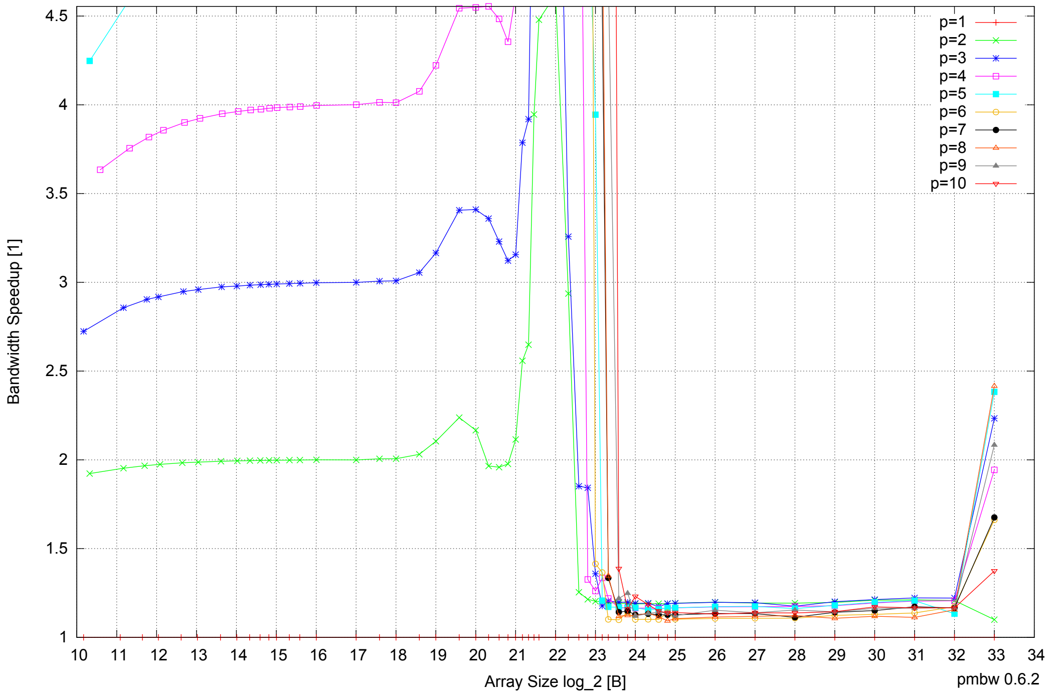
AMD Opteron 2350 16GB - Speedup of Parallel Memory Bandwidth (enlarged) - ScanWrite64PtrSimpleLoop
