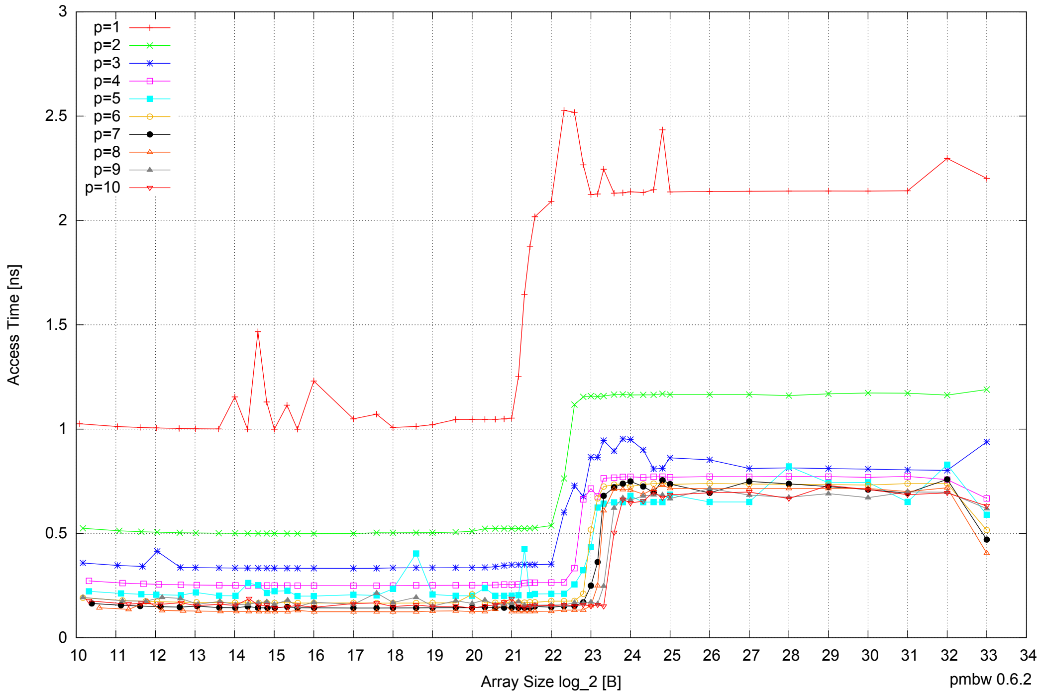
AMD Opteron 2350 16GB - Parallel Memory Access Time - ScanRead32PtrSimpleLoop
