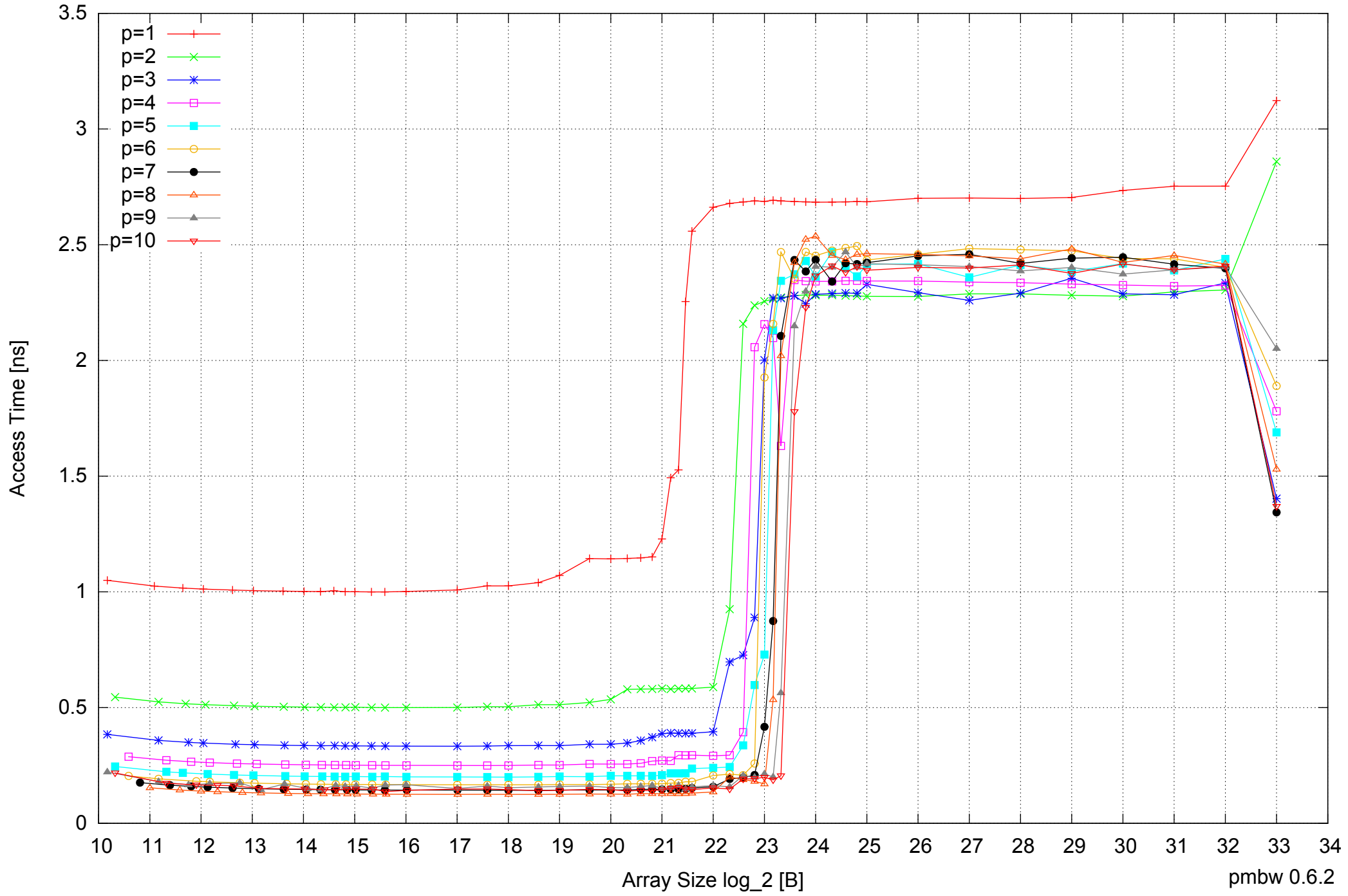
AMD Opteron 2350 16GB - Parallel Memory Access Time - ScanWrite64IndexSimpleLoop
