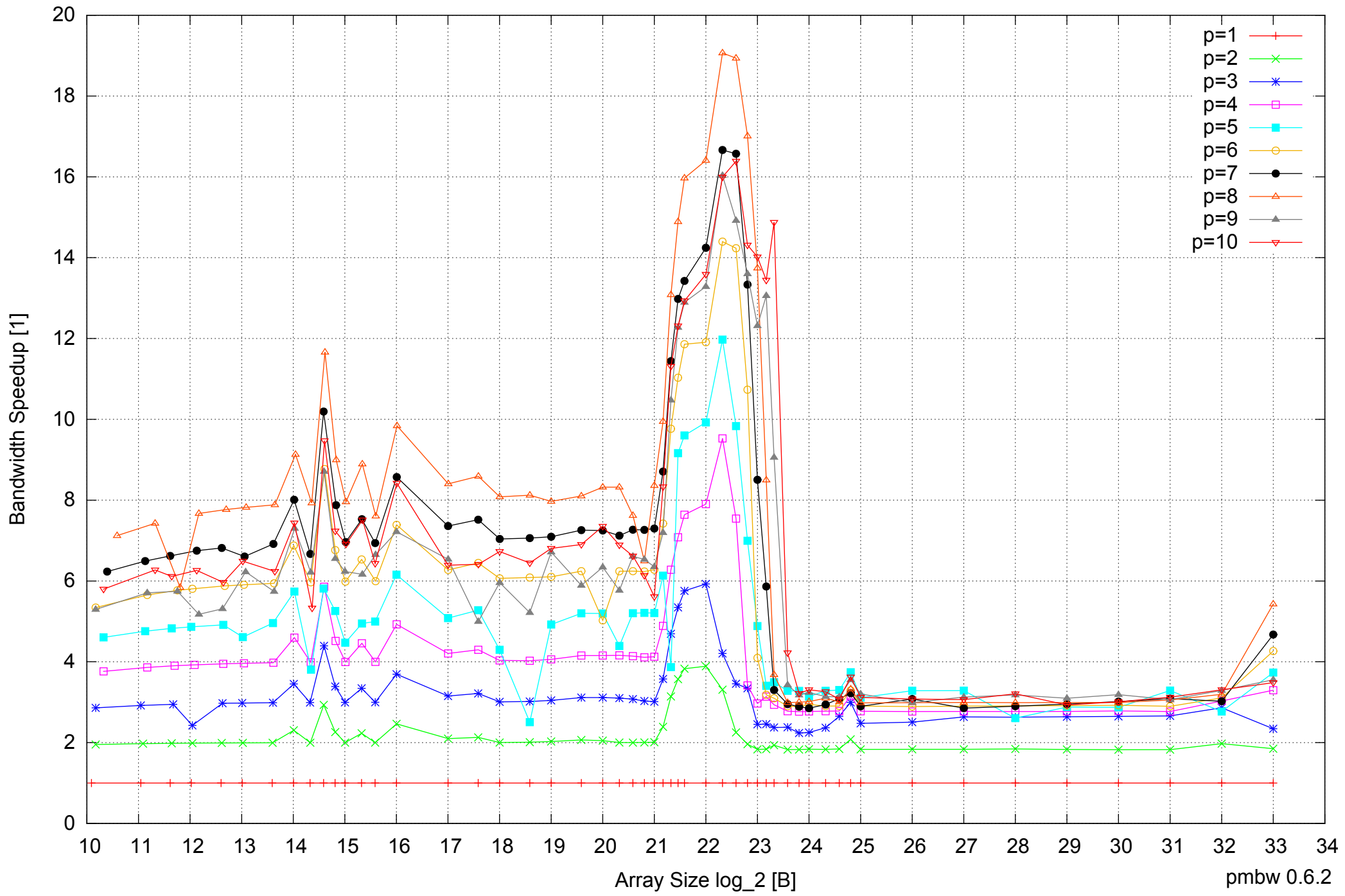
AMD Opteron 2350 16GB - Speedup of Parallel Memory Bandwidth - ScanRead32PtrSimpleLoop
