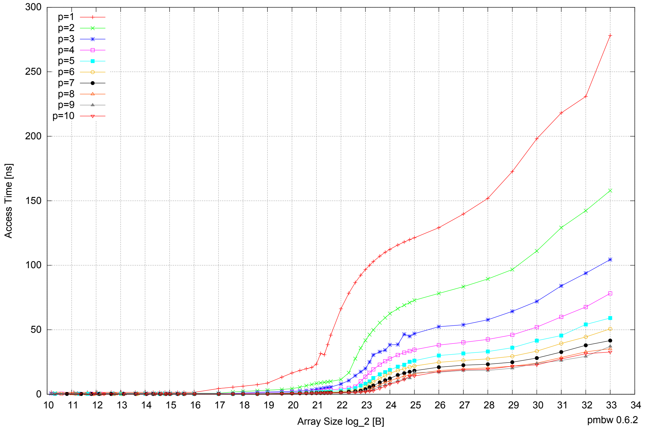
AMD Opteron 2350 16GB - Parallel Memory Access Time - PermRead64SimpleLoop
