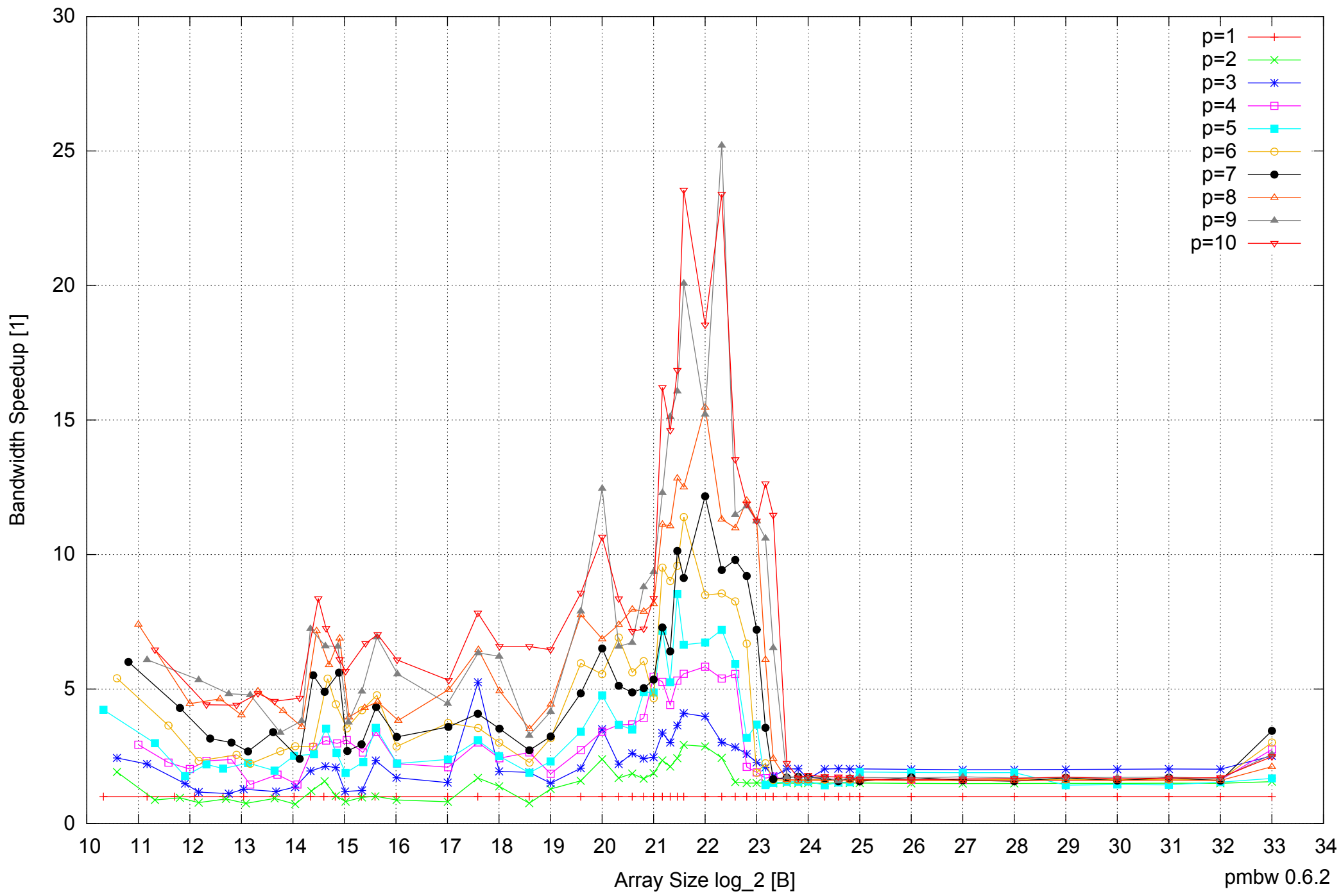
AMD Opteron 2350 16GB - Speedup of Parallel Memory Bandwidth - ScanRead128PtrSimpleLoop
