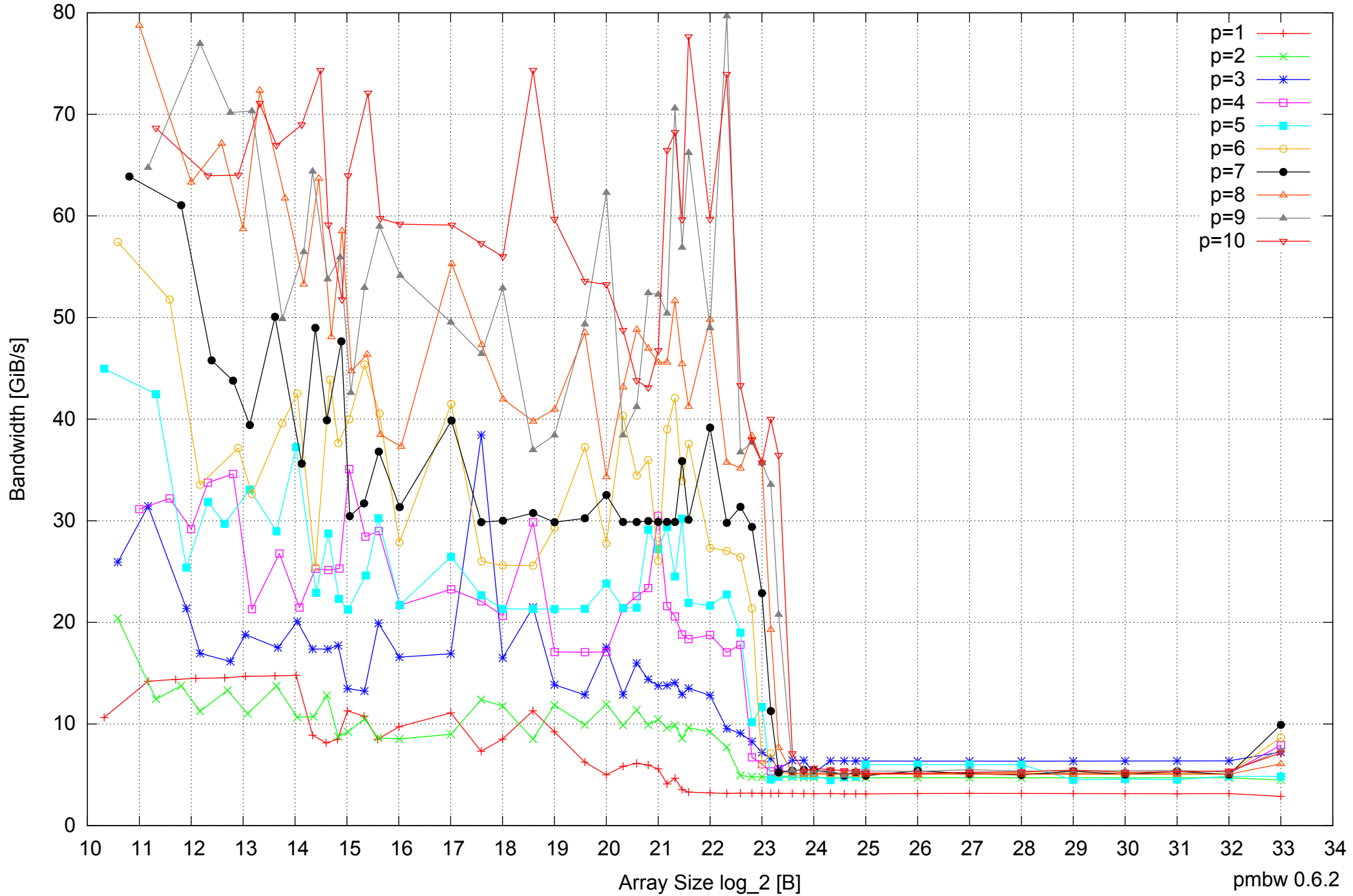
AMD Opteron 2350 16GB - Parallel Memory Bandwidth - ScanRead128PtrSimpleLoop
