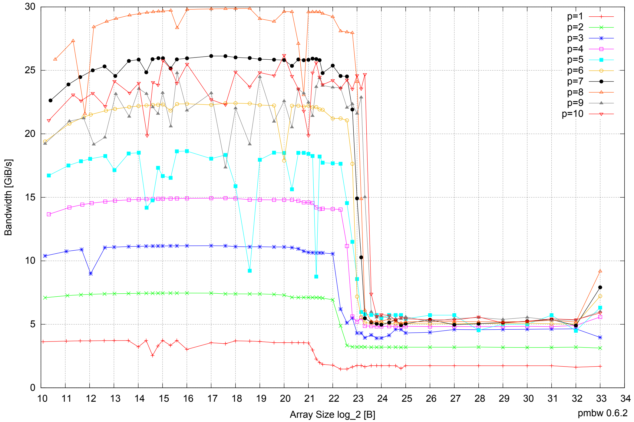
AMD Opteron 2350 16GB - Parallel Memory Bandwidth - ScanRead32PtrSimpleLoop
