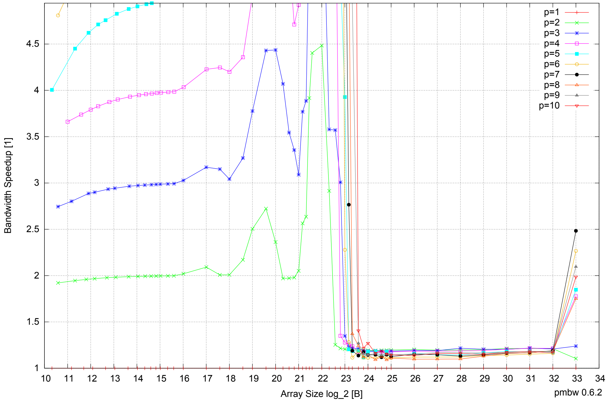
AMD Opteron 2350 16GB - Speedup of Parallel Memory Bandwidth (enlarged) - ScanWrite128PtrSimpleLoop
