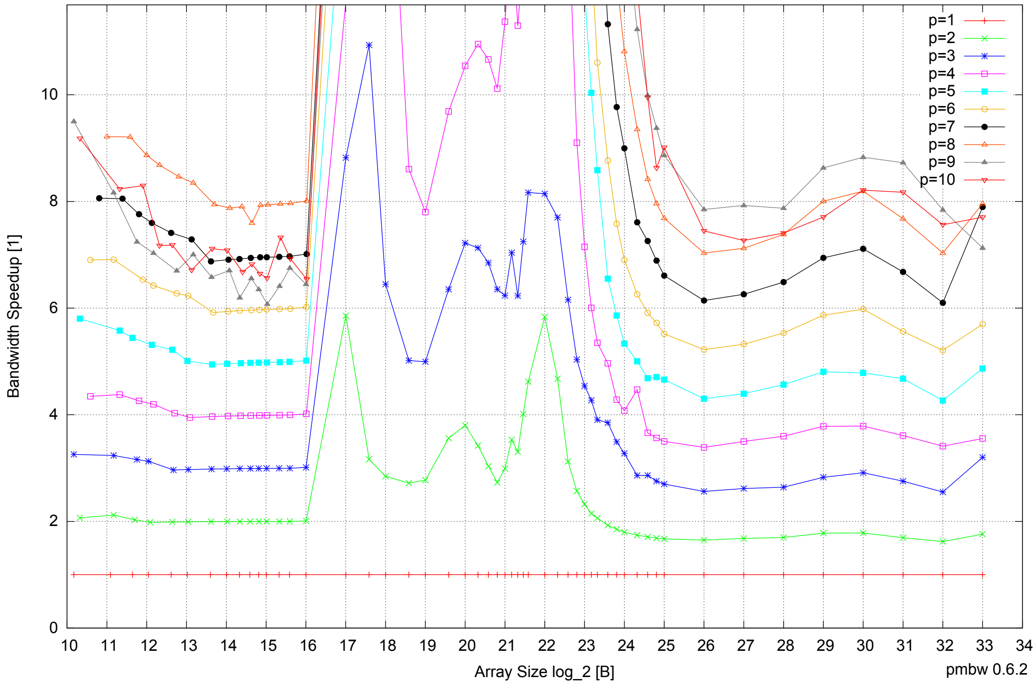
AMD Opteron 2350 16GB - Speedup of Parallel Memory Bandwidth (enlarged) - PermRead64UnrollLoop
