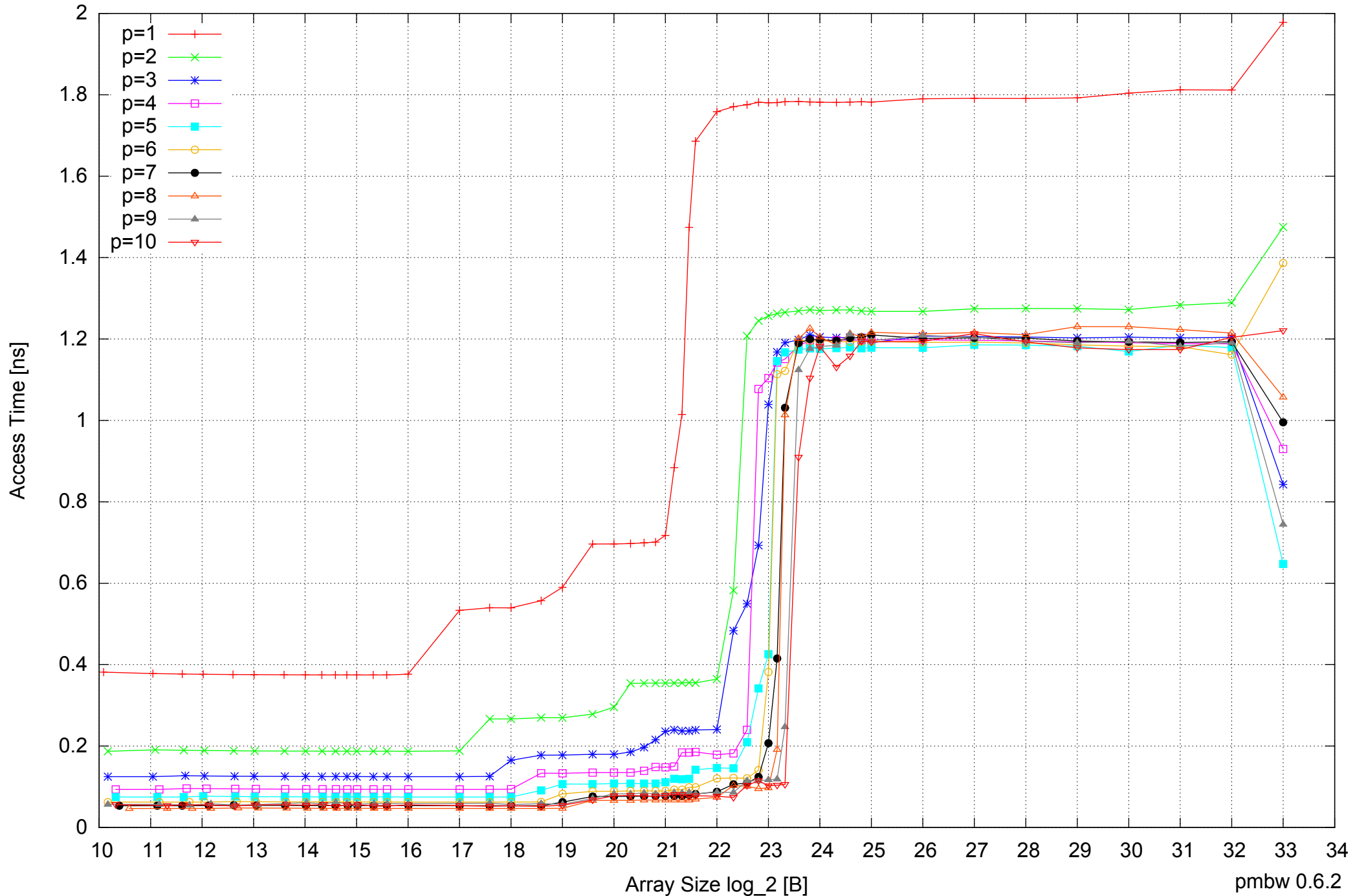
AMD Opteron 2350 16GB - Parallel Memory Access Time - ScanWrite32PtrUnrollLoop
