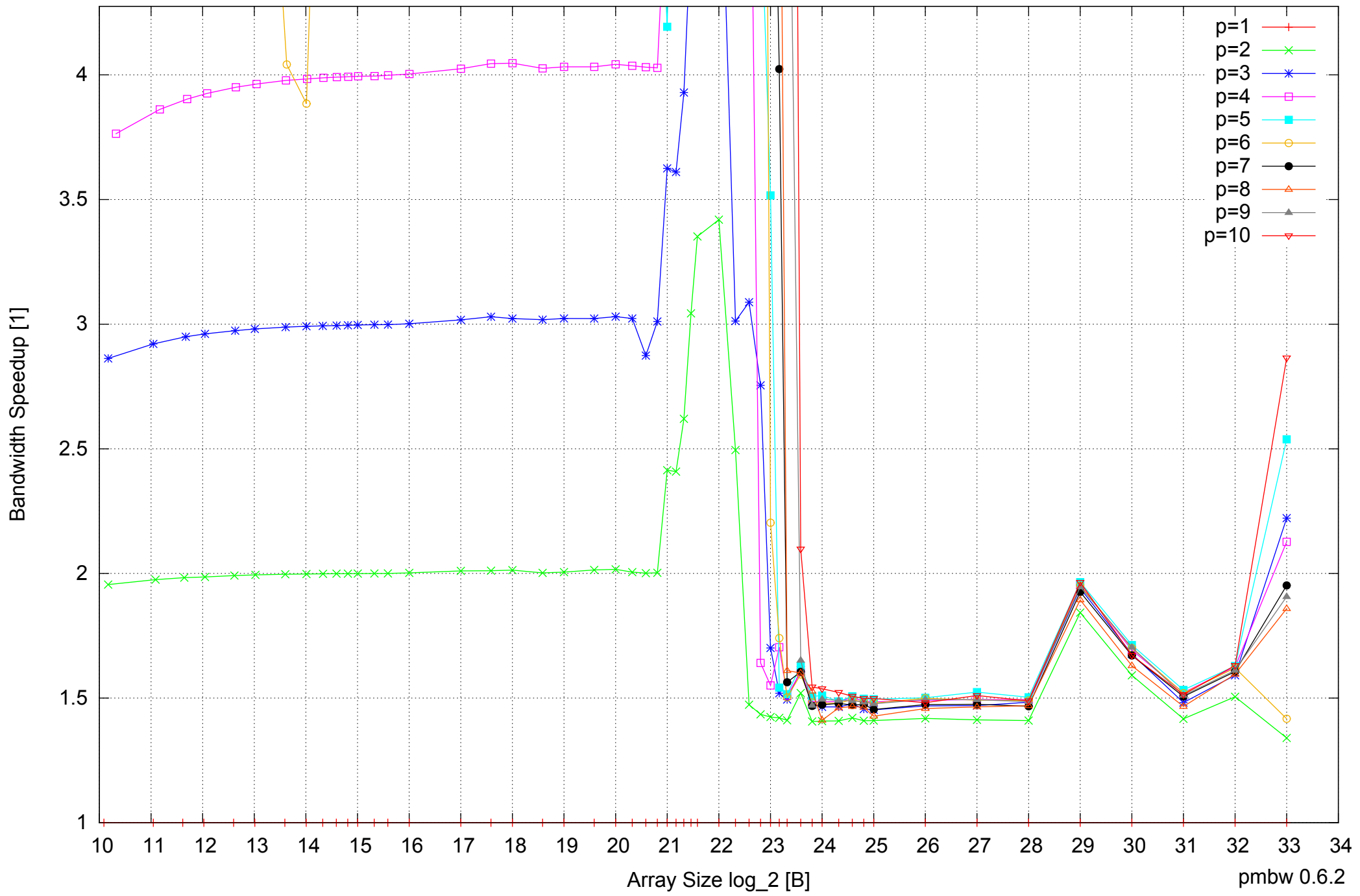
AMD Opteron 2350 16GB - Speedup of Parallel Memory Bandwidth (enlarged) - ScanWrite32PtrSimpleLoop
