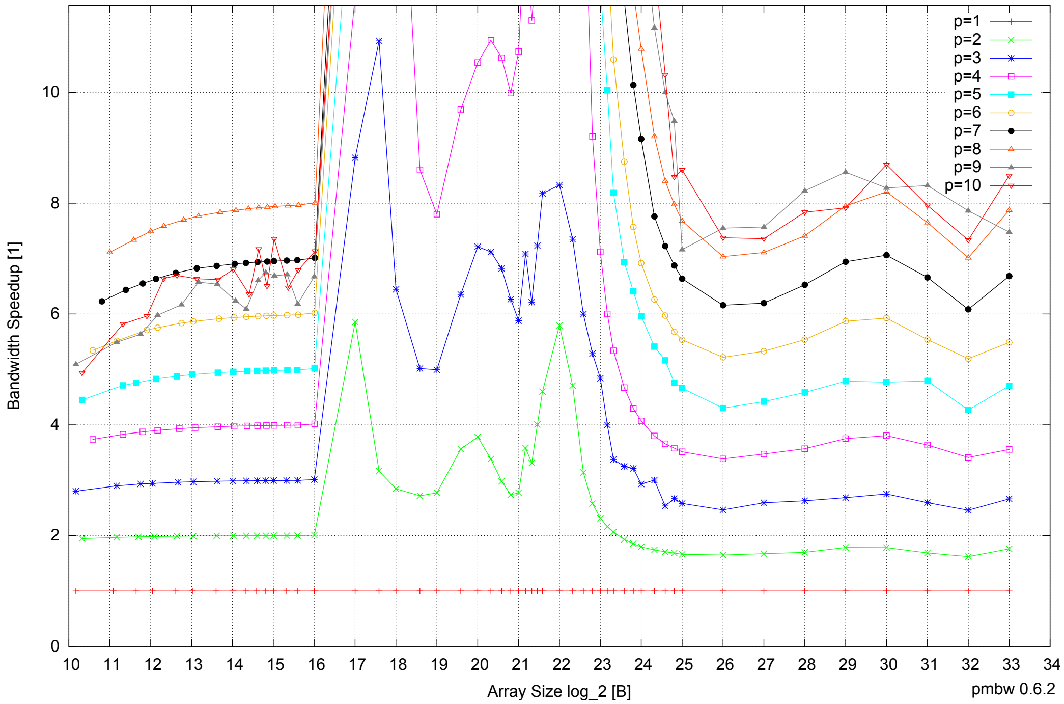
AMD Opteron 2350 16GB - Speedup of Parallel Memory Bandwidth (enlarged) - PermRead64SimpleLoop
