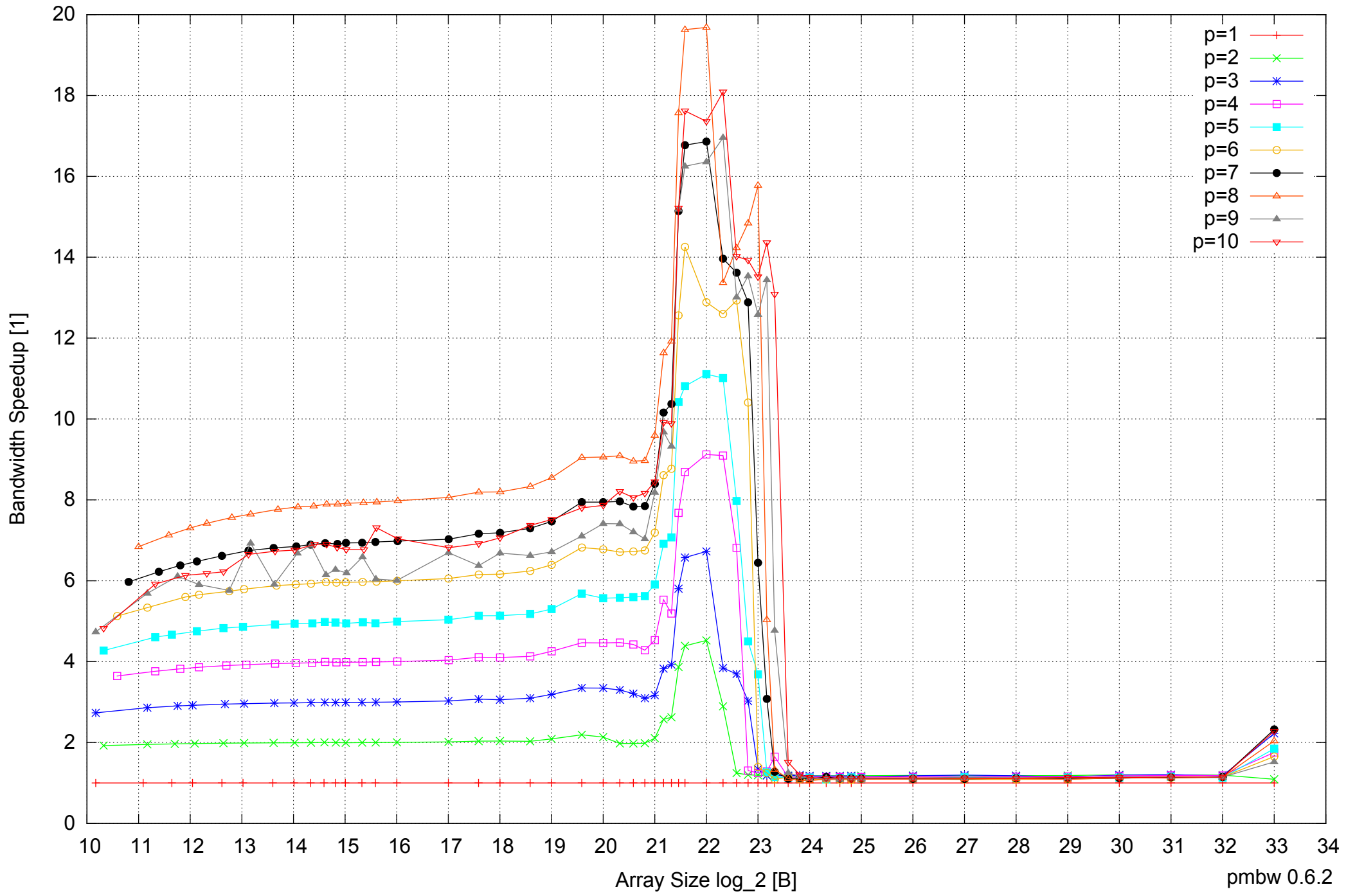
AMD Opteron 2350 16GB - Speedup of Parallel Memory Bandwidth - ScanWrite64IndexSimpleLoop
