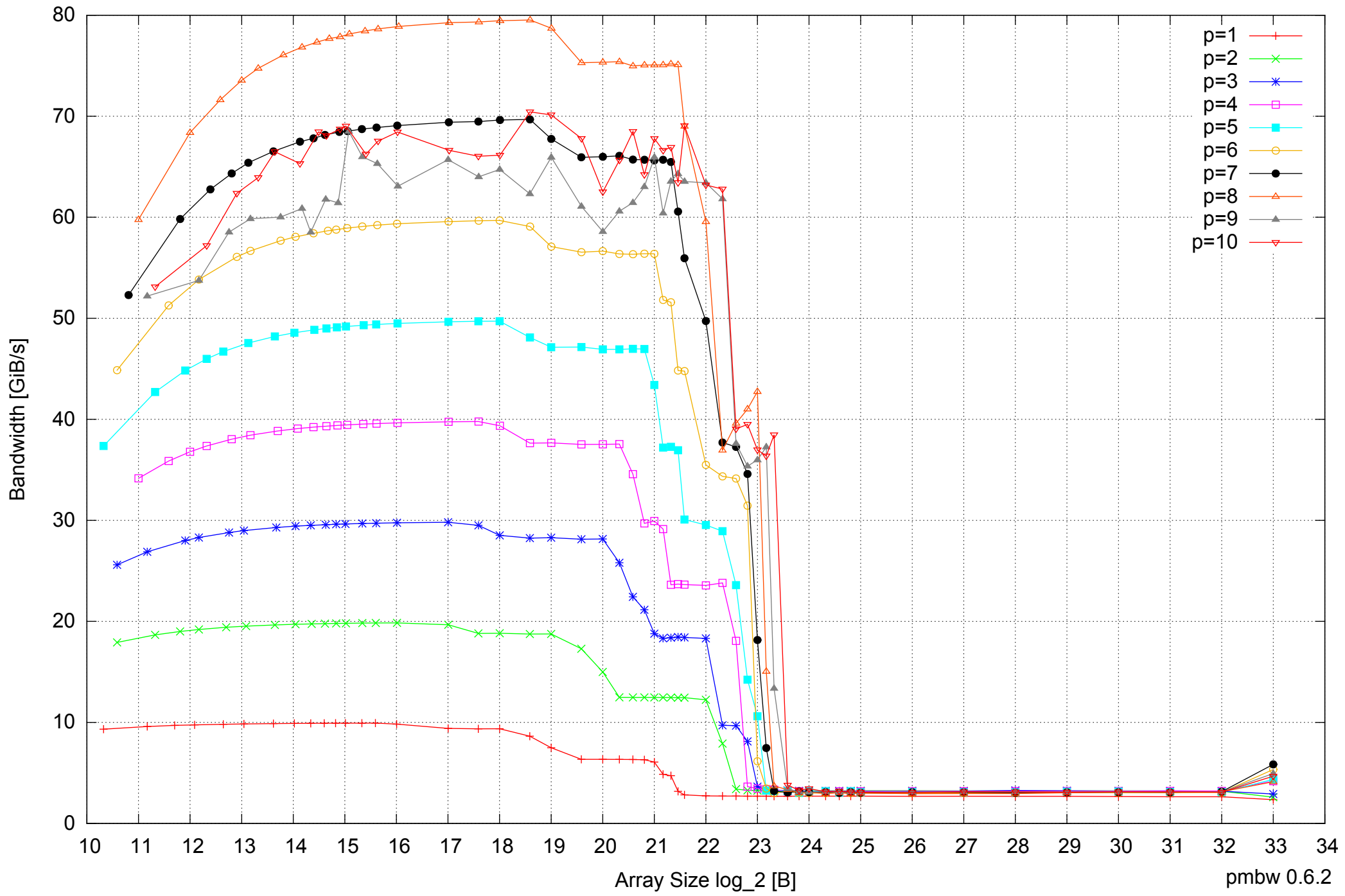
AMD Opteron 2350 16GB - Parallel Memory Bandwidth - ScanWrite128PtrSimpleLoop
