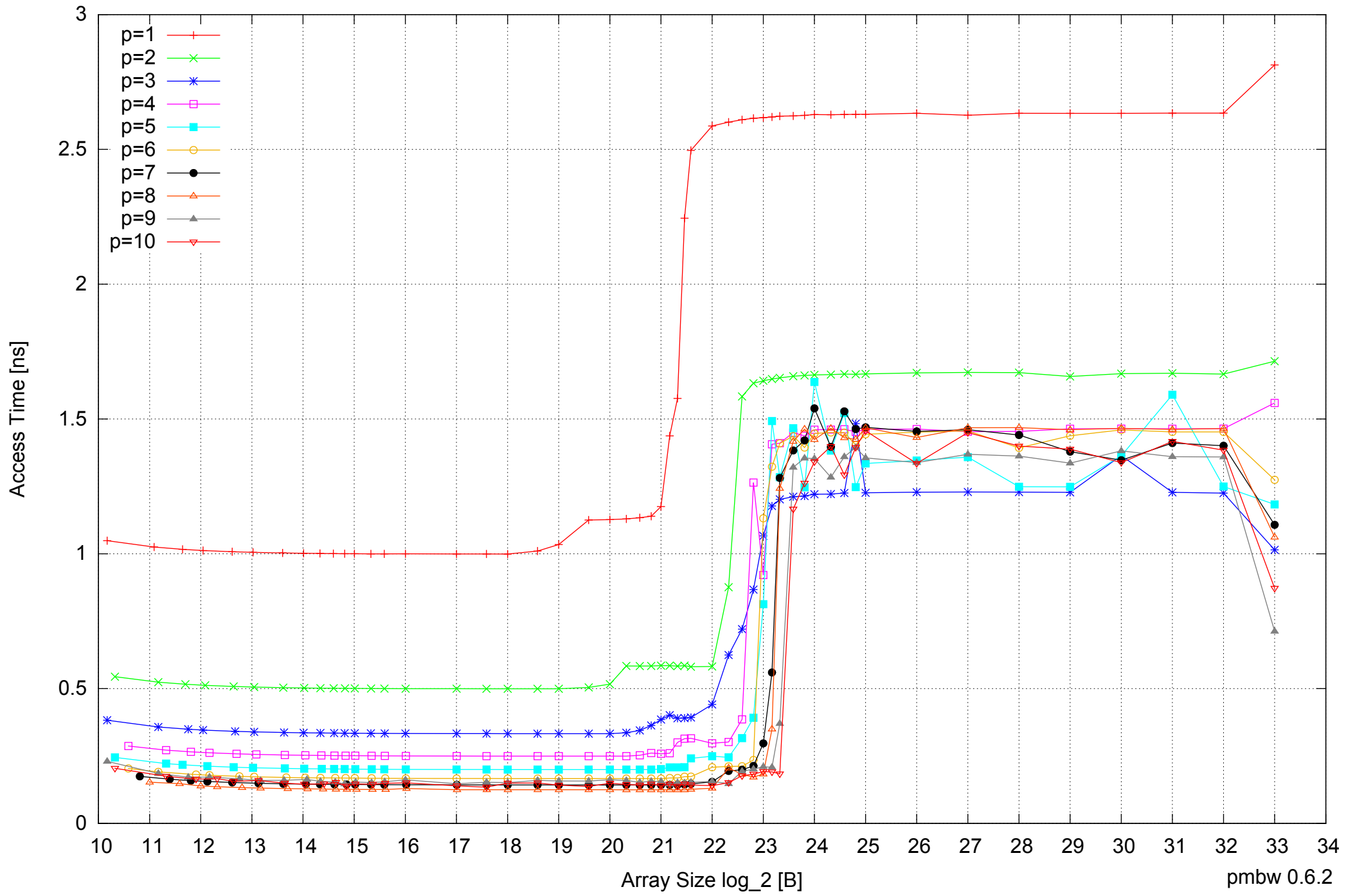
AMD Opteron 2350 16GB - Parallel Memory Access Time - ScanRead64IndexSimpleLoop
