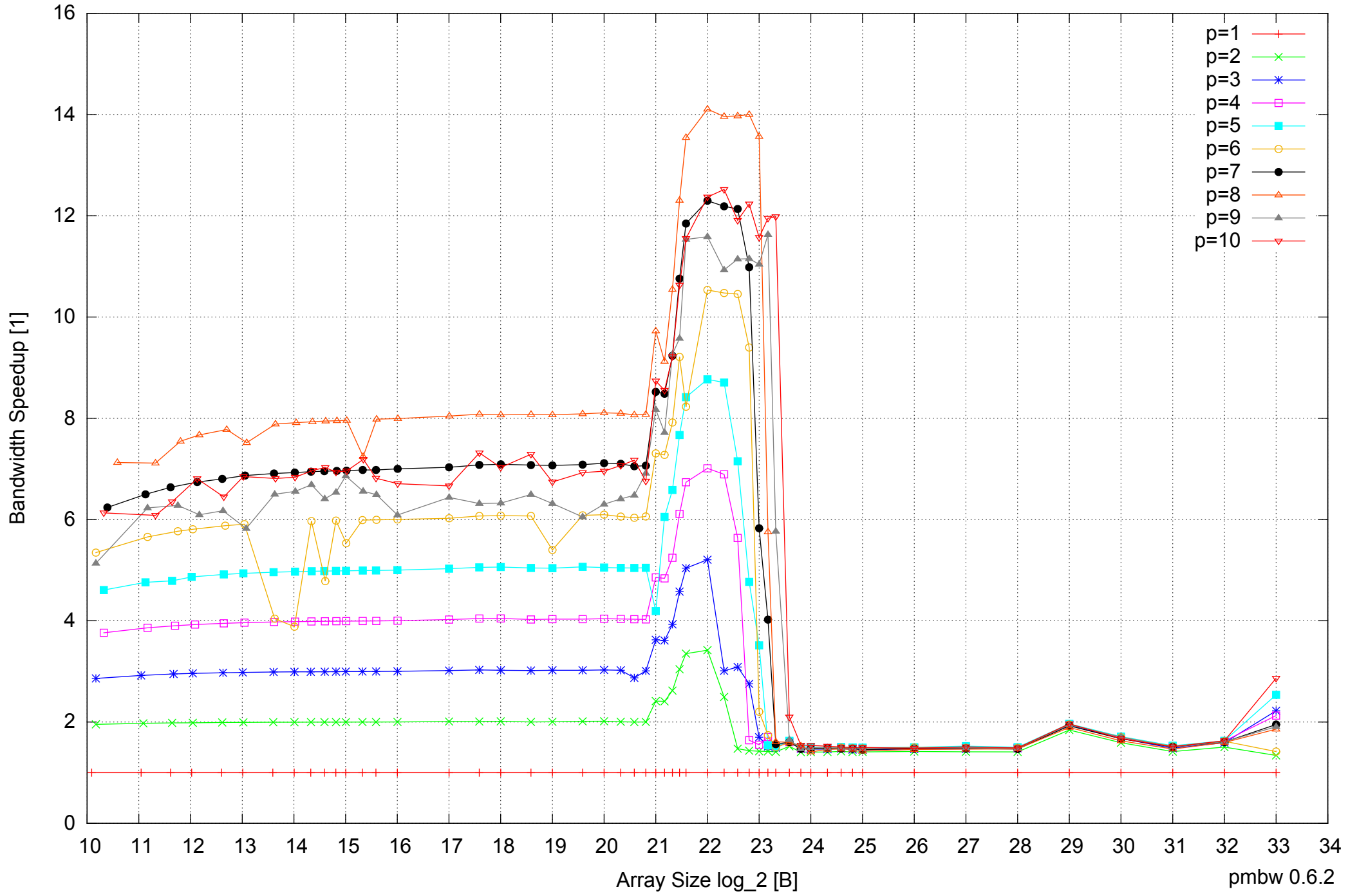
AMD Opteron 2350 16GB - Speedup of Parallel Memory Bandwidth - ScanWrite32PtrSimpleLoop
