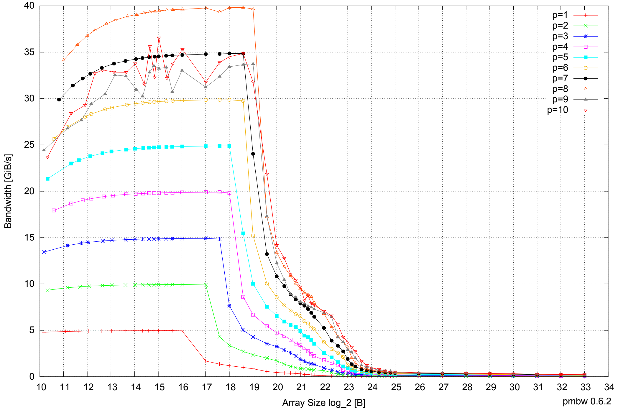
AMD Opteron 2350 16GB - Parallel Memory Bandwidth - PermRead64SimpleLoop
