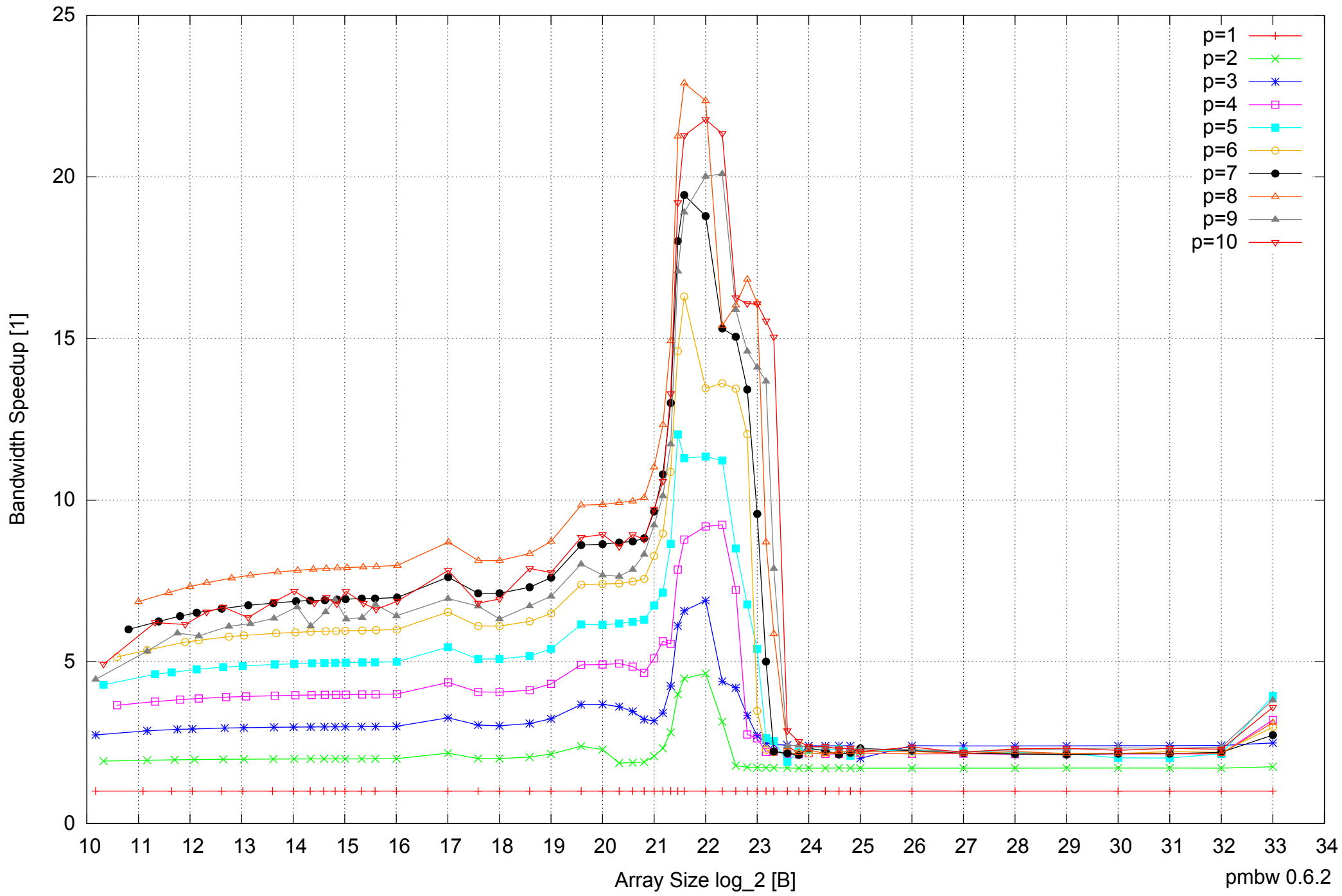
AMD Opteron 2350 16GB - Speedup of Parallel Memory Bandwidth - ScanRead64PtrSimpleLoop
