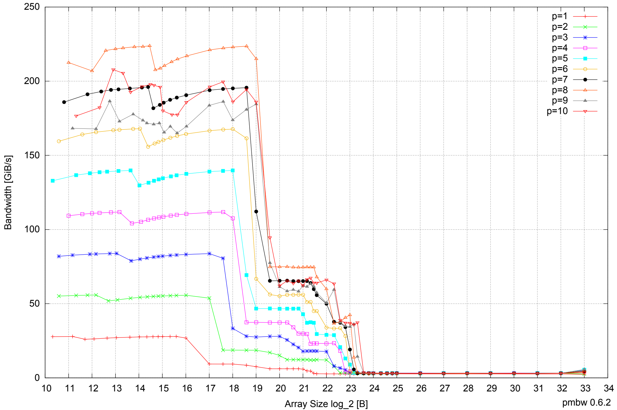
AMD Opteron 2350 16GB - Parallel Memory Bandwidth - ScanWrite128PtrUnrollLoop
