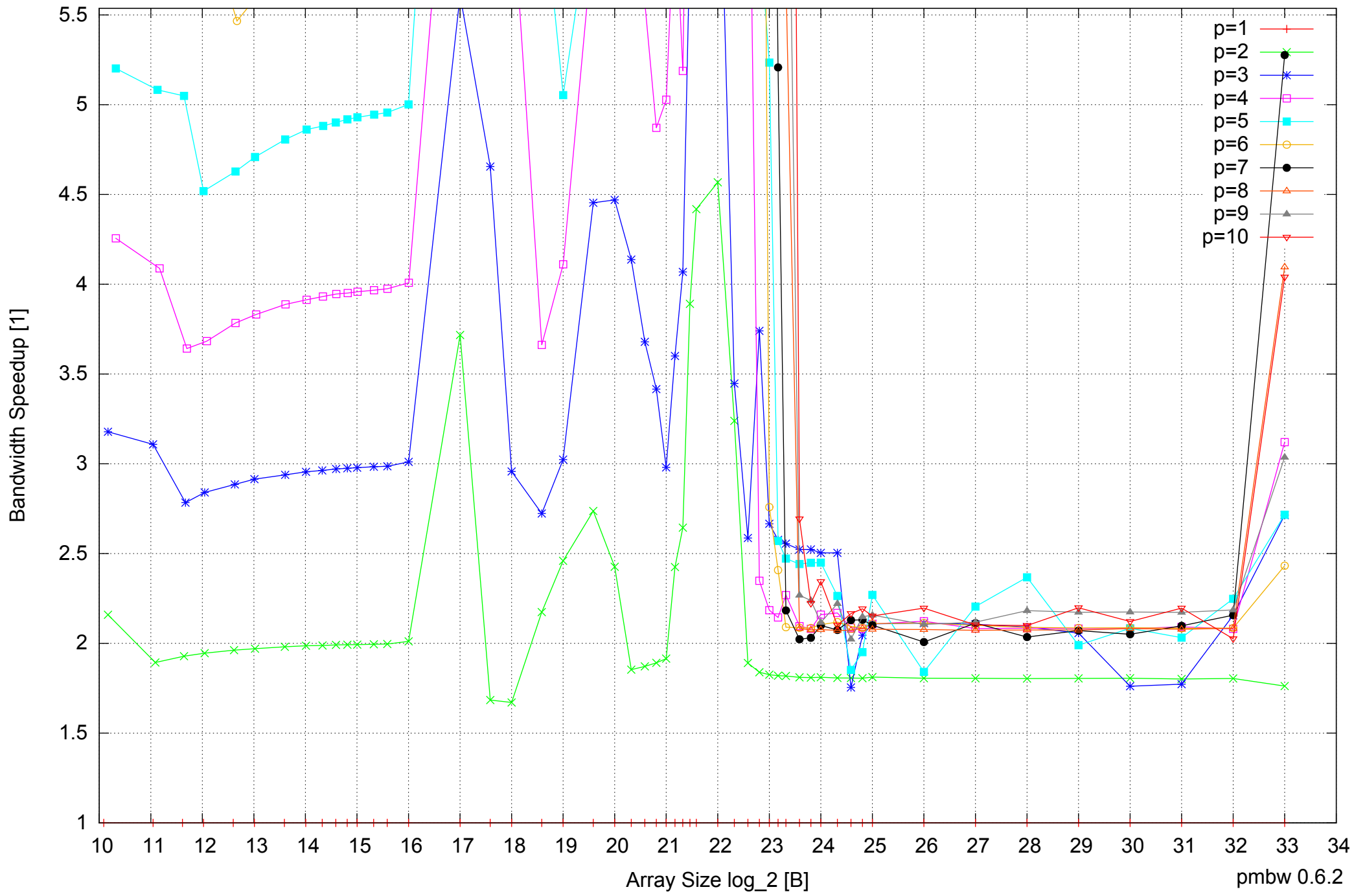
AMD Opteron 2350 16GB - Speedup of Parallel Memory Bandwidth (enlarged) - ScanRead32PtrUnrollLoop
