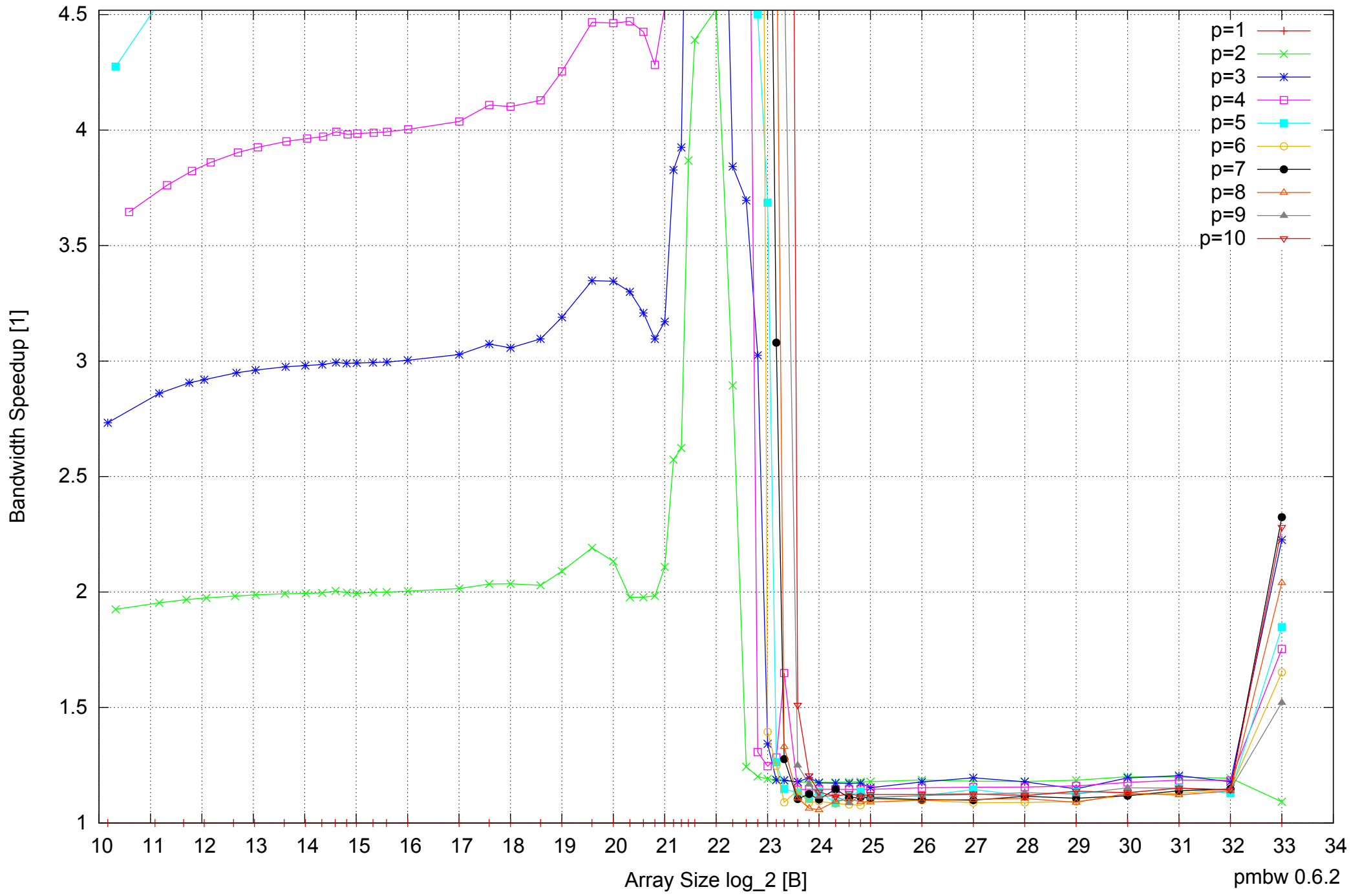
AMD Opteron 2350 16GB - Speedup of Parallel Memory Bandwidth (enlarged) - ScanWrite64IndexSimpleLoop
