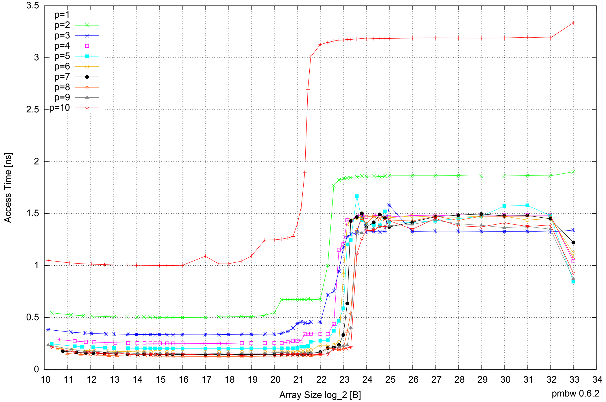
AMD Opteron 2350 16GB - Parallel Memory Access Time - ScanRead64PtrSimpleLoop
