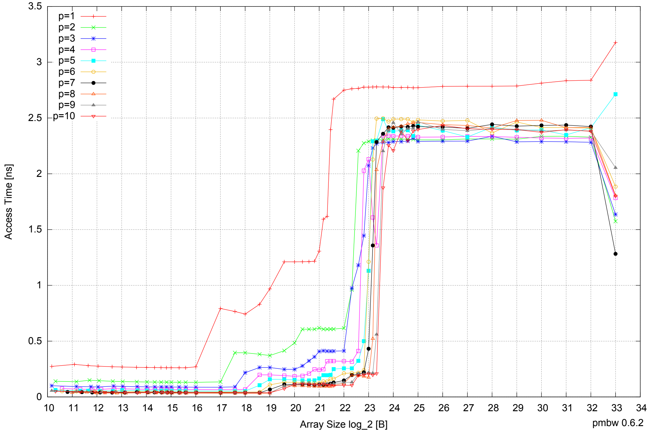
AMD Opteron 2350 16GB - Parallel Memory Access Time - ScanWrite64PtrUnrollLoop
