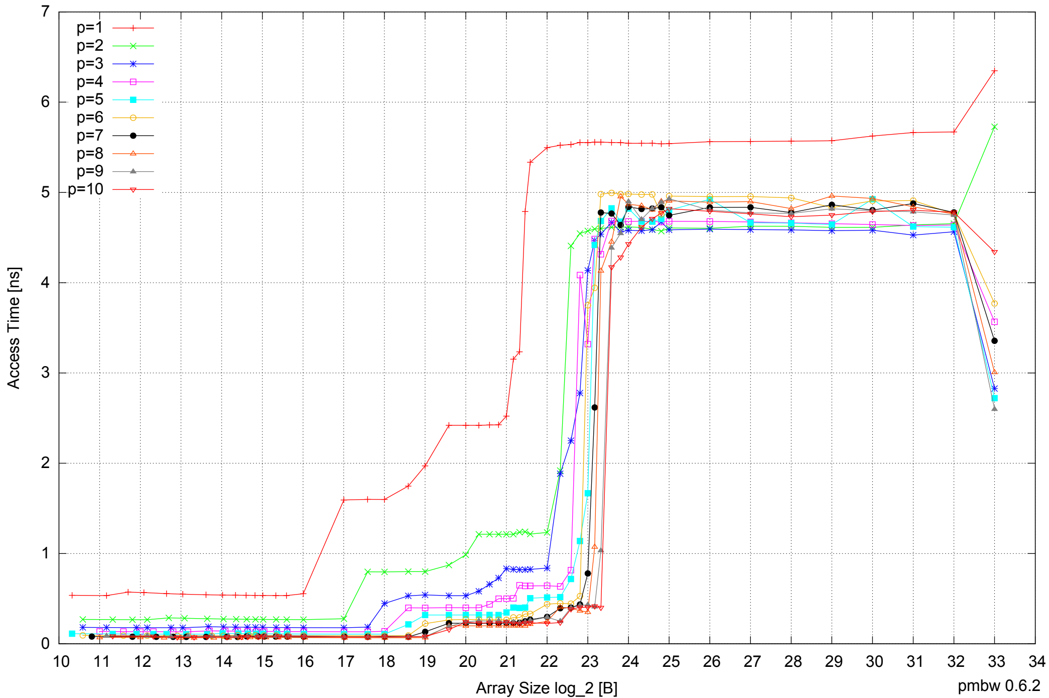
AMD Opteron 2350 16GB - Parallel Memory Access Time - ScanWrite128PtrUnrollLoop
