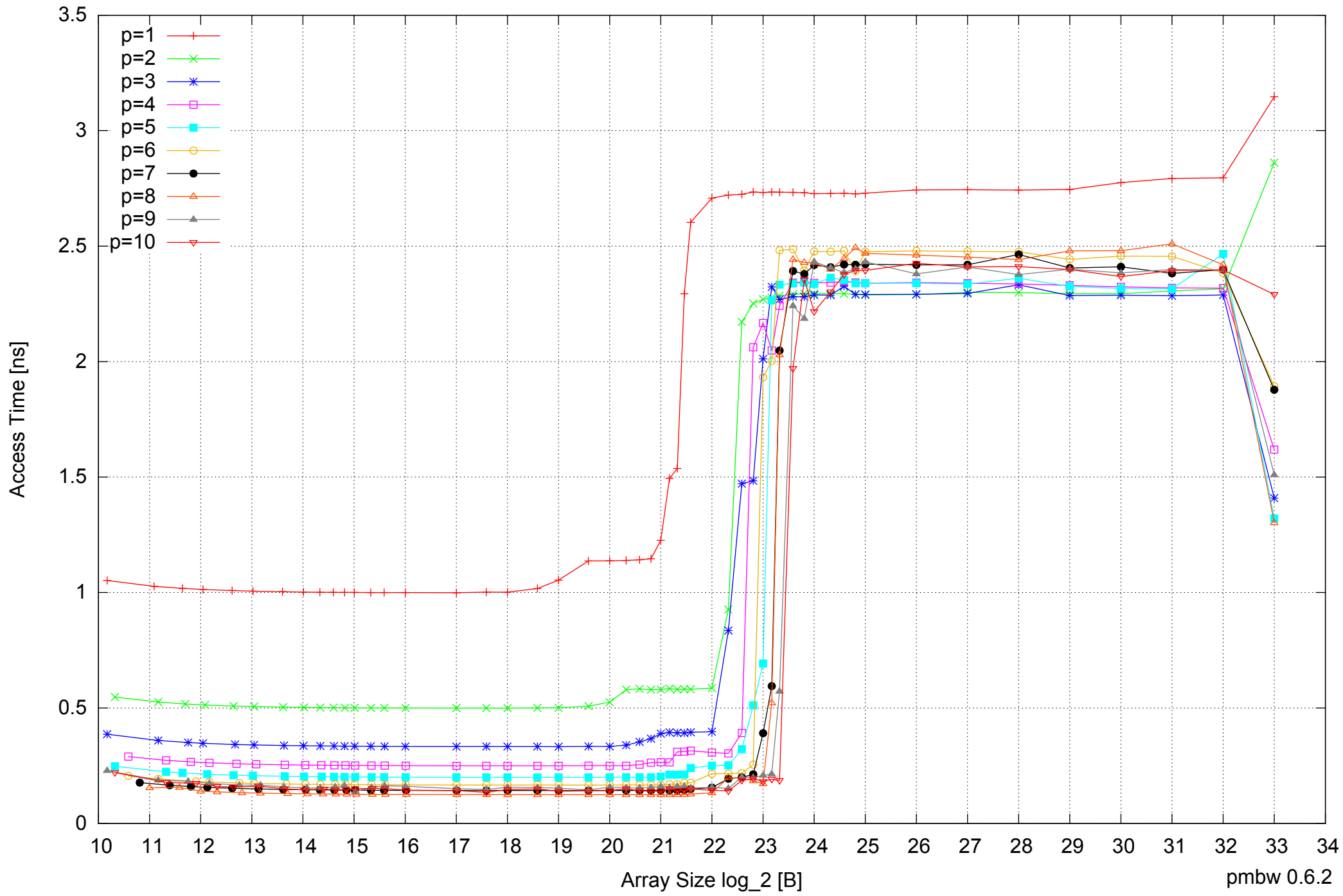
AMD Opteron 2350 16GB - Parallel Memory Access Time - ScanWrite64PtrSimpleLoop
