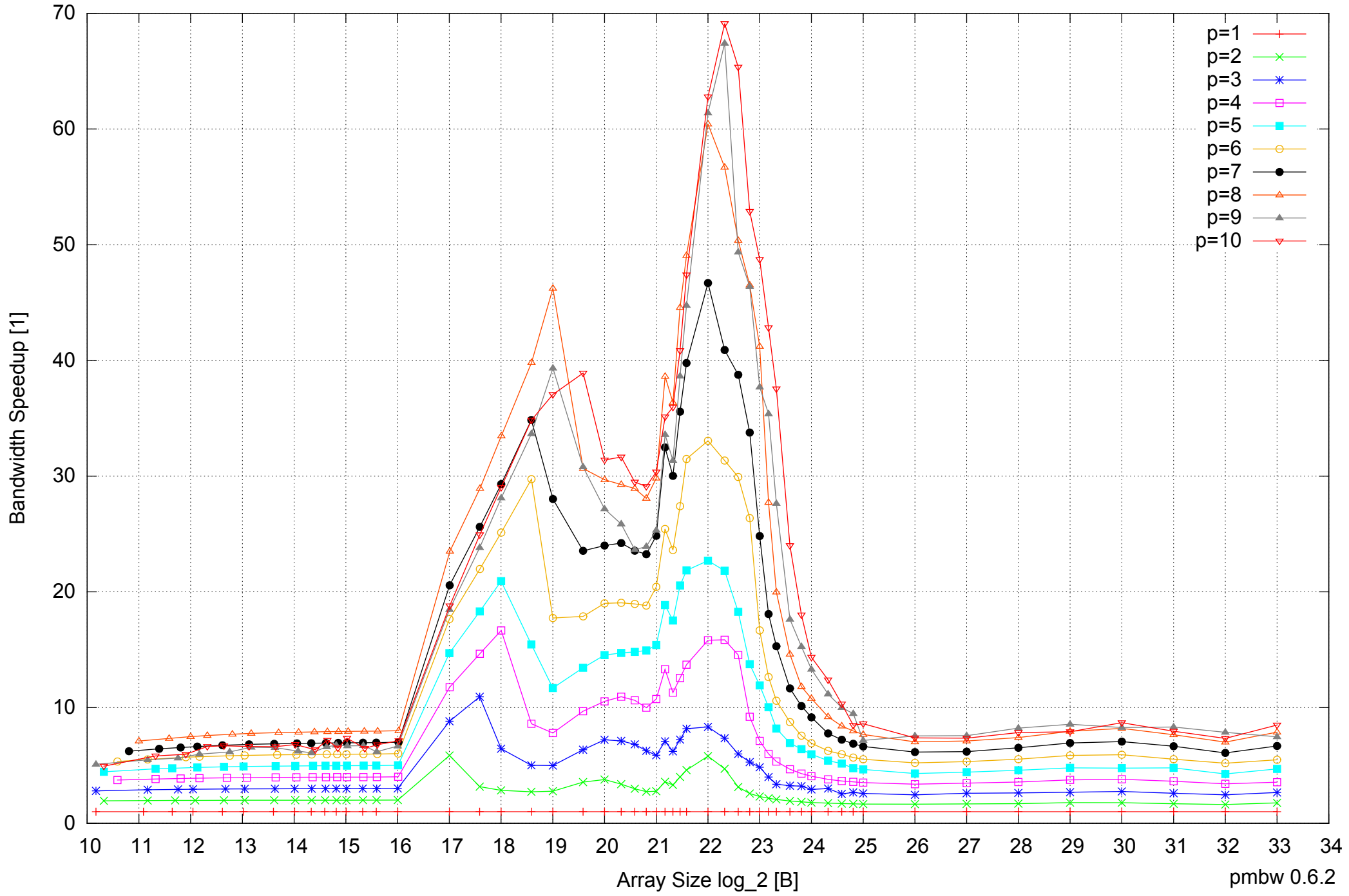
AMD Opteron 2350 16GB - Speedup of Parallel Memory Bandwidth - PermRead64SimpleLoop
