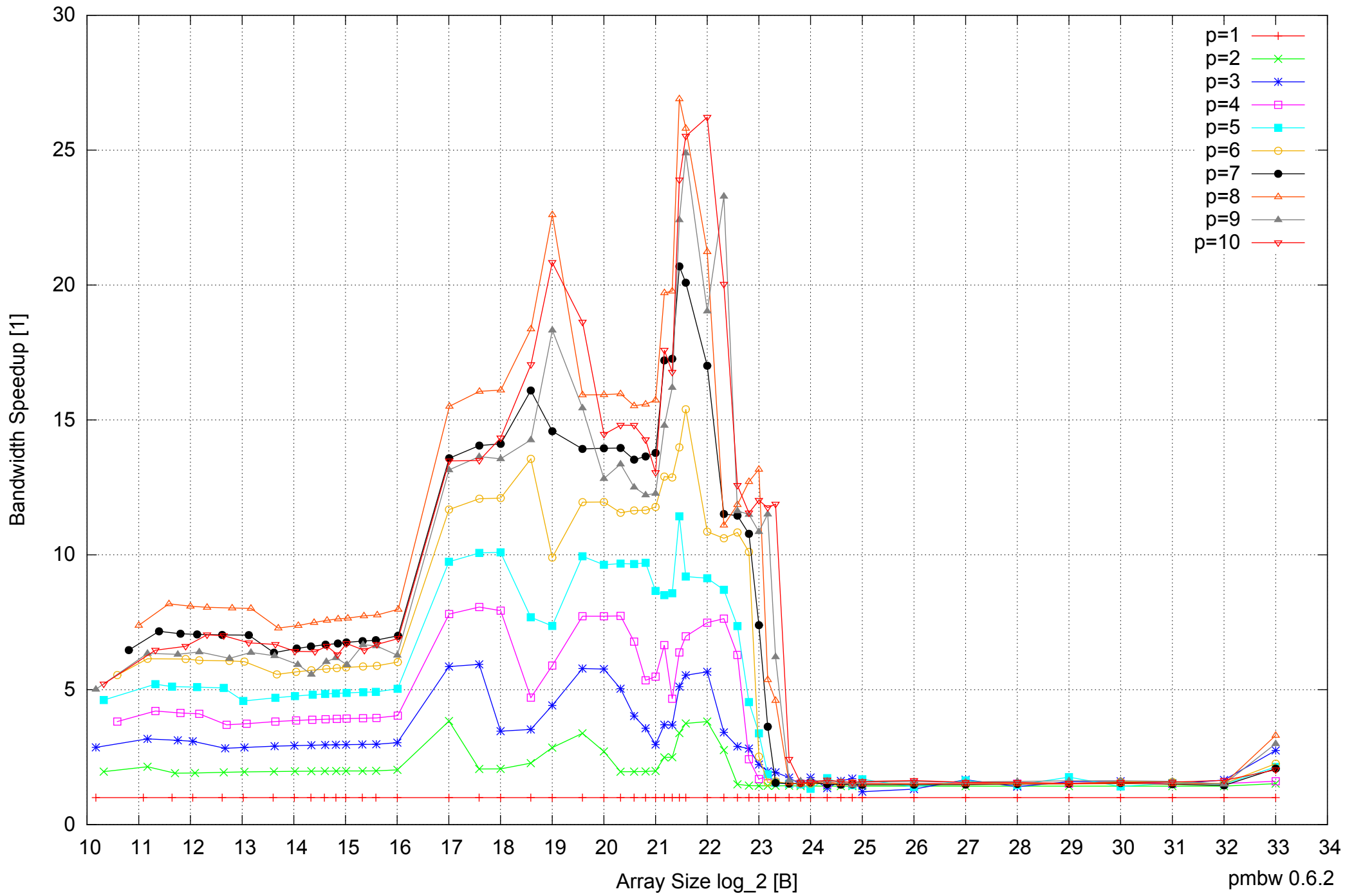
AMD Opteron 2350 16GB - Speedup of Parallel Memory Bandwidth - ScanRead64PtrUnrollLoop
