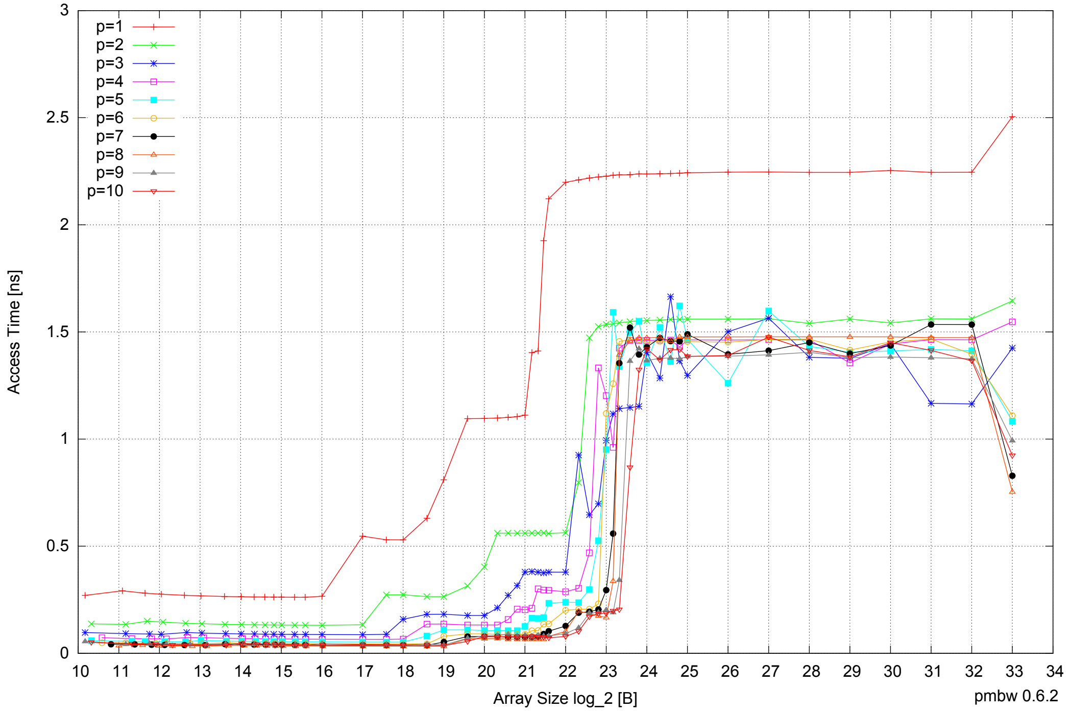
AMD Opteron 2350 16GB - Parallel Memory Access Time - ScanRead64IndexUnrollLoop
