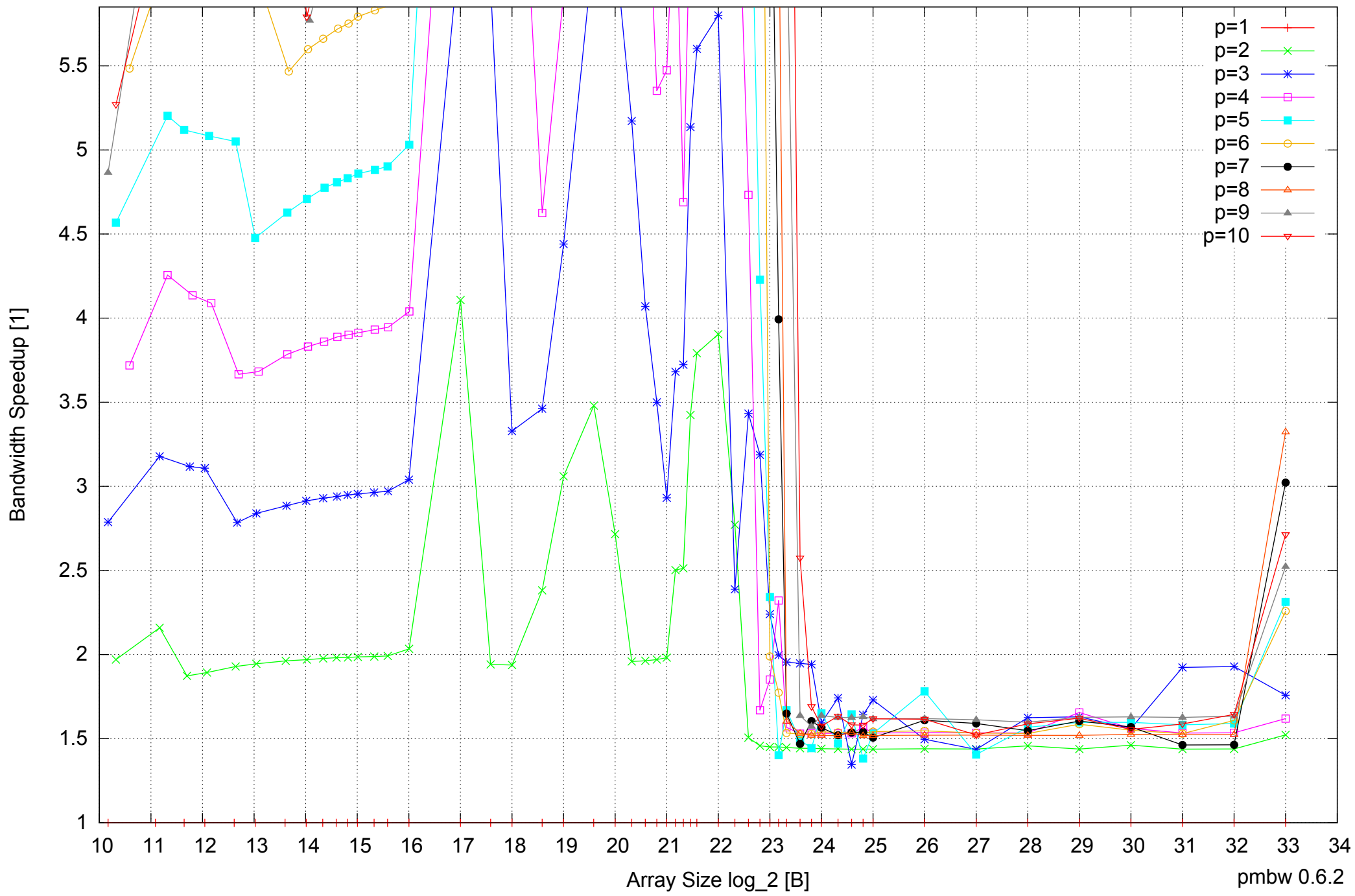
AMD Opteron 2350 16GB - Speedup of Parallel Memory Bandwidth (enlarged) - ScanRead64IndexUnrollLoop
