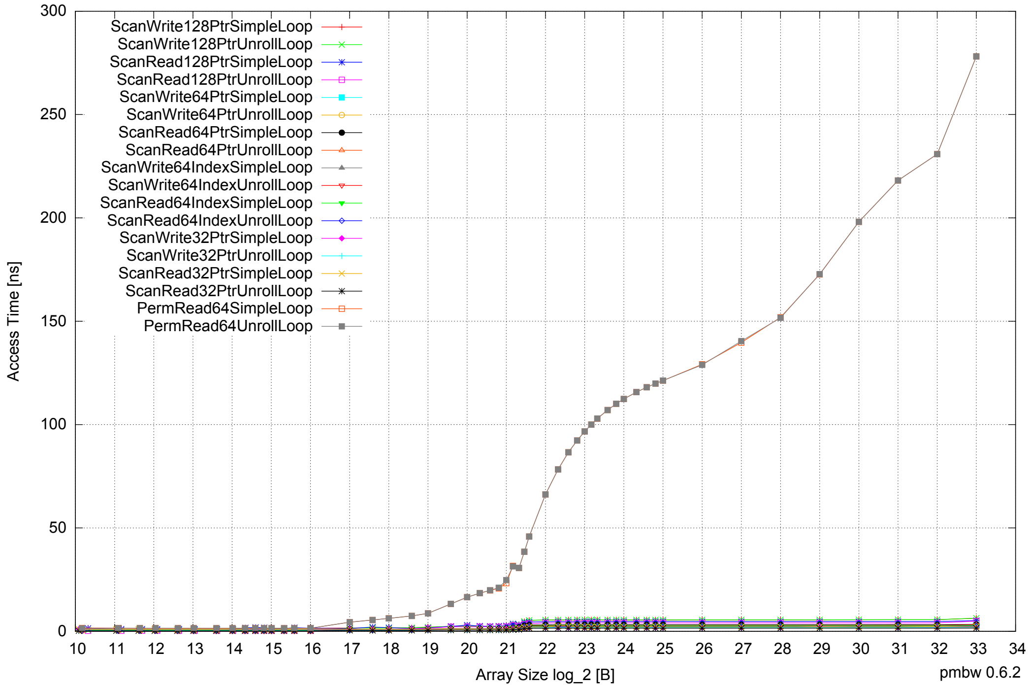
AMD Optron 2350 16GB - One Thread Memory Latency (Access Time)
