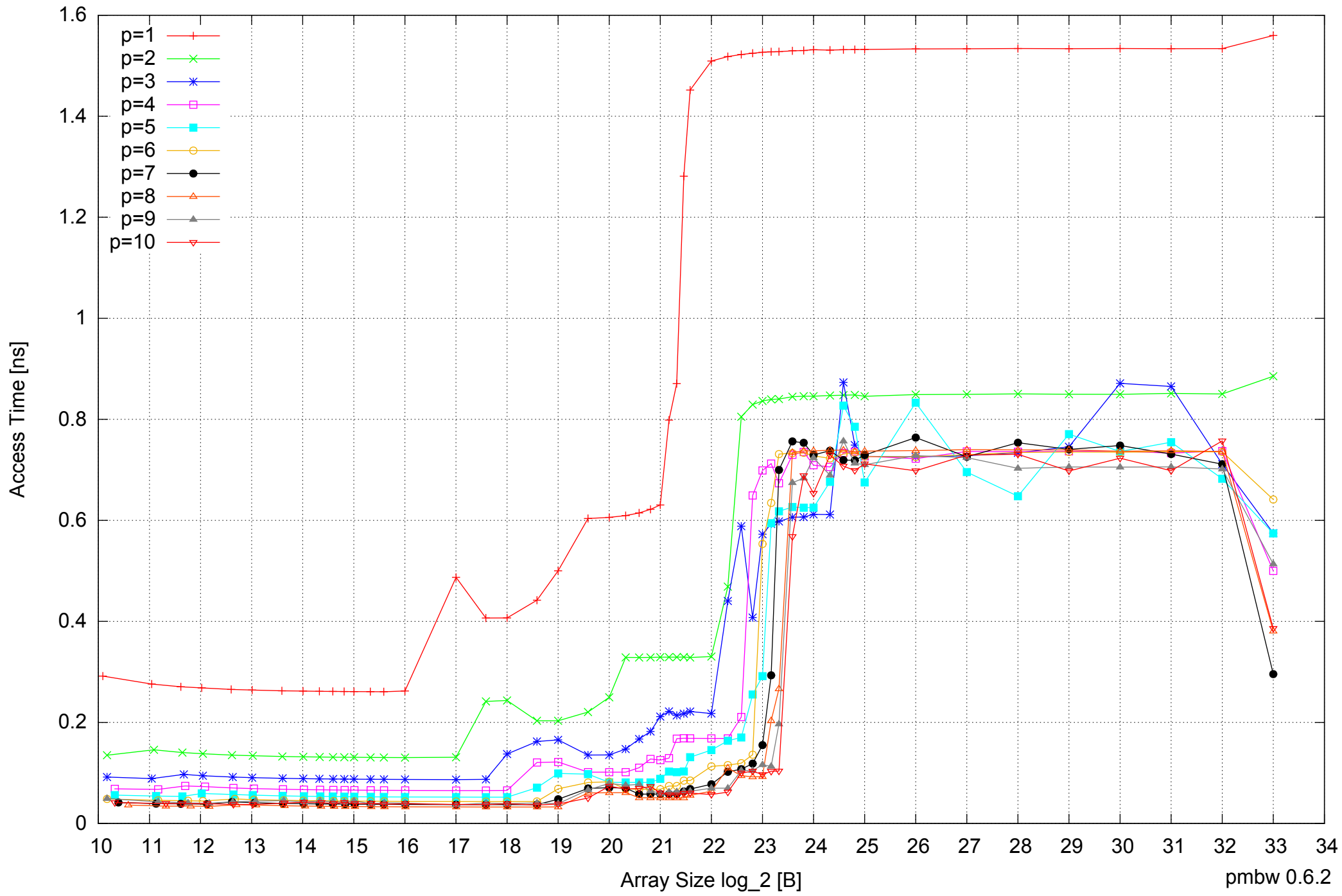
AMD Opteron 2350 16GB - Parallel Memory Access Time - ScanRead32PtrUnrollLoop
