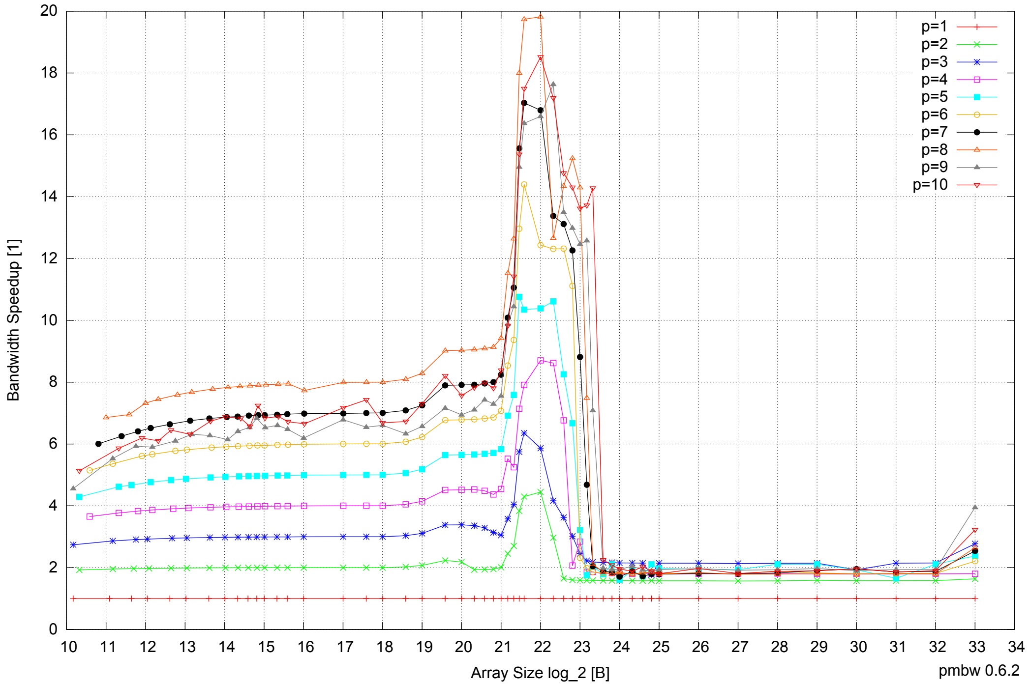
AMD Opteron 2350 16GB - Speedup of Parallel Memory Bandwidth - ScanRead64IndexSimpleLoop
