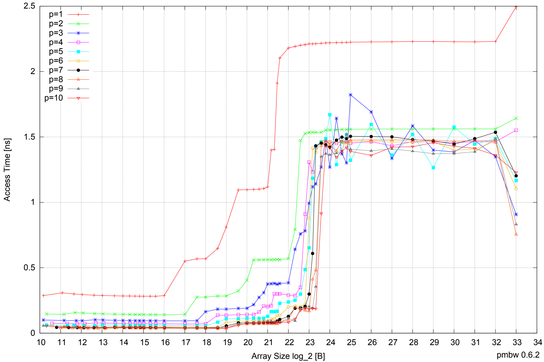
AMD Opteron 2350 16GB - Parallel Memory Access Time - ScanRead64PtrUnrollLoop
