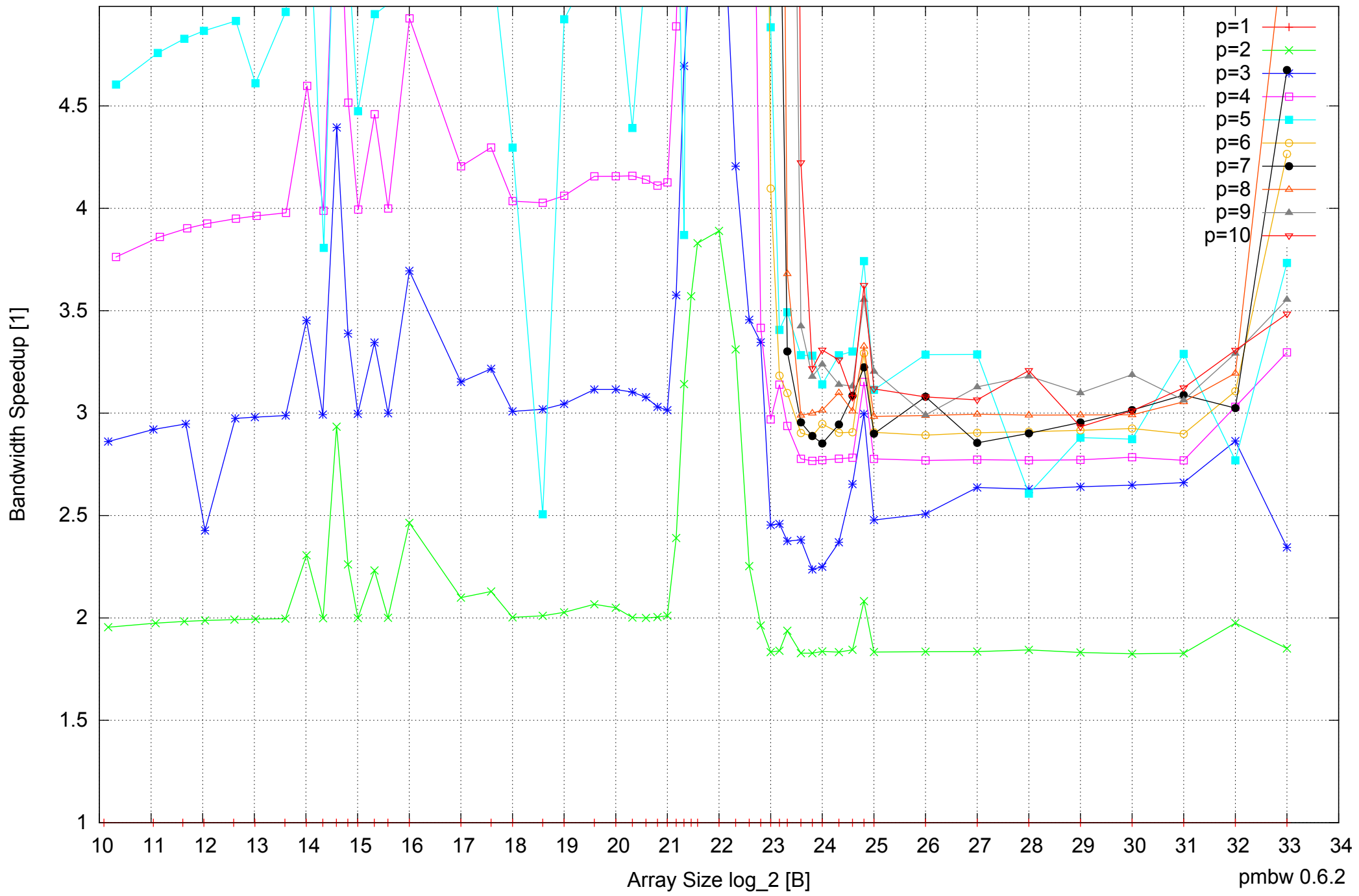
AMD Opteron 2350 16GB - Speedup of Parallel Memory Bandwidth (enlarged) - ScanRead32PtrSimpleLoop
