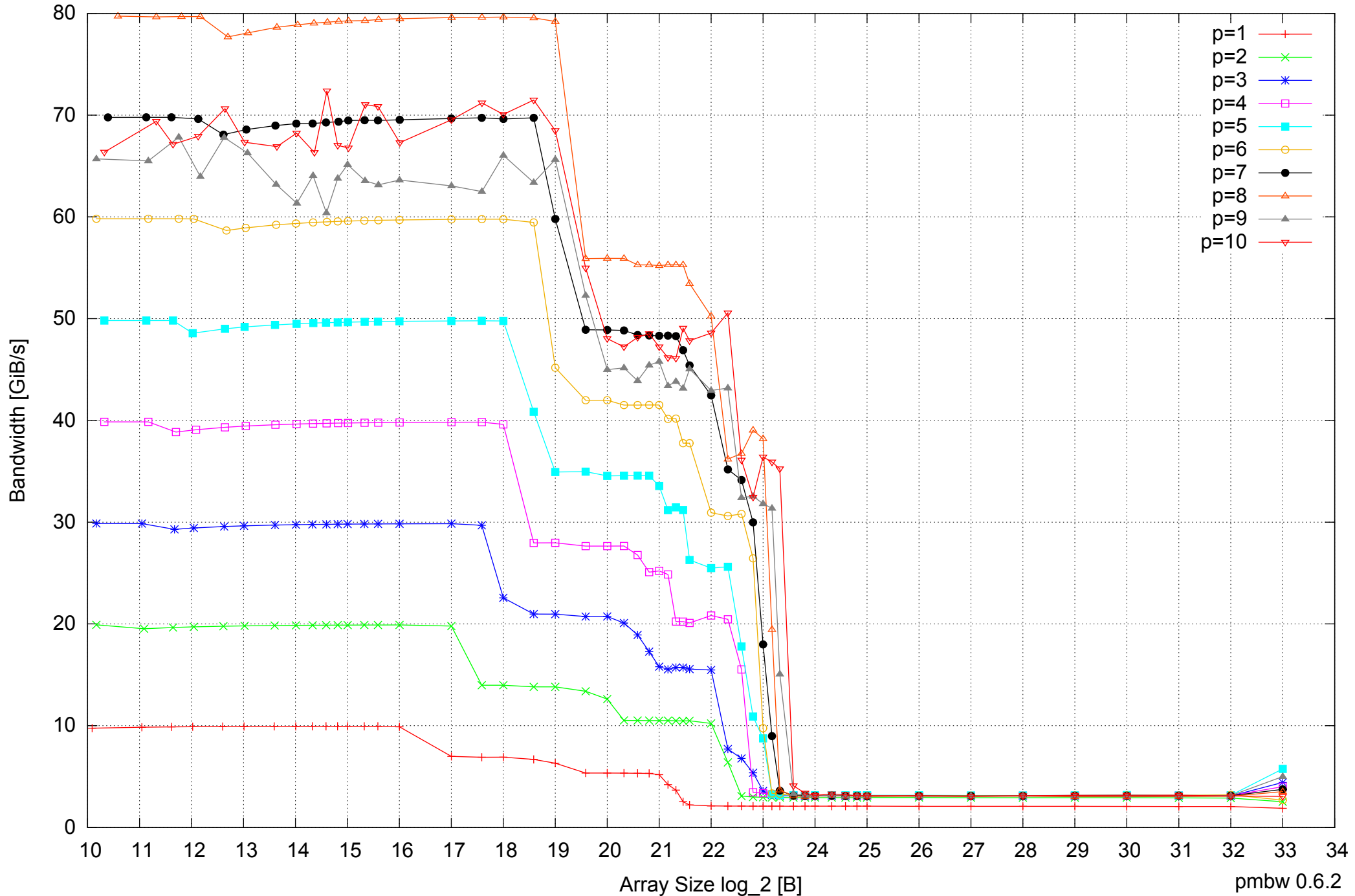
AMD Opteron 2350 16GB - Parallel Memory Bandwidth - ScanWrite32PtrUnrollLoop
