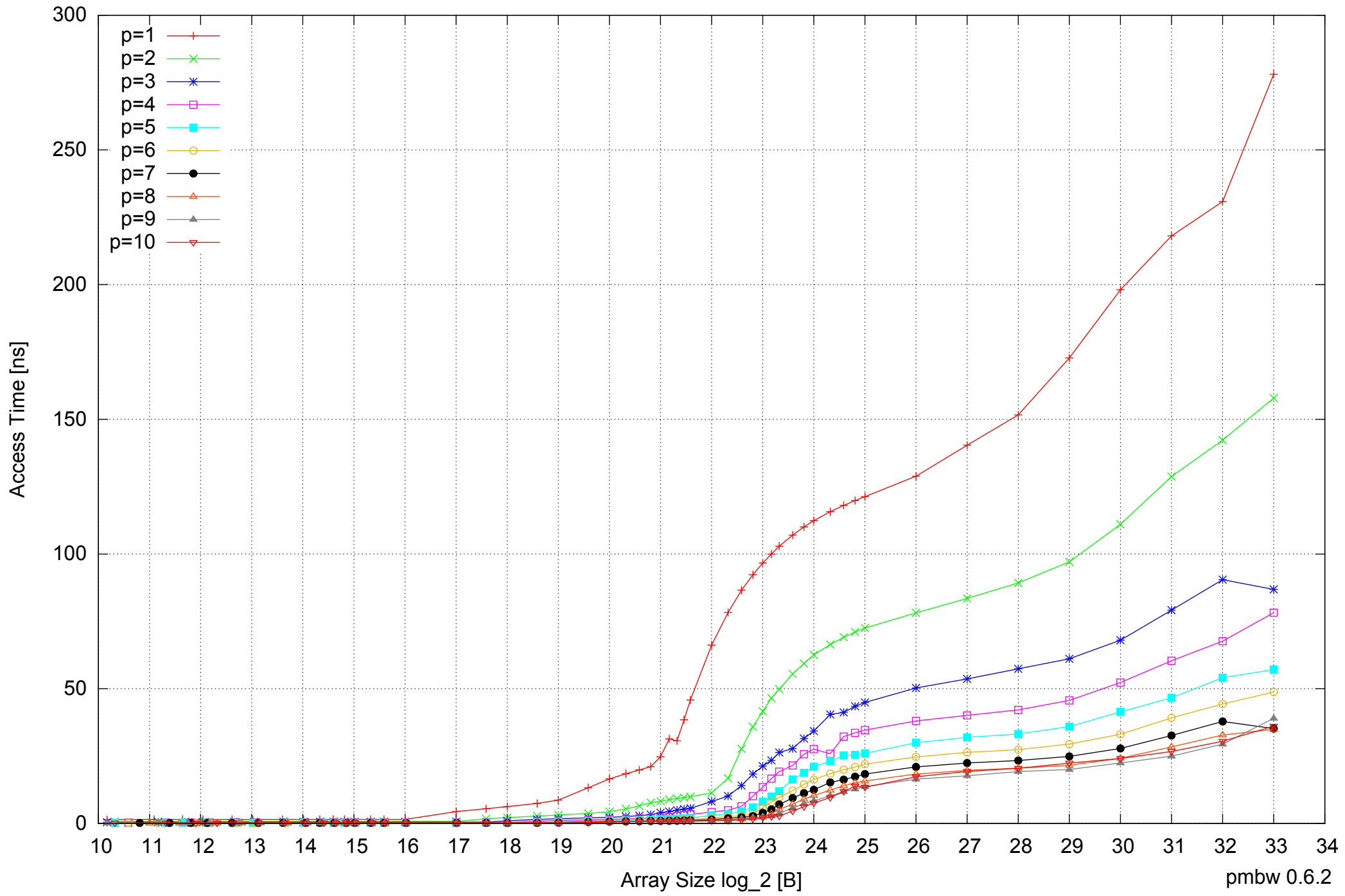
AMD Opteron 2350 16GB - Parallel Memory Access Time - PermRead64UnrollLoop
