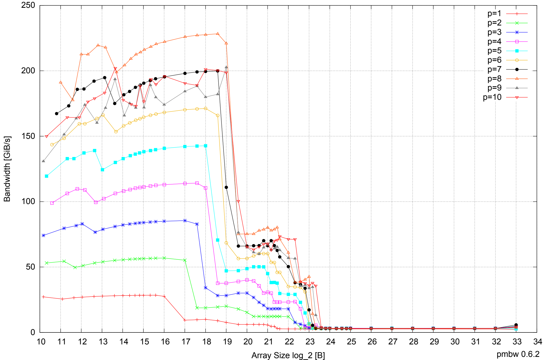
AMD Opteron 2350 16GB - Parallel Memory Bandwidth - ScanWrite64PtrUnrollLoop
