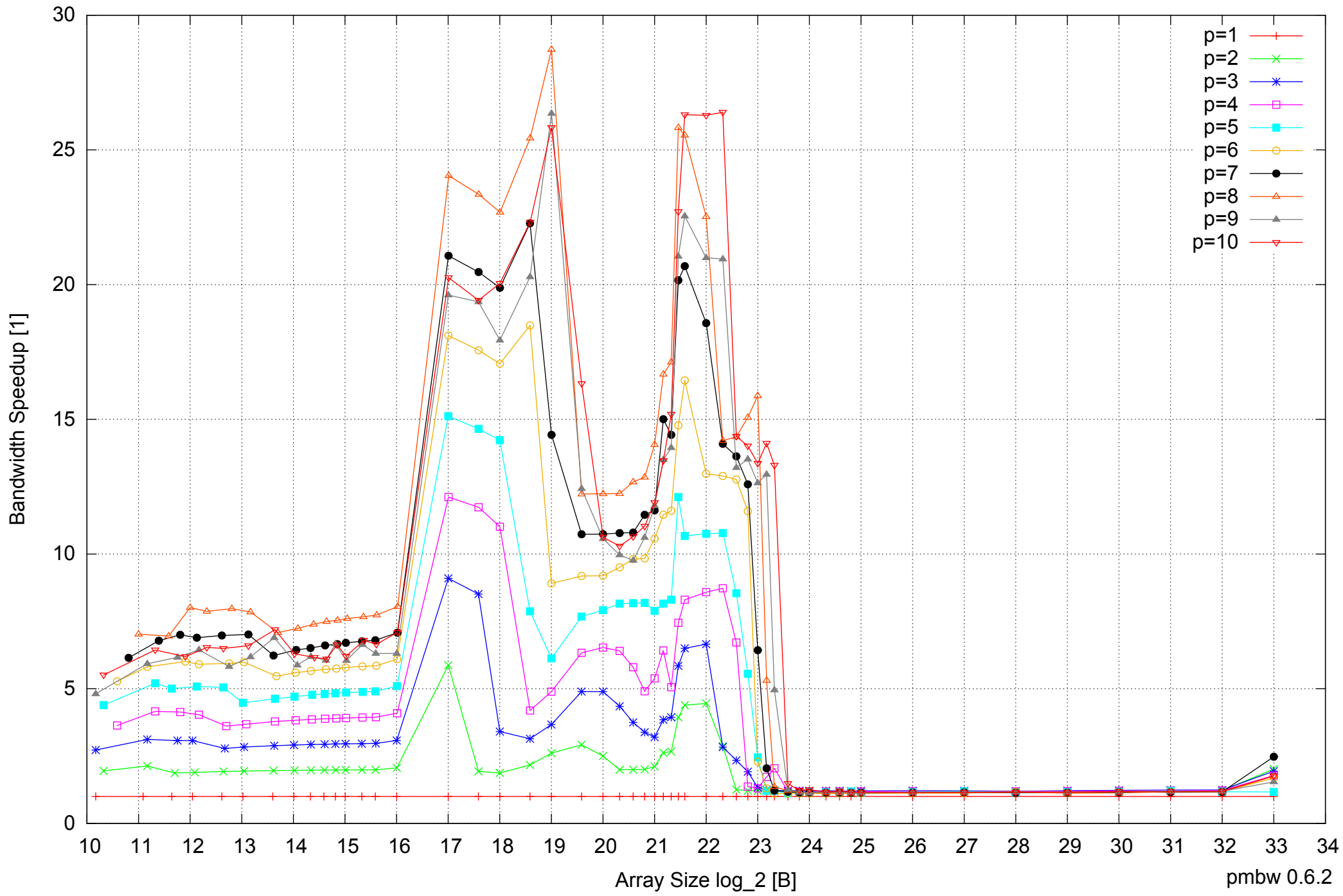
AMD Opteron 2350 16GB - Speedup of Parallel Memory Bandwidth - ScanWrite64PtrUnrollLoop
