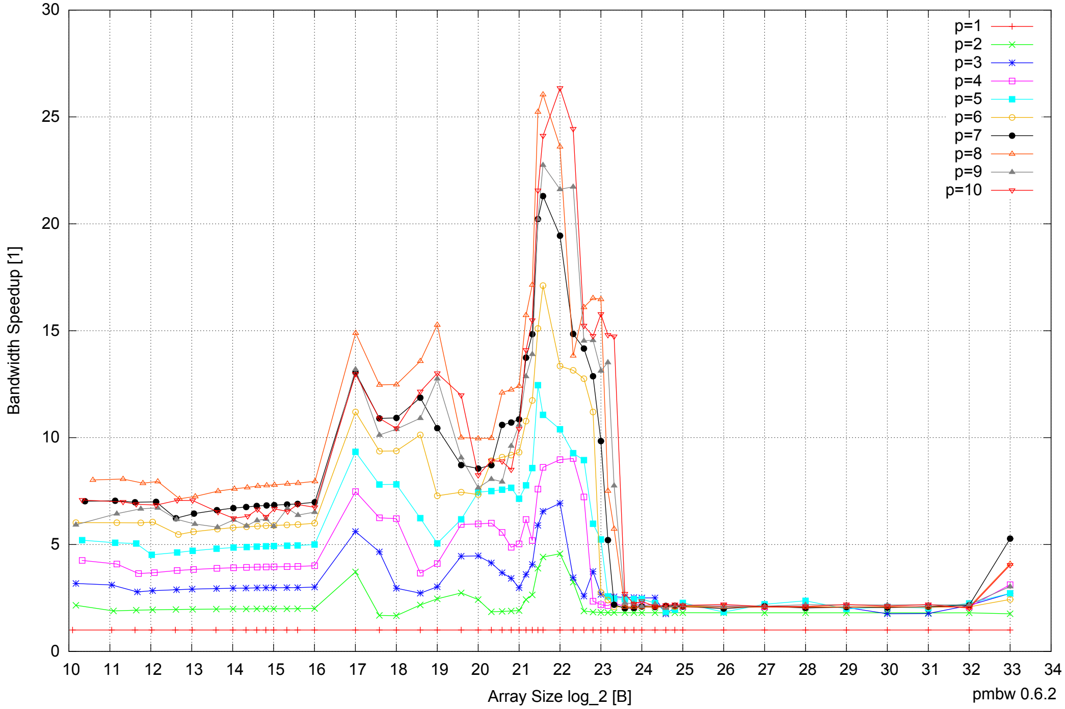
AMD Opteron 2350 16GB - Speedup of Parallel Memory Bandwidth - ScanRead32PtrUnrollLoop
