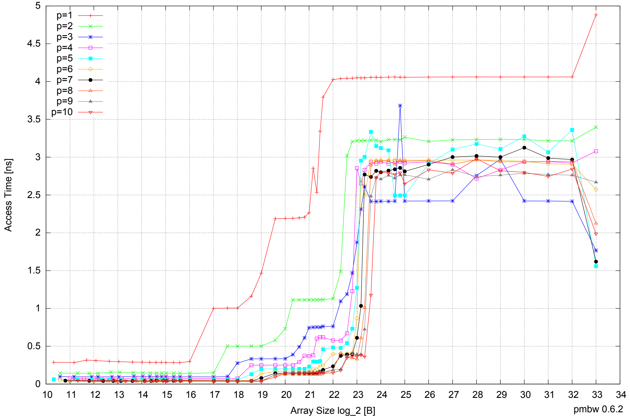
AMD Opteron 2350 16GB - Parallel Memory Access Time - ScanRead128PtrUnrollLoop
