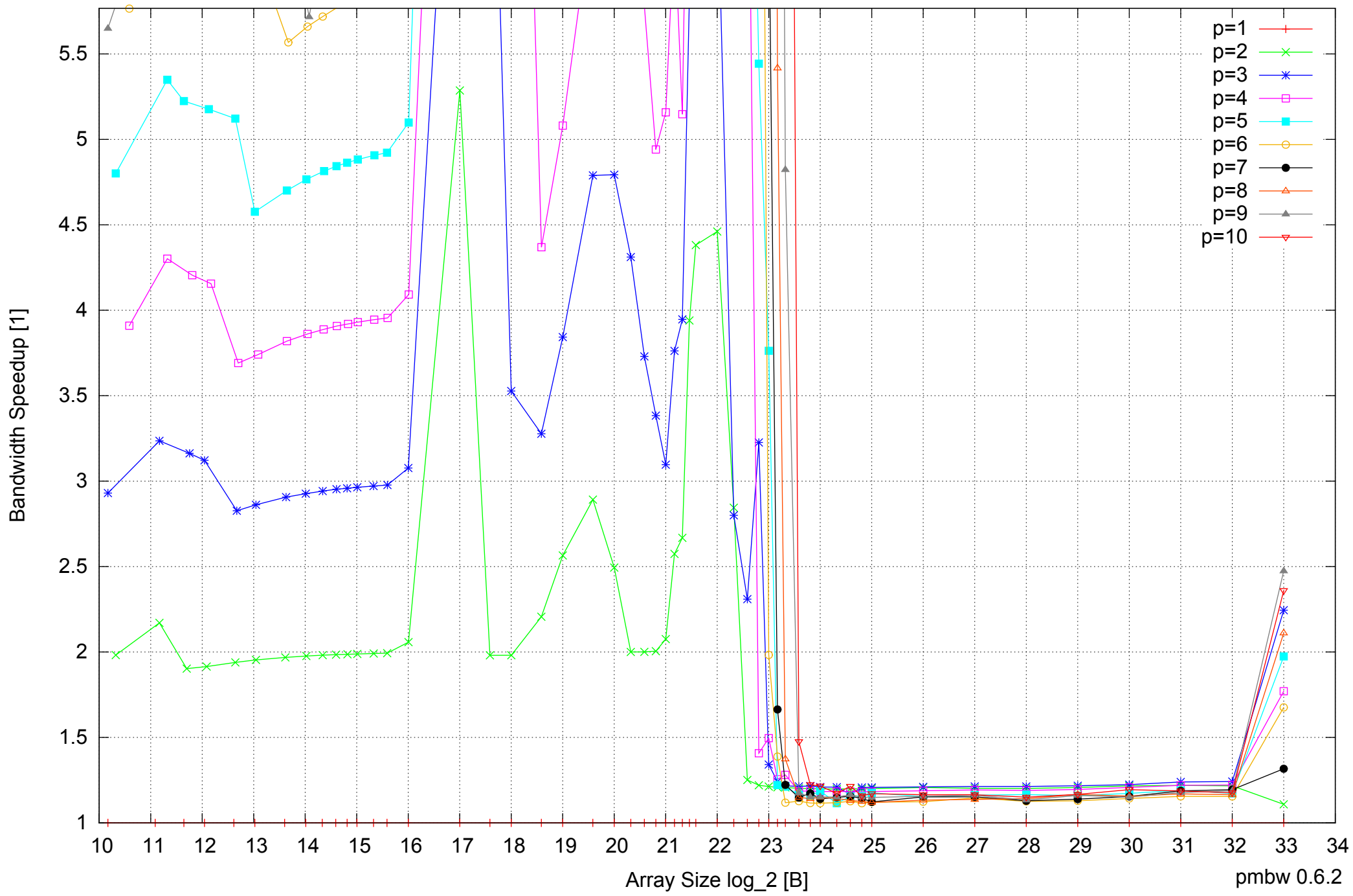
AMD Opteron 2350 16GB - Speedup of Parallel Memory Bandwidth (enlarged) - ScanWrite64IndexUnrollLoop
