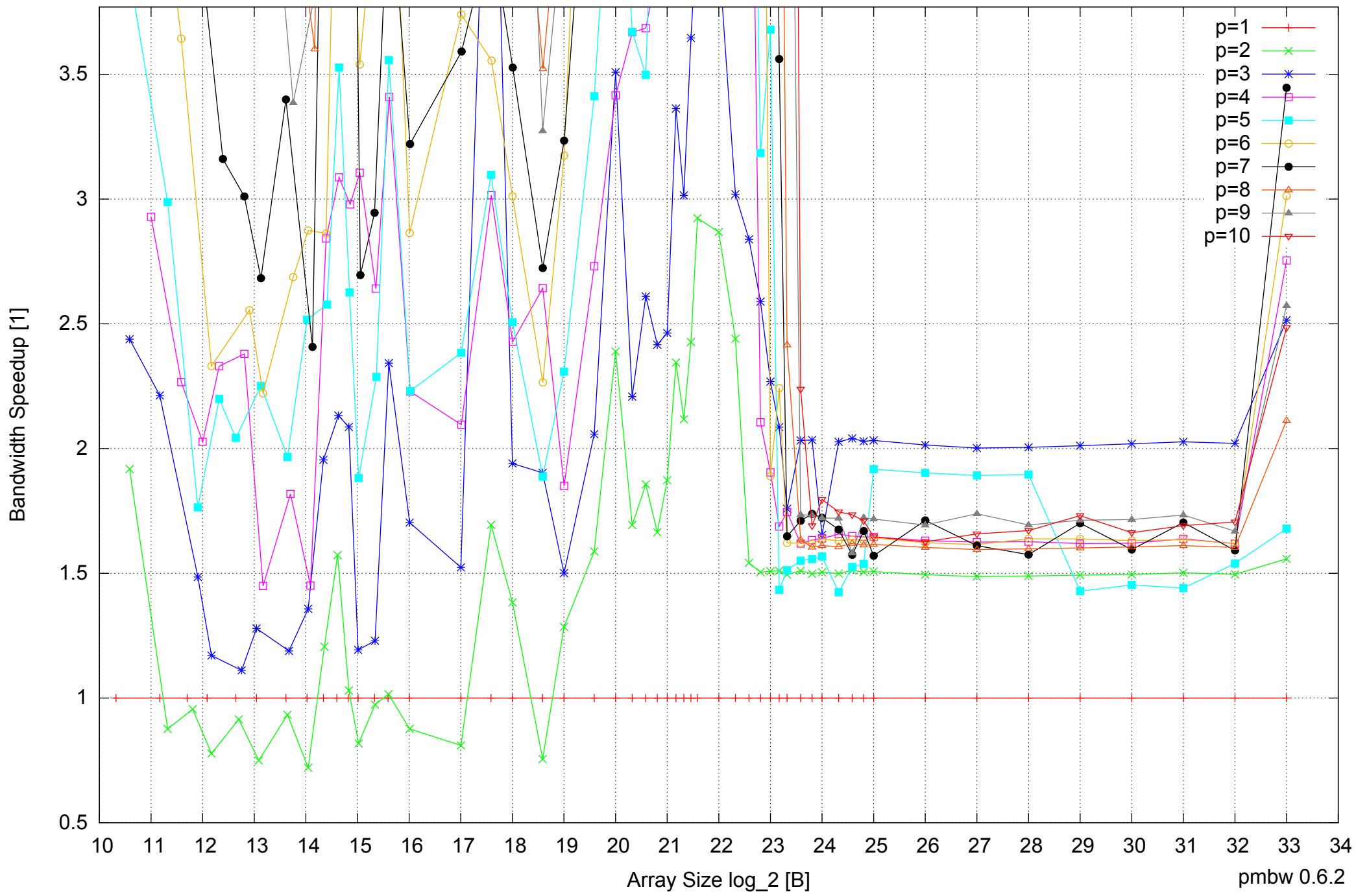
AMD Opteron 2350 16GB - Speedup of Parallel Memory Bandwidth (enlarged) - ScanRead128PtrSimpleLoop
