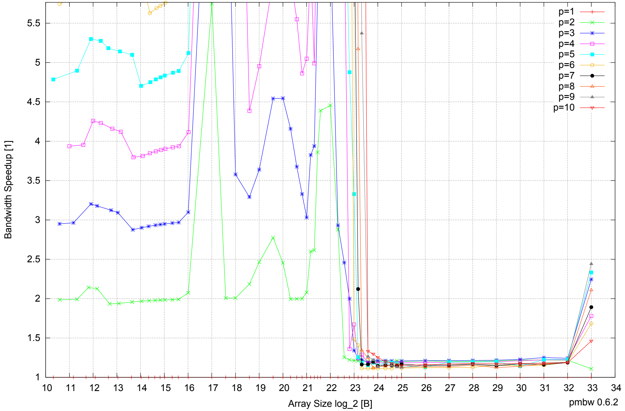
AMD Optron 2350 16GB - Speedup of Parallel Memory Bandwidth (enlarged) - ScanWrite128PtrUnrollLoop
