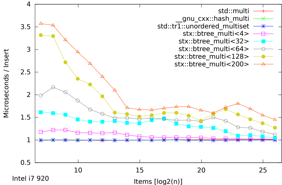
Speed Test - Ratio Multiset / Multimap - Find Only (125-65536000 Items)
