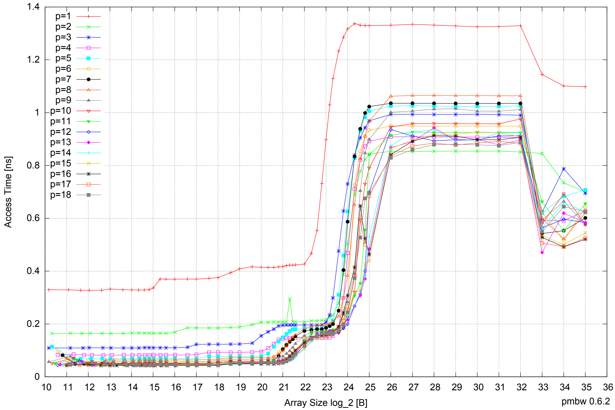
Intel Xeon X5550 48GB - Parallel Memory Access Time - ScanWrite64IndexUnrollLoop
