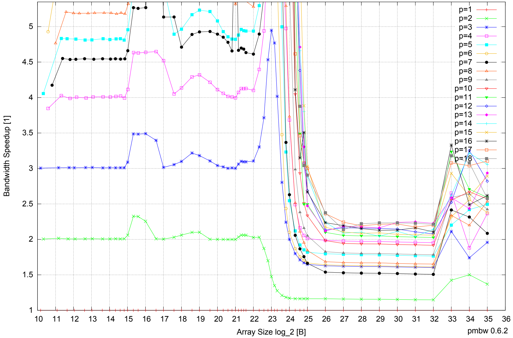
Intel Xeon X5550 48GB - Speedup of Parallel Memory Bandwidth (enlarged) - ScanRead64PtrUnrollLoop
