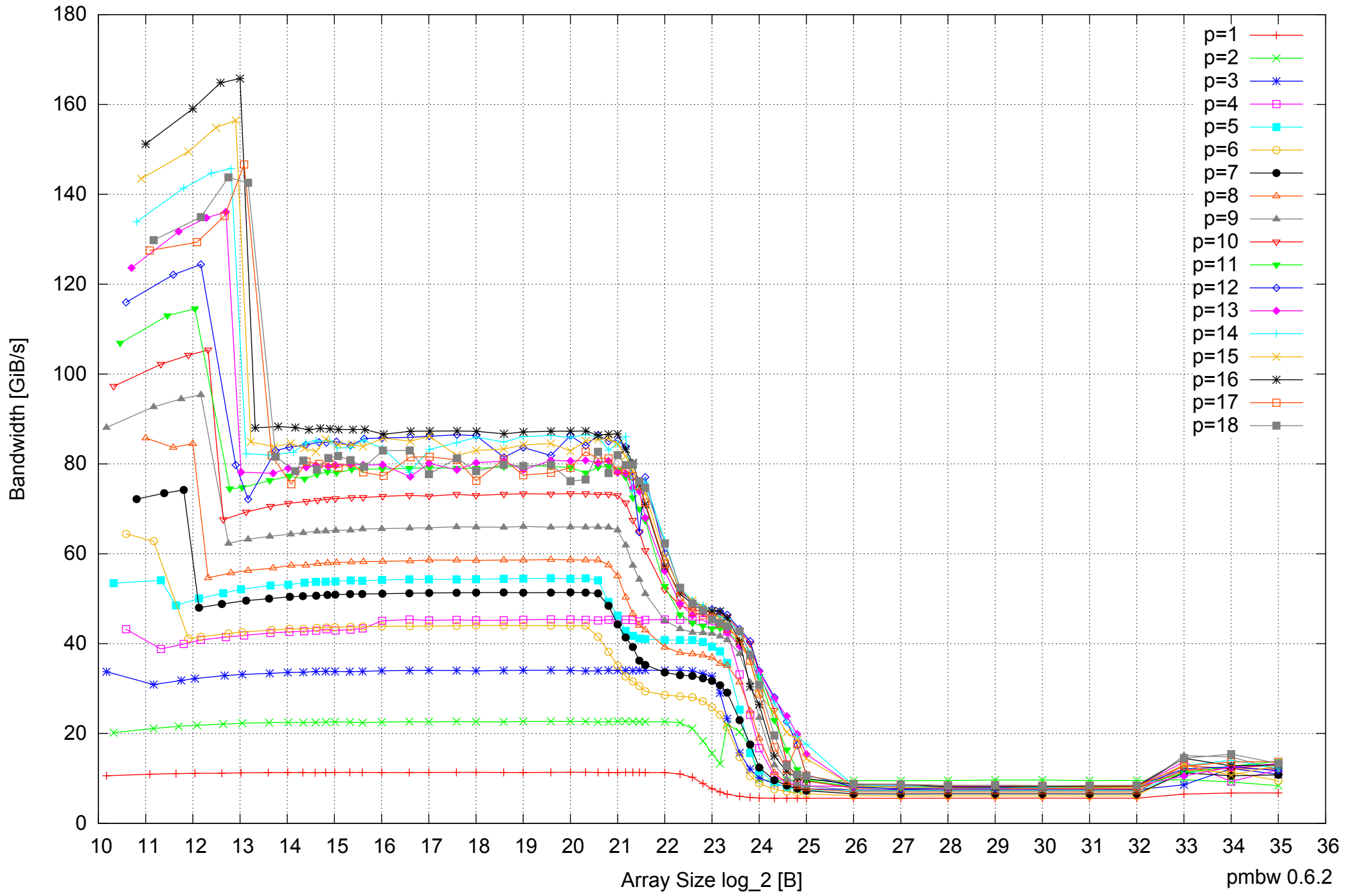
Intel Xeon X5550 48GB - Parallel Memory Bandwidth - ScanWrite64PtrSimpleLoop
