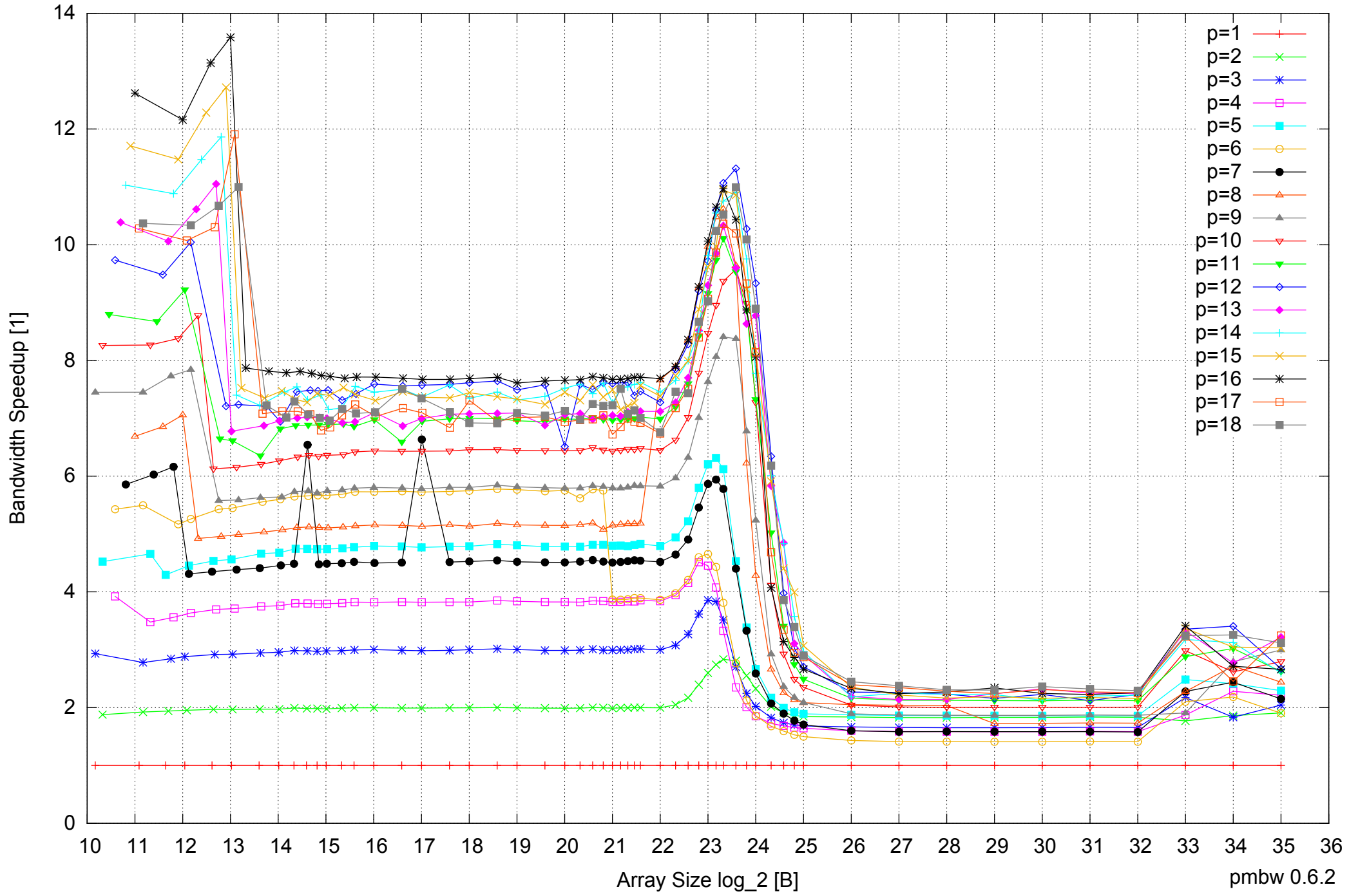
Intel Xeon X5550 48GB - Speedup of Parallel Memory Bandwidth - ScanRead64IndexSimpleLoop
