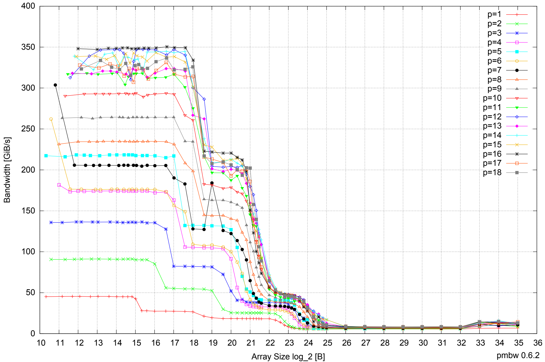
Intel Xeon X5550 48GB - Parallel Memory Bandwidth - ScanWrite128PtrUnrollLoop
