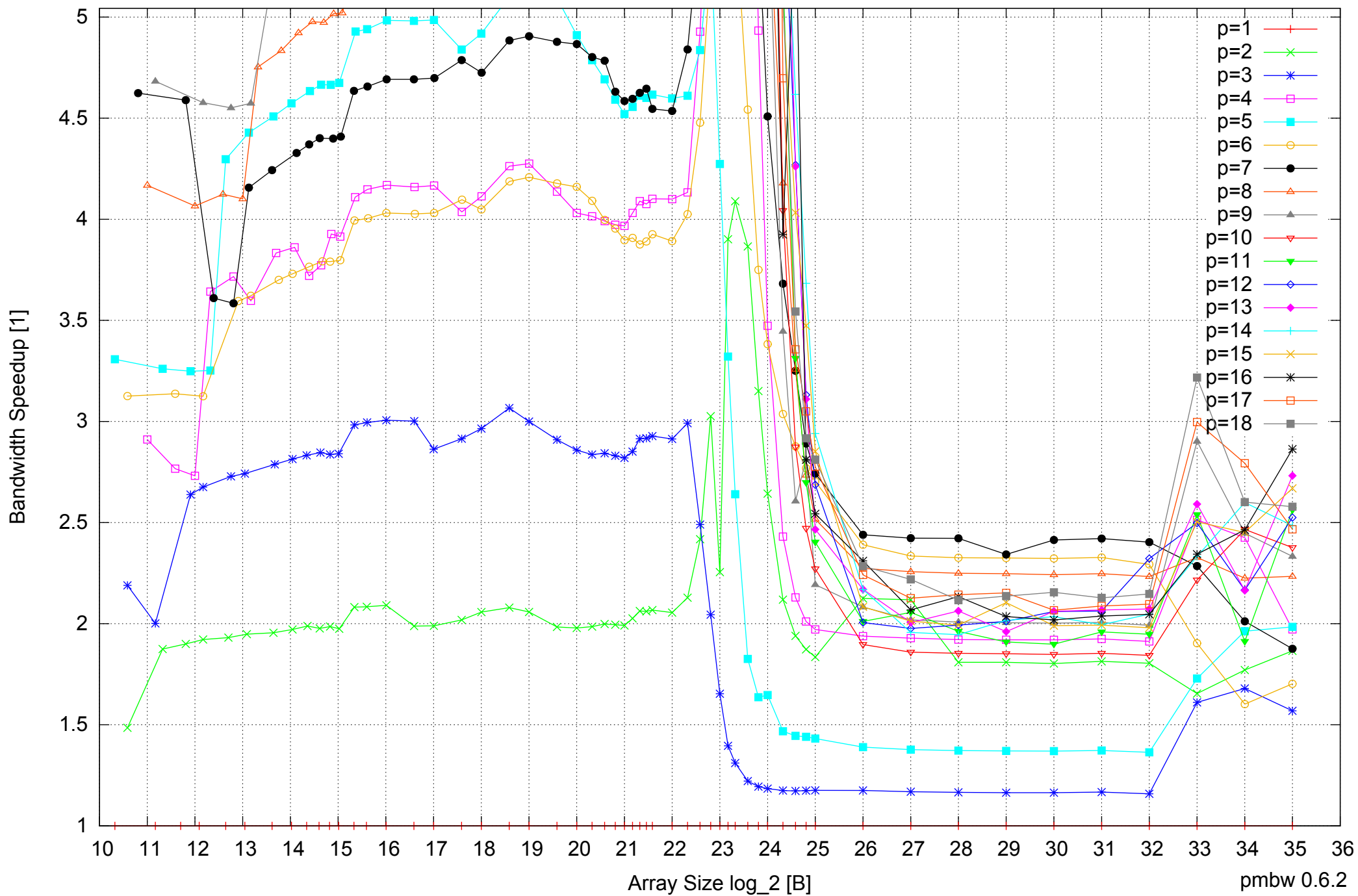
Intel Xeon X5550 48GB - Speedup of Parallel Memory Bandwidth (enlarged) - ScanRead128PtrSimpleLoop
