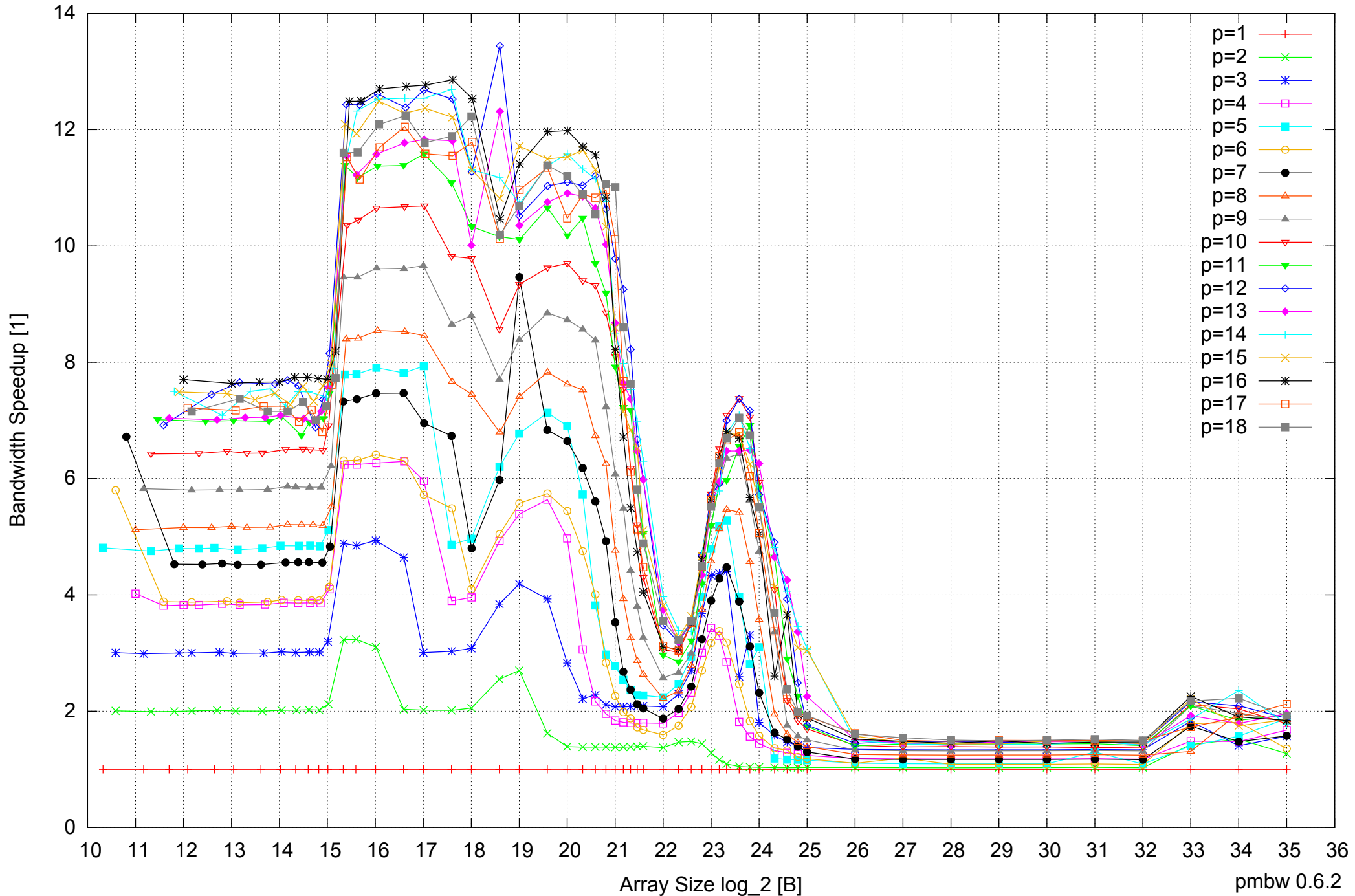
Intel Xeon X5550 48GB - Speedup of Parallel Memory Bandwidth - ScanWrite128PtrUnrollLoop
