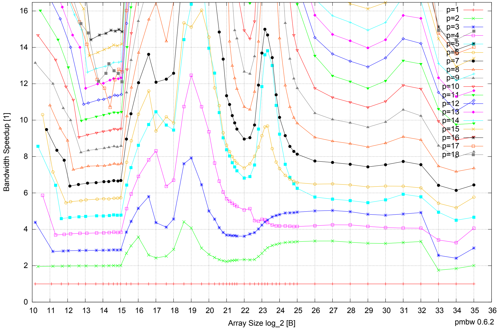
Intel Xeon X5550 48GB - Speedup of Parallel Memory Bandwidth (enlarged) - PermRead64SimpleLoop
