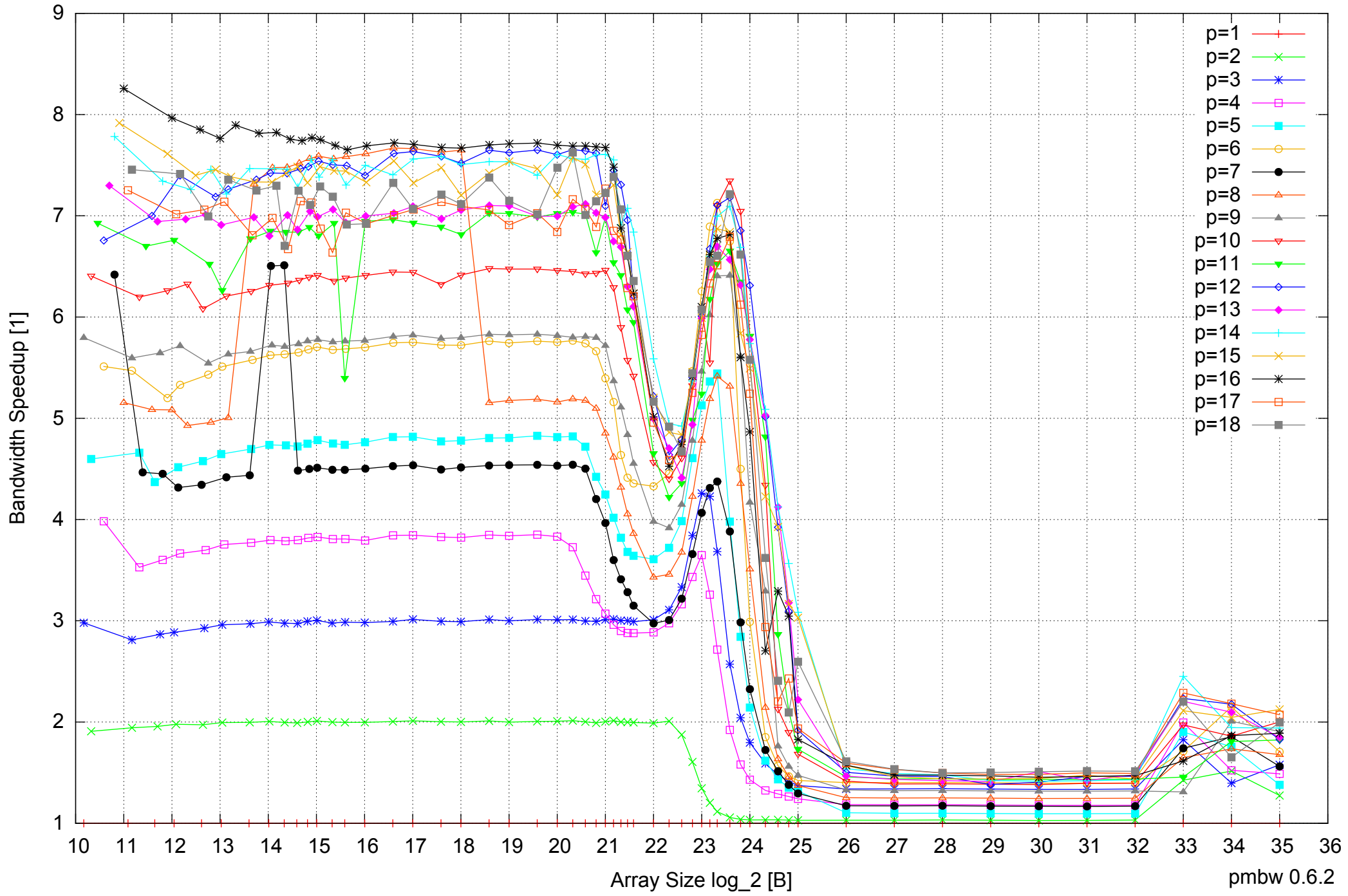
Intel Xeon X5550 48GB - Speedup of Parallel Memory Bandwidth - ScanWrite64IndexSimpleLoop
