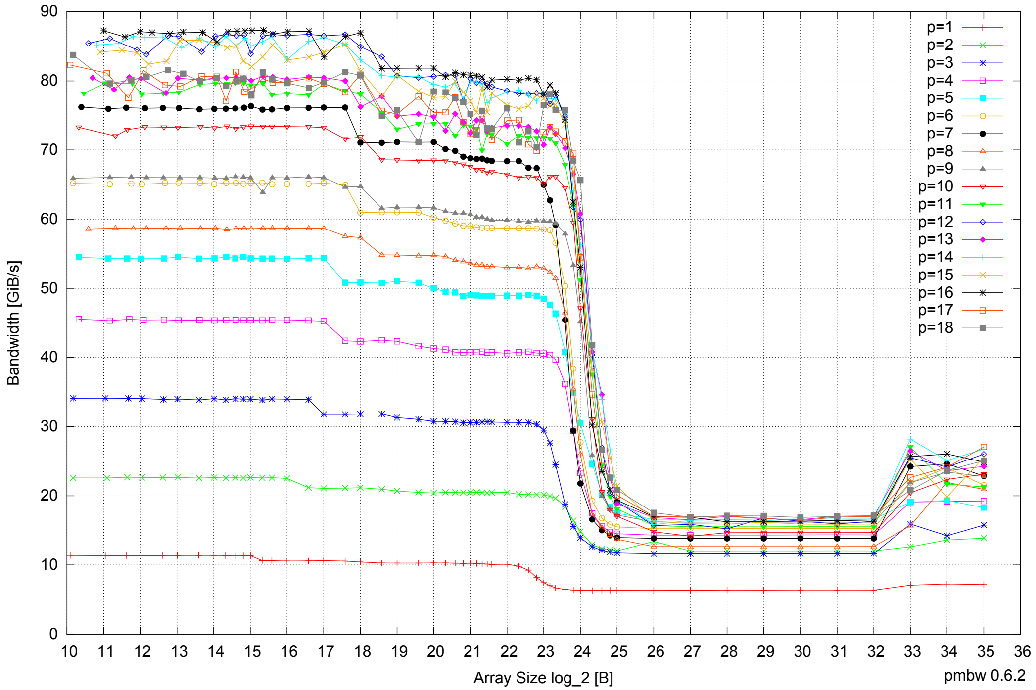
Intel Xeon X5550 48GB - Parallel Memory Bandwidth - ScanRead32PtrUnrollLoop
