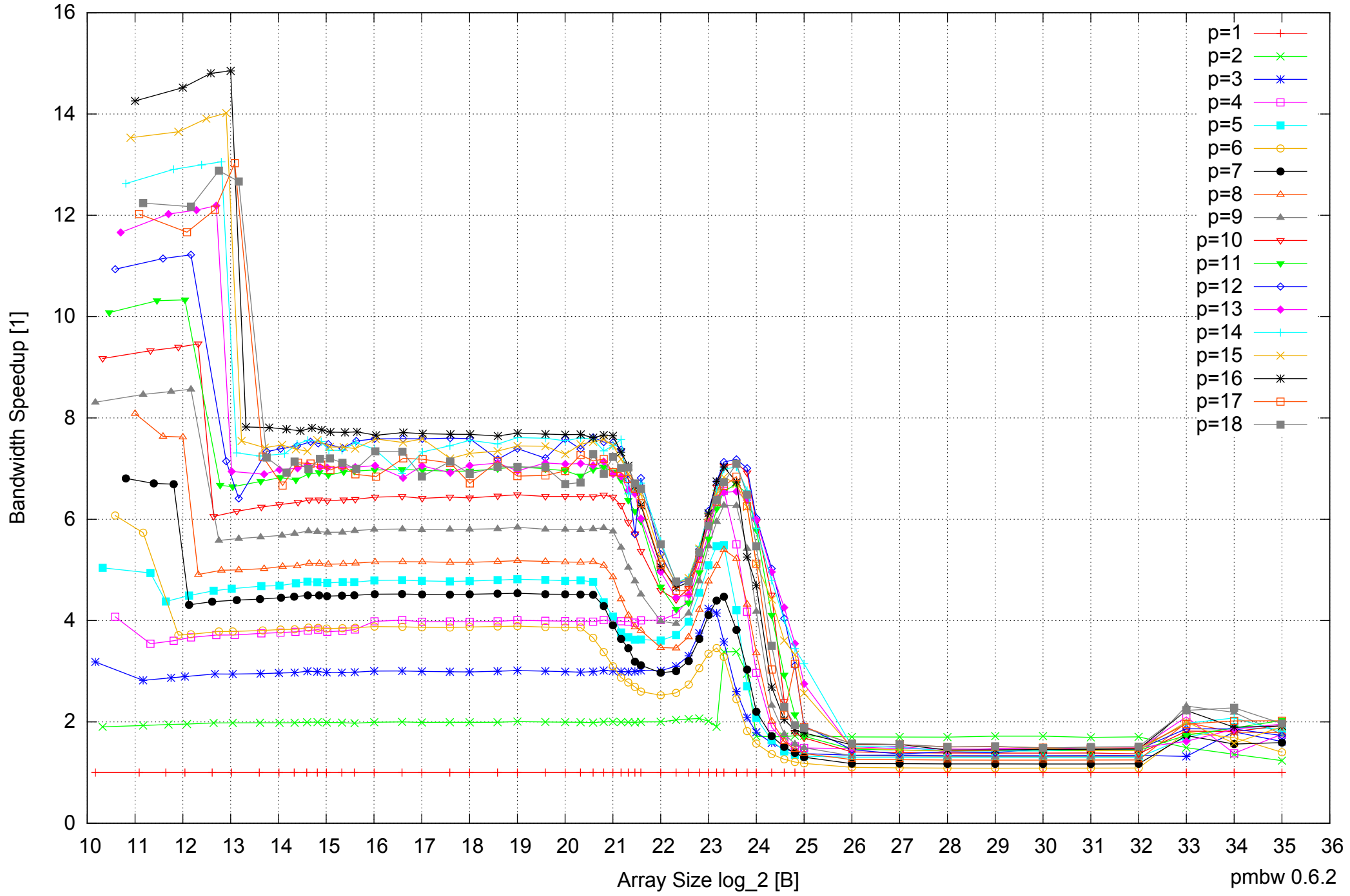
Intel Xeon X5550 48GB - Speedup of Parallel Memory Bandwidth - ScanWrite64PtrSimpleLoop
