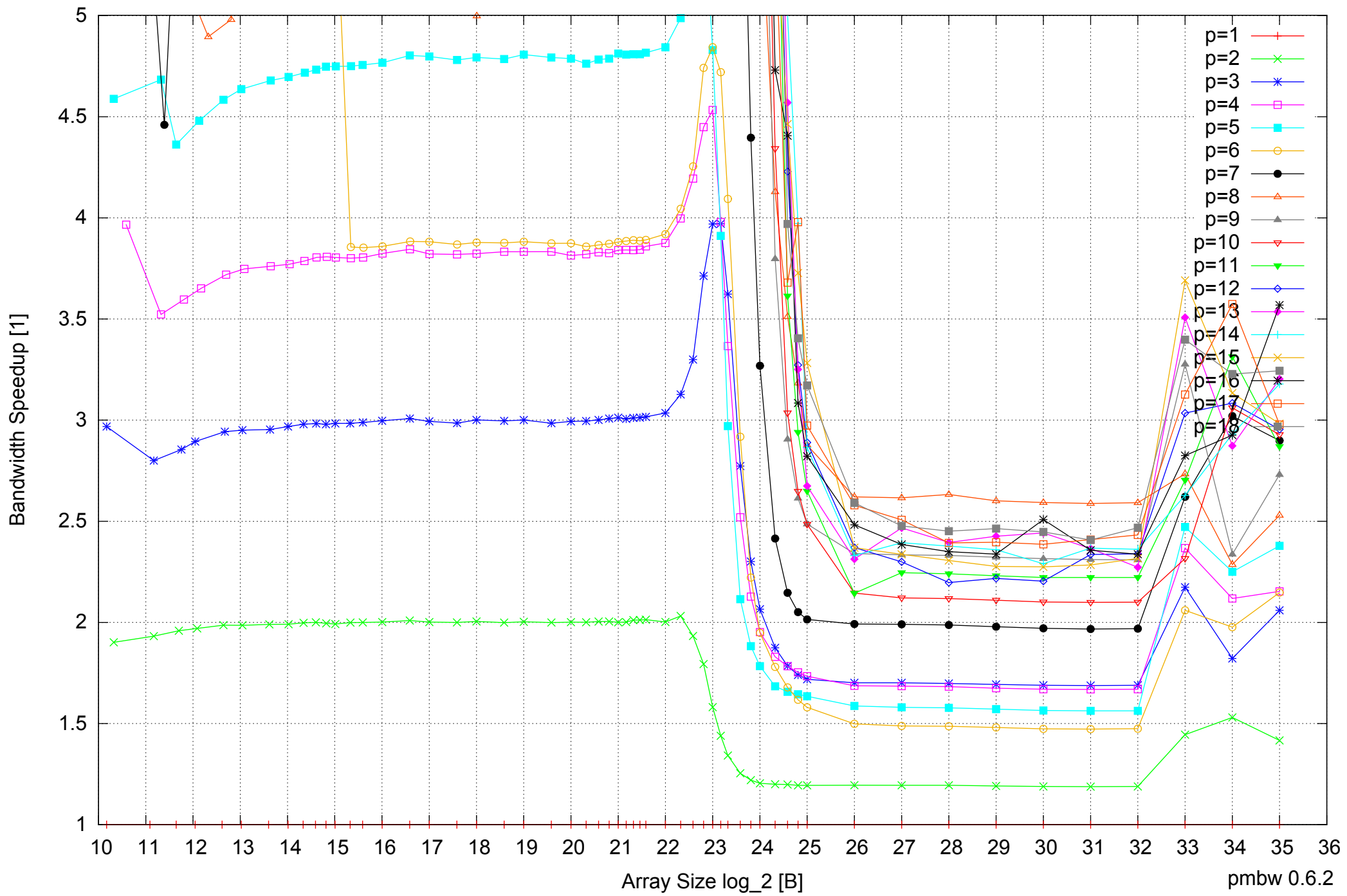
Intel Xeon X5550 48GB - Speedup of Parallel Memory Bandwidth (enlarged) - ScanRead64PtrSimpleLoop
