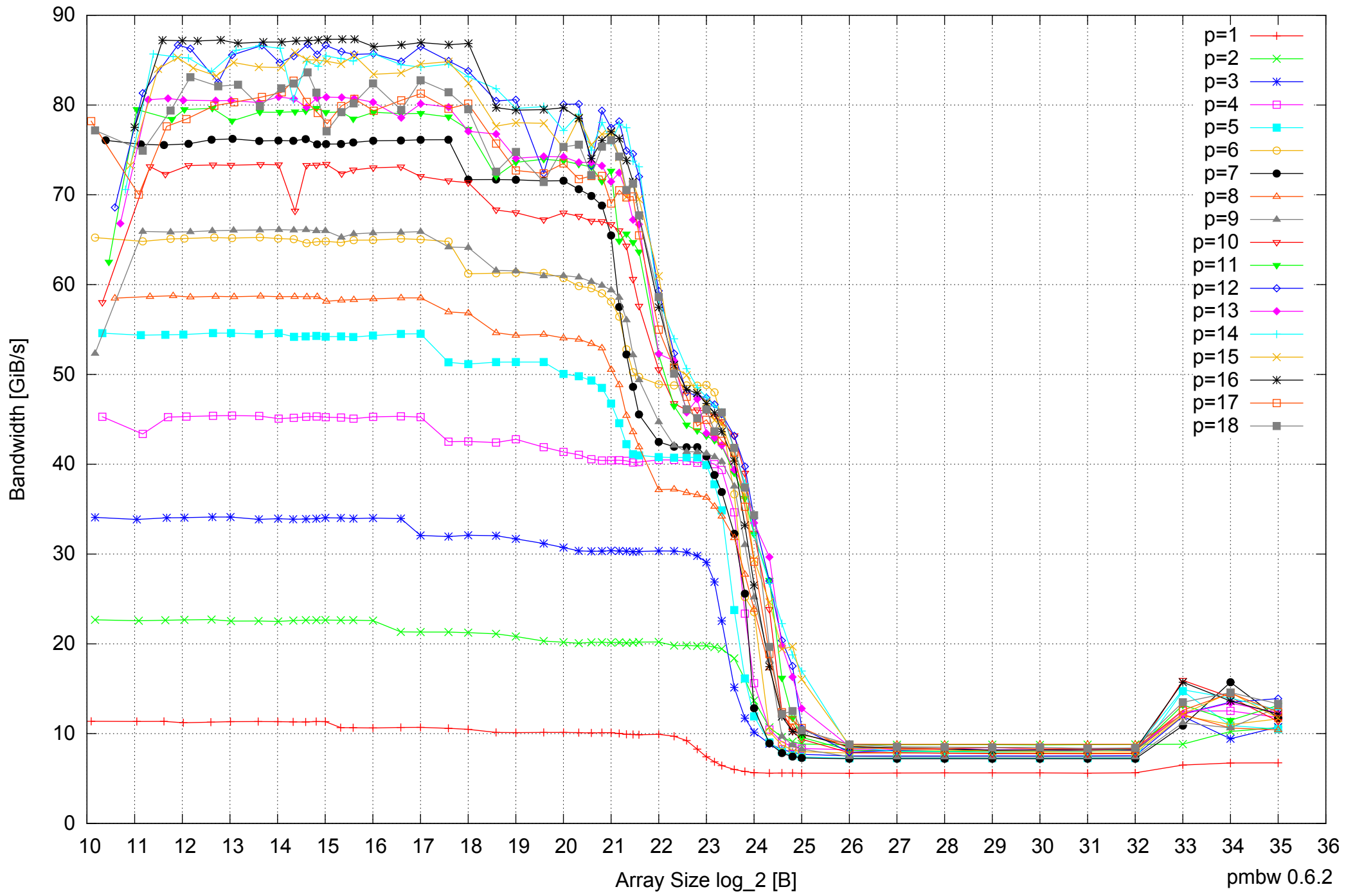
Intel Xeon X5550 48GB - Parallel Memory Bandwidth - ScanWrite32PtrUnrollLoop
