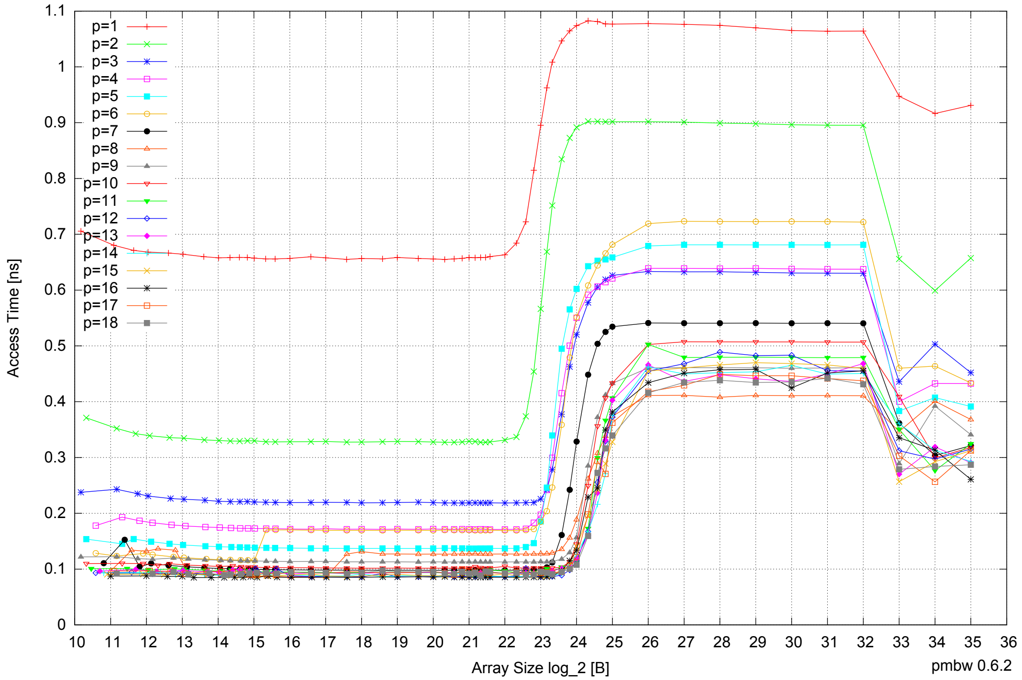
Intel Xeon X5550 48GB - Parallel Memory Access Time - ScanRead64PtrSimpleLoop
