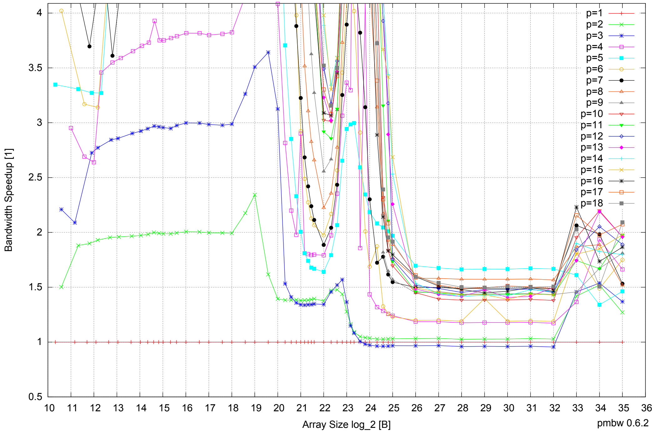
Intel Xeon X5550 48GB - Speedup of Parallel Memory Bandwidth (enlarged) - ScanWrite128PtrSimpleLoop
