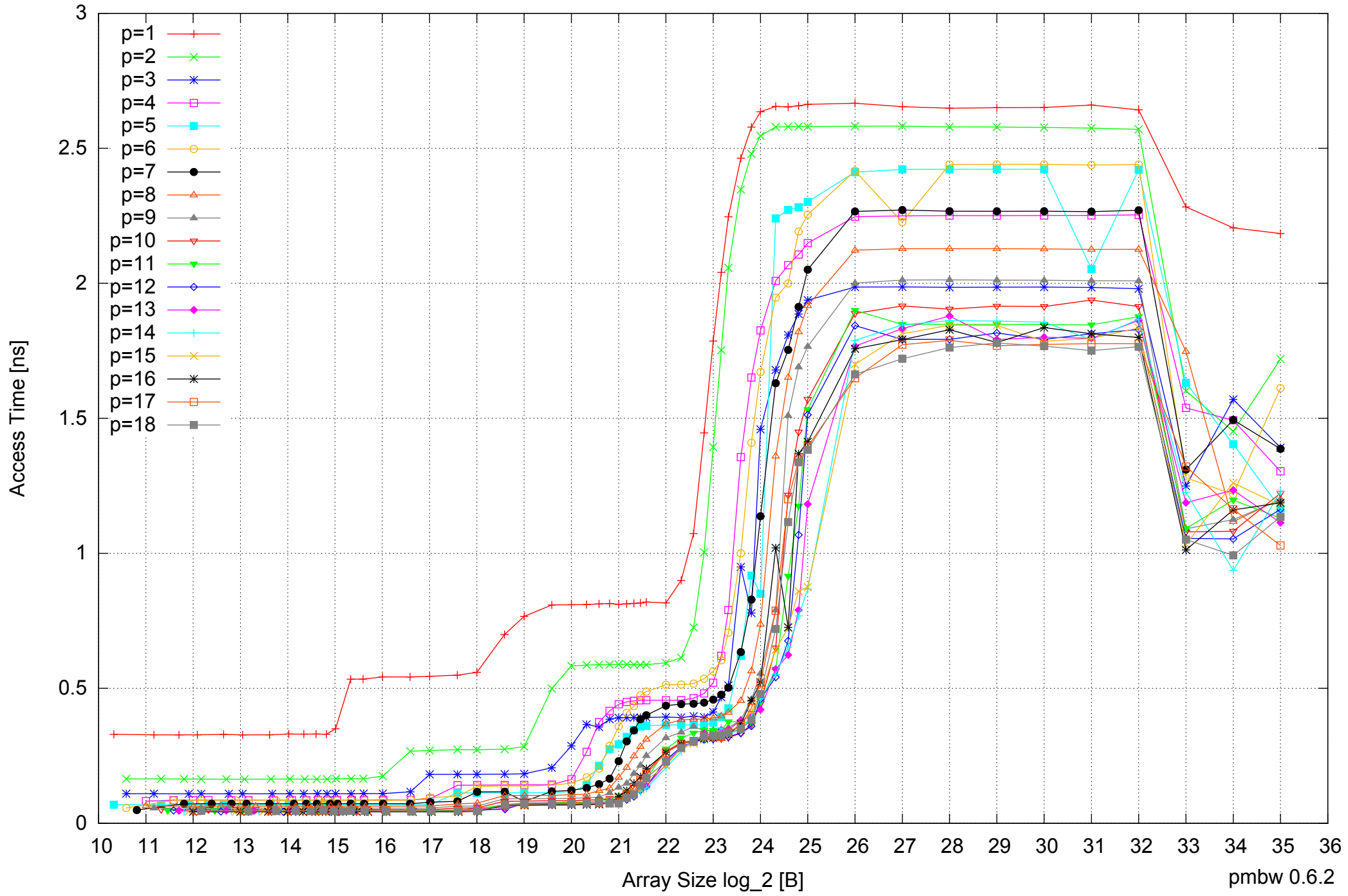
Intel Xeon X5550 48GB - Parallel Memory Access Time - ScanWrite128PtrUnrollLoop
