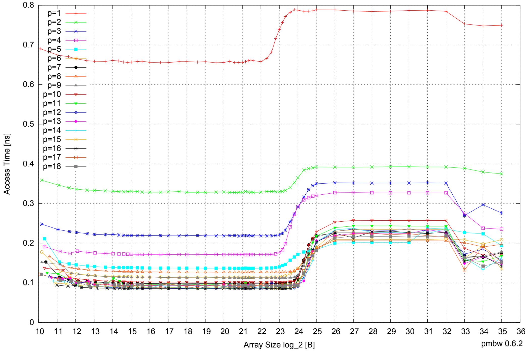
Intel Xeon X5550 48GB - Parallel Memory Access Time - ScanRead32PtrSimpleLoop
