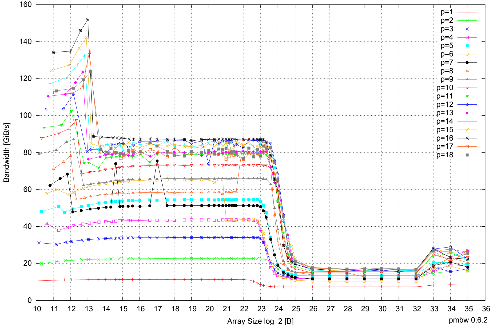
Intel Xeon X5550 48GB - Parallel Memory Bandwidth - ScanRead64IndexSimpleLoop
