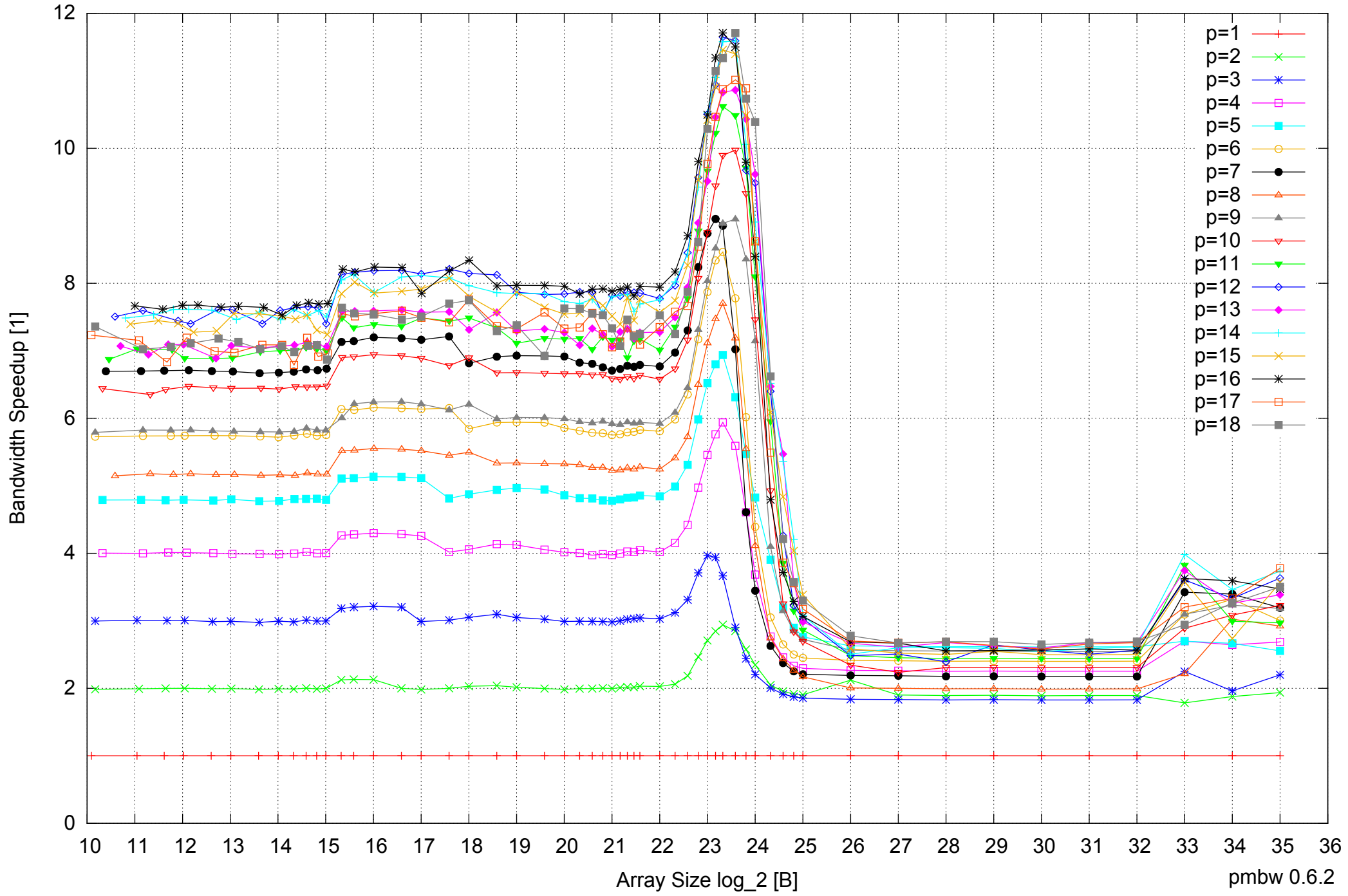
Intel Xeon X5550 48GB - Speedup of Parallel Memory Bandwidth - ScanRead32PtrUnrollLoop
