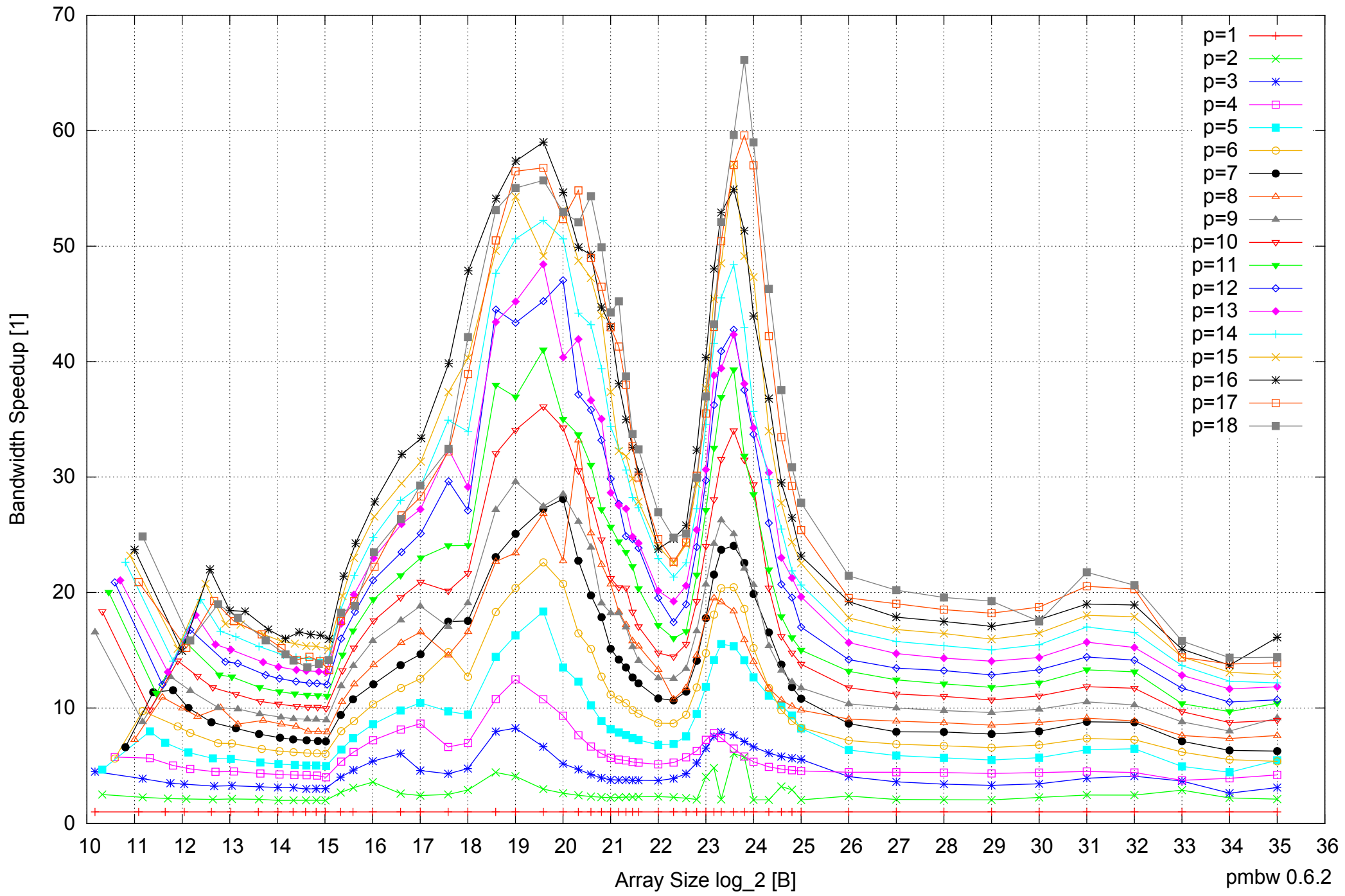
Intel Xeon X5550 48GB - Speedup of Parallel Memory Bandwidth - PermRead64UnrollLoop
