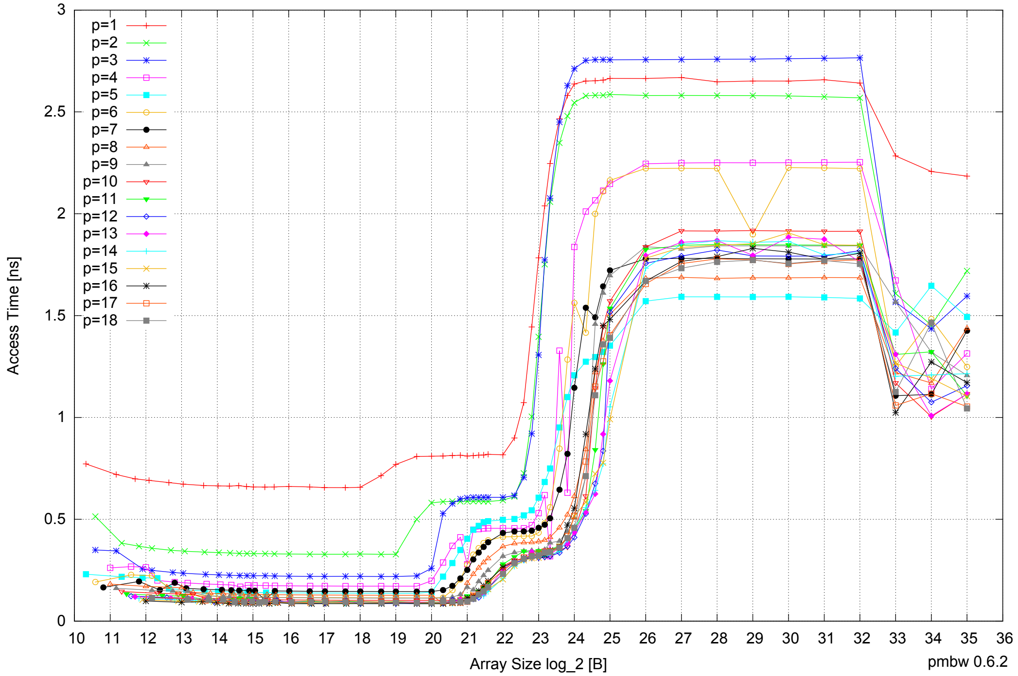
Intel Xeon X5550 48GB - Parallel Memory Access Time - ScanWrite128PtrSimpleLoop
