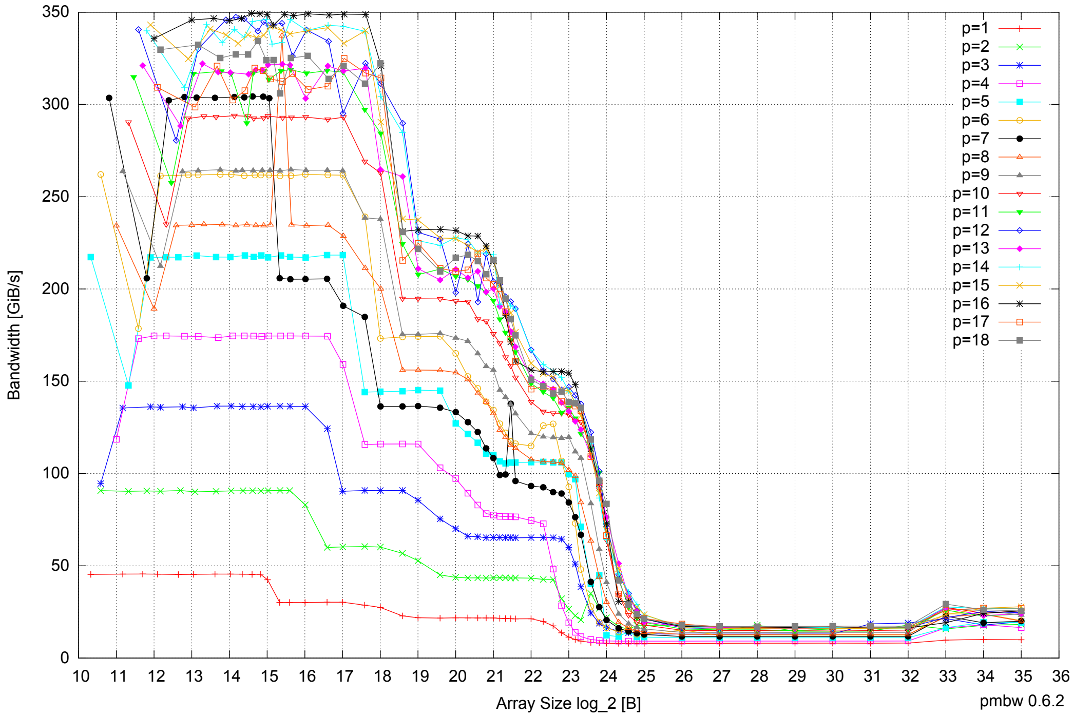
Intel Xeon X5550 48GB - Parallel Memory Bandwidth - ScanRead128PtrUnrollLoop
