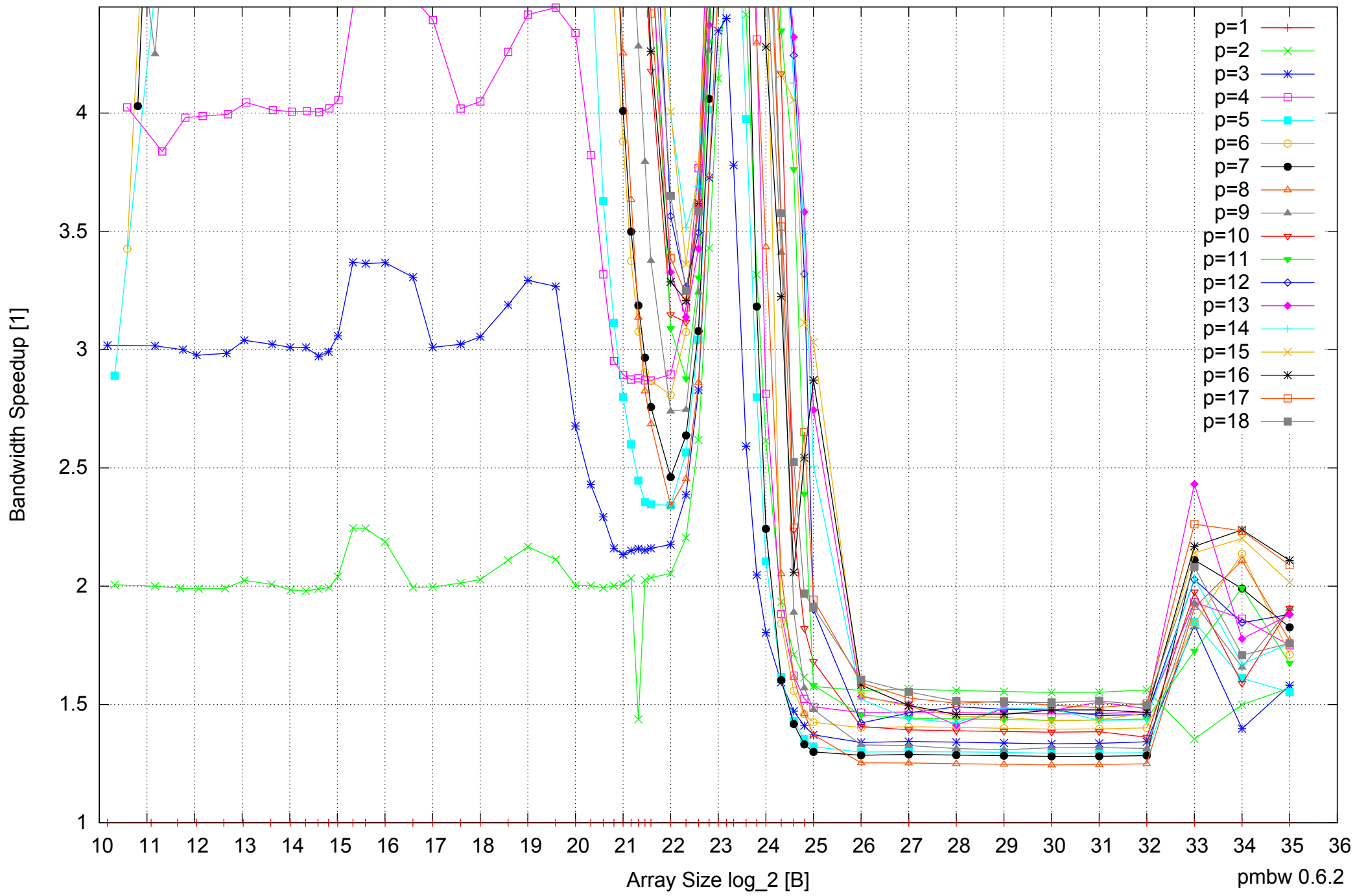
Intel Xeon X5550 48GB - Speedup of Parallel Memory Bandwidth (enlarged) - ScanWrite64IndexUnrollLoop
