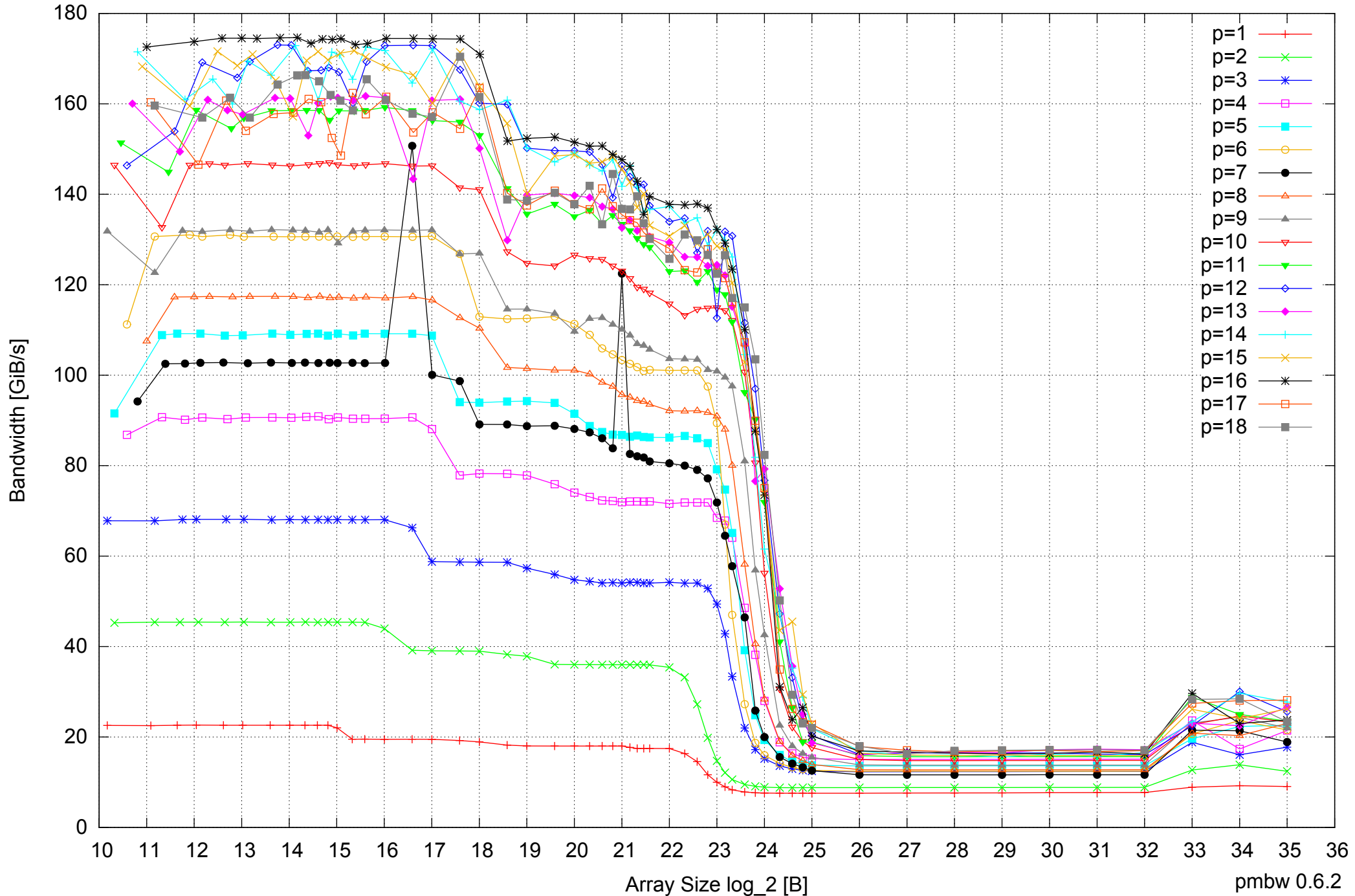
Intel Xeon X5550 48GB - Parallel Memory Bandwidth - ScanRead64PtrUnrollLoop
