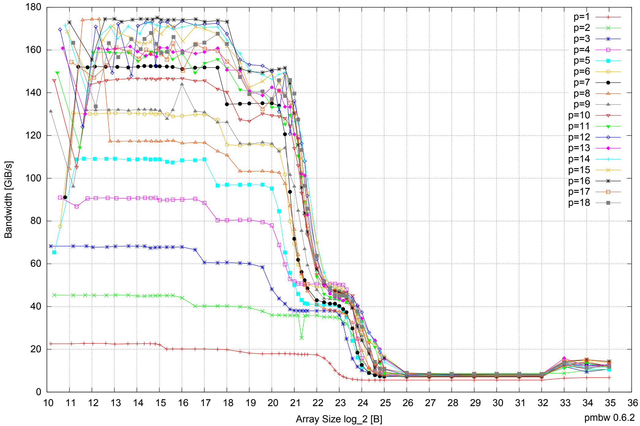
Intel Xeon X5550 48GB - Parallel Memory Bandwidth - ScanWrite64IndexUnrollLoop
