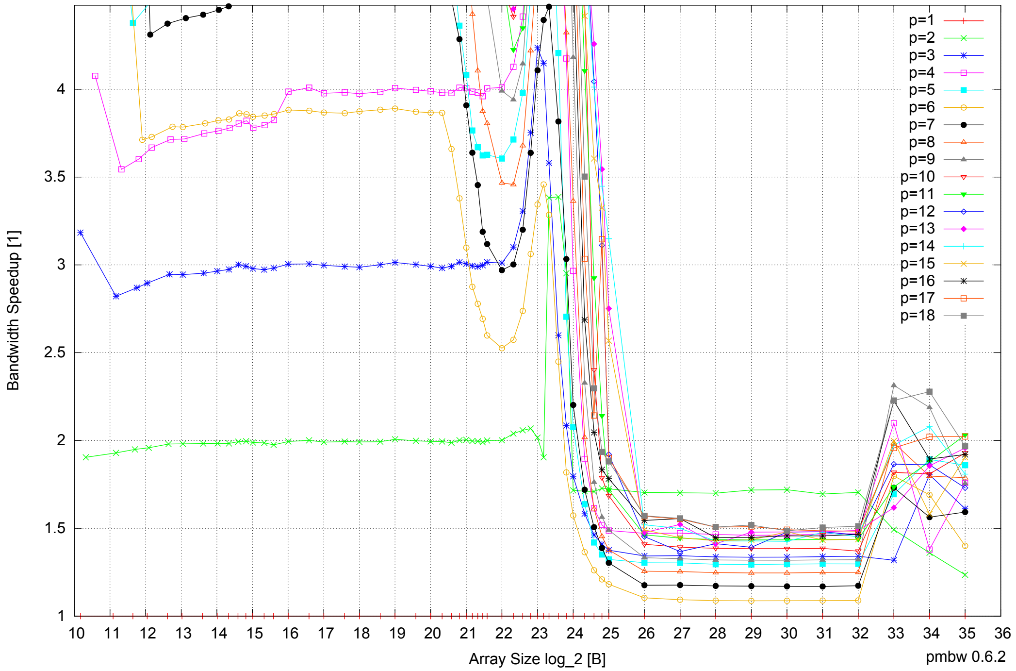
Intel Xeon X5550 48GB - Speedup of Parallel Memory Bandwidth (enlarged) - ScanWrite64PtrSimpleLoop
