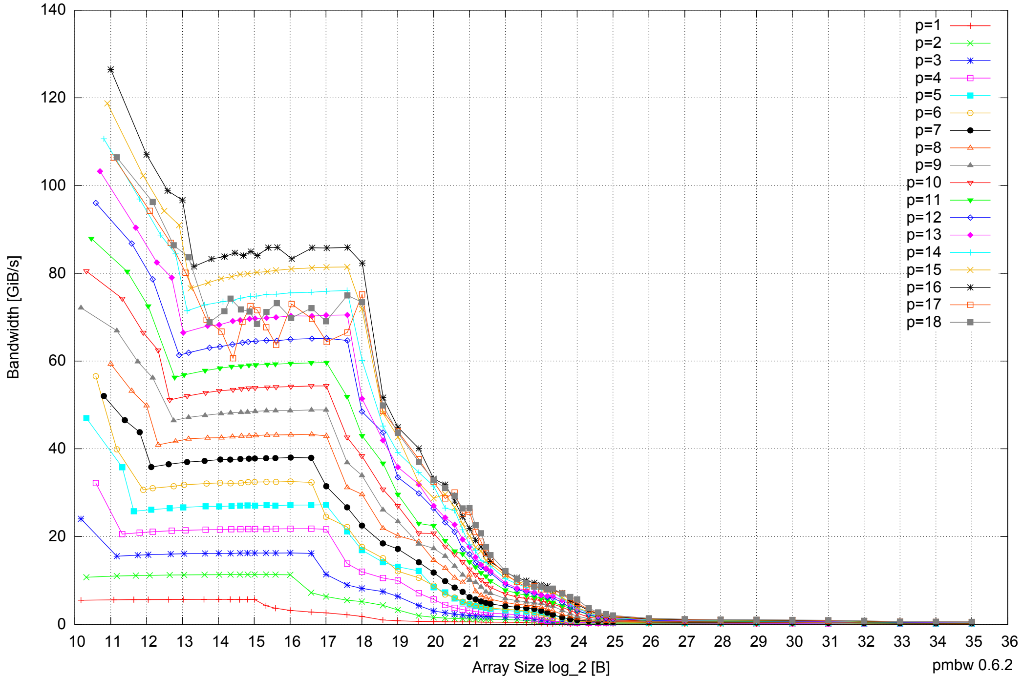
Intel Xeon X5550 48GB - Parallel Memory Bandwidth - PermRead64SimpleLoop
