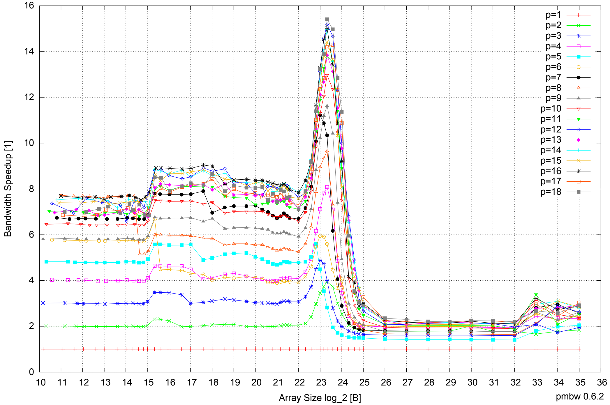
Intel Xeon X5550 48GB - Speedup of Parallel Memory Bandwidth - ScanRead64IndexUnrollLoop
