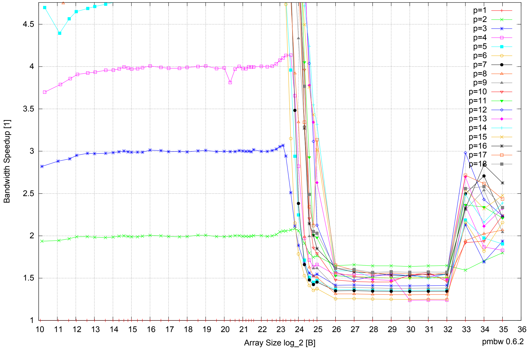
Intel Xeon X5550 48GB - Speedup of Parallel Memory Bandwidth (enlarged) - ScanWrite32PtrSimpleLoop
