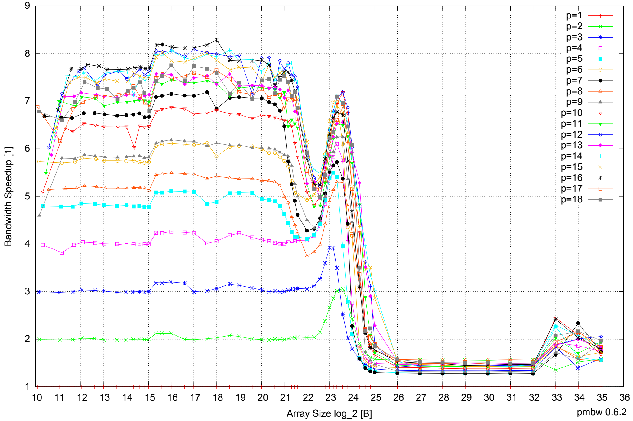
Intel Xeon X5550 48GB - Speedup of Parallel Memory Bandwidth - ScanWrite32PtrUnrollLoop
