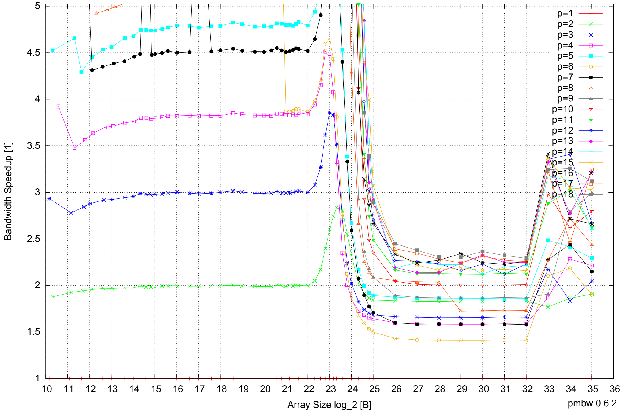
Intel Xeon X5550 48GB - Speedup of Parallel Memory Bandwidth (enlarged) - ScanRead64IndexSimpleLoop
