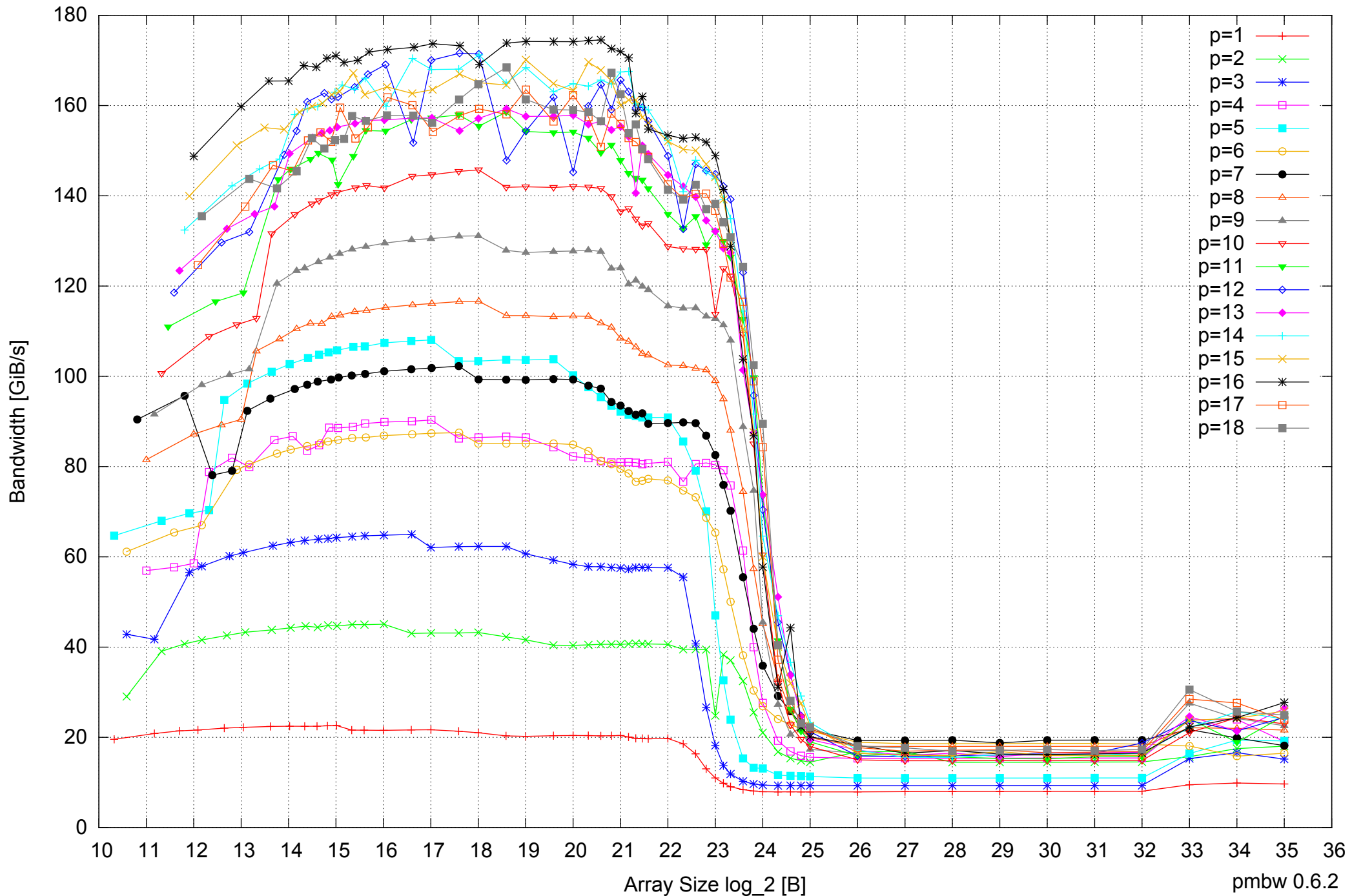
Intel Xeon X5550 48GB - Parallel Memory Bandwidth - ScanRead128PtrSimpleLoop
