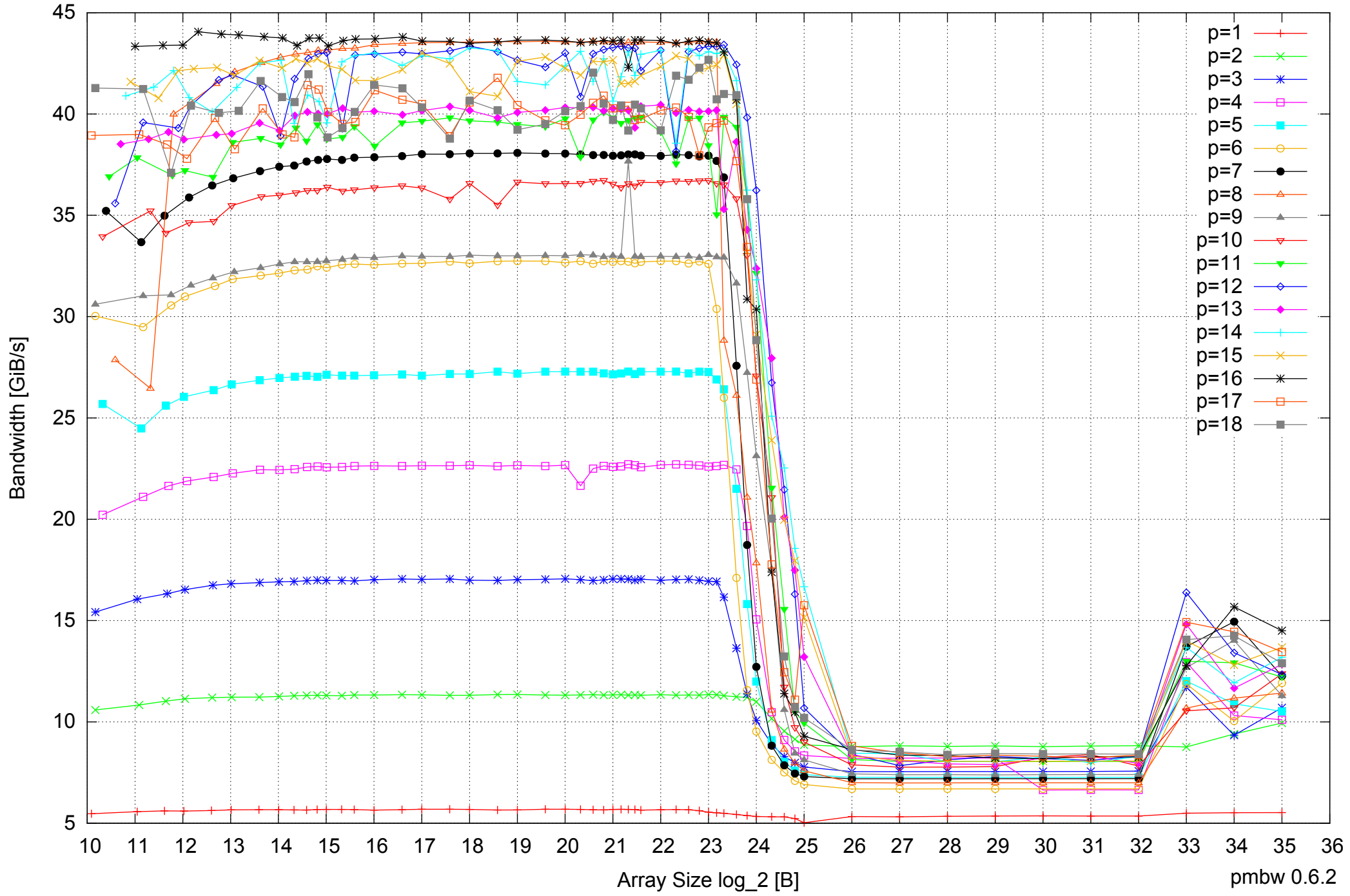
Intel Xeon X5550 48GB - Parallel Memory Bandwidth - ScanWrite32PtrSimpleLoop
