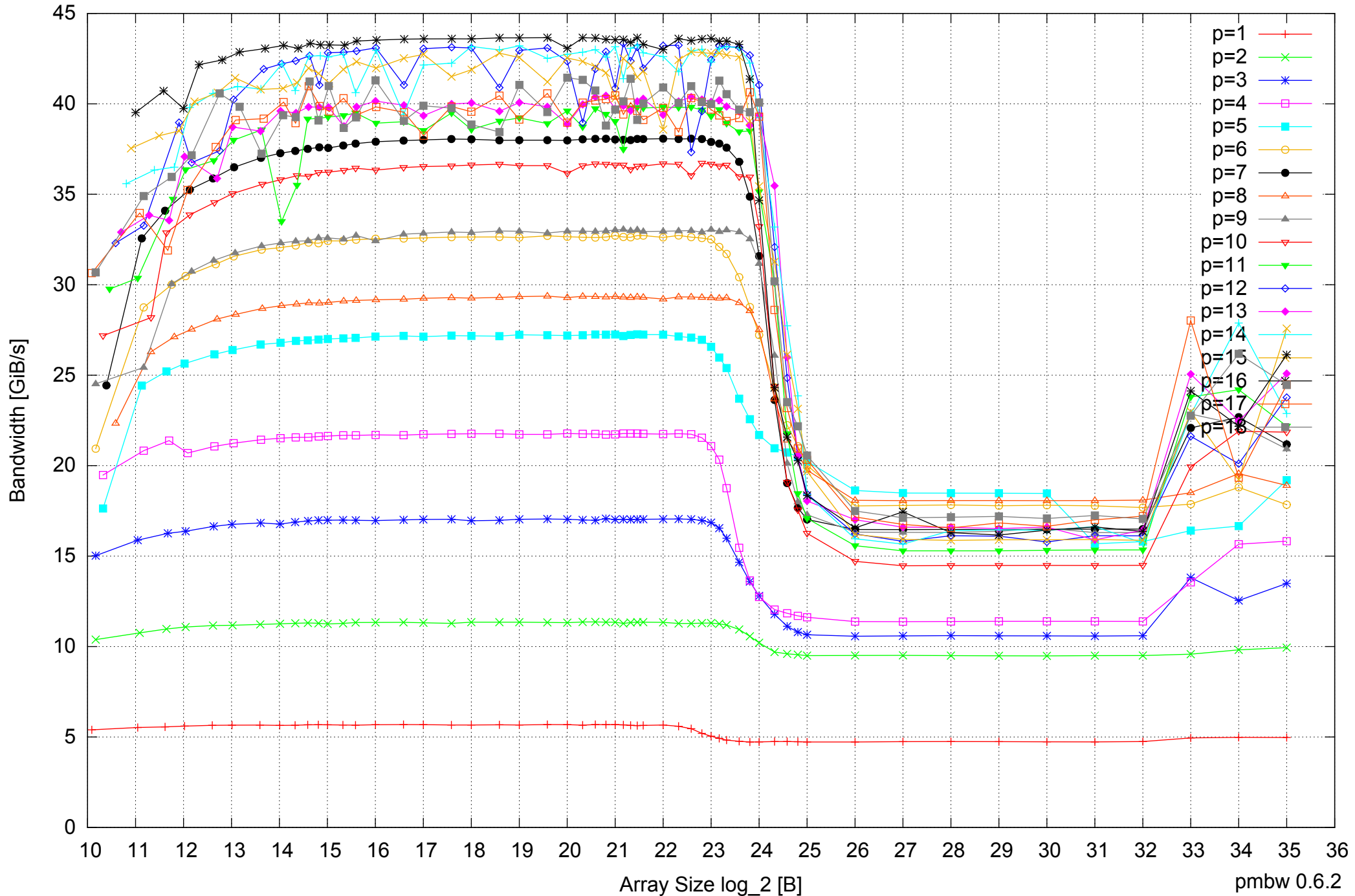
Intel Xeon X5550 48GB - Parallel Memory Bandwidth - ScanRead32PtrSimpleLoop
