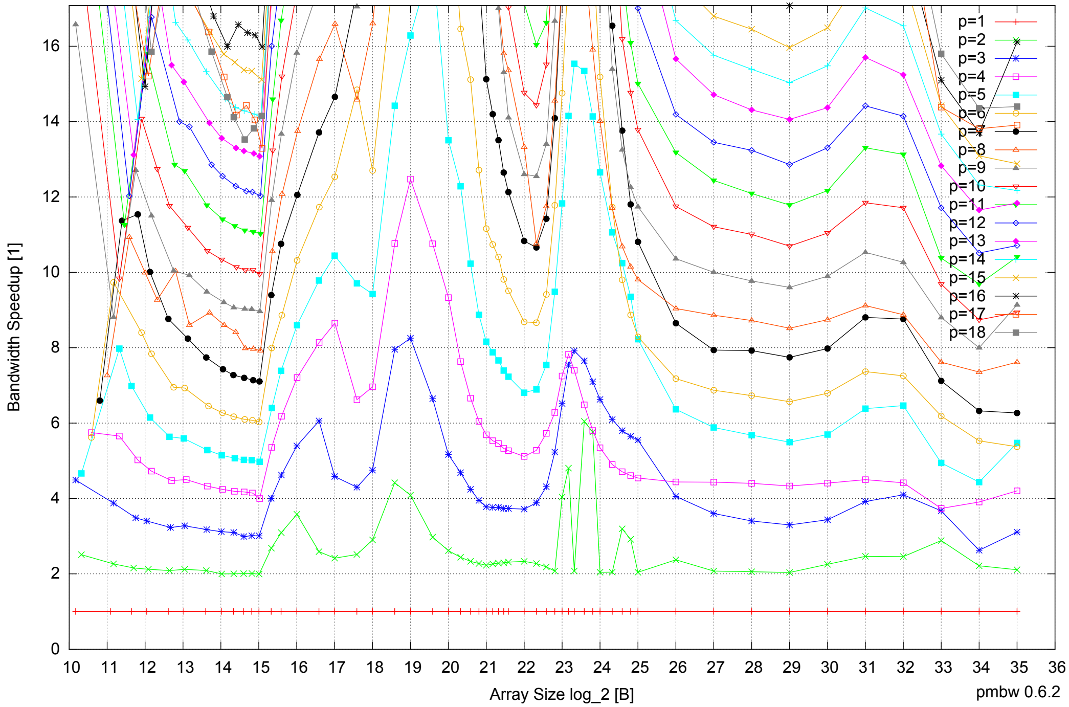
Intel Xeon X5550 48GB - Speedup of Parallel Memory Bandwidth (enlarged) - PermRead64UnrollLoop
