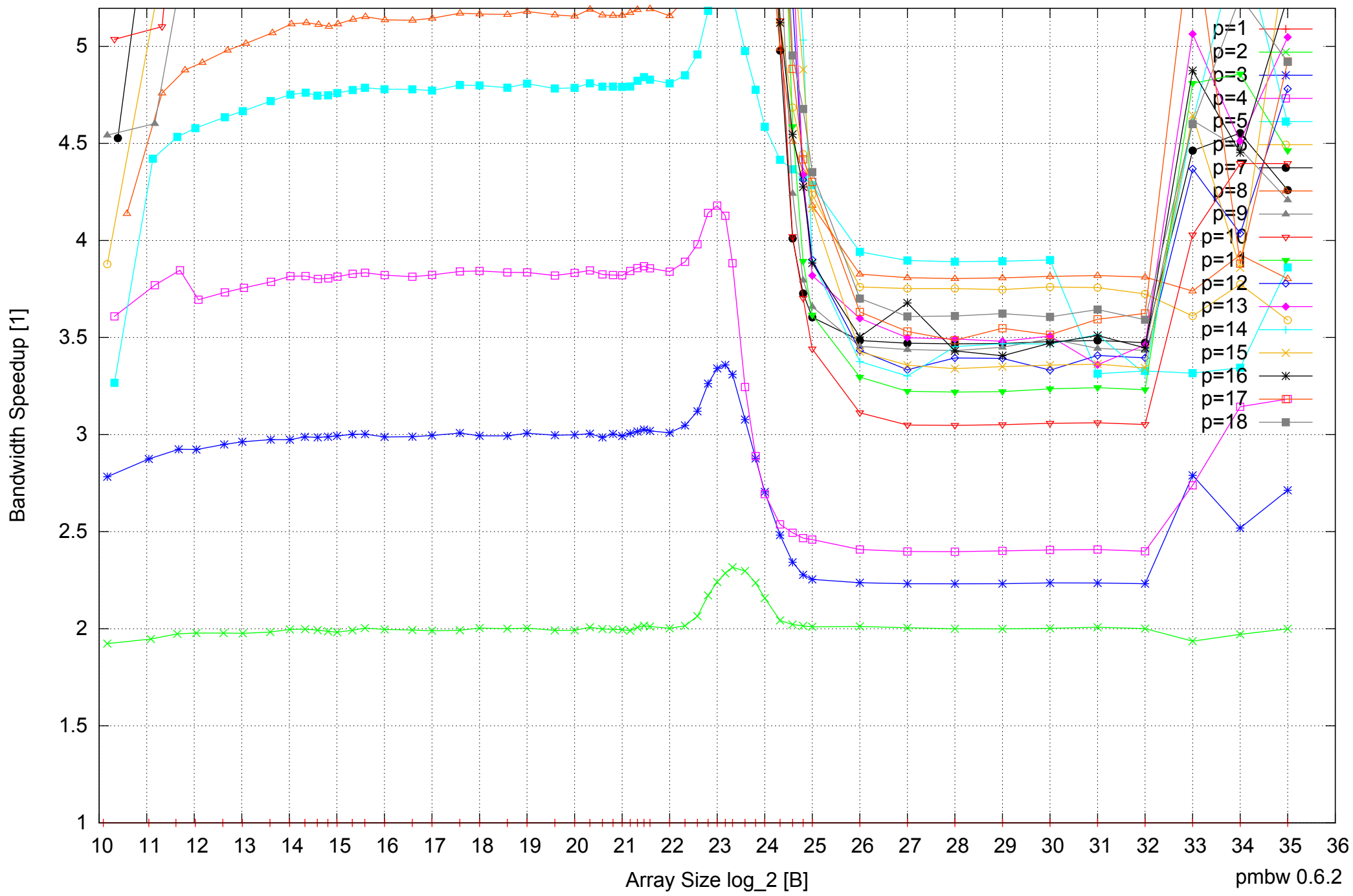
Intel Xeon X5550 48GB - Speedup of Parallel Memory Bandwidth (enlarged) - ScanRead32PtrSimpleLoop
