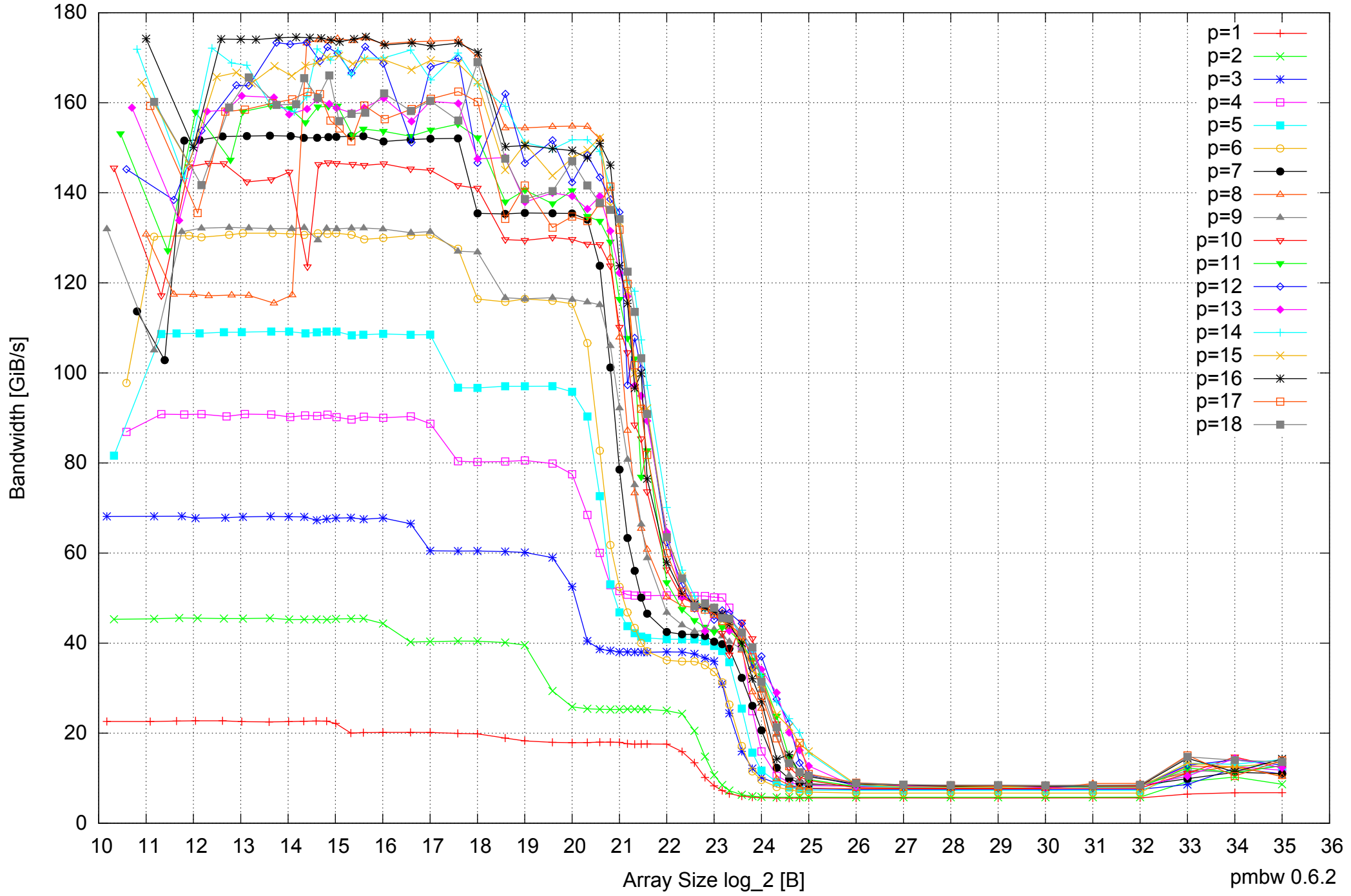
Intel Xeon X5550 48GB - Parallel Memory Bandwidth - ScanWrite64PtrUnrollLoop
