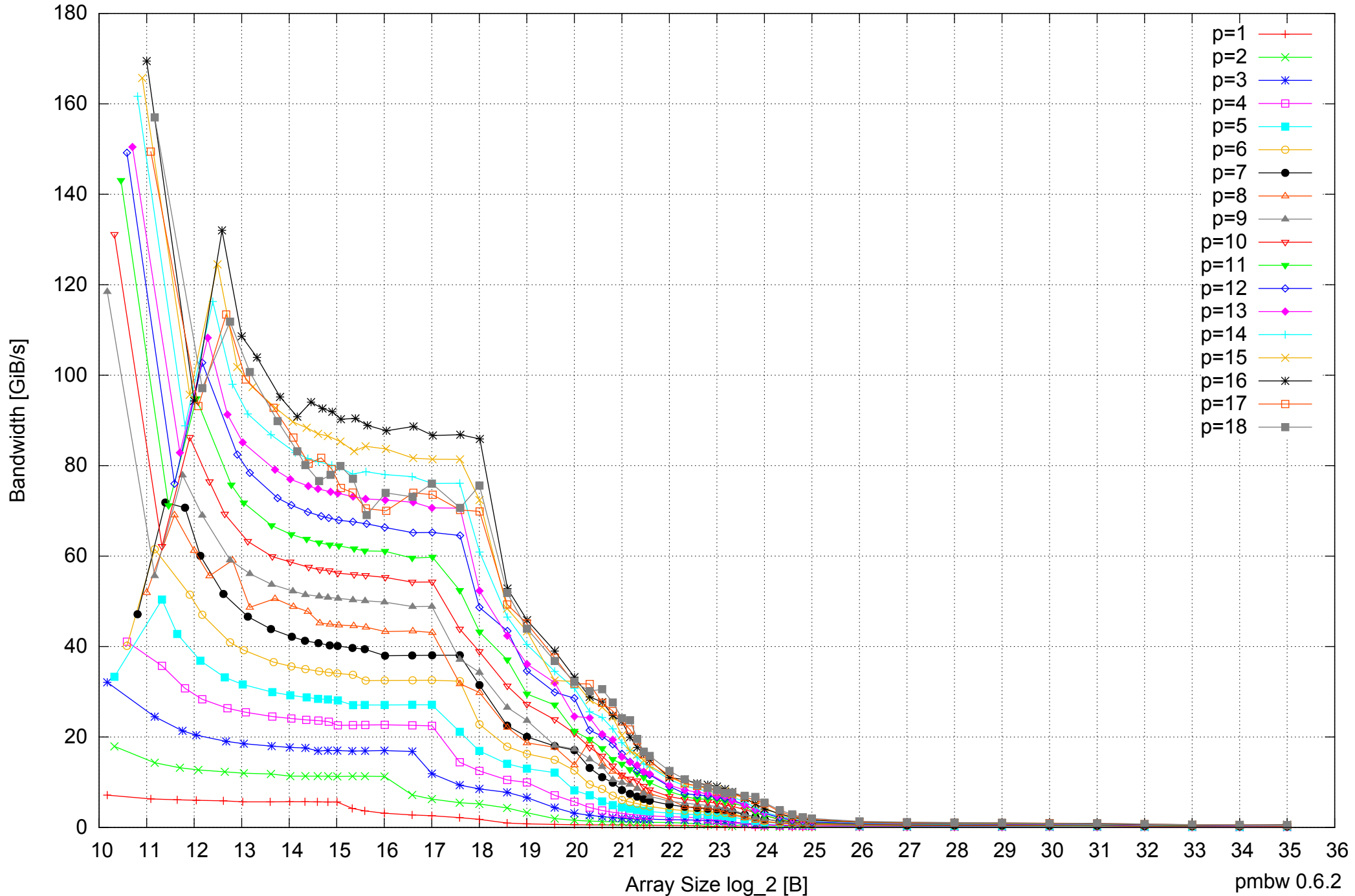
Intel Xeon X5550 48GB - Parallel Memory Bandwidth - PermRead64UnrollLoop
