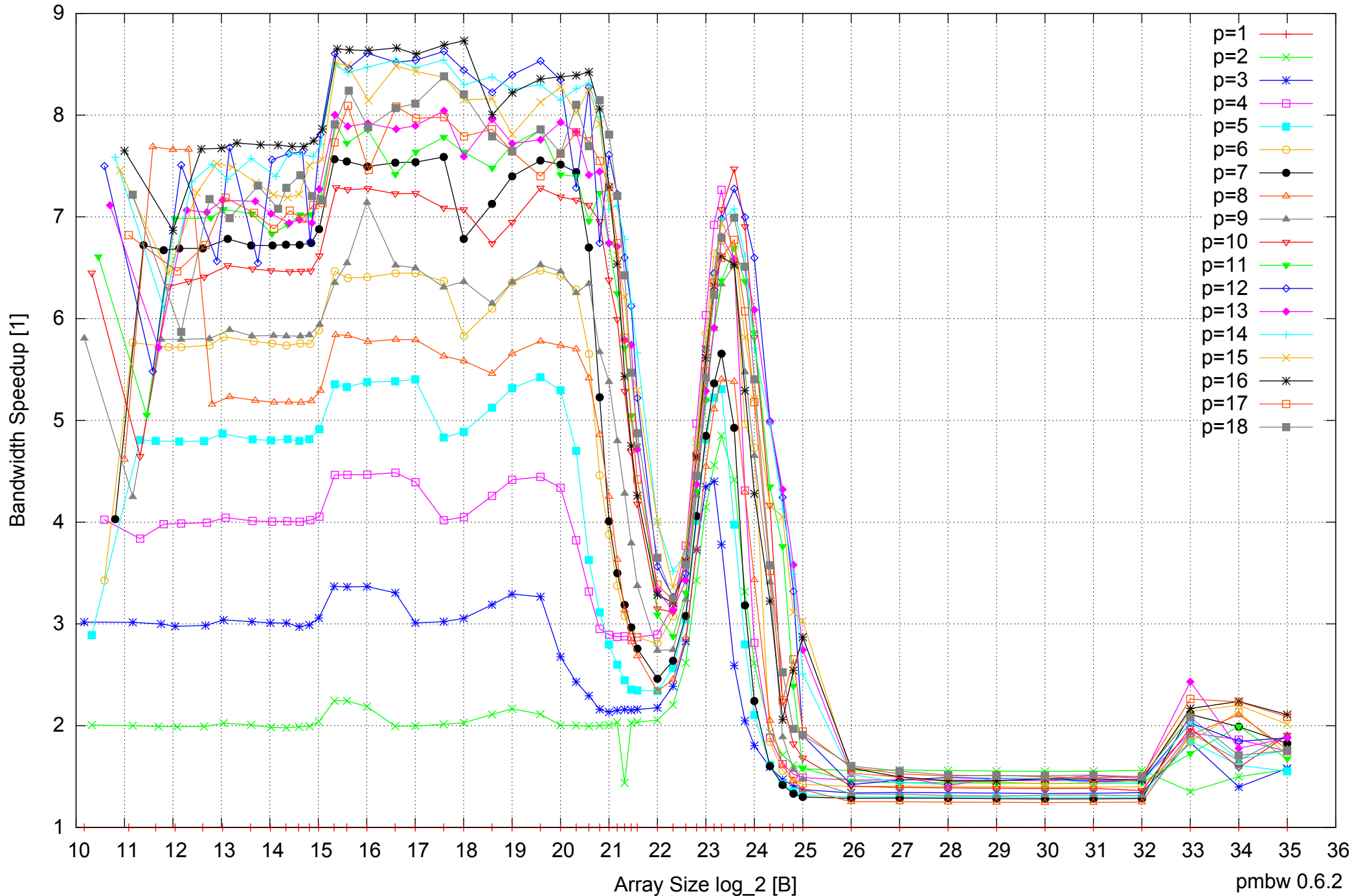
Intel Xeon X5550 48GB - Speedup of Parallel Memory Bandwidth - ScanWrite64IndexUnrollLoop
