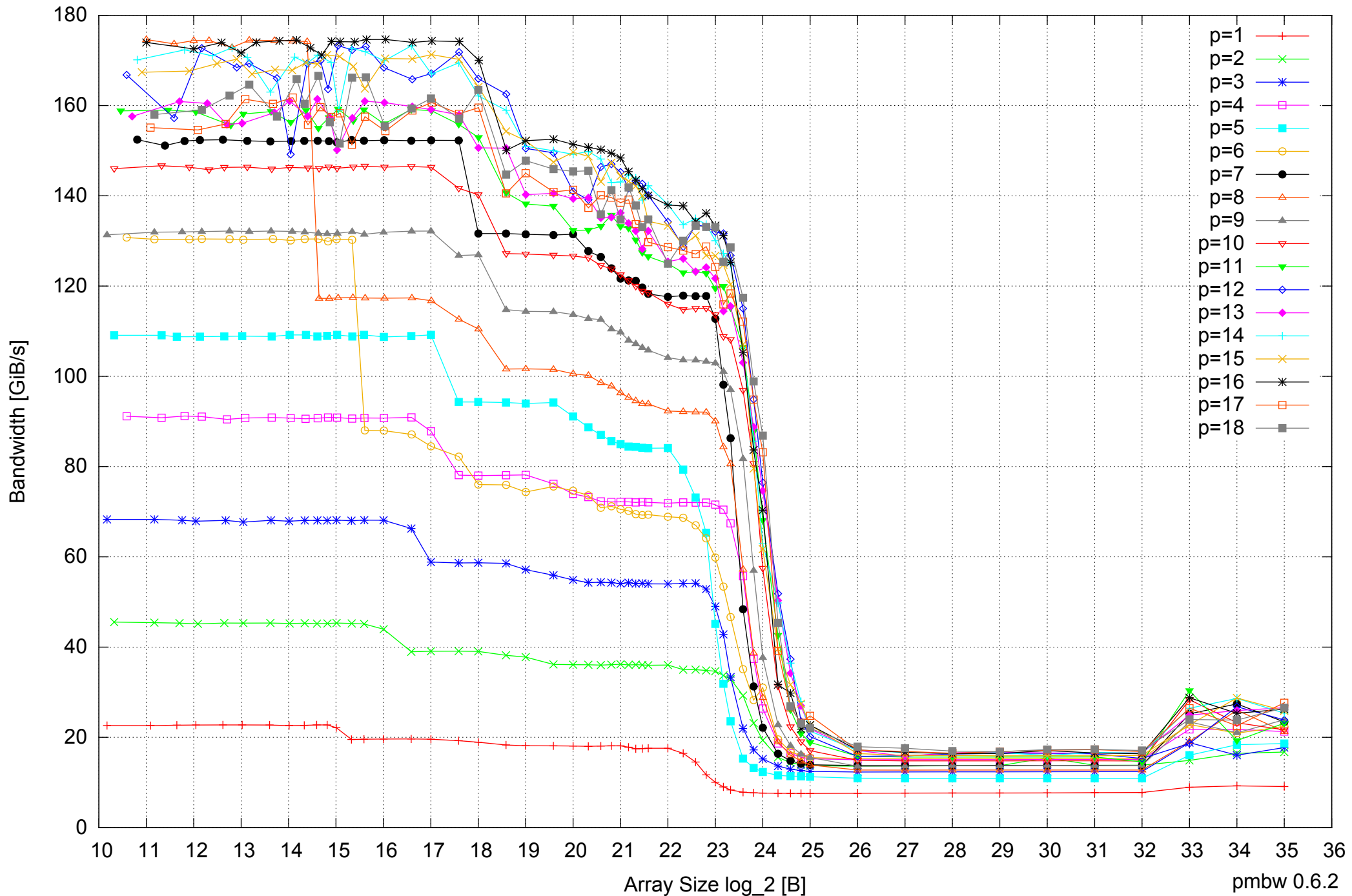
Intel Xeon X5550 48GB - Parallel Memory Bandwidth - ScanRead64IndexUnrollLoop
