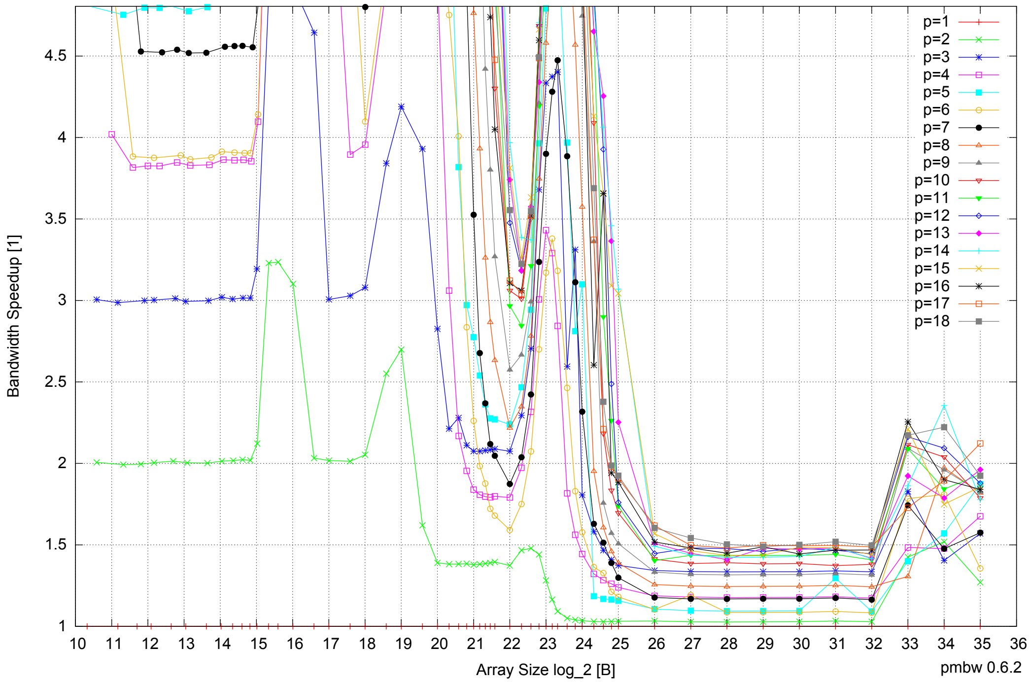
Intel Xeon X5550 48GB - Speedup of Parallel Memory Bandwidth (enlarged) - ScanWrite128PtrUnrollLoop
