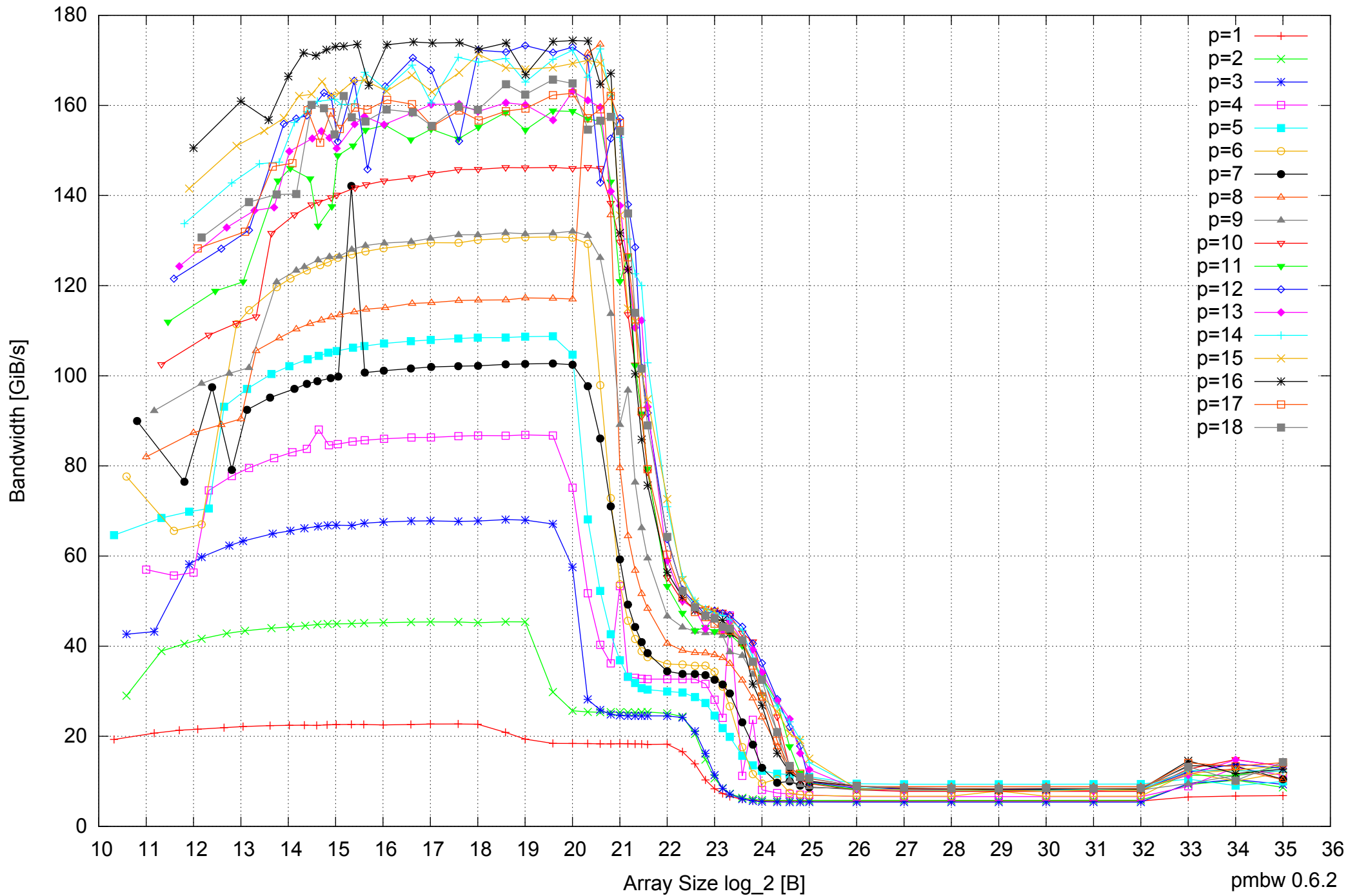
Intel Xeon X5550 48GB - Parallel Memory Bandwidth - ScanWrite128PtrSimpleLoop
