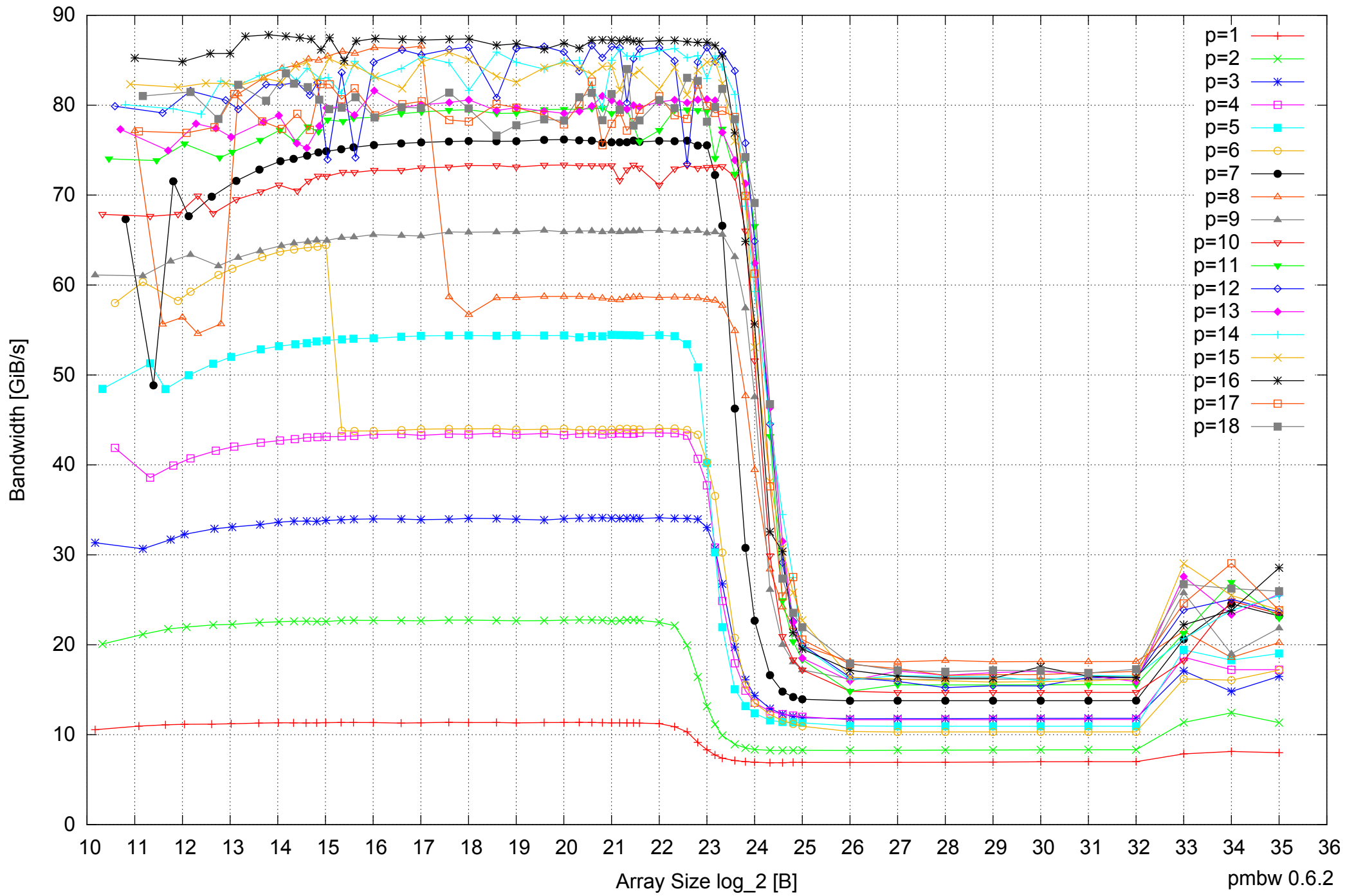
Intel Xeon X5550 48GB - Parallel Memory Bandwidth - ScanRead64PtrSimpleLoop
