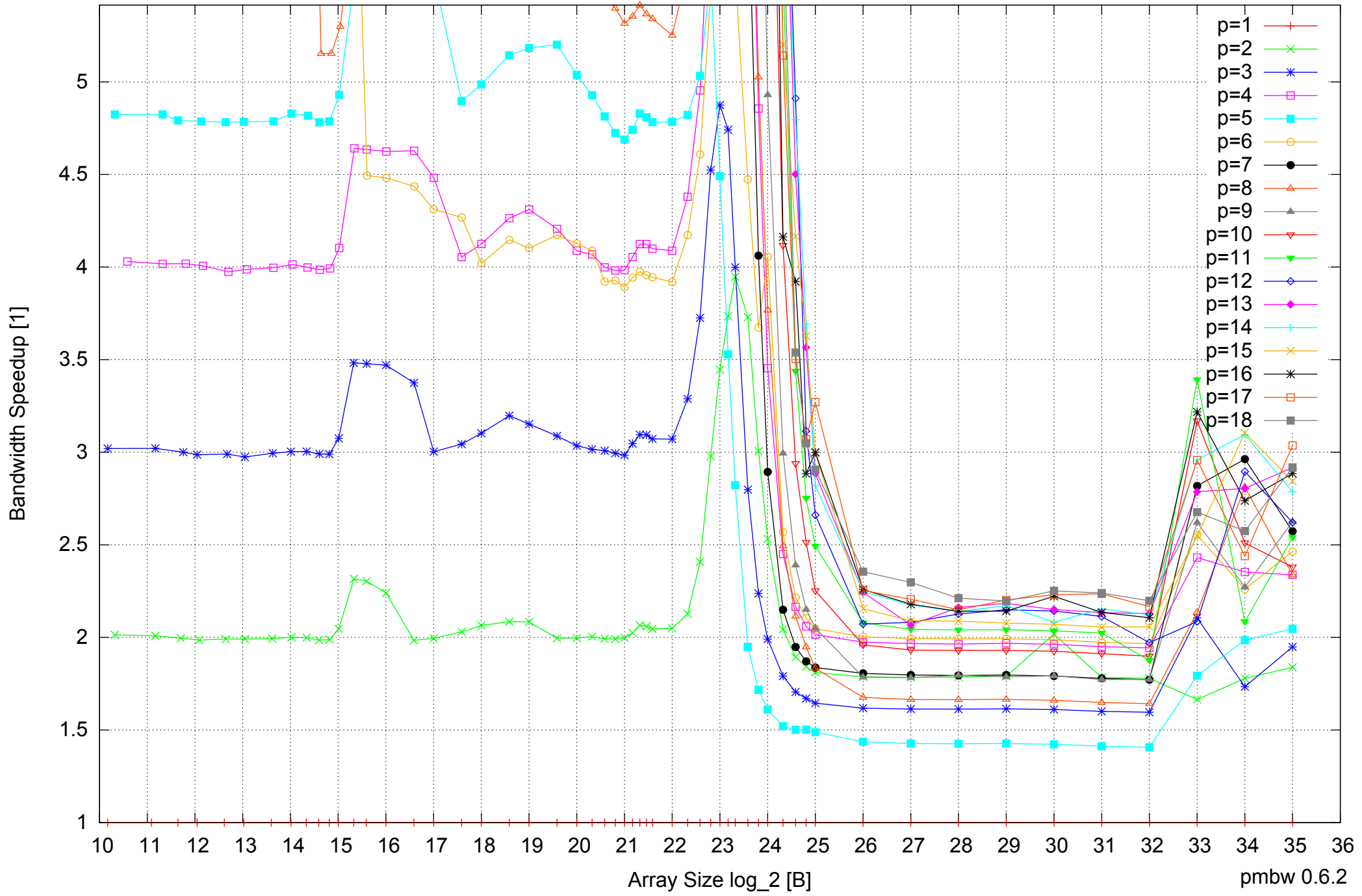
Intel Xeon X5550 48GB - Speedup of Parallel Memory Bandwidth (enlarged) - ScanRead64IndexUnrollLoop
