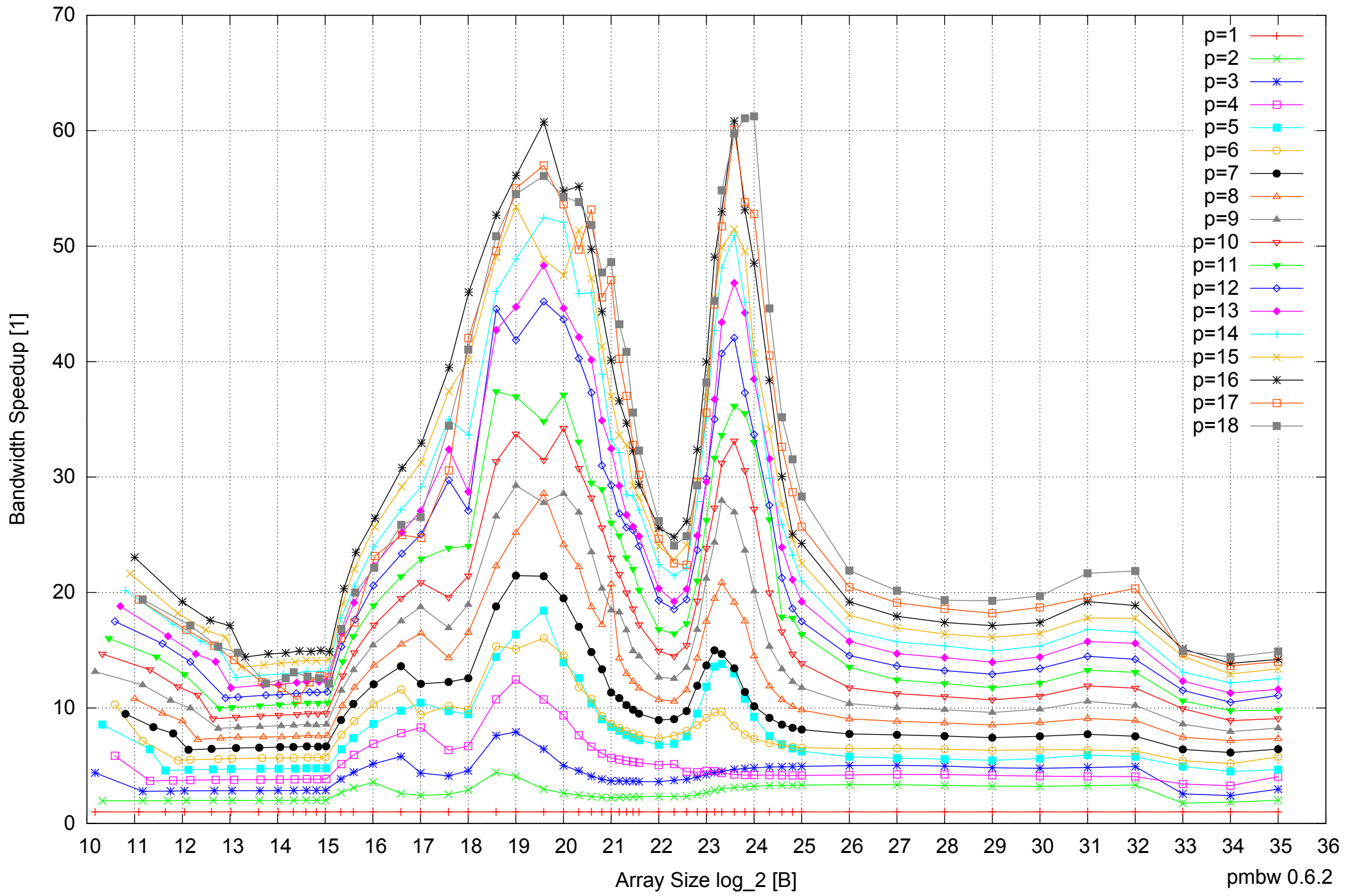
Intel Xeon X5550 48GB - Speedup of Parallel Memory Bandwidth - PermRead64SimpleLoop
