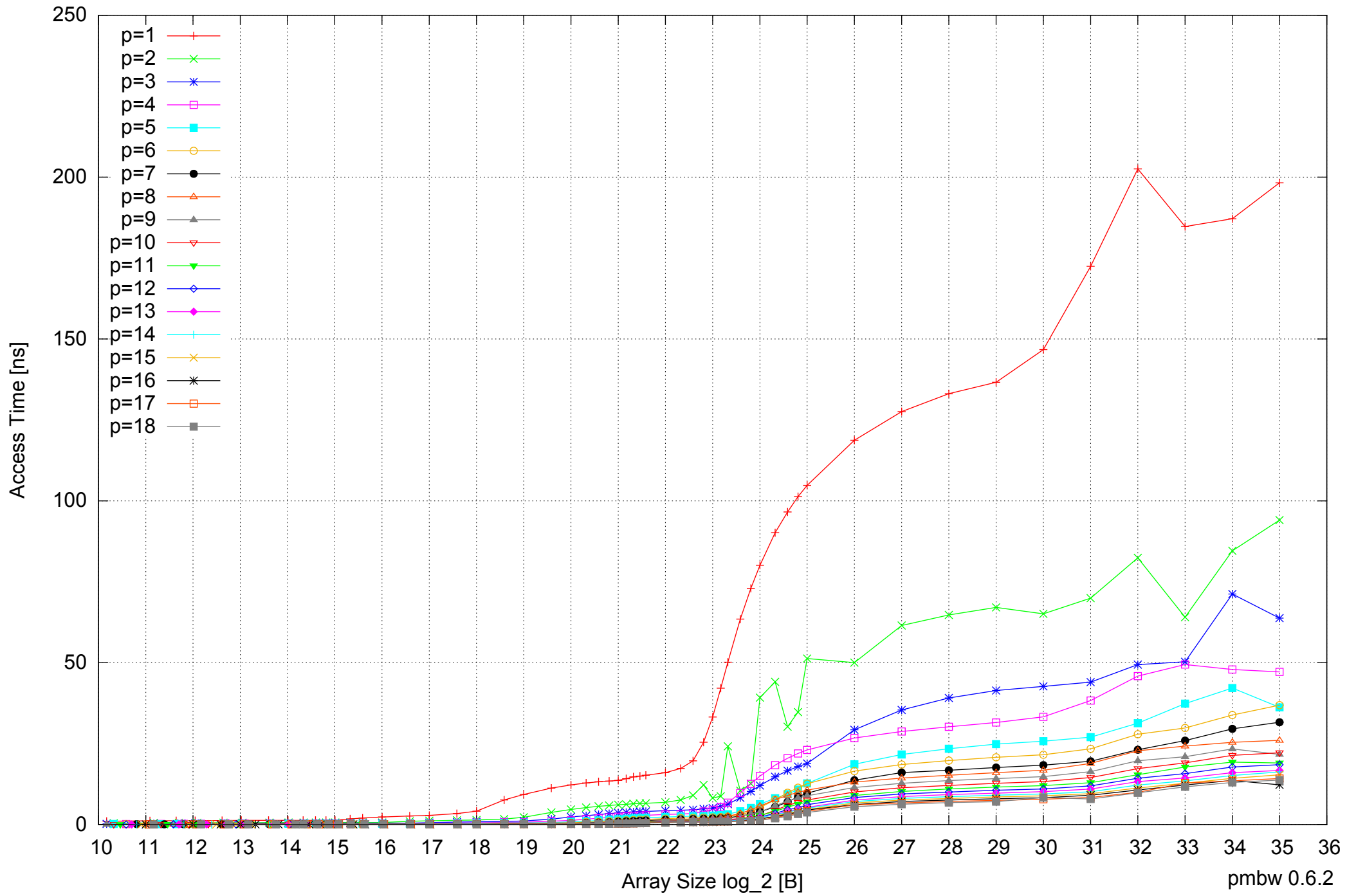
Intel Xeon X5550 48GB - Parallel Memory Access Time - PermRead64UnrollLoop
