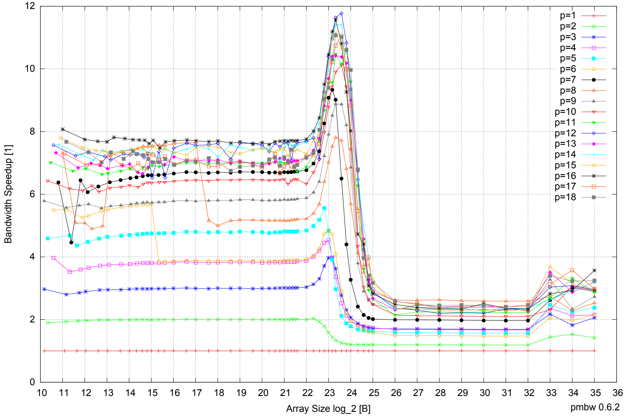
Intel Xeon X5550 48GB - Speedup of Parallel Memory Bandwidth - ScanRead64PtrSimpleLoop
