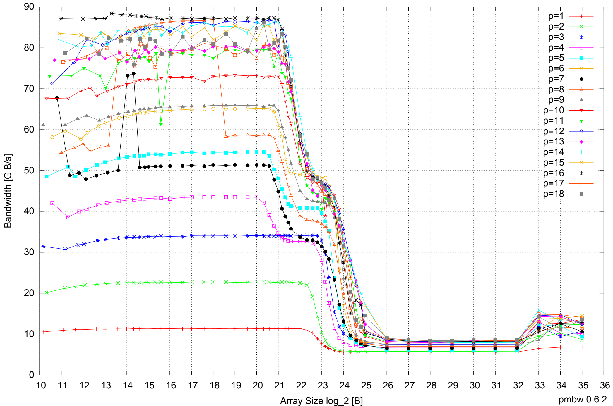
Intel Xeon X5550 48GB - Parallel Memory Bandwidth - ScanWrite64IndexSimpleLoop
