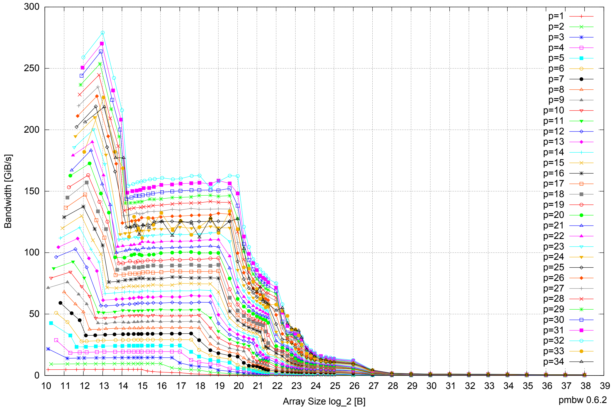
Intel Xeon E7-8837 512GB - Parallel Memory Bandwidth - PermRead64SimpleLoop
