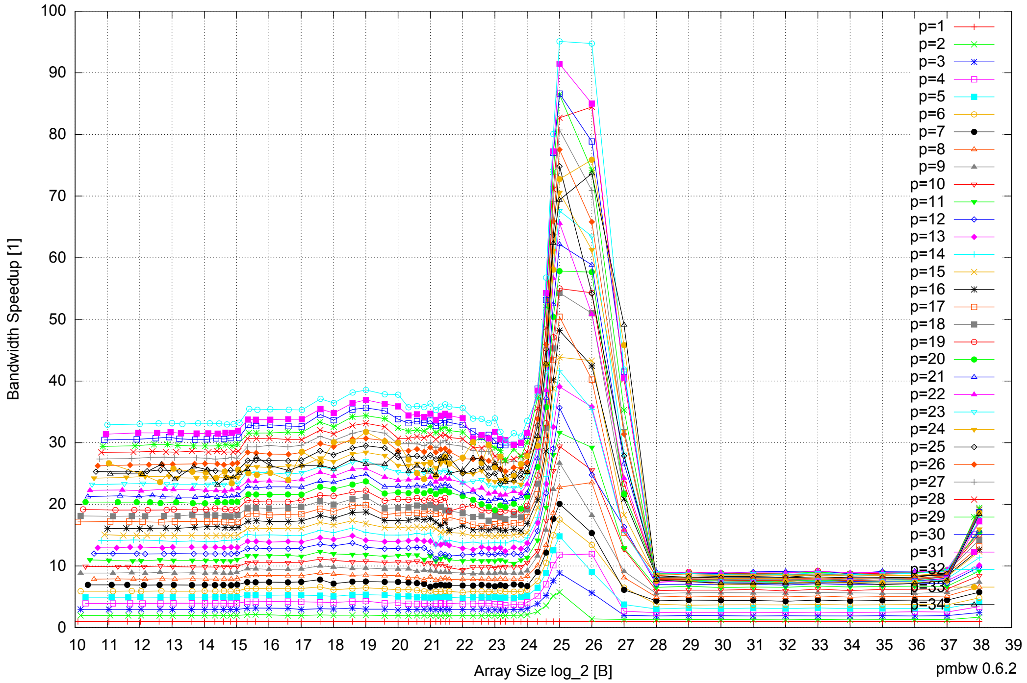
Intel Xeon E7-8837 512GB - Speedup of Parallel Memory Bandwidth - ScanRead32PtrUnrollLoop
