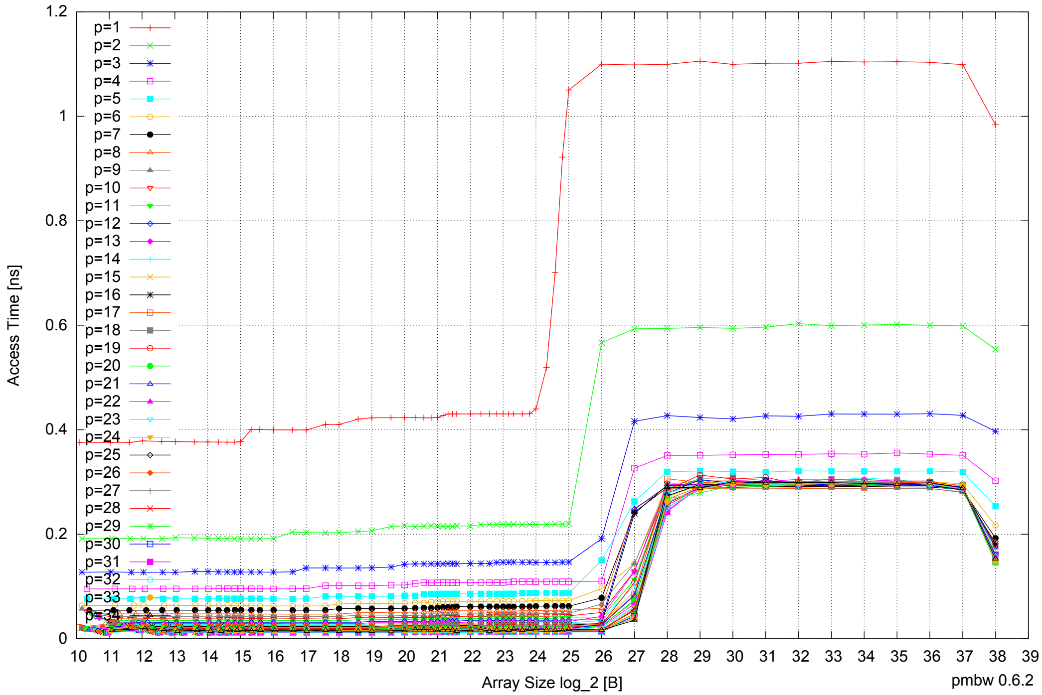
Intel Xeon E7-8837 512GB - Parallel Memory Access Time - ScanWrite32PtrUnrollLoop
