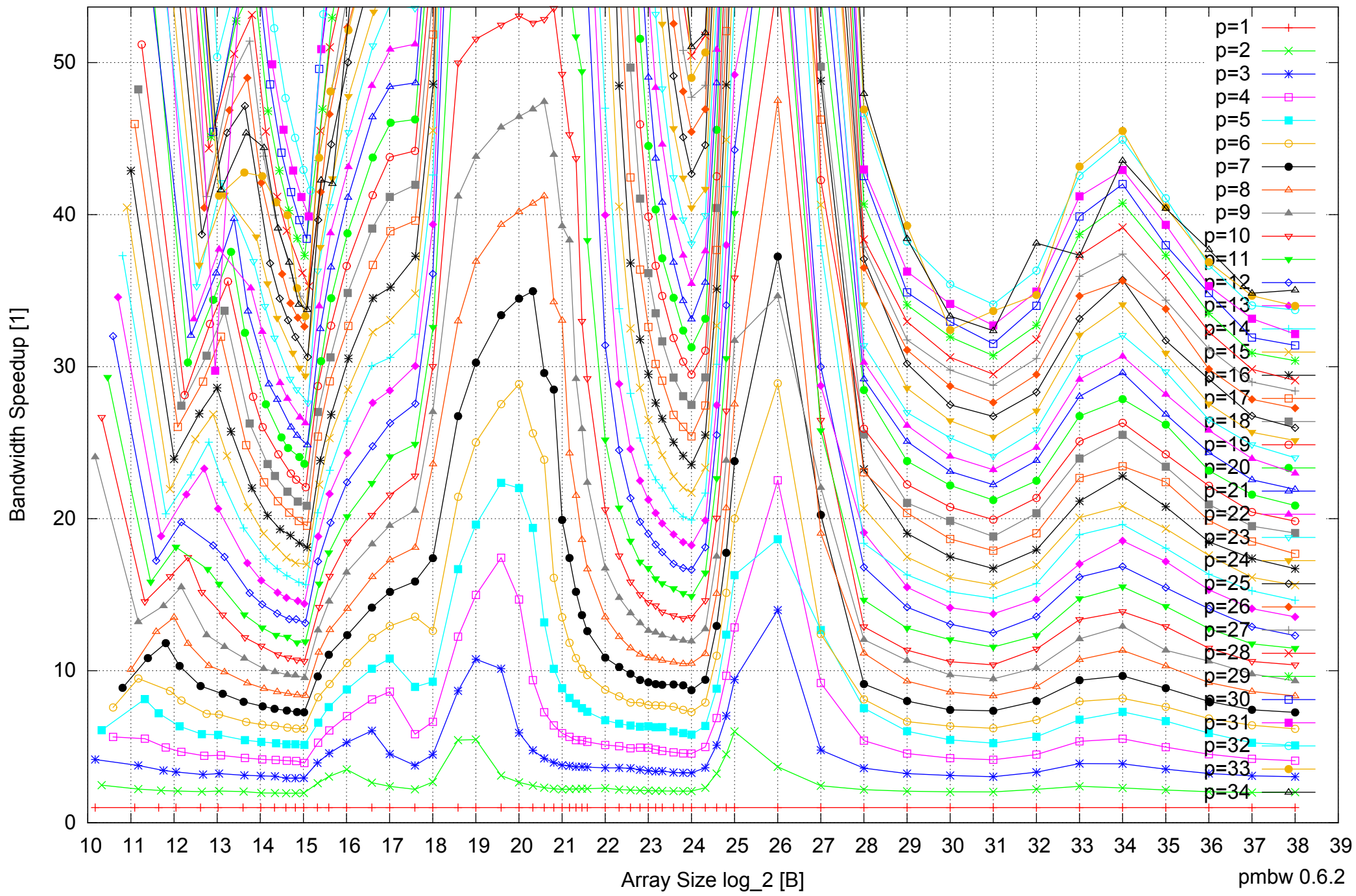
Intel Xeon E7-8837 512GB - Speedup of Parallel Memory Bandwidth (enlarged) - PermRead64UnrollLoop
