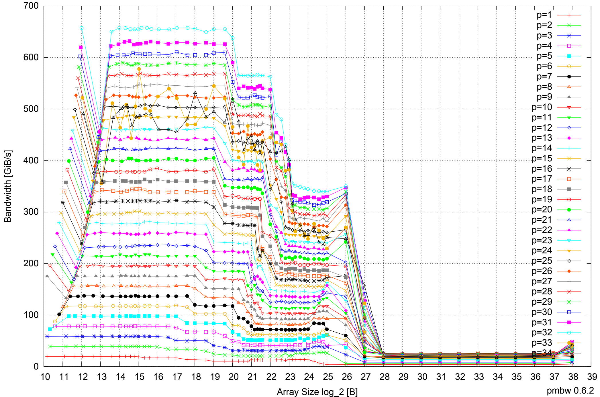
Intel Xeon E7-8837 512GB - Parallel Memory Bandwidth - ScanRead64PtrUnrollLoop
