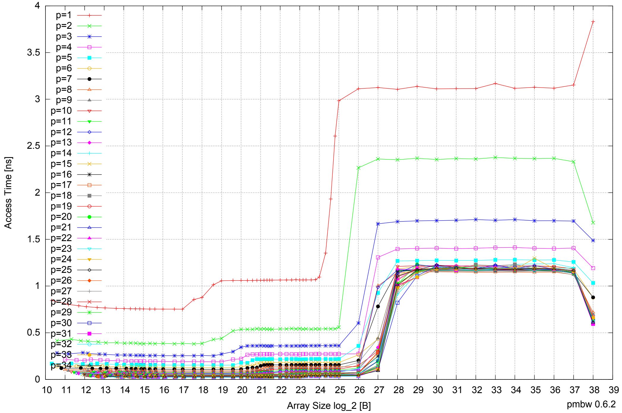
Intel Xeon E7-8837 512GB - Parallel Memory Access Time - ScanWrite128PtrSimpleLoop
