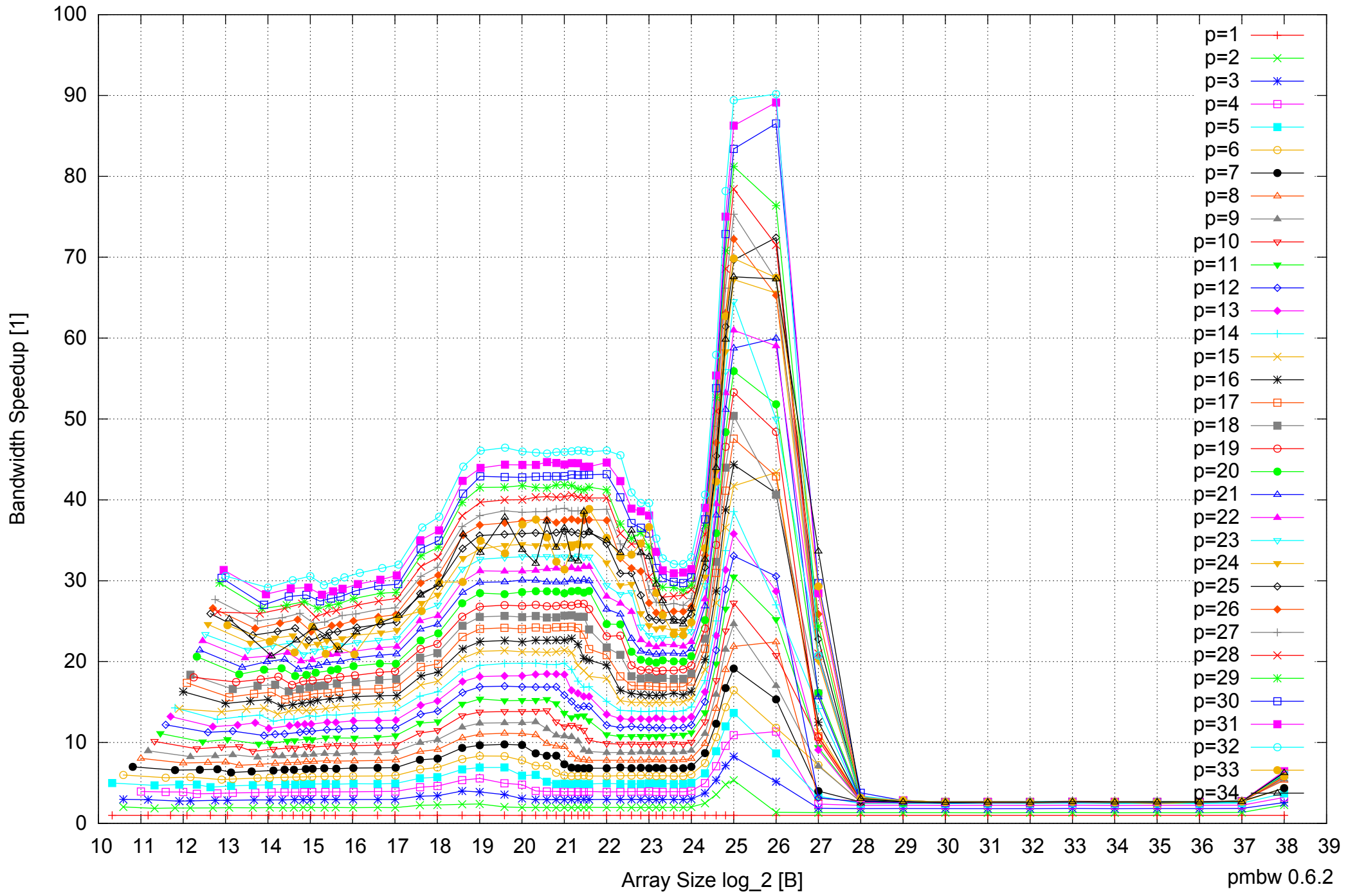
Intel Xeon E7-8837 512GB - Speedup of Parallel Memory Bandwidth - ScanWrite128PtrSimpleLoop
