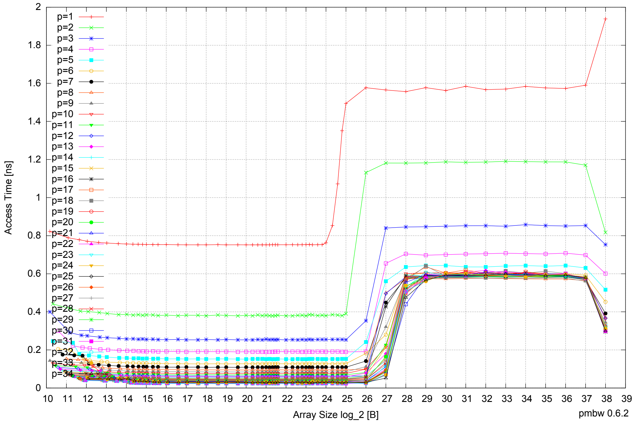
Intel Xeon E7-8837 512GB - Parallel Memory Access Time - ScanWrite64IndexSimpleLoop
