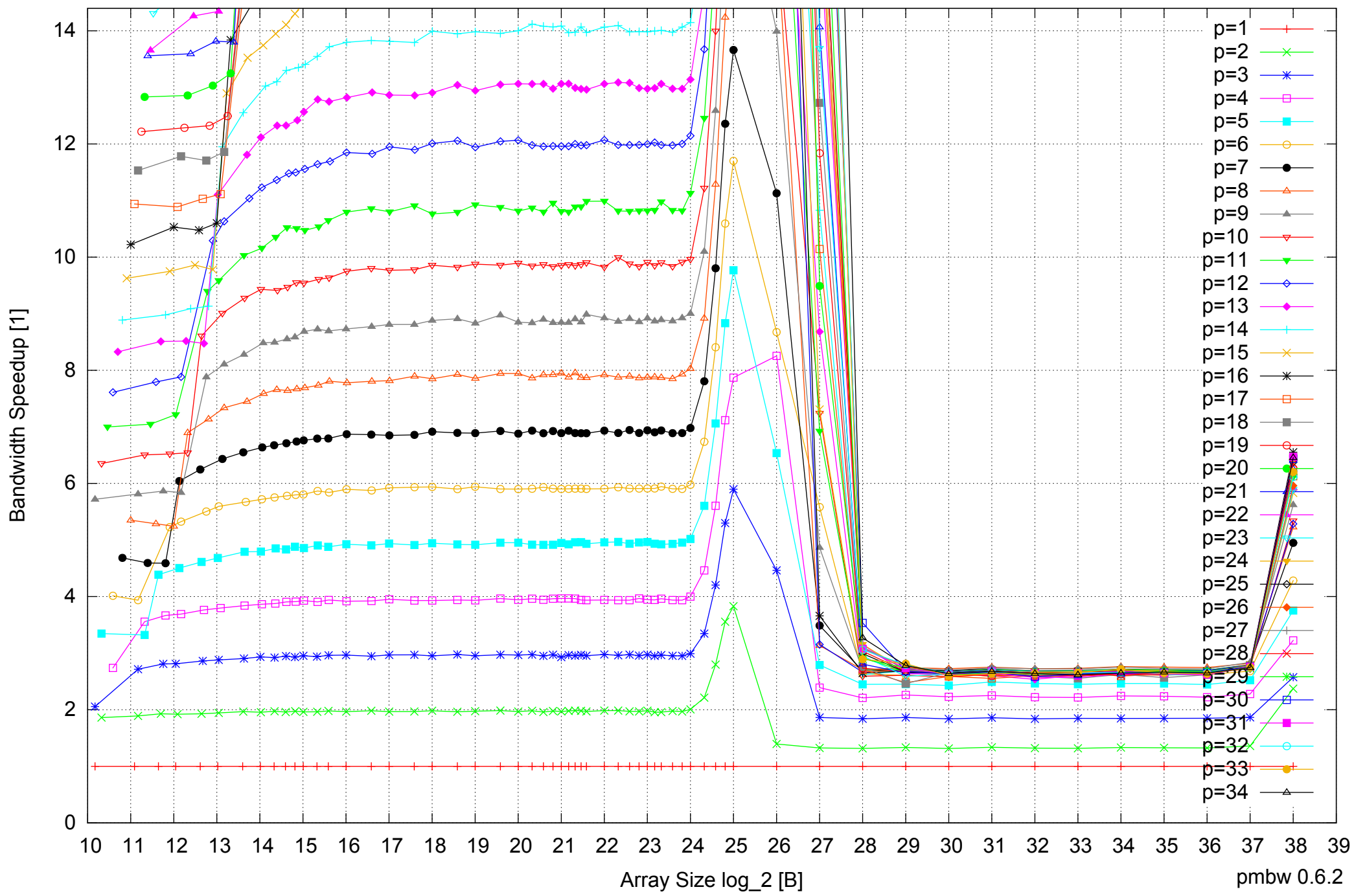
Intel Xeon E7-8837 512GB - Speedup of Parallel Memory Bandwidth (enlarged) - ScanWrite64IndexSimpleLoop
