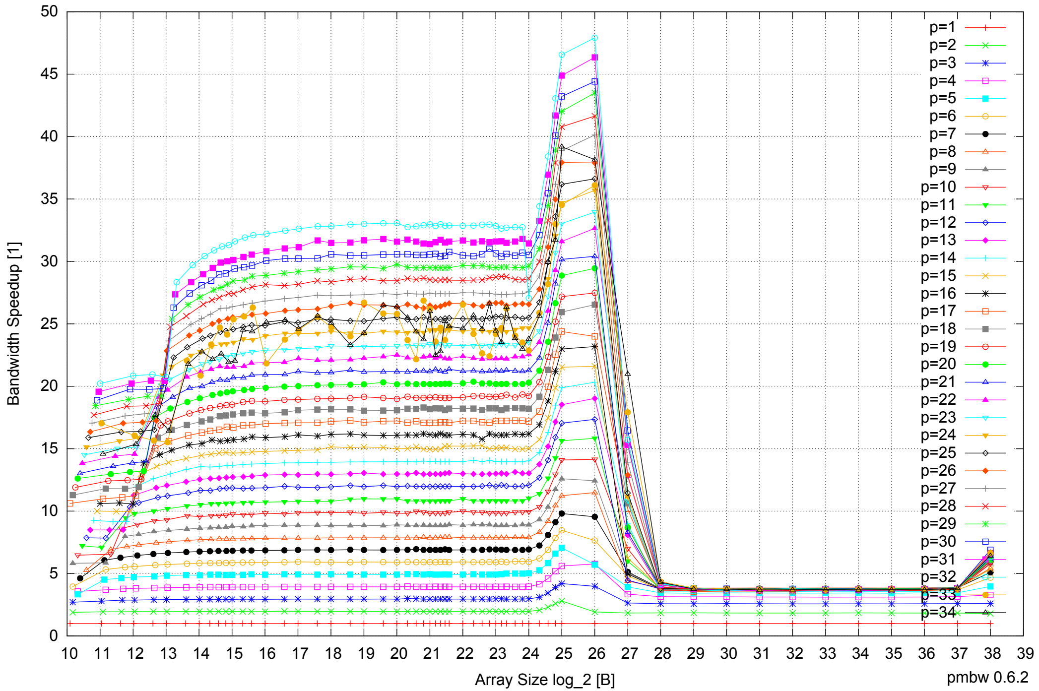
Intel Xeon E7-8837 512GB - Speedup of Parallel Memory Bandwidth - ScanWrite32PtrSimpleLoop
