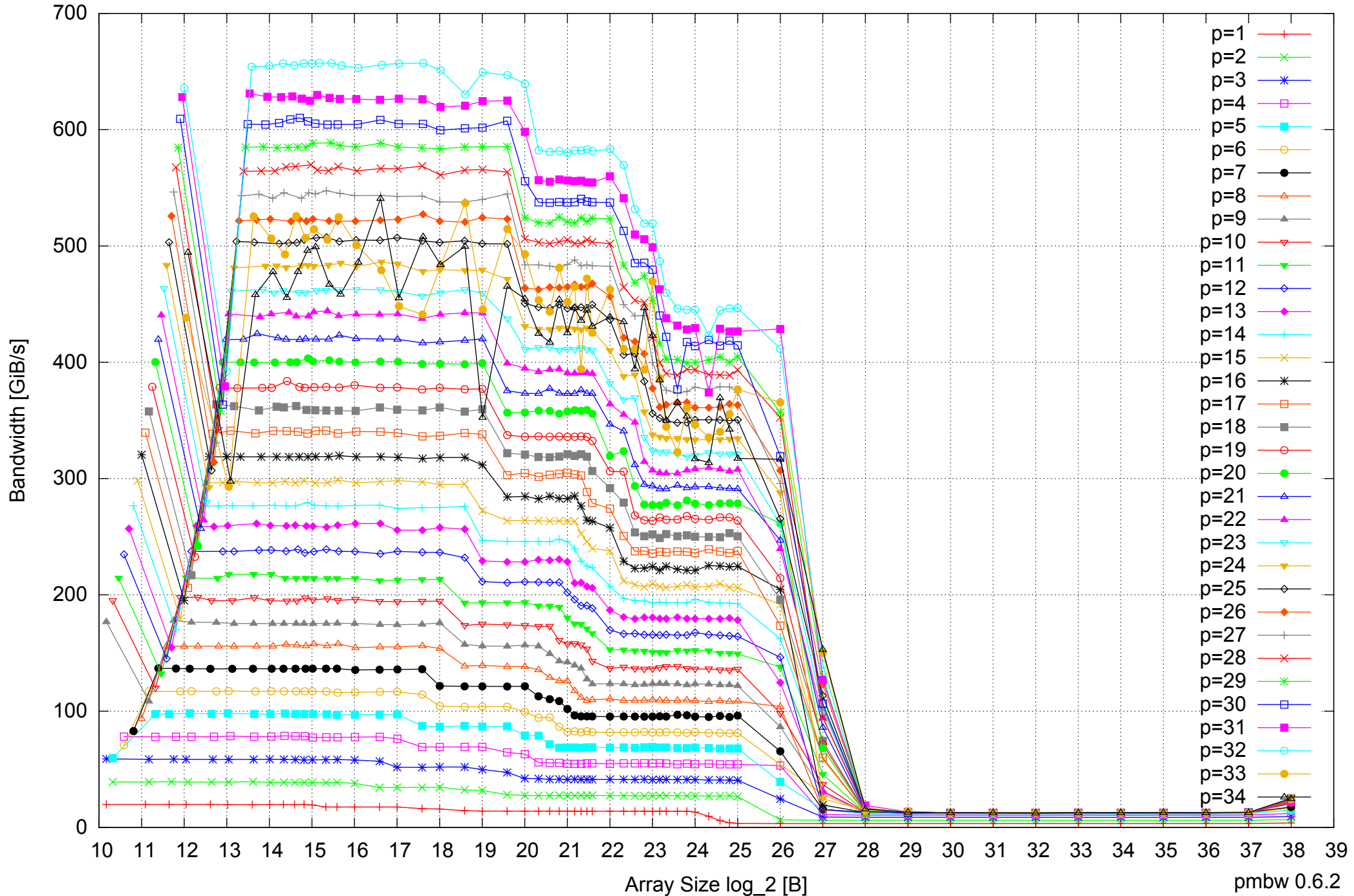
Intel Xeon E7-8837 512GB - Parallel Memory Bandwidth - ScanWrite64IndexUnrollLoop
