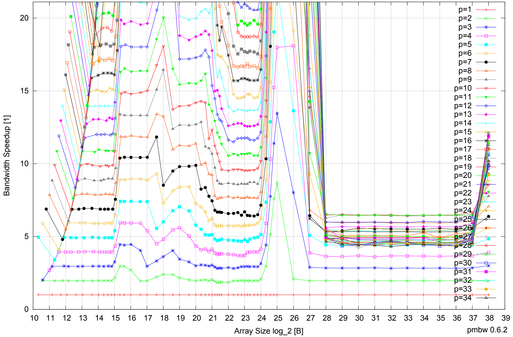
Intel Xeon E7-8837 512GB - Speedup of Parallel Memory Bandwidth (enlarged) - ScanRead128PtrUnrollLoop
