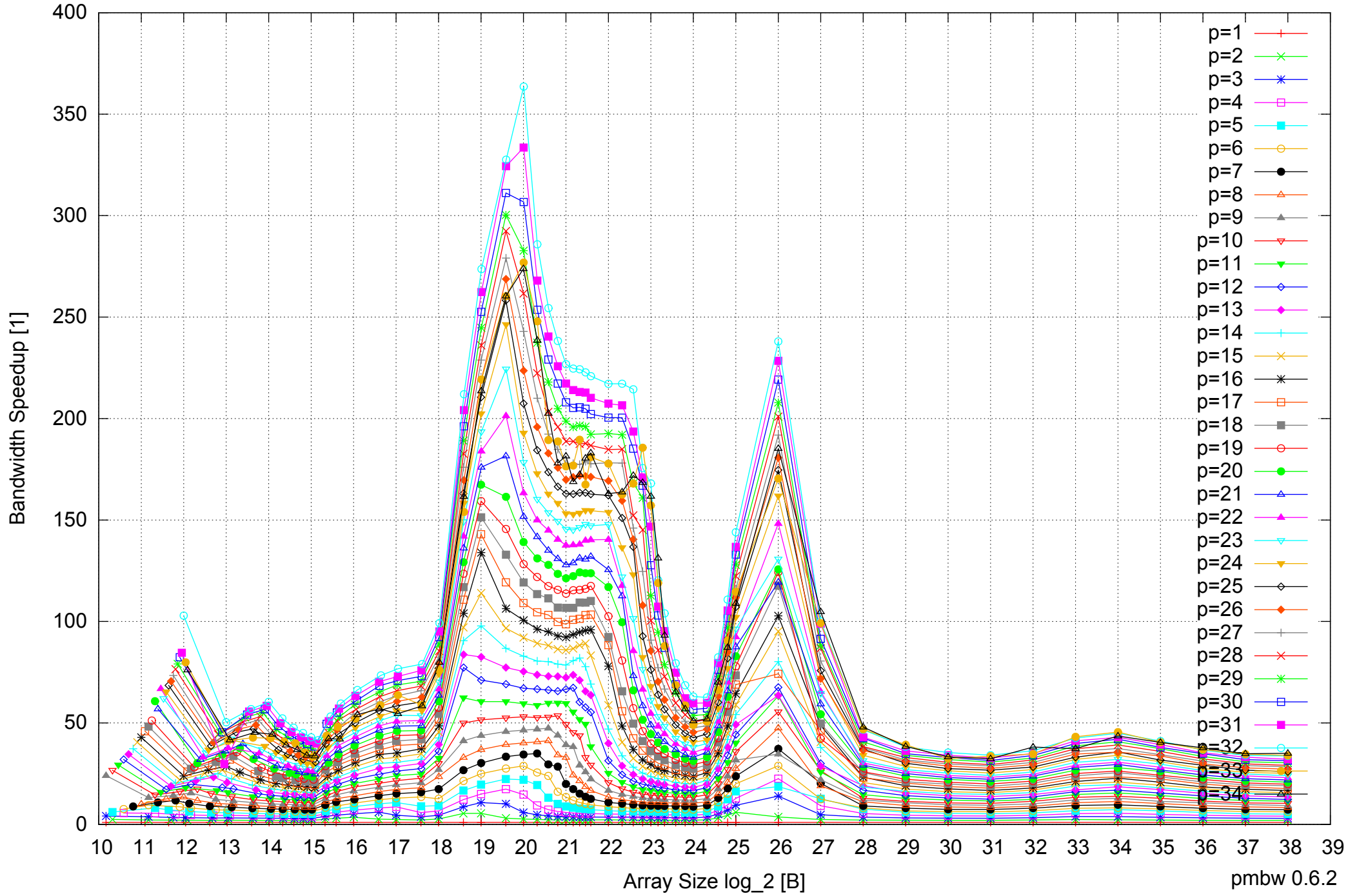
Intel Xeon E7-8837 512GB - Speedup of Parallel Memory Bandwidth - PermRead64UnrollLoop
