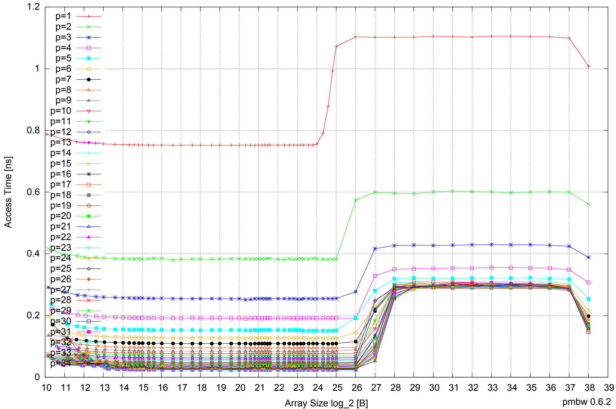
Intel Xeon E7-8837 512GB - Parallel Memory Access Time - ScanWrite32PtrSimpleLoop
