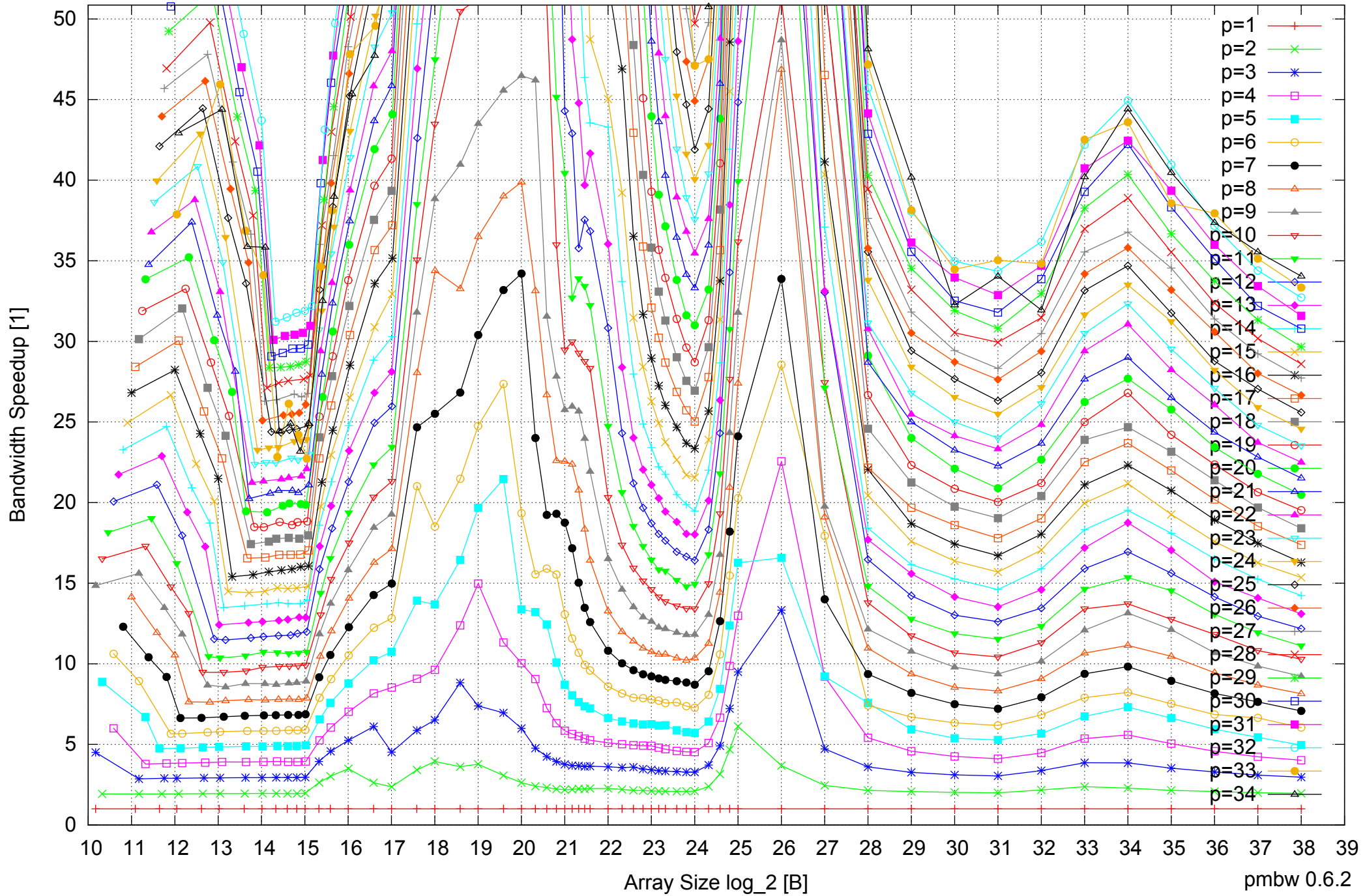
Intel Xeon E7-8837 512GB - Speedup of Parallel Memory Bandwidth (enlarged) - PermRead64SimpleLoop
