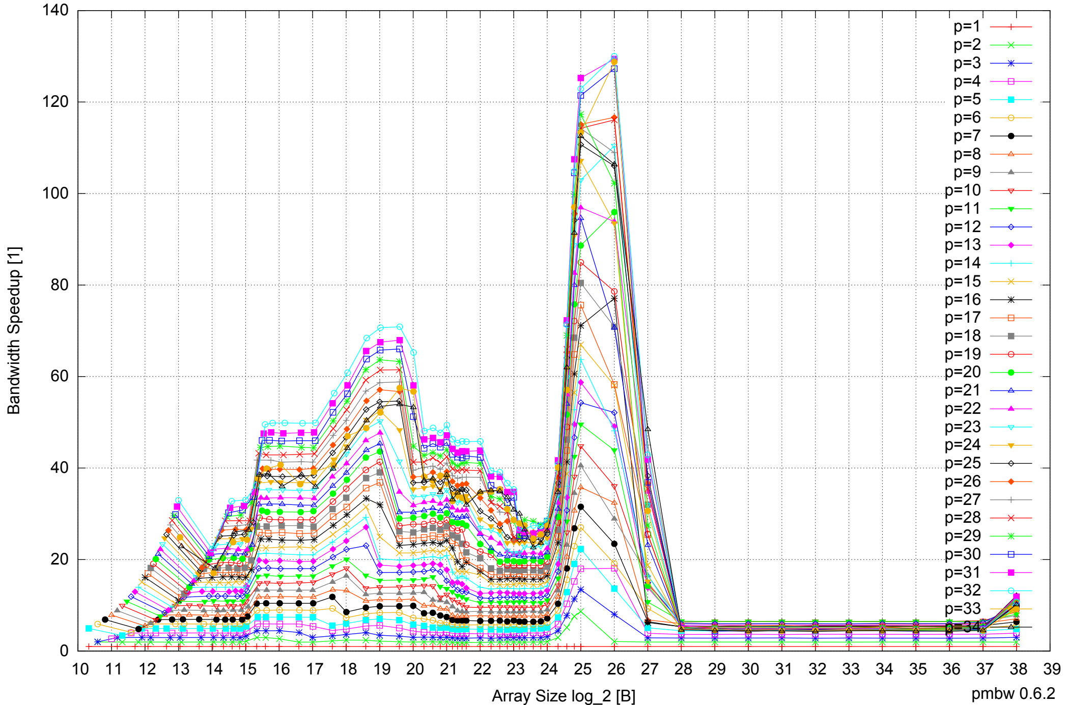
Intel Xeon E7-8837 512GB - Speedup of Parallel Memory Bandwidth - ScanRead128PtrUnrollLoop
