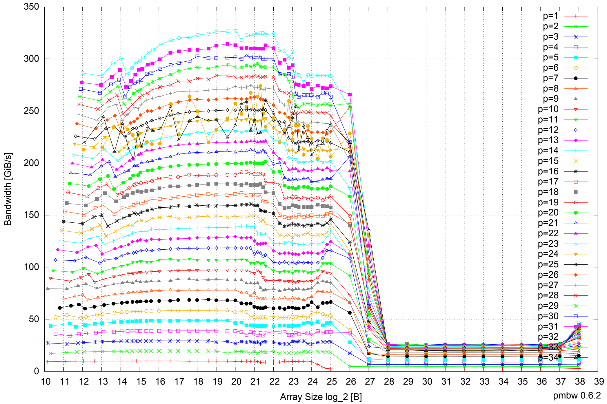
Intel Xeon E7-8837 512GB - Parallel Memory Bandwidth - ScanRead64IndexSimpleLoop
