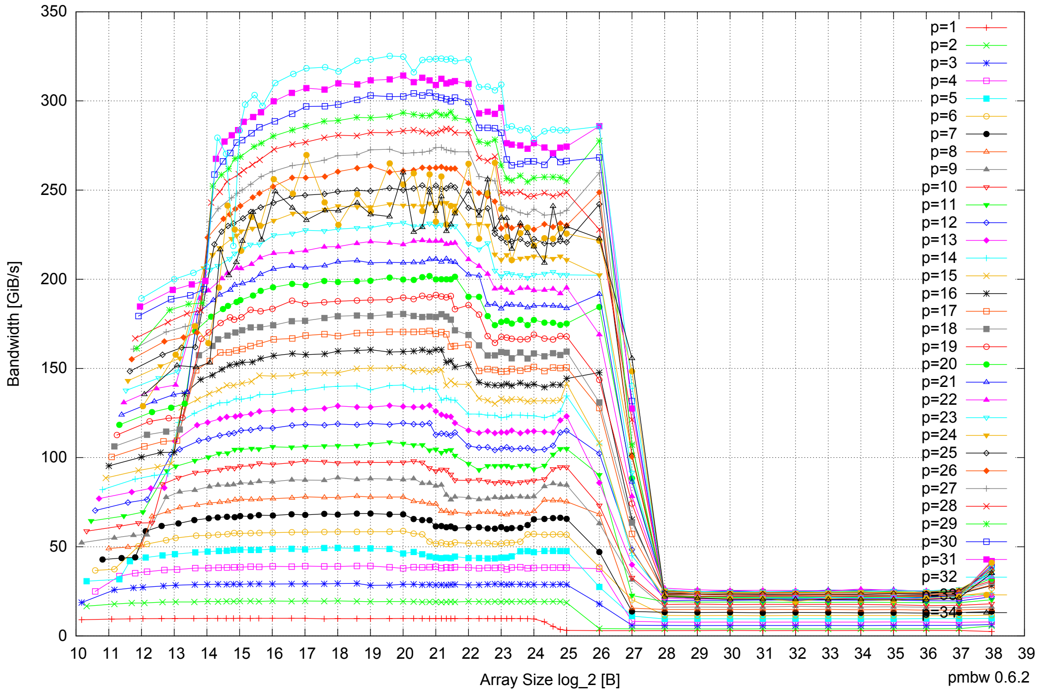
Intel Xeon E7-8837 512GB - Parallel Memory Bandwidth - ScanRead64PtrSimpleLoop
