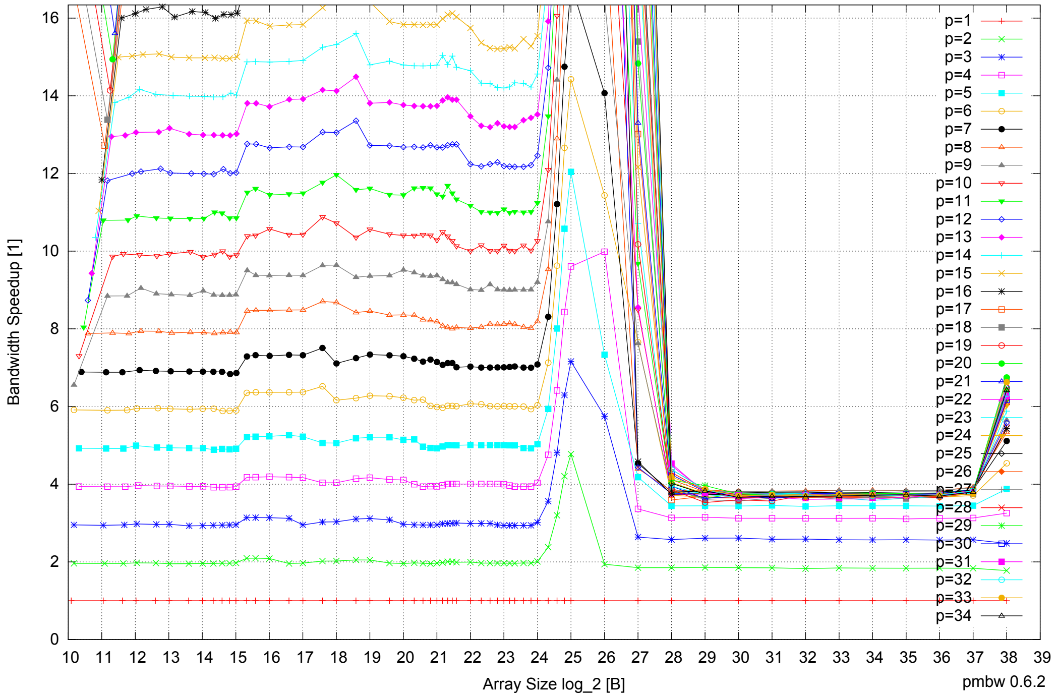
Intel Xeon E7-8837 512GB - Speedup of Parallel Memory Bandwidth (enlarged) - ScanWrite32PtrUnrollLoop
