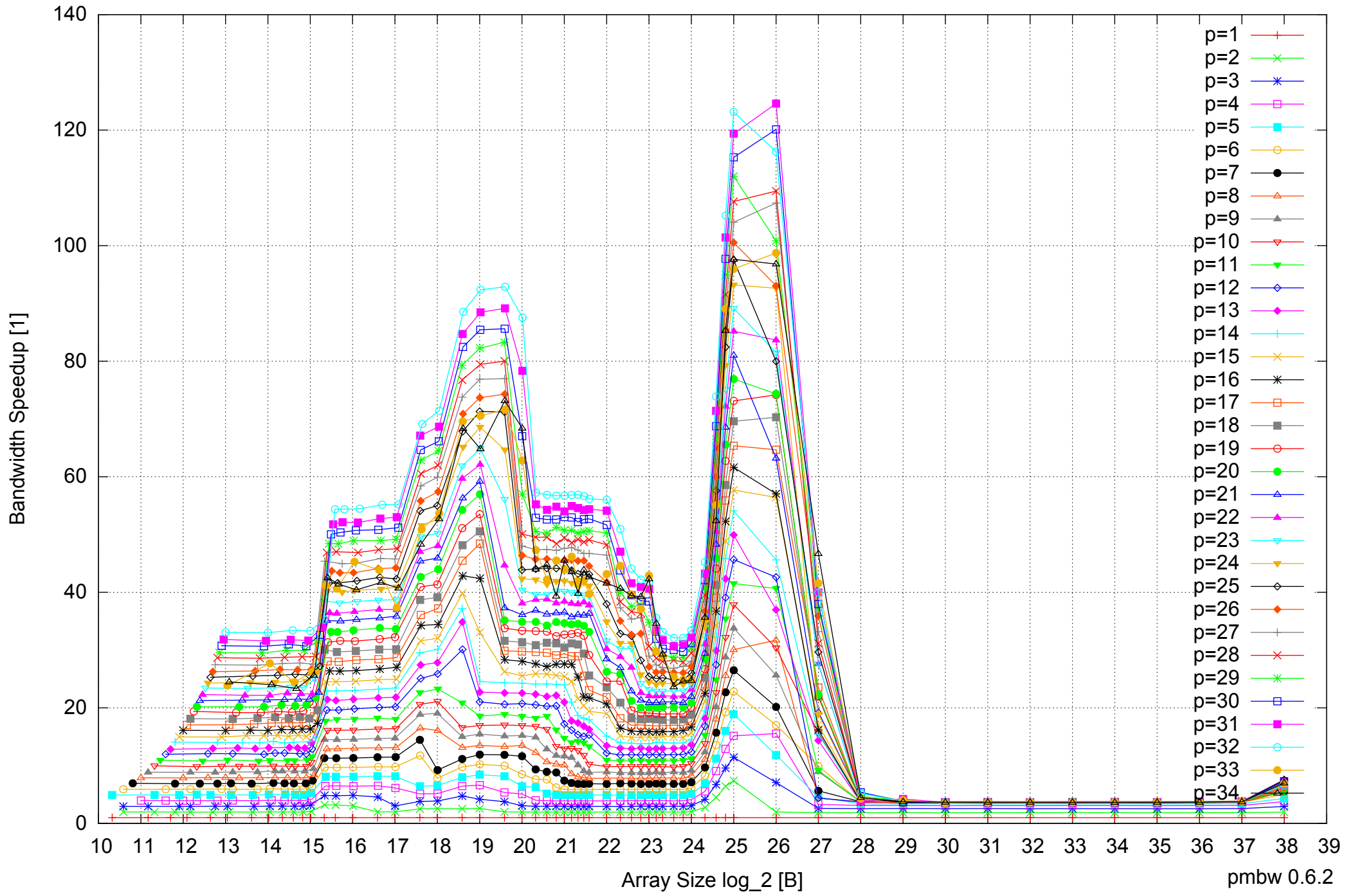
Intel Xeon E7-8837 512GB - Speedup of Parallel Memory Bandwidth - ScanWrite128PtrUnrollLoop
