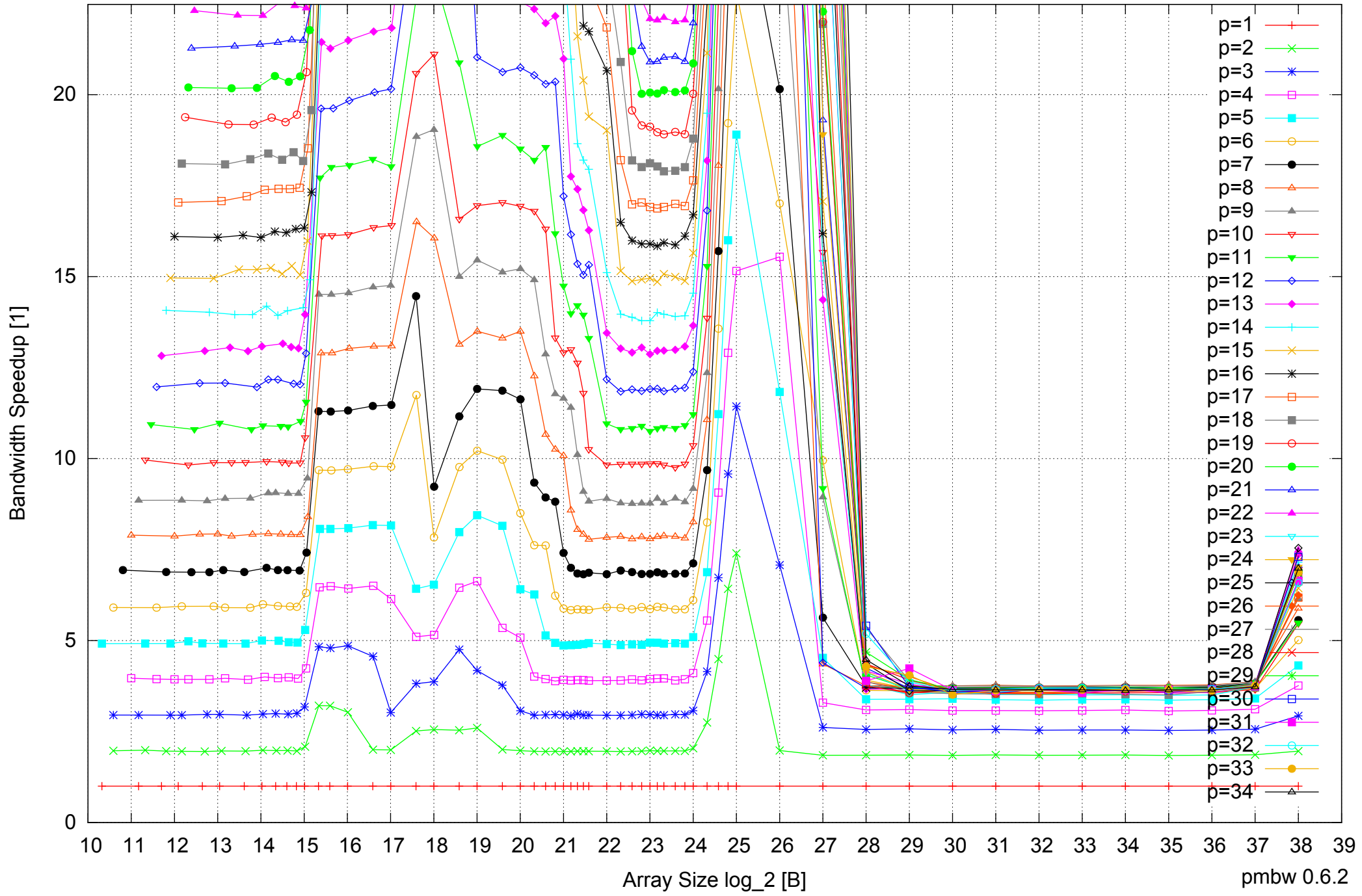
Intel Xeon E7-8837 512GB - Speedup of Parallel Memory Bandwidth (enlarged) - ScanWrite128PtrUnrollLoop
