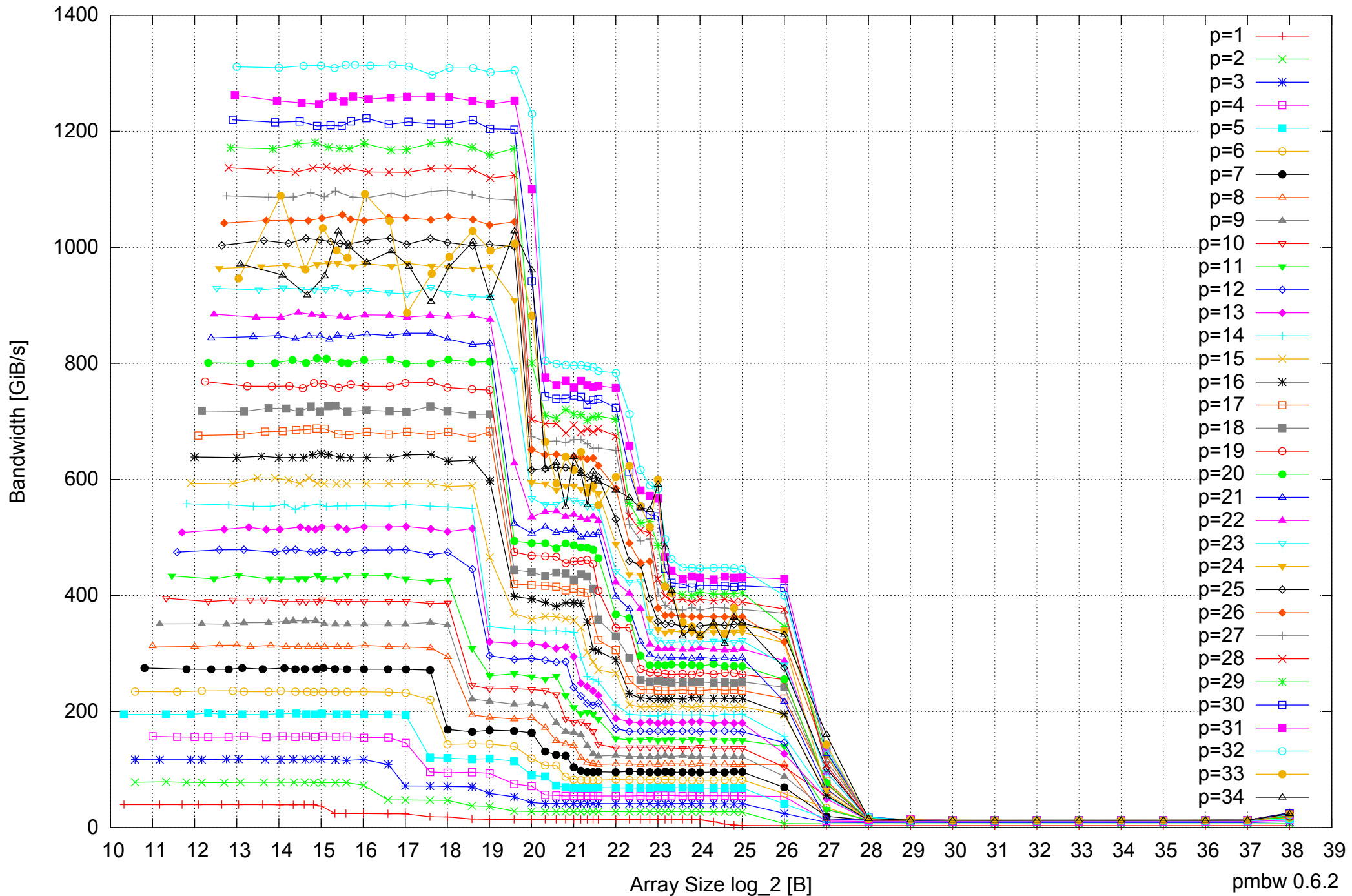
Intel Xeon E7-8837 512GB - Parallel Memory Bandwidth - ScanWrite128PtrUnrollLoop
