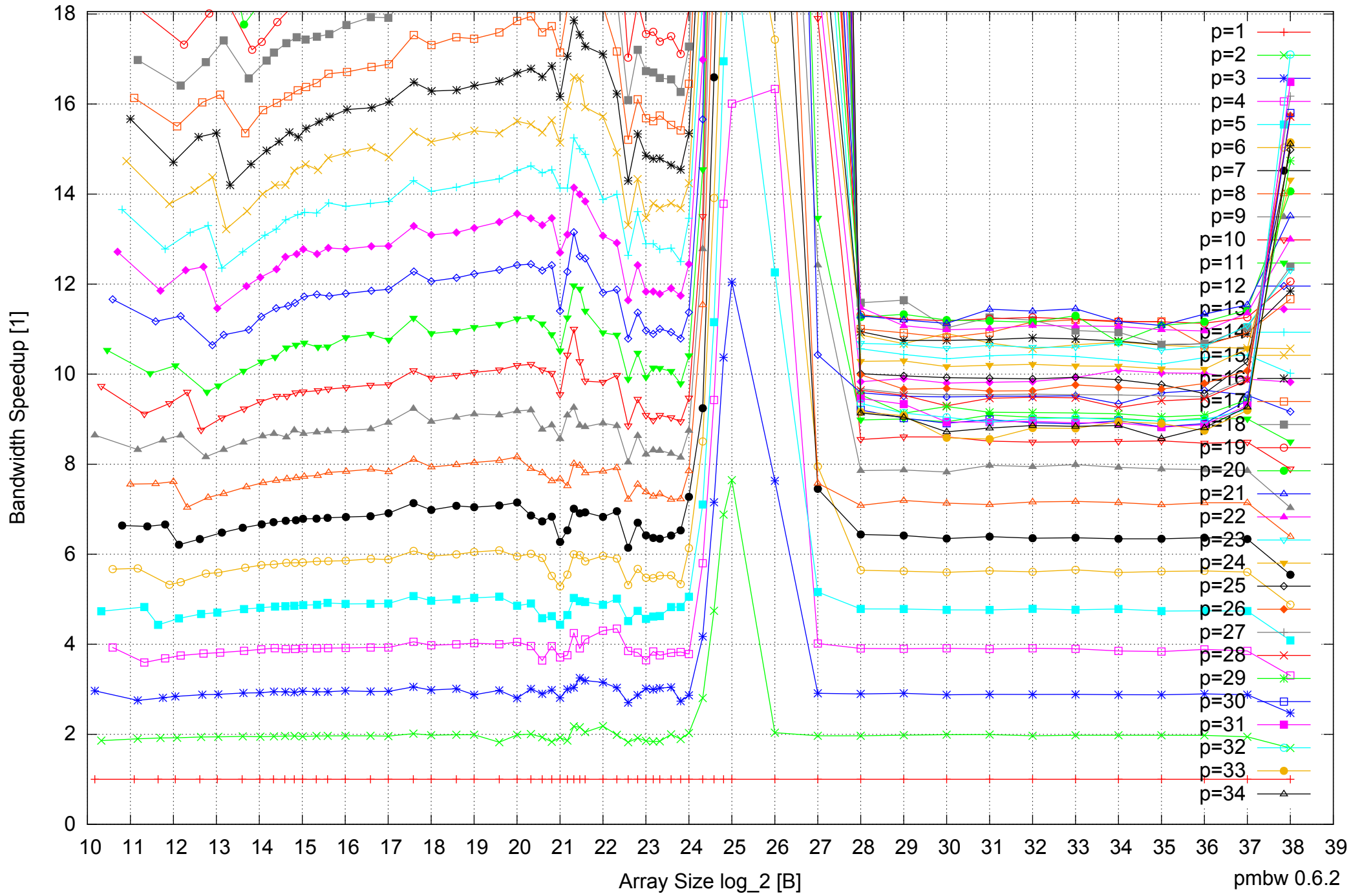
Intel Xeon E7-8837 512GB - Speedup of Parallel Memory Bandwidth (enlarged) - ScanRead64IndexSimpleLoop
