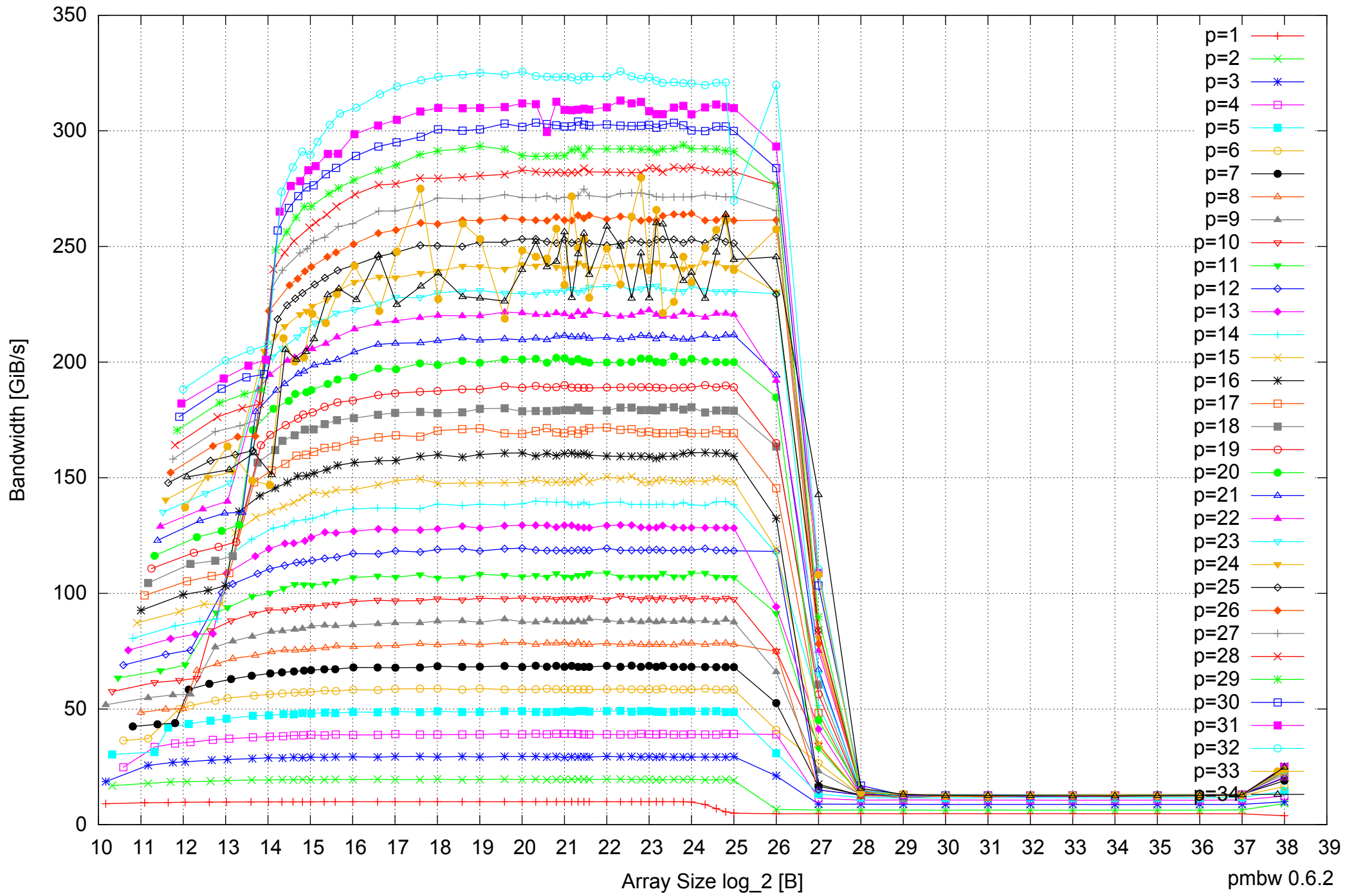
Intel Xeon E7-8837 512GB - Parallel Memory Bandwidth - ScanWrite64IndexSimpleLoop
