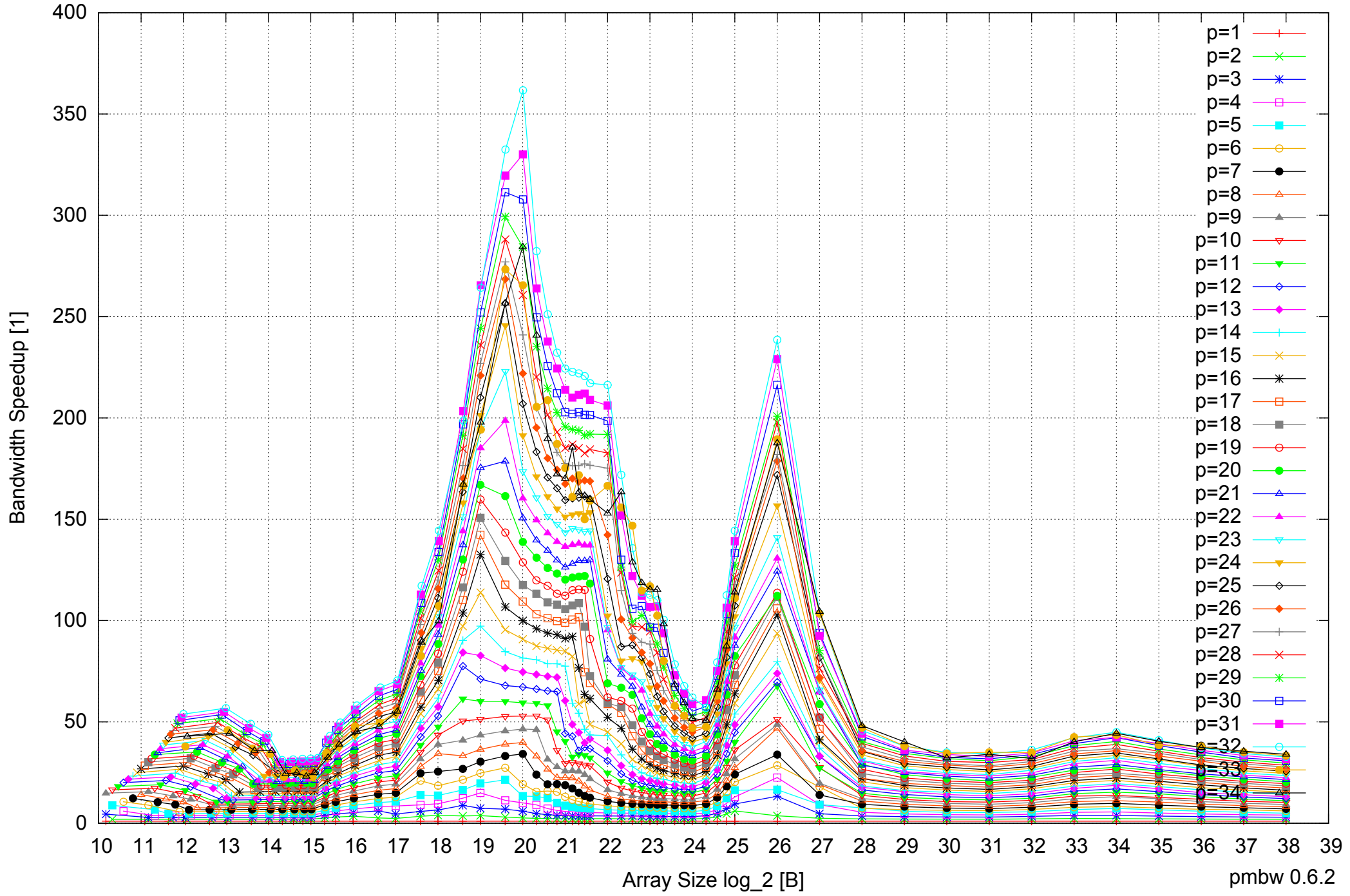
Intel Xeon E7-8837 512GB - Speedup of Parallel Memory Bandwidth - PermRead64SimpleLoop
