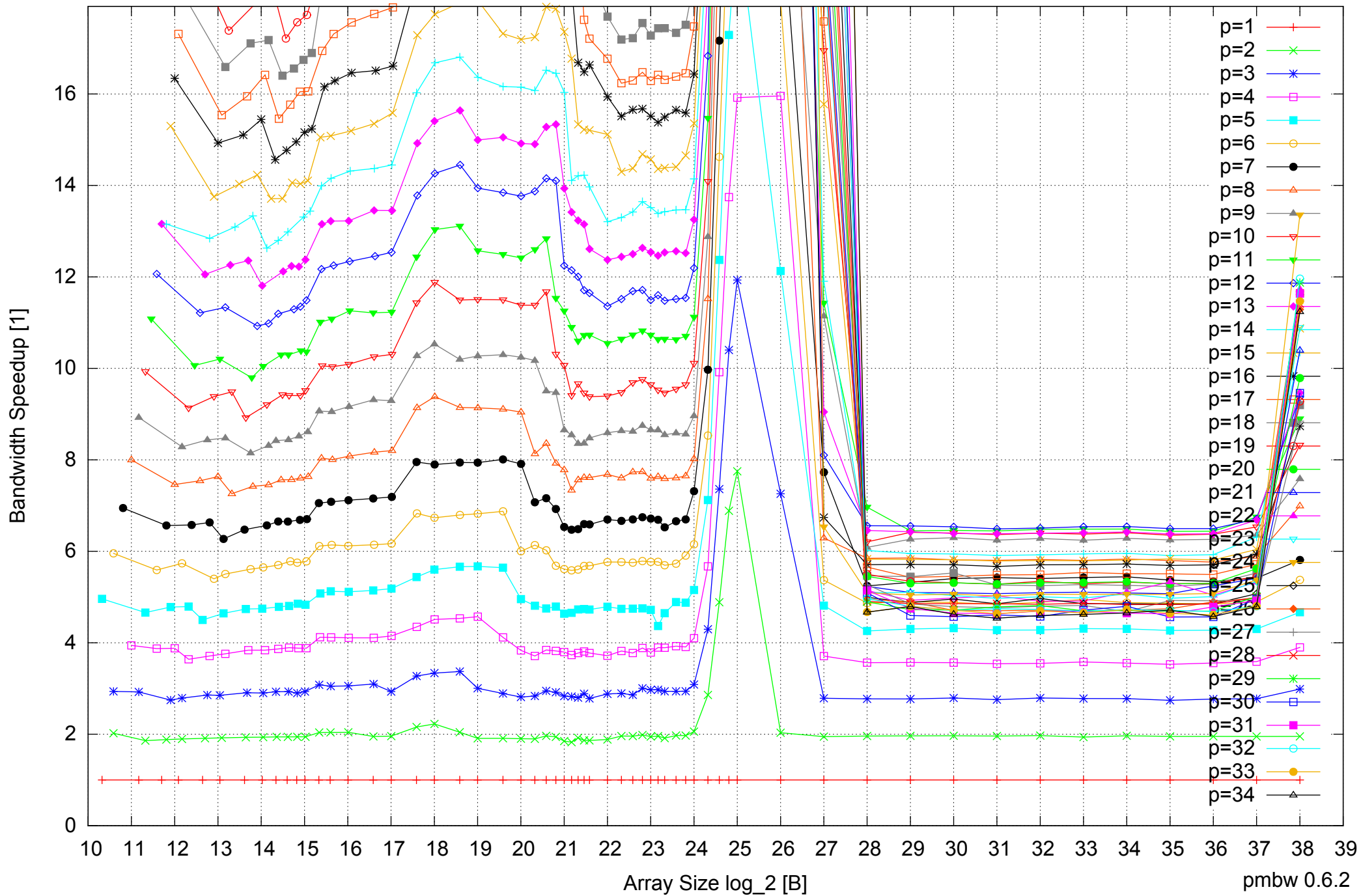
Intel Xeon E7-8837 512GB - Speedup of Parallel Memory Bandwidth (enlarged) - ScanRead128PtrSimpleLoop
