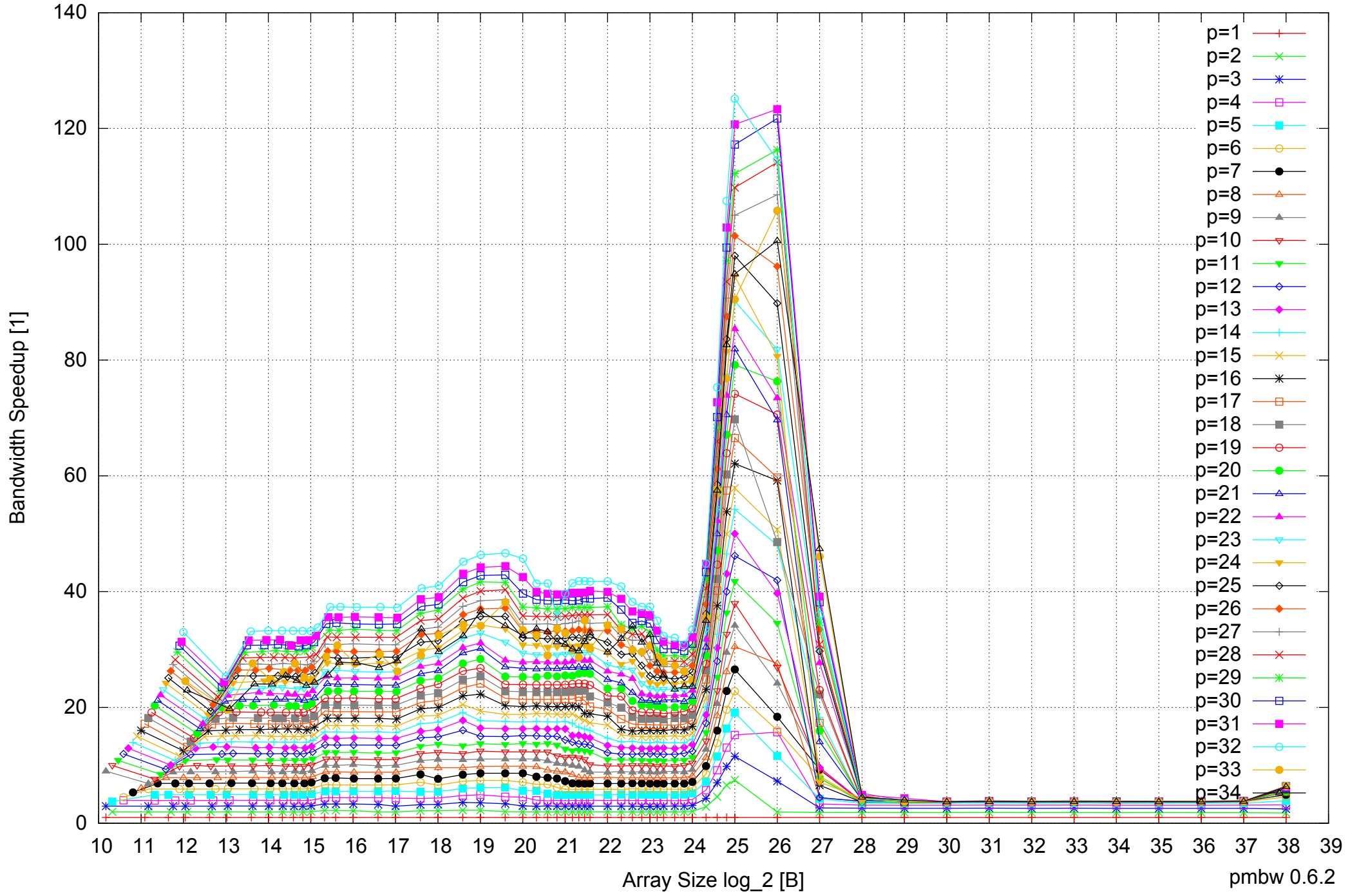
Intel Xeon E7-8837 512GB - Speedup of Parallel Memory Bandwidth - ScanWrite64PtrUnrollLoop
