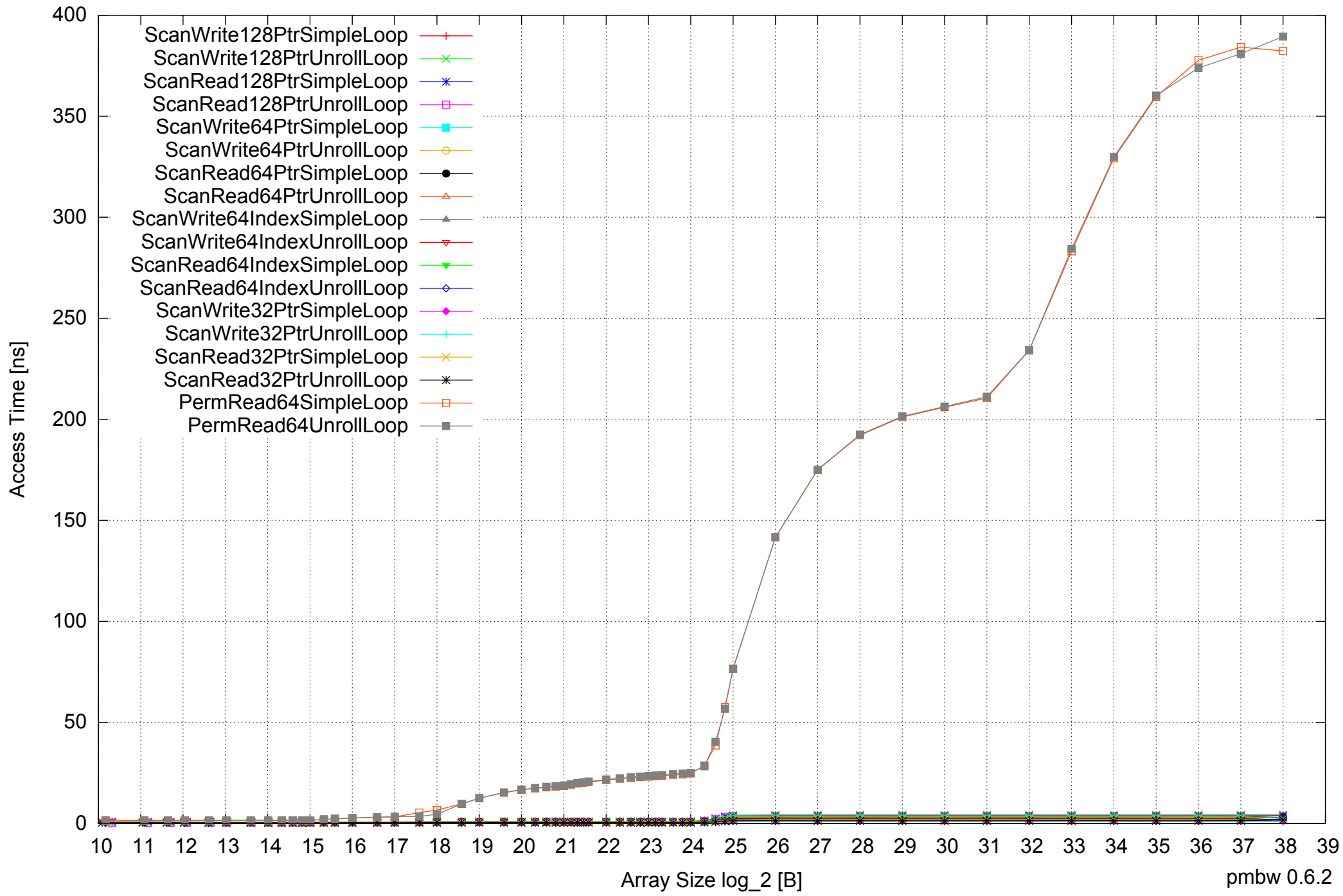
Intel Xeon E7-8837 512GB - One Thread Memory Latency (Access Time)
