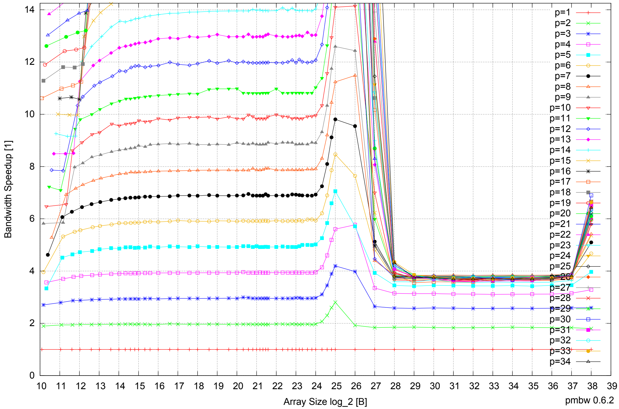
Intel Xeon E7-8837 512GB - Speedup of Parallel Memory Bandwidth (enlarged) - ScanWrite32PtrSimpleLoop
