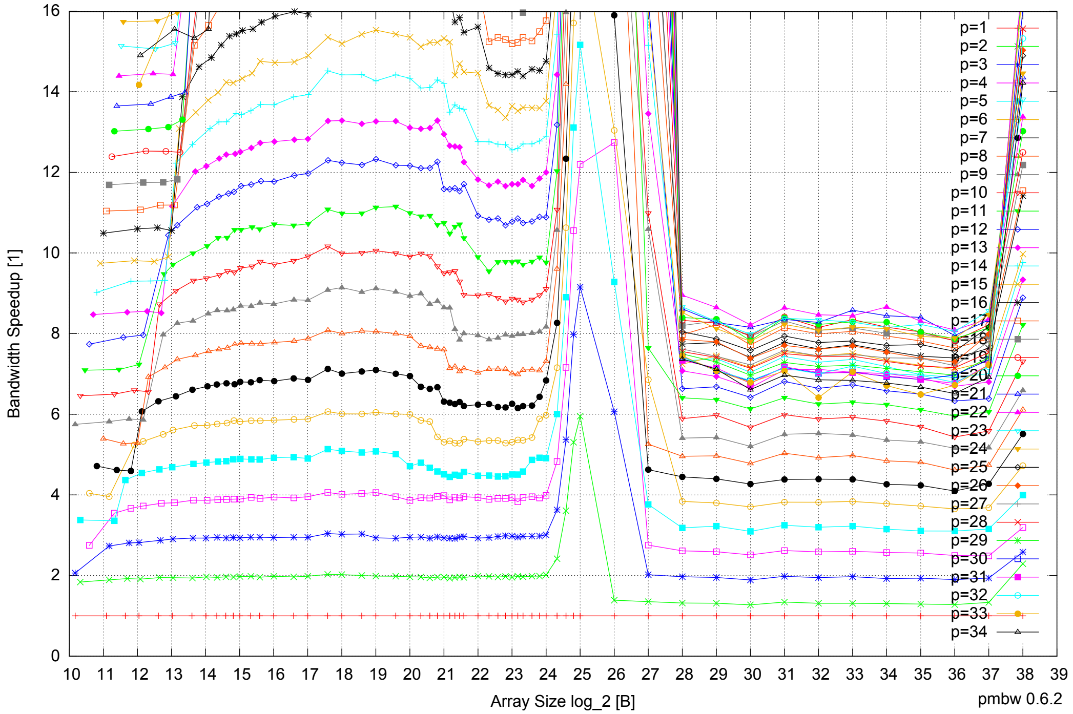
Intel Xeon E7-8837 512GB - Speedup of Parallel Memory Bandwidth (enlarged) - ScanRead64PtrSimpleLoop
