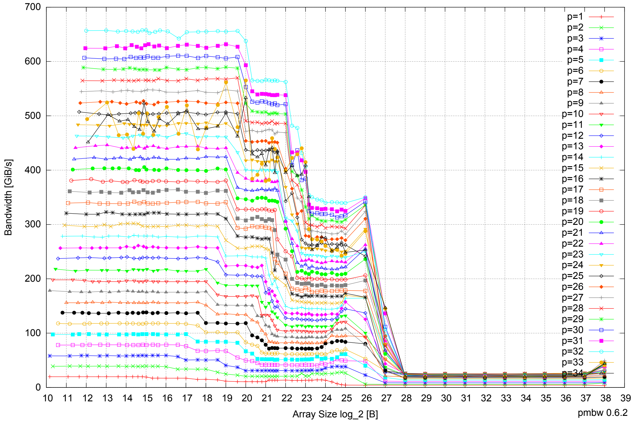
Intel Xeon E7-8837 512GB - Parallel Memory Bandwidth - ScanRead64IndexUnrollLoop
