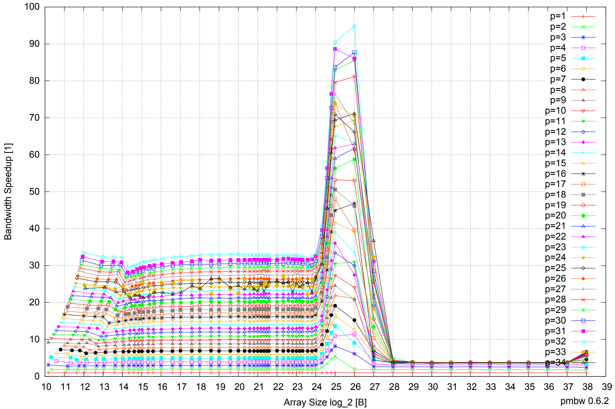
Intel Xeon E7-8837 512GB - Speedup of Parallel Memory Bandwidth - ScanWrite64PtrSimpleLoop
