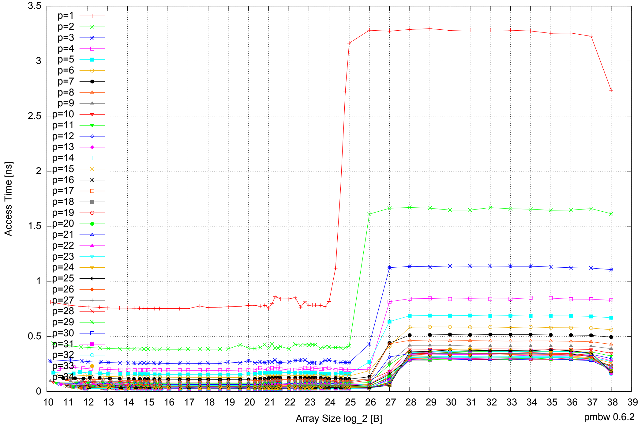
Intel Xeon E7-8837 512GB - Parallel Memory Access Time - ScanRead64IndexSimpleLoop
