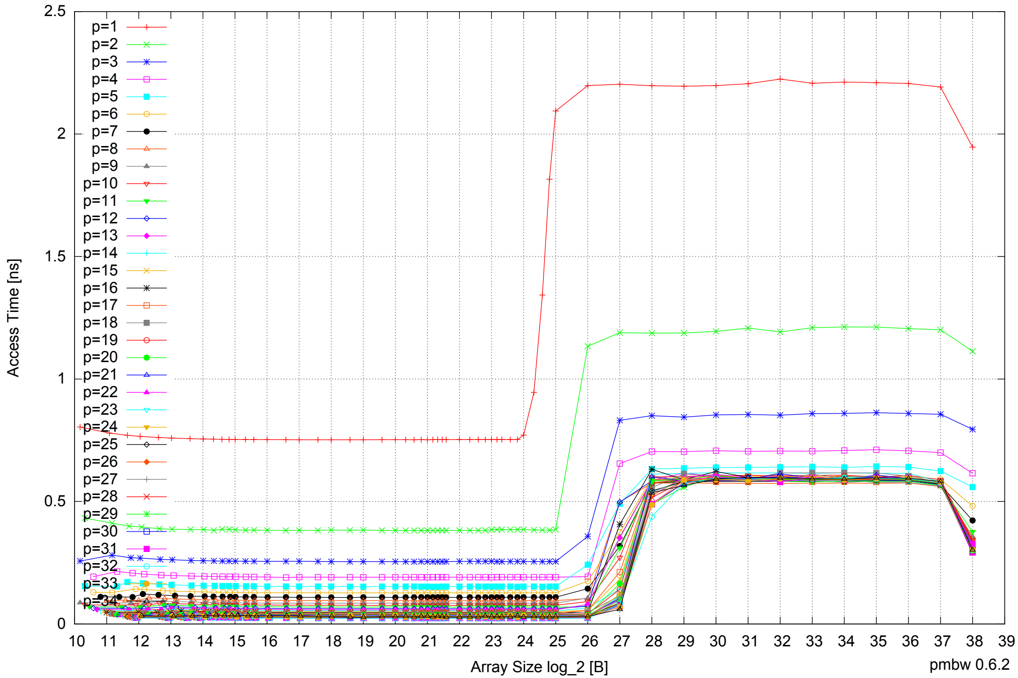
Intel Xeon E7-8837 512GB - Parallel Memory Access Time - ScanWrite64PtrSimpleLoop
