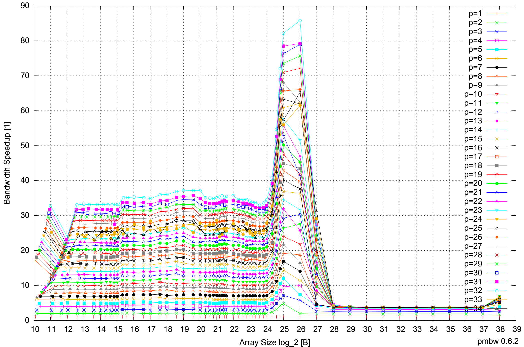
Intel Xeon E7-8837 512GB - Speedup of Parallel Memory Bandwidth - ScanWrite32PtrUnrollLoop
