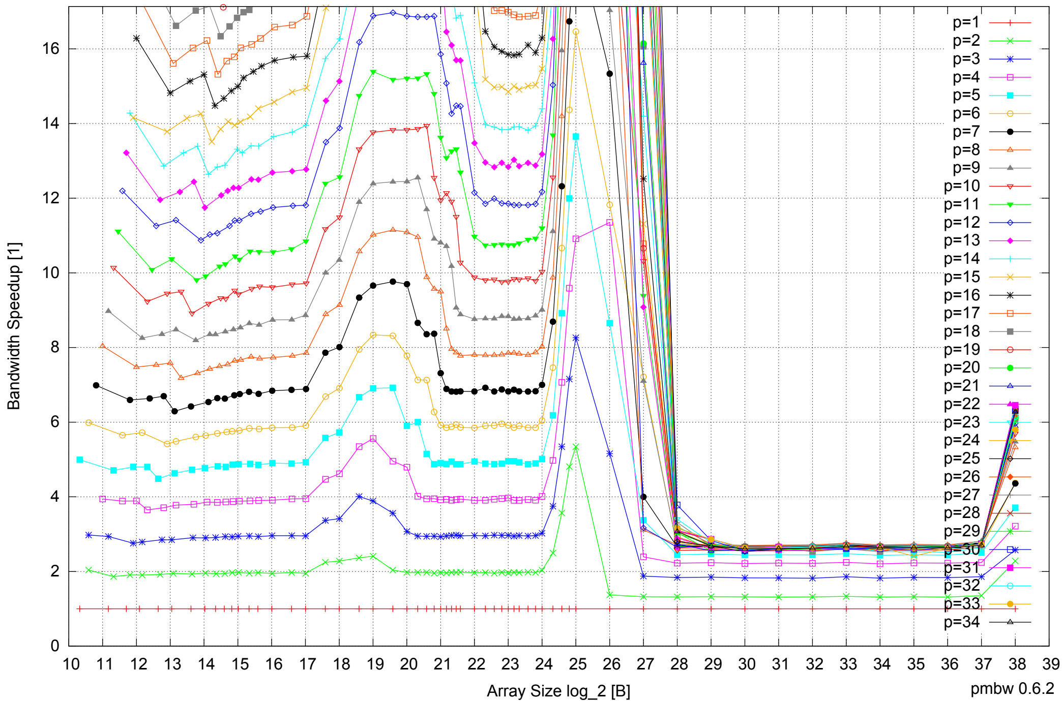
Intel Xeon E7-8837 512GB - Speedup of Parallel Memory Bandwidth (enlarged) - ScanWrite128PtrSimpleLoop
