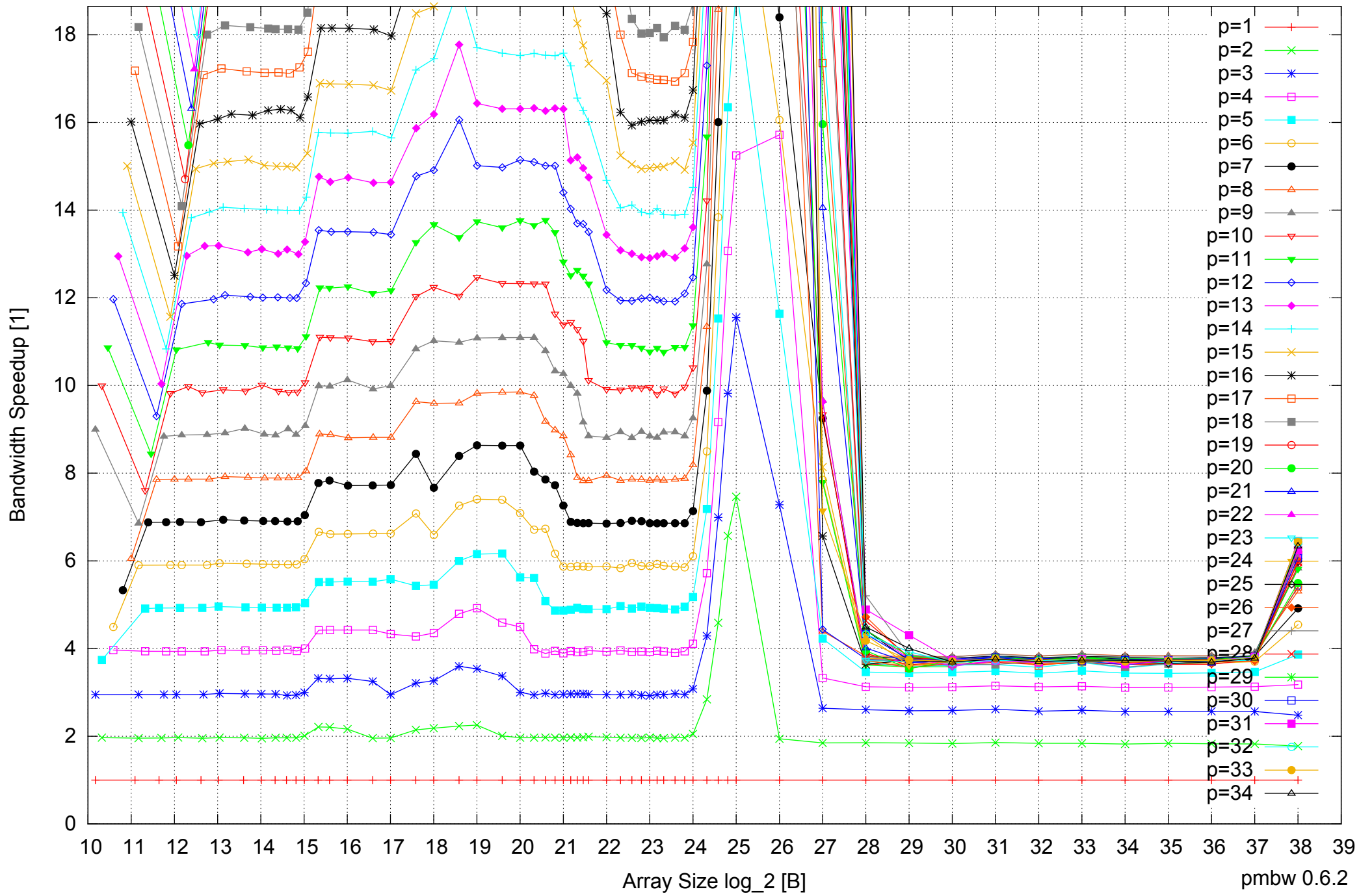
Intel Xeon E7-8837 512GB - Speedup of Parallel Memory Bandwidth (enlarged) - ScanWrite64PtrUnrollLoop
