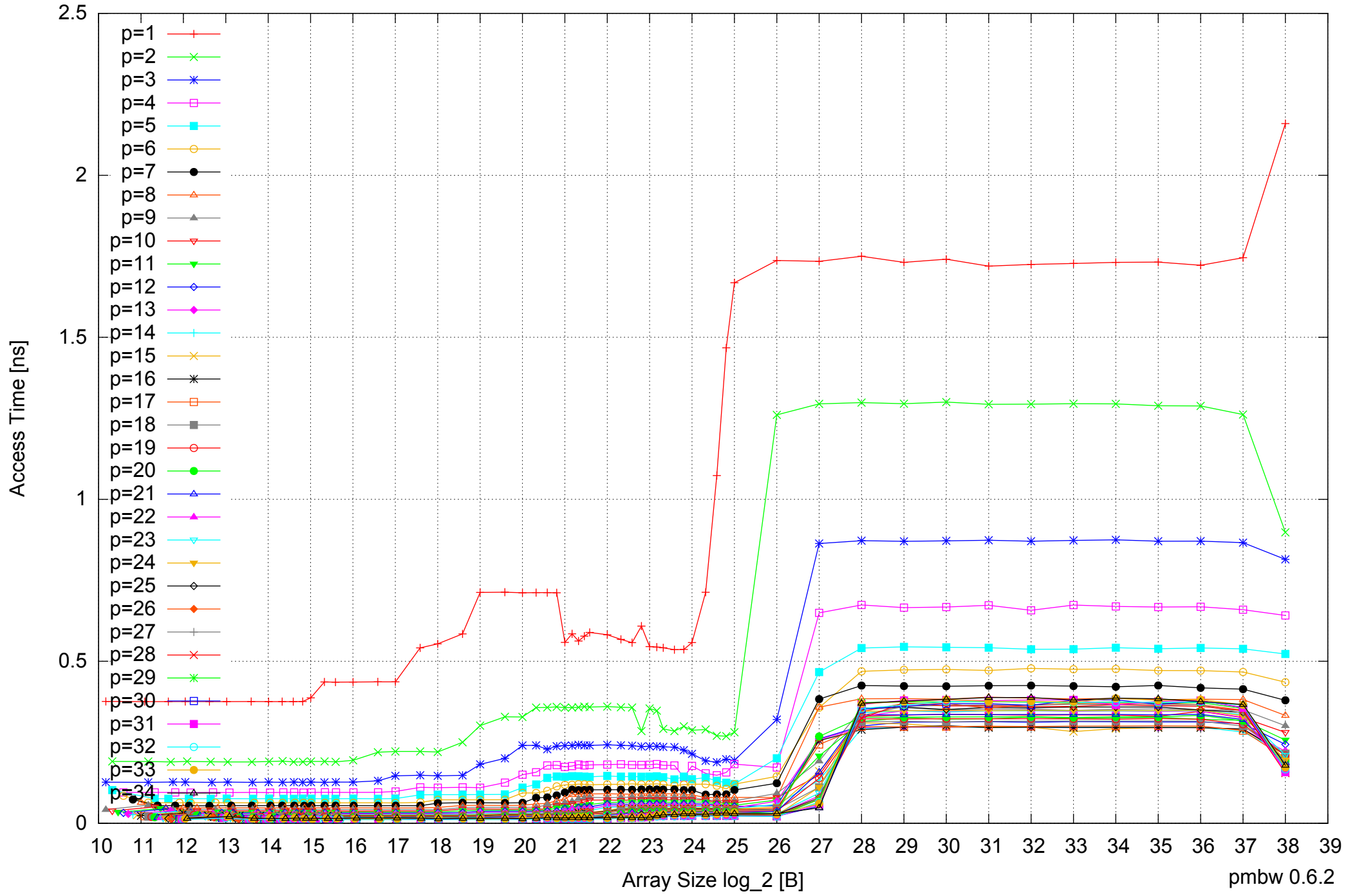
Intel Xeon E7-8837 512GB - Parallel Memory Access Time - ScanRead64PtrUnrollLoop
