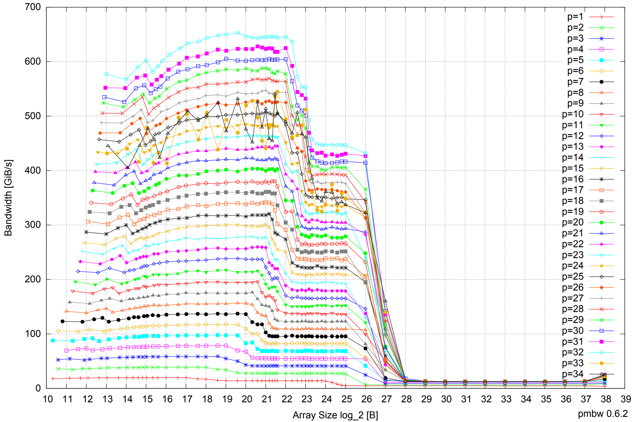
Intel Xeon E7-8837 512GB - Parallel Memory Bandwidth - ScanWrite128PtrSimpleLoop
