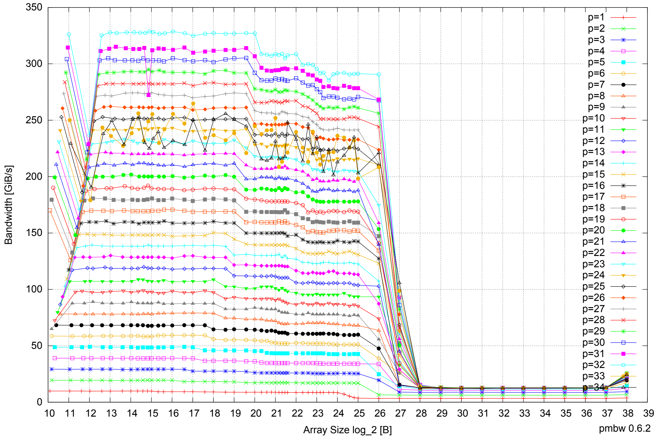
Intel Xeon E7-8837 512GB - Parallel Memory Bandwidth - ScanWrite32PtrUnrollLoop
