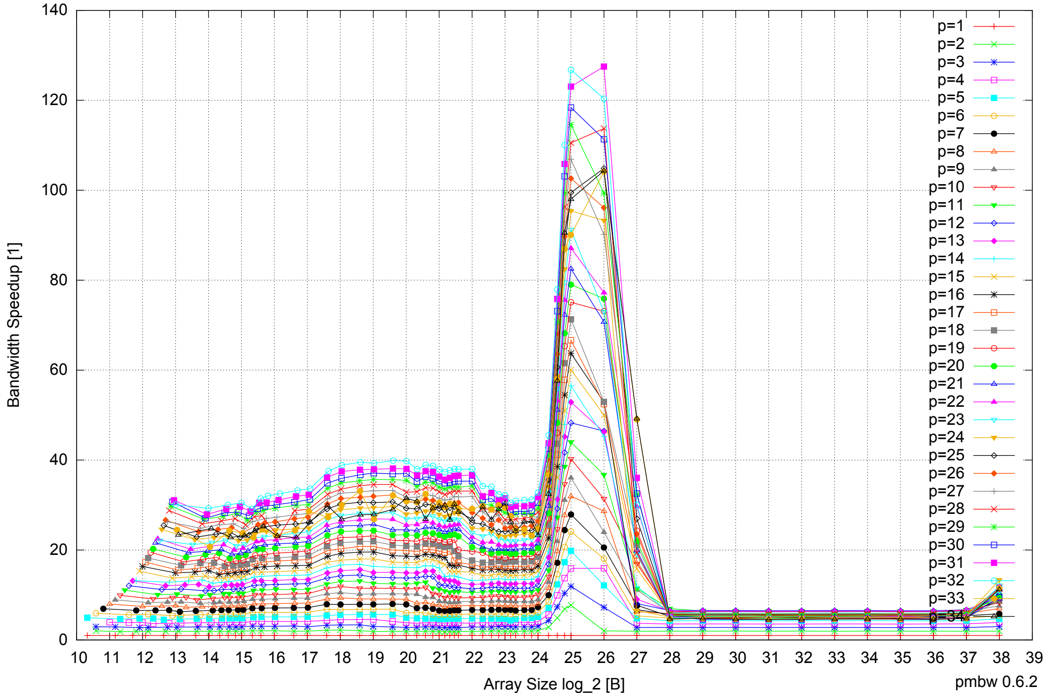
Intel Xeon E7-8837 512GB - Speedup of Parallel Memory Bandwidth - ScanRead128PtrSimpleLoop
