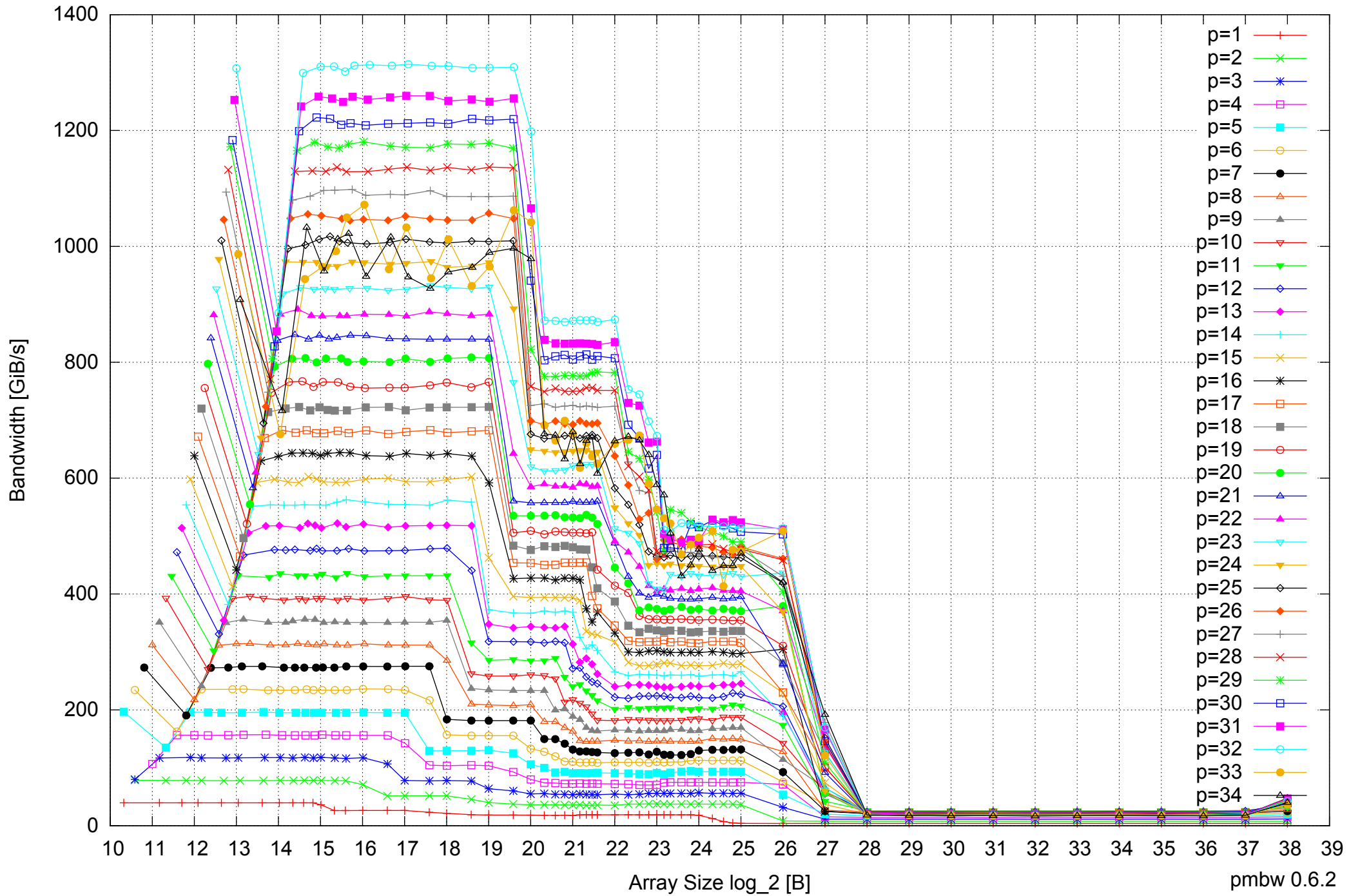
Intel Xeon E7-8837 512GB - Parallel Memory Bandwidth - ScanRead128PtrUnrollLoop
