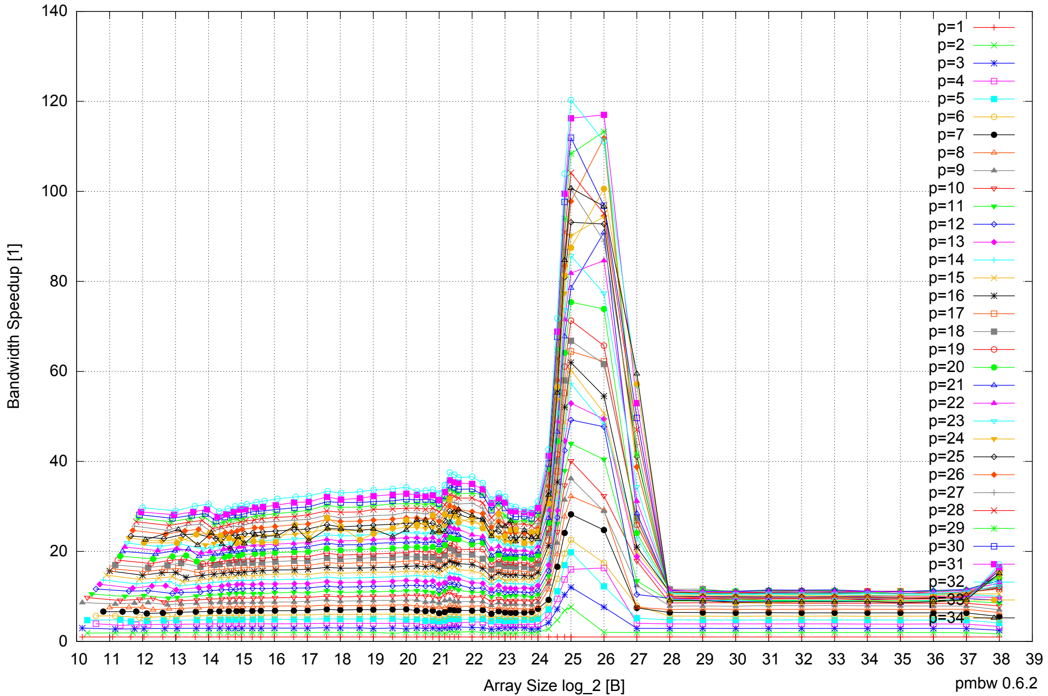
Intel Xeon E7-8837 512GB - Speedup of Parallel Memory Bandwidth - ScanRead64IndexSimpleLoop
