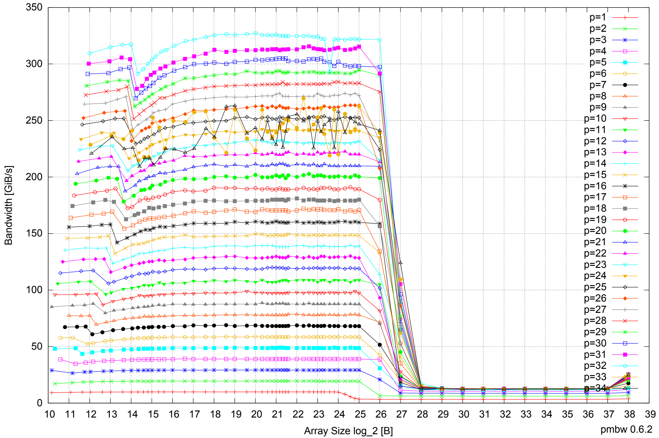
Intel Xeon E7-8837 512GB - Parallel Memory Bandwidth - ScanWrite64PtrSimpleLoop
