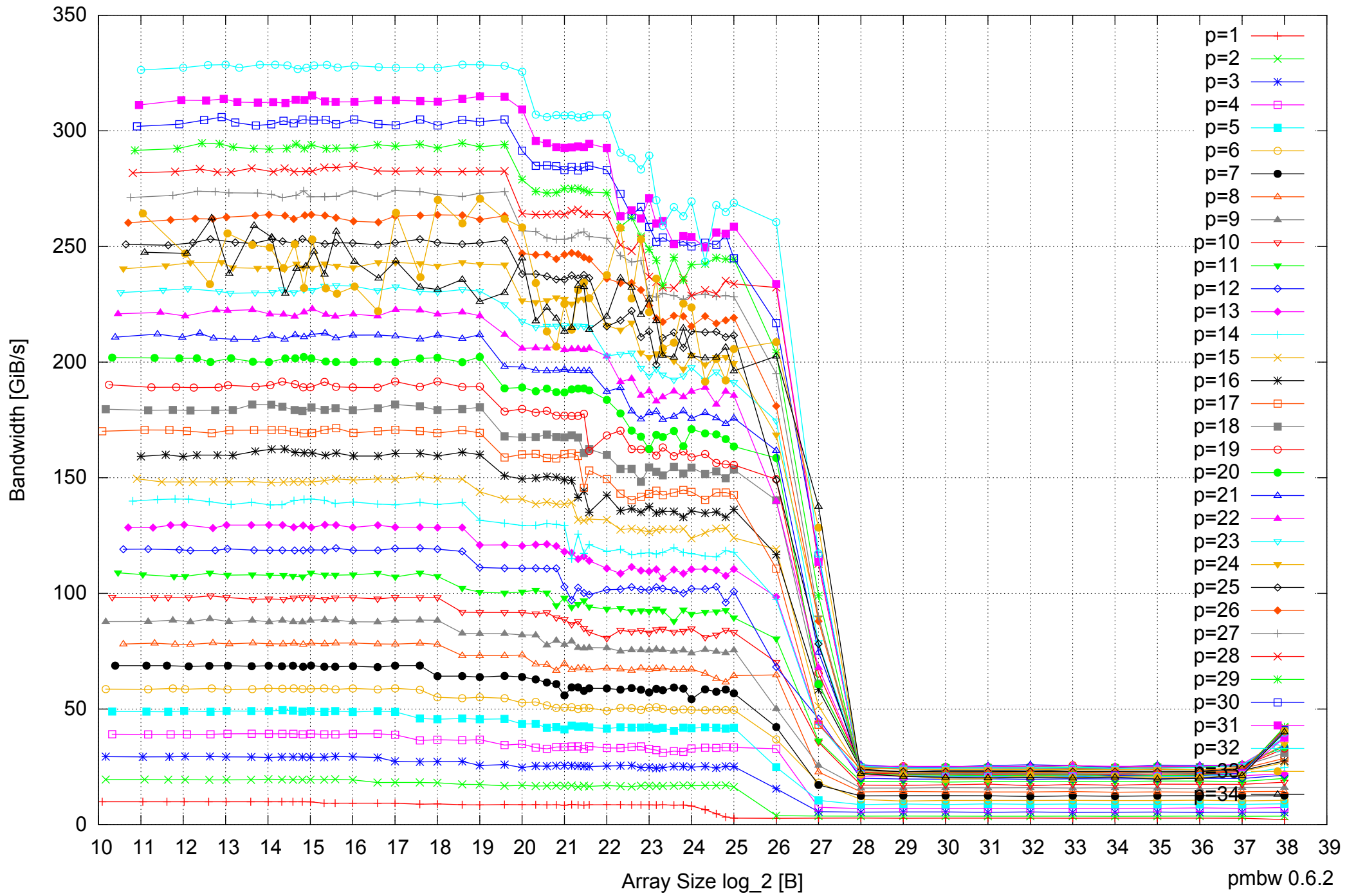
Intel Xeon E7-8837 512GB - Parallel Memory Bandwidth - ScanRead32PtrUnrollLoop
