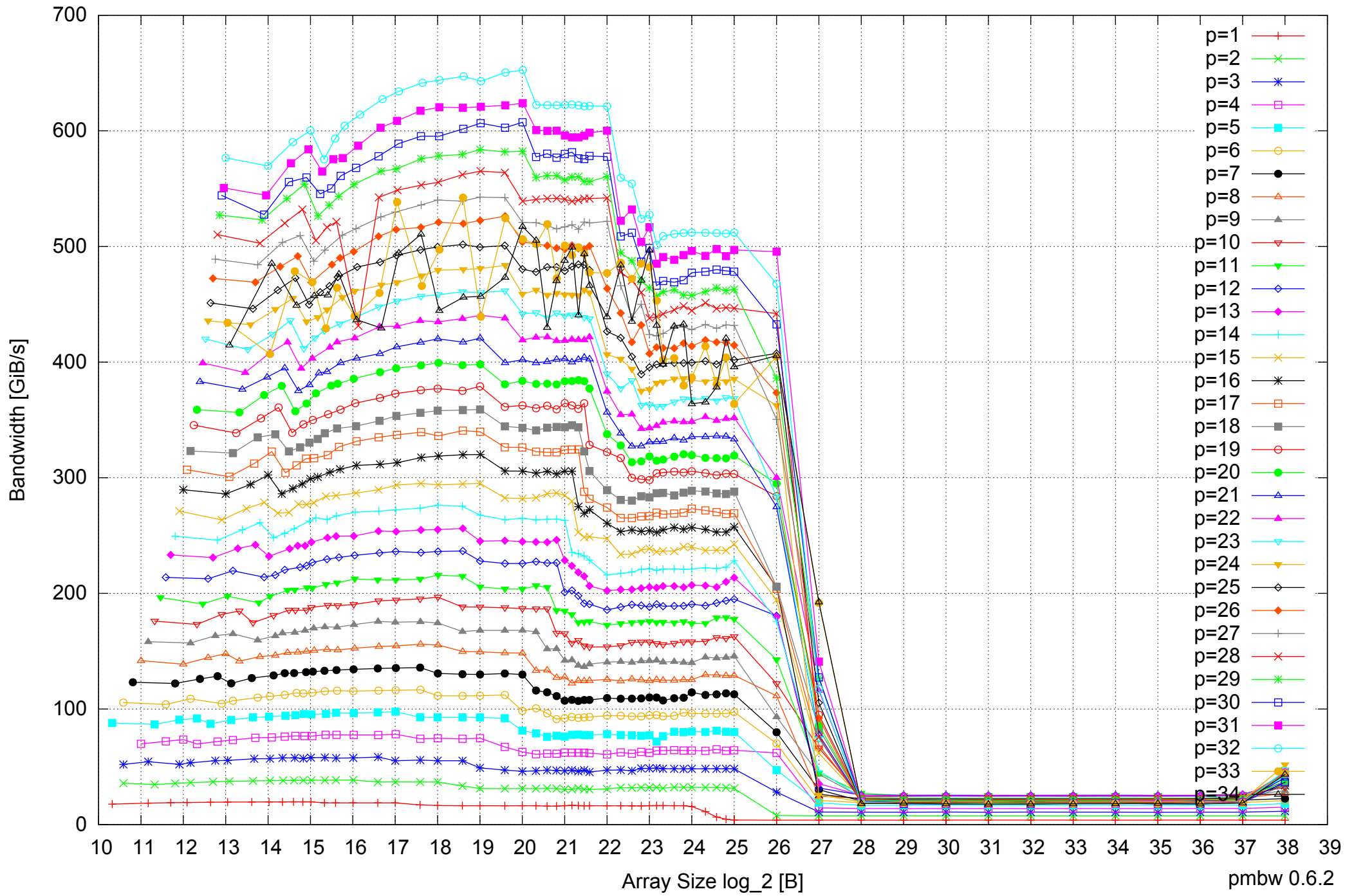
Intel Xeon E7-8837 512GB - Parallel Memory Bandwidth - ScanRead128PtrSimpleLoop
