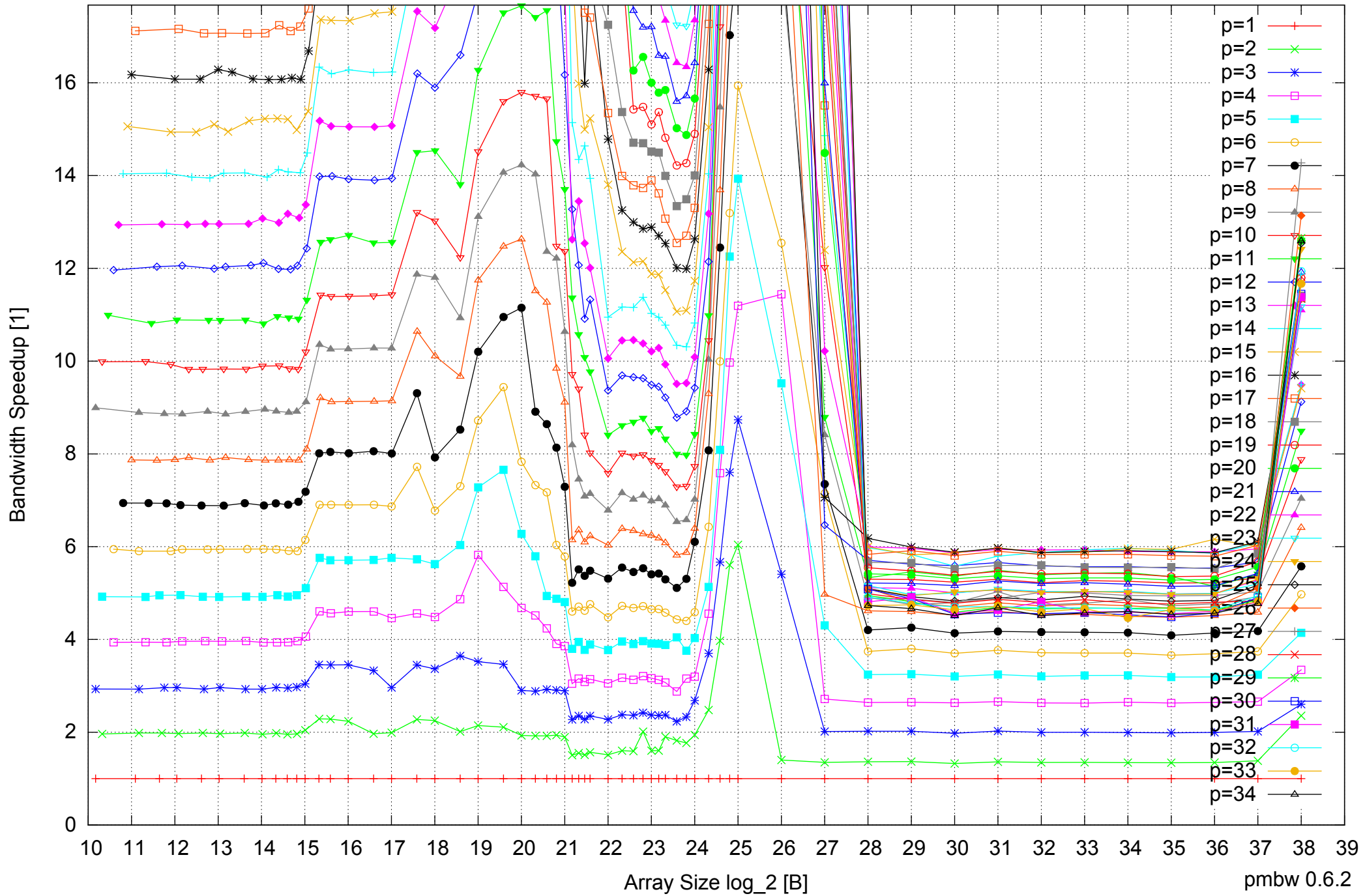
Intel Xeon E7-8837 512GB - Speedup of Parallel Memory Bandwidth (enlarged) - ScanRead64IndexUnrollLoop
