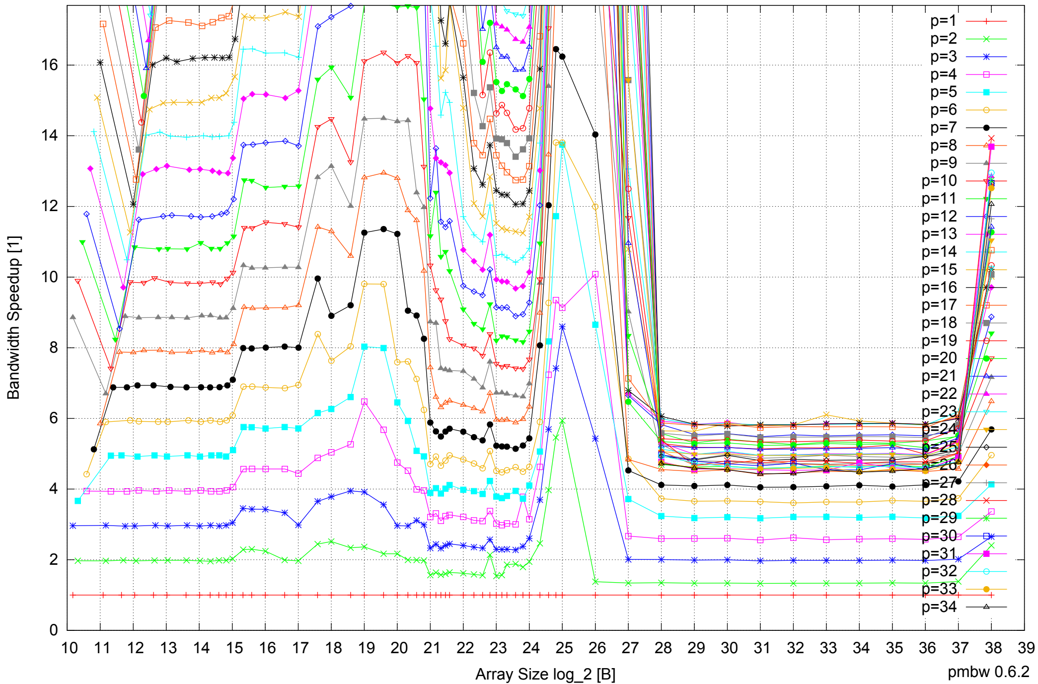
Intel Xeon E7-8837 512GB - Speedup of Parallel Memory Bandwidth (enlarged) - ScanRead64PtrUnrollLoop
