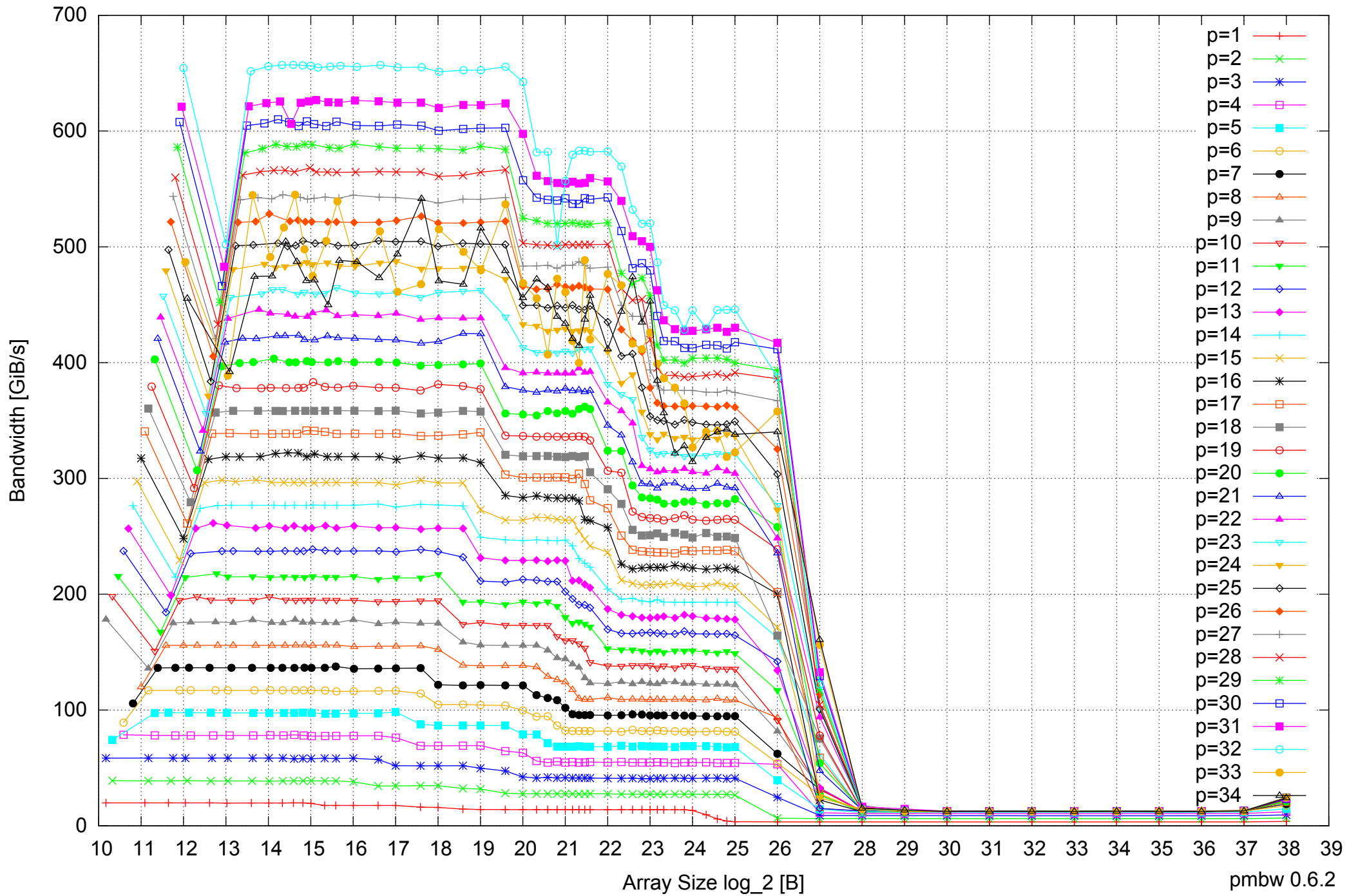
Intel Xeon E7-8837 512GB - Parallel Memory Bandwidth - ScanWrite64PtrUnrollLoop
