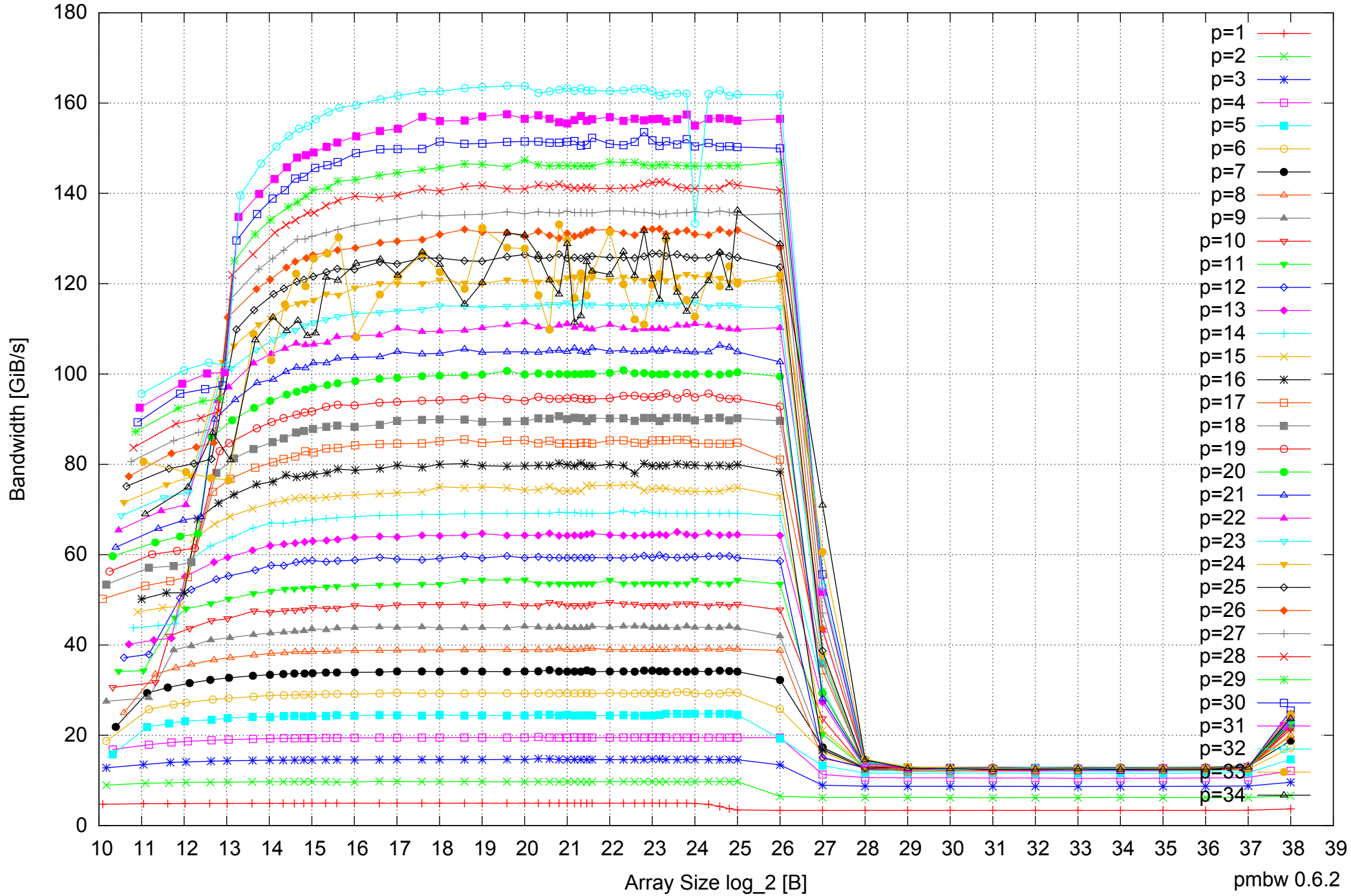
Intel Xeon E7-8837 512GB - Parallel Memory Bandwidth - ScanWrite32PtrSimpleLoop
