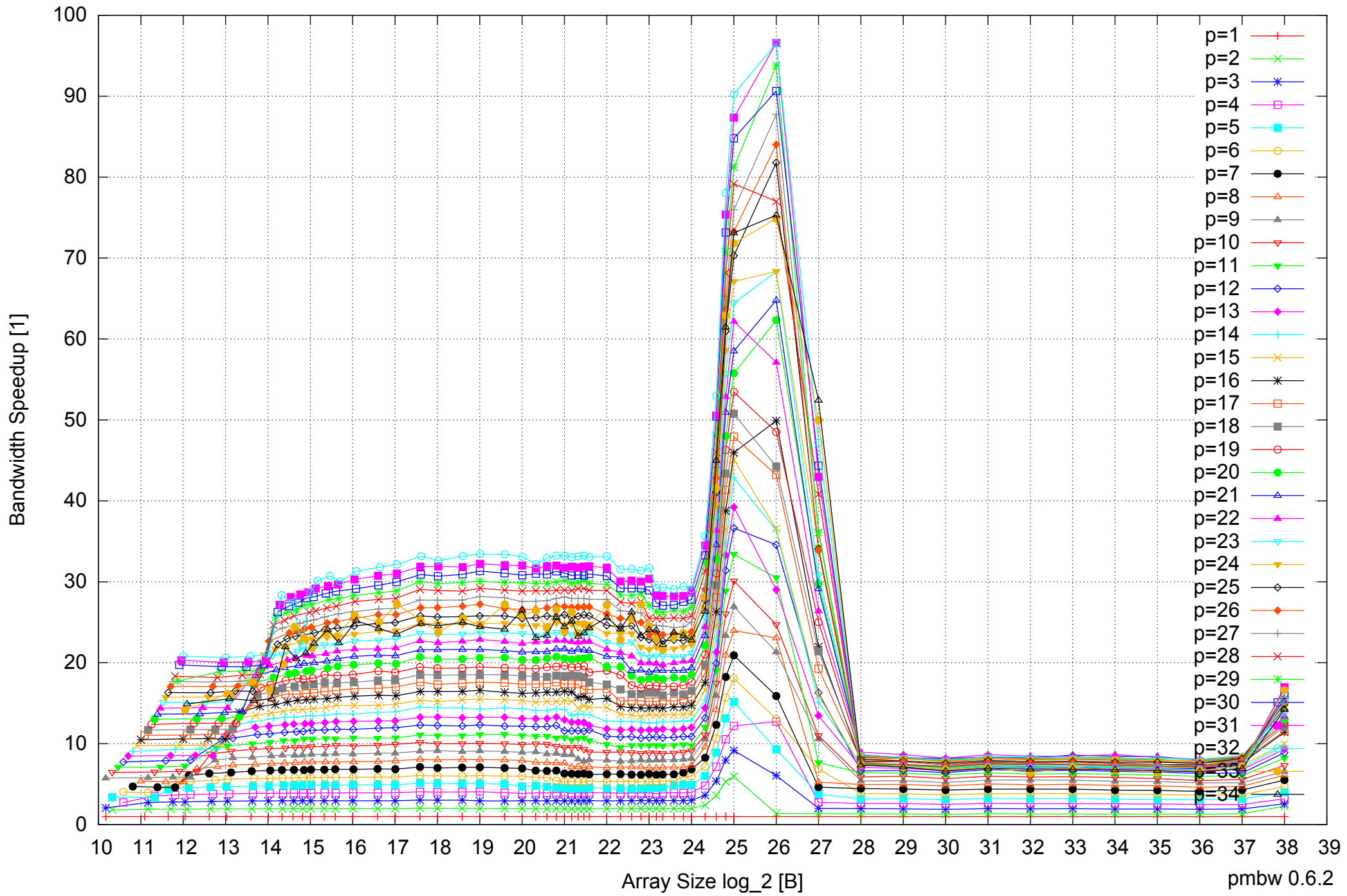
Intel Xeon E7-8837 512GB - Speedup of Parallel Memory Bandwidth - ScanRead64PtrSimpleLoop
