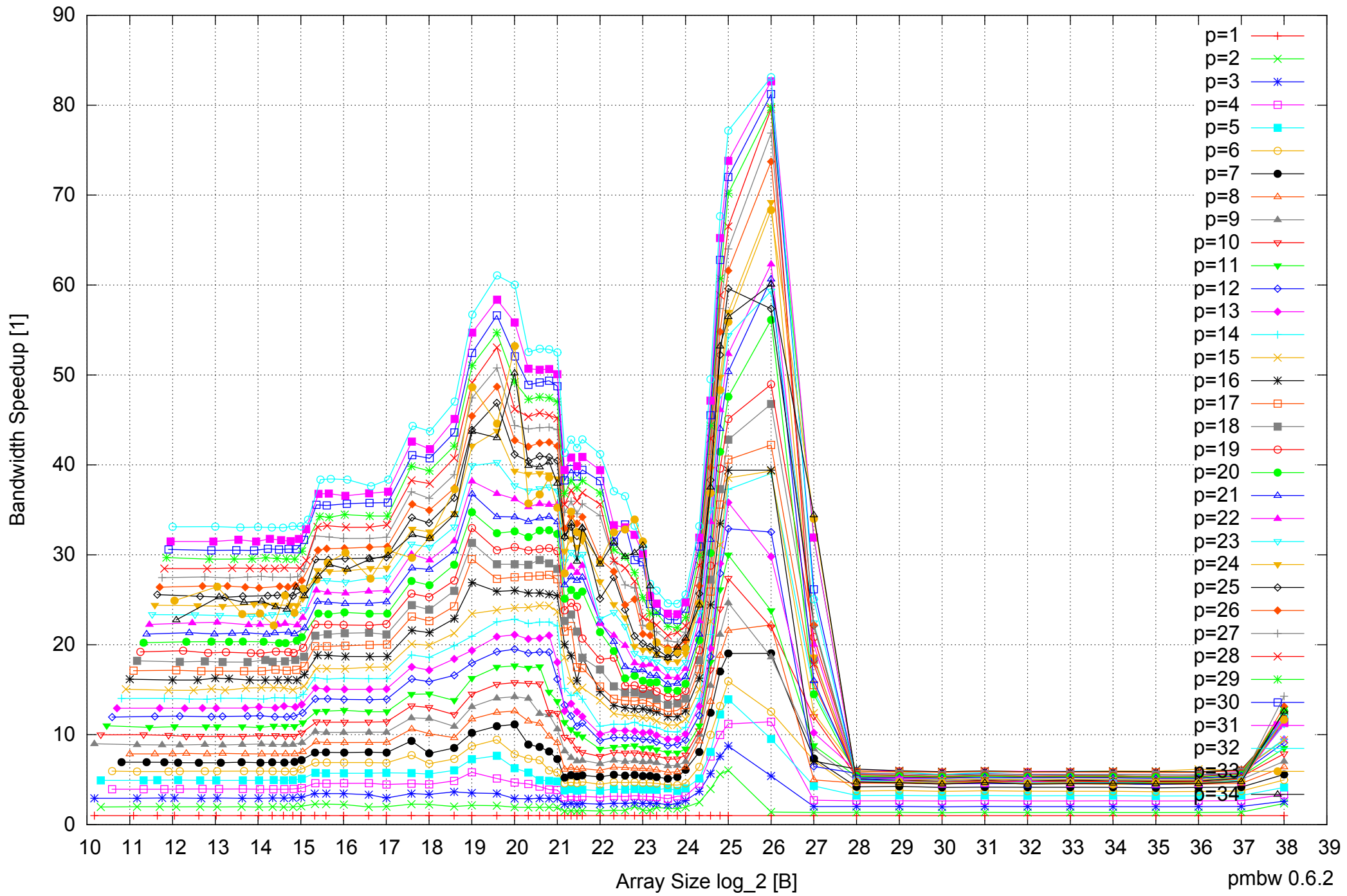
Intel Xeon E7-8837 512GB - Speedup of Parallel Memory Bandwidth - ScanRead64IndexUnrollLoop
