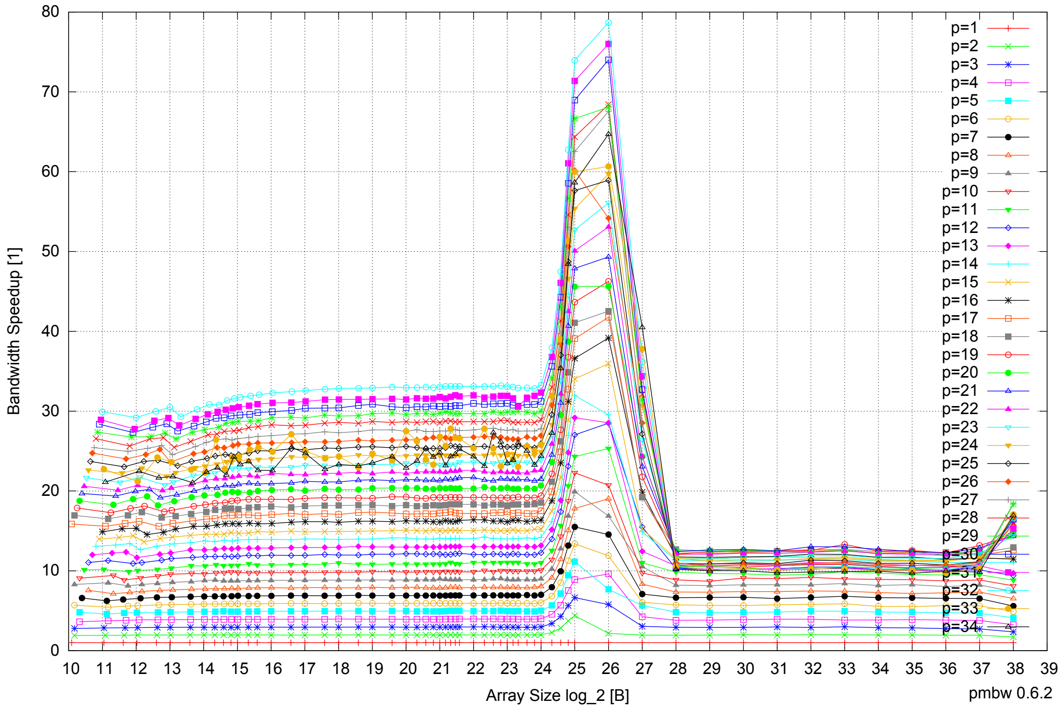
Intel Xeon E7-8837 512GB - Speedup of Parallel Memory Bandwidth - ScanRead32PtrSimpleLoop
