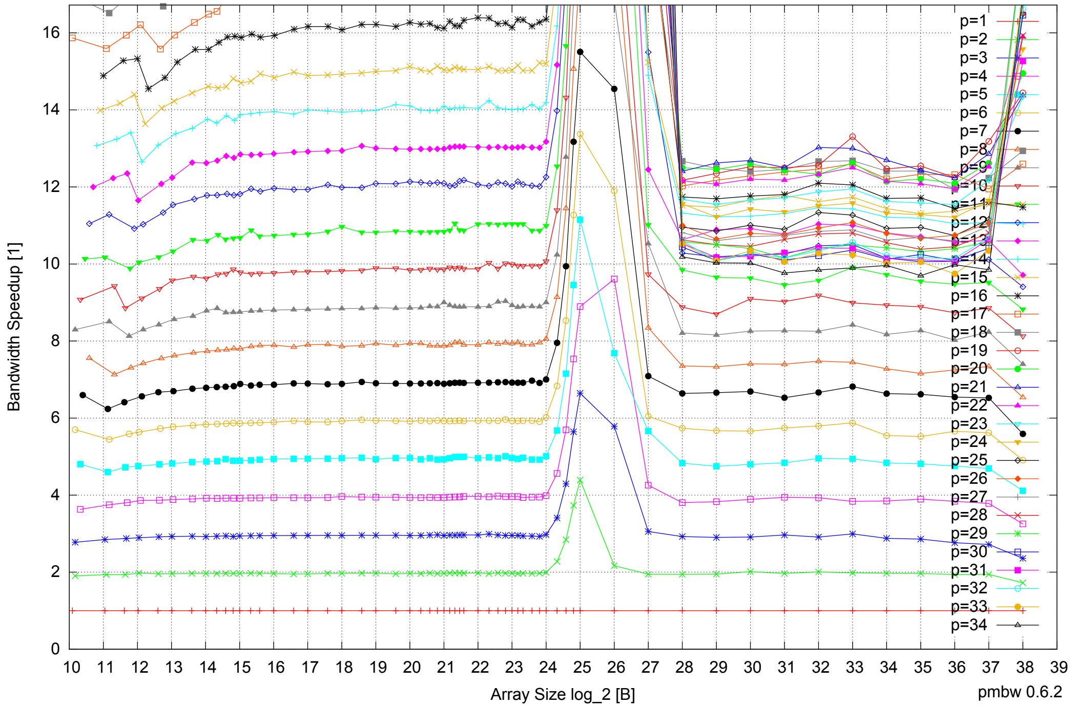
Intel Xeon E7-8837 512GB - Speedup of Parallel Memory Bandwidth (enlarged) - ScanRead32PtrSimpleLoop
