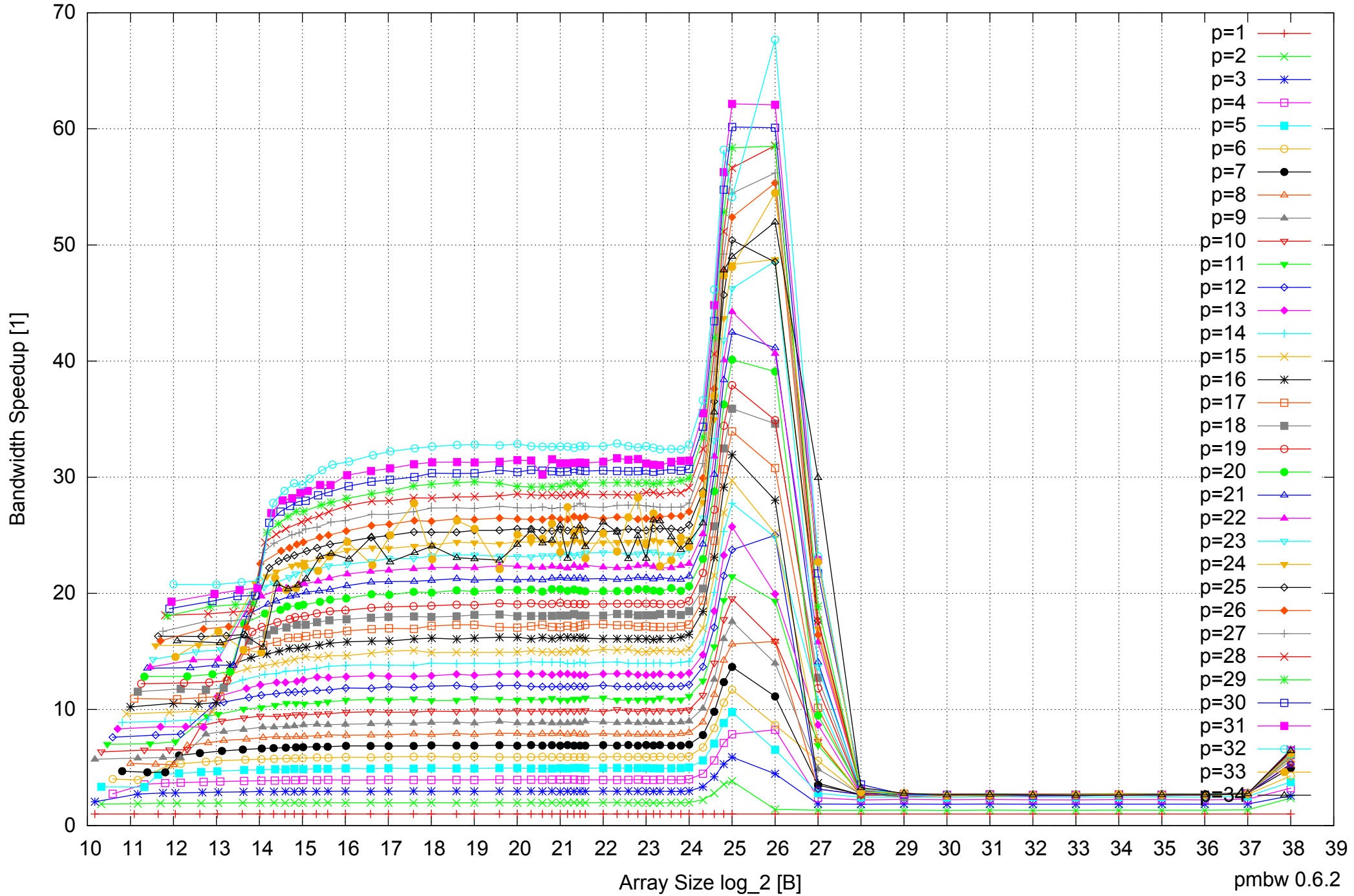
Intel Xeon E7-8837 512GB - Speedup of Parallel Memory Bandwidth - ScanWrite64IndexSimpleLoop
