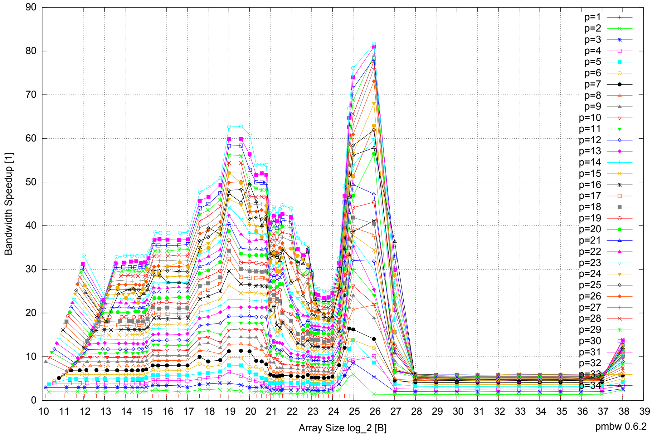
Intel Xeon E7-8837 512GB - Speedup of Parallel Memory Bandwidth - ScanRead64PtrUnrollLoop
