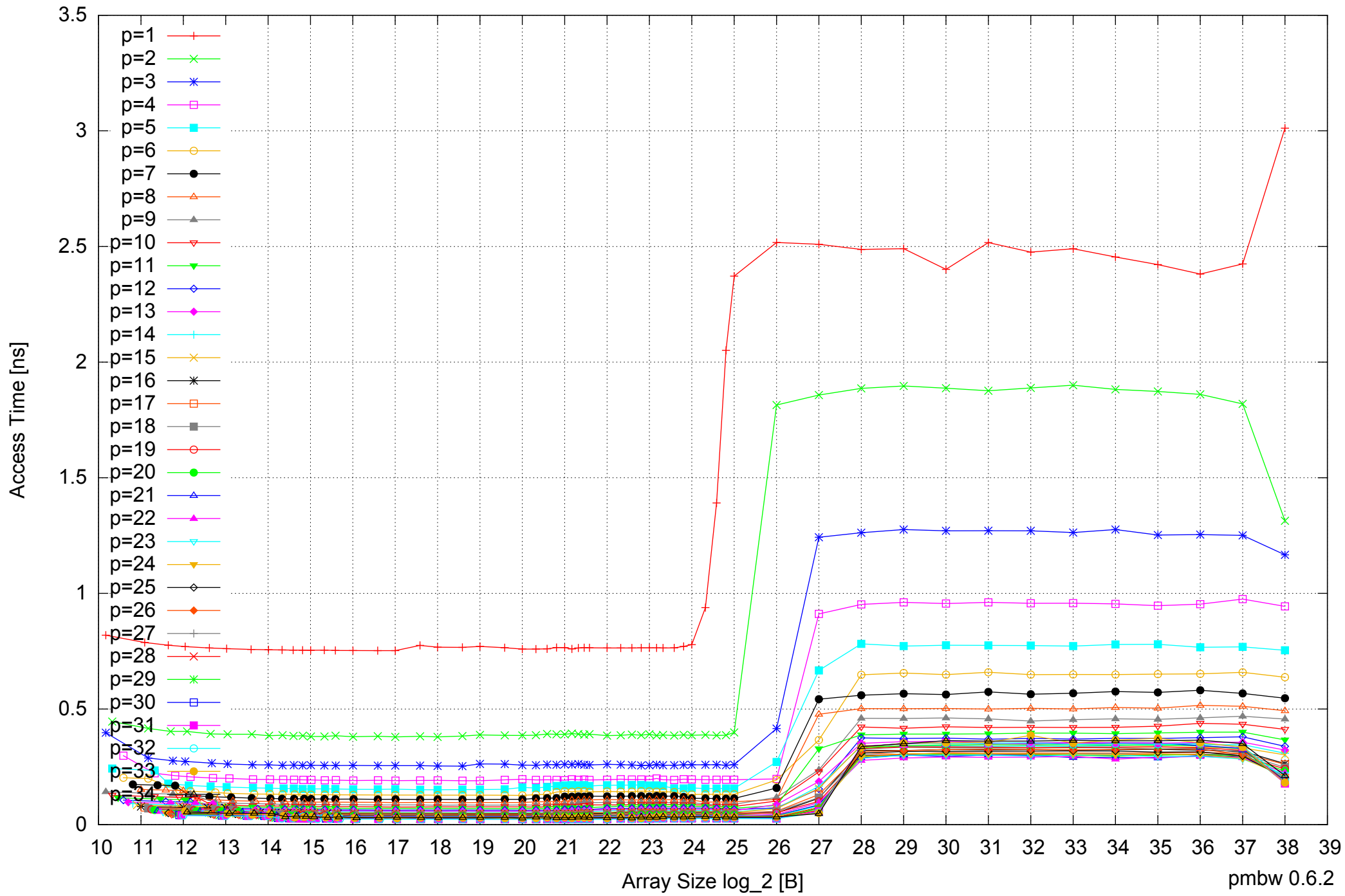
Intel Xeon E7-8837 512GB - Parallel Memory Access Time - ScanRead64PtrSimpleLoop
