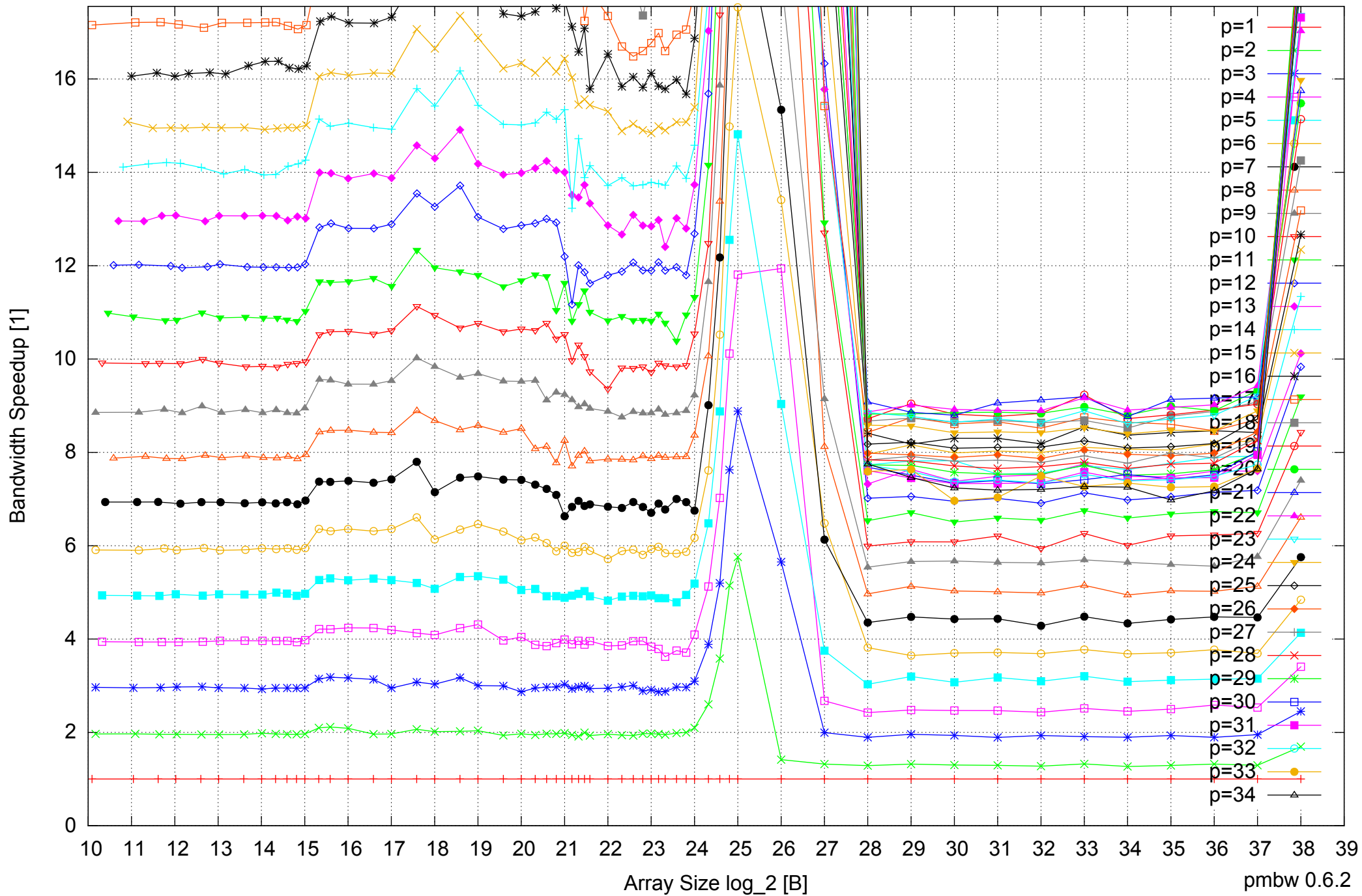
Intel Xeon E7-8837 512GB - Speedup of Parallel Memory Bandwidth (enlarged) - ScanRead32PtrUnrollLoop
