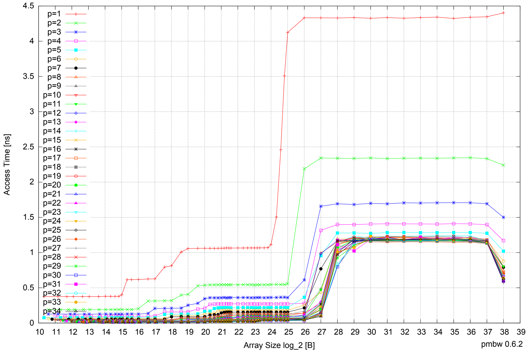
Intel Xeon E7-8837 512GB - Parallel Memory Access Time - ScanWrite128PtrUnrollLoop
