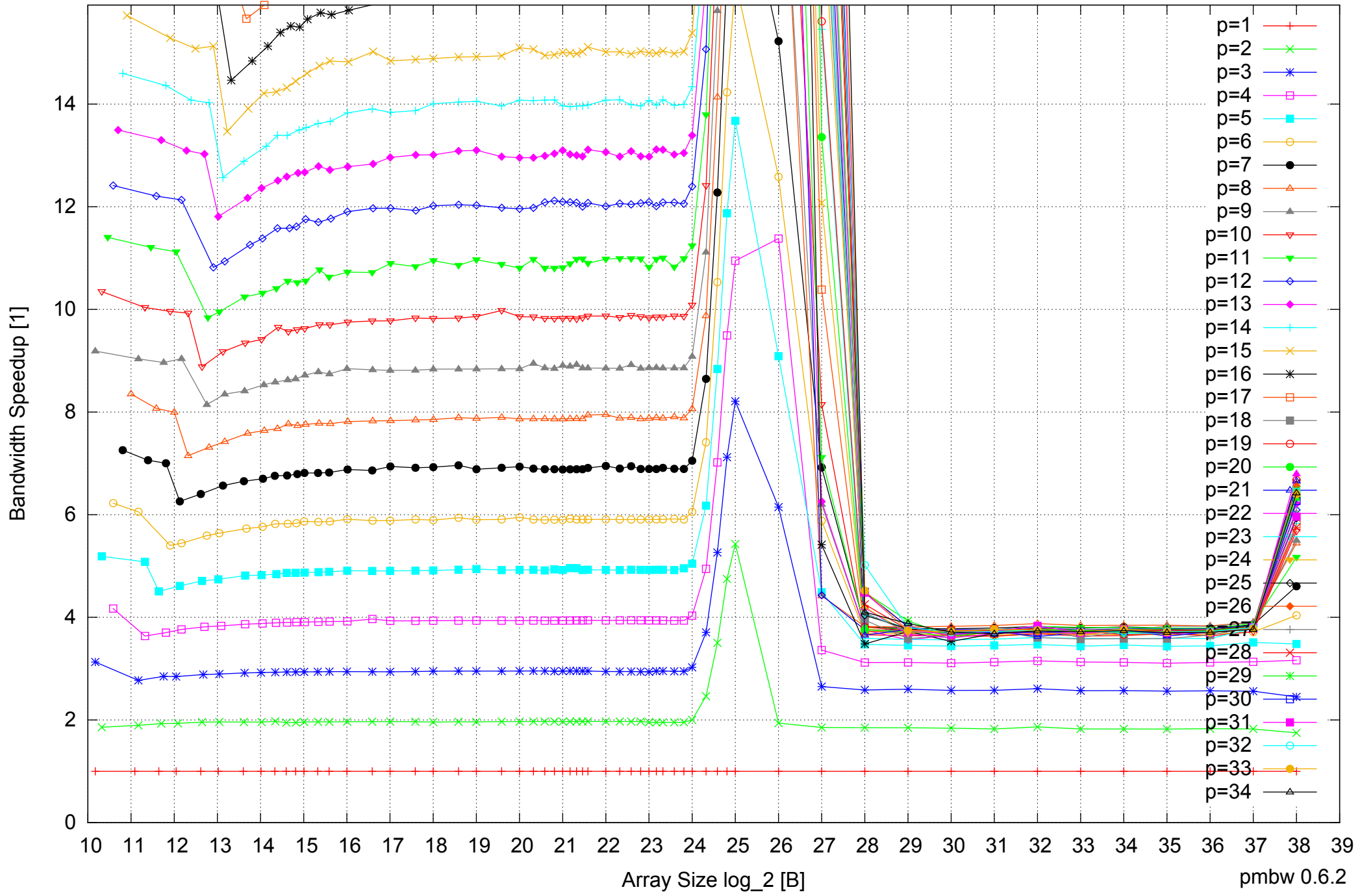
Intel Xeon E7-8837 512GB - Speedup of Parallel Memory Bandwidth (enlarged) - ScanWrite64PtrSimpleLoop
