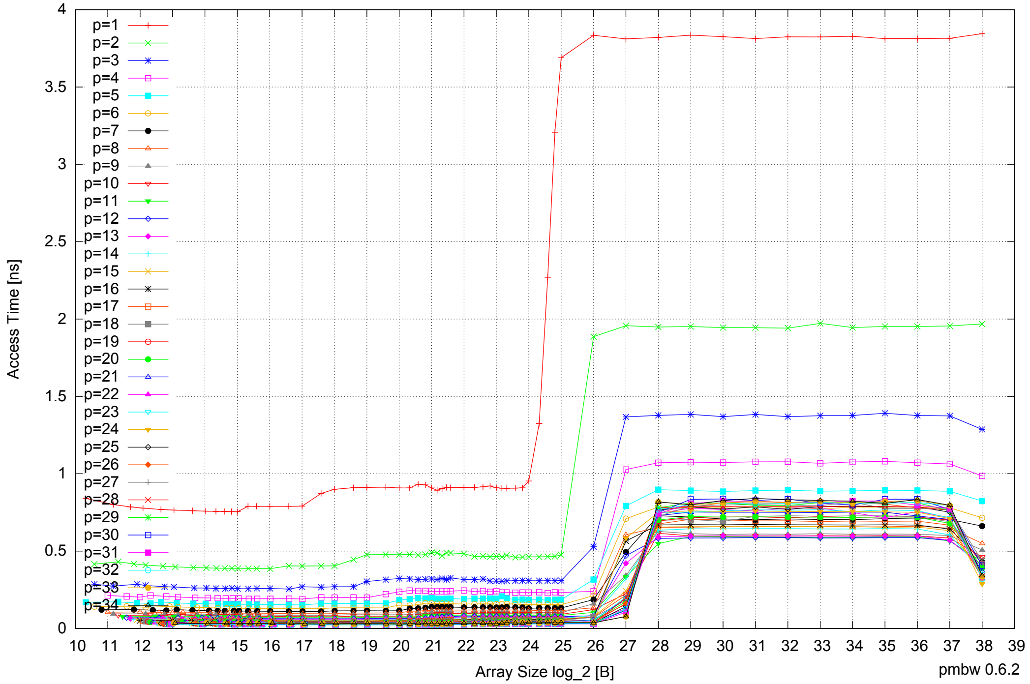
Intel Xeon E7-8837 512GB - Parallel Memory Access Time - ScanRead128PtrSimpleLoop
