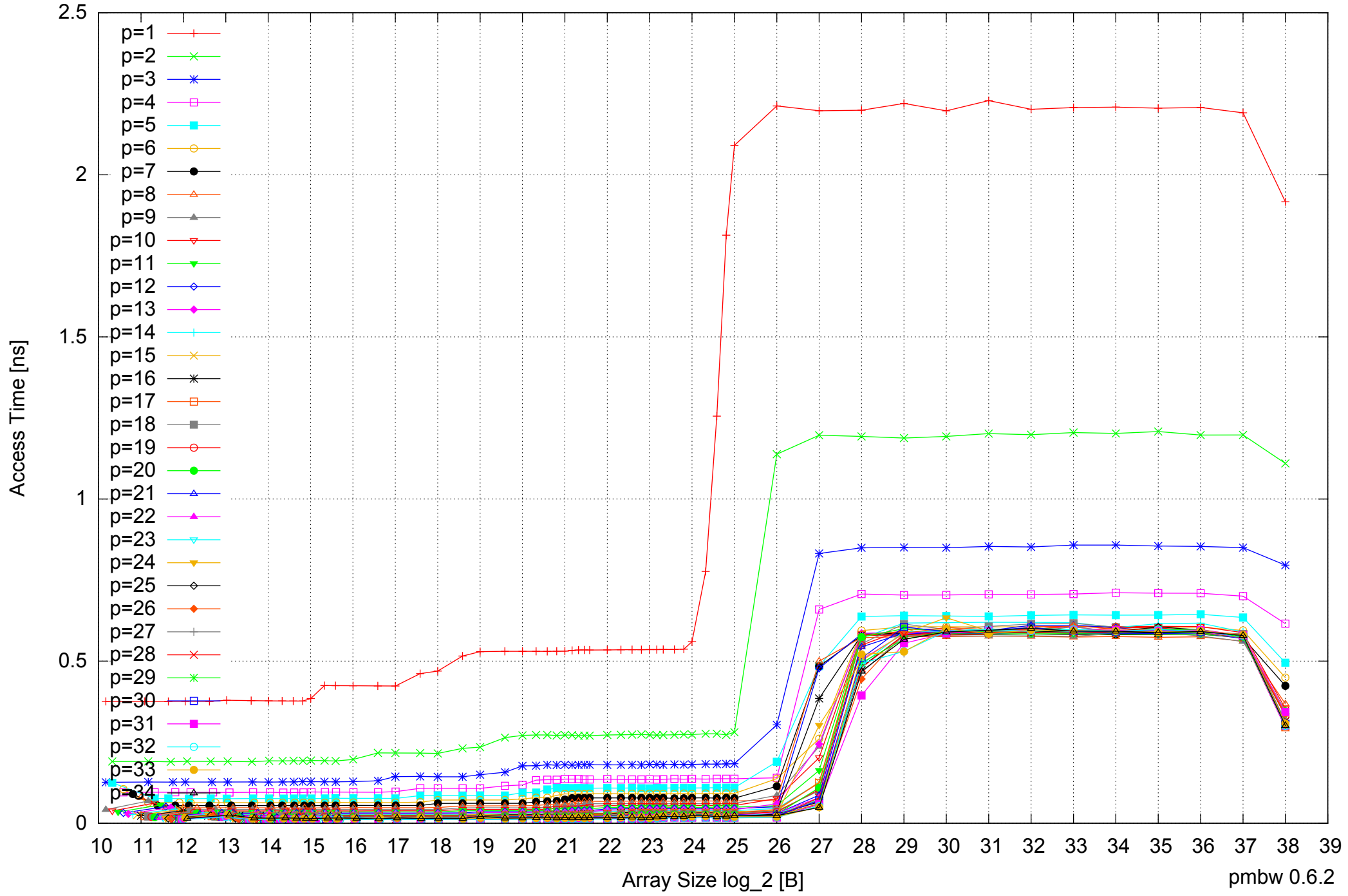
Intel Xeon E7-8837 512GB - Parallel Memory Access Time - ScanWrite64IndexUnrollLoop
