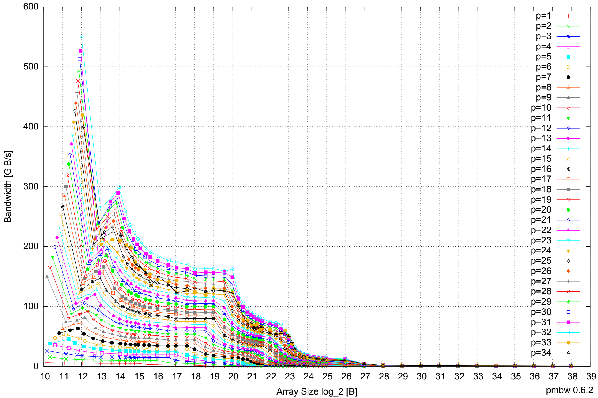
Intel Xeon E7-8837 512GB - Parallel Memory Bandwidth - PermRead64UnrollLoop
