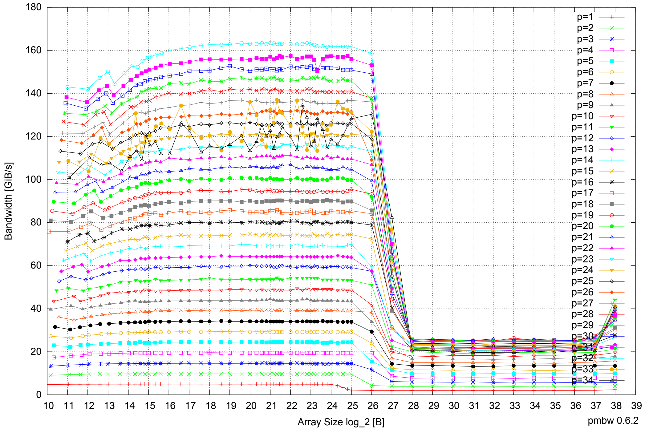
Intel Xeon E7-8837 512GB - Parallel Memory Bandwidth - ScanRead32PtrSimpleLoop
