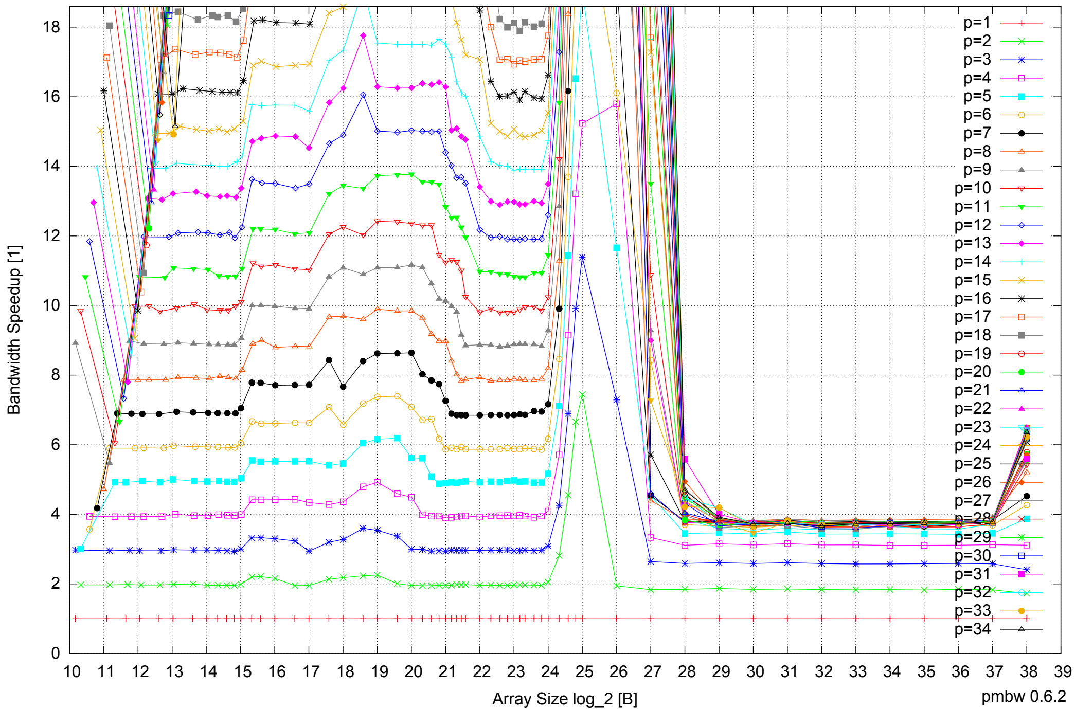
Intel Xeon E7-8837 512GB - Speedup of Parallel Memory Bandwidth (enlarged) - ScanWrite64IndexUnrollLoop
