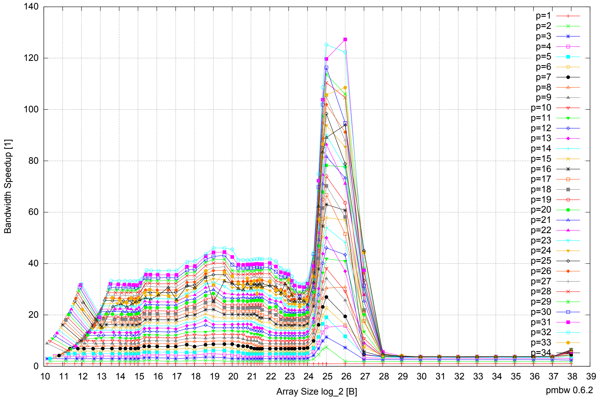
Intel Xeon E7-8837 512GB - Speedup of Parallel Memory Bandwidth - ScanWrite64IndexUnrollLoop
