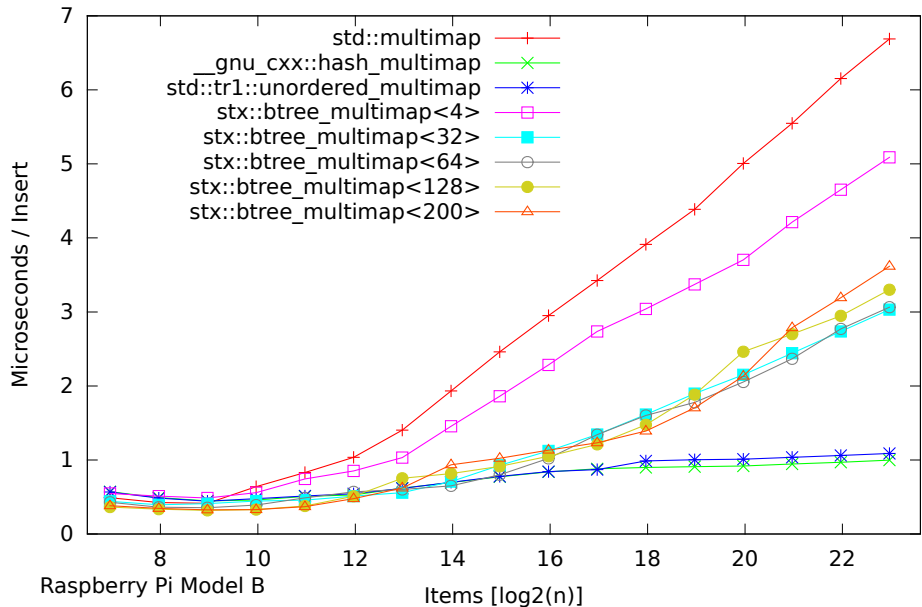
Speed Test Multimap - Normalized Time - Find Only (125-8192000 Items)
