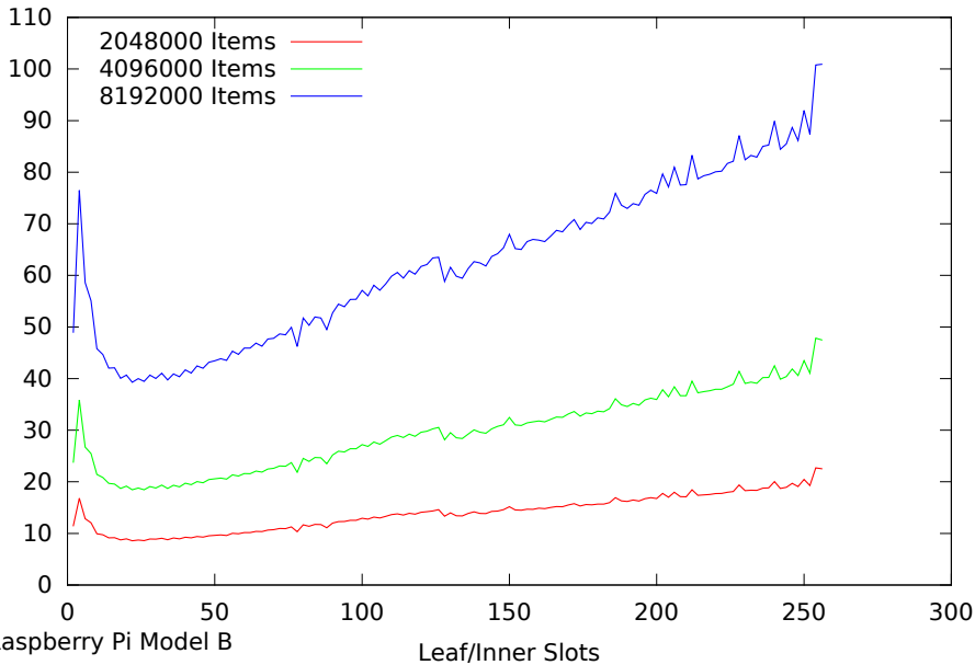
Speed Test - Finding the Best Slot Size - Insertion Only - Plotted by Slots in B+ Tree
