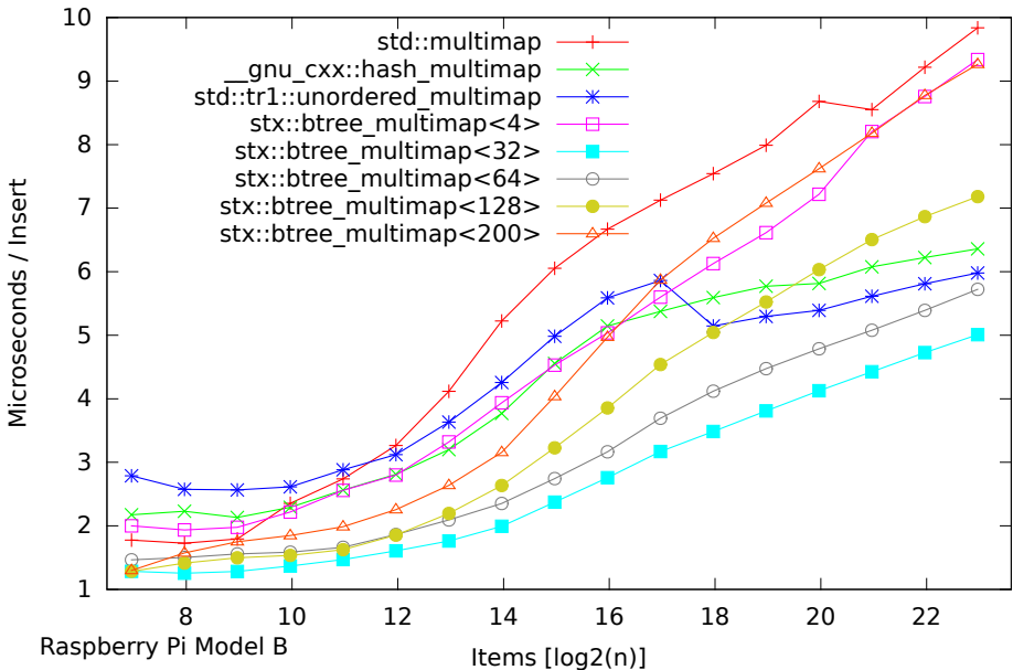
Speed Test Multimap - Normalized Time - Insertion Only (125-8192000 Items)
