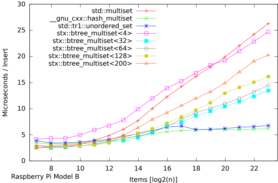
Speed Test Multiset - Normalized Time - Insert/Find/Erased (125-8192000 Items)
