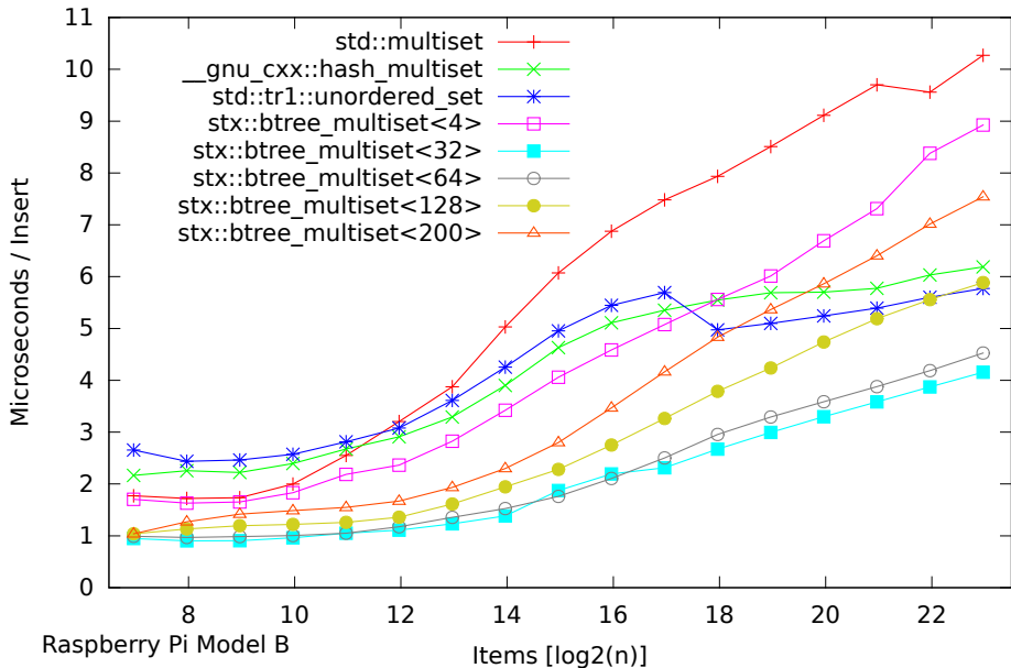
Speed Test Multiset - Normalized Time - Insertion Only (125-8192000 Items)
