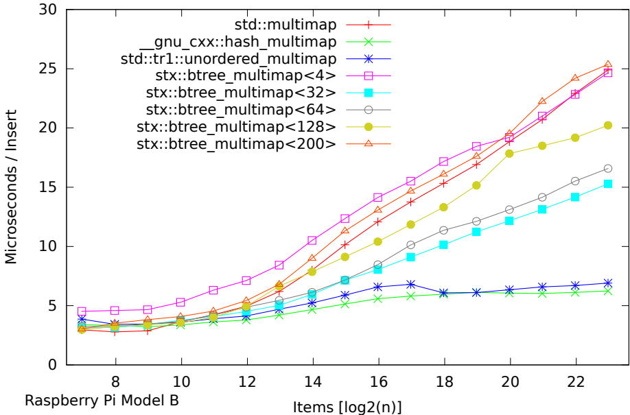
Speed Test Multimap - Normalized Time - Insert/Find/Erased (125-8192000 Items)
