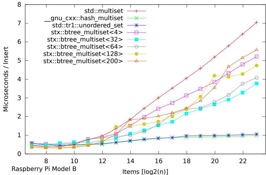
Speed Test Multiset - Normalized Time - Find Only (125-8192000 Items)
