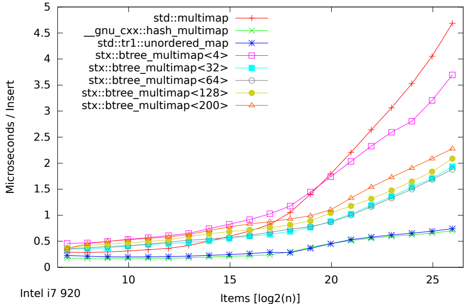
Speed Test Multimap - Normalized Time - Insert/Find/Erace (125-65536000 Items)
