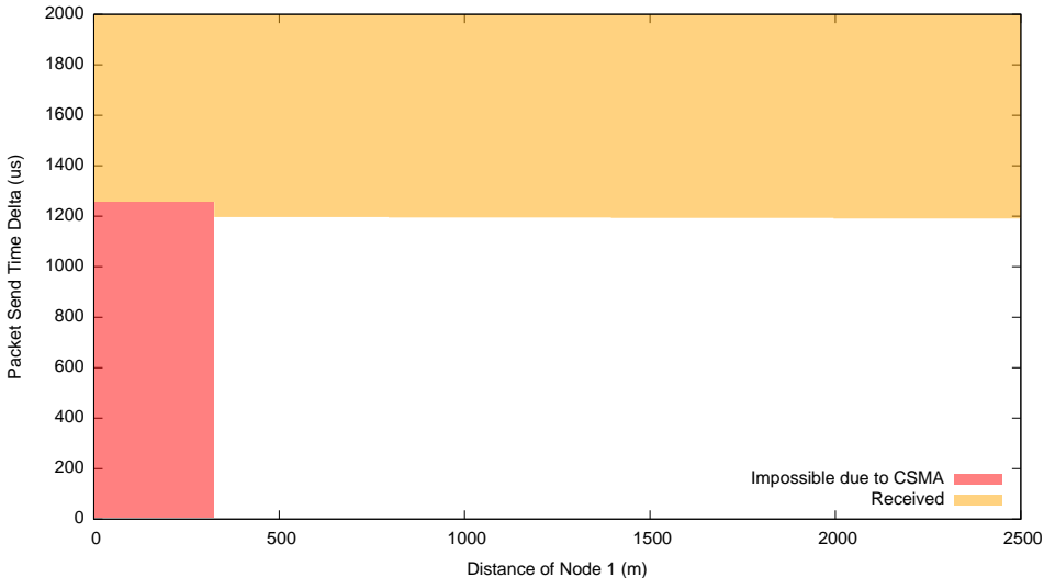
Three Wireless Nodes - Reception on Node 0 of Packet from Node 2 (Non-moving Interferer)
