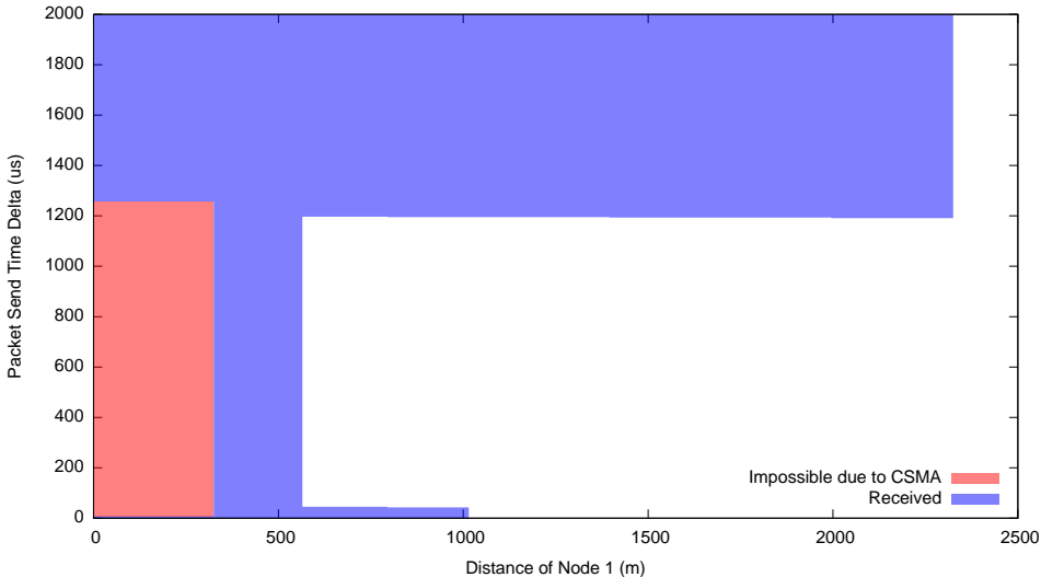
Three Wireless Nodes - Reception on Node 0 of Packets from Node 1 (Moving Near Sender)
