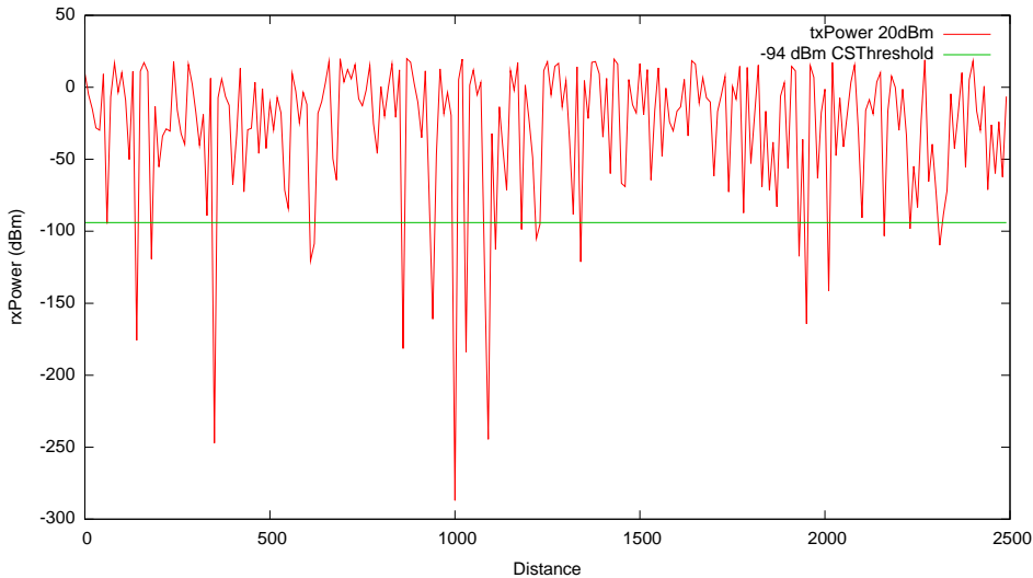
ns3::RandomPropagationLossModel with Exponential Distribution
