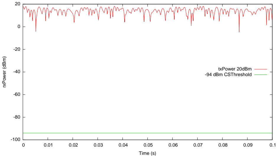
ns3::JakesPropagationLossModel (with 477.9 Hz shift and 0.1 millisecond resolution)
