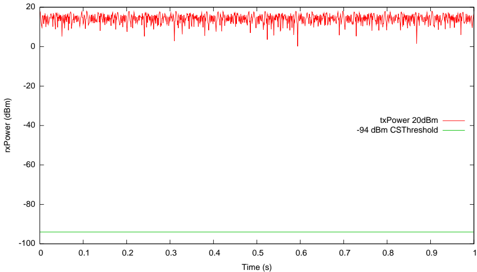
ns3::JakesPropagationLossModel (with 477.9 Hz shift and 1 millsec resolution)
