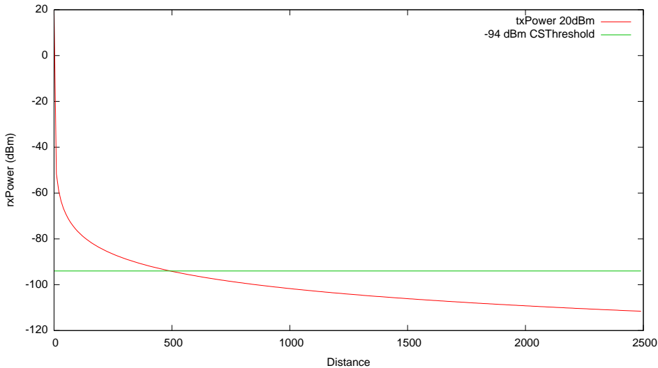
ns3::LogDistancePropagationLossModel (Exponent = 2.5)
