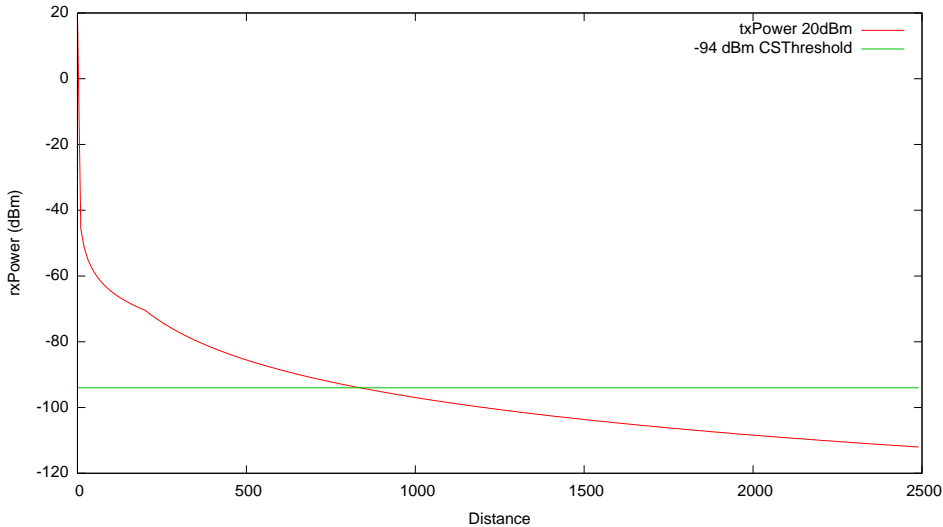
ns3::ThreeLogDistancePropagationLossModel (Defaults)
