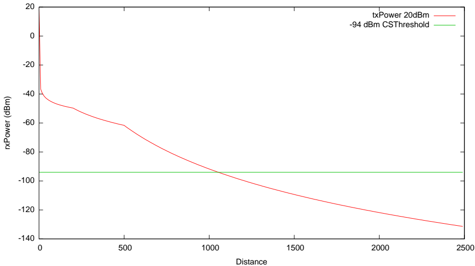
ns3::ThreeLogDistancePropagationLossModel (Exponents 1.0, 3.0 and 10.0)
